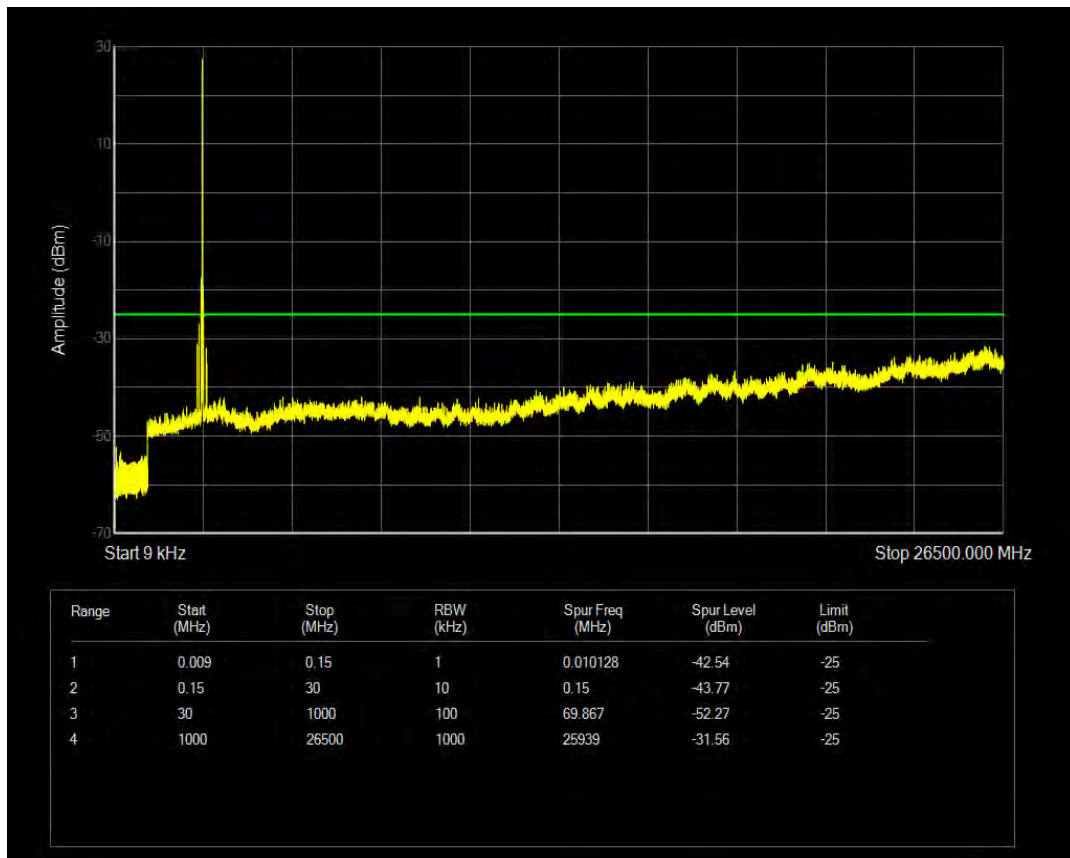
Band41 16QAM BW=20MHz Channel=41090 RB Size=100 Position=#0
