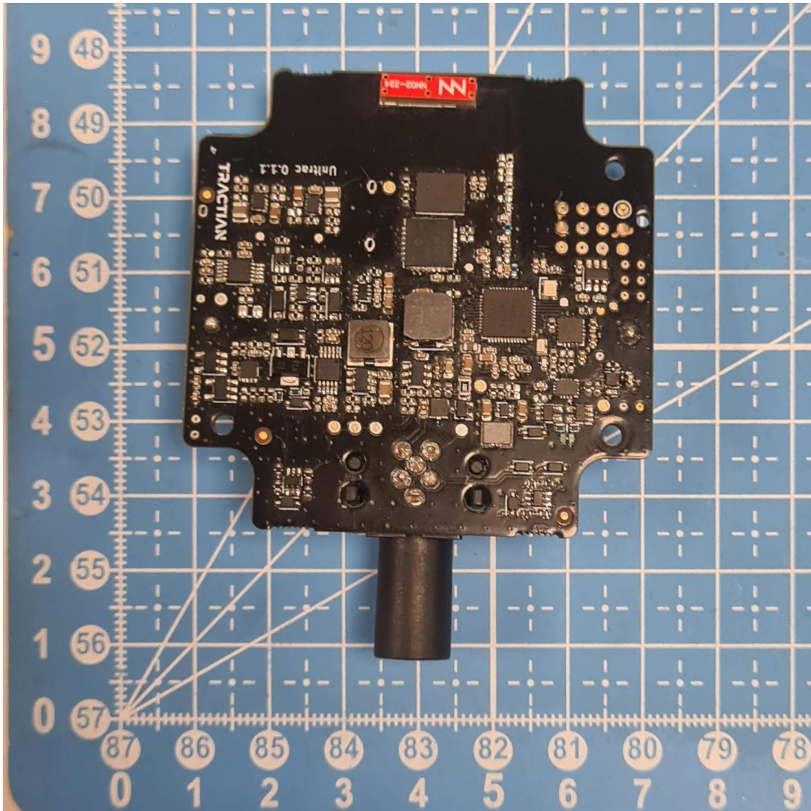
Figure 2 - Uni Trac - PCB - Top
