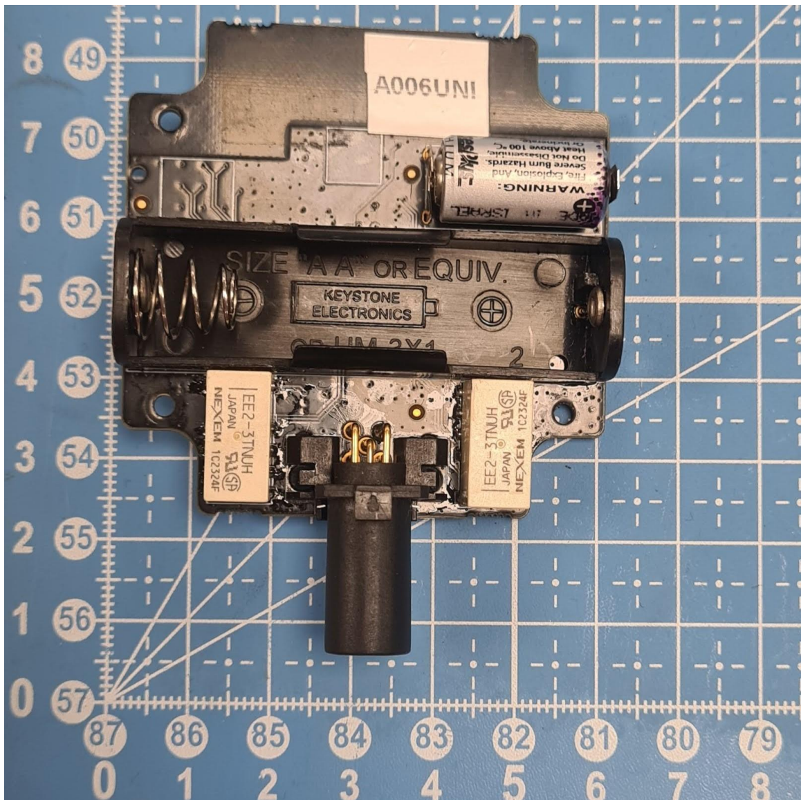
Figure 1 - Uni Trac - PCB Bottom
