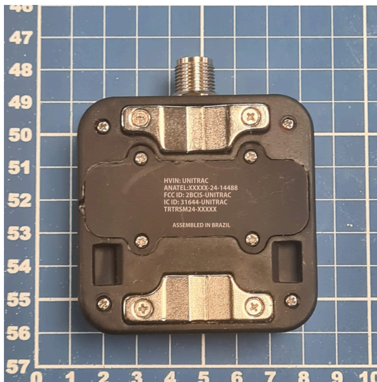
Figure 2 - Bottom View
