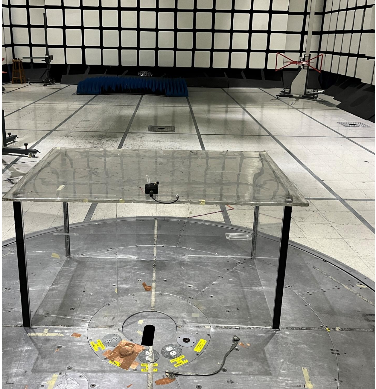
Radiated Emissions 30MHz – 1GHz
