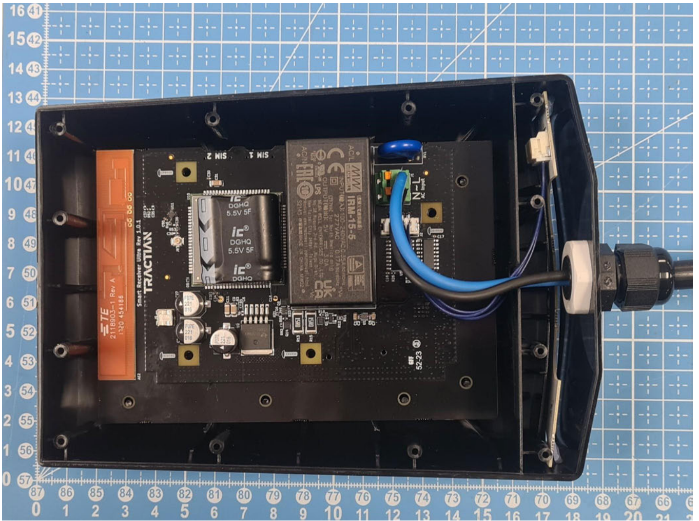
Figure 5 - PCB mounted inside the enclosure
