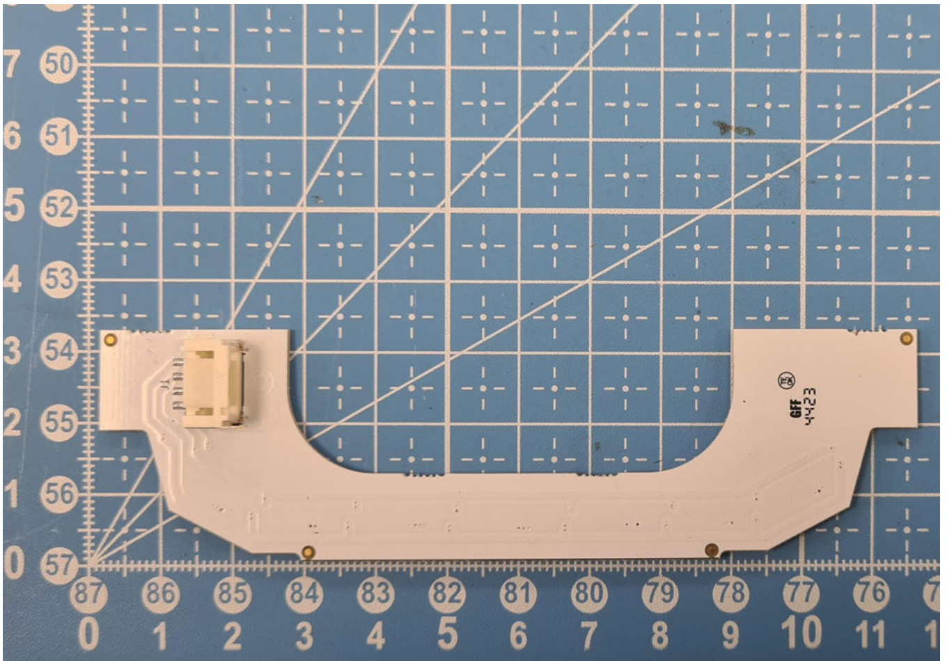
Figure 4 - Led Bar - PCB - Bottom
