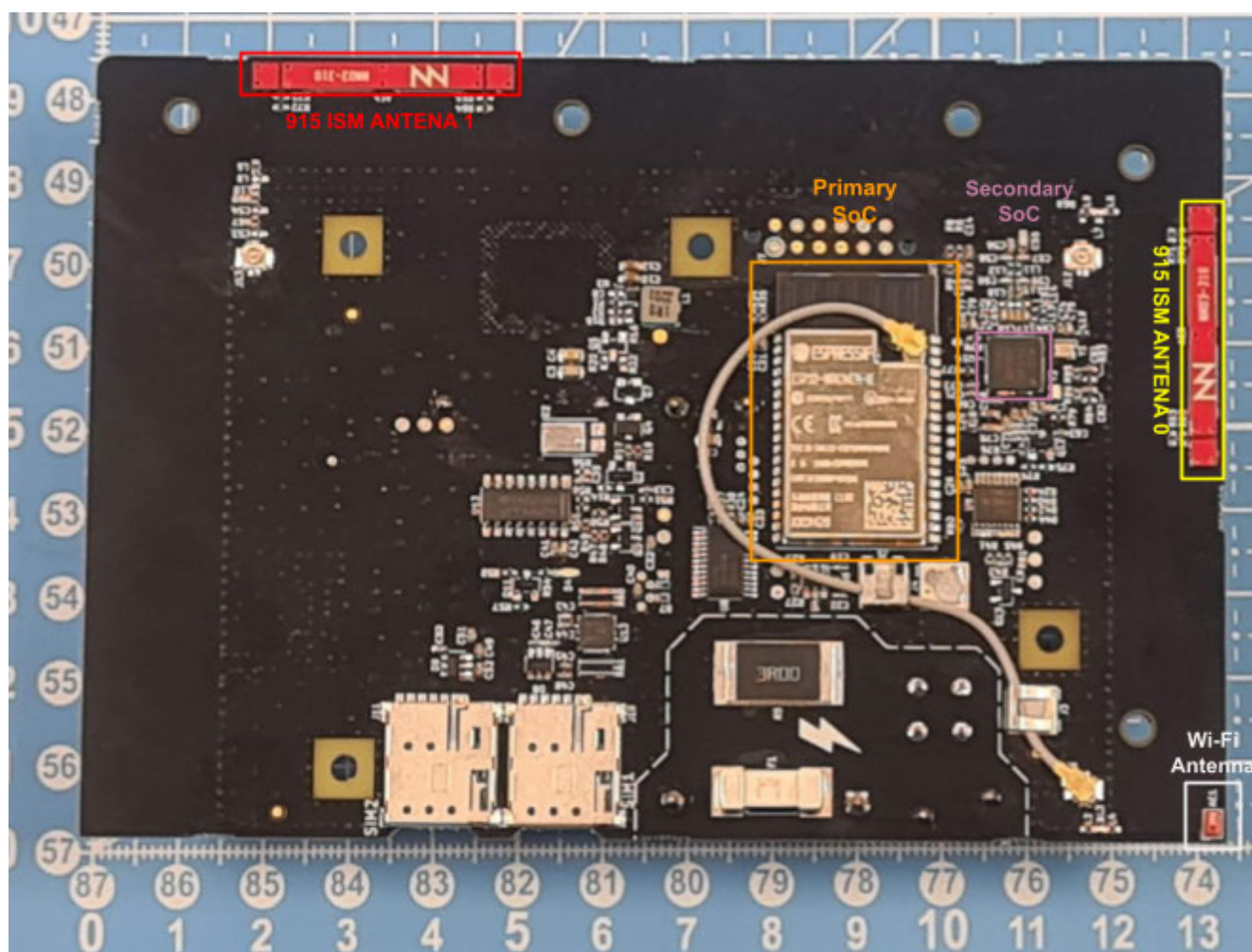
Figure 2 - Smart Receiver Ultra - PCB - Bottom
