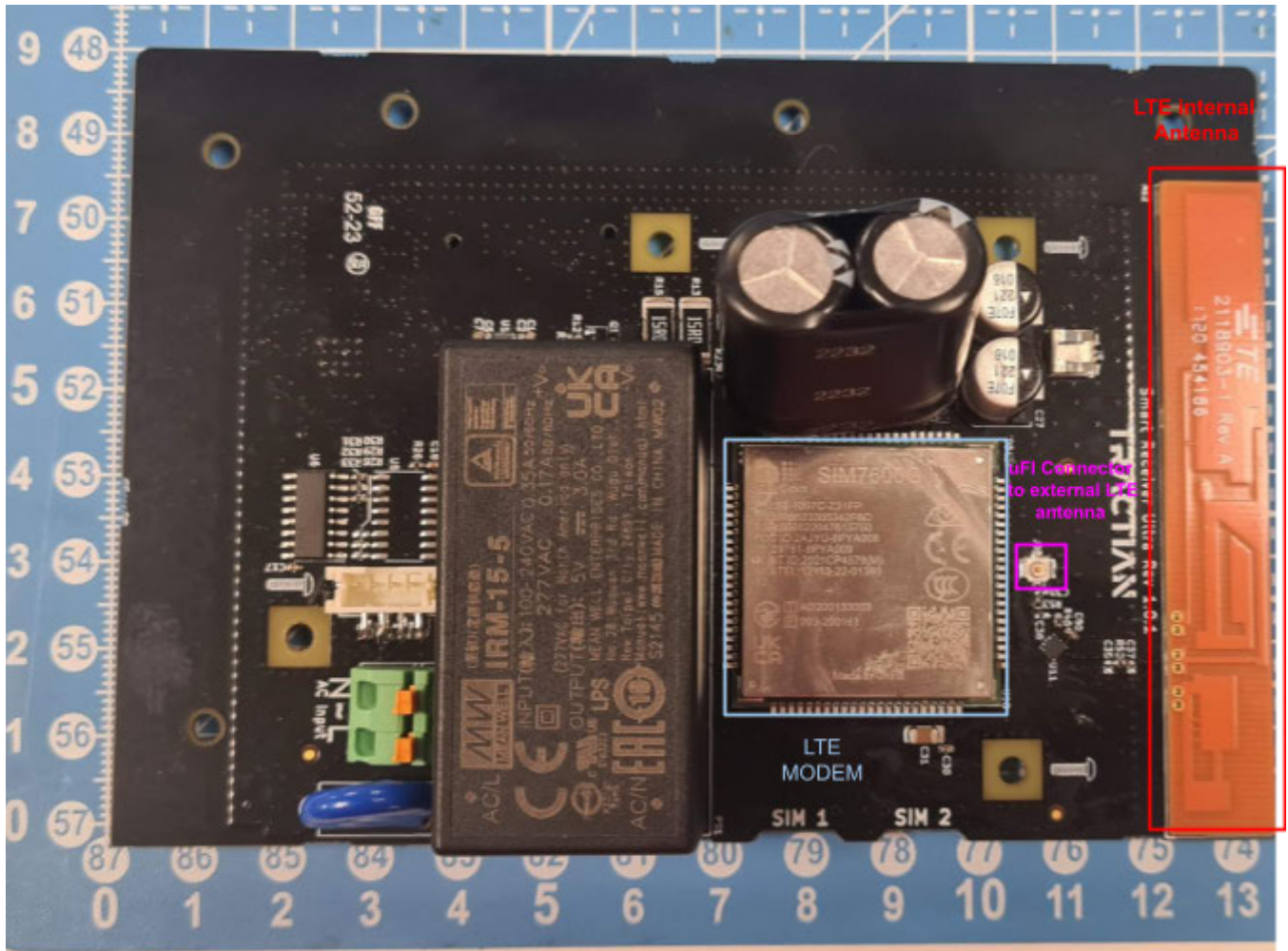
Figure 1 - Smart Receiver Ultra - PCB - Top
