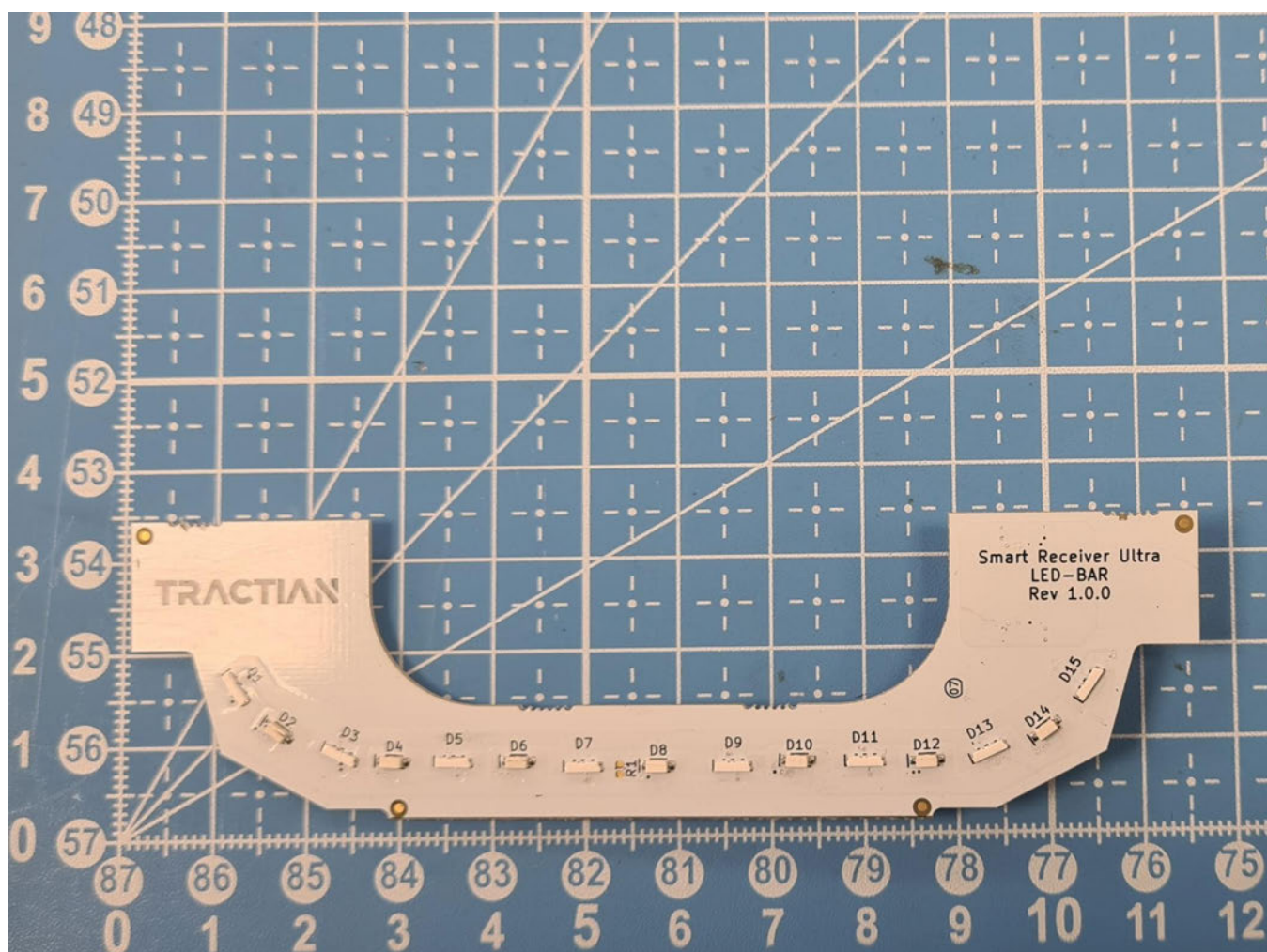
Figure 3 - Led Bar - PCB - Top
