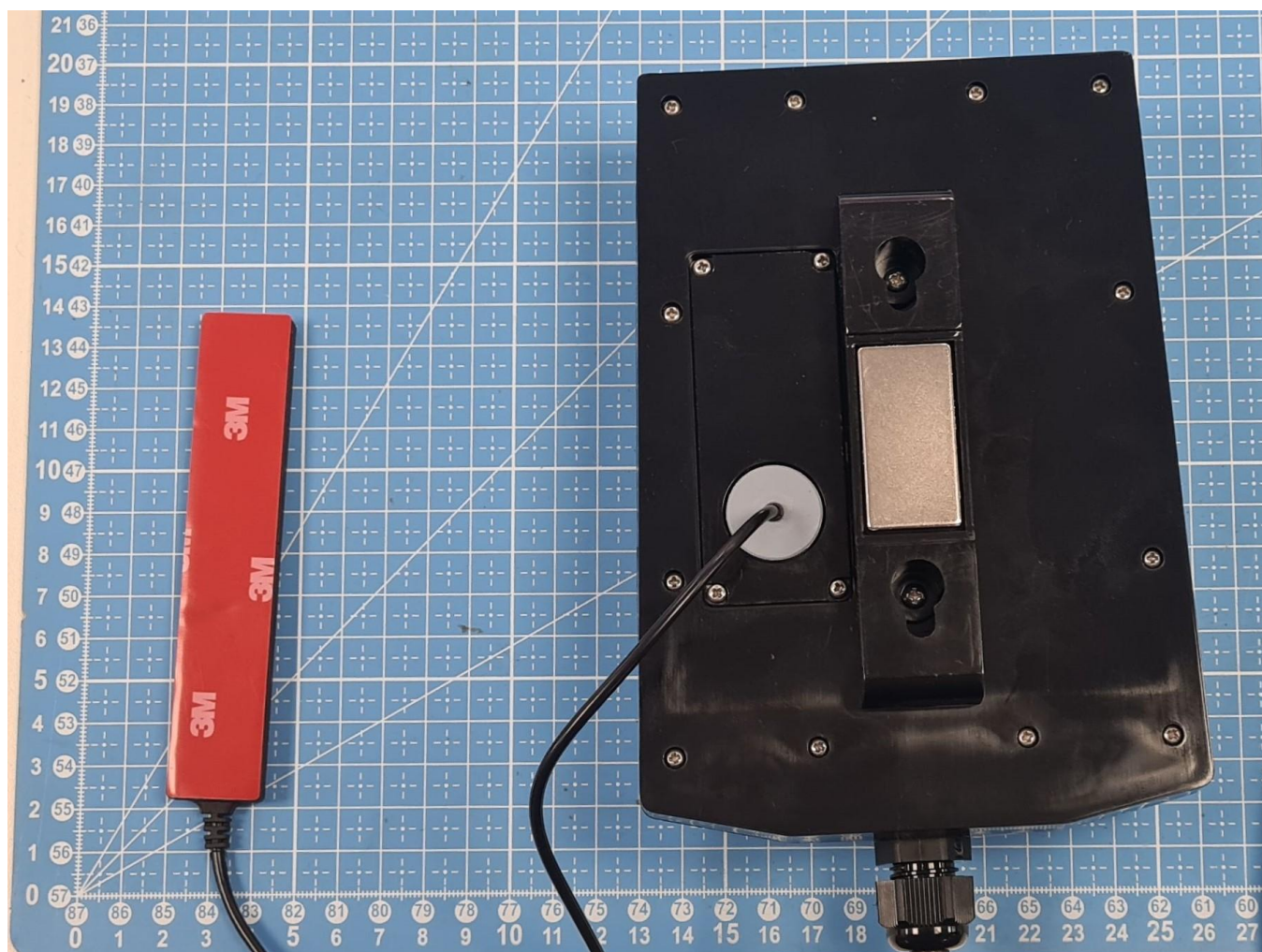
Figure 8 - Smart Receiver Ultra - External Antenna - Rear Fixation tape
