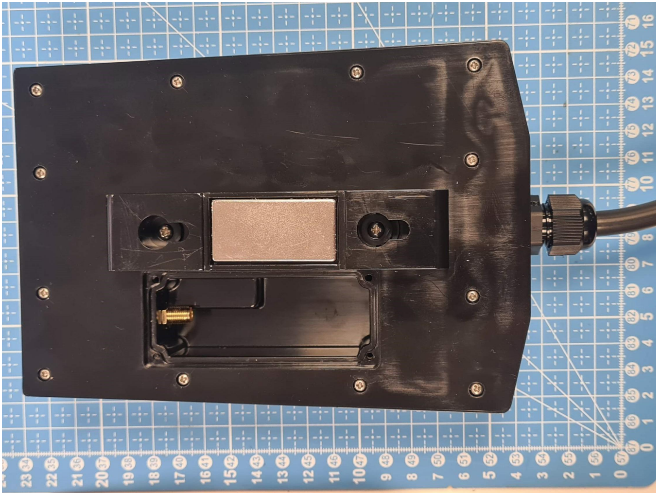
Figure 9 - Smart Receiver Ultra - SMA connector to LTE Antenna
