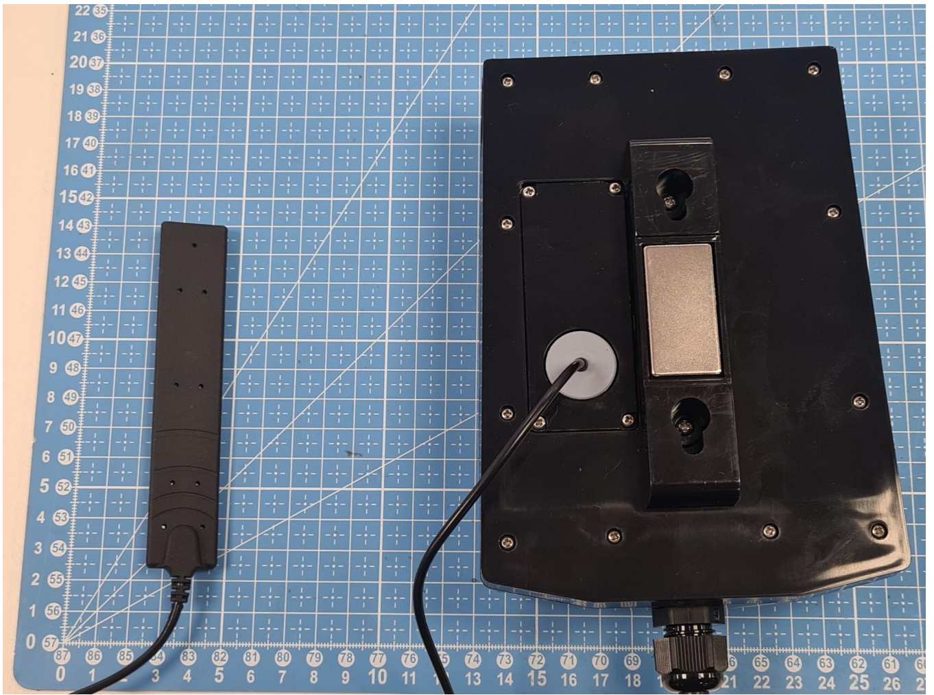
Figure 7 - Smart Receiver Ultra - External Antenna - Front
