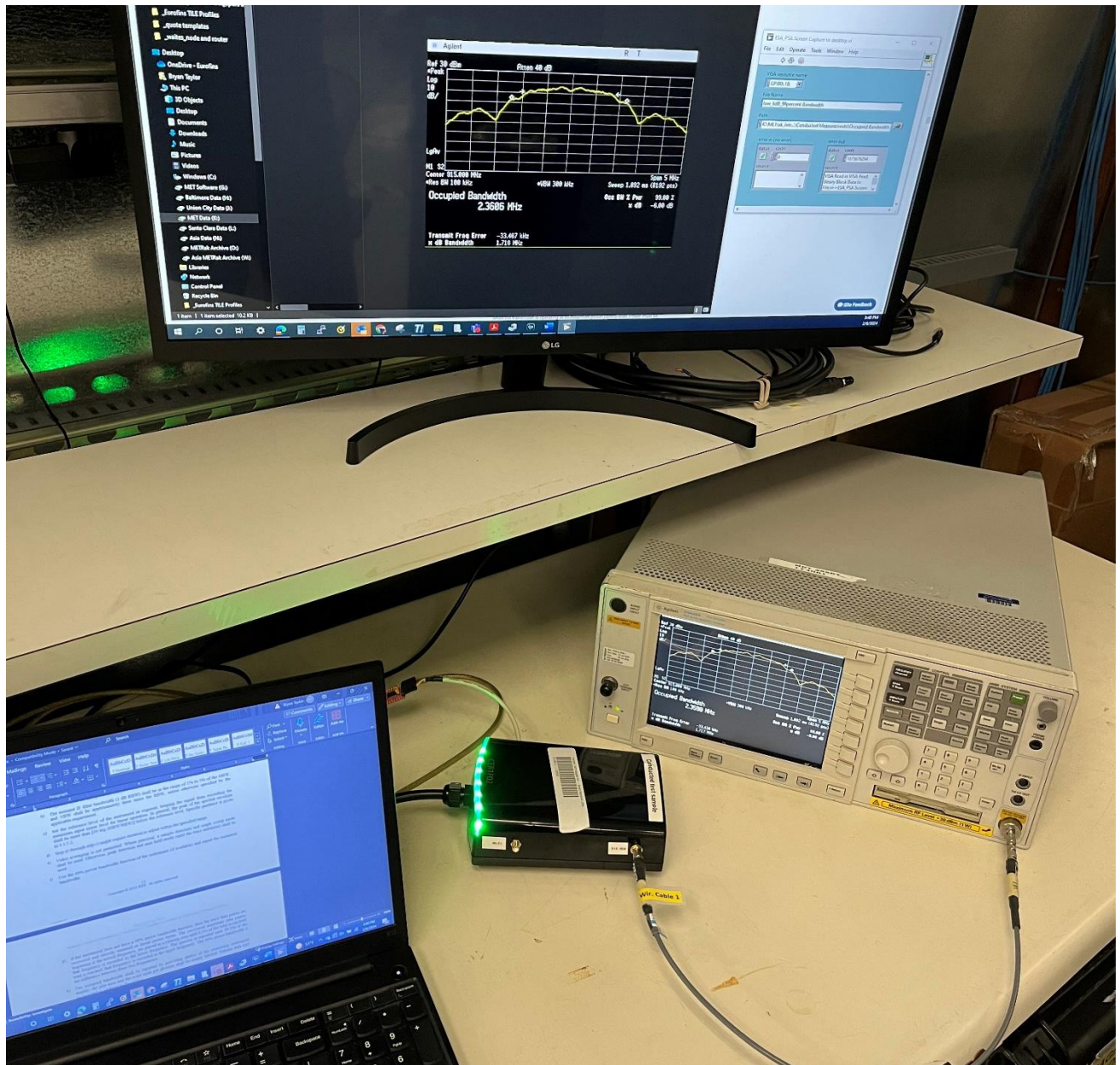
Antenna Port Conducted Measurements
