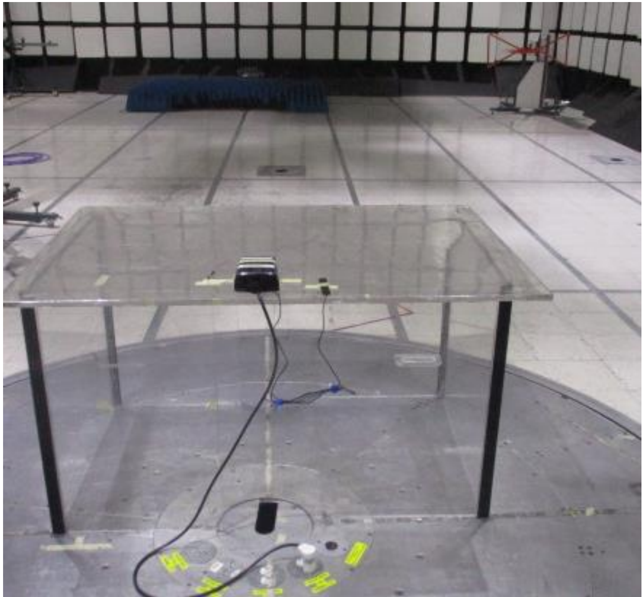
Radiated Emissions Below 1GHz (Back Side)
