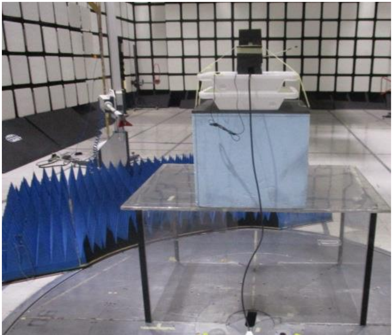
Radiated Emissions Above 1GHz (Back Side)
