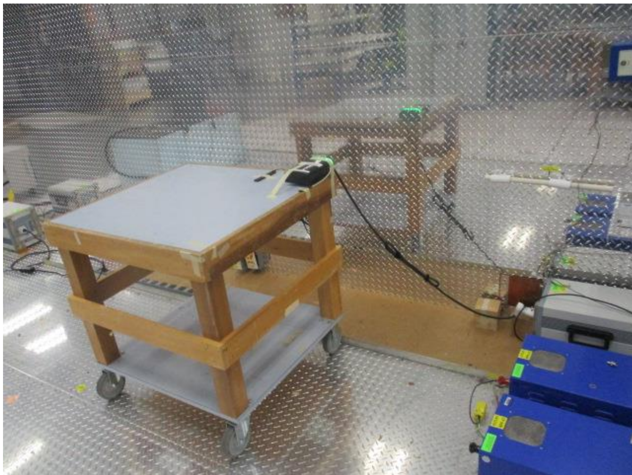
Conducted Emissions on AC Mains
