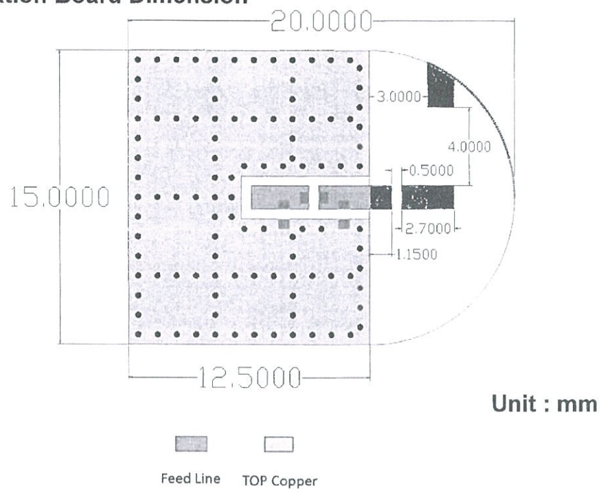
Evaluation Board Dimension
