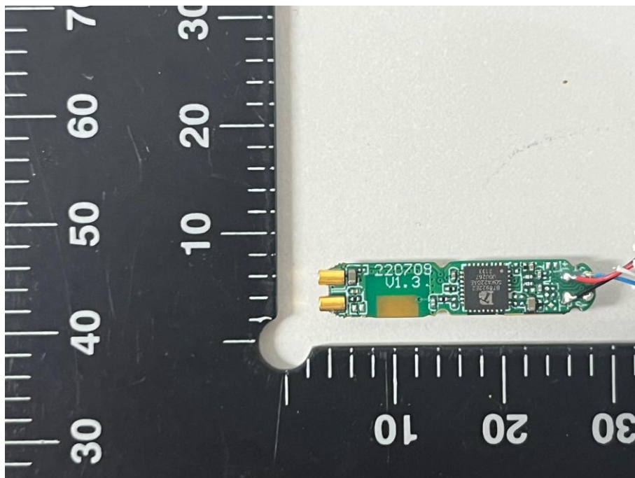
Earphone board - Bottom_Left
