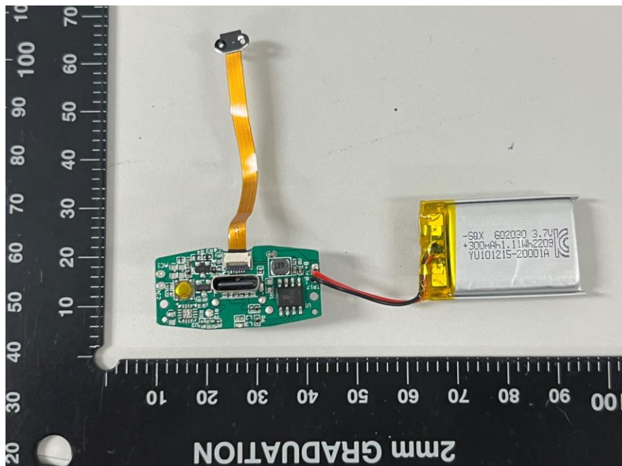
Charging case board - Top
