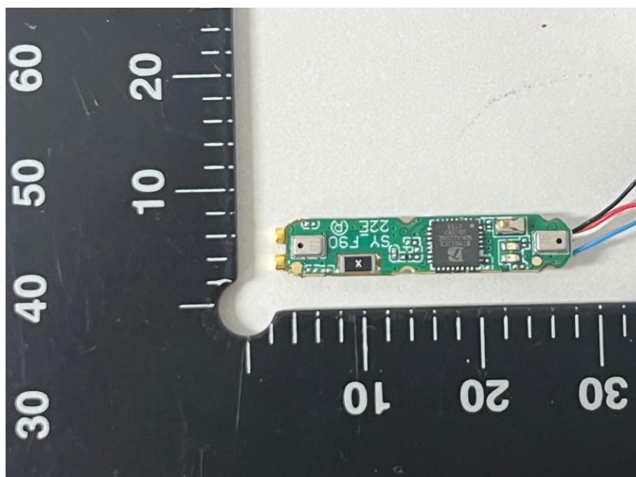
Earphone board - Top_Right
