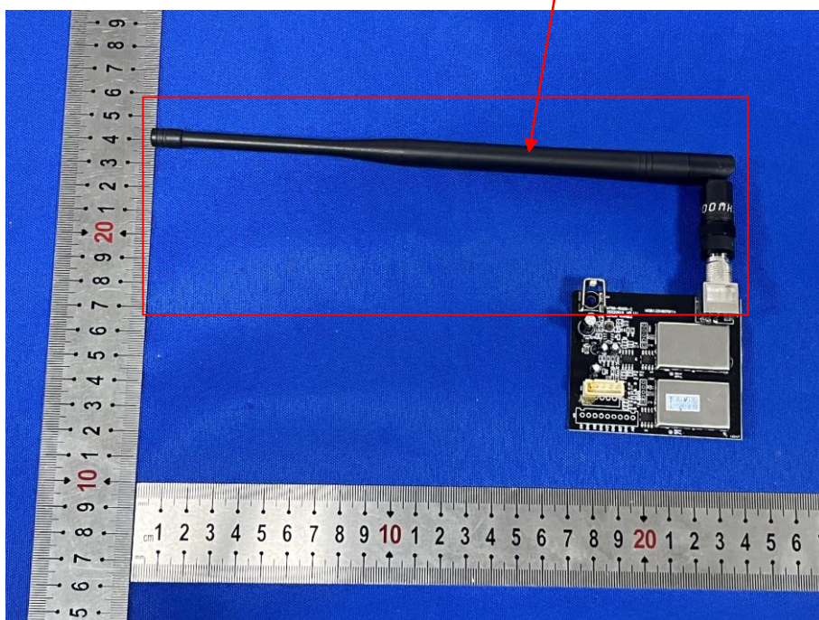
Receiving Antenna
