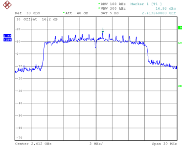
Reference Level-CH01
