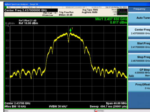
Channel 06 (2437MHz)
