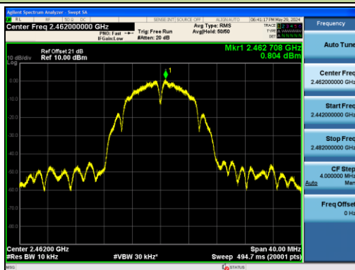
Channel 11 (2462MHz)
