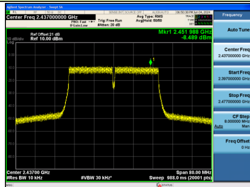
Channel 06 (2437MHz)
