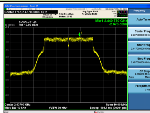
Channel 06 (2437MHz)
