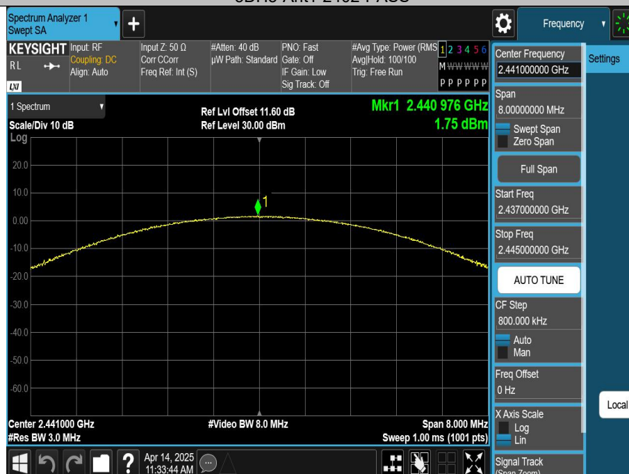
3DH5-Ant1-2441-PASS
