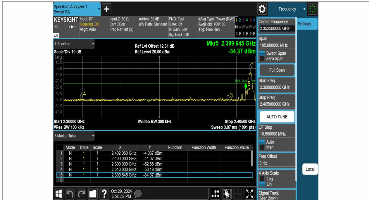
BLE_2M-Ant1-2402-PASS
