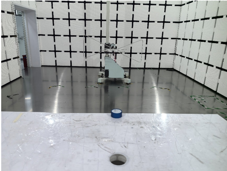
Radiated Emission
