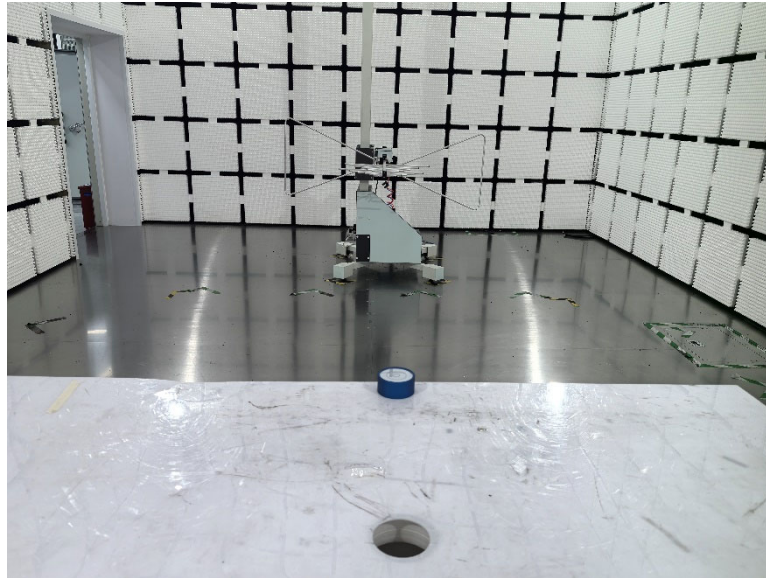
Radiated Emissions
