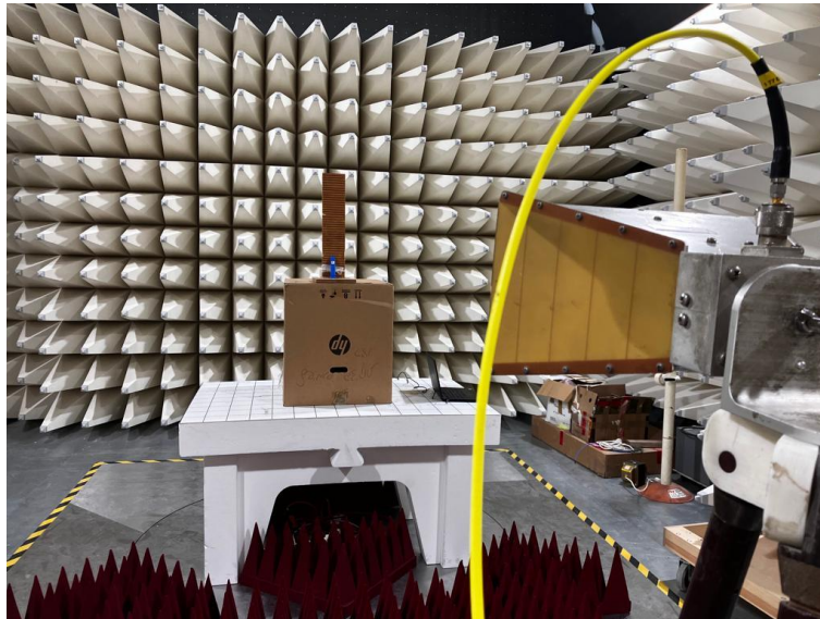
Figure 3. Radiated Emission Test, 1-18GHz
