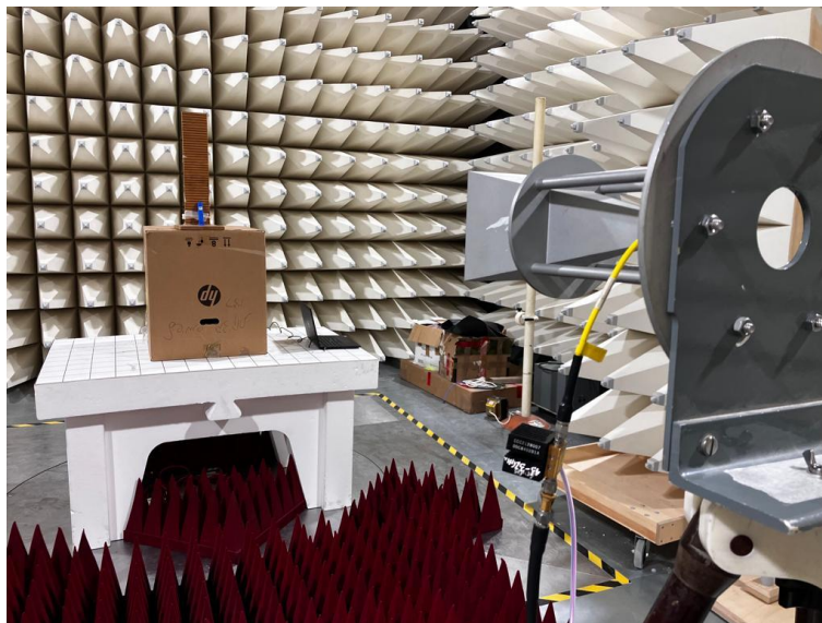
Figure 4. Radiated Emission Test, 18-25GHz
