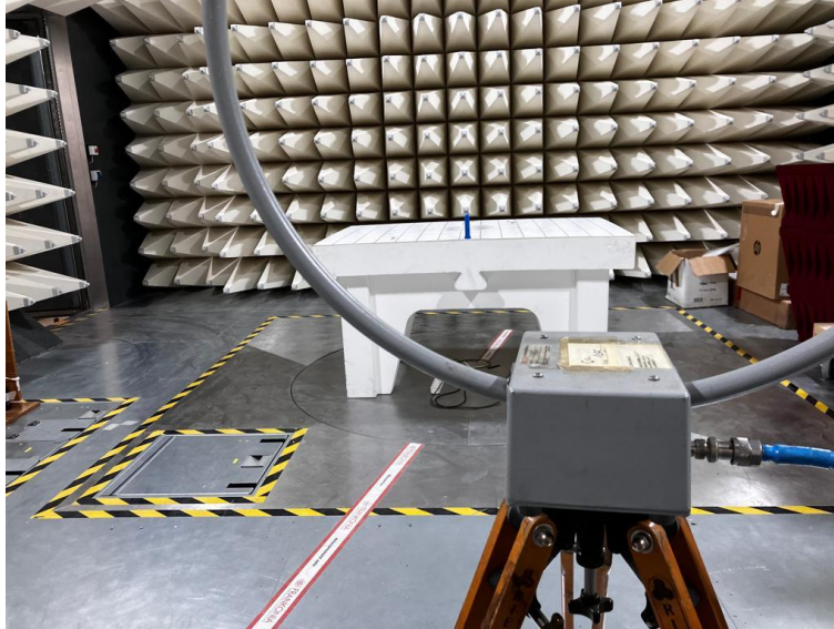
Figure 1. Radiated Emission Test, 0.009-30MHz
