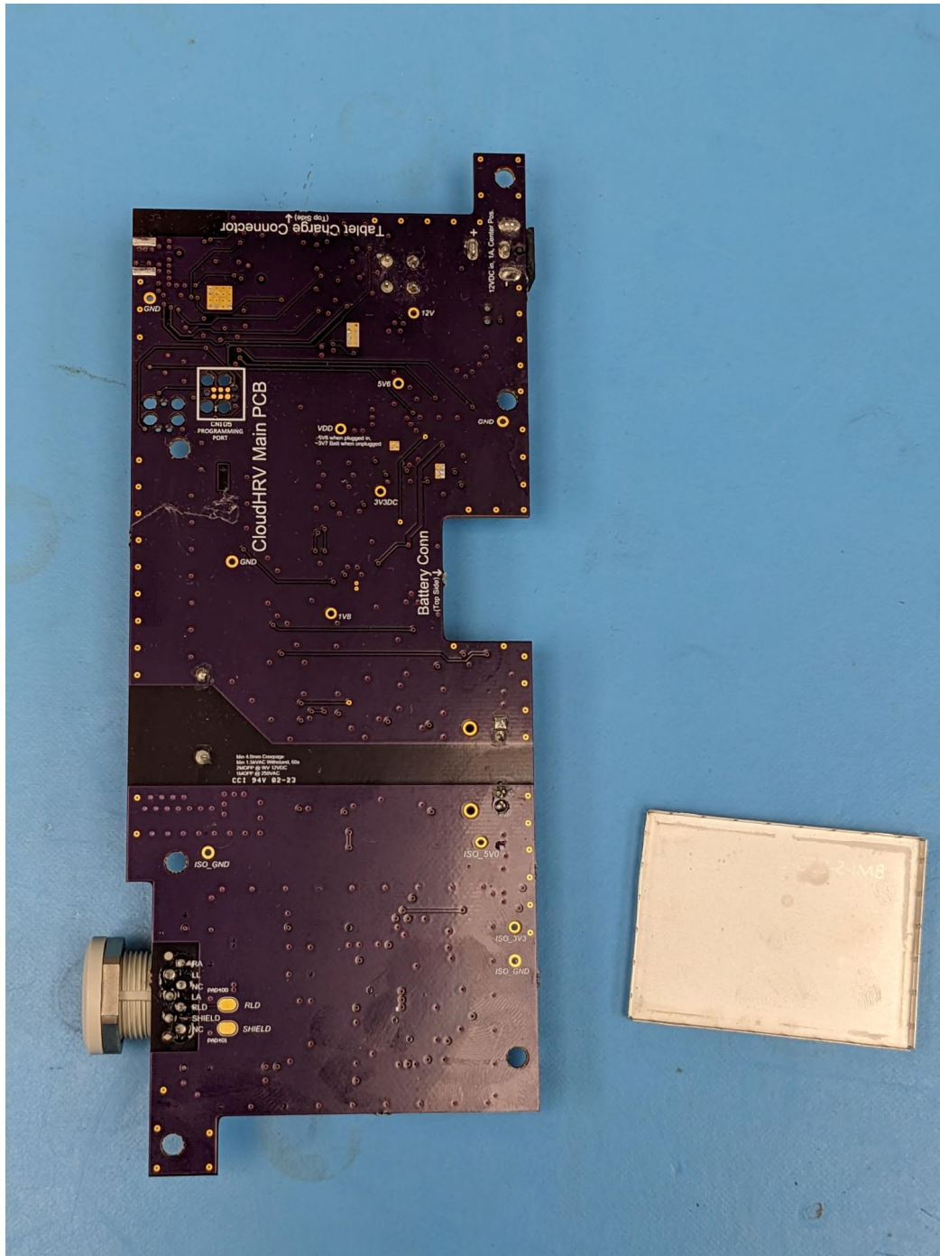
Figure 2 – EUT Internal Photo Back
