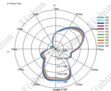
(2) Z-Y Plane(unit:dBi):
