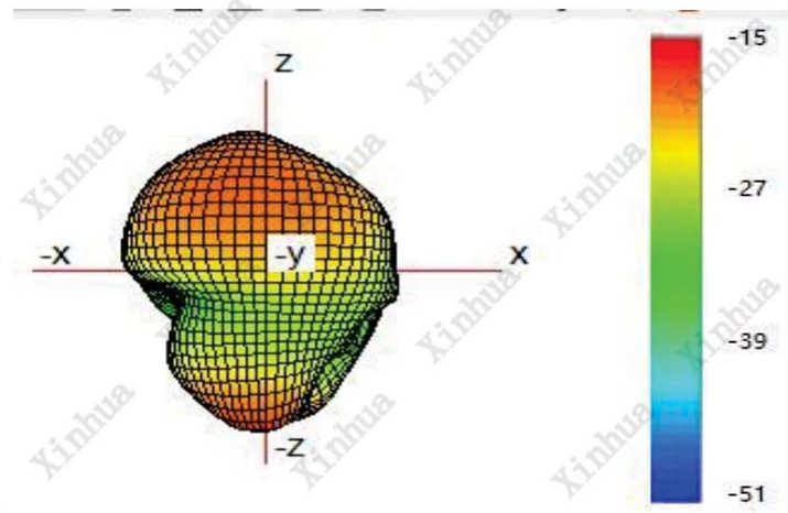
(6) Typical Free Space 3D Radiation Pattern at 438MHz(unit:dBi)
