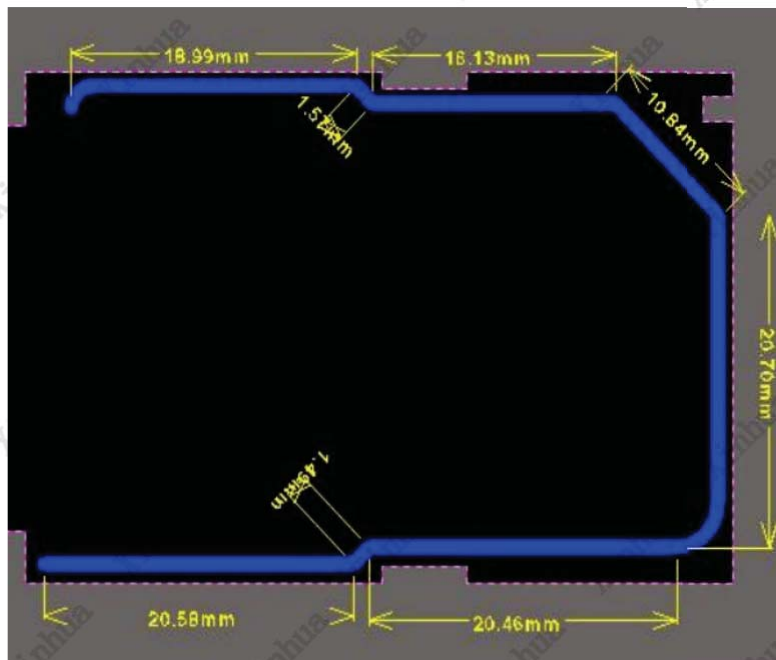
Antenna Dimensions
