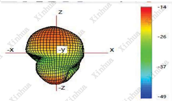
(4) Typicall Free Space 3D Radiation Pattern at 428MHz(unit:dBi)
