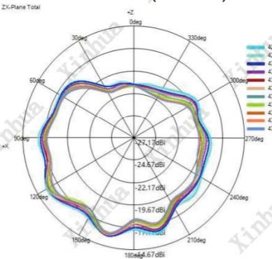
(3) Z-X Plane(unit:dBi):
