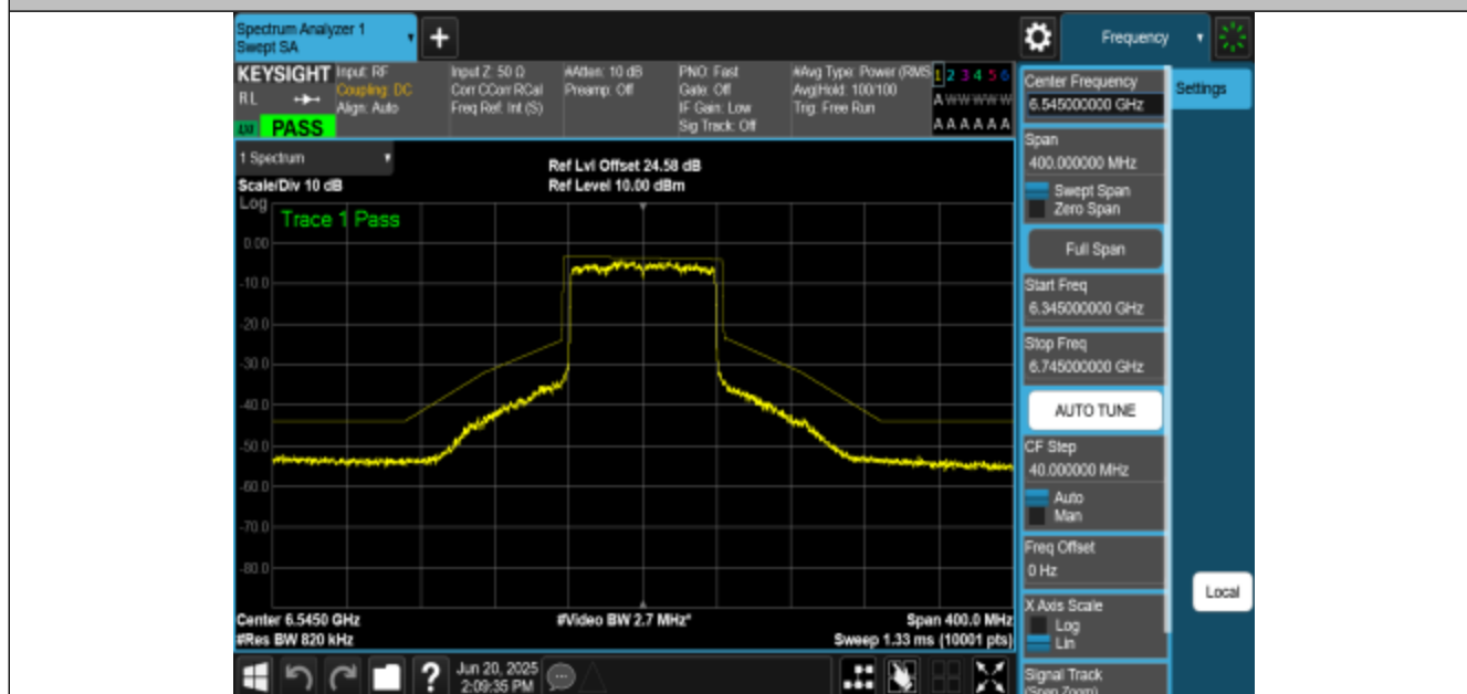
NTNV-11BE80MIMO-Ant2-6545-PASS
