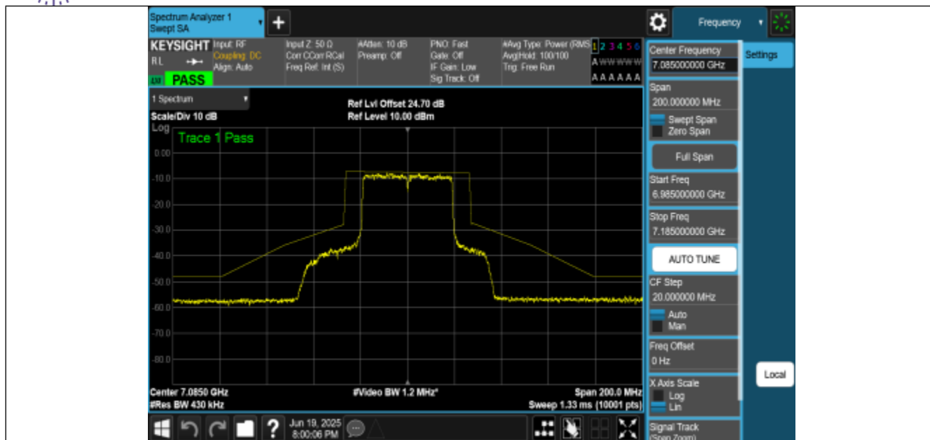
NTNV-11BE40MIMO-Ant1-7085-PASS
