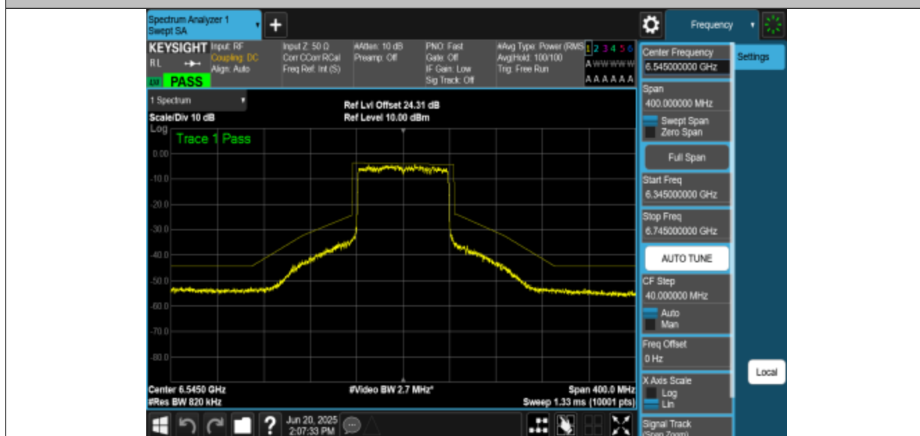
NTNV-11BE80MIMO-Ant0-6545-PASS
