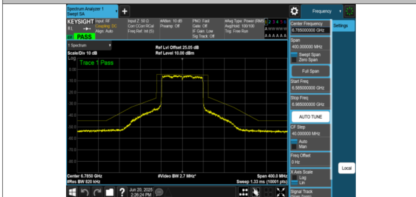
NTNV-11BE80MIMO-Ant2-6785-PASS
