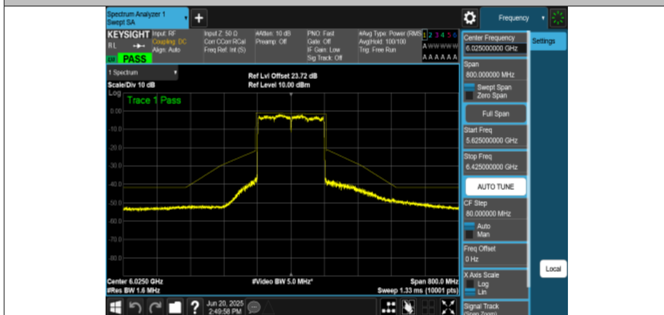
NTNV-11BE160MIMO-Ant2-6025-PASS
