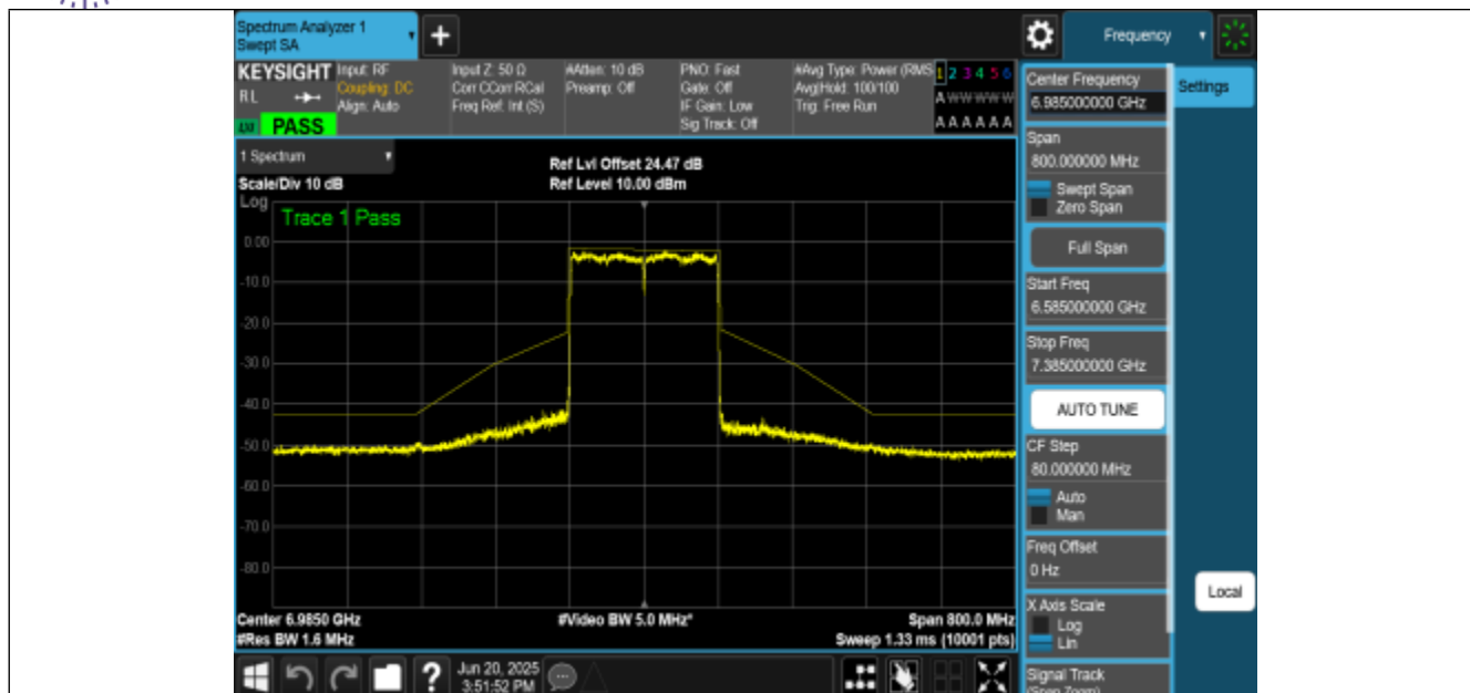
NTNV-11BE160MIMO-Ant1-6985-PASS
