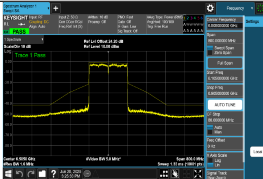
NTNV-11BE160MIMO-Ant2-6505-PASS
