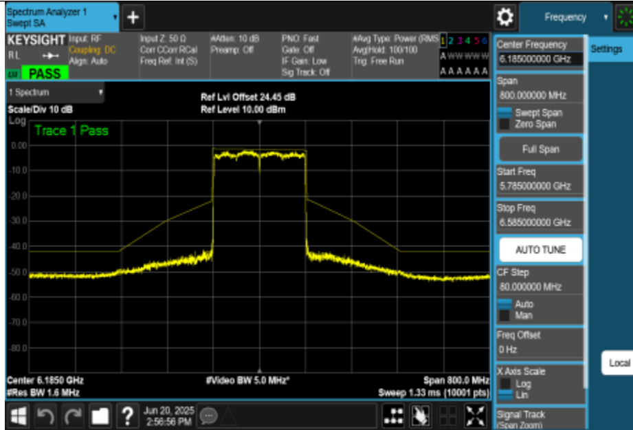
NTVN-11BE160MIMO-Ant3-6185-PASS
