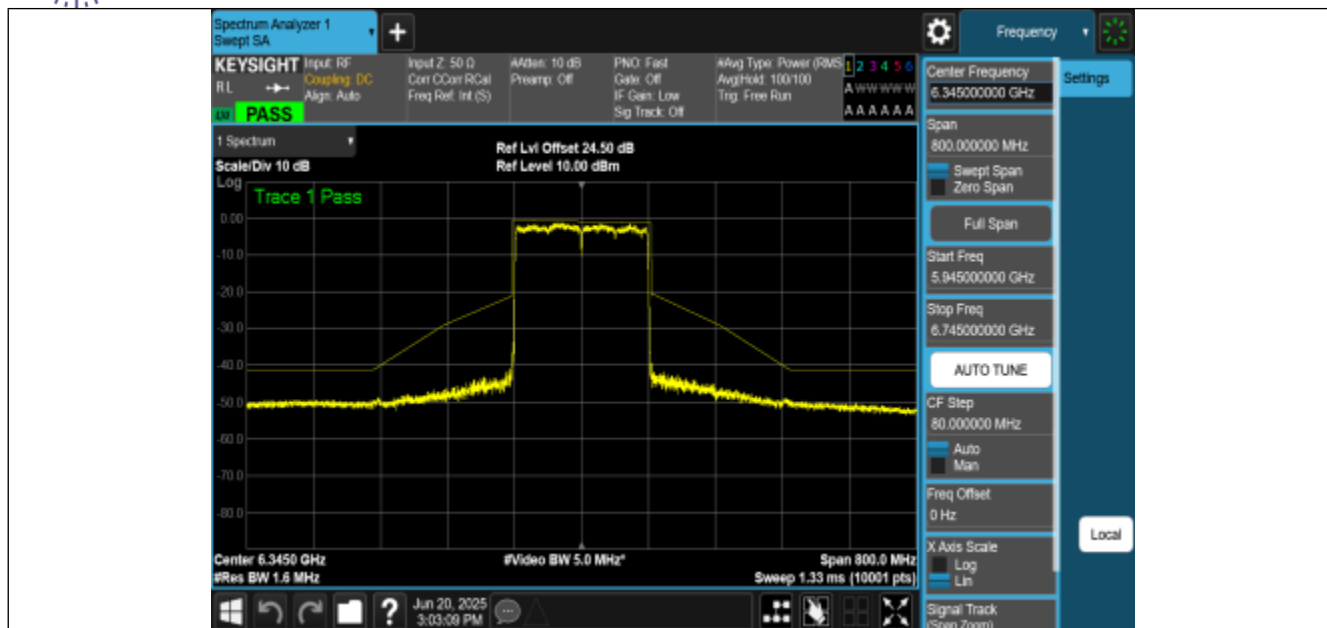
NTNV-11BE160MIMO-Ant1-6345-PASS
