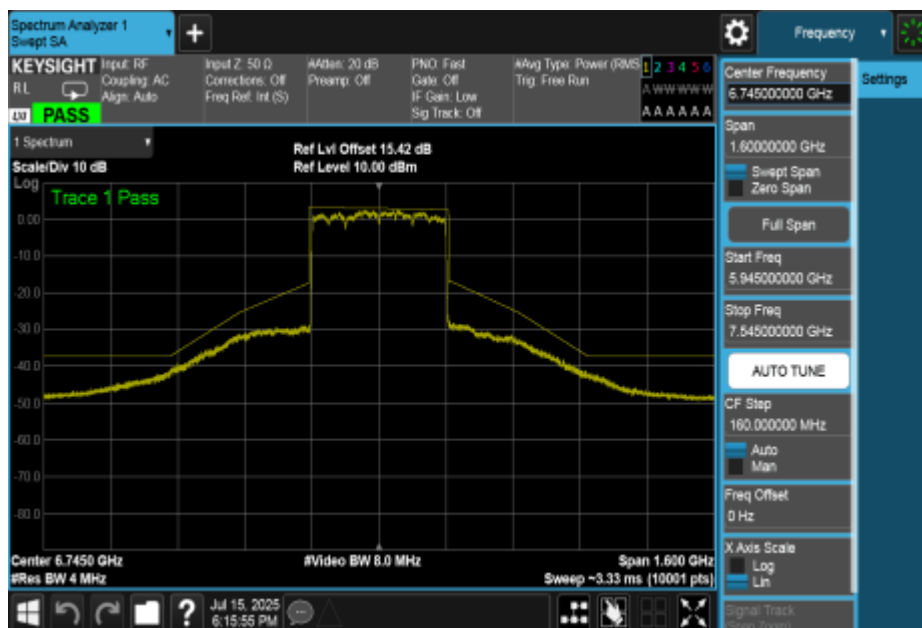
NTNV-11BE320MIMO-Ant0-6745-PASS
