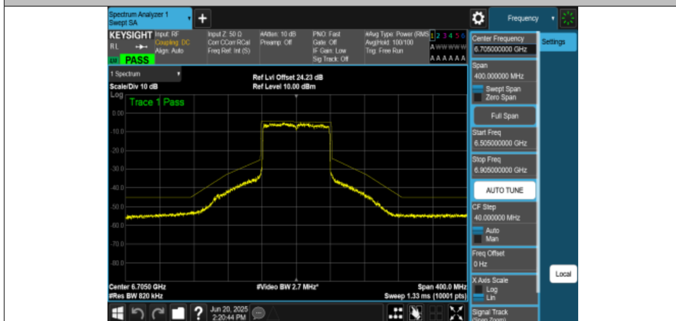
NTNV-11BE80MIMO-Ant2-6705-PASS
