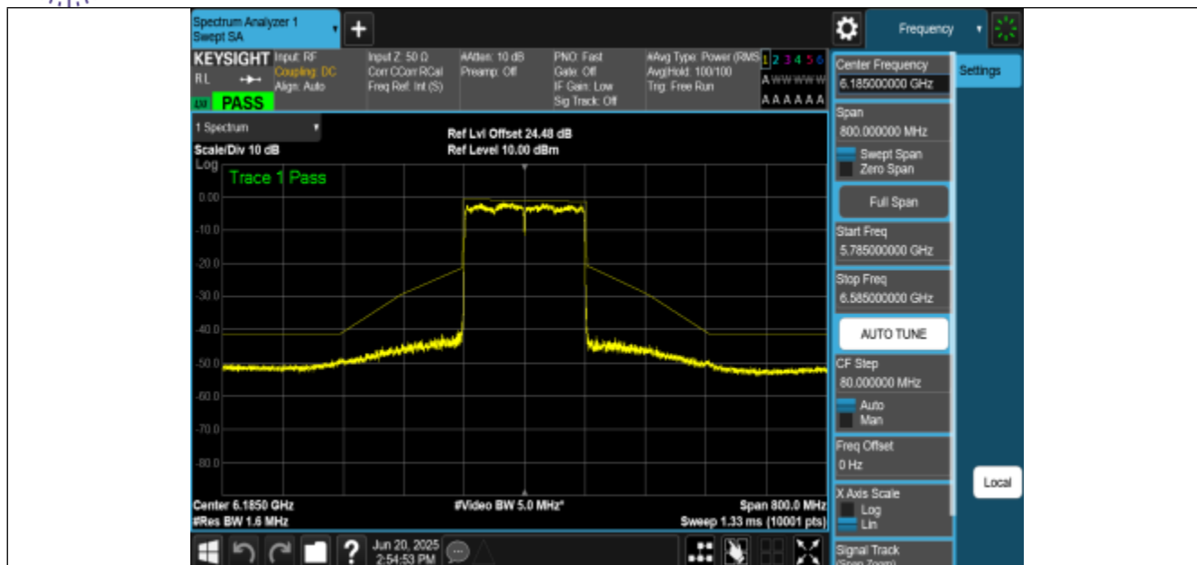
NTNV-11BE160MIMO-Ant1-6185-PASS
