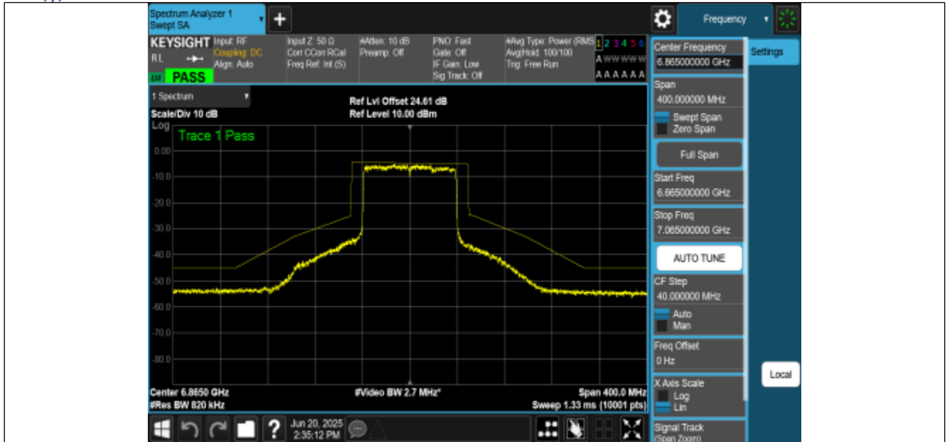
NTNV-11BE80MIMO-Ant3-6865-PASS
