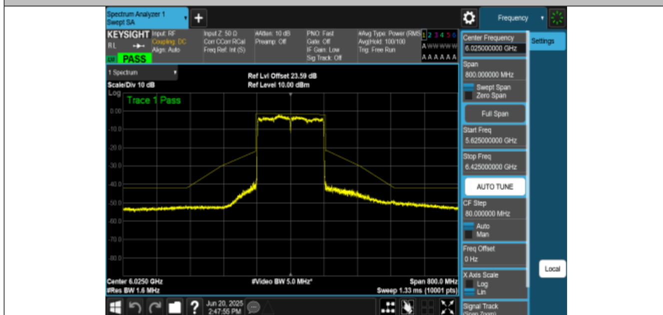
NTNV-11BE160MIMO-Ant0-6025-PASS
