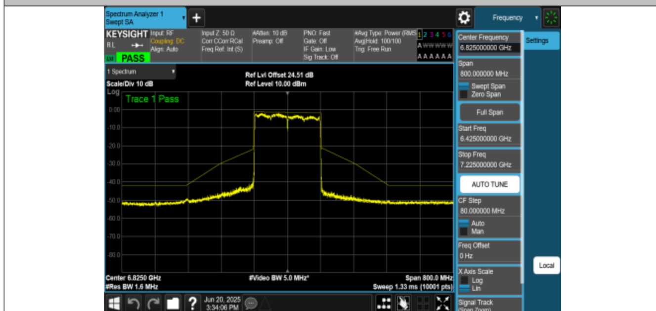
NTNV-11BE160MIMO-Ant0-6825-PASS
