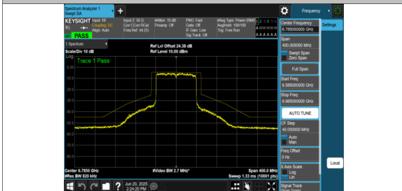
NTNV-11BE80MIMO-Ant0-6785-PASS
