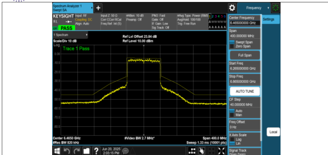
NTNV-11BE80MIMO-Ant1-6465-PASS
