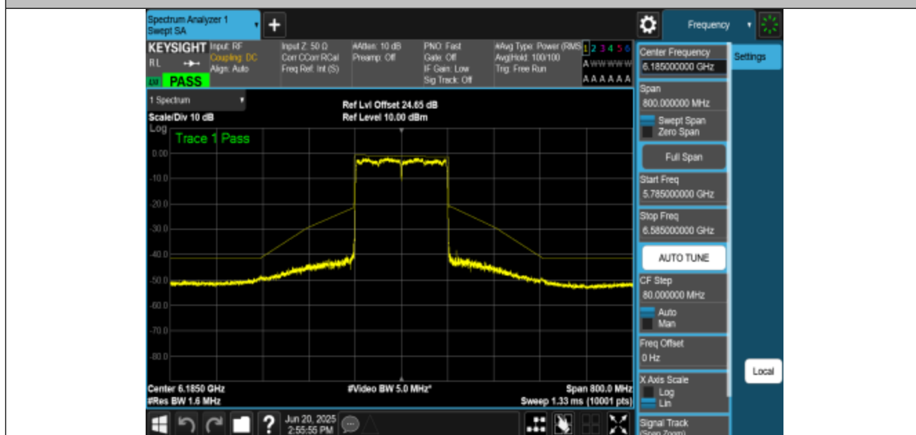
NTNV-11BE160MIMO-Ant2-6185-PASS
