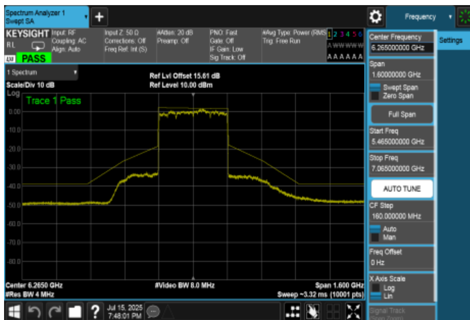
NTNV-11BE320MIMO-Ant3-6265-PASS
