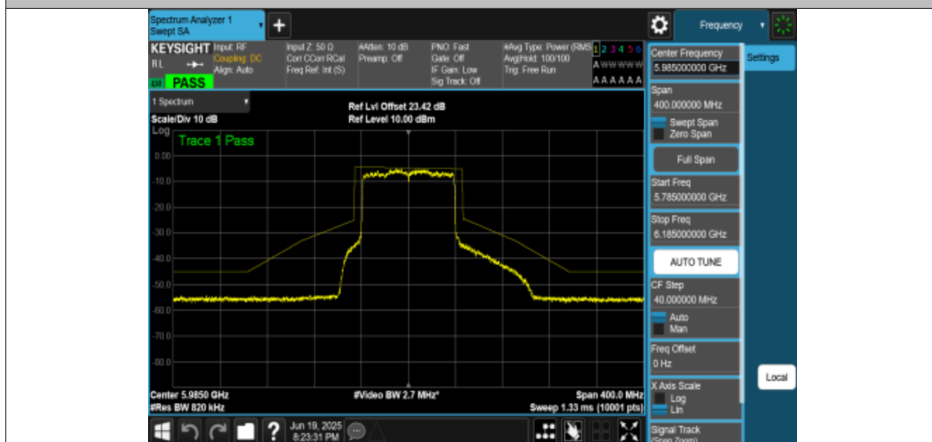
NTNV-11BE80MIMO-Ant0-5985-PASS
