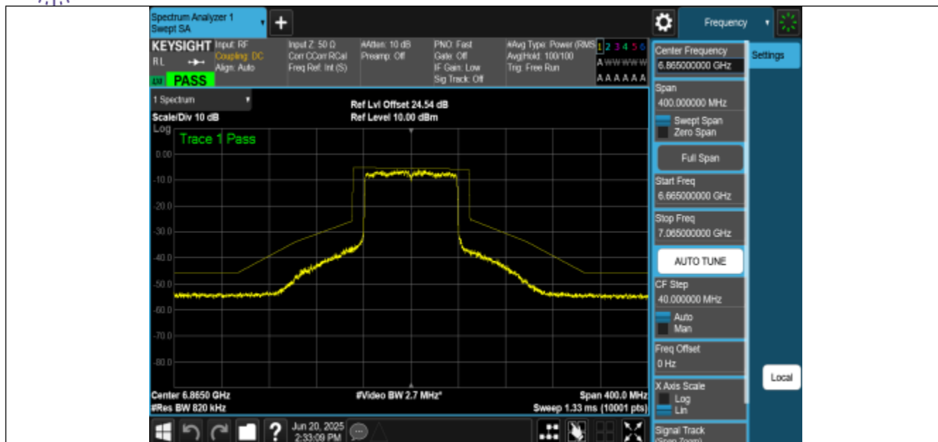
NTNV-11BE80MIMO-Ant1-6865-PASS
