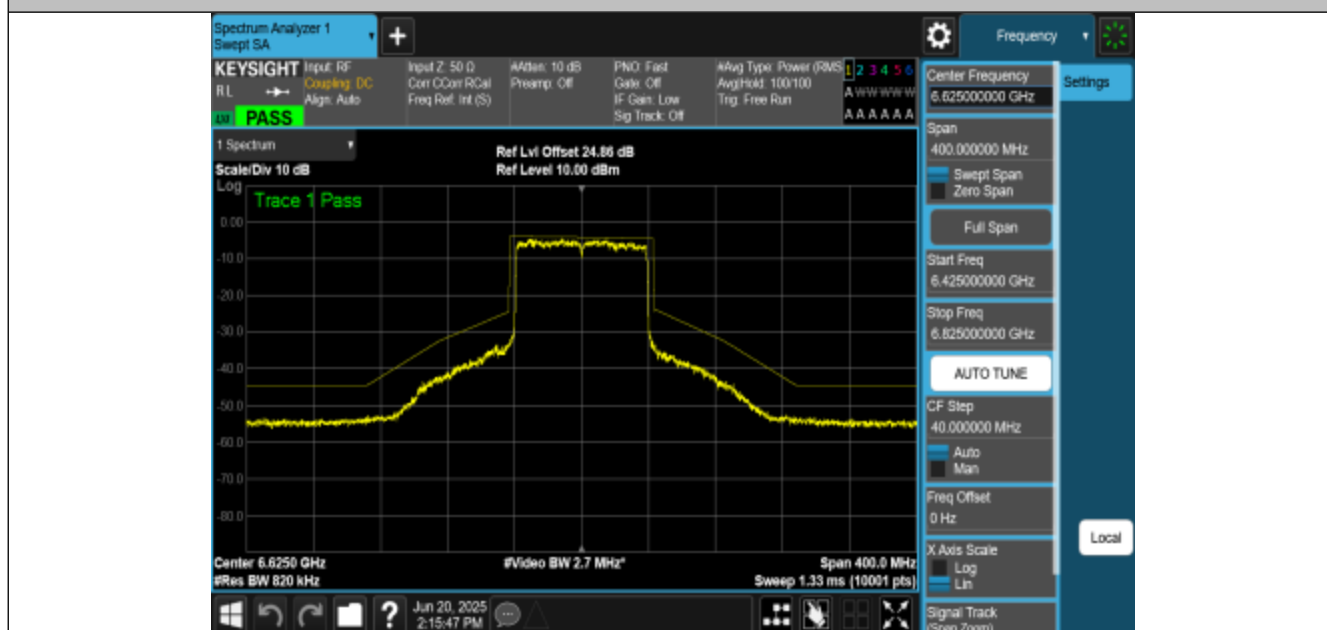
NTNV-11BE80MIMO-Ant2-6625-PASS
