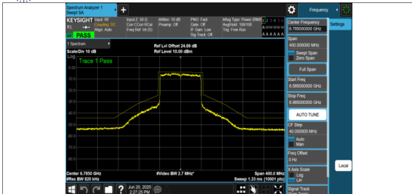
NTNV-11BE80MIMO-Ant3-6785-PASS
