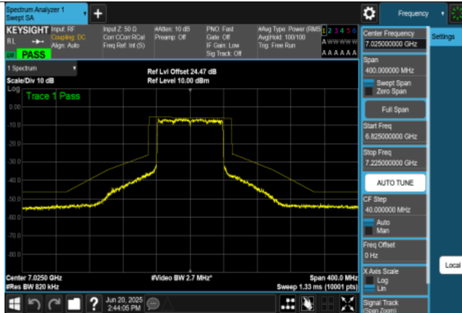
NTNV-11BE80MIMO-Ant1-7025-PASS
