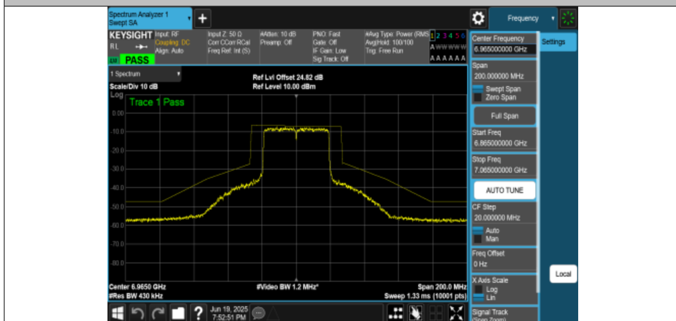
NTNV-11BE40MIMO-Ant0-6965-PASS
