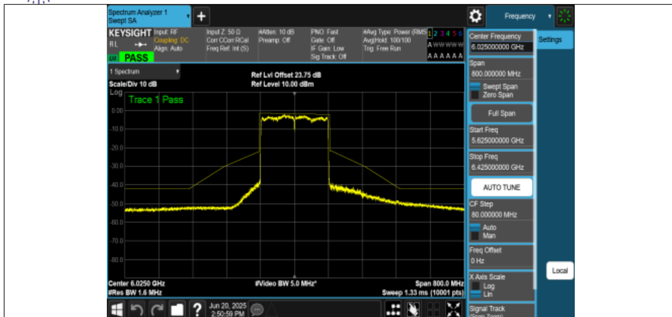
NTNV-11BE160MIMO-Ant3-6025-PASS
