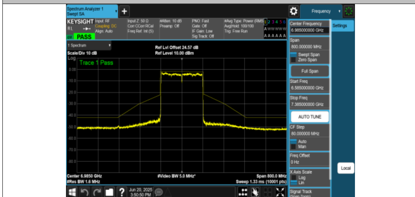
NTNV-11BE160MIMO-Ant0-6985-PASS
