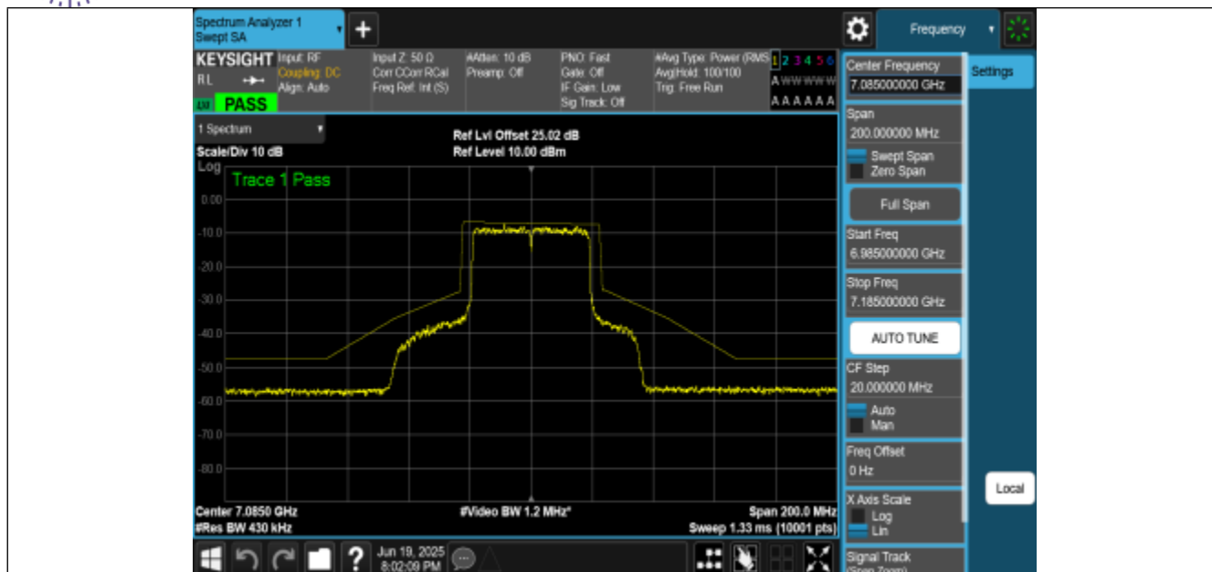
NTNV-11BE40MIMO-Ant3-7085-PASS
