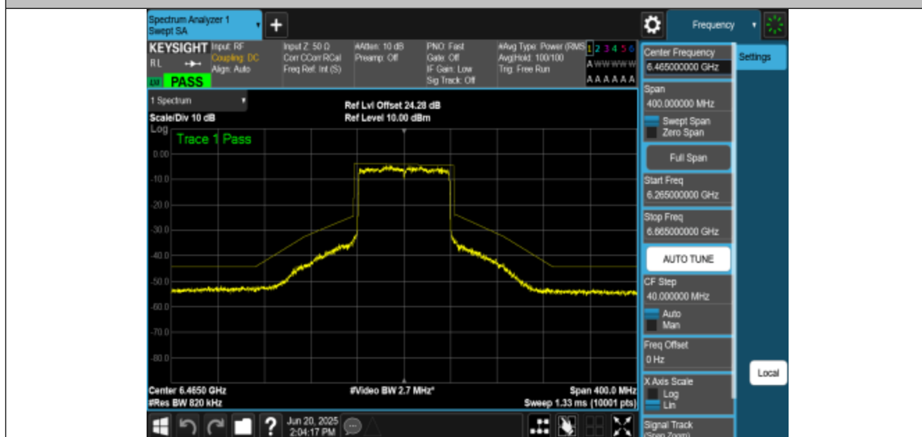
NTNV-11BE80MIMO-Ant2-6465-PASS
