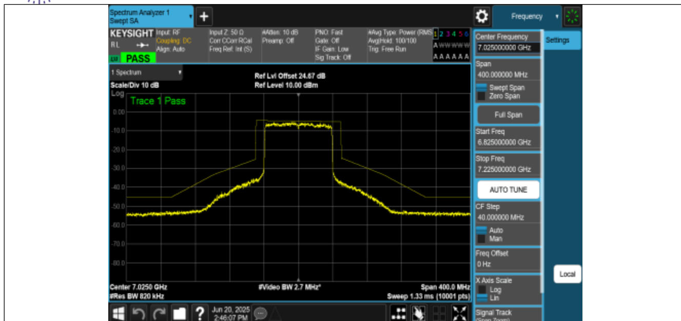
NTNV-11BE80MIMO-Ant3-7025-PASS
