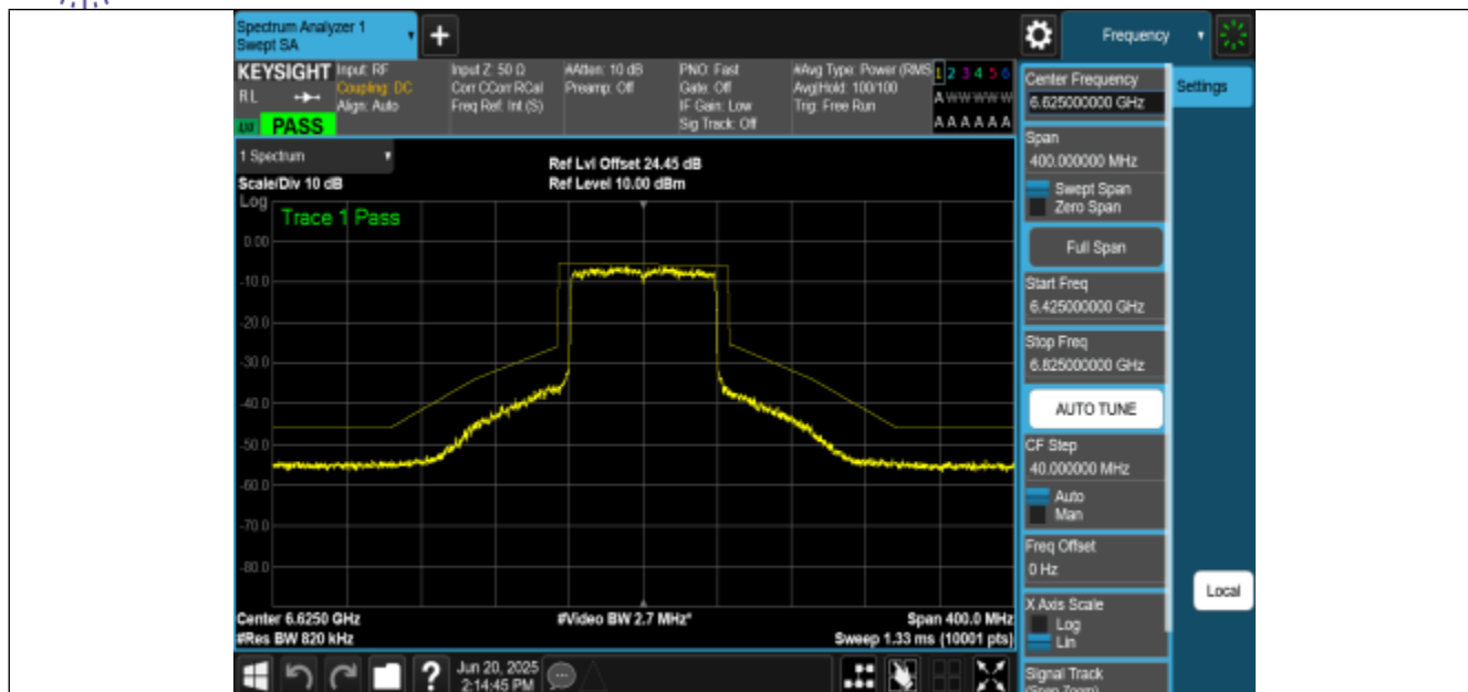
NTNV-11BE80MIMO-Ant1-6625-PASS
