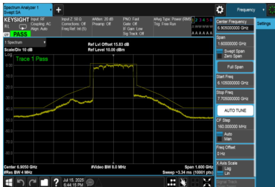
NTNV-11BE320MIMO-Ant2-6905-PASS
