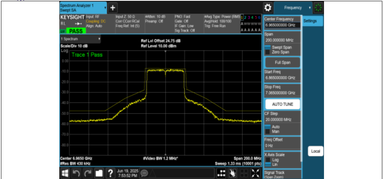
NTNV-11BE40MIMO-Ant1-6965-PASS
