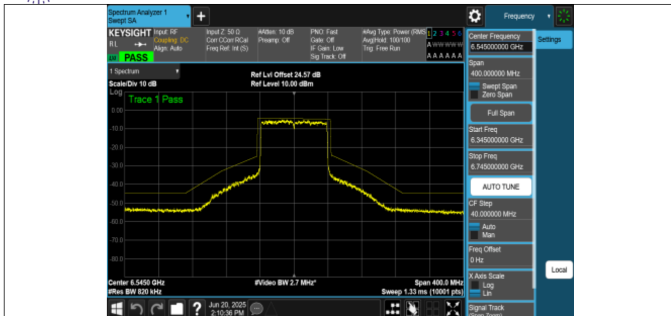
NTNV-11BE80MIMO-Ant3-6545-PASS
