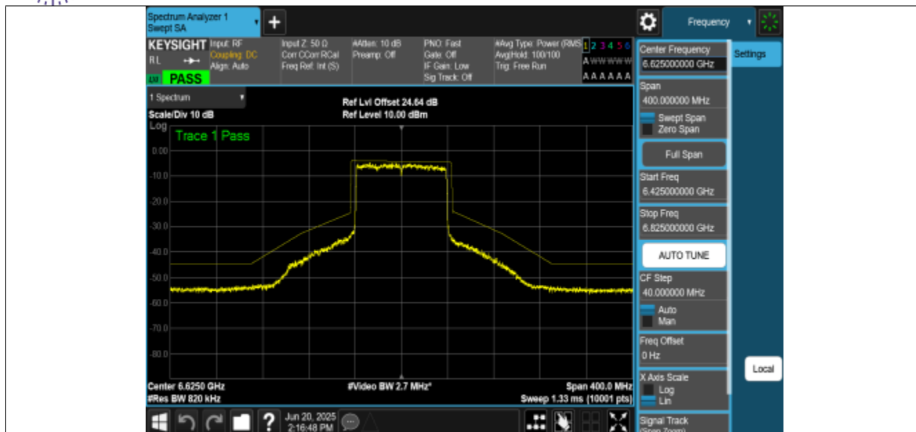
NTNV-11BE80MIMO-Ant3-6625-PASS
