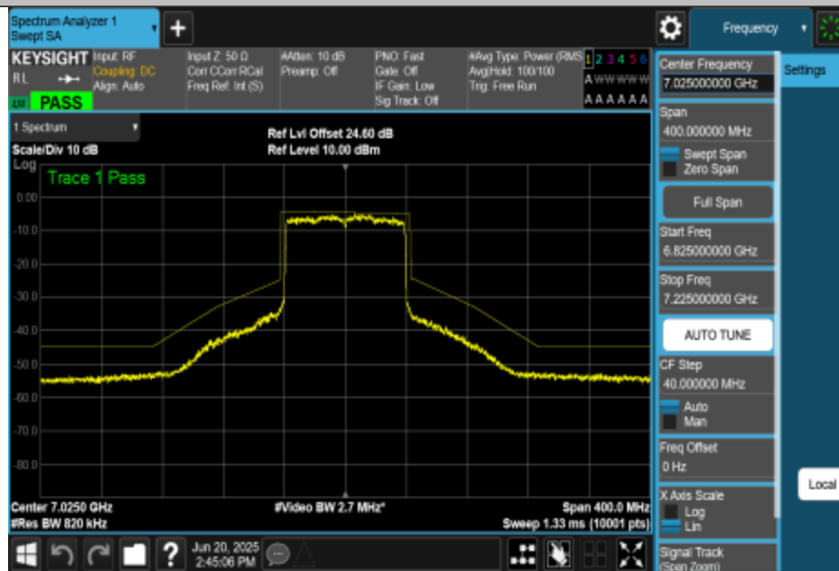
NTNV-11BE80MIMO-Ant2-7025-PASS
