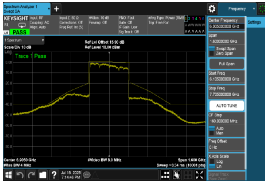
NTNV-11BE320MIMO-Ant3-6905-PASS
