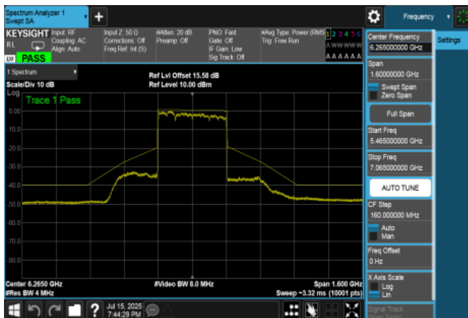
NTNV-11BE320MIMO-Ant2-6265-PASS
