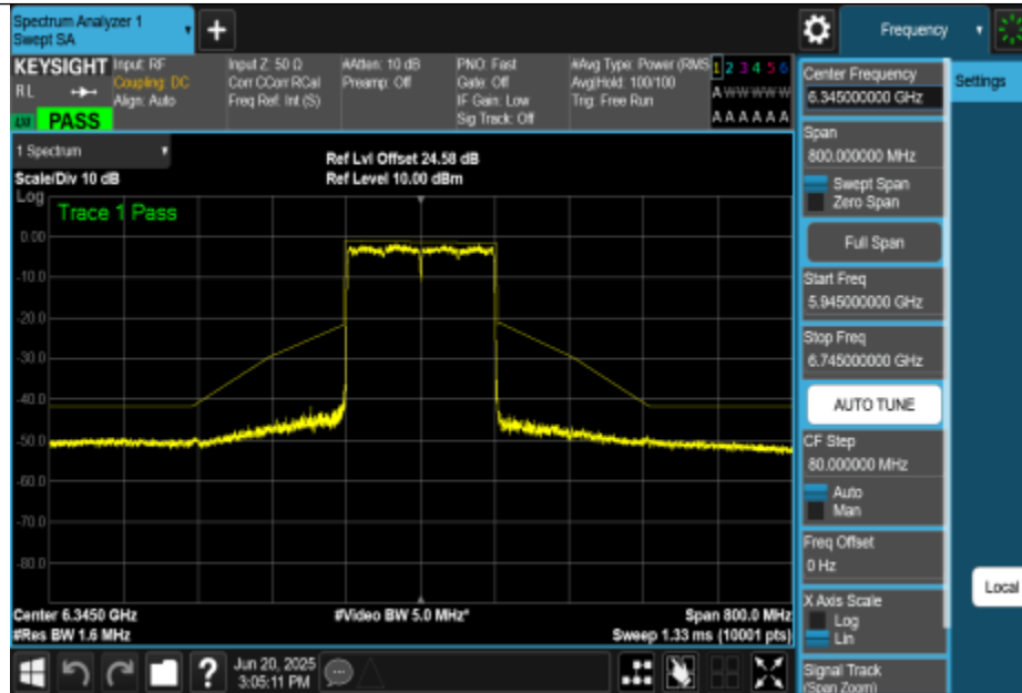
NTNV-11BE160MIMO-Ant3-6345-PASS
