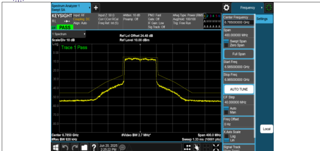
NTNV-11BE80MIMO-Ant1-6785-PASS
