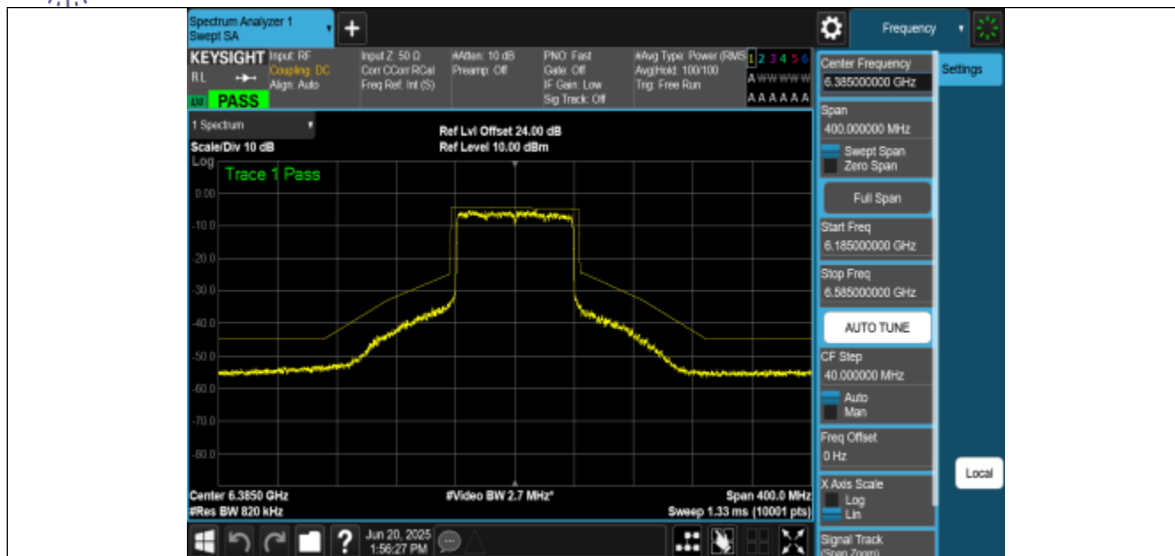
NTNV-11BE80MIMO-Ant1-6385-PASS
