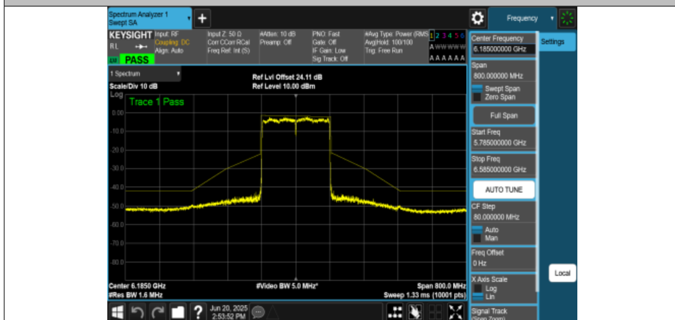
NTNV-11BE160MIMO-Ant0-6185-PASS
