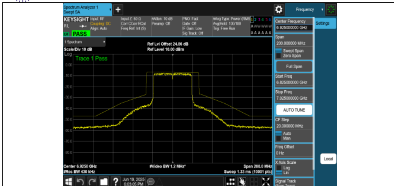
NTNV-11BE40MIMO-Ant3-6925-PASS
