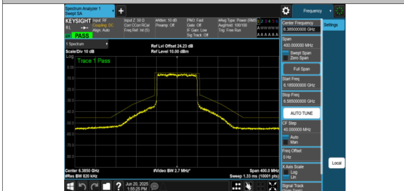
NTNV-11BE80MIMO-Ant0-6385-PASS
