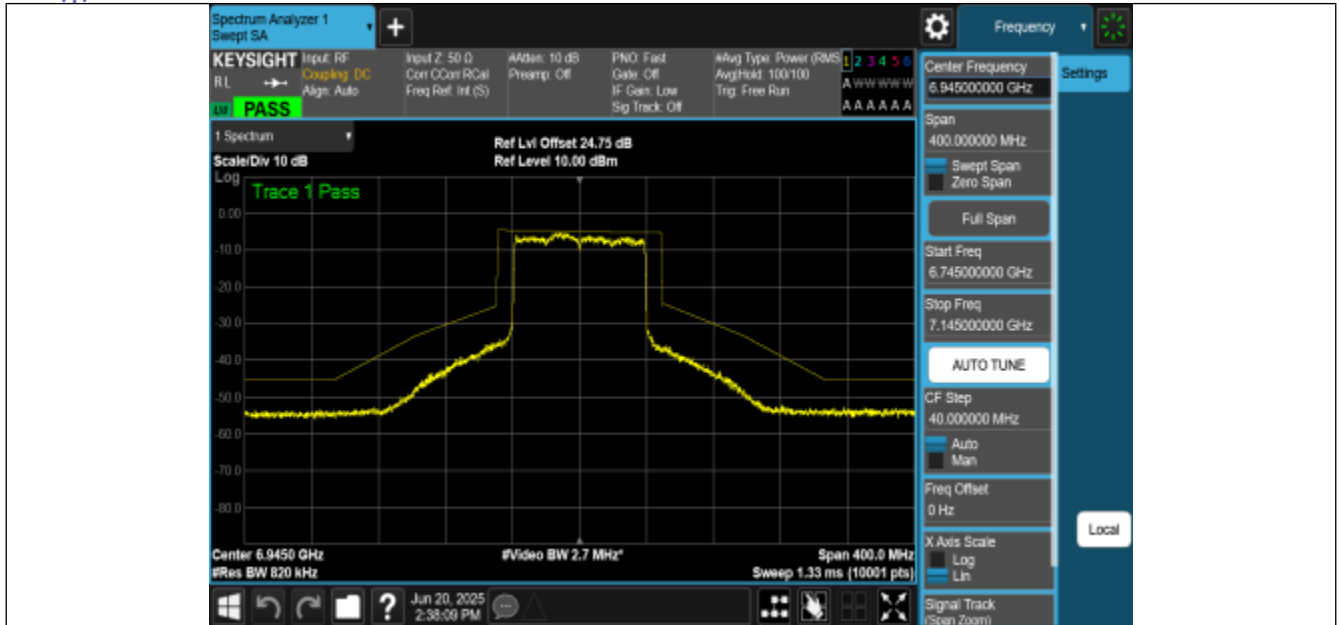
NTNV-11BE80MIMO-Ant1-6945-PASS
