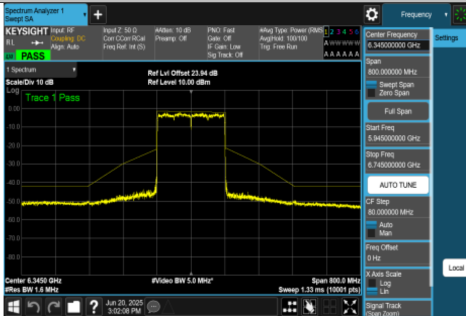
NTVN-11BE160MIMO-Ant0-6345-PASS
