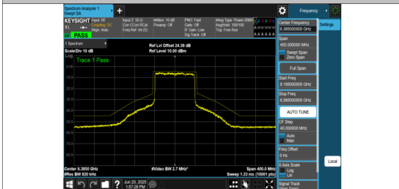
NTNV-11BE80MIMO-Ant2-6385-PASS
