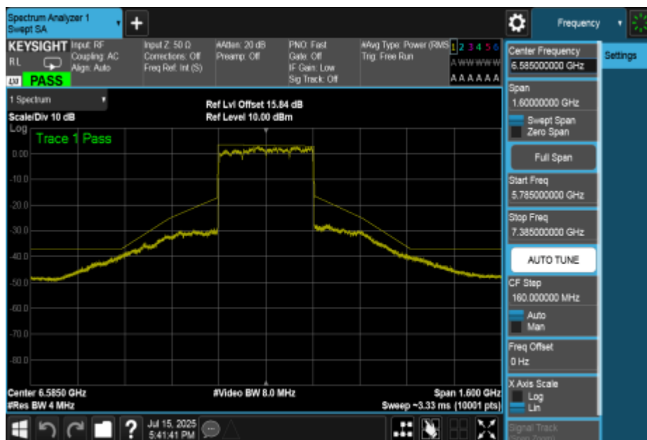
NTNV-11BE320MIMO-Ant0-6585-PASS
