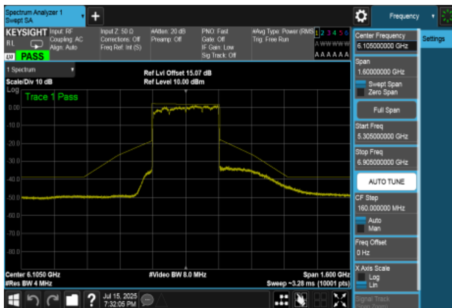
NTNV-11BE320MIMO-Ant3-6105-PASS
