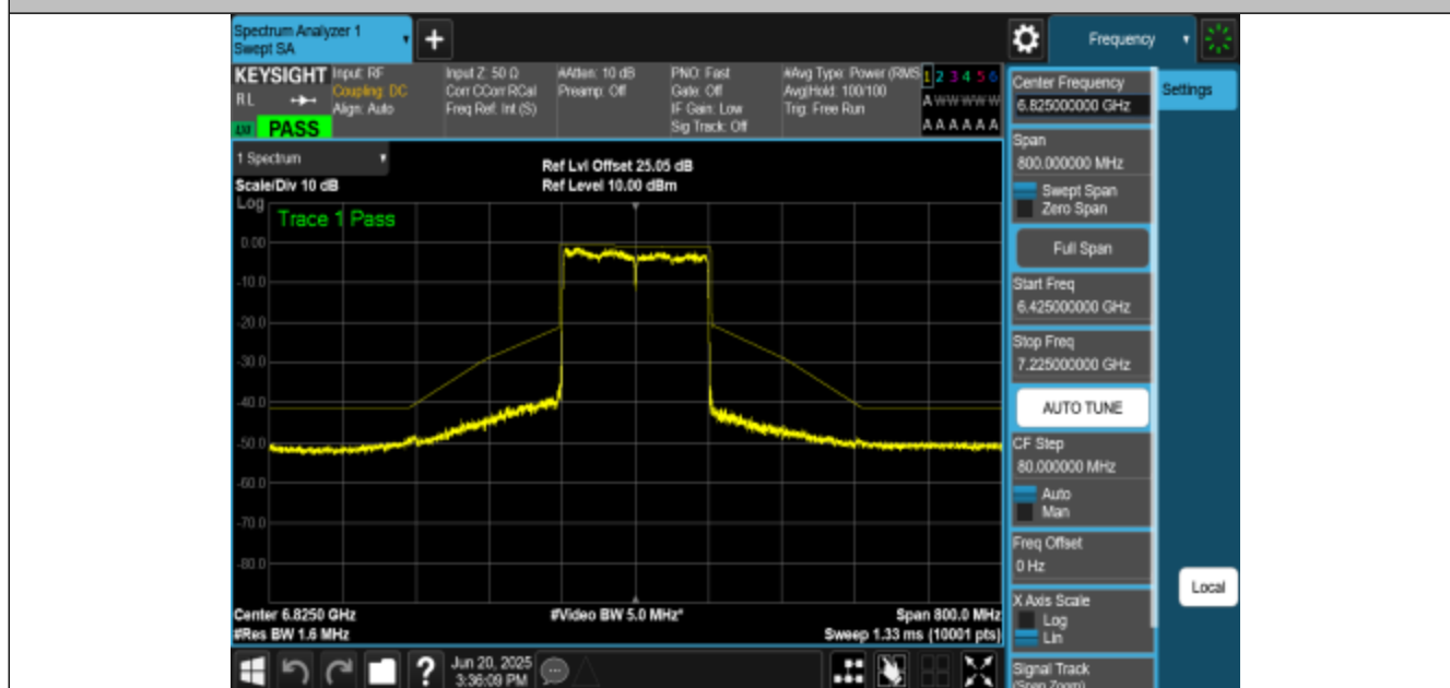
NTNV-11BE160MIMO-Ant2-6825-PASS
