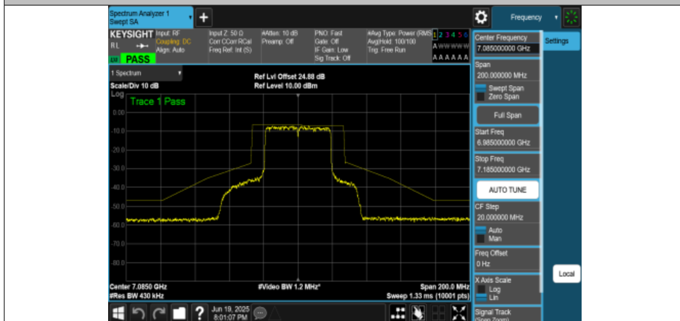
NTNV-11BE40MIMO-Ant2-7085-PASS
