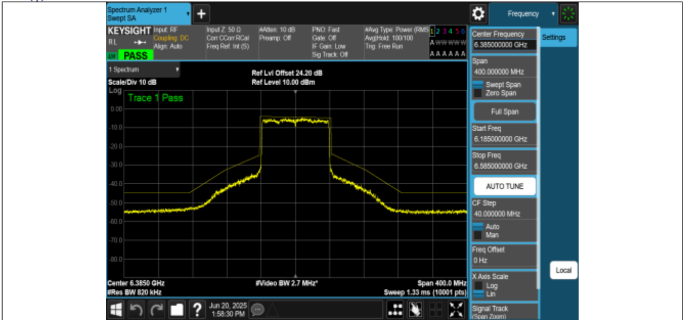
NTNV-11BE80MIMO-Ant3-6385-PASS
