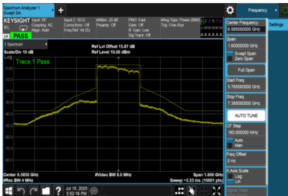
NTNV-11BE320MIMO-Ant3-6585-PASS
