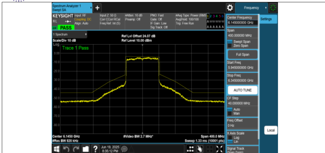
NTNV-11BE80MIMO-Ant3-6145-PASS
