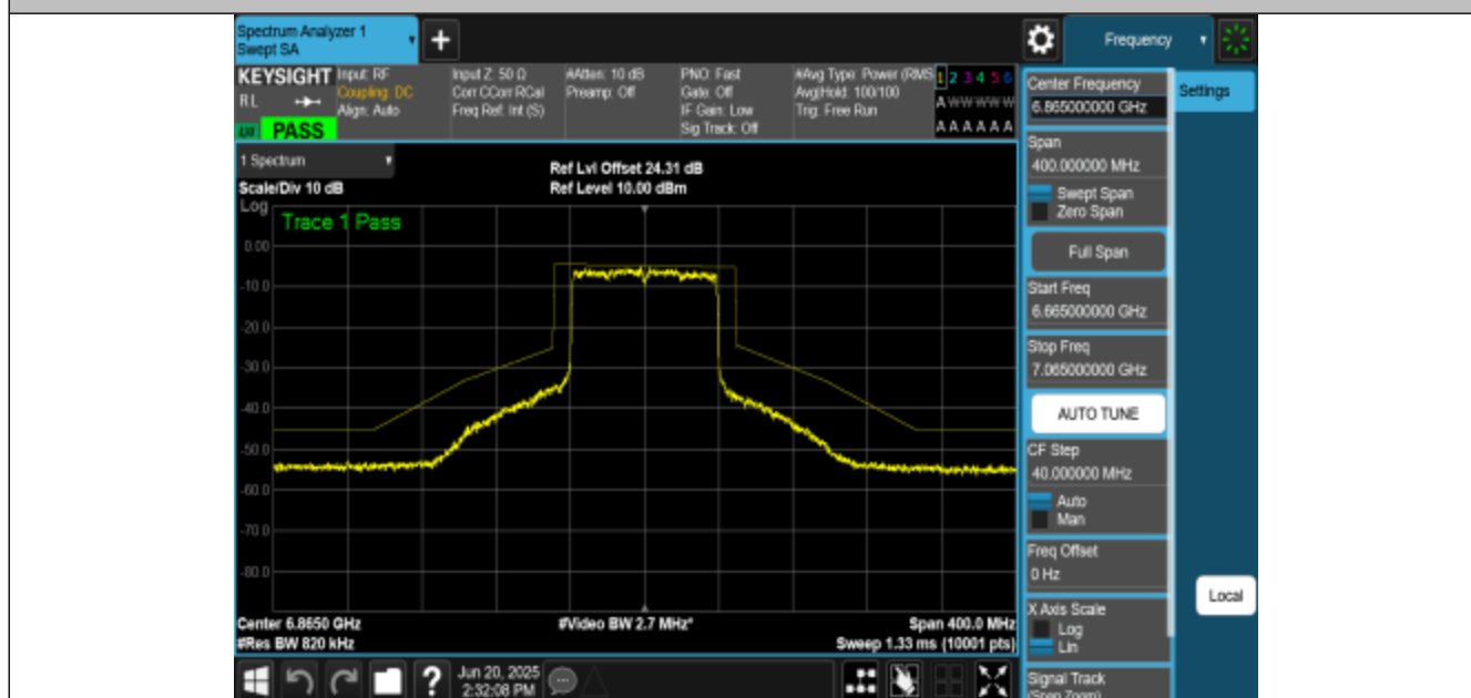
NTNV-11BE80MIMO-Ant0-6865-PASS
