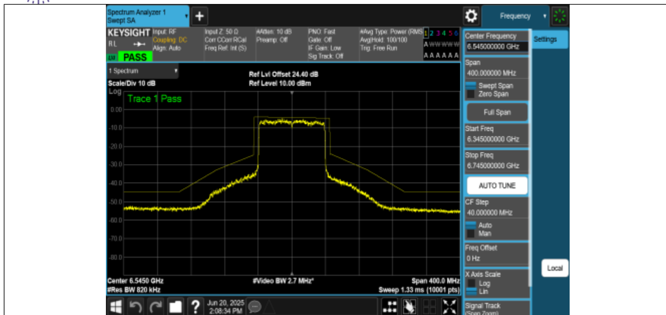
NTNV-11BE80MIMO-Ant1-6545-PASS
