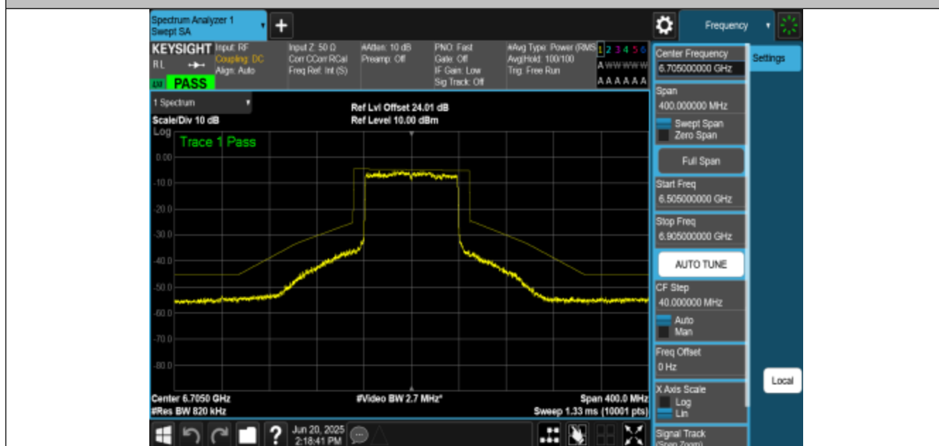
NTNV-11BE80MIMO-Ant0-6705-PASS
