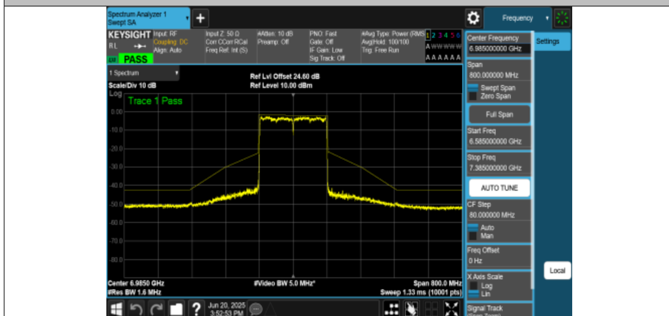
NTNV-11BE160MIMO-Ant2-6985-PASS
