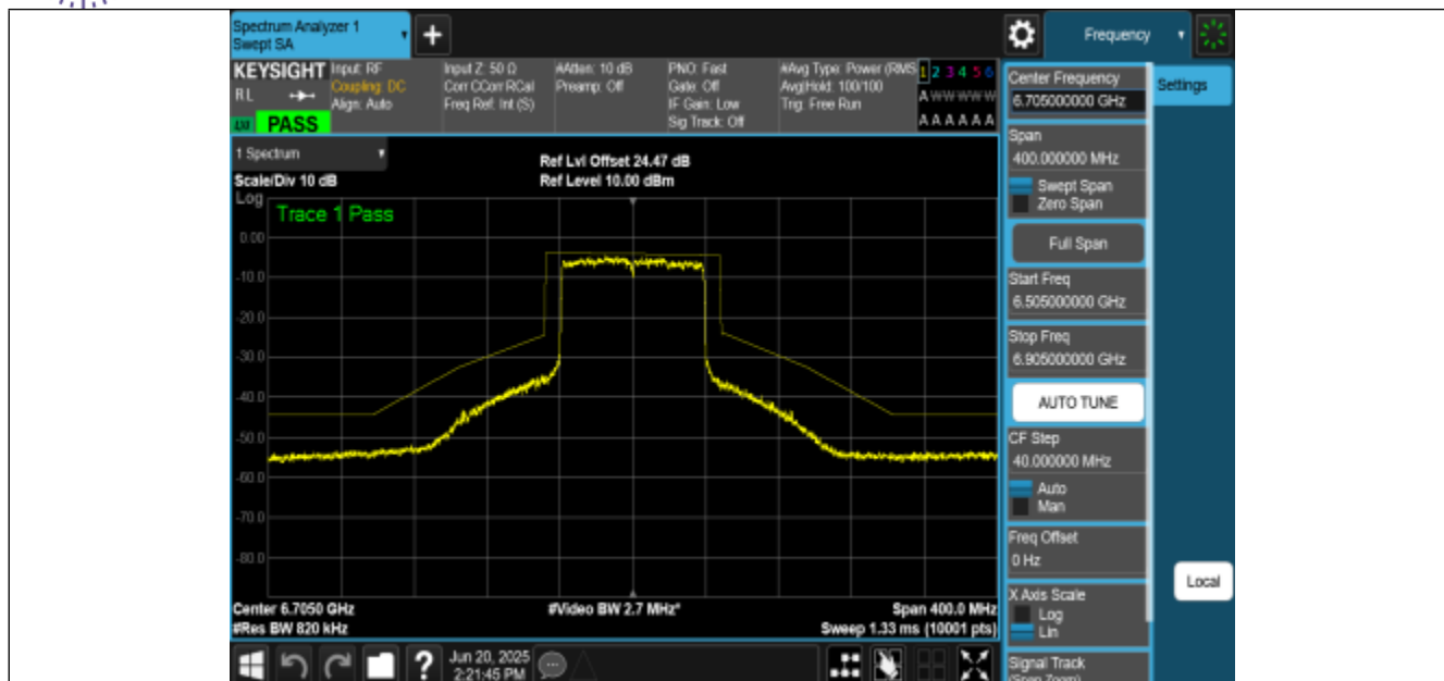
NTNV-11BE80MIMO-Ant3-6705-PASS
