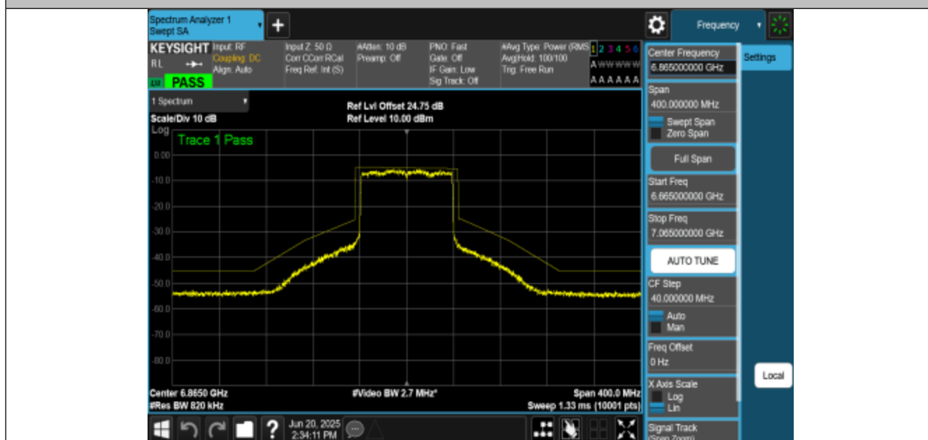
NTNV-11BE80MIMO-Ant2-6865-PASS
