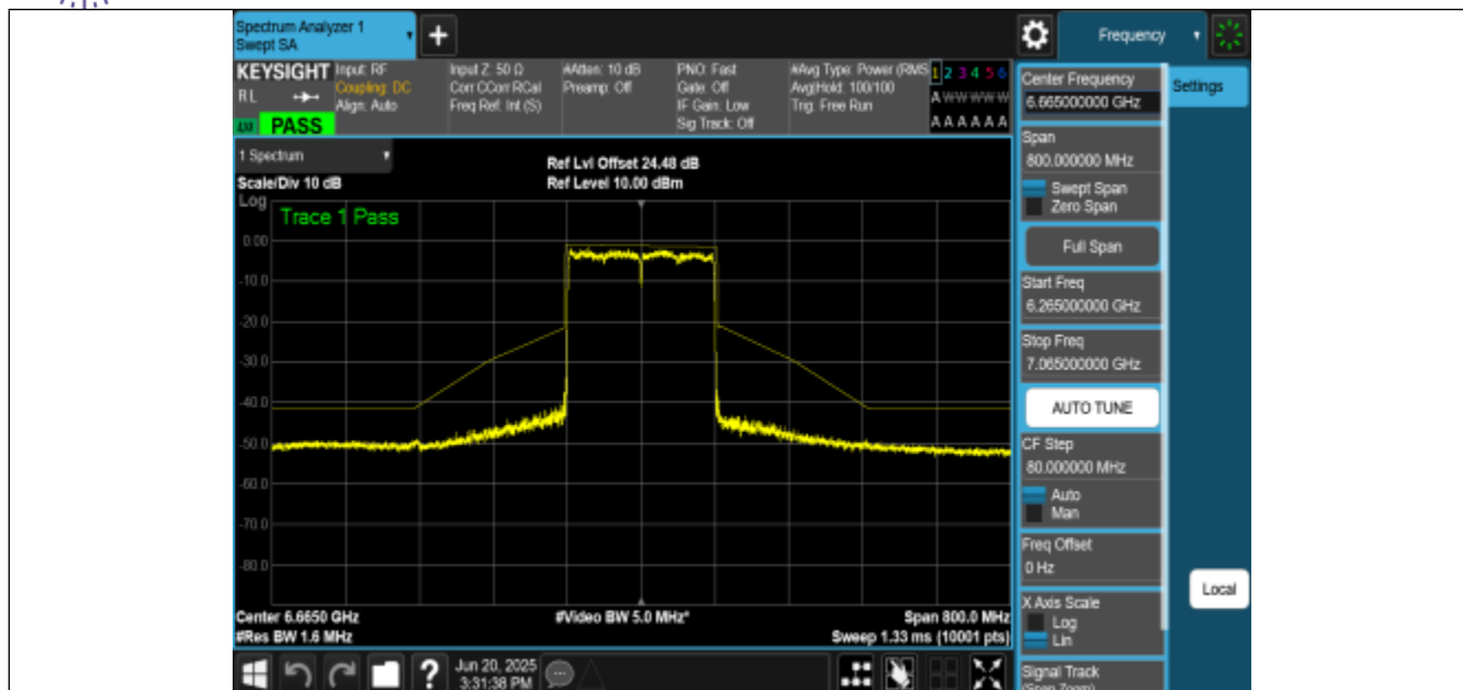
NTNV-11BE160MIMO-Ant3-6665-PASS
