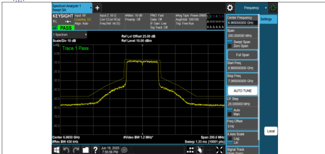
NTNV-11BE40MIMO-Ant3-6965-PASS
