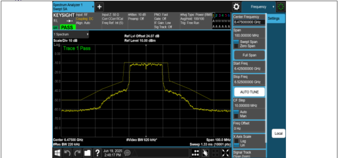
NTNV-11BE20MIMO-Ant0-6475-PASS
