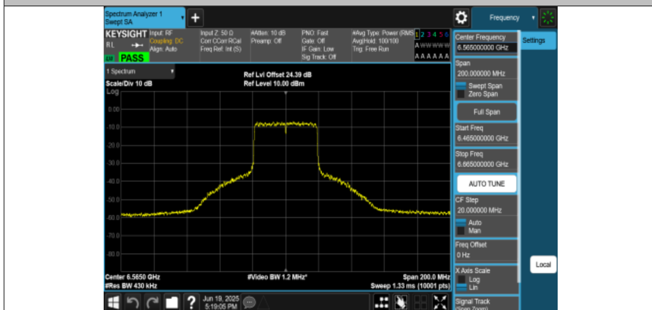
NTNV-11BE40MIMO-Ant0-6565-PASS
