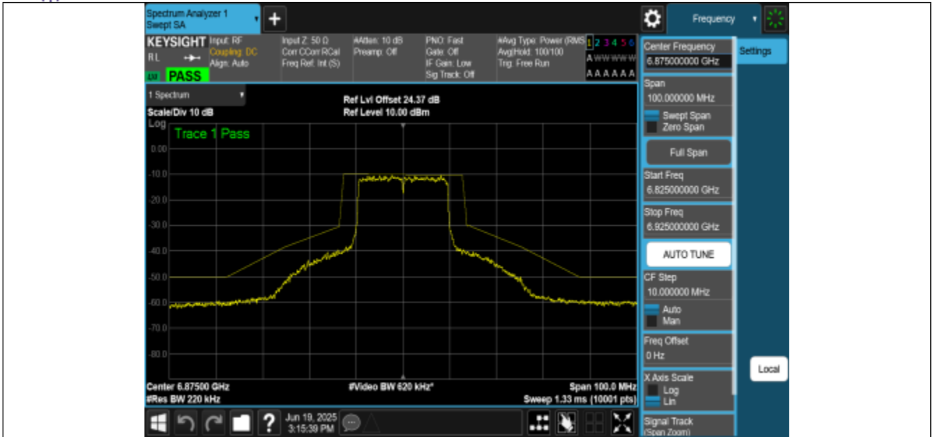
NTNV-11BE20MIMO-Ant0-6875-PASS
