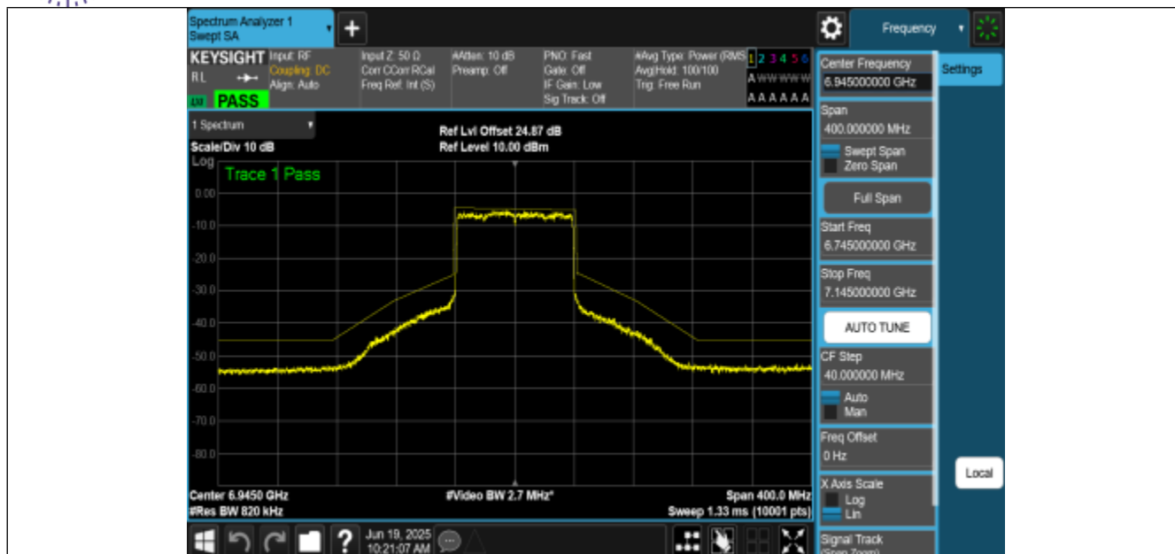
NTNV-11AX80MIMO-Ant2-6945-PASS
