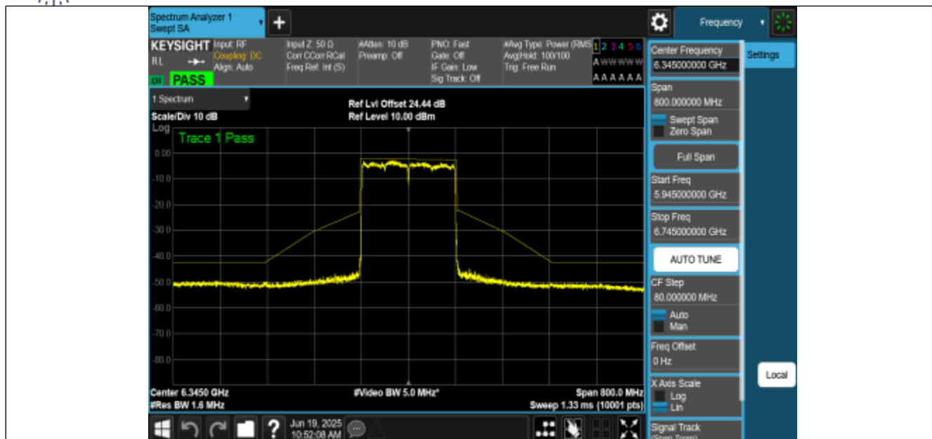
NTNV-11AX160MIMO-Ant2-6345-PASS
