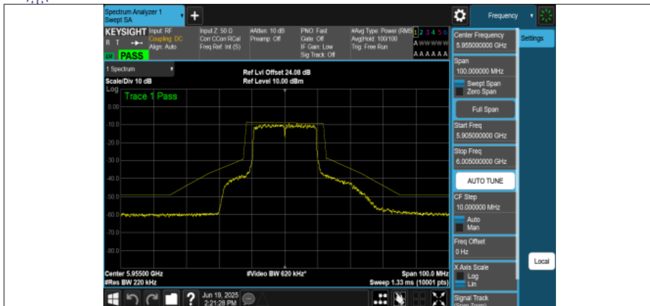
NTNV-11BE20MIMO-Ant0-5955-PASS
