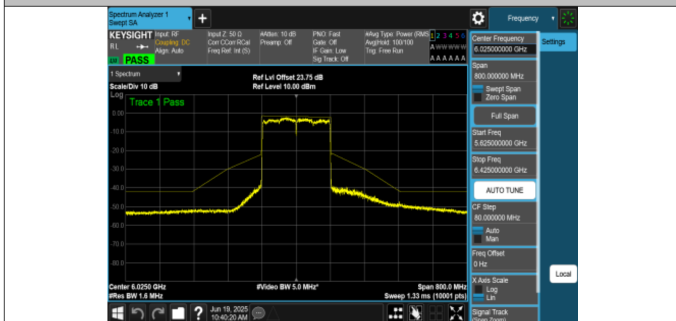
NTNV-11AX160MIMO-Ant3-6025-PASS
