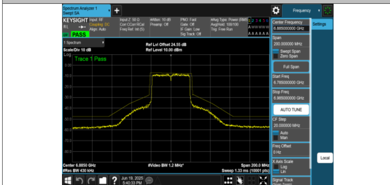
NTNV-11BE40MIMO-Ant2-6885-PASS
