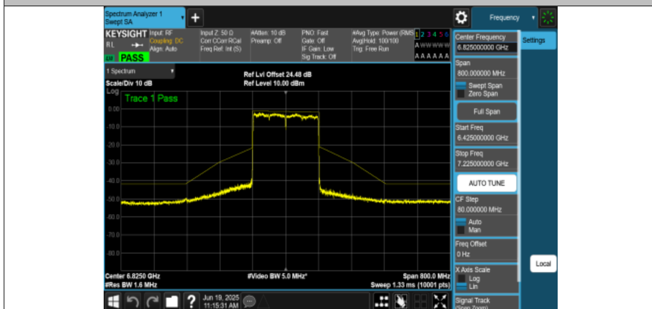
NTNV-11AX160MIMO-Ant1-6825-PASS
