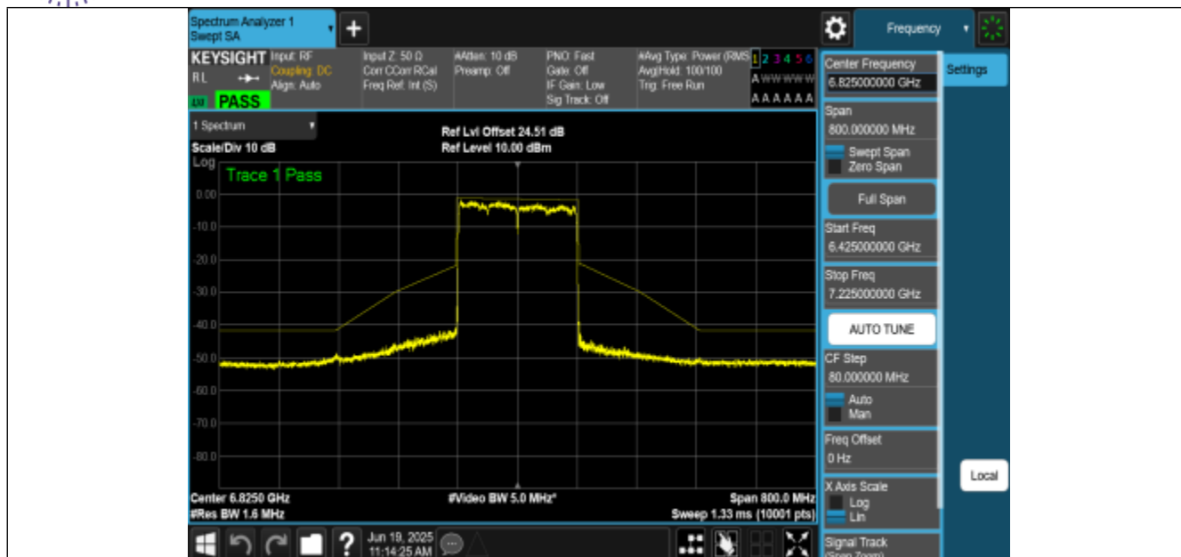
NTNV-11AX160MIMO-Ant0-6825-PASS
