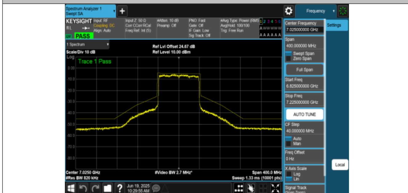
NTN-11AX80MIMO-Ant3-7025-PASS
