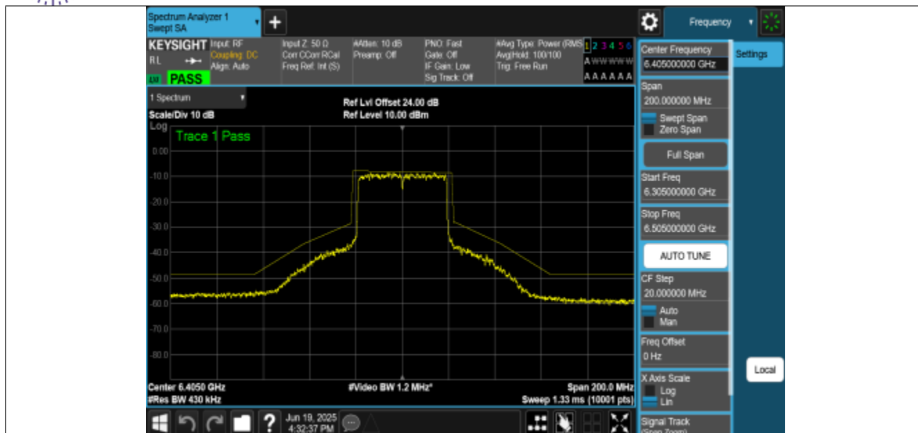
NTNV-11BE40MIMO-Ant1-6405-PASS
