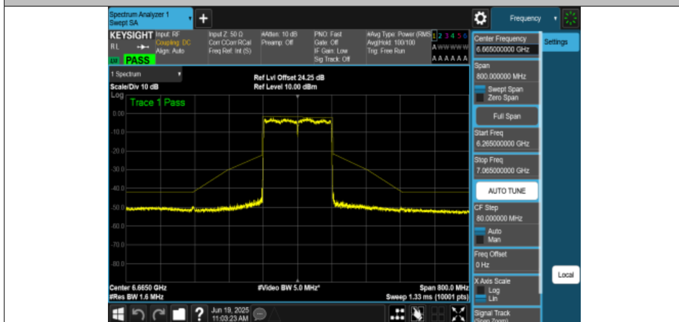
NTNV-11AX160MIMO-Ant1-6665-PASS
