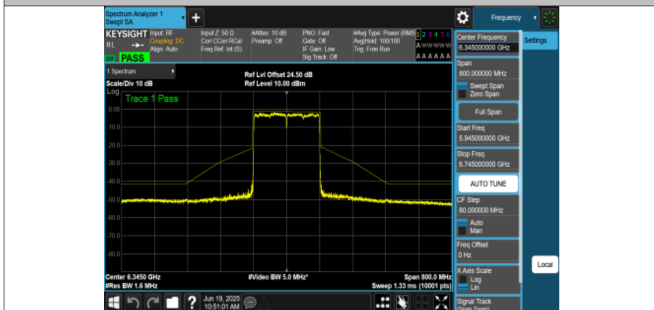
NTNV-11AX160MIMO-Ant1-6345-PASS
