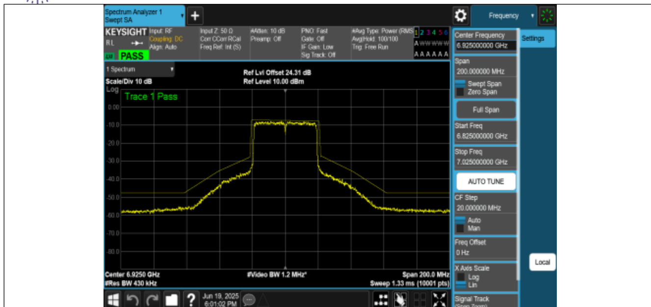
NTNV-11BE40MIMO-Ant1-6925-PASS
