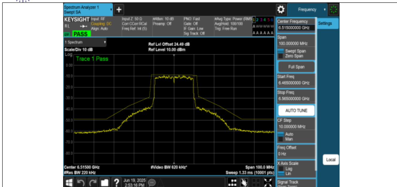
NTNV-11BE20MIMO-Ant0-6515-PASS
