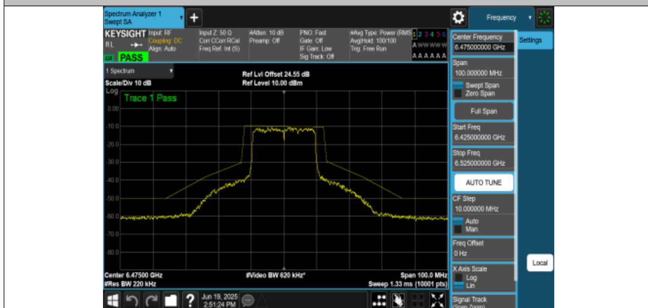
NTNV-11BE20MIMO-Ant3-6475-PASS
