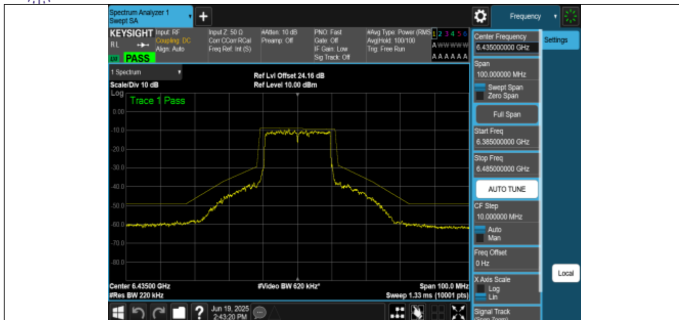
NTNV-11BE20MIMO-Ant0-6435-PASS
