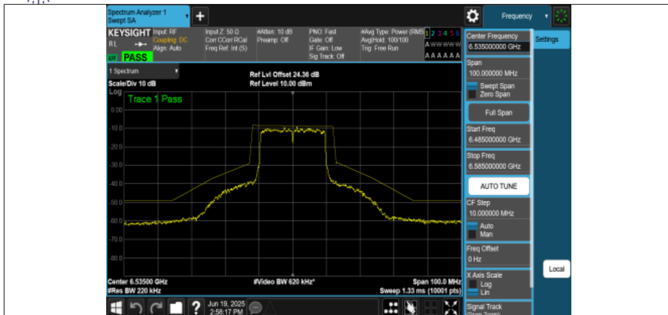
NTNV-11BE20MIMO-Ant0-6535-PASS
