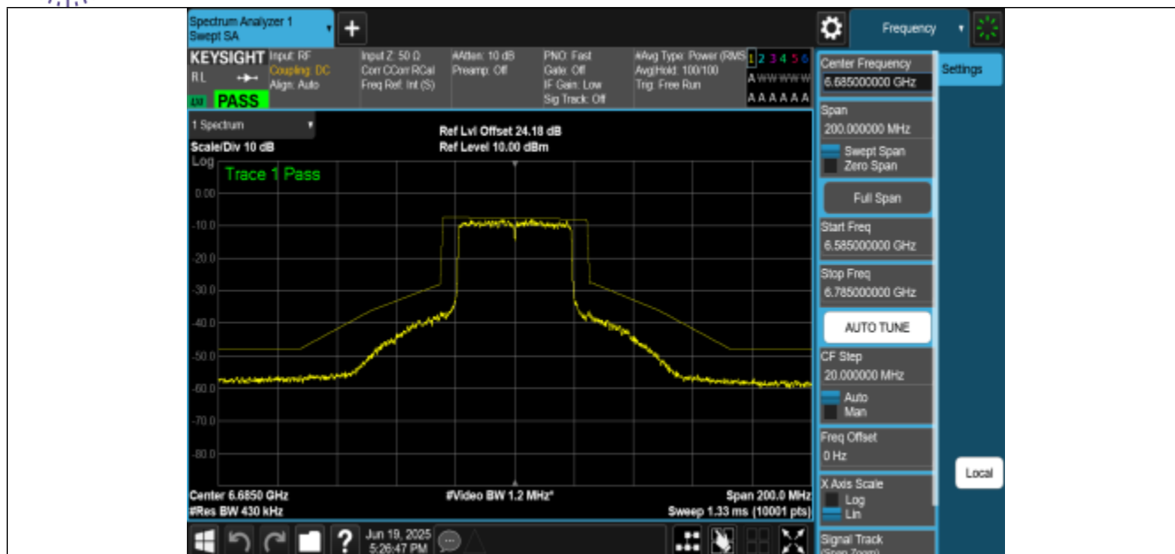
NTNV-11BE40MIMO-Ant1-6685-PASS
