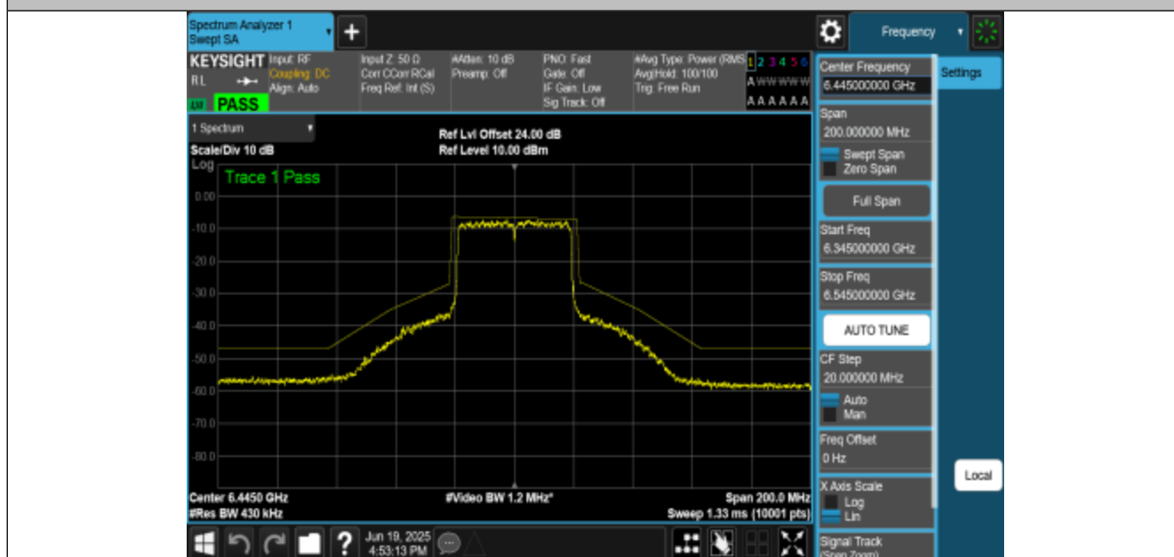
NTNV-11BE40MIMO-Ant0-6445-PASS
