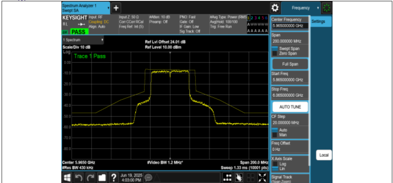
NTNV-11BE40MIMO-Ant0-5965-PASS
