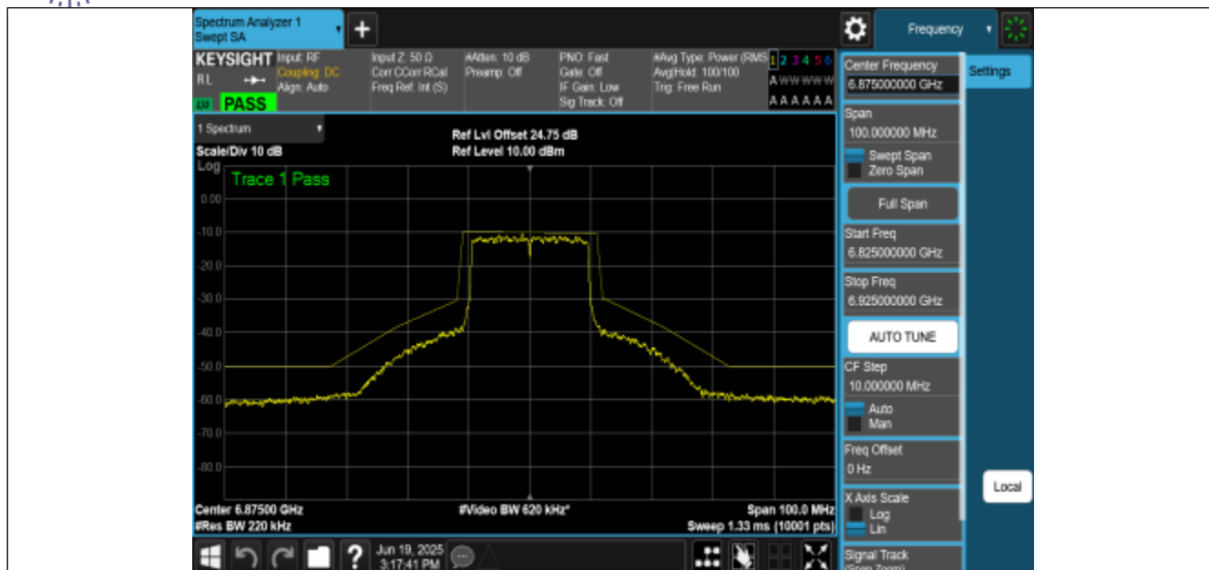
NTNV-11BE20MIMO-Ant2-6875-PASS
