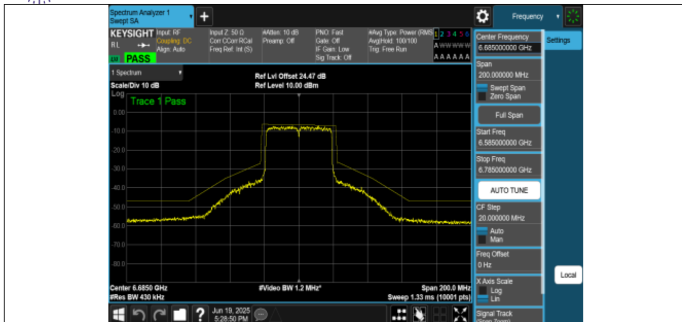
NTNV-11BE40MIMO-Ant3-6685-PASS
