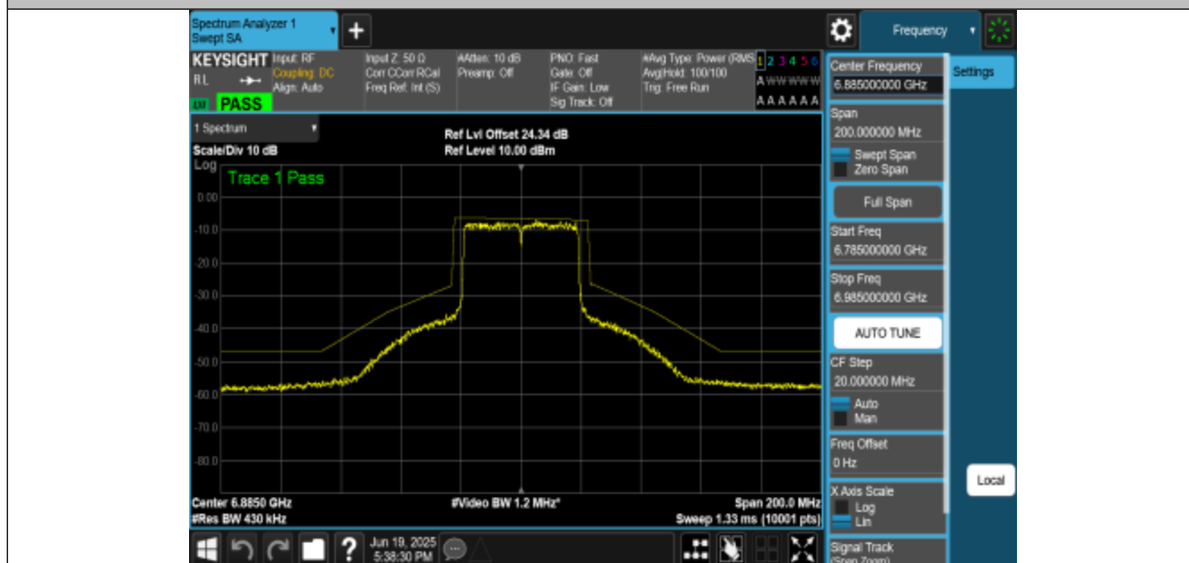
NTNV-11BE40MIMO-Ant0-6885-PASS
