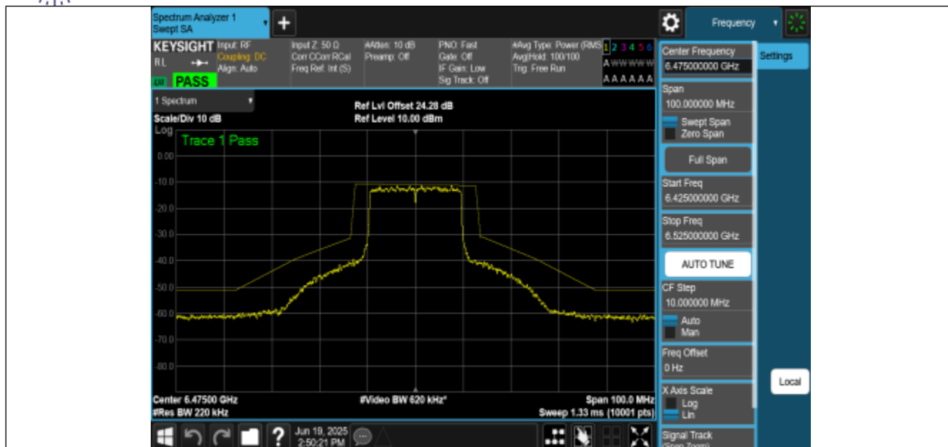
NTNV-11BE20MIMO-Ant2-6475-PASS
