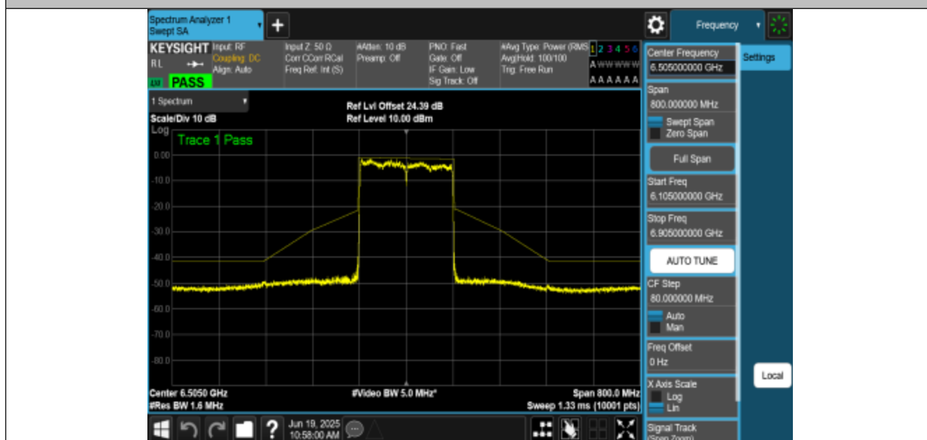
NTNV-11AX160MIMO-Ant1-6505-PASS
