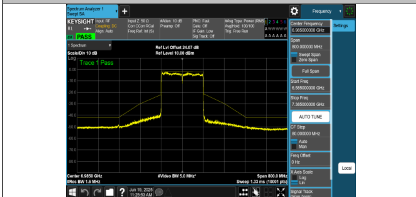
NTNV-11AX160MIMO-Ant3-6985-PASS
