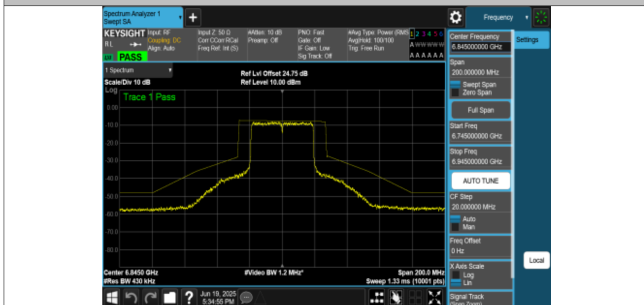
NTNV-11BE40MIMO-Ant2-6845-PASS
