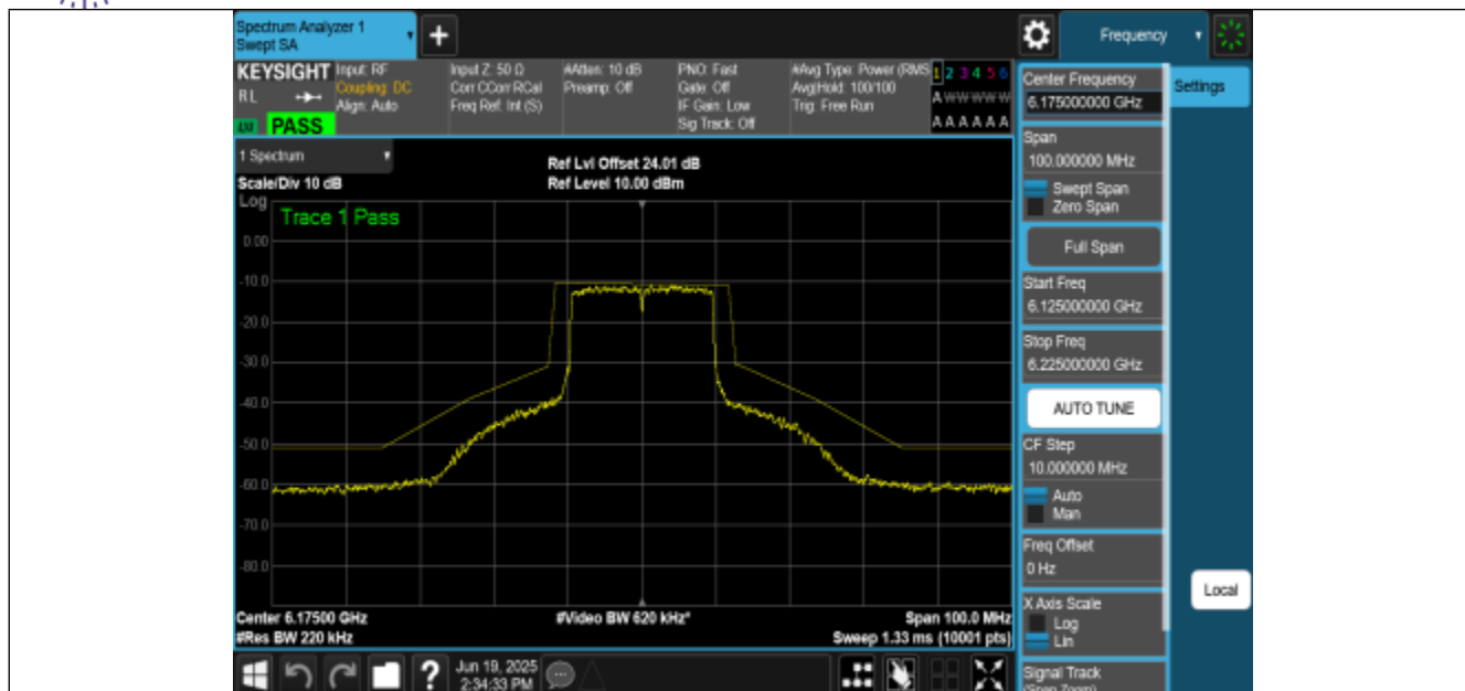
NTNV-11BE20MIMO-Ant2-6175-PASS
