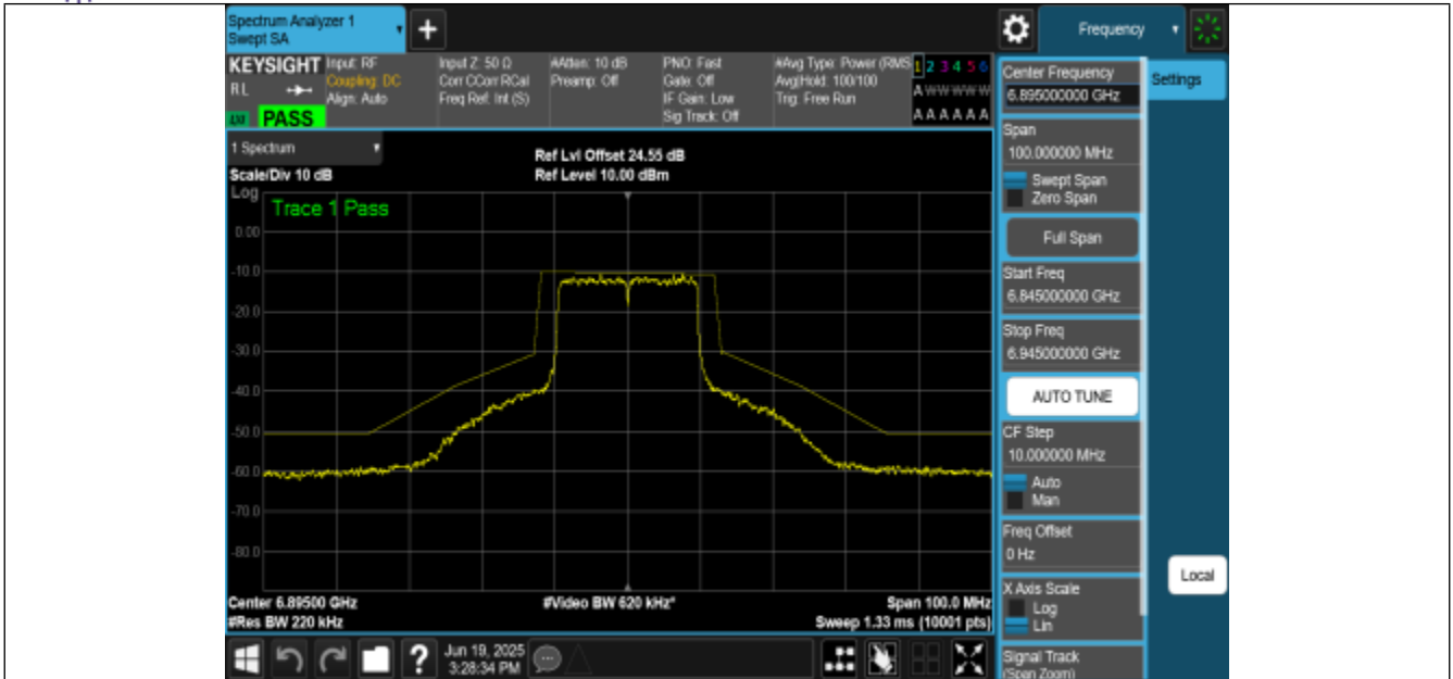
NTNV-11BE20MIMO-Ant2-6895-PASS
