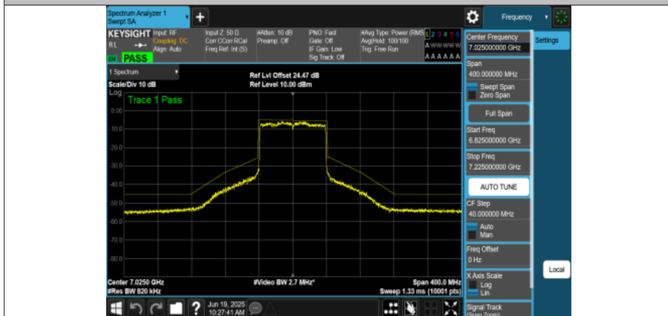
NTNV-11AX80MIMO-Ant1-7025-PASS
