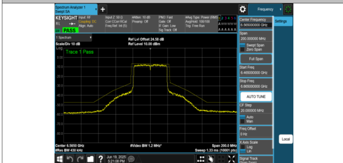
NTNV-11BE40MIMO-Ant2-6565-PASS
