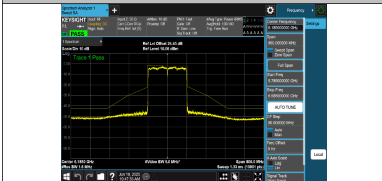
NTNV-11AX160MIMO-Ant3-6185-PASS
