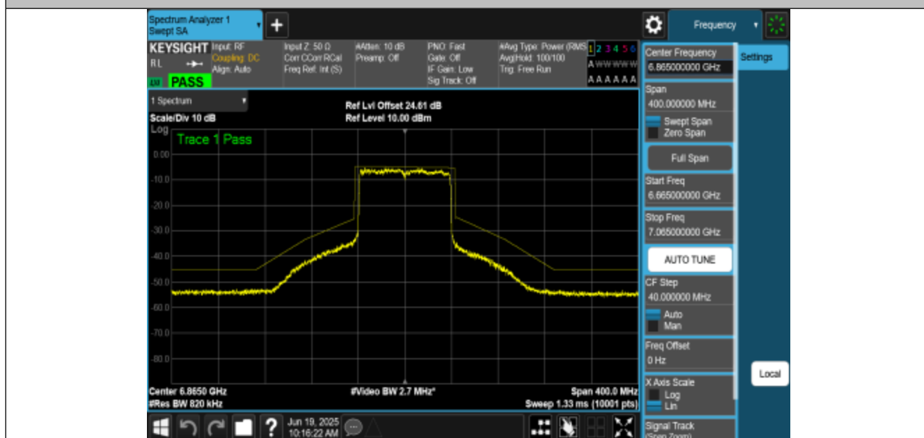
NTNV-11AX80MIMO-Ant3-6865-PASS
