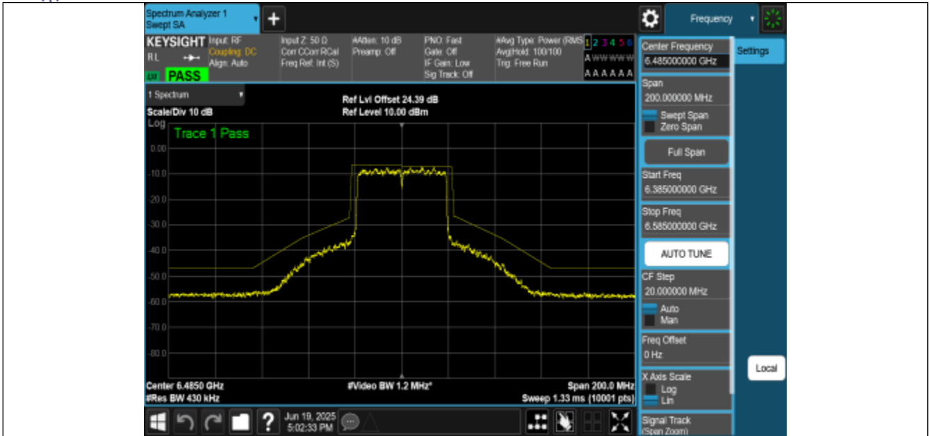
NTNV-11BE40MIMO-Ant1-6485-PASS
