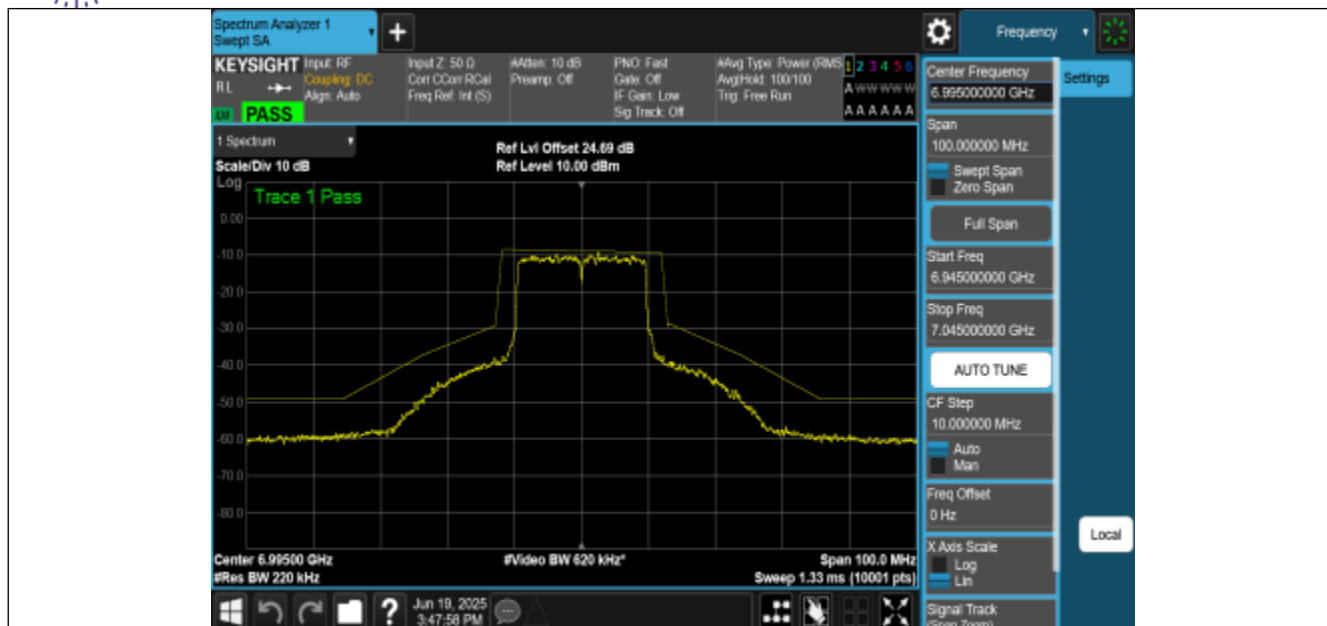
NTNV-11BE20MIMO-Ant0-6995-PASS
