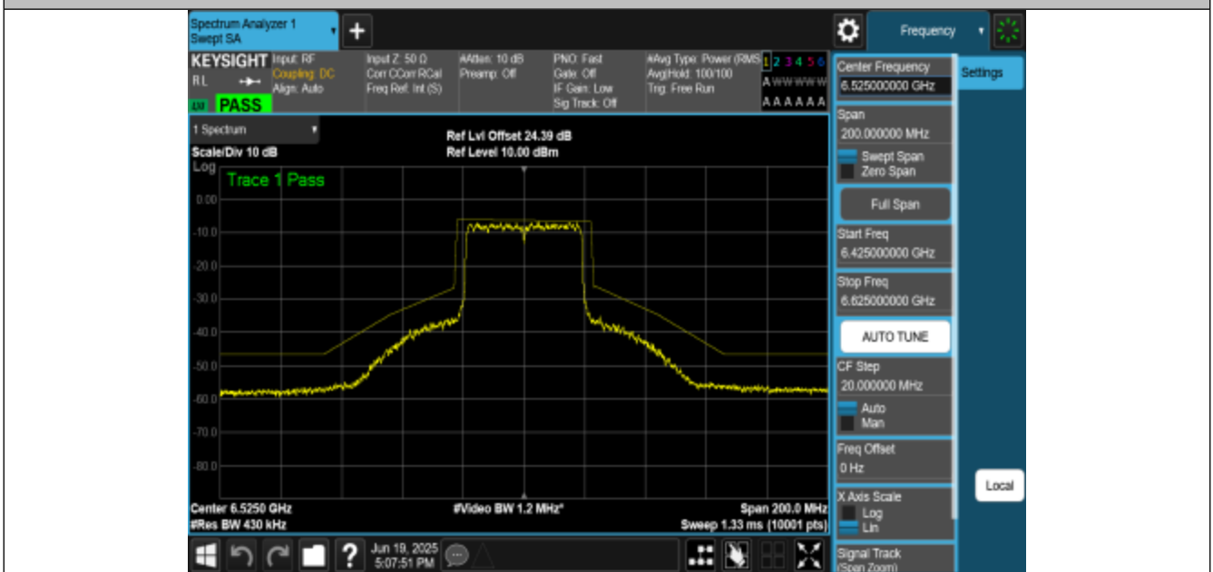
NTNV-11BE40MIMO-Ant0-6525-PASS
