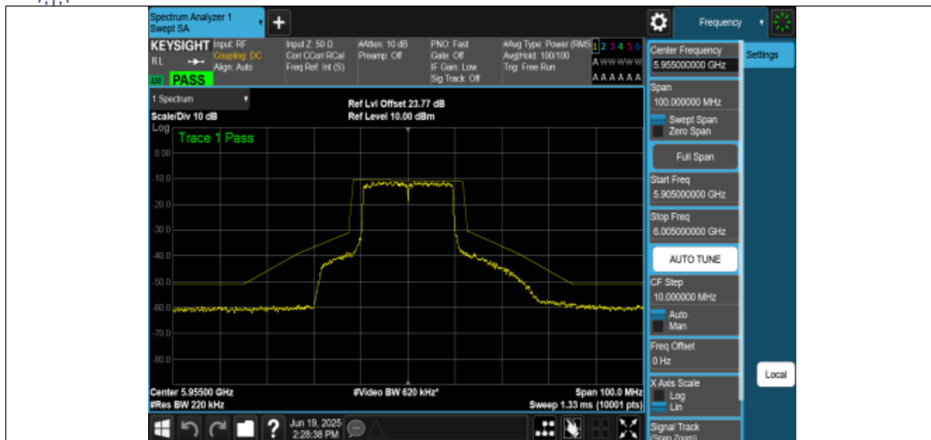
NTNV-11BE20MIMO-Ant2-5955-PASS
