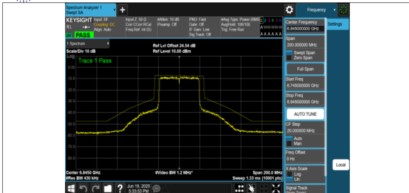
NTNV-11BE40MIMO-Ant1-6845-PASS
