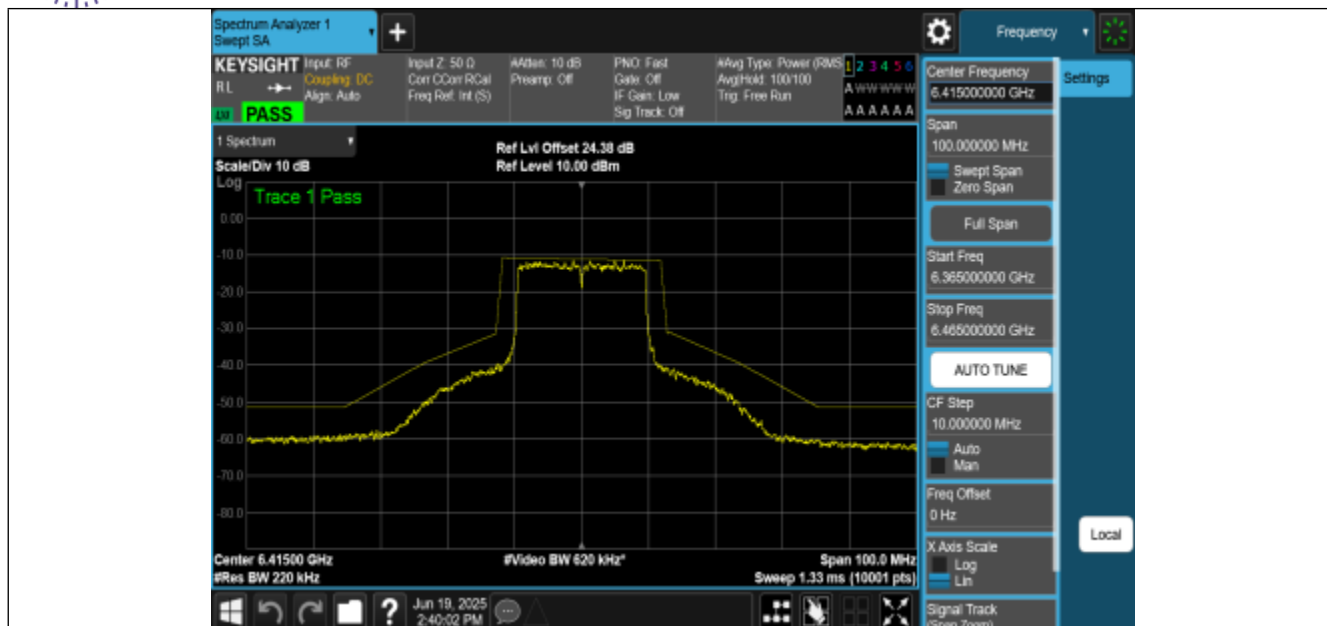
NTNV-11BE20MIMO-Ant2-6415-PASS
