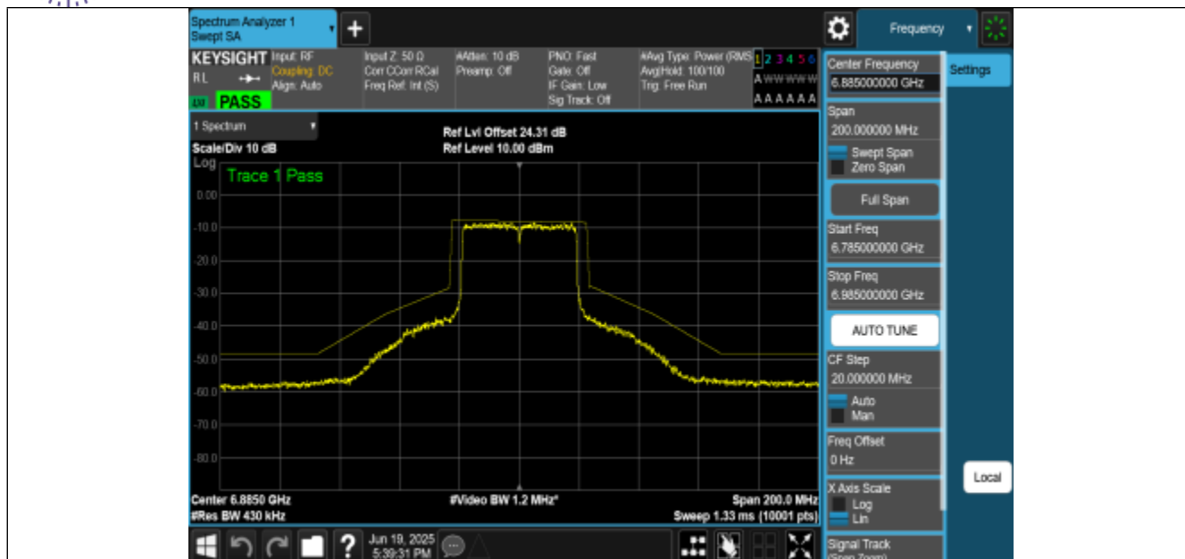
NTNV-11BE40MIMO-Ant1-6885-PASS
