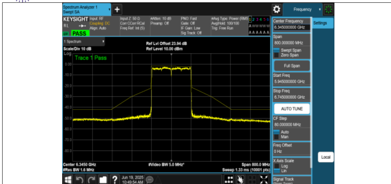
NTNV-11AX160MIMO-Ant0-6345-PASS
