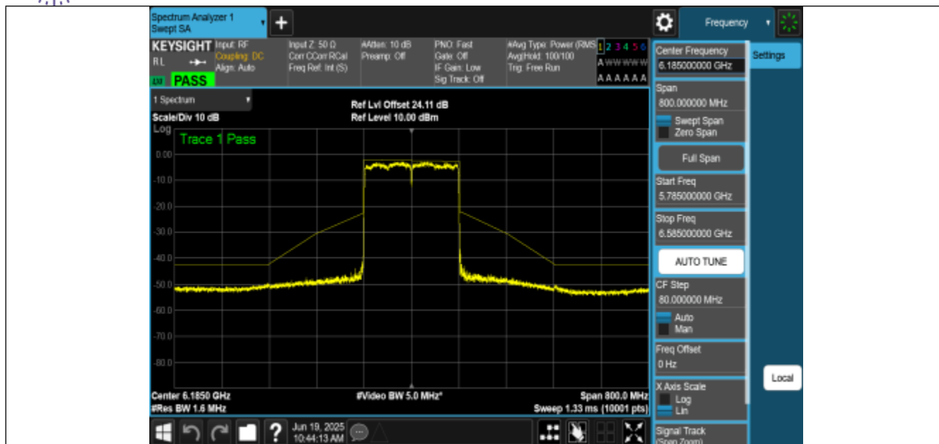
NTNV-11AX160MIMO-Ant0-6185-PASS
