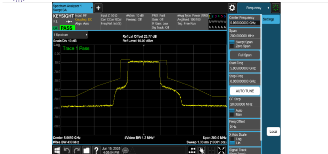
NTNV-11BE40MIMO-Ant2-5965-PASS
