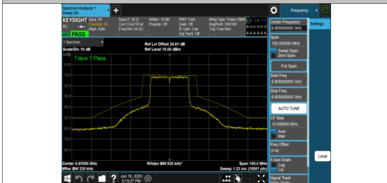
NTNV-11BE20MIMO-Ant3-6855-PASS
