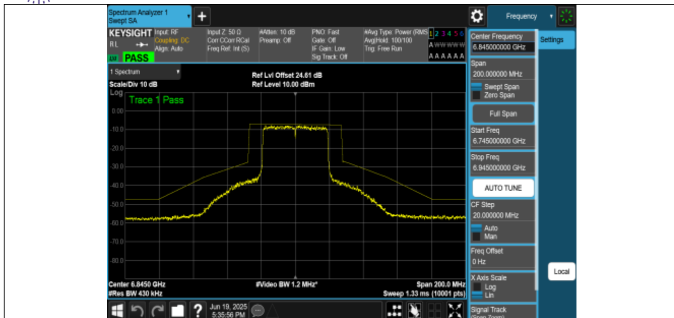
NTNV-11BE40MIMO-Ant3-6845-PASS
