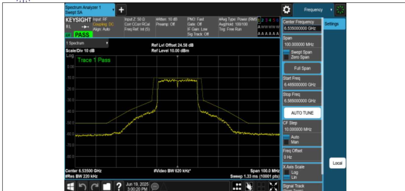
NTNV-11BE20MIMO-Ant2-6535-PASS
