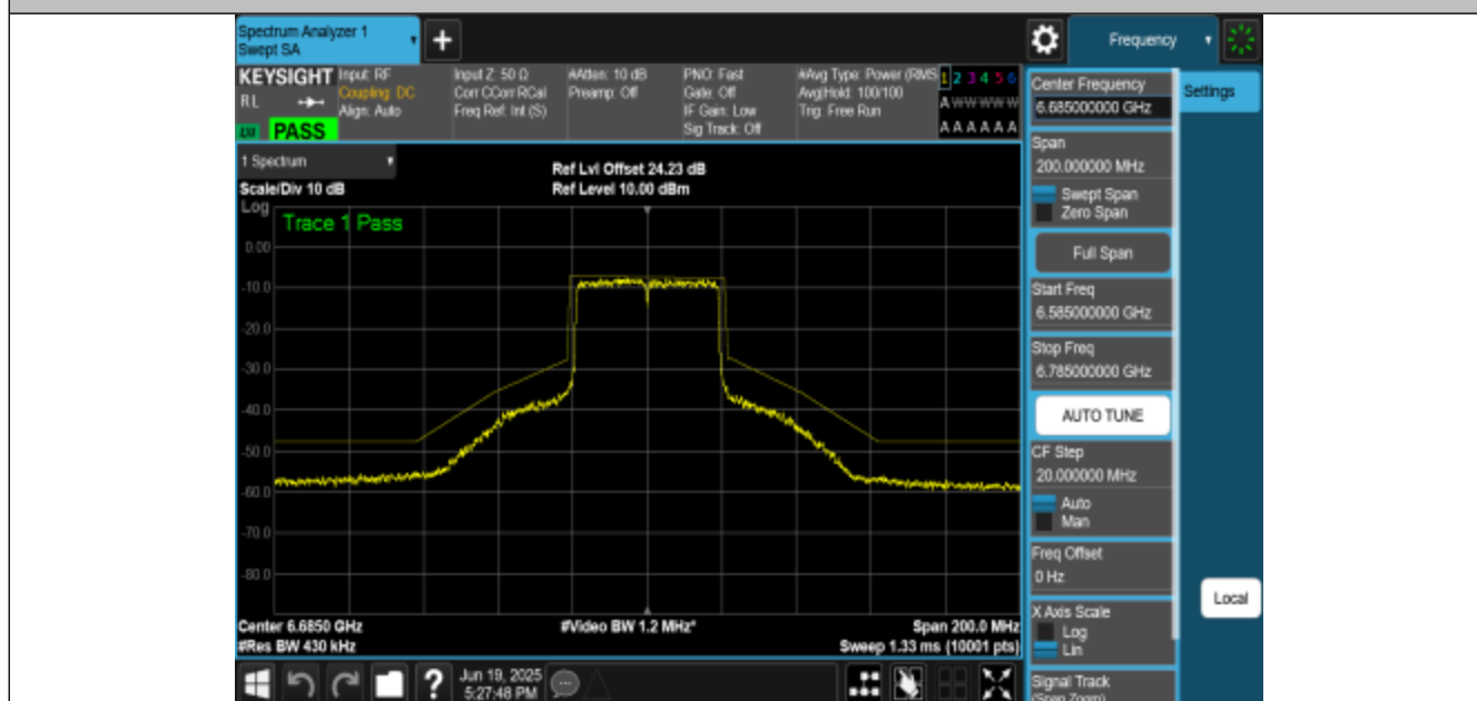
NTNV-11BE40MIMO-Ant2-6685-PASS
