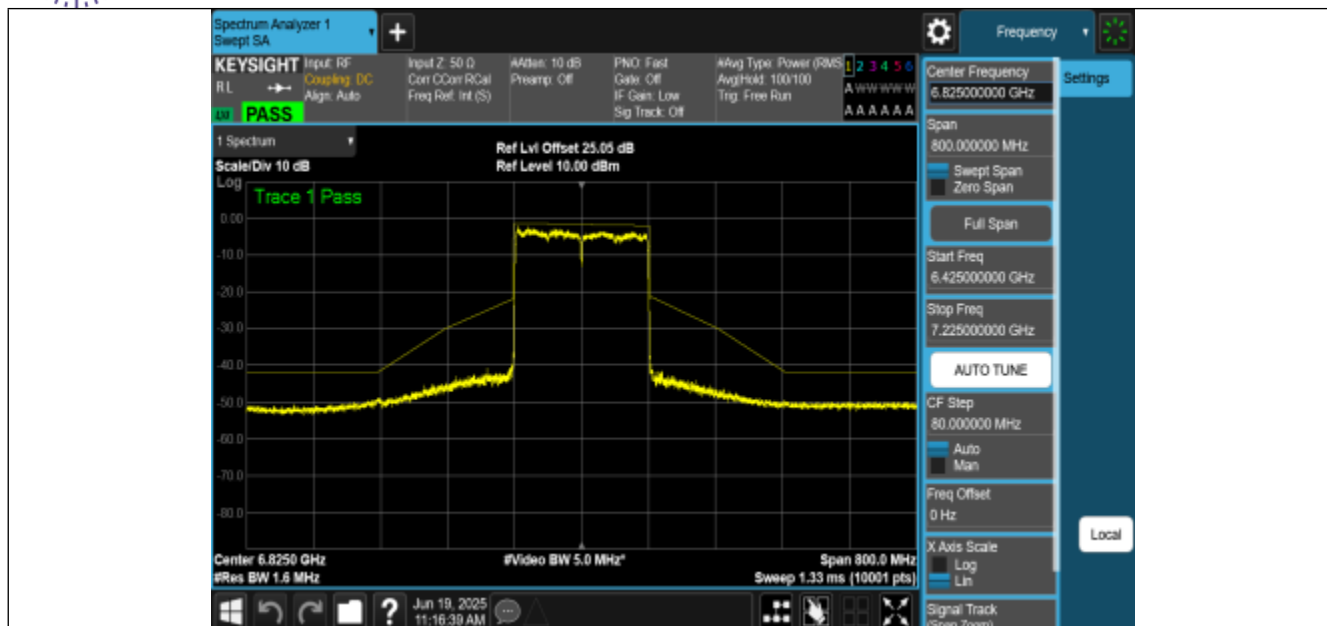
NTNV-11AX160MIMO-Ant2-6825-PASS
