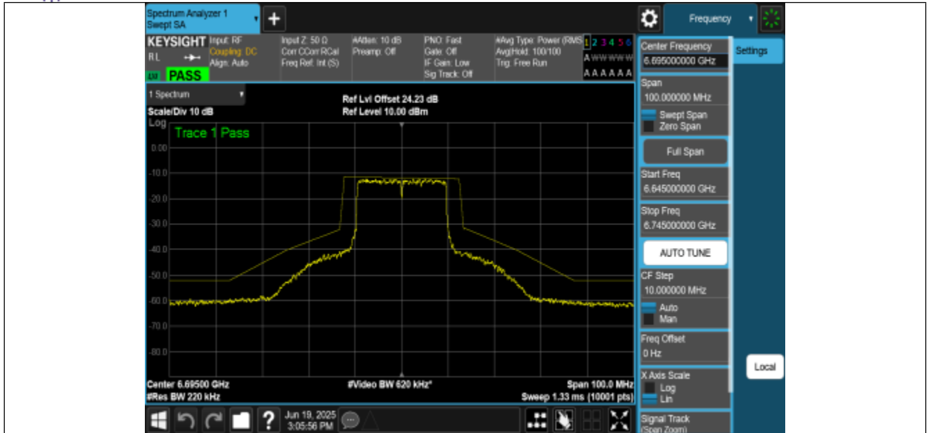
NTNV-11BE20MIMO-Ant2-6695-PASS
