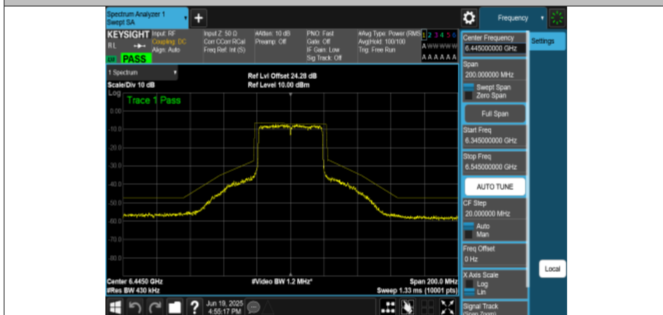
NTNV-11BE40MIMO-Ant2-6445-PASS
