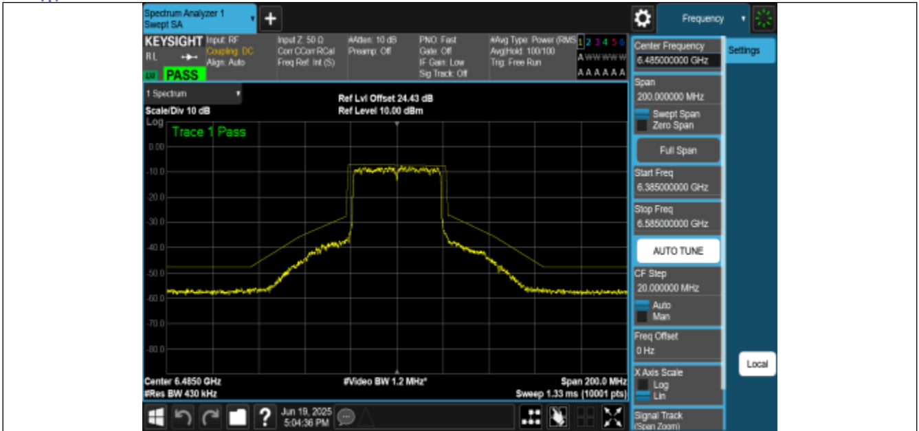
NTNV-11BE40MIMO-Ant3-6485-PASS
