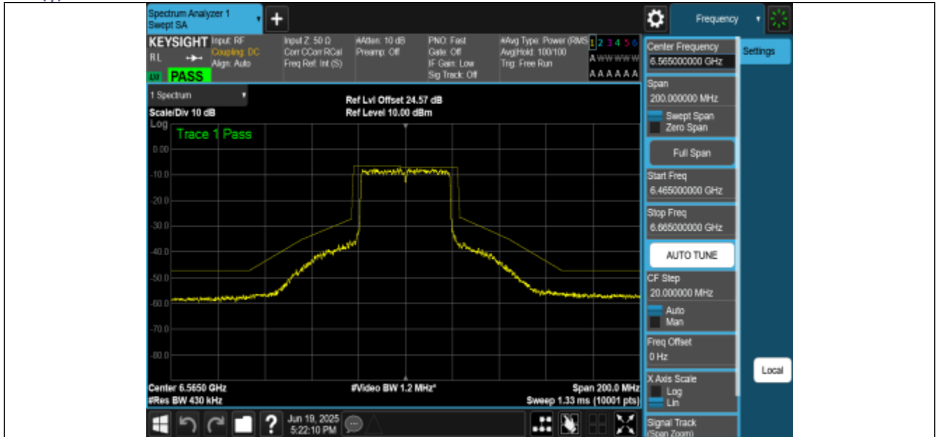
NTNV-11BE40MIMO-Ant3-6565-PASS
