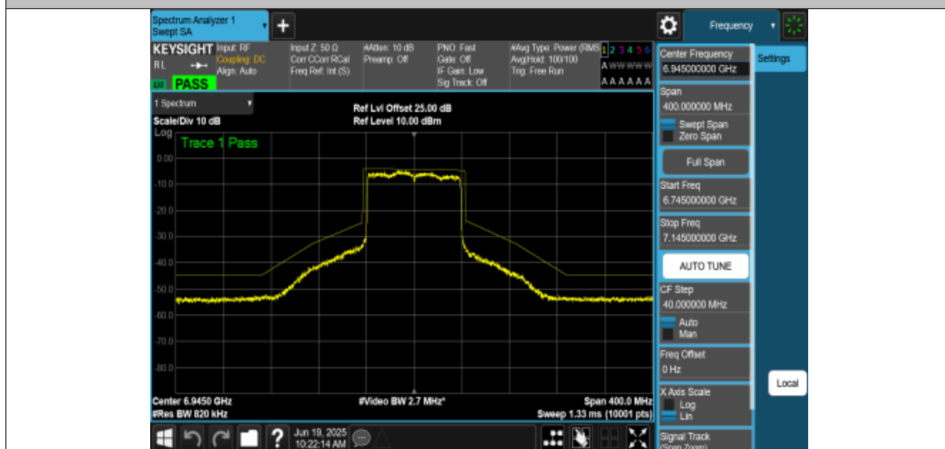
NTNV-11AX80MIMO-Ant3-6945-PASS
