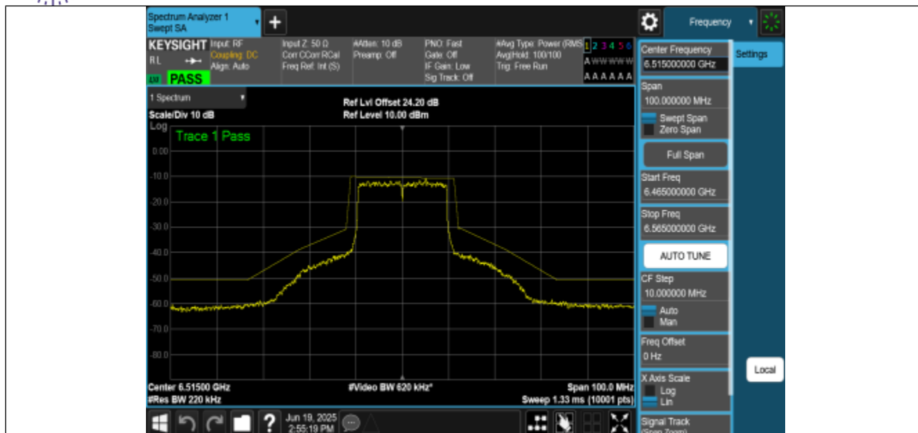
NTNV-11BE20MIMO-Ant2-6515-PASS
