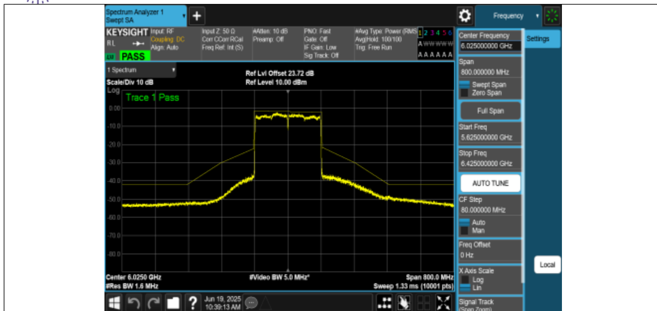
NTNV-11AX160MIMO-Ant2-6025-PASS
