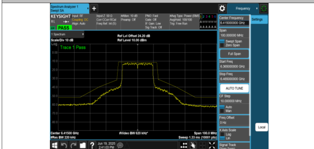
NTNV-11BE20MIMO-Ant3-6415-PASS
