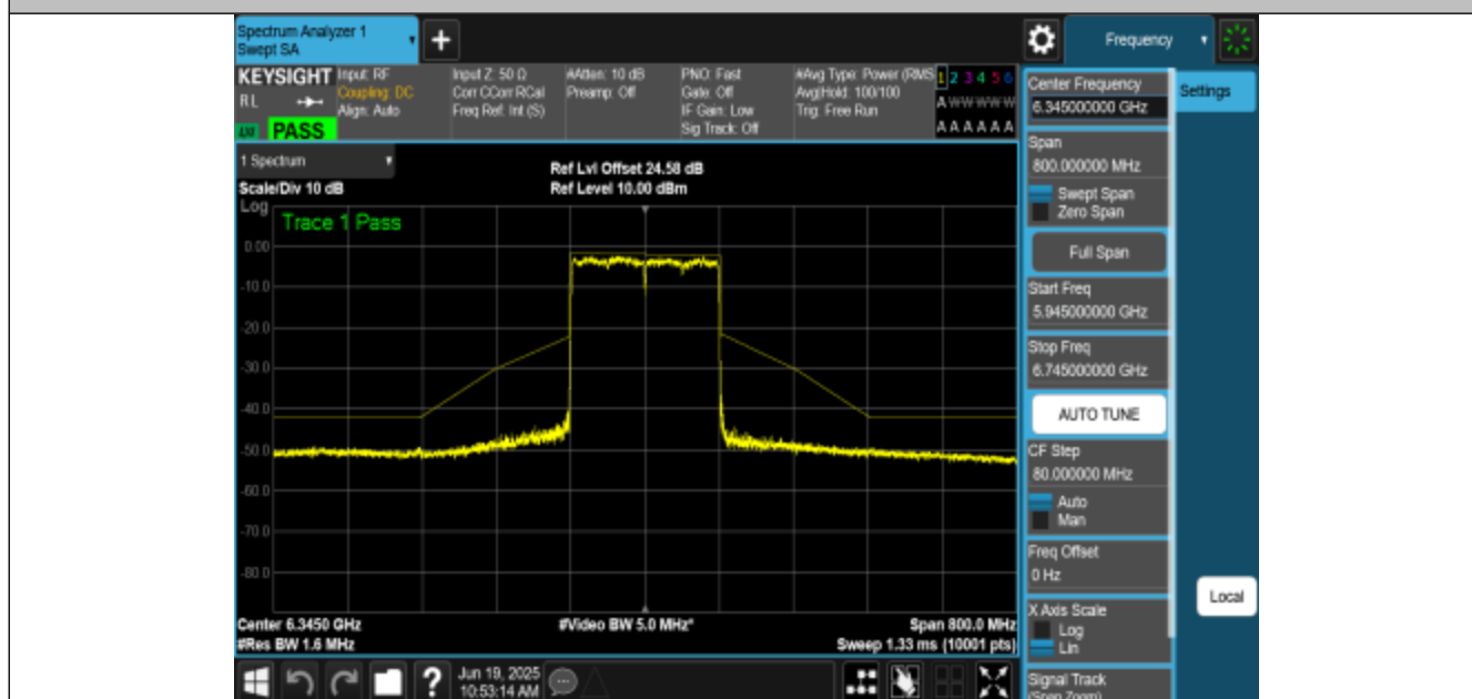
NTNV-11AX160MIMO-Ant3-6345-PASS
