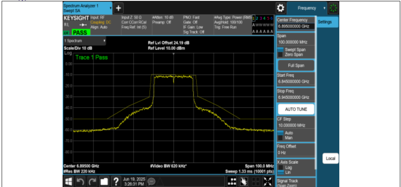
NTNV-11BE20MIMO-Ant0-6895-PASS
