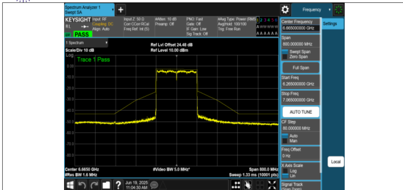
NTNV-11AX160MIMO-Ant2-6665-PASS
