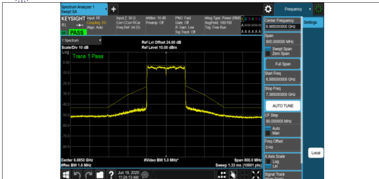
NTNV-11AX160MIMO-Ant2-6985-PASS
