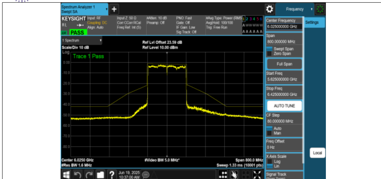
NTNV-11AX160MIMO-Ant0-6025-PASS
