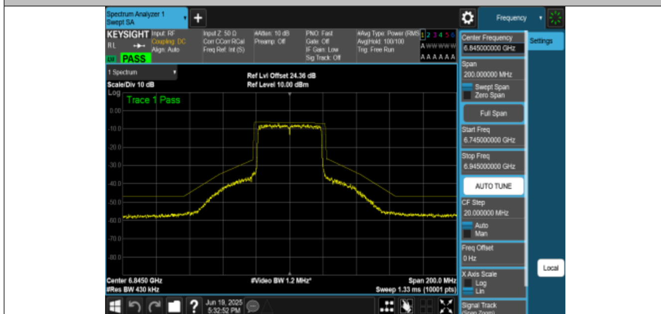
NTNV-11BE40MIMO-Ant0-6845-PASS
