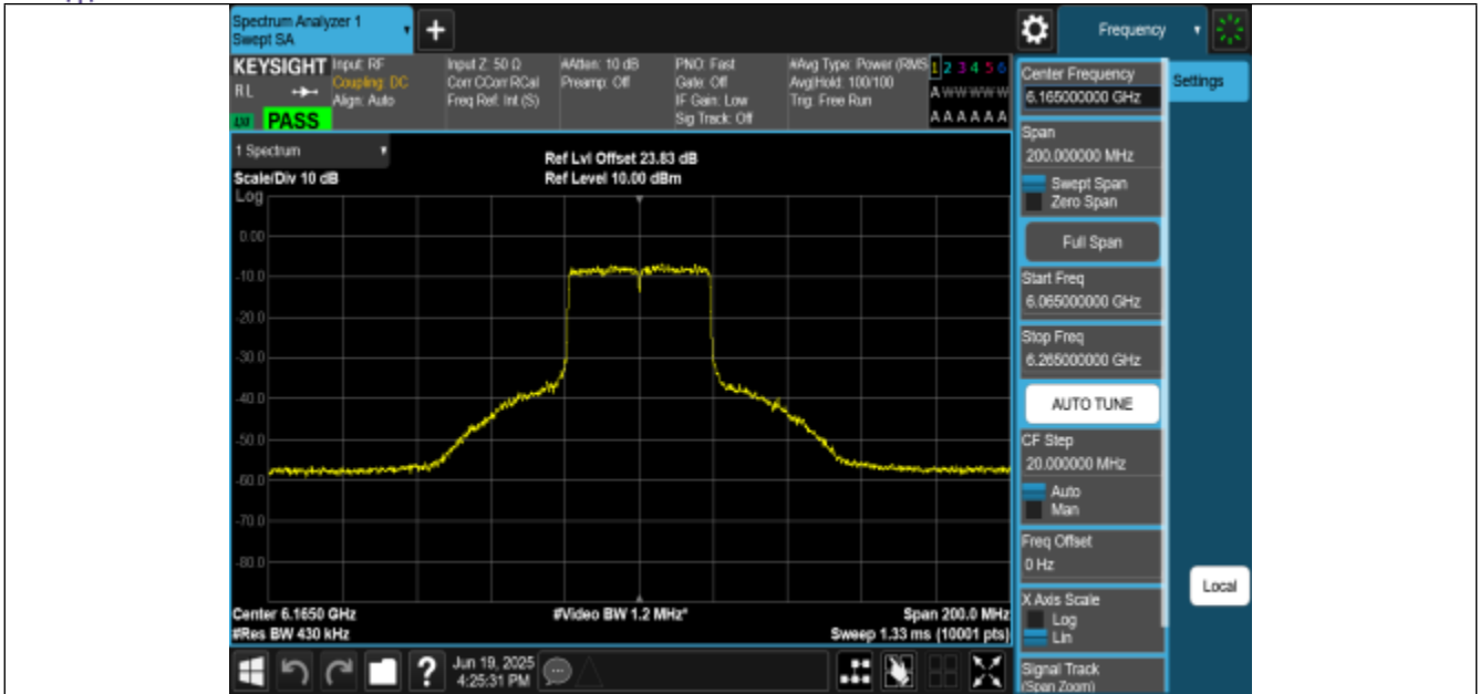
NTNV-11BE40MIMO-Ant0-6165-PASS
