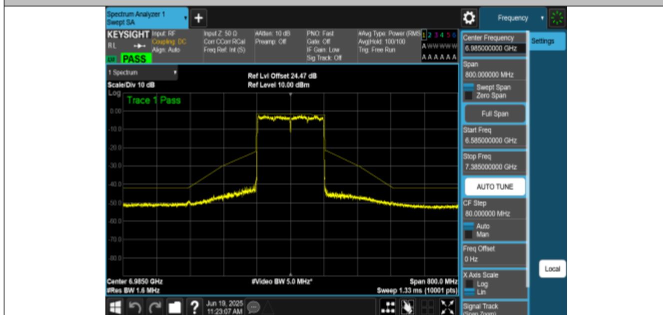
NTNV-11AX160MIMO-Ant1-6985-PASS
