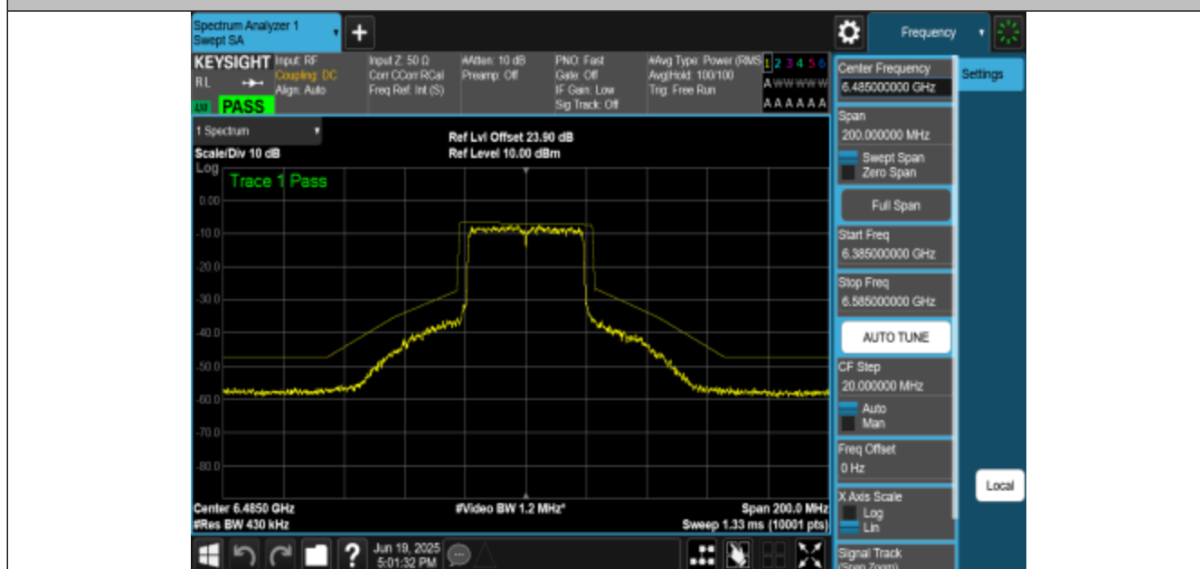
NTNV-11BE40MIMO-Ant0-6485-PASS
