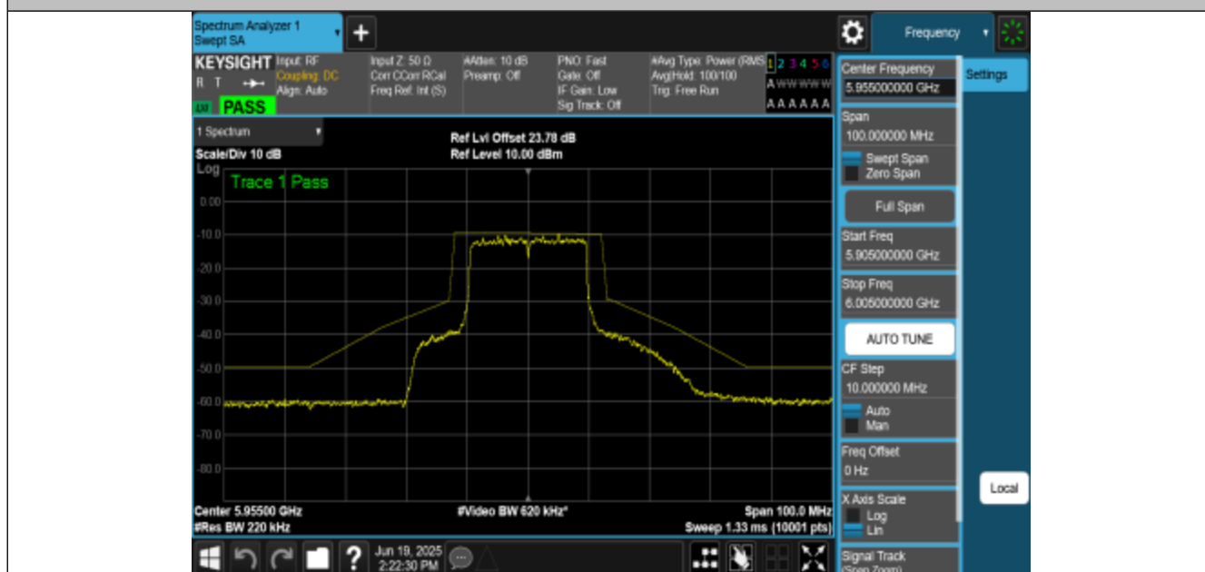
NTNV-11BE20MIMO-Ant1-5955-PASS
