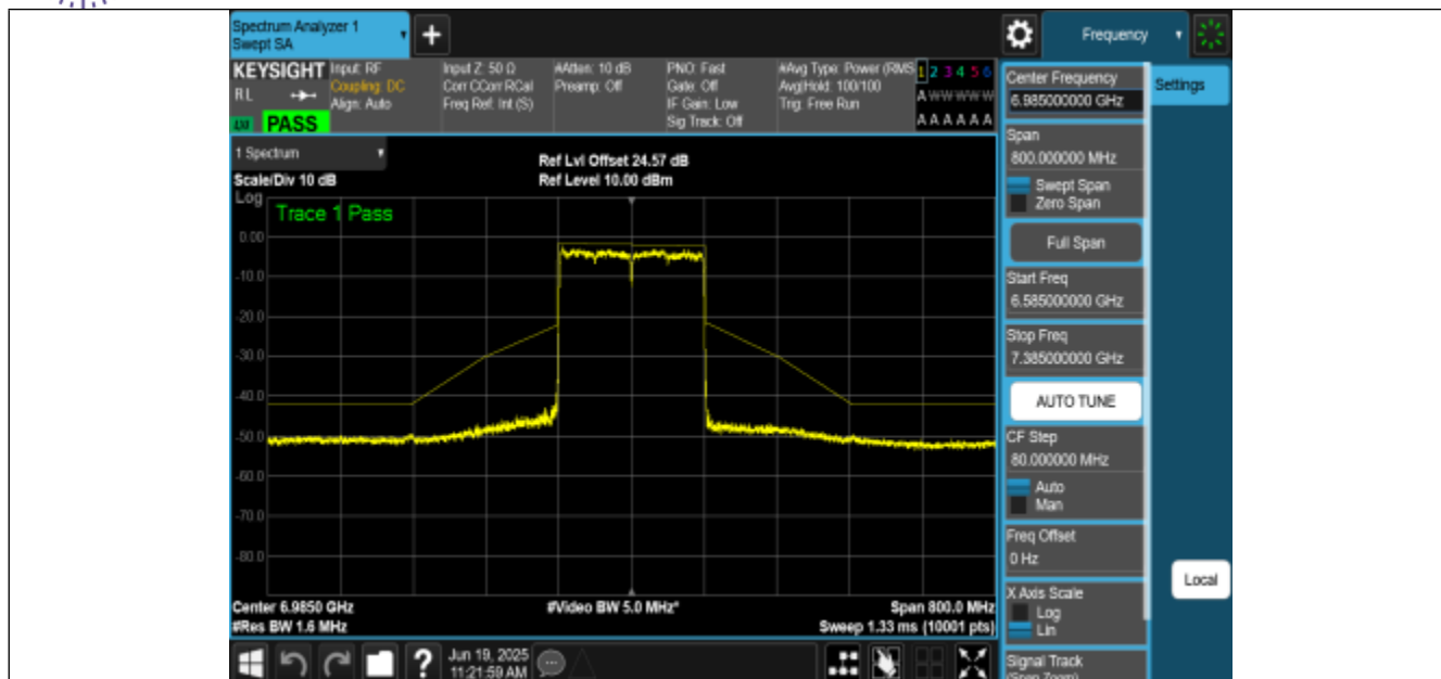
NTNV-11AX160MIMO-Ant0-6985-PASS
