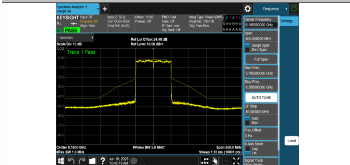
NTNV-11AX160MIMO-Ant1-6185-PASS
