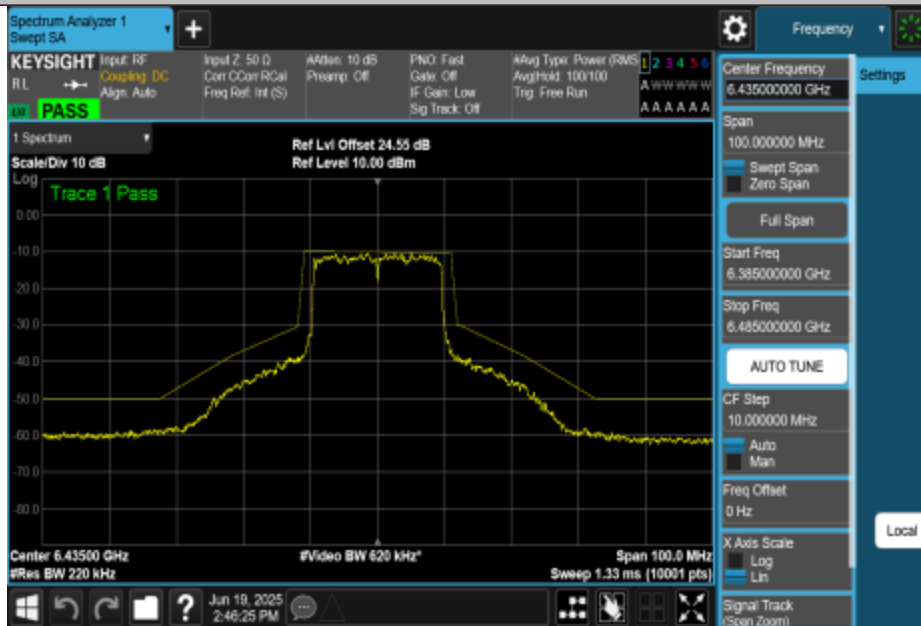
NTNV-11BE20MIMO-Ant3-6435-PASS
