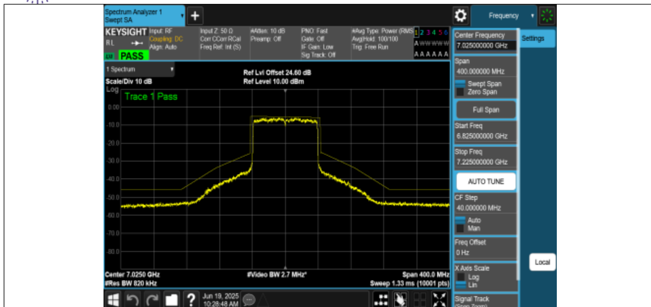
NTN-11AX80MIMO-Ant2-7025-PASS
