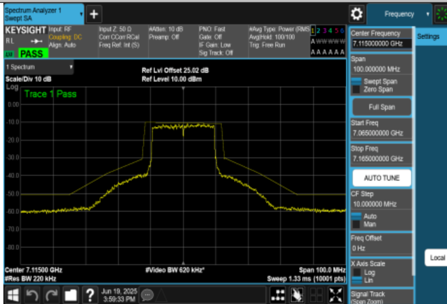
NTNV-11BE20MIMO-Ant3-7115-PASS
