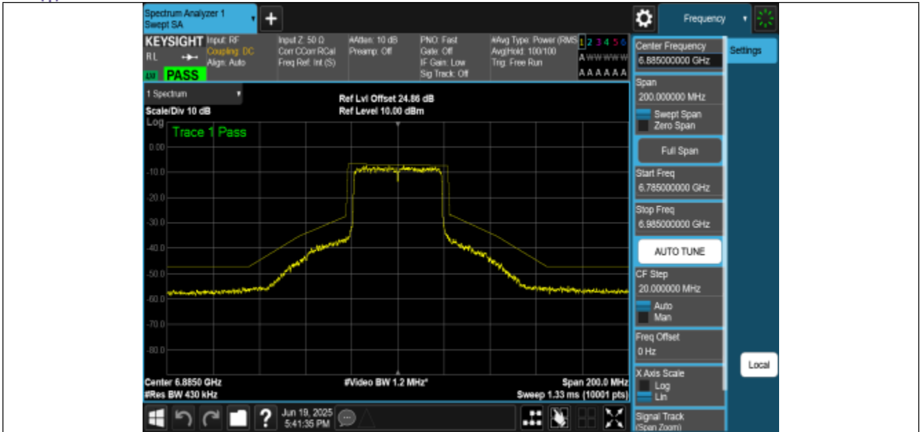
NTNV-11BE40MIMO-Ant3-6885-PASS
