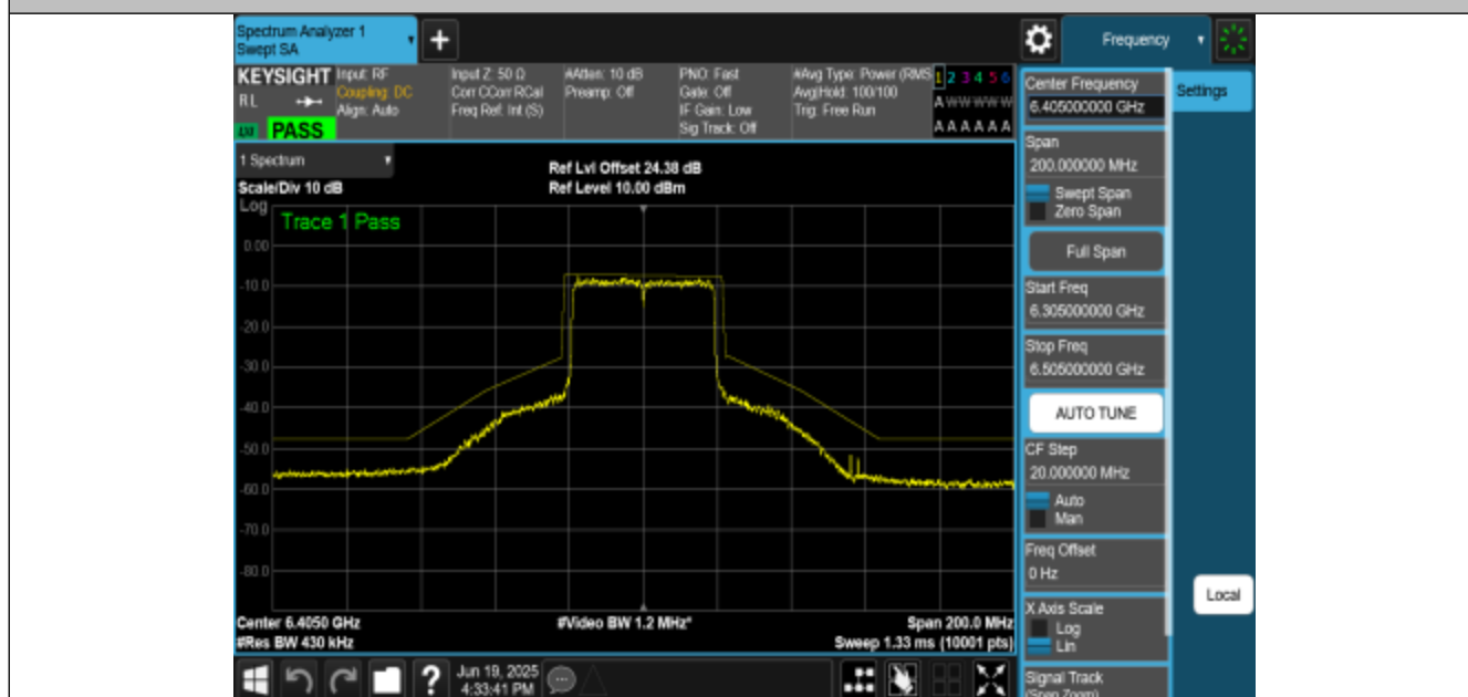
NTNV-11BE40MIMO-Ant2-6405-PASS
