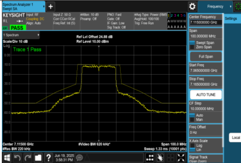
NTNV-11BE20MIMO-Ant2-7115-PASS
