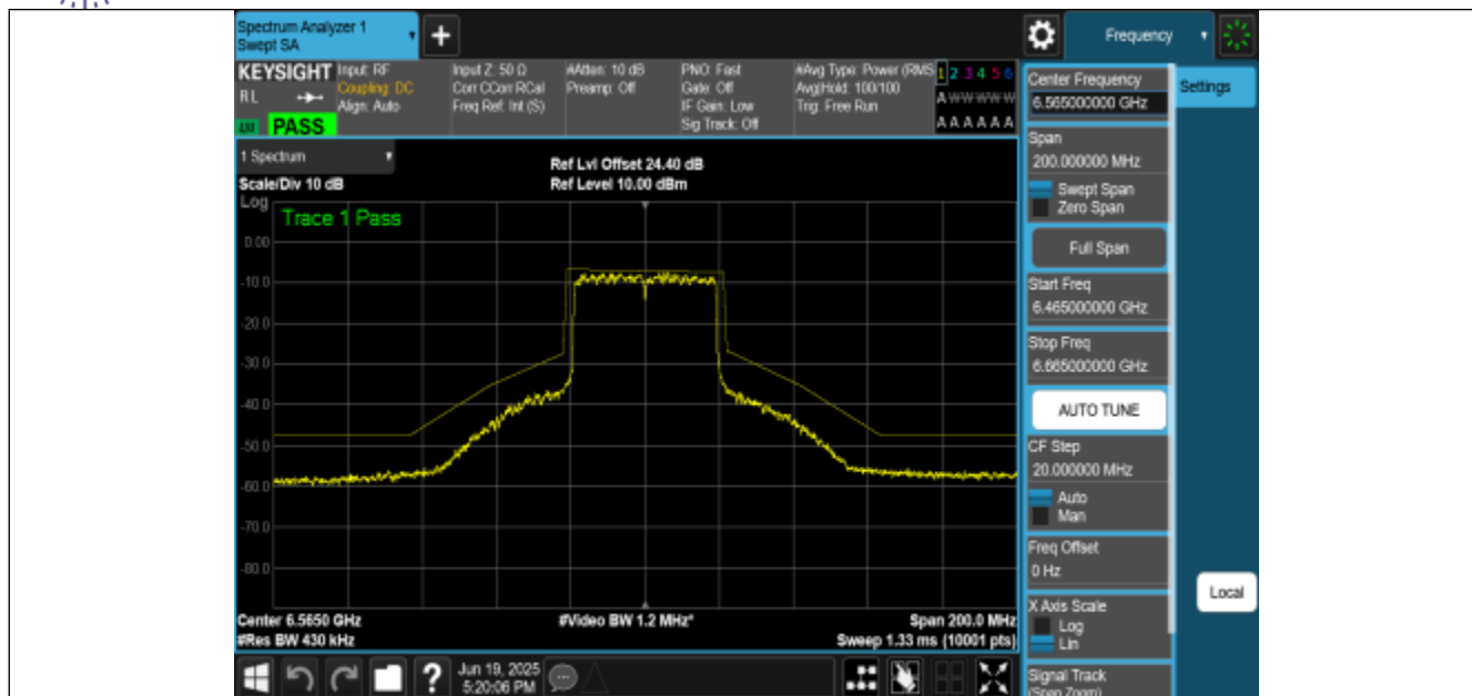
NTNV-11BE40MIMO-Ant1-6565-PASS
