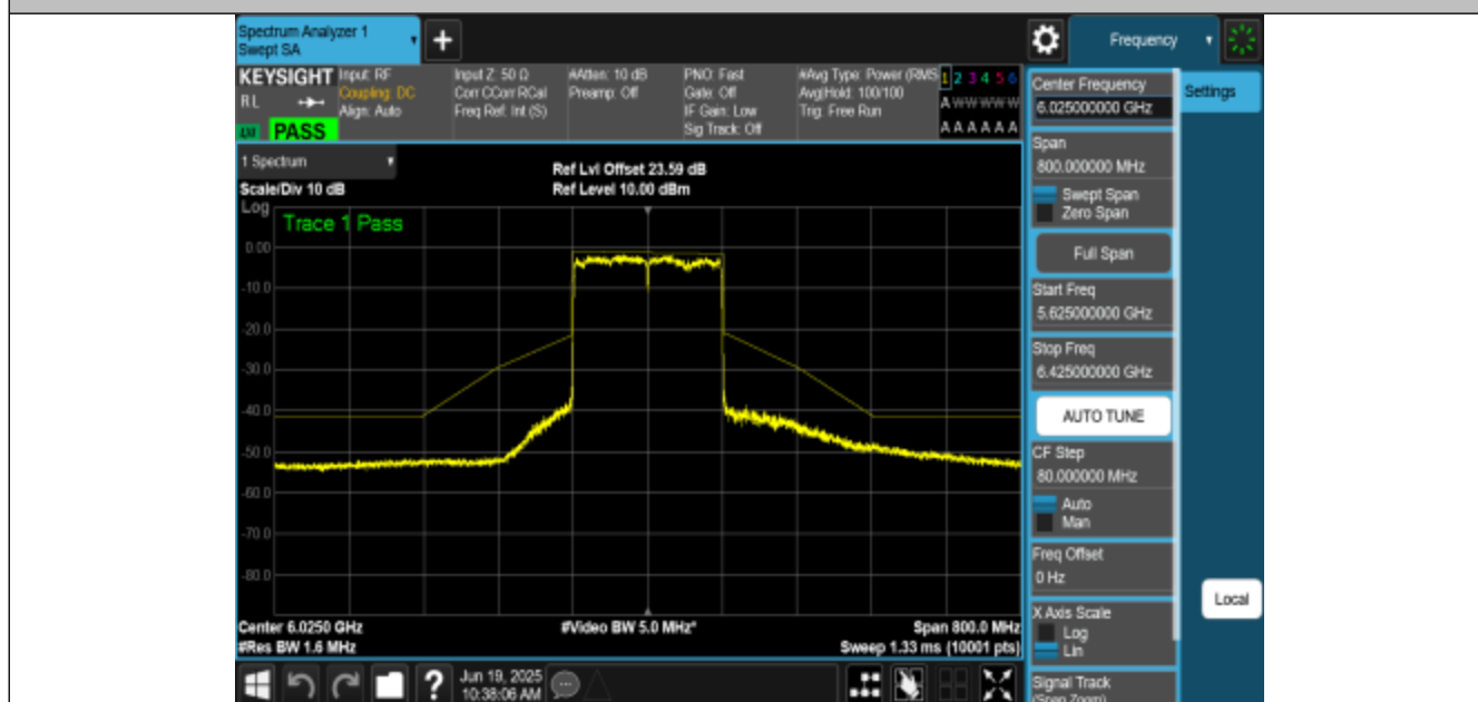
NTNV-11AX160MIMO-Ant1-6025-PASS
