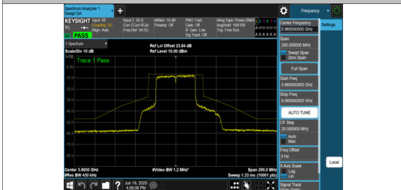
NTNV-11BE40MIMO-Ant3-5965-PASS
