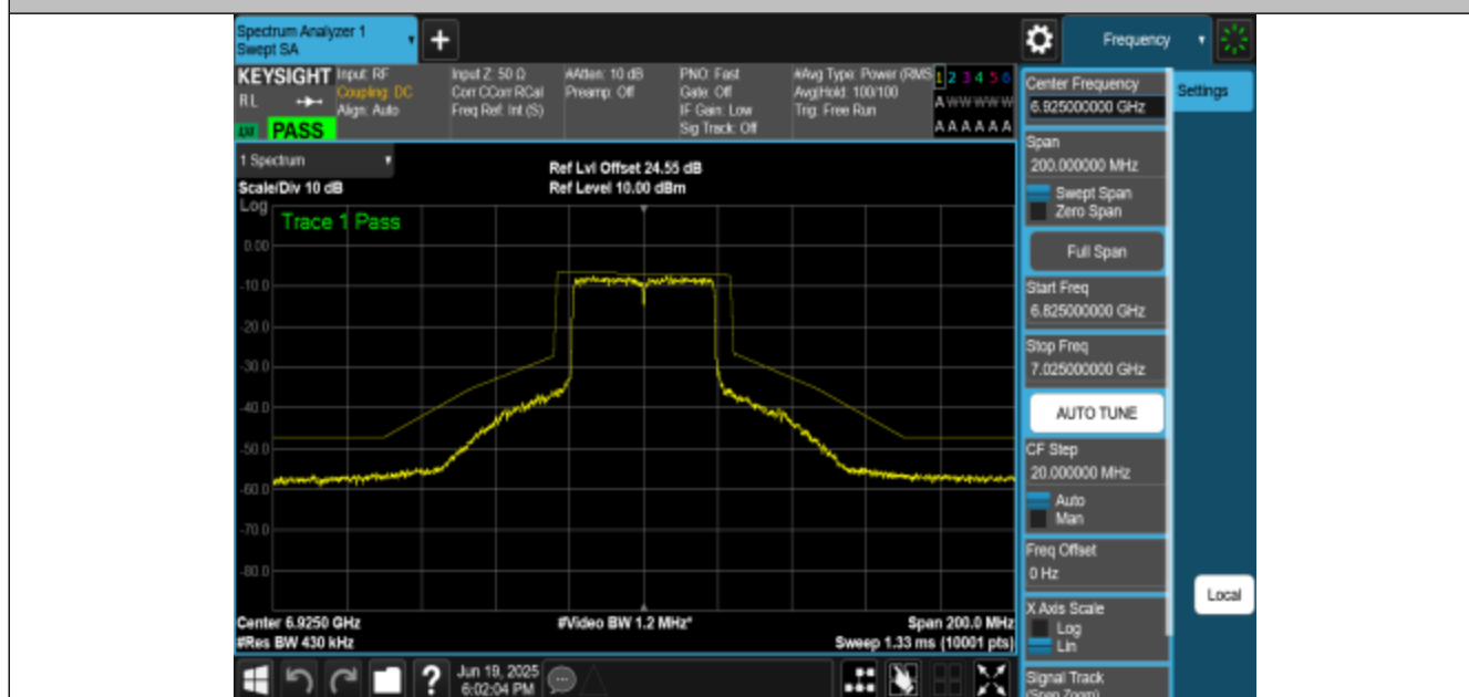
NTNV-11BE40MIMO-Ant2-6925-PASS
