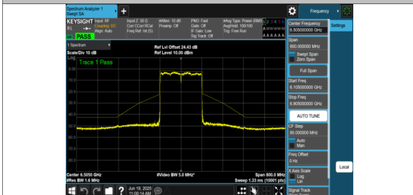
NTNV-11AX160MIMO-Ant3-6505-PASS
