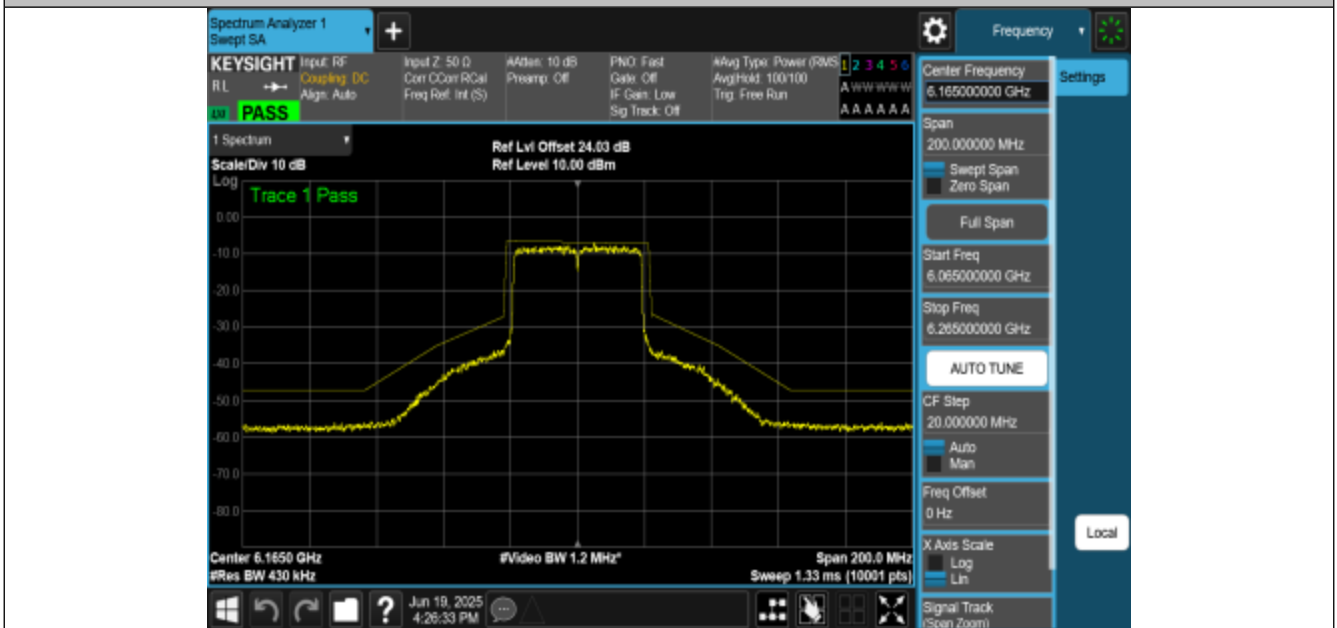
NTNV-11BE40MIMO-Ant1-6165-PASS
