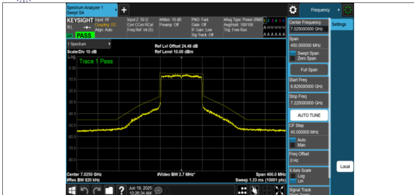
NTNV-11AX80MIMO-Ant0-7025-PASS
