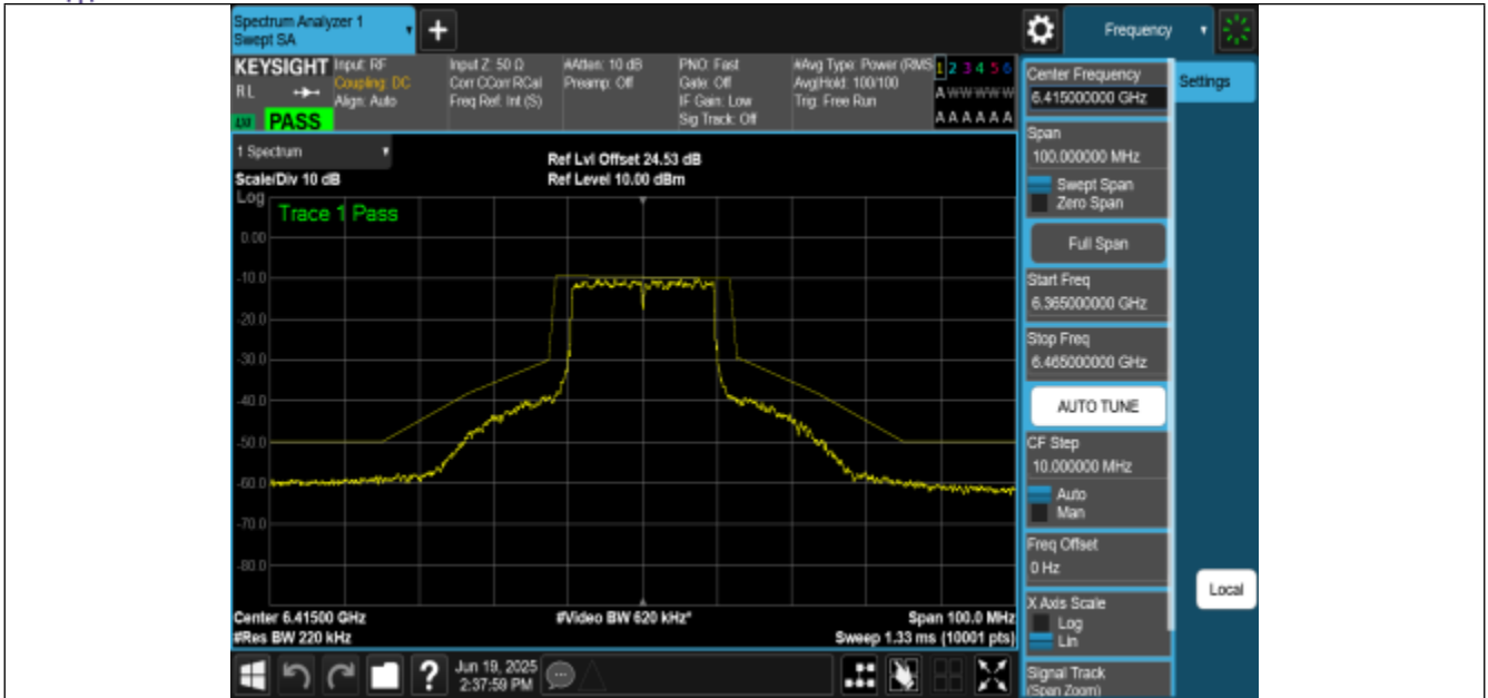
NTNV-11BE20MIMO-Ant0-6415-PASS
