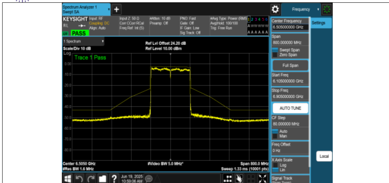
NTNV-11AX160MIMO-Ant2-6505-PASS
