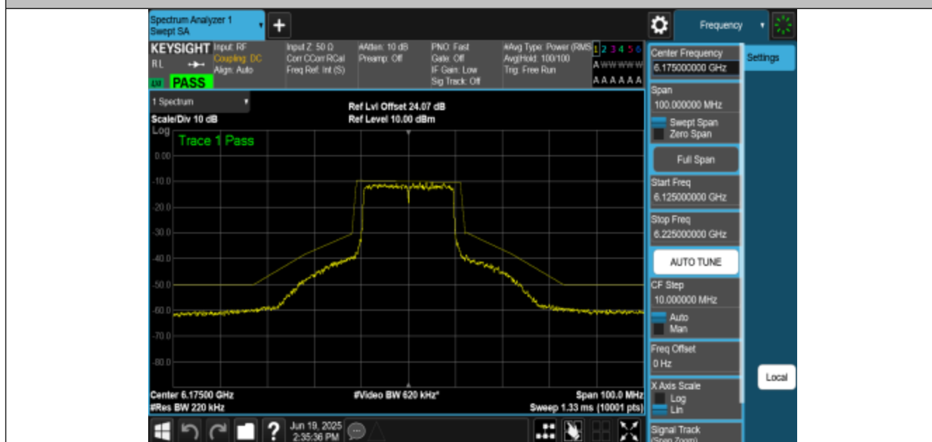
NTNV-11BE20MIMO-Ant3-6175-PASS
