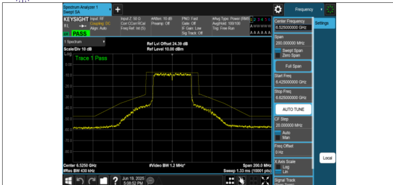
NTNV-11BE40MIMO-Ant1-6525-PASS
