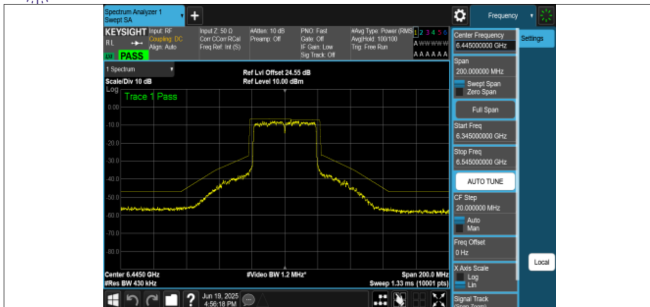
NTNV-11BE40MIMO-Ant3-6445-PASS
