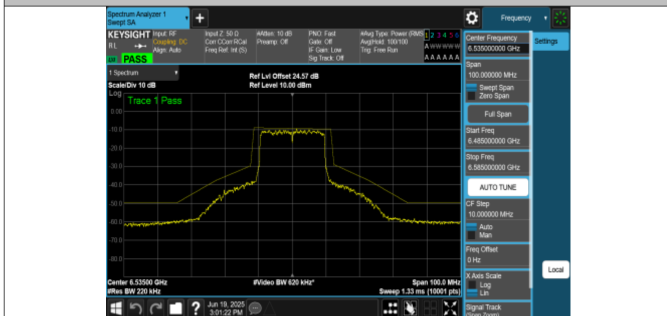
NTNV-11BE20MIMO-Ant3-6535-PASS
