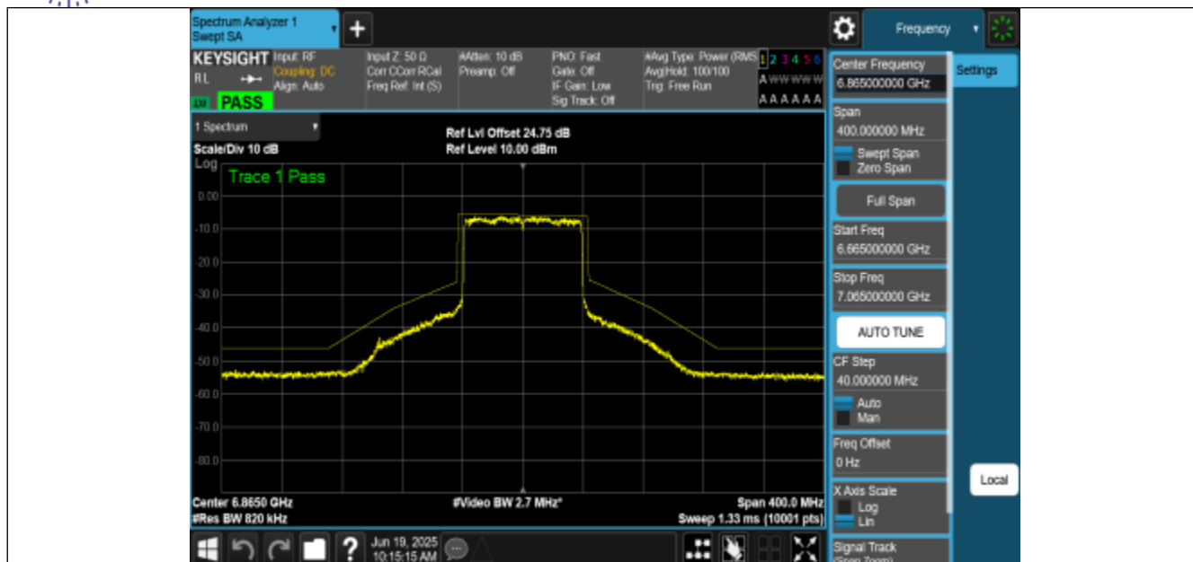
NTNV-11AX80MIMO-Ant2-6865-PASS
