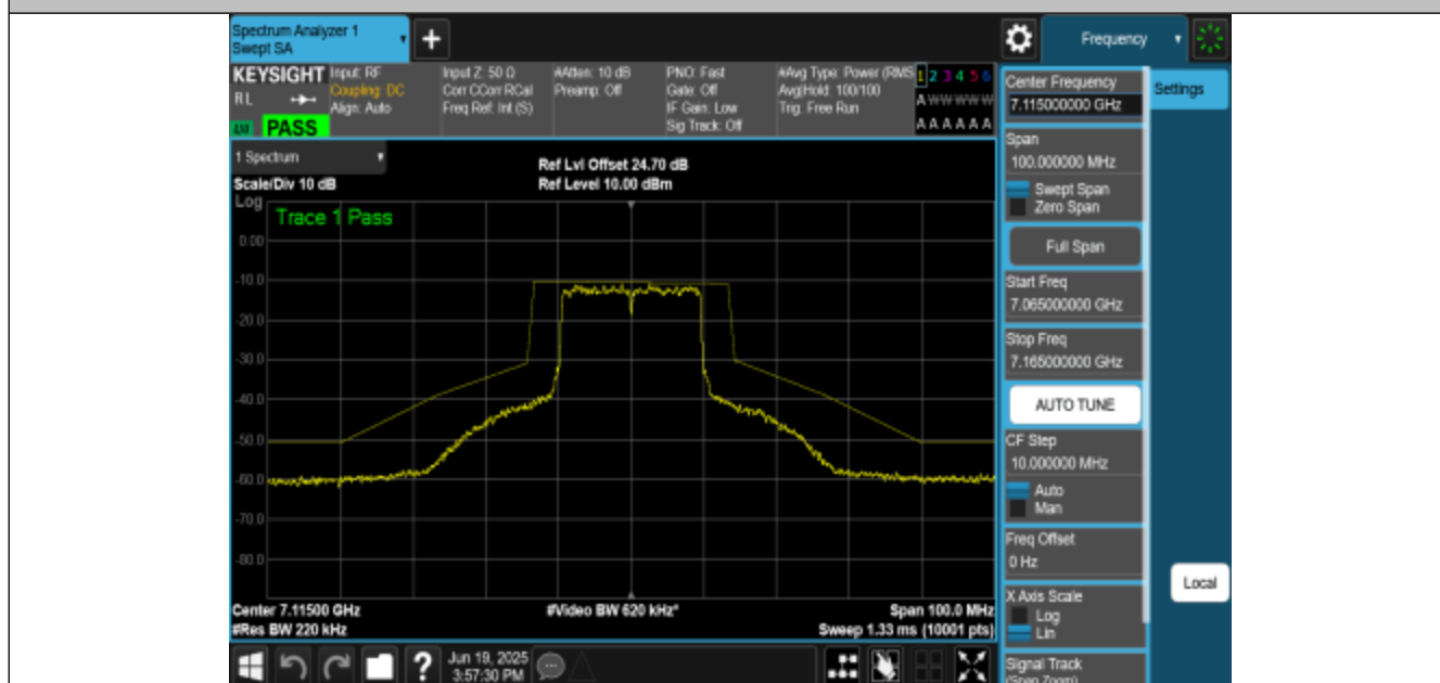
NTNV-11BE20MIMO-Ant1-7115-PASS
