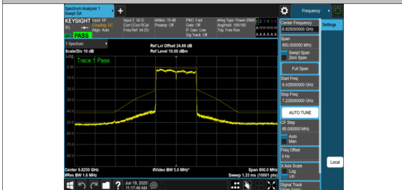
NTNV-11AX160MIMO-Ant3-6825-PASS
