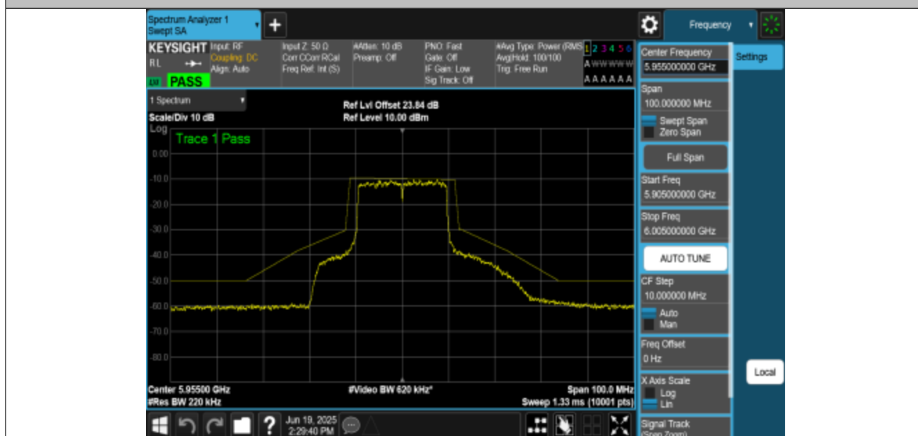
NTNV-11BE20MIMO-Ant3-5955-PASS
