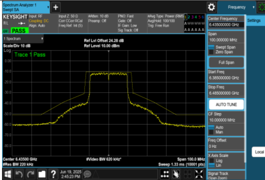
NTNV-11BE20MIMO-Ant2-6435-PASS
