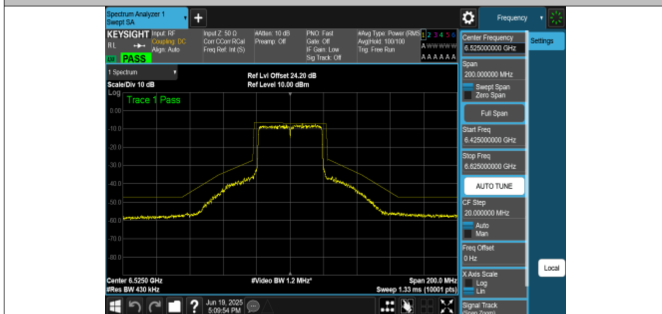
NTNV-11BE40MIMO-Ant2-6525-PASS
