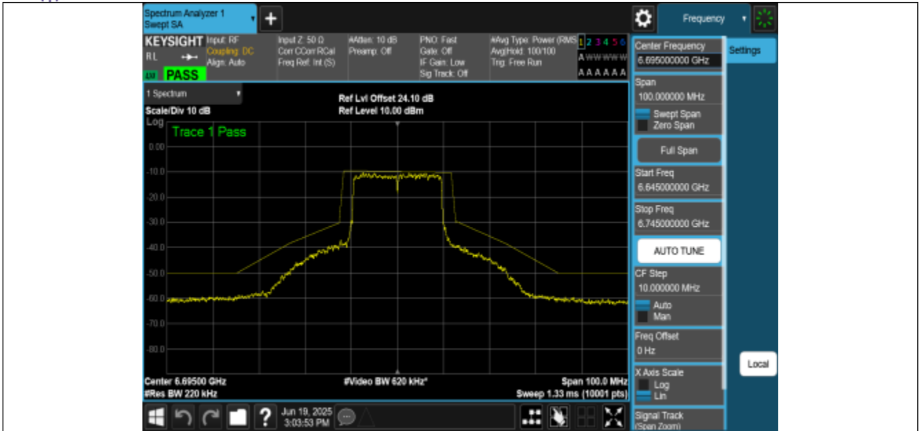
NTNV-11BE20MIMO-Ant0-6695-PASS
