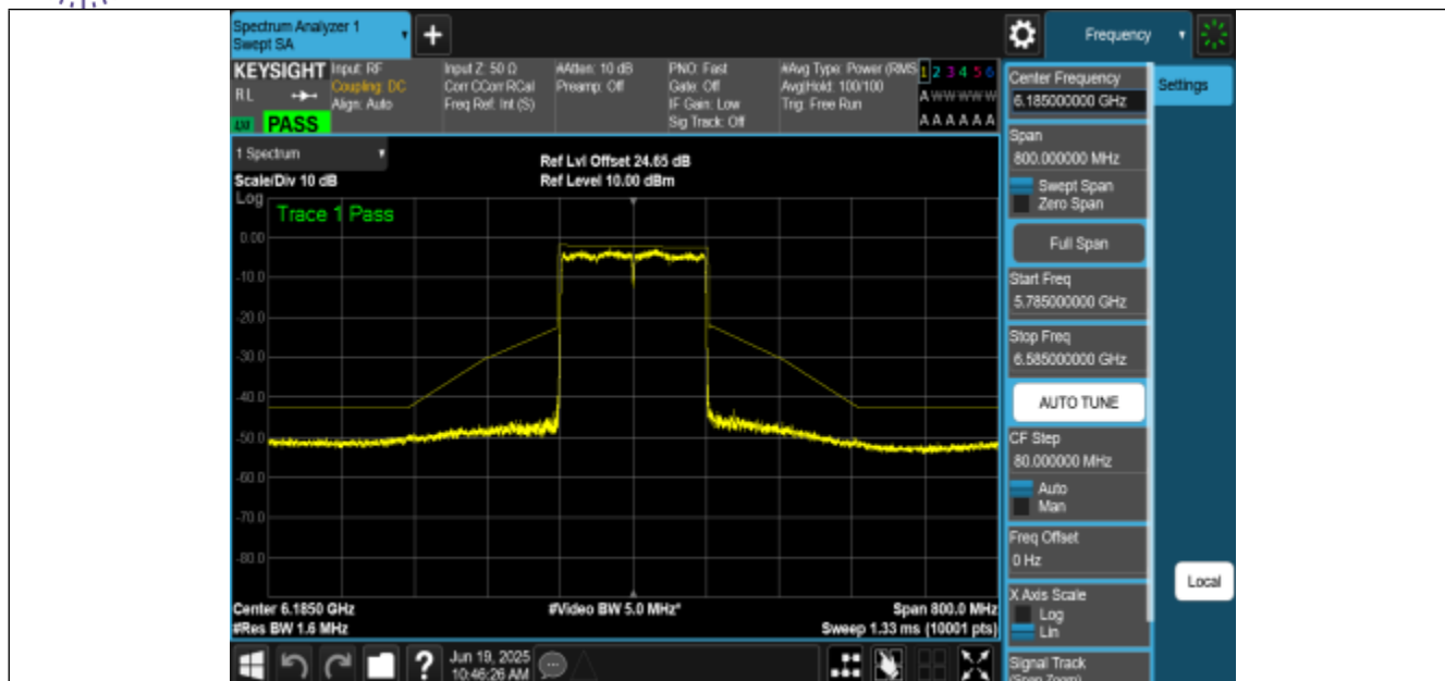
NTNV-11AX160MIMO-Ant2-6185-PASS
