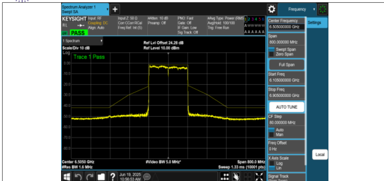
NTNV-11AX160MIMO-Ant0-6505-PASS
