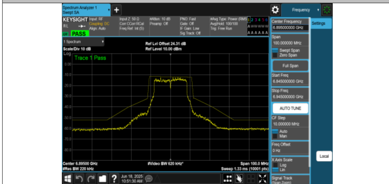
NTNV-11A-CDD-Ant1-6895-PASS
