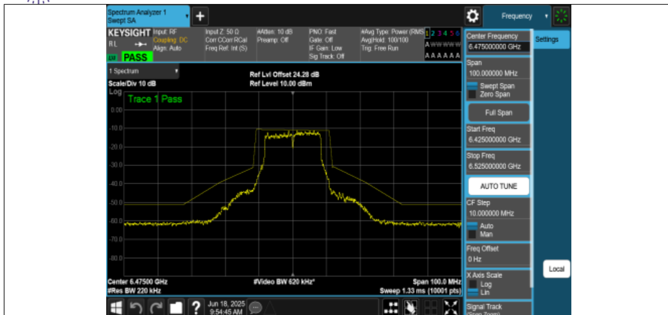
NTNV-11A-CDD-Ant2-6475-PASS
