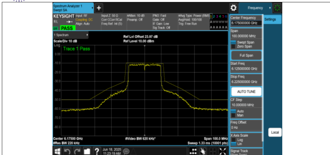
NTNV-11AX20MIMO-Ant0-6175-PASS
