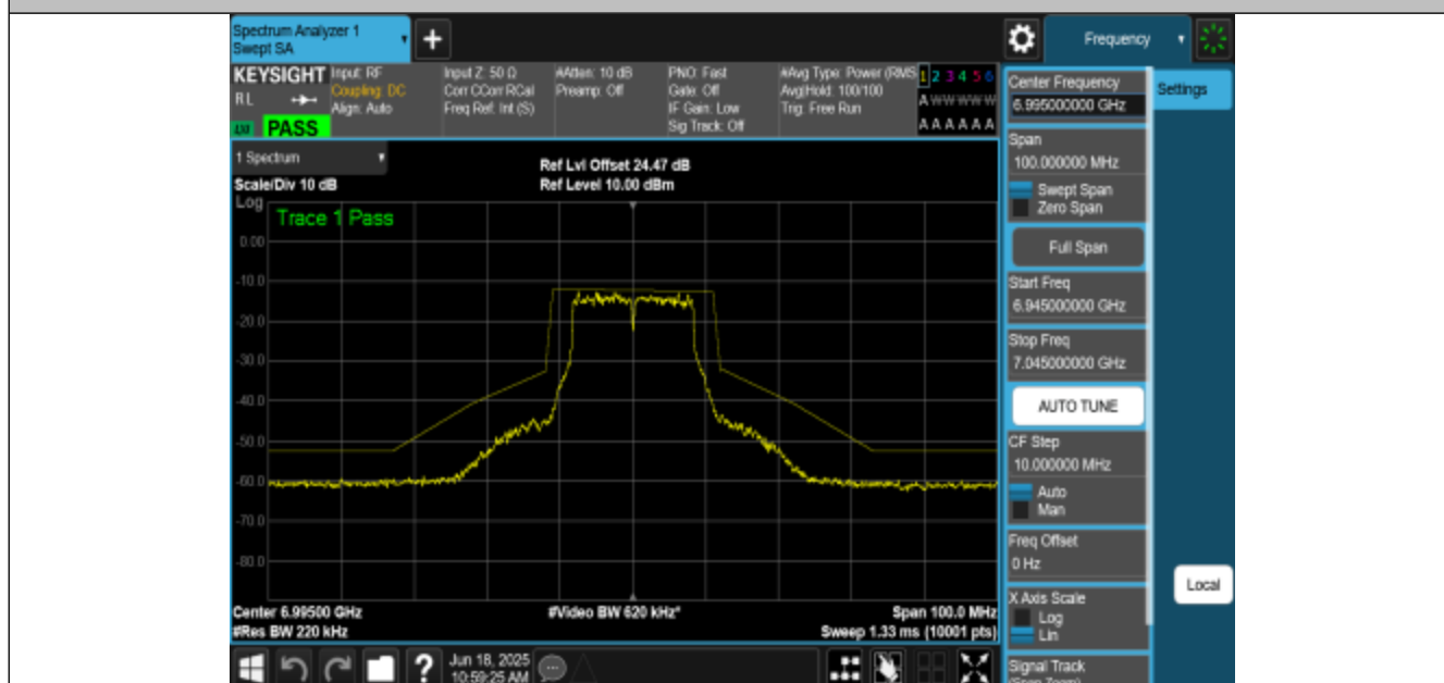
NTNV-11A-CDD-Ant1-6995-PASS
