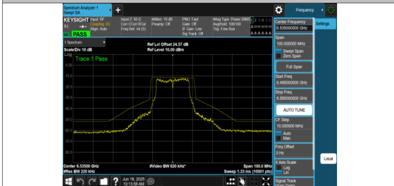
NTNV-11A-CDD-Ant3-6535-PASS
