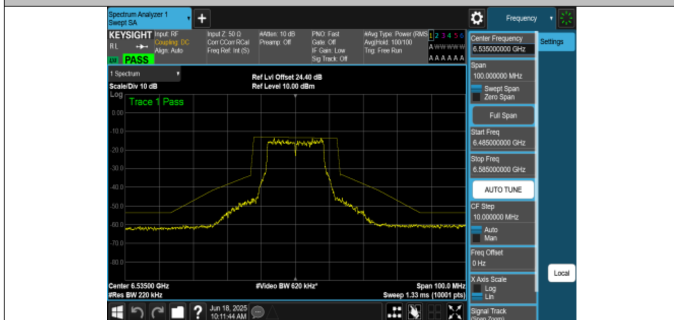
NTNV-11A-CDD-Ant1-6535-PASS
