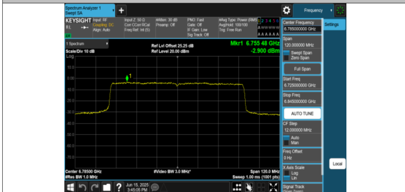
11BE80MIMO-Ant3-6785-PASS
