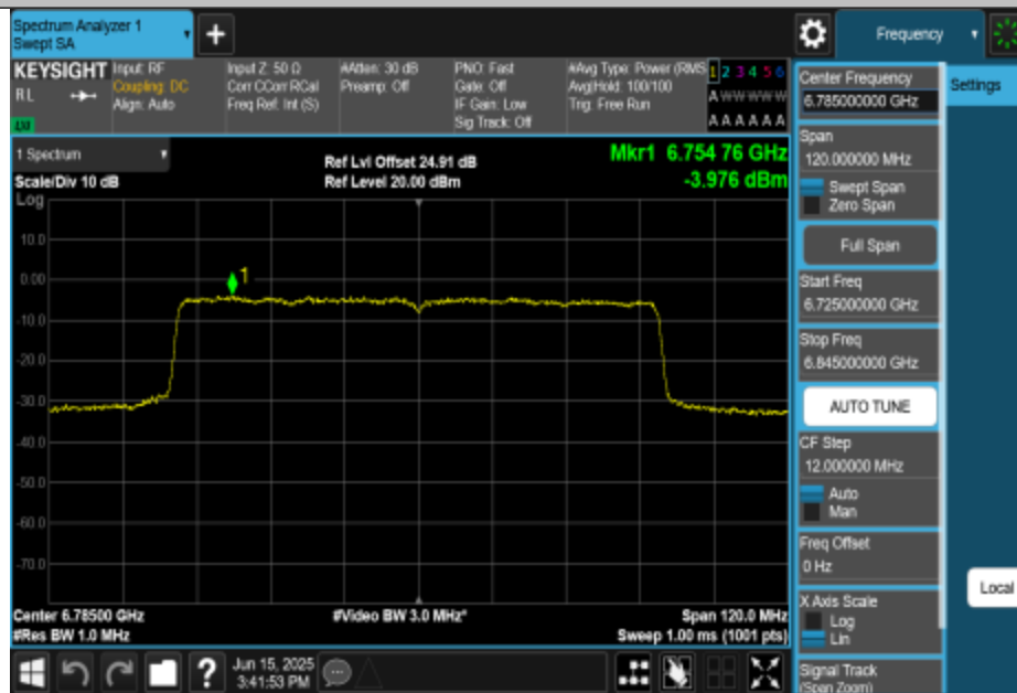
11BE80MIMO-Ant1-6785-PASS
