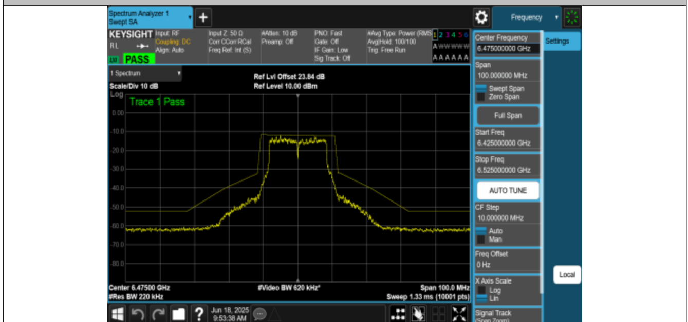
NTNV-11A-CDD-Ant1-6475-PASS
