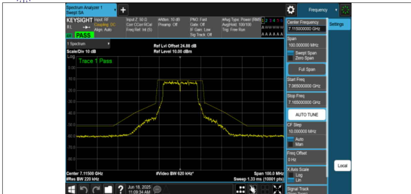
NTNV-11A-CDD-Ant2-7115-PASS
