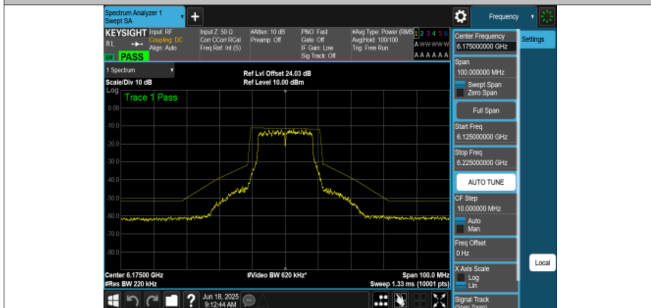
NTNV-11A-CDD-Ant1-6175-PASS
