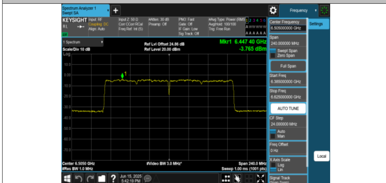
11BE160MIMO-Ant3-6505-PASS
