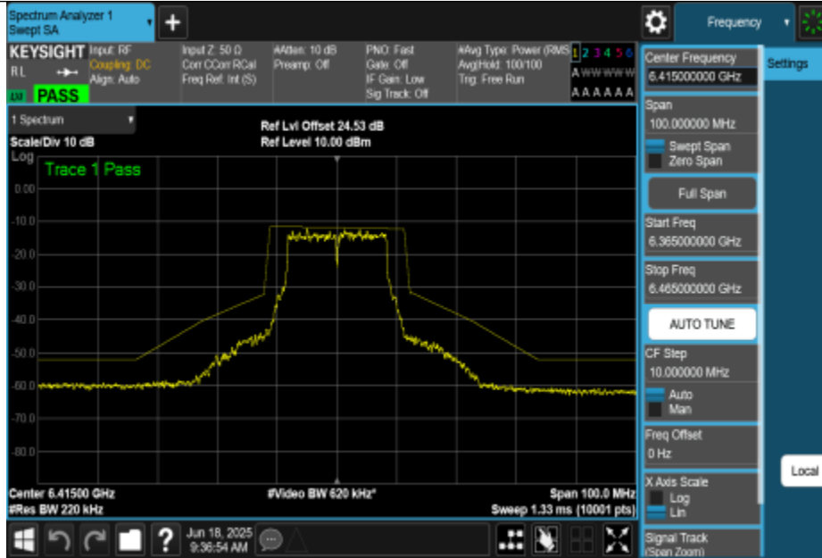
NTNV-11A-CDD-Ant0-6415-PASS
