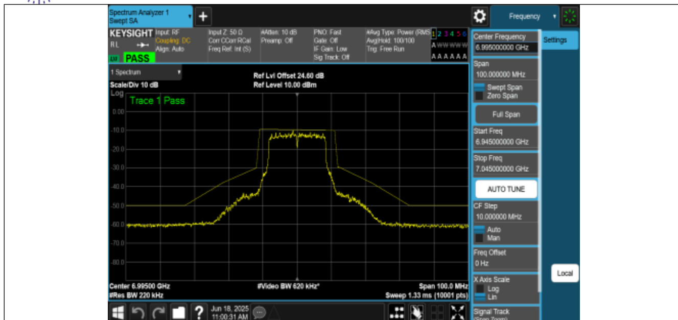
NTNV-11A-CDD-Ant2-6995-PASS
