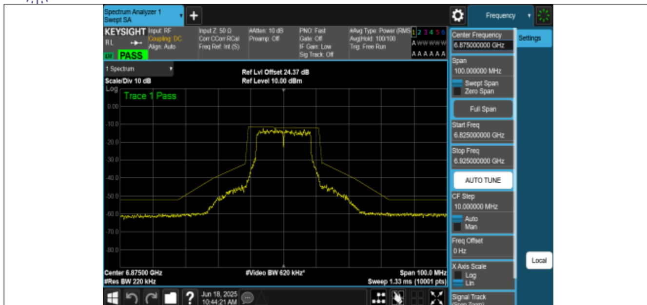
NTNV-11A-CDD-Ant0-6875-PASS
