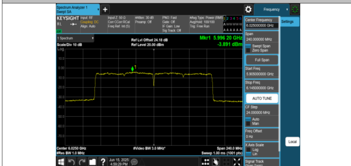
11BE160MIMO-Ant3-6025-PASS
