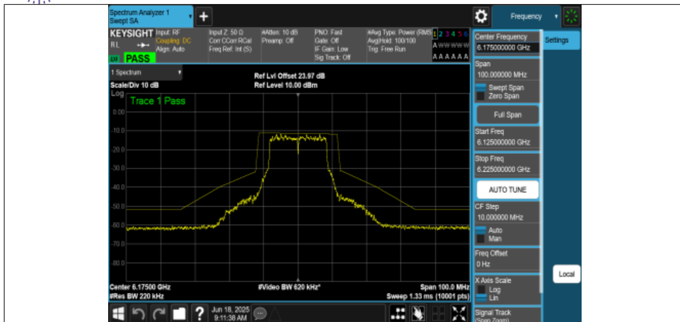
NTNV-11A-CDD-Ant0-6175-PASS
