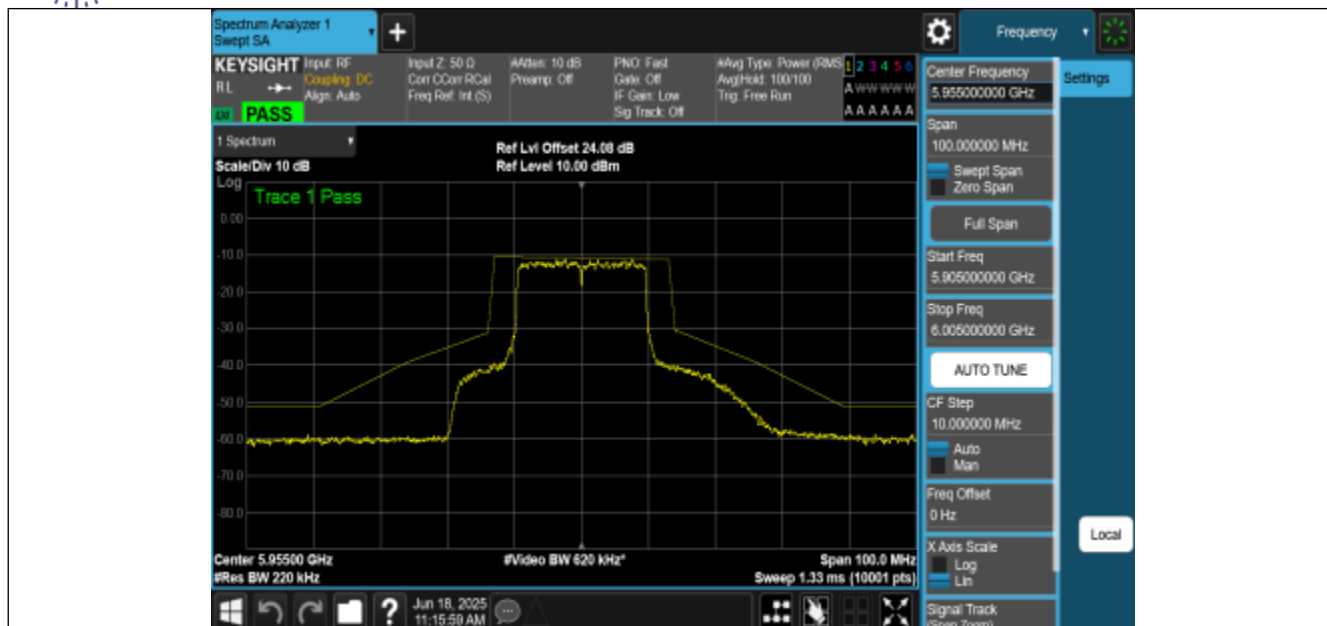
NTNV-11AX20MIMO-Ant0-5955-PASS
