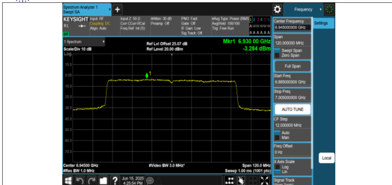
11BE80MIMO-Ant0-6945-PASS
