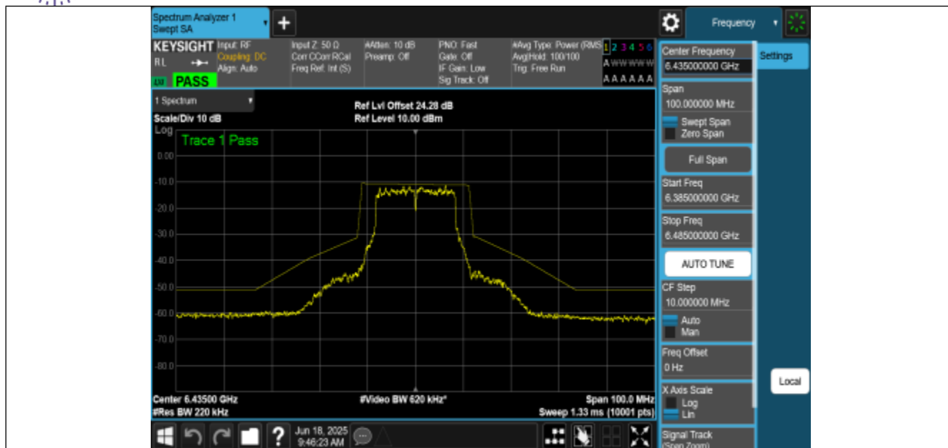
NTNV-11A-CDD-Ant2-6435-PASS
