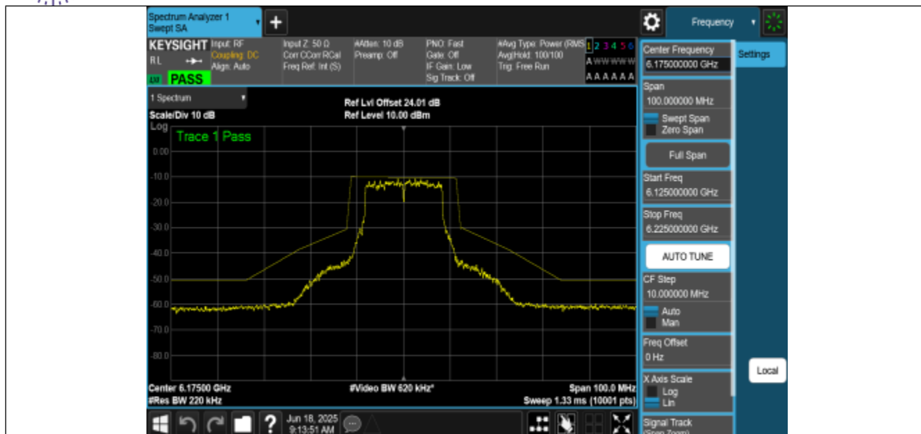
NTNV-11A-CDD-Ant2-6175-PASS
