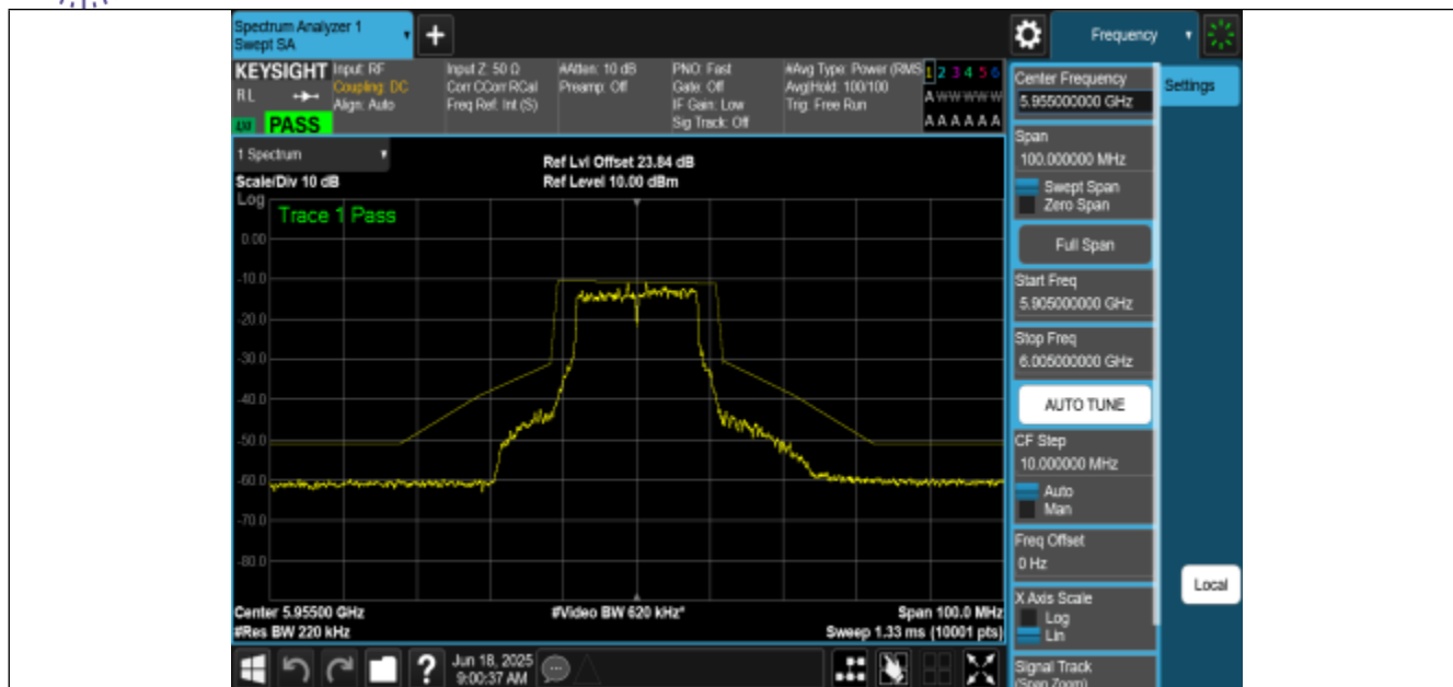
NTNV-11A-CDD-Ant3-5955-PASS
