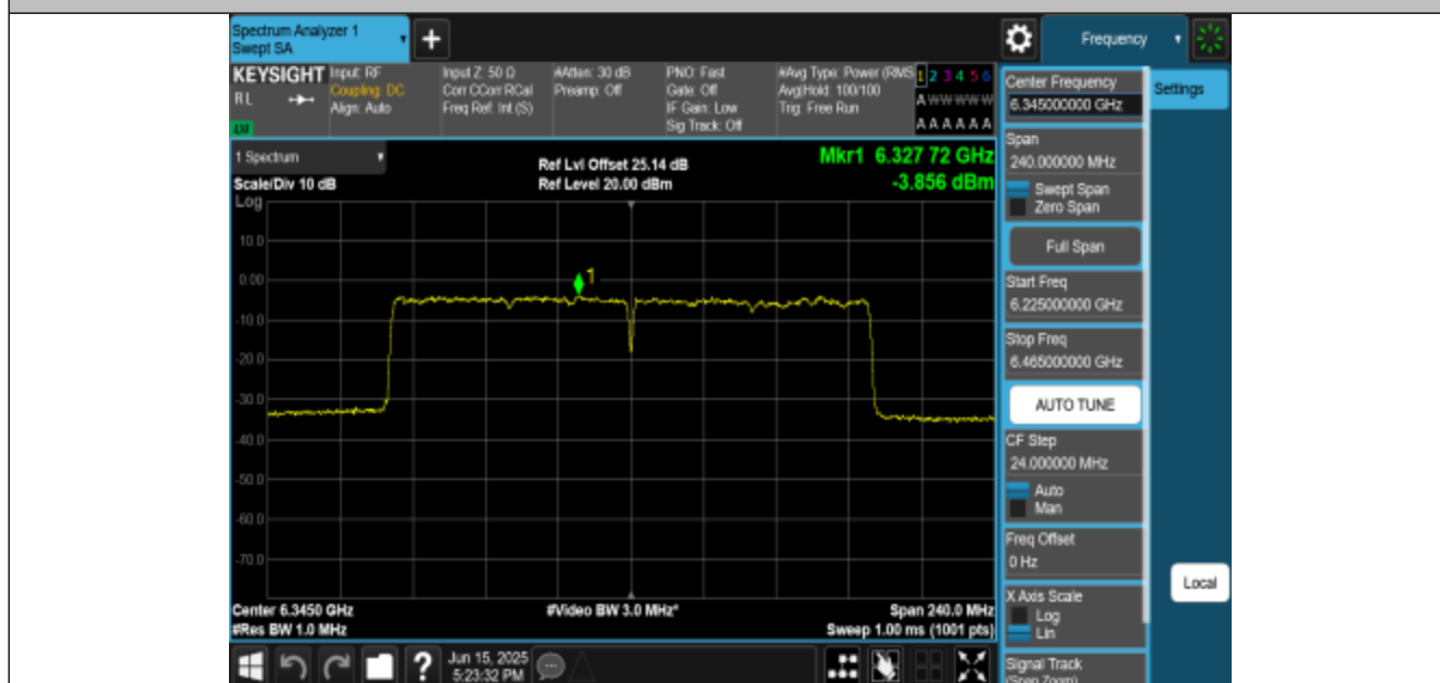
11BE160MIMO-Ant3-6345-PASS
