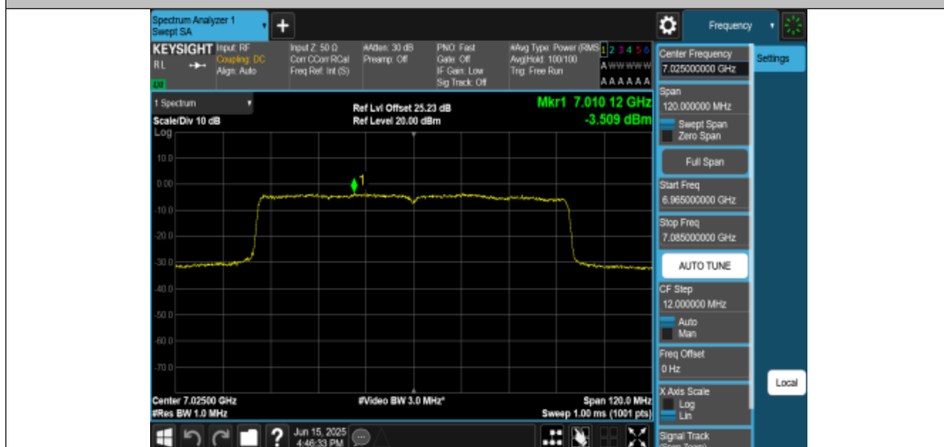
11BE80MIMO-Ant3-7025-PASS
