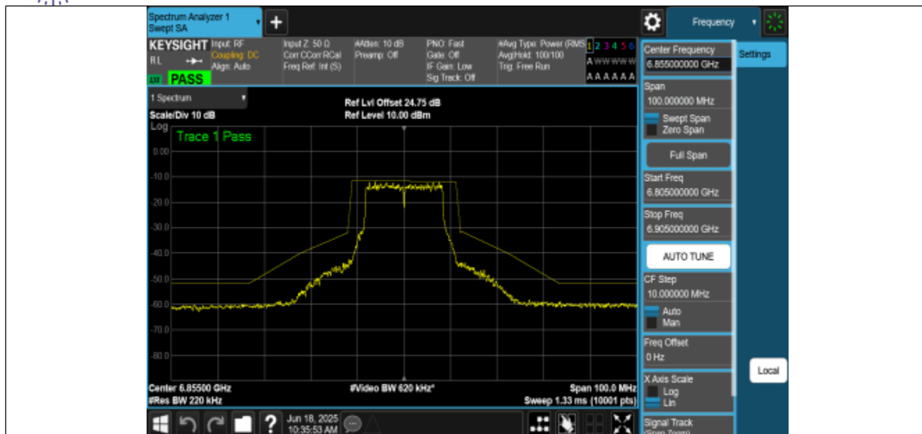
NTNV-11A-CDD-Ant2-6855-PASS
