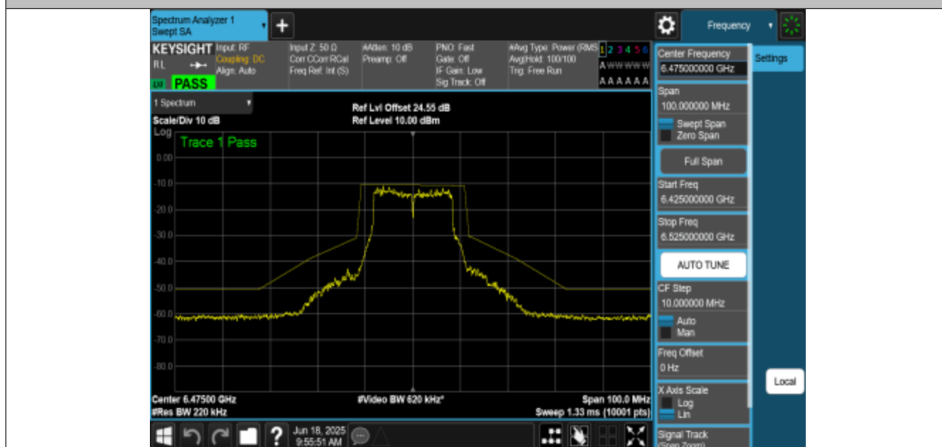
NTNV-11A-CDD-Ant3-6475-PASS
