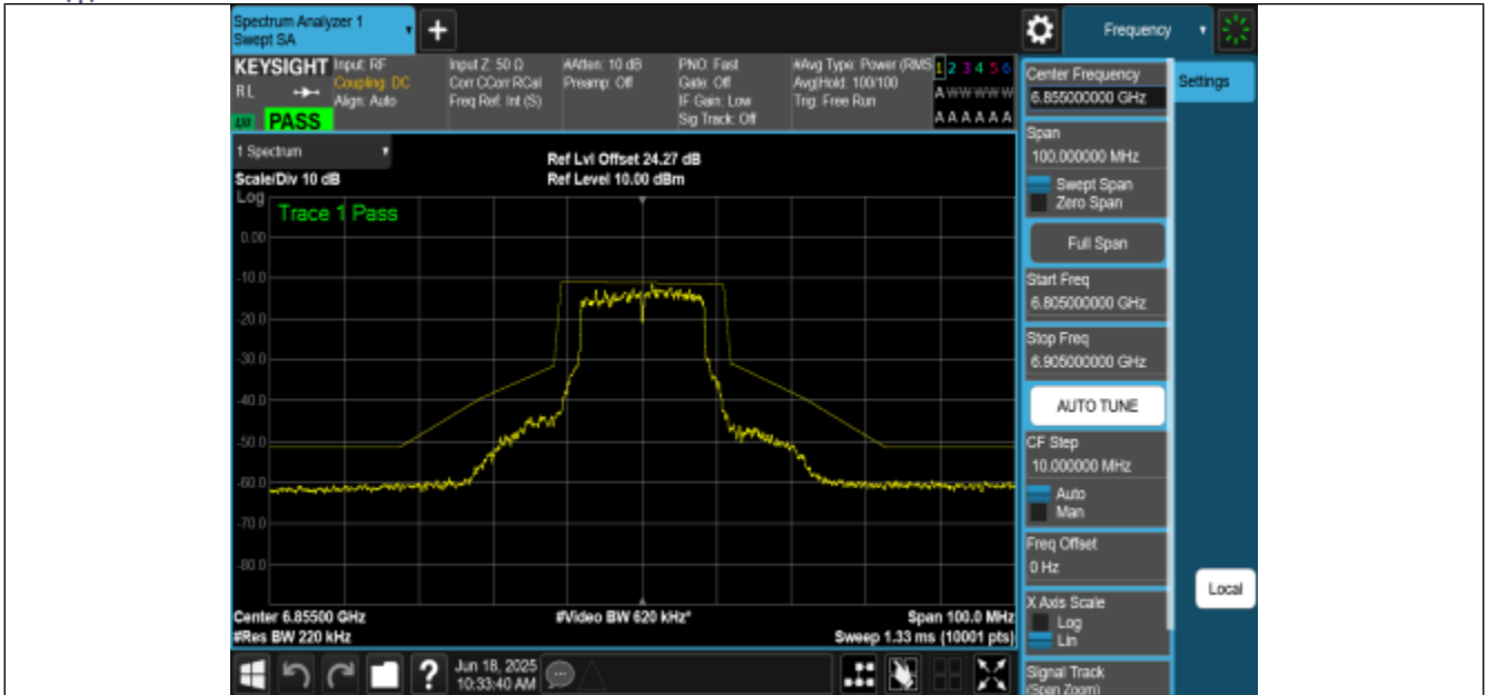
NTNV-11A-CDD-Ant0-6855-PASS
