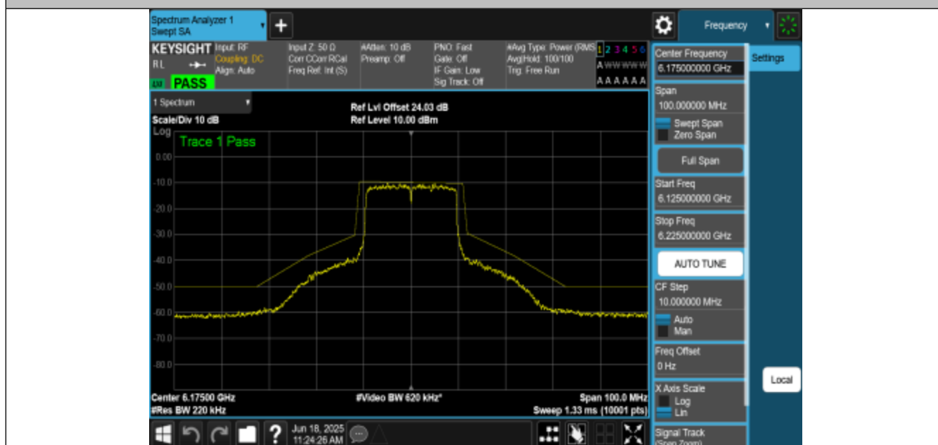
NTNV-11AX20MIMO-Ant1-6175-PASS
