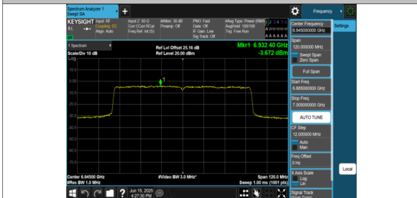
11BE80MIMO-Ant1-6945-PASS
