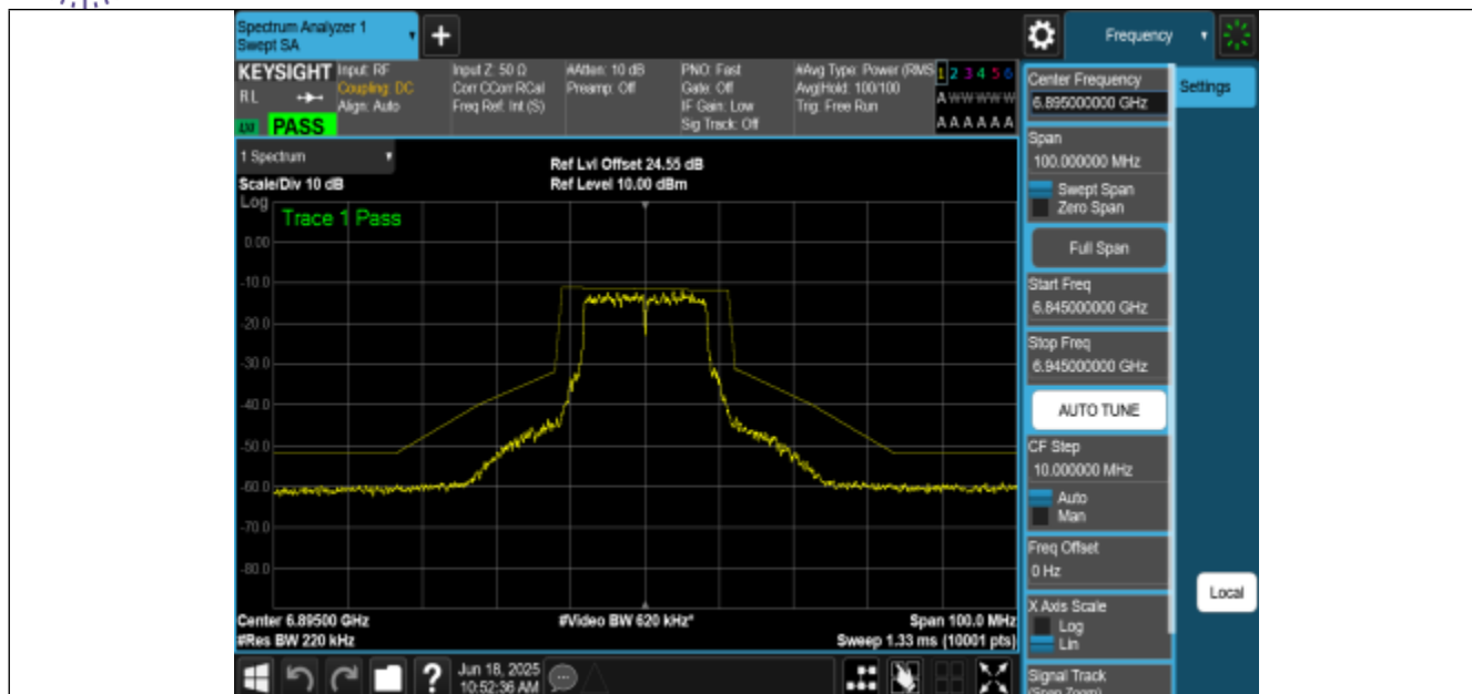
NTNV-11A-CDD-Ant2-6895-PASS
