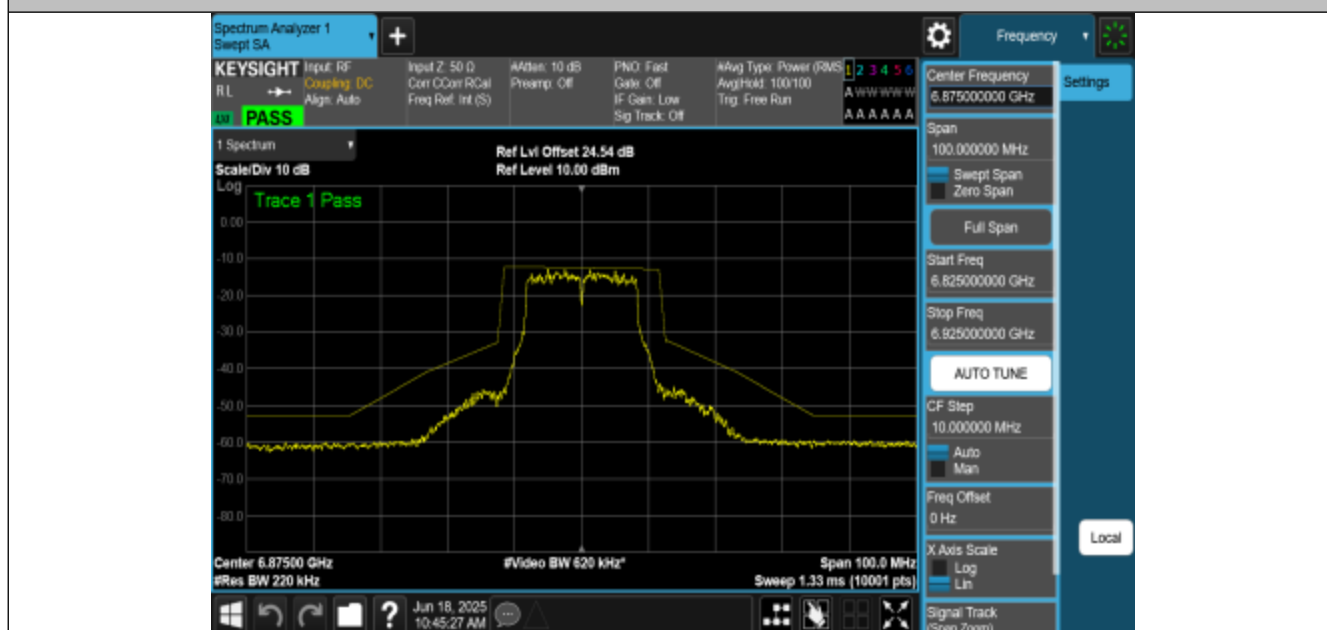
NTNV-11A-CDD-Ant1-6875-PASS
