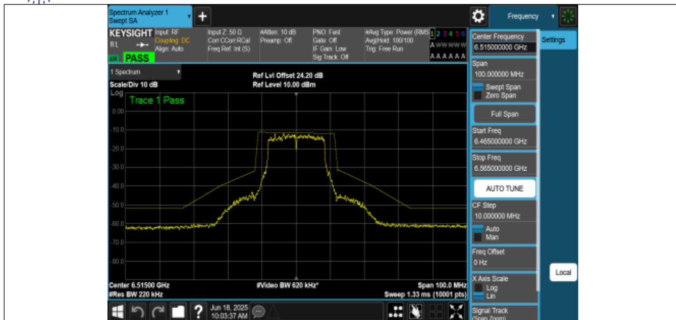
NTNV-11A-CDD-Ant2-6515-PASS
