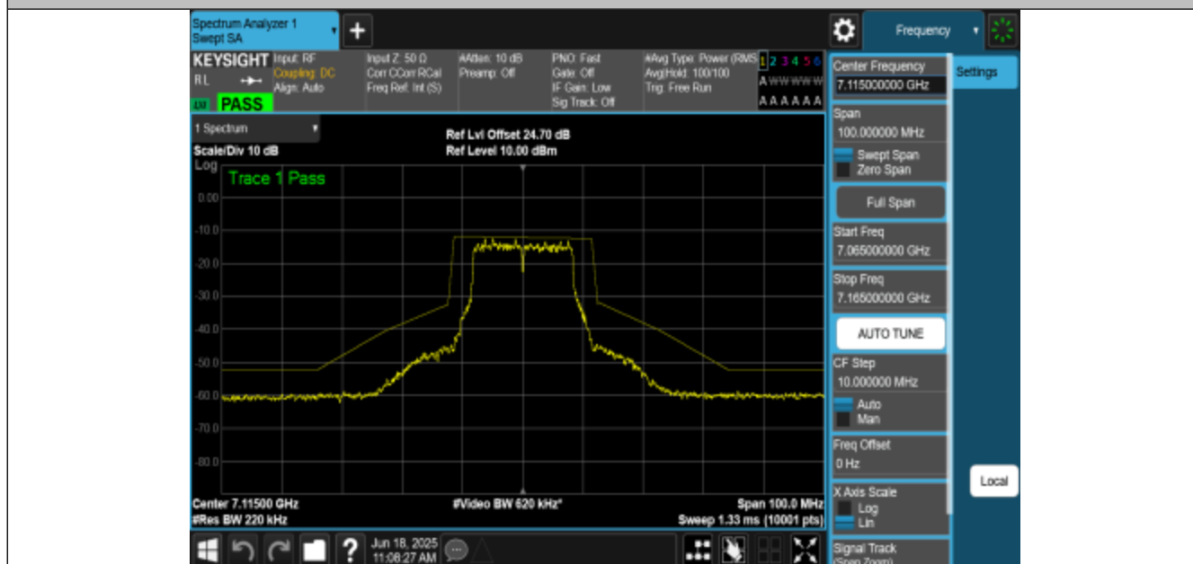
NTNV-11A-CDD-Ant1-7115-PASS
