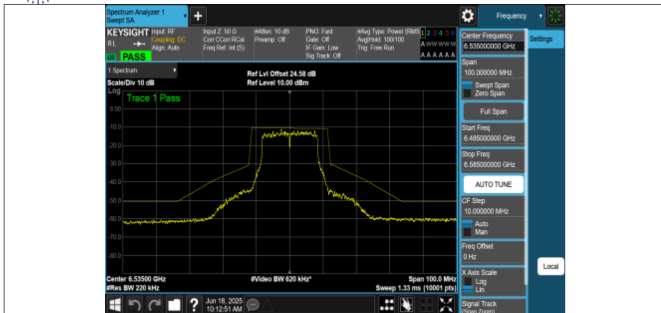
NTNV-11A-CDD-Ant2-6535-PASS
