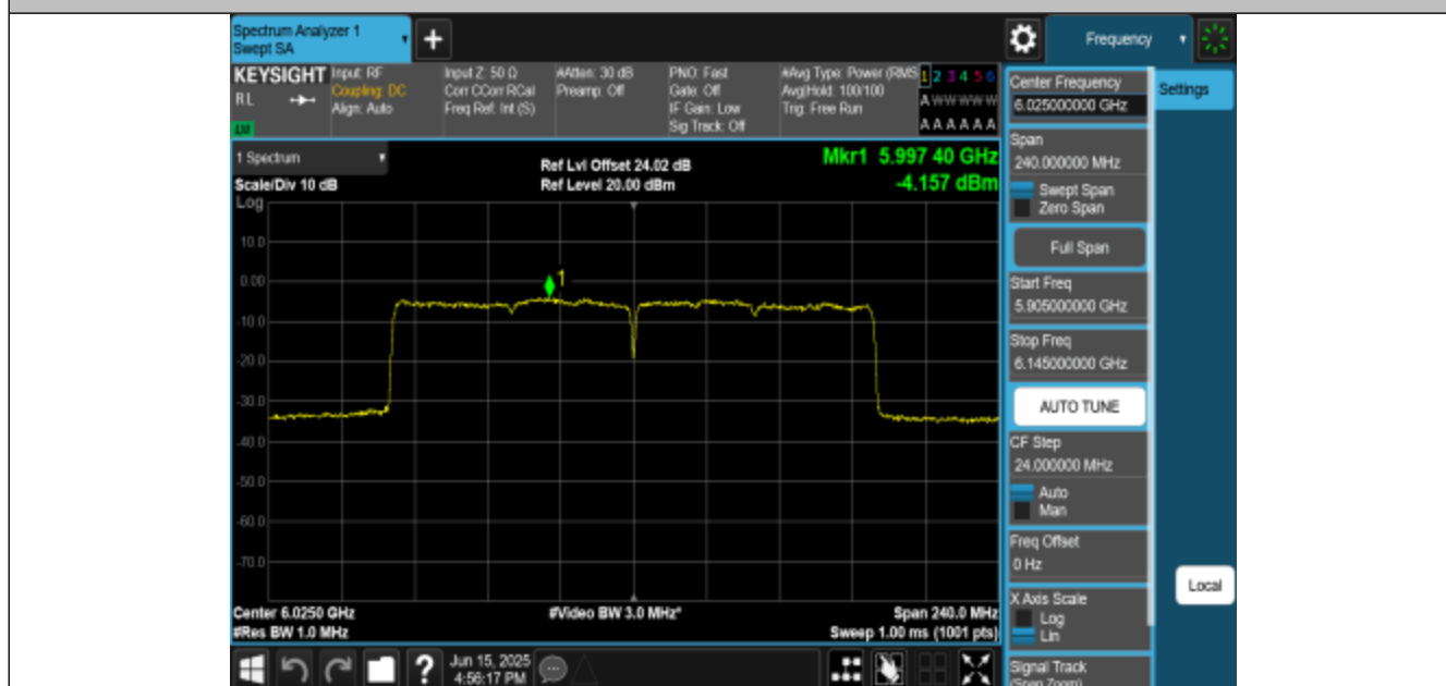
11BE160MIMO-Ant1-6025-PASS
