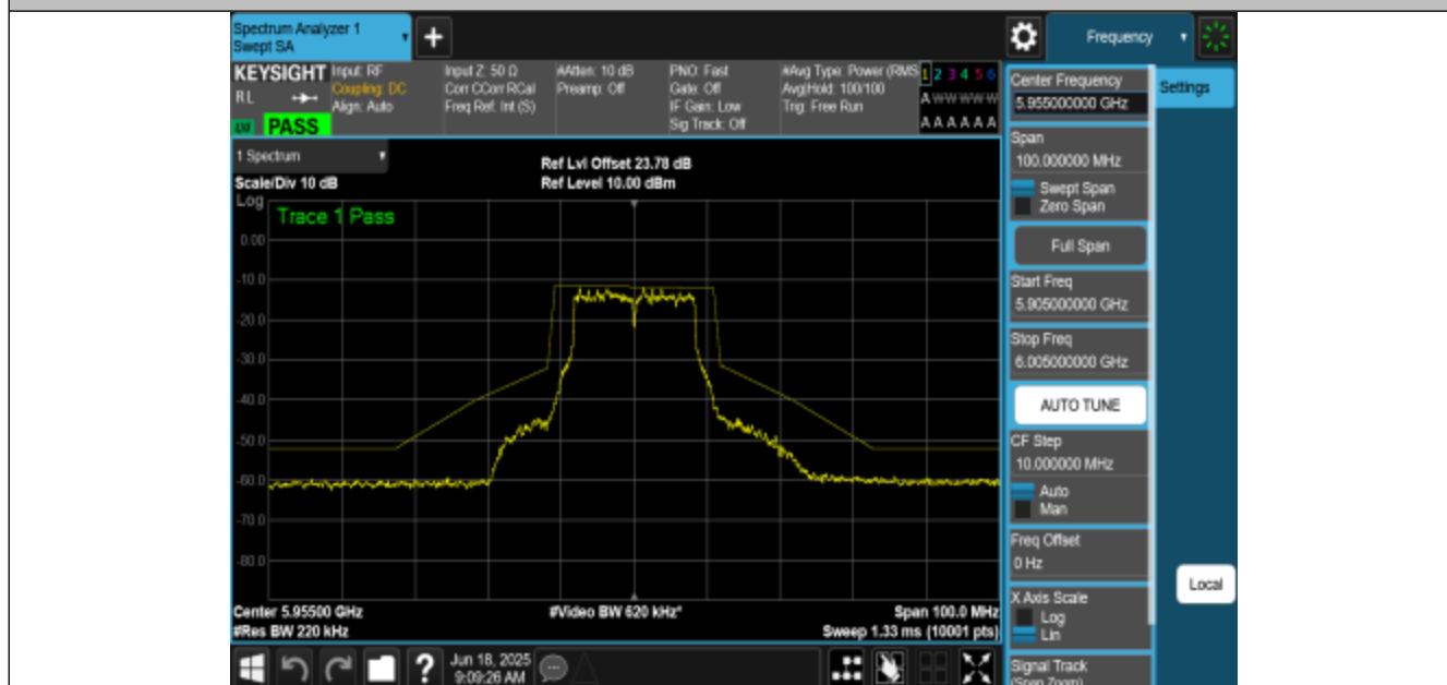
NTNV-11A-CDD-Ant1-5955-PASS
