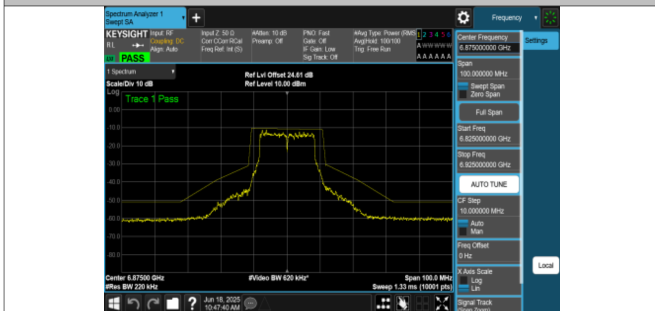
NTNV-11A-CDD-Ant3-6875-PASS
