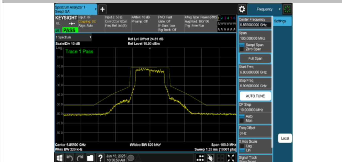
NTNV-11A-CDD-Ant3-6855-PASS
