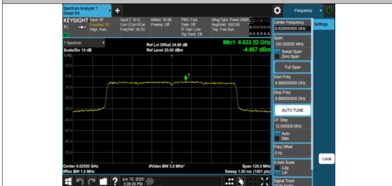
11BE80MIMO-Ant1-6625-PASS
