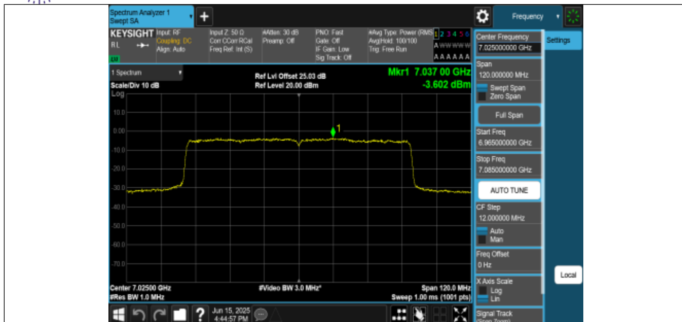
11BE80MIMO-Ant2-7025-PASS
