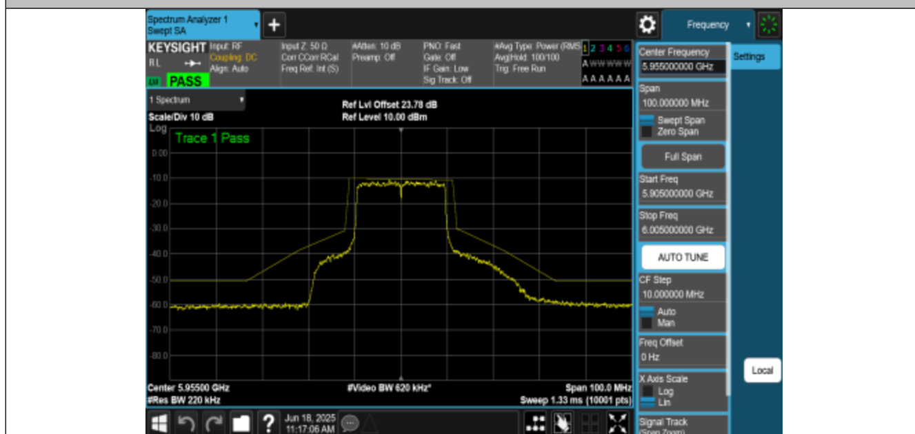
NTNV-11AX20MIMO-Ant1-5955-PASS
