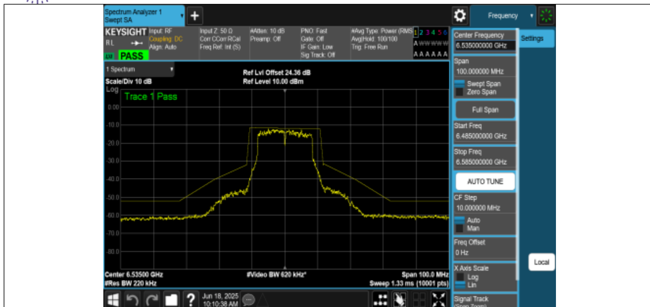
NTNV-11A-CDD-Ant0-6535-PASS
