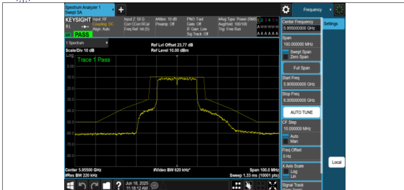
NTNV-11AX20MIMO-Ant2-5955-PASS
