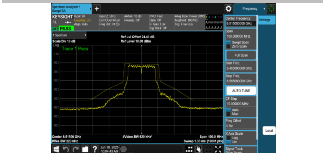
NTNV-11A-CDD-Ant3-6515-PASS
