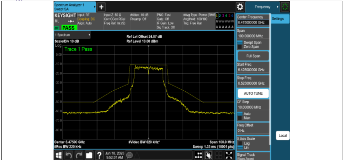
NTNV-11A-CDD-Ant0-6475-PASS
