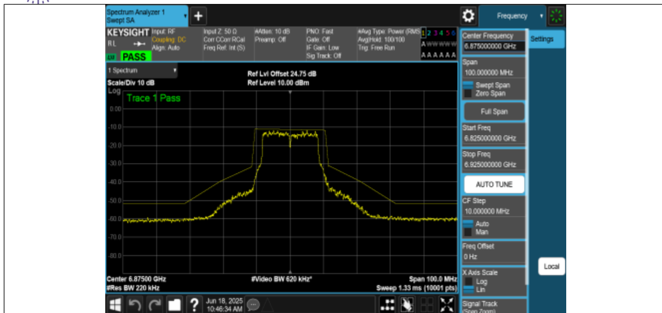
NTNV-11A-CDD-Ant2-6875-PASS
