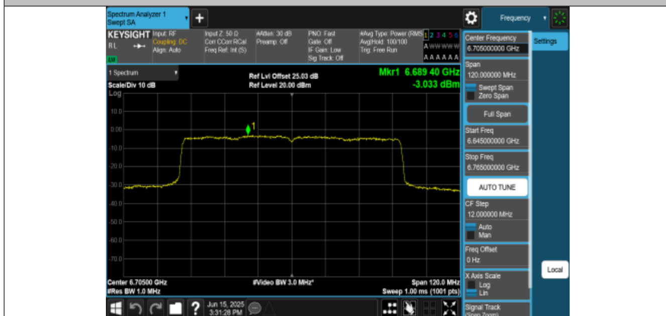
11BE80MIMO-Ant3-6705-PASS
