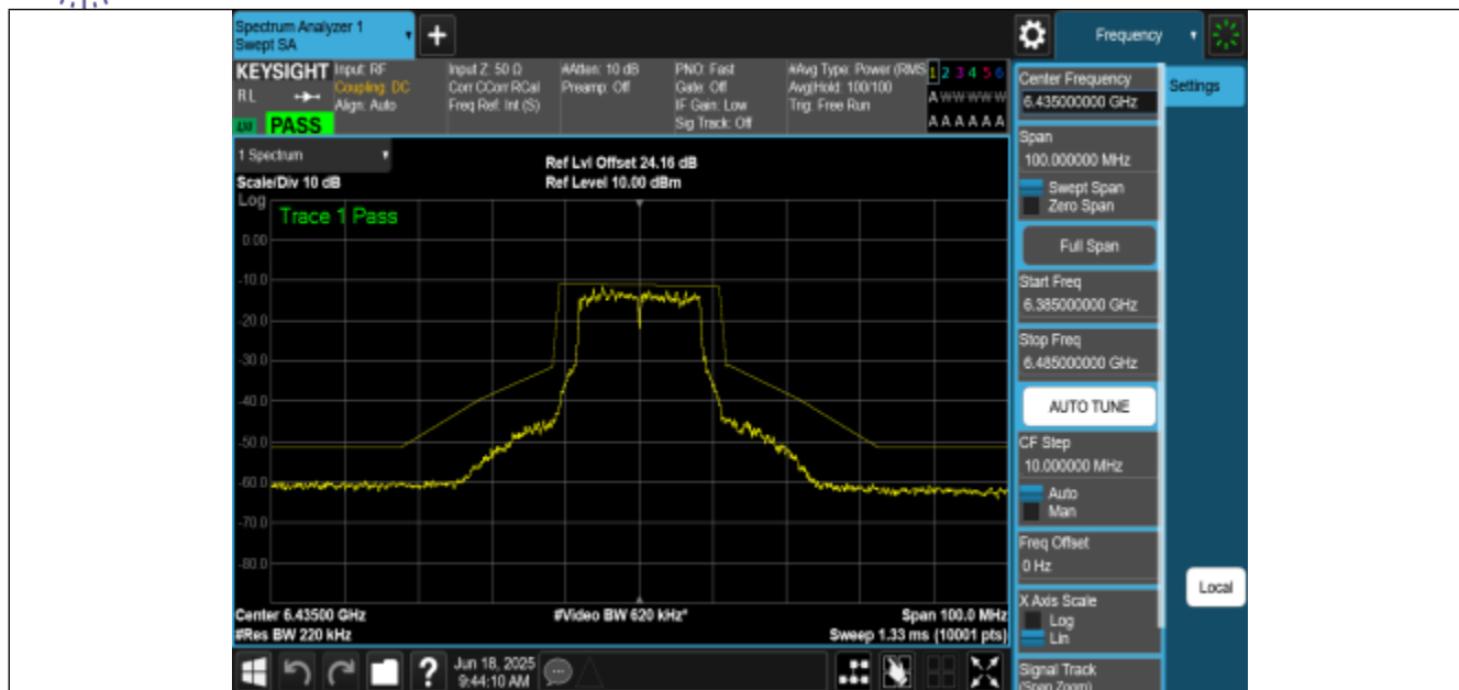
NTNV-11A-CDD-Ant0-6435-PASS
