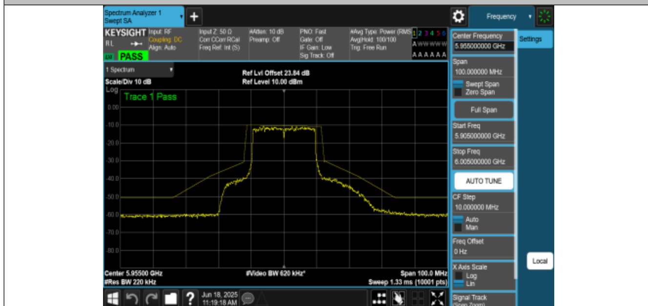
NTNV-11AX20MIMO-Ant3-5955-PASS
