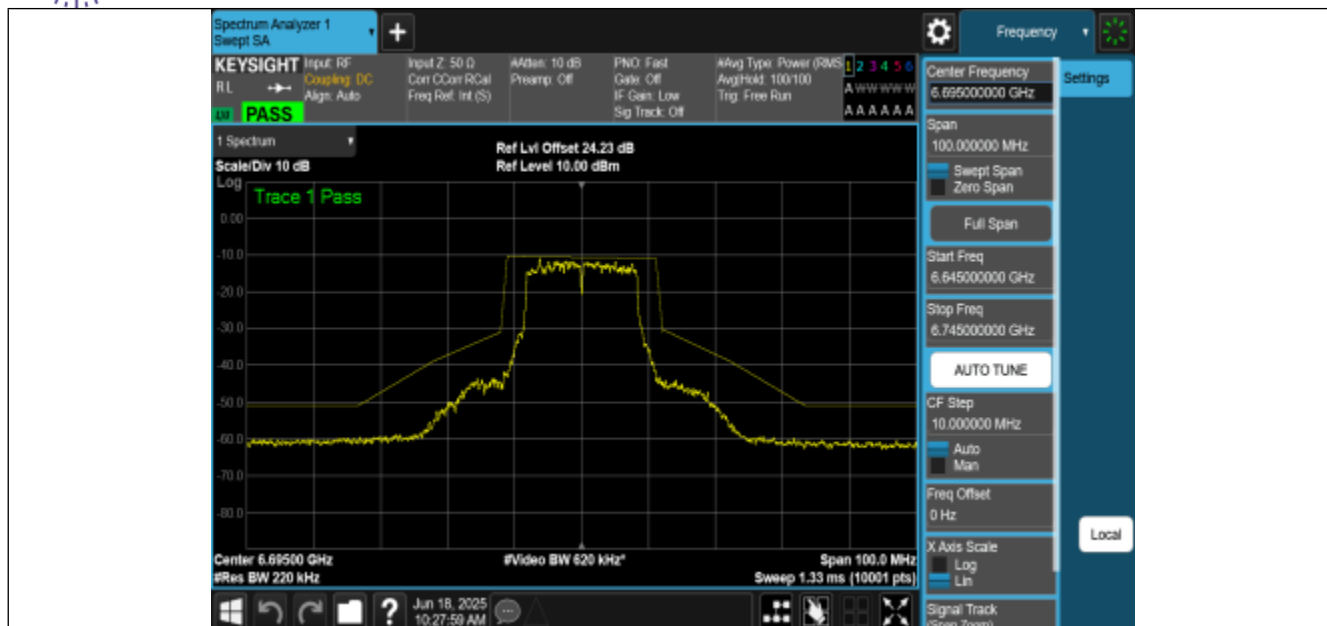
NTNV-11A-CDD-Ant2-6695-PASS
