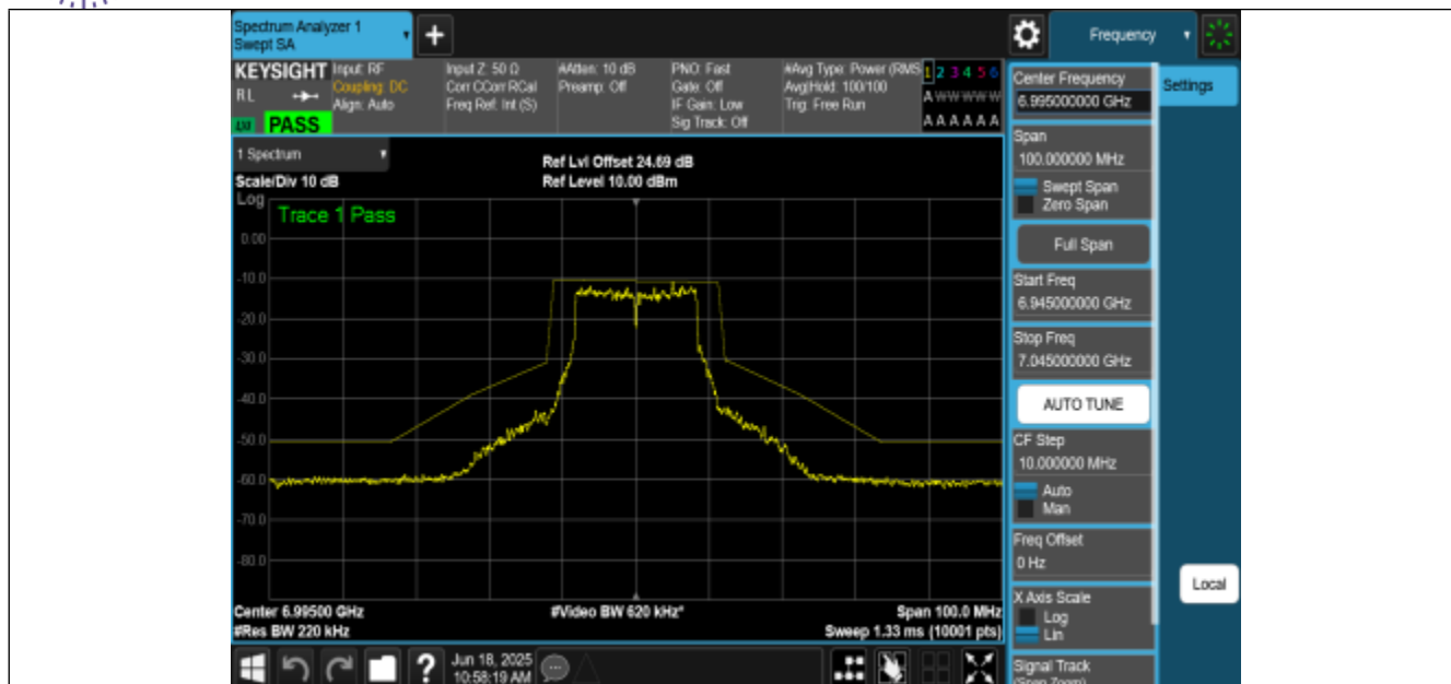
NTNV-11A-CDD-Ant0-6995-PASS
