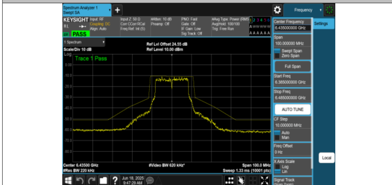
NTNV-11A-CDD-Ant3-6435-PASS
