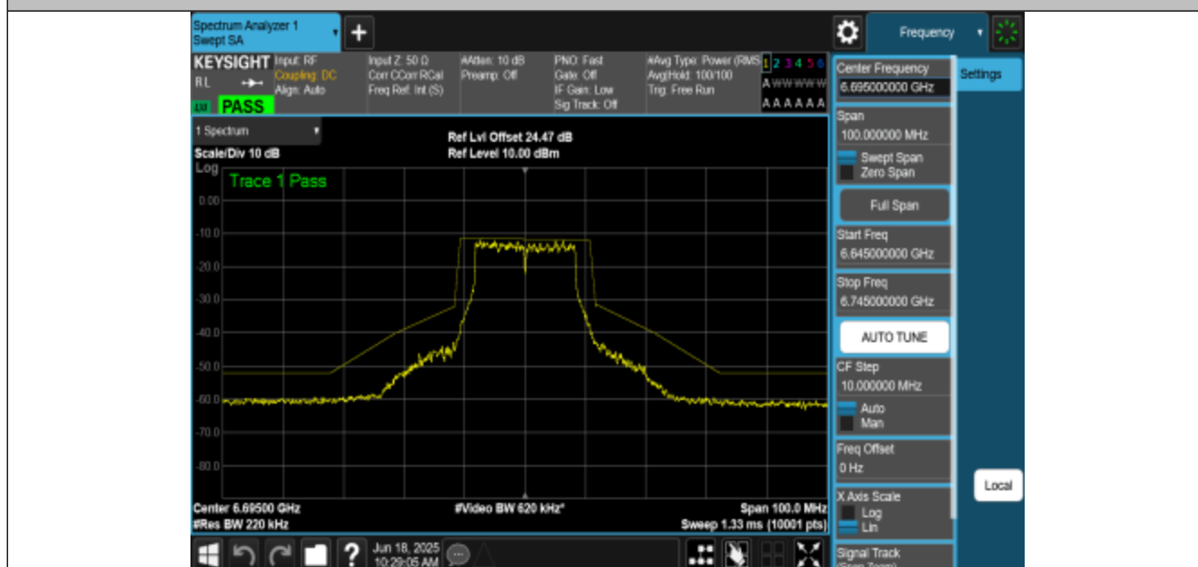
NTNV-11A-CDD-Ant3-6695-PASS
