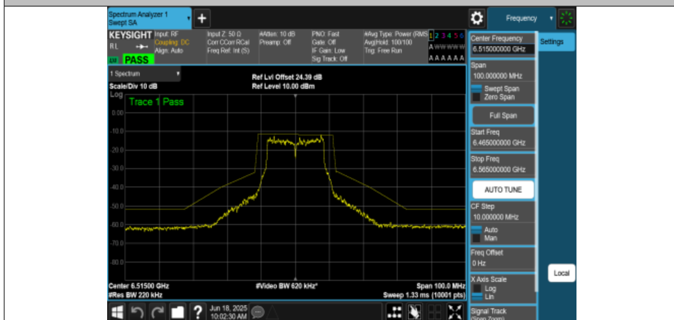
NTNV-11A-CDD-Ant1-6515-PASS
