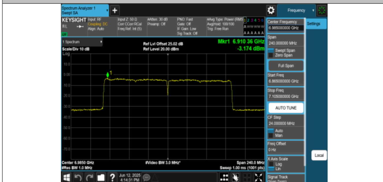
11AX160MIMO-Ant3-6985-PASS
