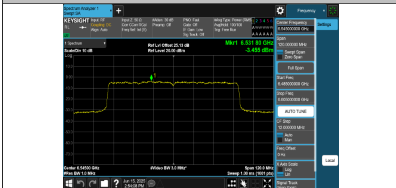
11BE80MIMO-Ant3-6545-PASS
