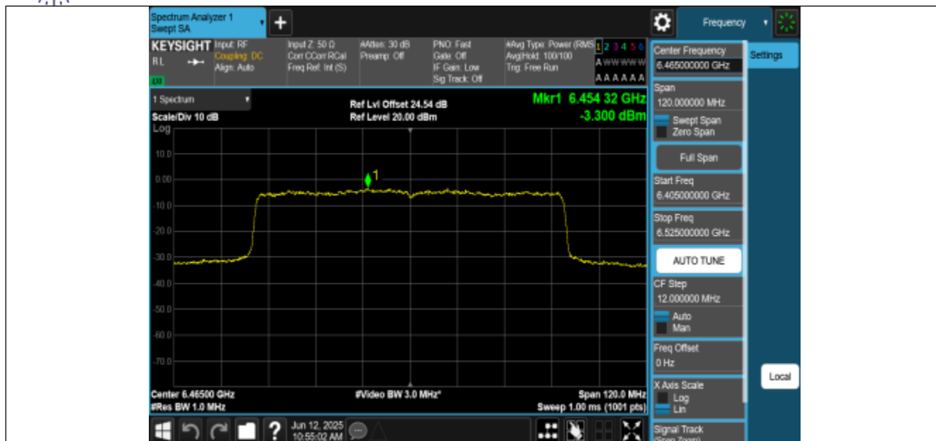
11AX80MIMO-Ant0-6465-PASS
