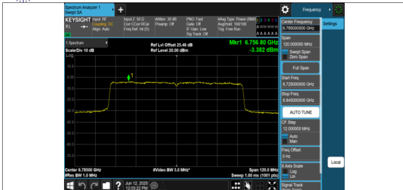
11AX80MIMO-Ant2-6785-PASS
