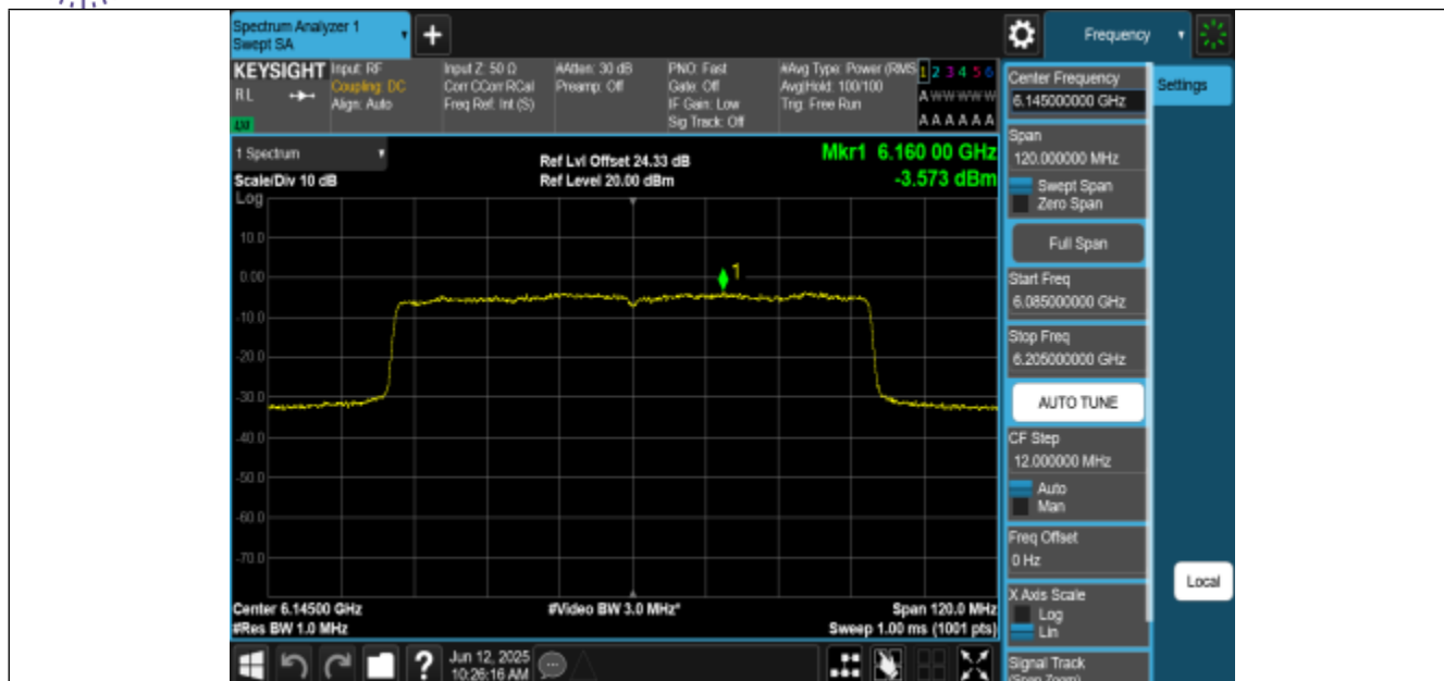
11AX80MIMO-Ant0-6145-PASS
