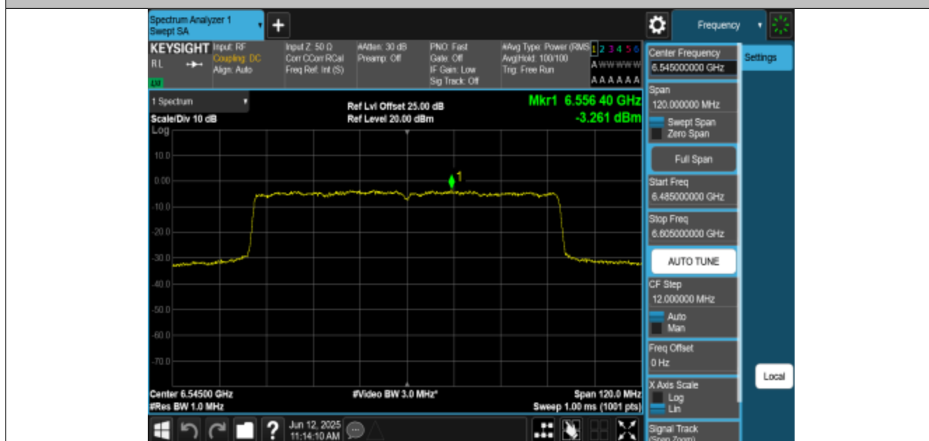
11AX80MIMO-Ant3-6545-PASS
