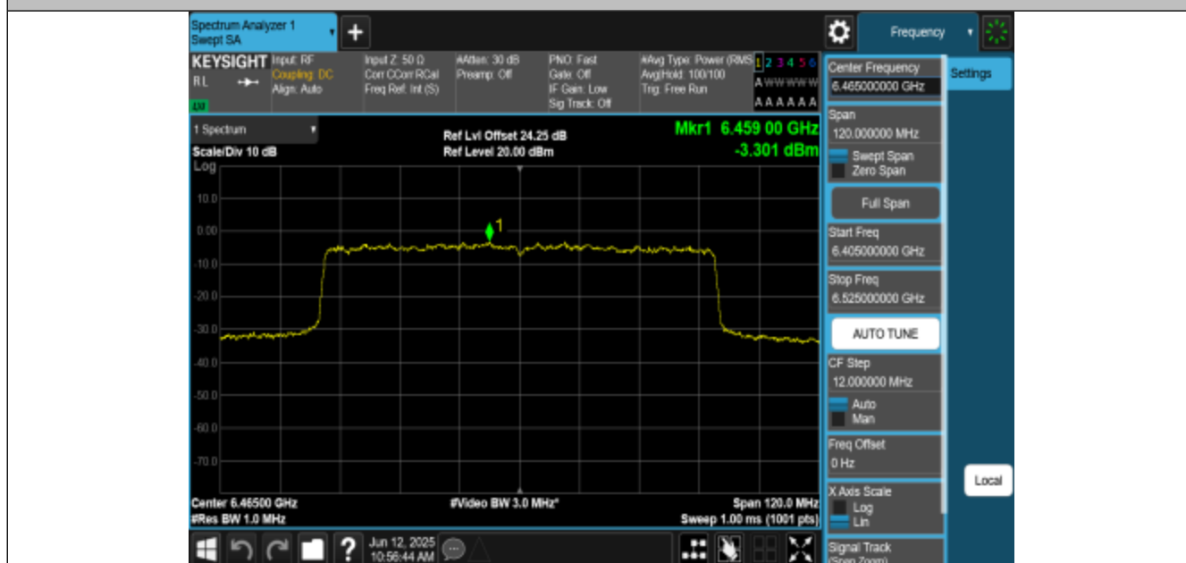
11AX80MIMO-Ant1-6465-PASS
