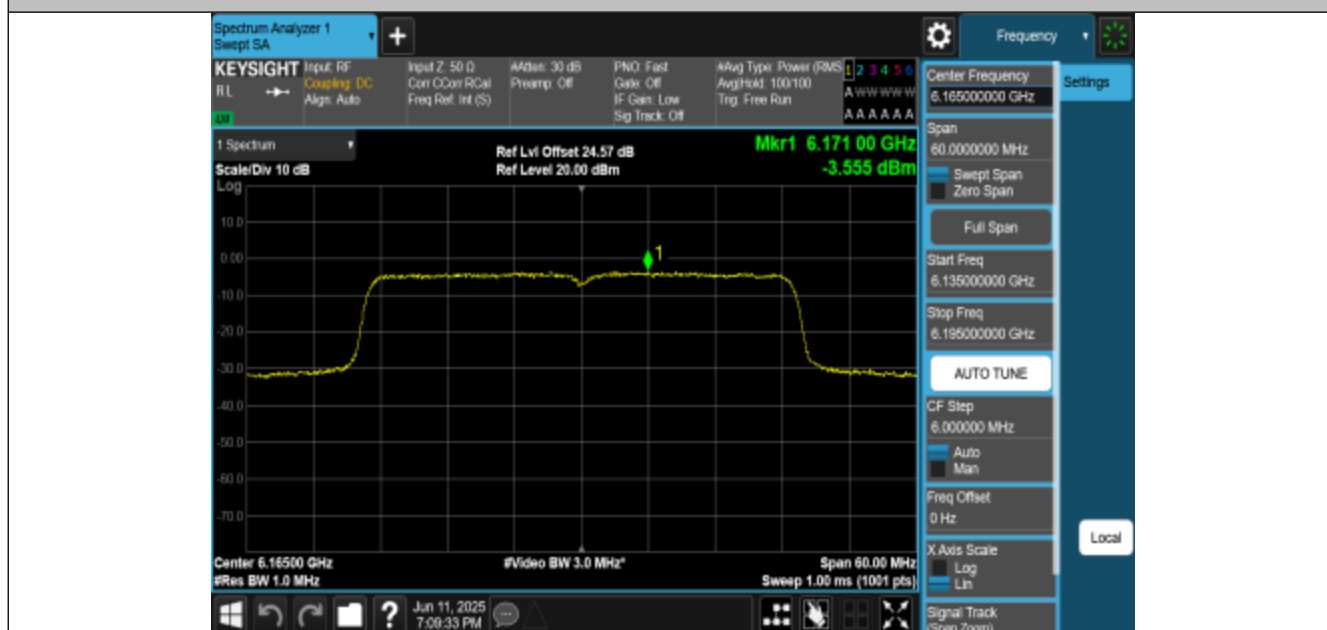
11AX40MIMO-Ant1-6165-PASS
