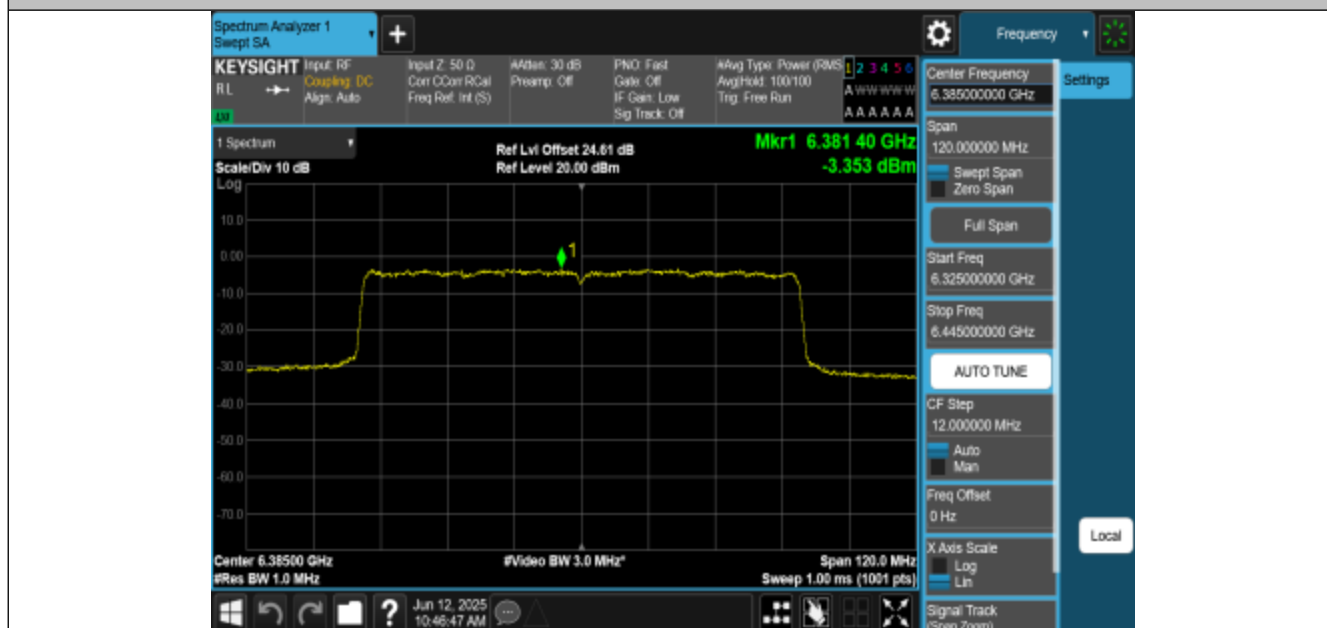
11AX80MIMO-Ant3-6385-PASS
