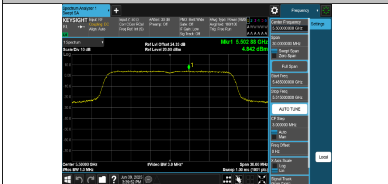
11BE20MIMO-Ant3-5500-PASS
