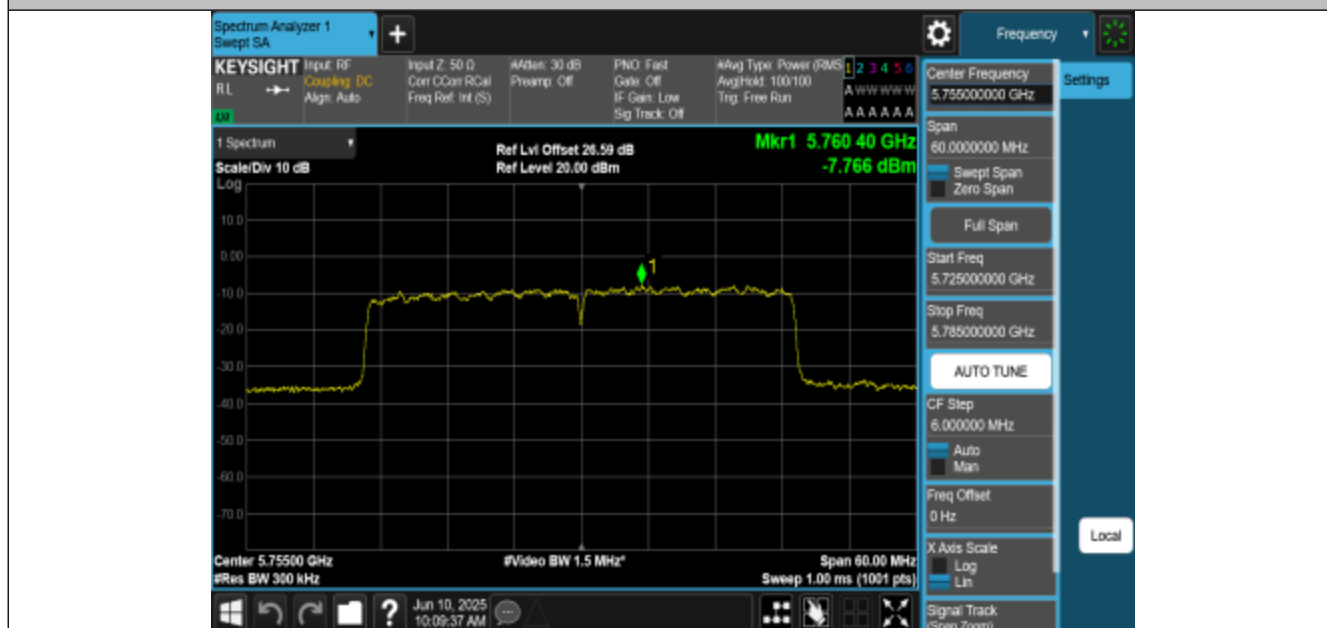
11BE40MIMO-Ant1-5755-PASS
