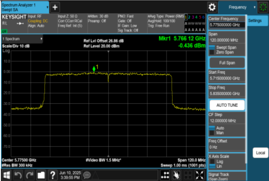
11BE80MIMO-Ant2-5775-PASS
