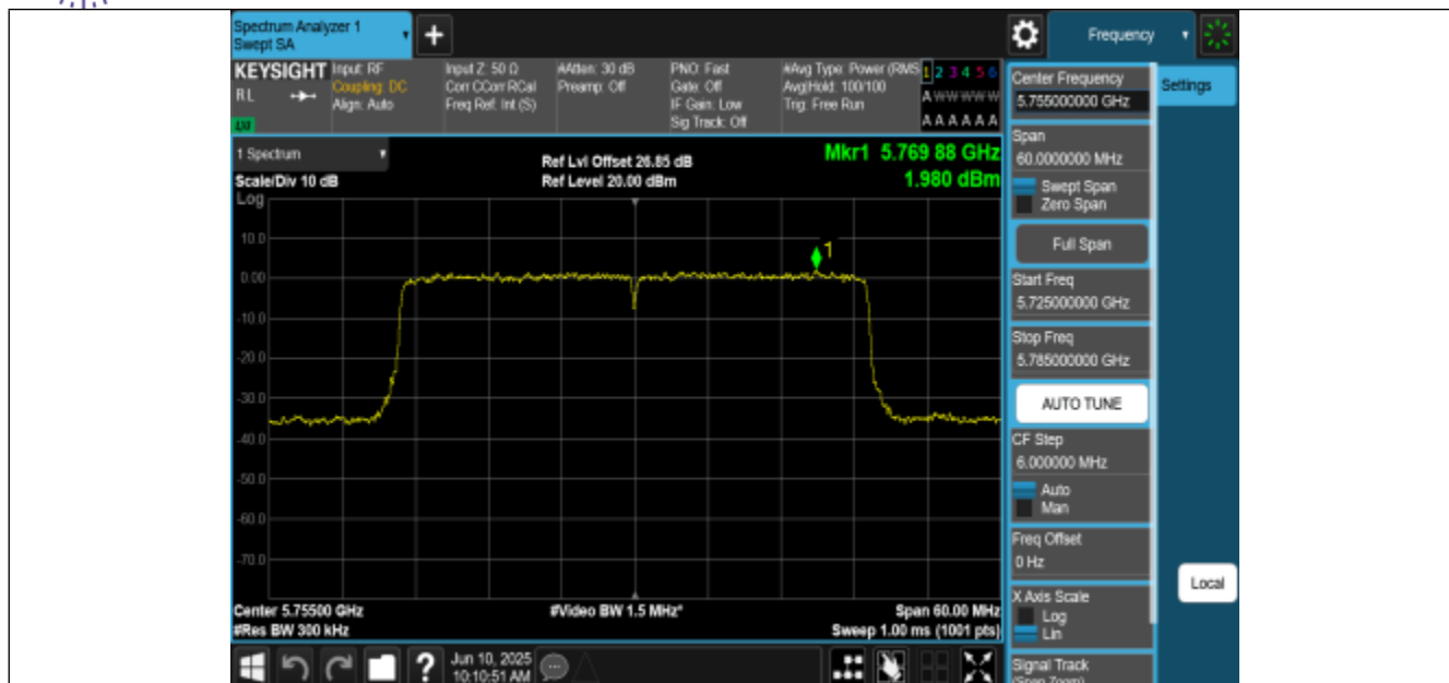
11BE40MIMO-Ant2-5755-PASS
