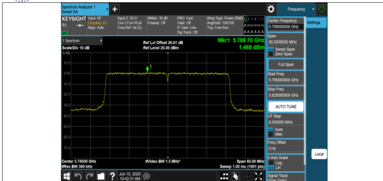
11BE40MIMO-Ant2-5795-PASS
