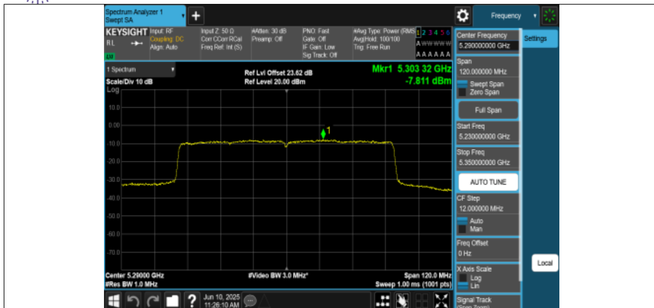
11BE80MIMO-Ant0-5290-PASS
