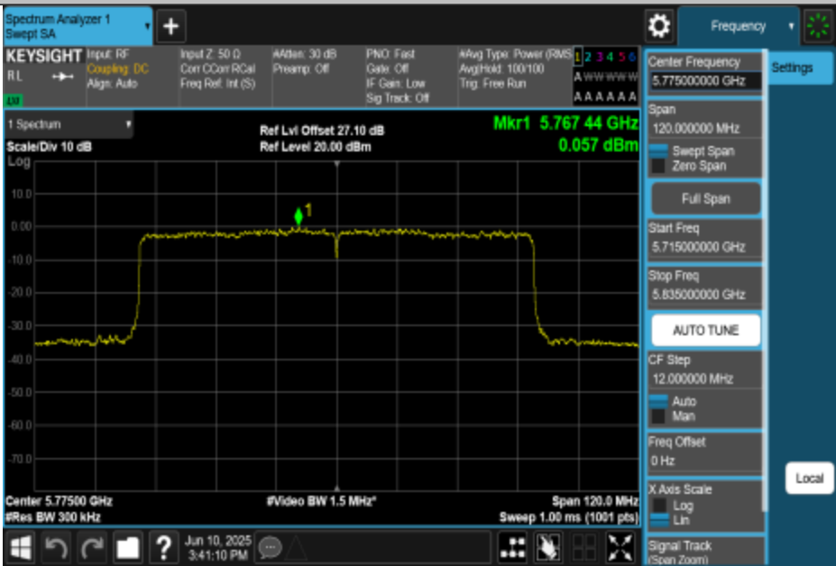
11BE80MIMO-Ant3-5775-PASS
