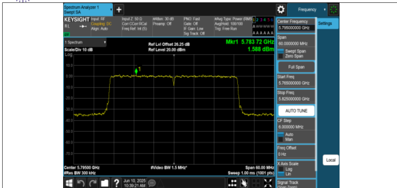
11BE40MIMO-Ant0-5795-PASS
