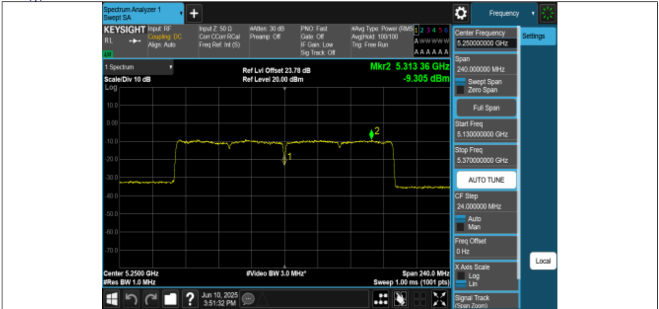
11BE160MIMO-Ant0-5250_UNII-2A-PASS
