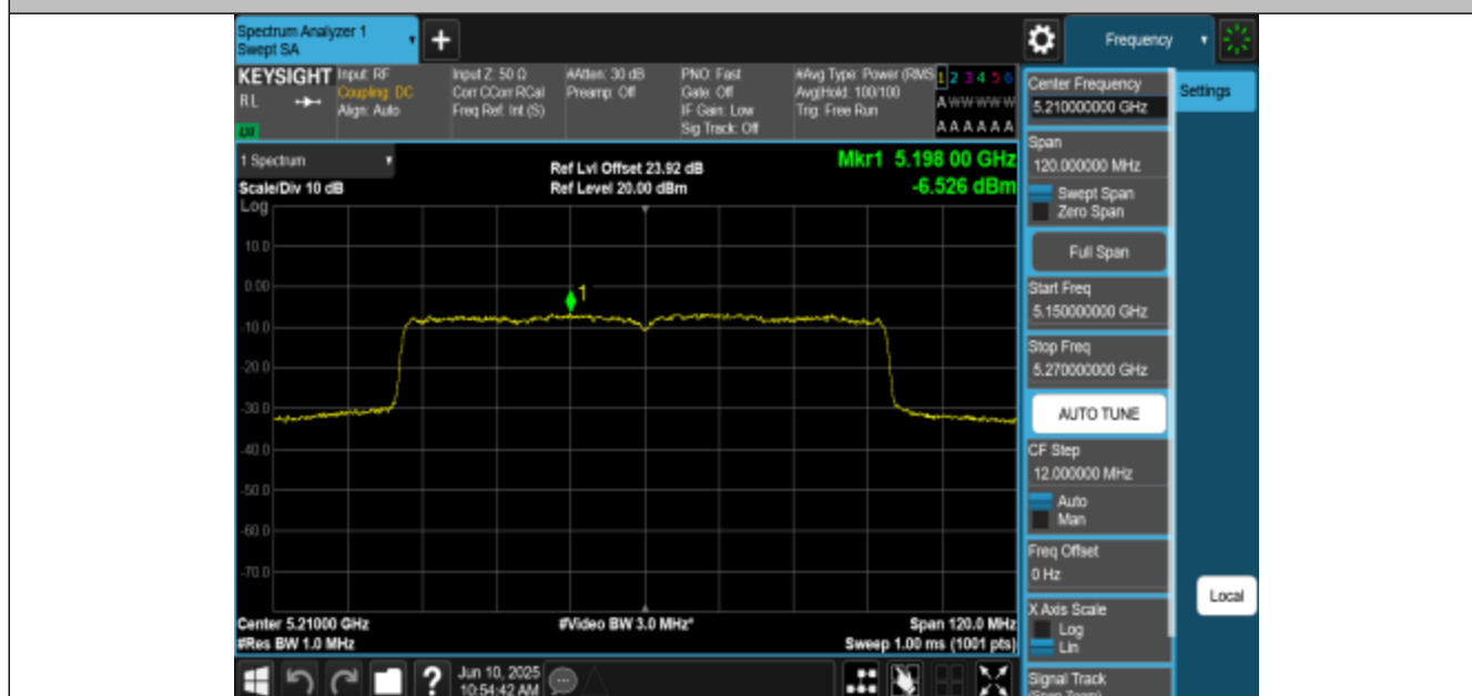
11BE80MIMO-Ant1-5210-PASS
