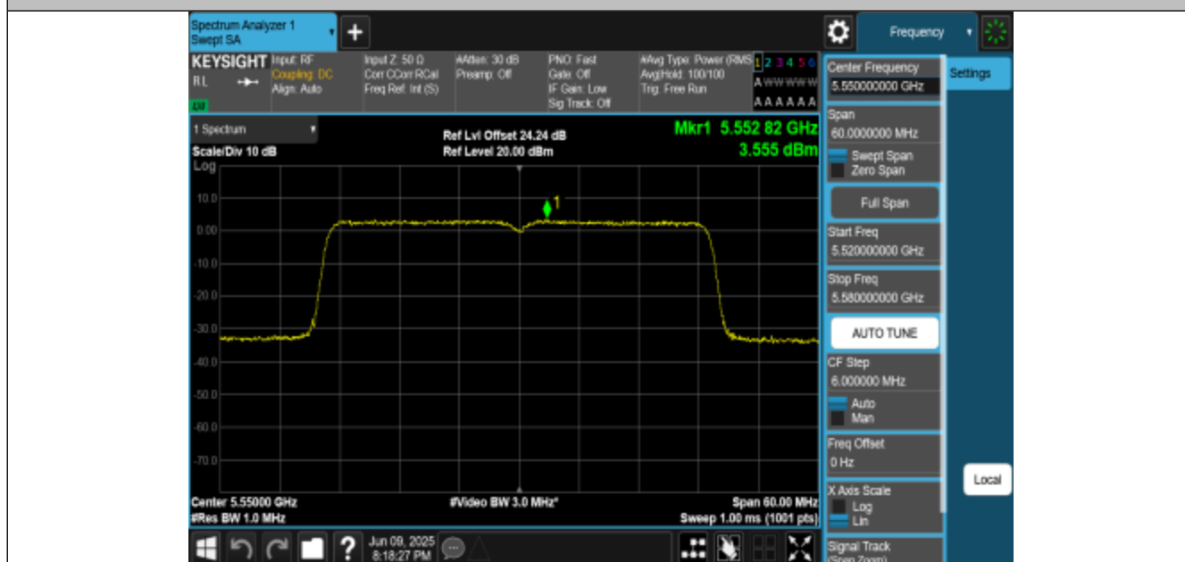
11BE40MIMO-Ant3-5550-PASS
