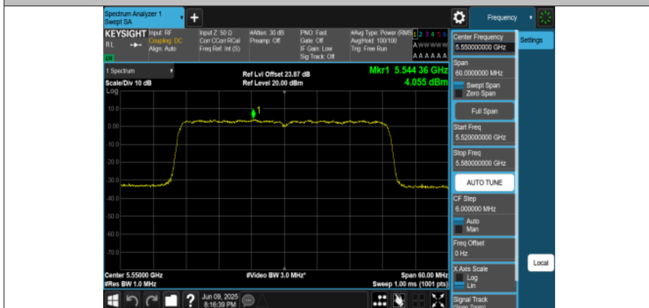
11BE40MIMO-Ant1-5550-PASS
