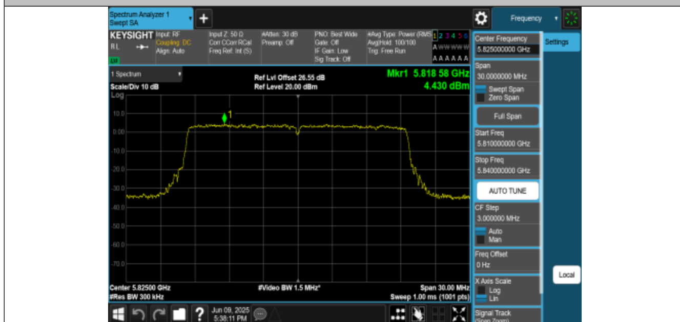
11BE20MIMO-Ant1-5825-PASS
