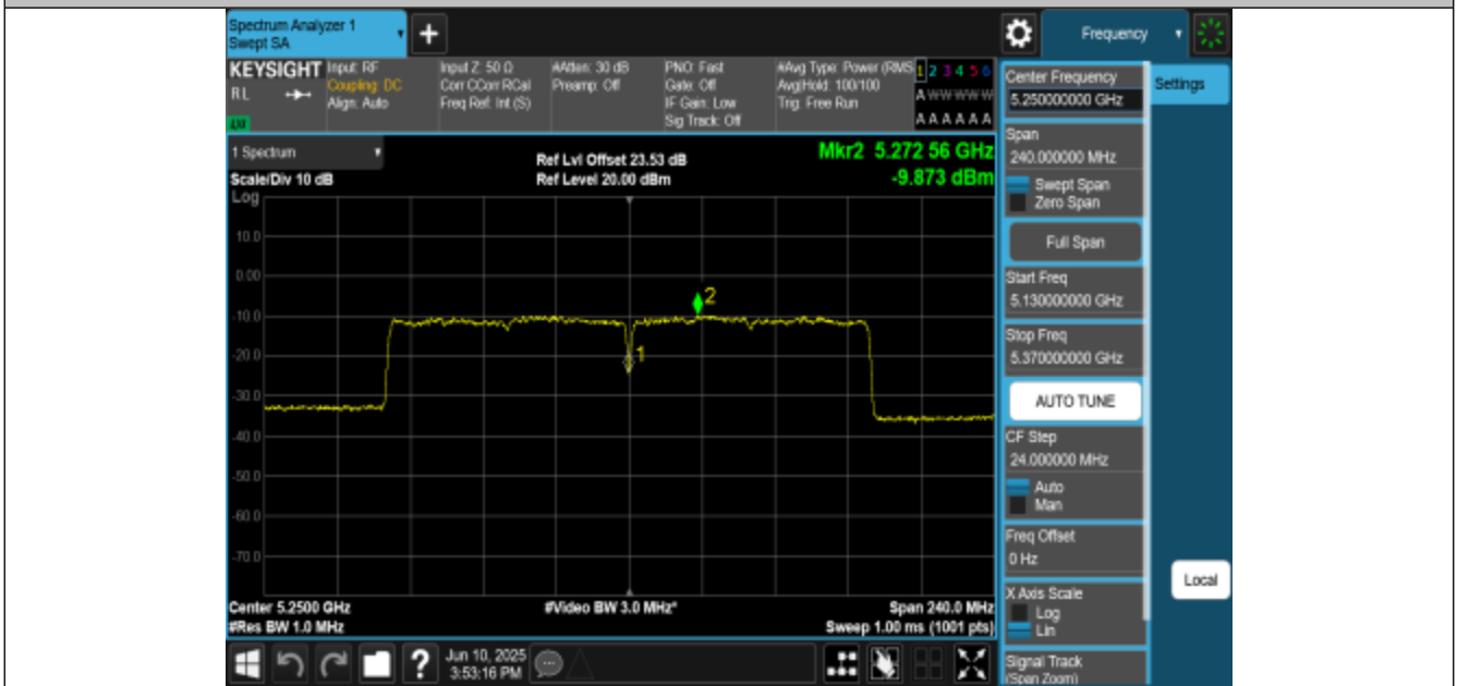
11BE160MIMO-Ant1-5250_UNII-2A-PASS
