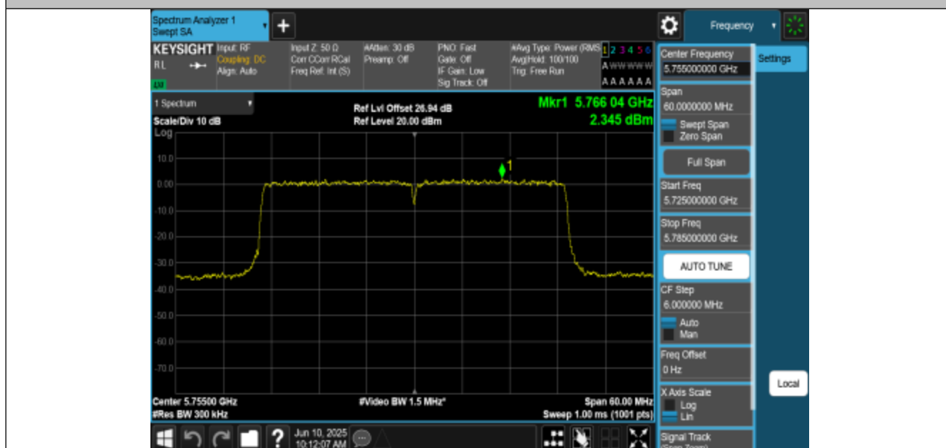
11BE40MIMO-Ant3-5755-PASS
