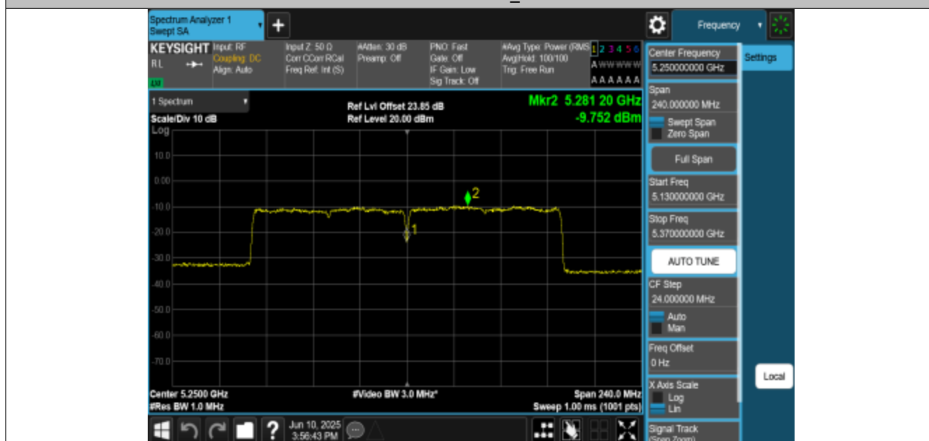
11BE160MIMO-Ant3-5250_UNII-2A-PASS
