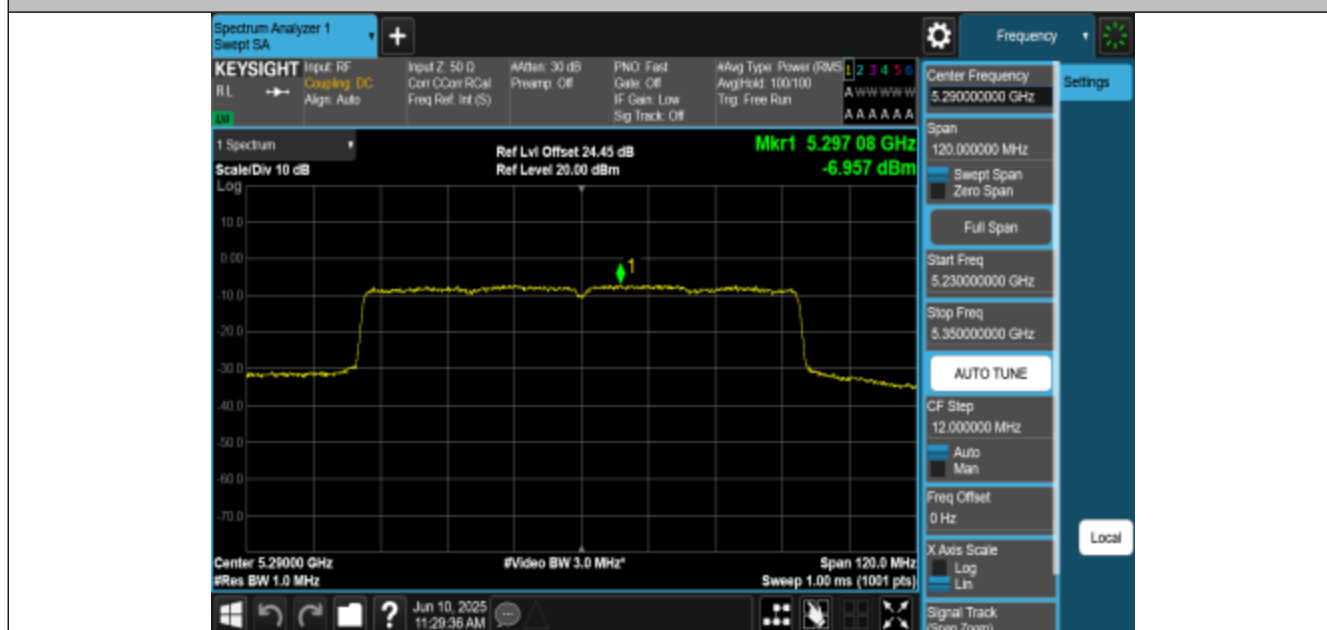
11BE80MIMO-Ant3-5290-PASS
