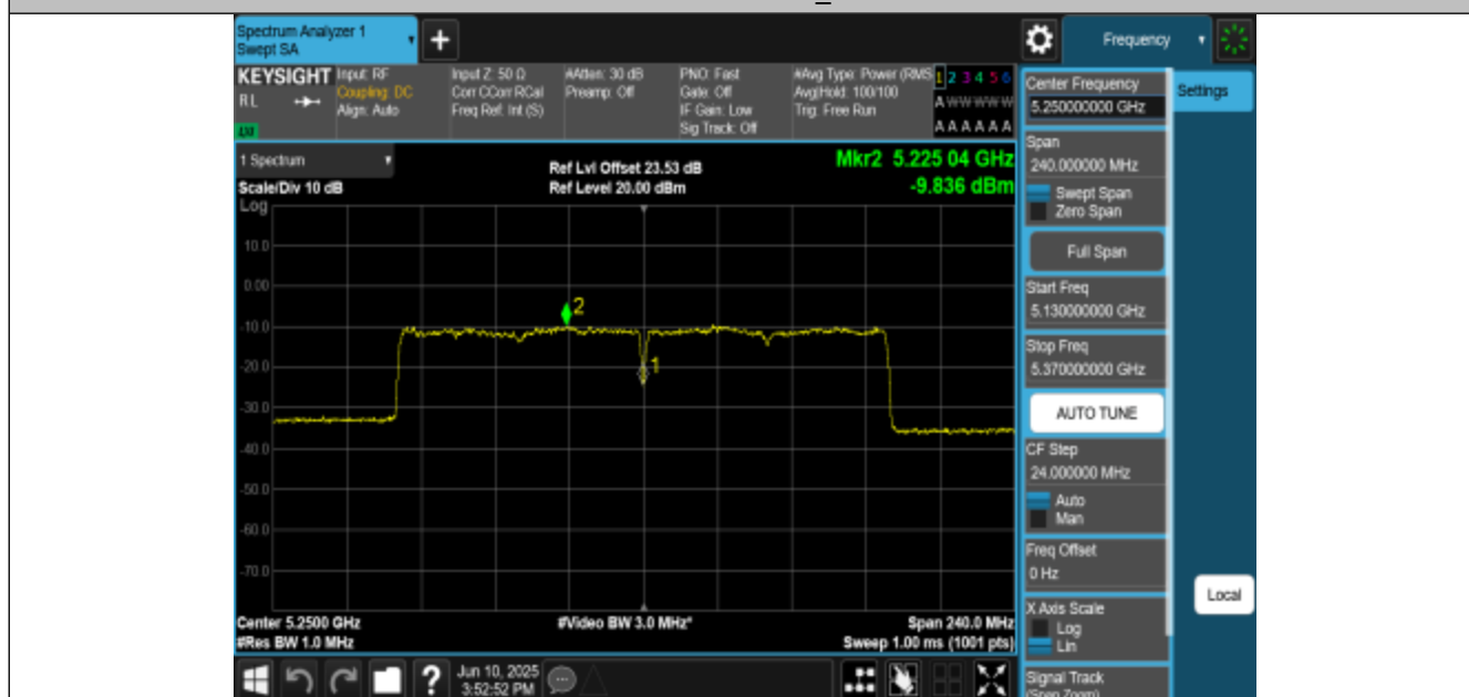
11BE160MIMO-Ant1-5250_U11-1-PASS
