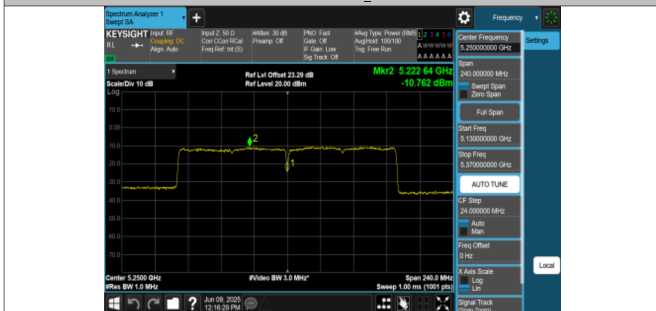
11AX160MIMO-Ant3-5250_UHII-1-PASS
