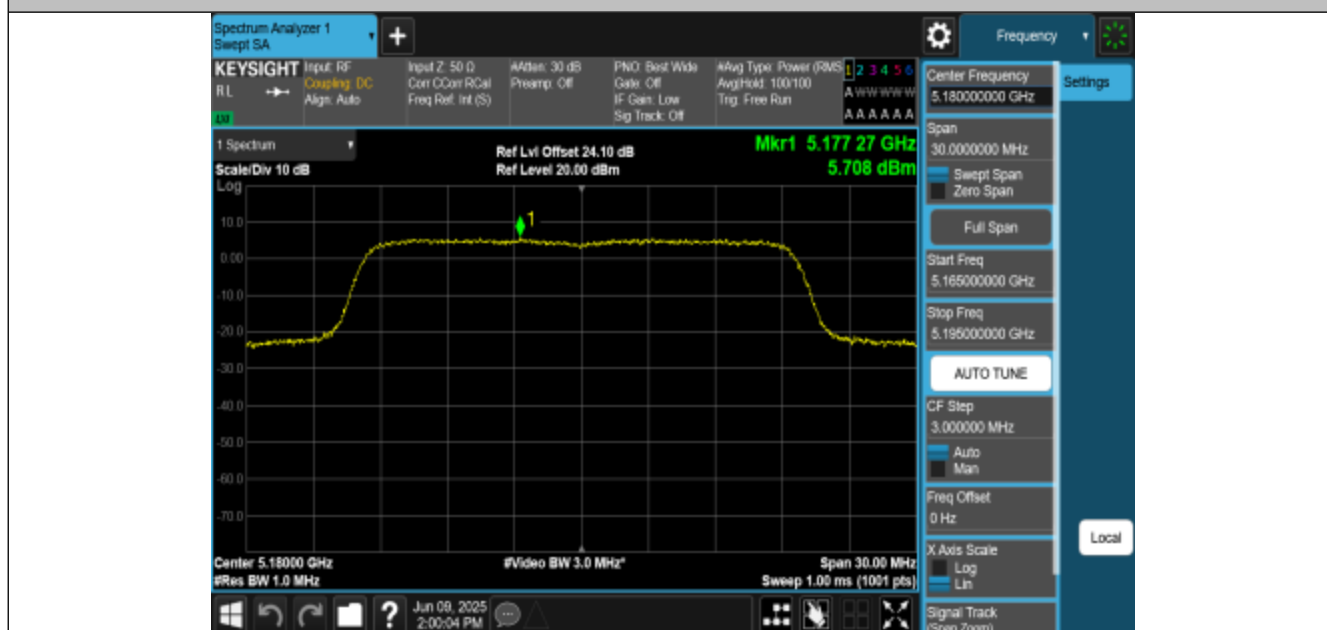
11BE20MIMO-Ant3-5180-PASS
