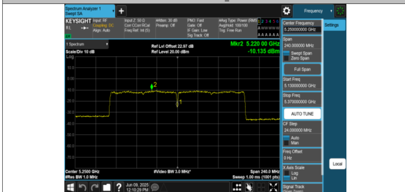
11AX160MIMO-Ant1-5250_UHII-1-PASS
