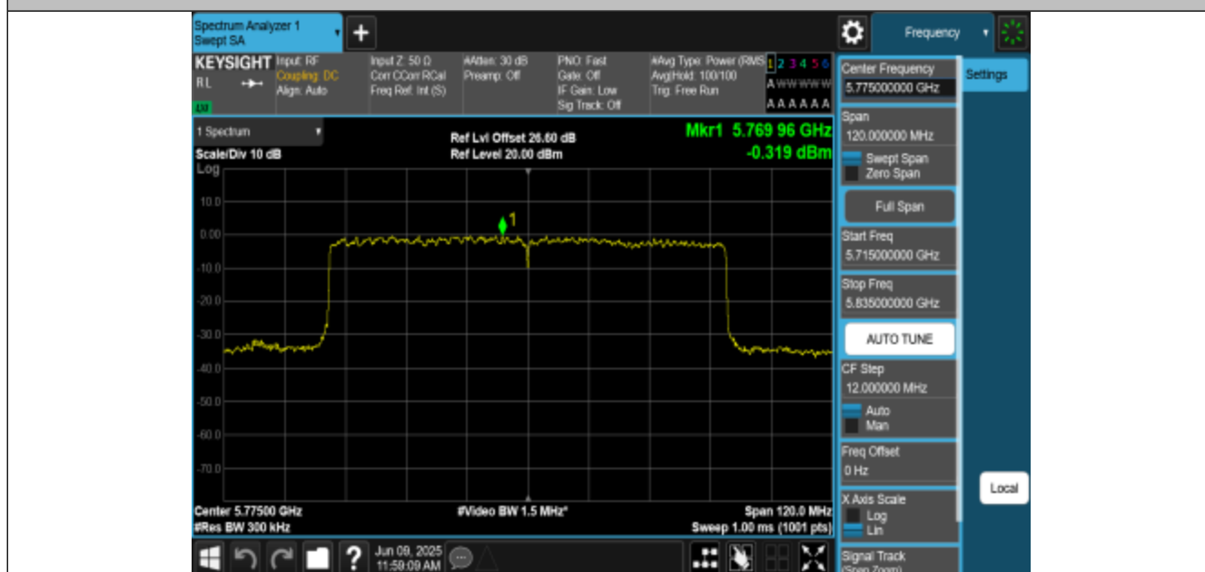
11AX80MIMO-Ant1-5775-PASS
