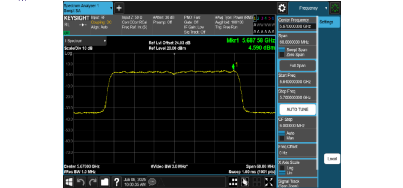
11AX40MIMO-Ant0-5670-PASS
