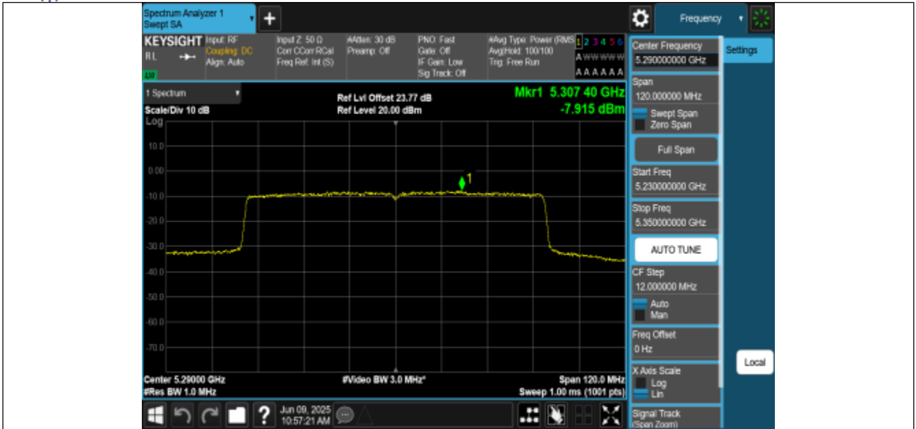
11AX80MIMO-Ant0-5290-PASS
