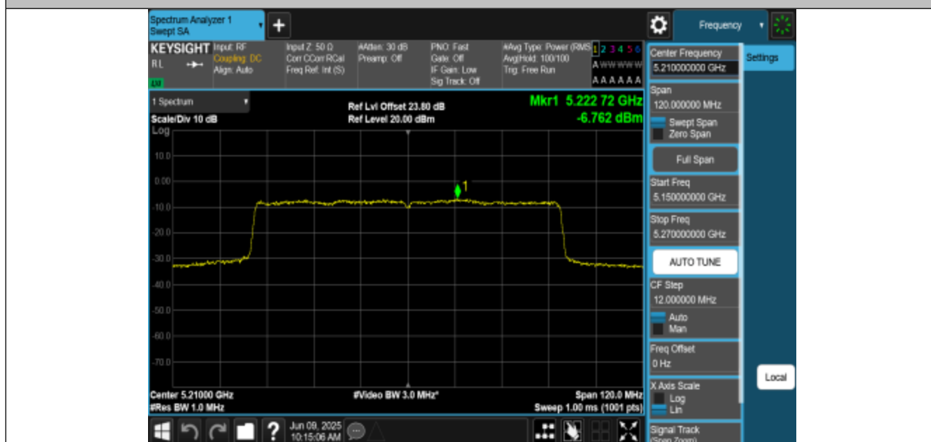
11AX80MIMO-Ant3-5210-PASS
