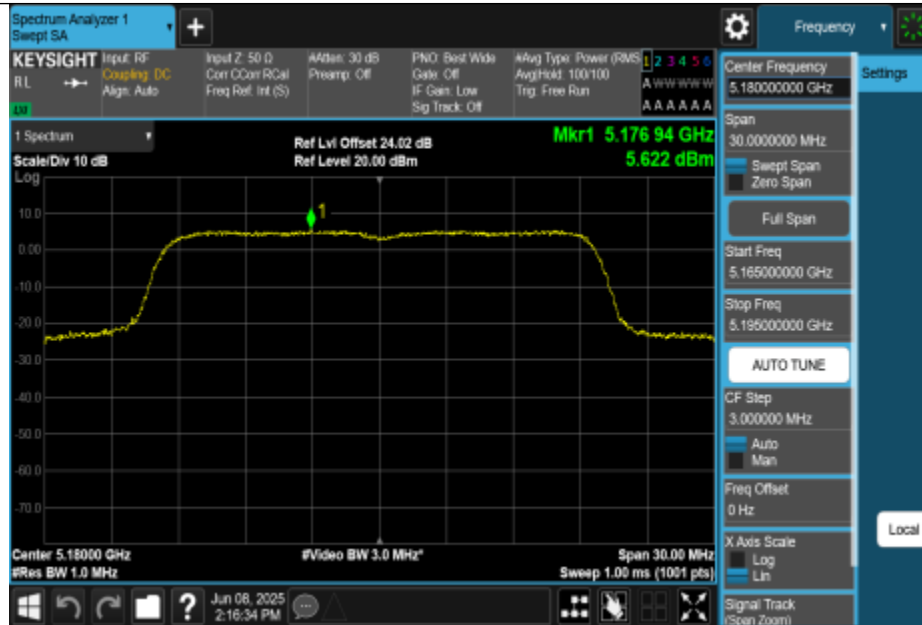
11AX20MIMO-Ant2-5180-PASS
