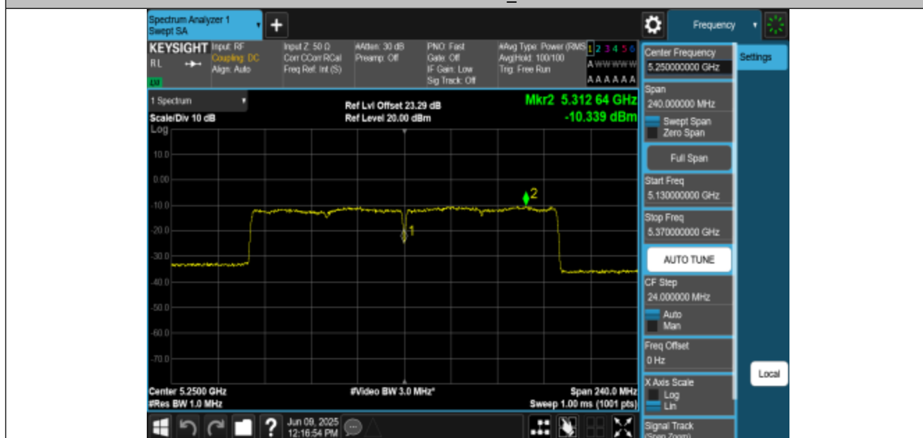
11AX160MIMO-Ant3-5250_UNII-2A-PASS
