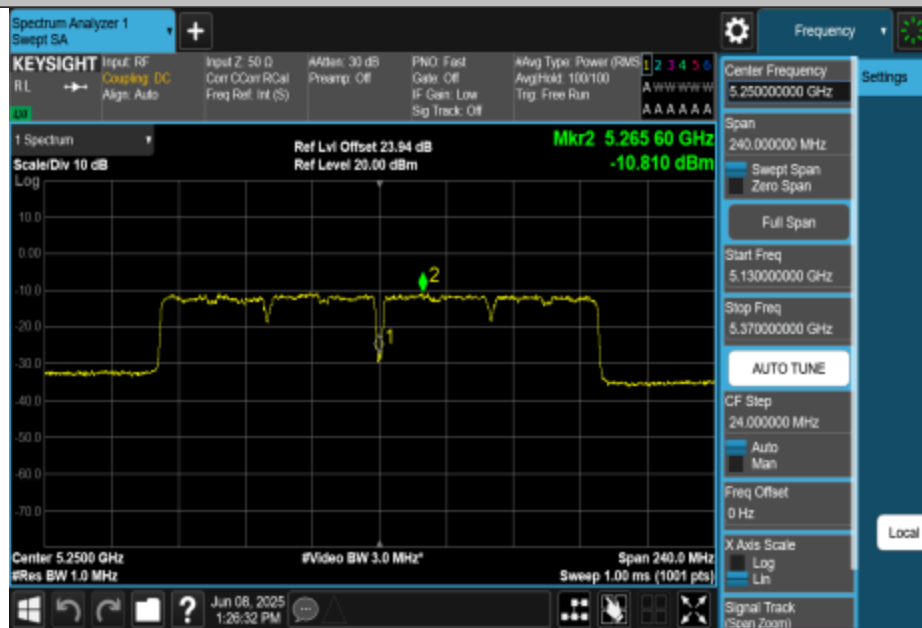
11AC160MIMO-Ant1-5250_UNII-2A-PASS
