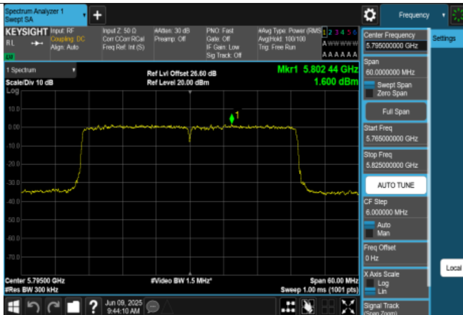
11AX40MIMO-Ant2-5795-PASS
