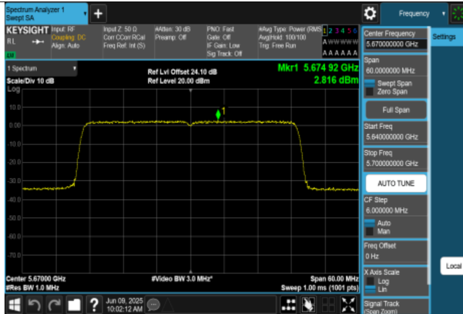
11AX40MIMO-Ant2-5670-PASS
