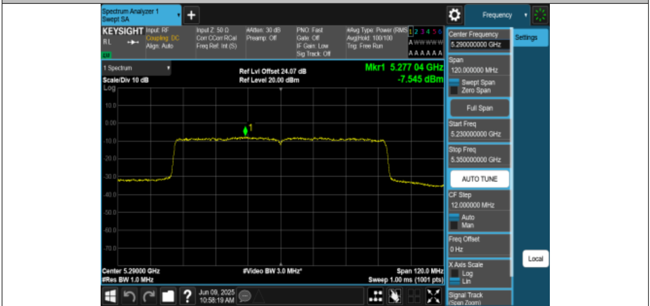
11AX80MIMO-Ant1-5290-PASS
