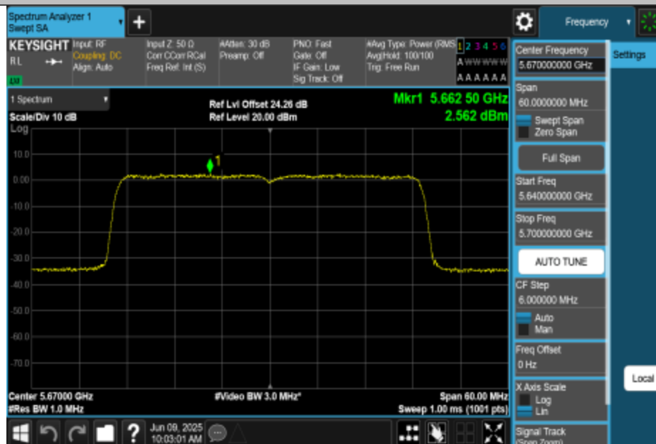
11AX40MIMO-Ant3-5670-PASS
