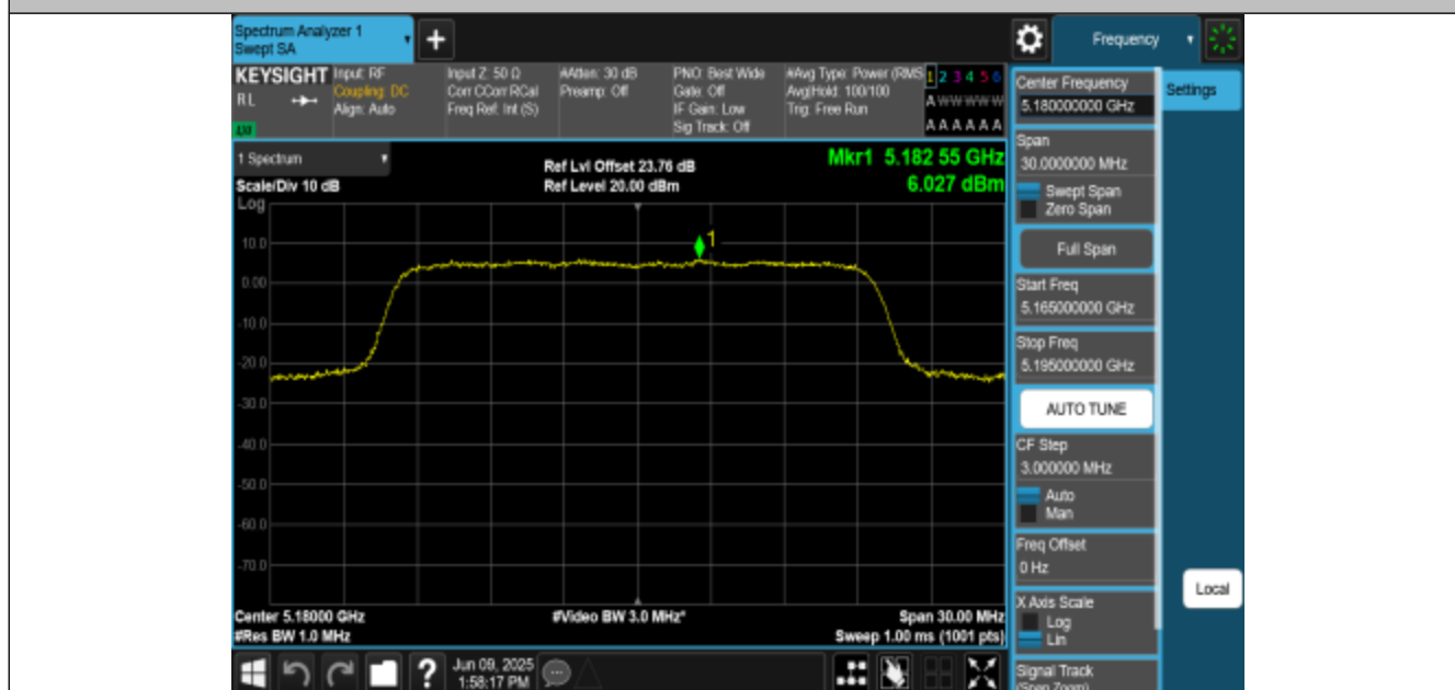
11BE20MIMO-Ant1-5180-PASS
