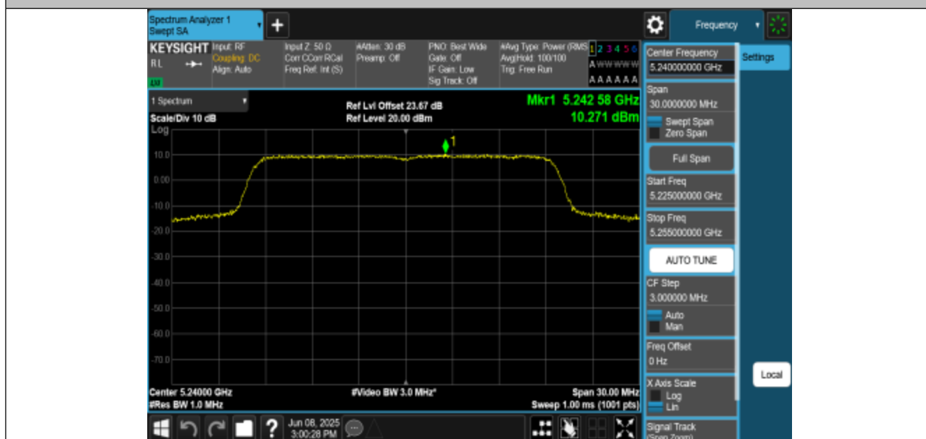
11AX20MIMO-Ant3-5240-PASS
