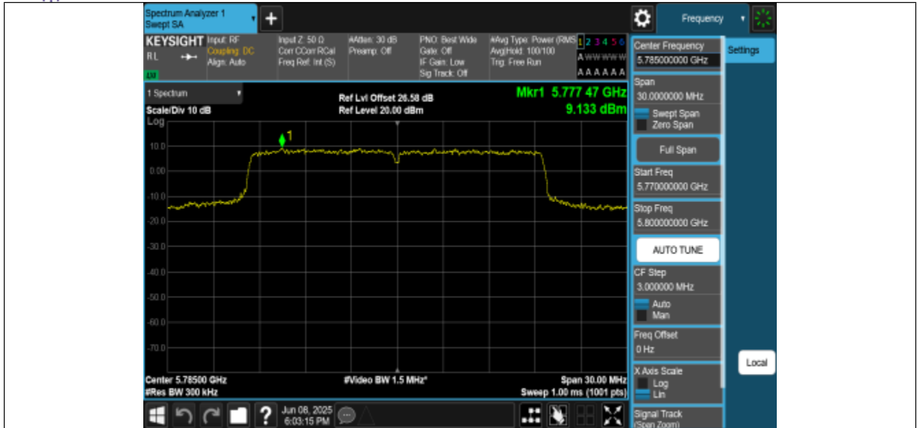
11AX20MIMO-Ant2-5785-PASS
