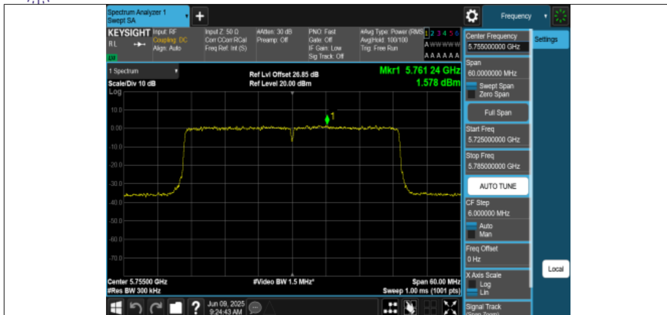
11AX40MIMO-Ant2-5755-PASS
