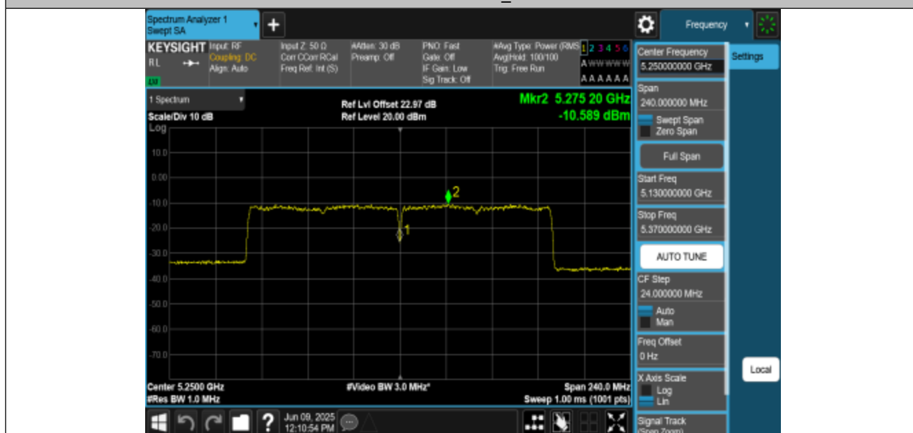
11AX160MIMO-Ant1-5250_UNII-2A-PASS
