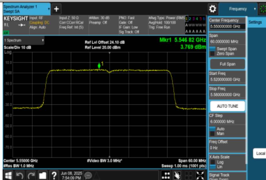
11AX40MIMO-Ant3-5550-PASS
