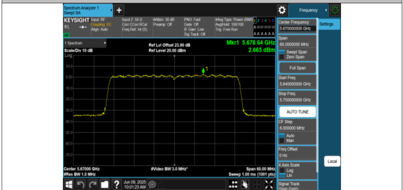
11AX40MIMO-Ant1-5670-PASS
