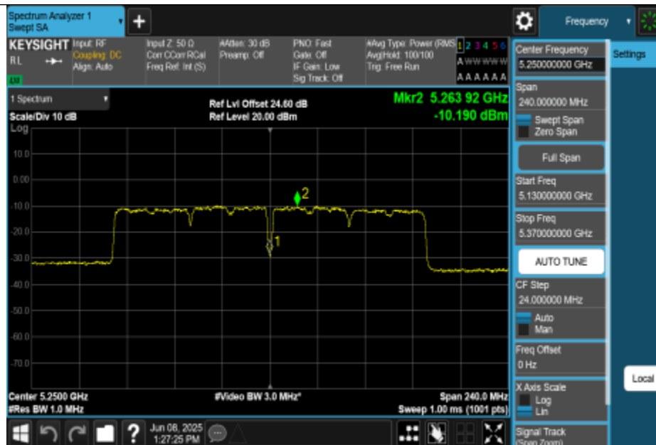
11AC160MIMO-Ant2-5250_UNII-2A-PASS
