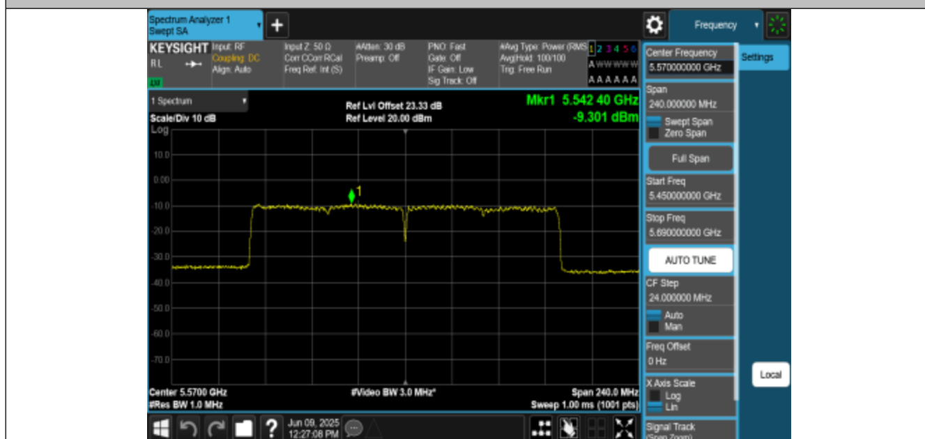
11AX160MIMO-Ant1-5570-PASS
