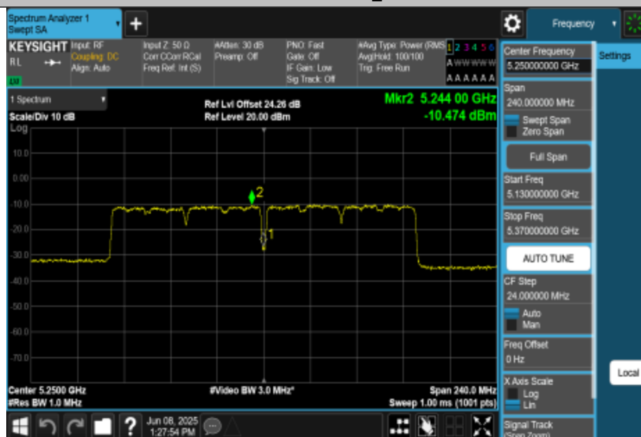
11AC160MIMO-Ant3-5250_UNII-1-PASS
