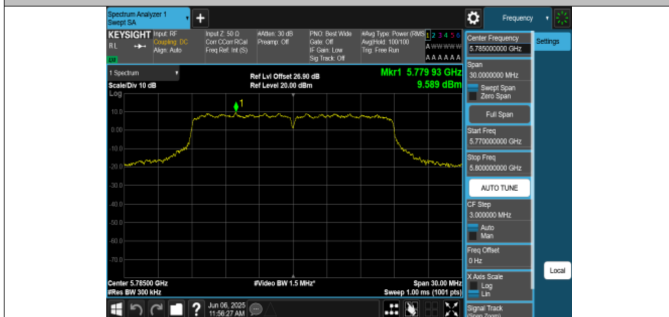
11AC20MIMO-Ant3-5785-PASS
