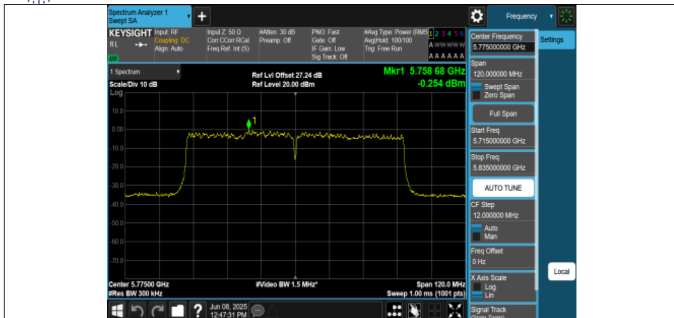
11AC80MIMO-Ant0-5775-PASS
