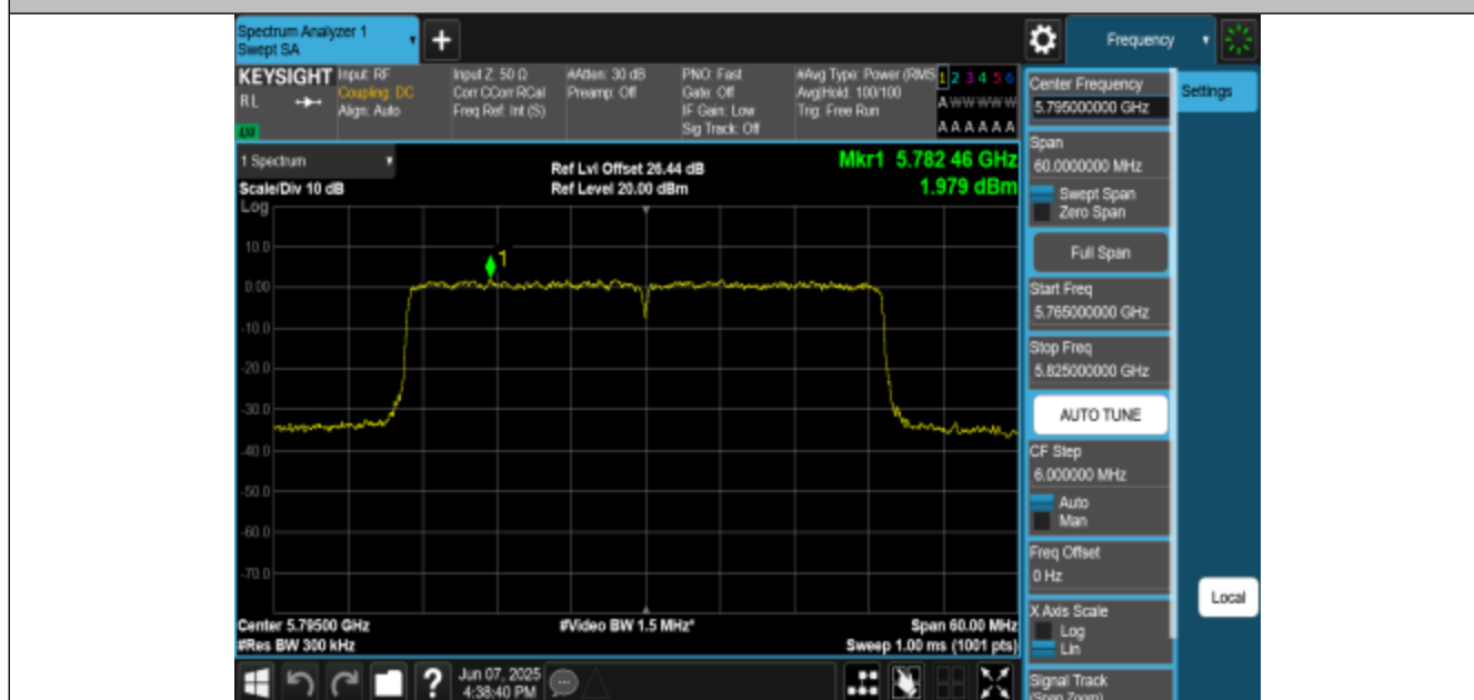
11AC40MIMO-Ant1-5795-PASS
