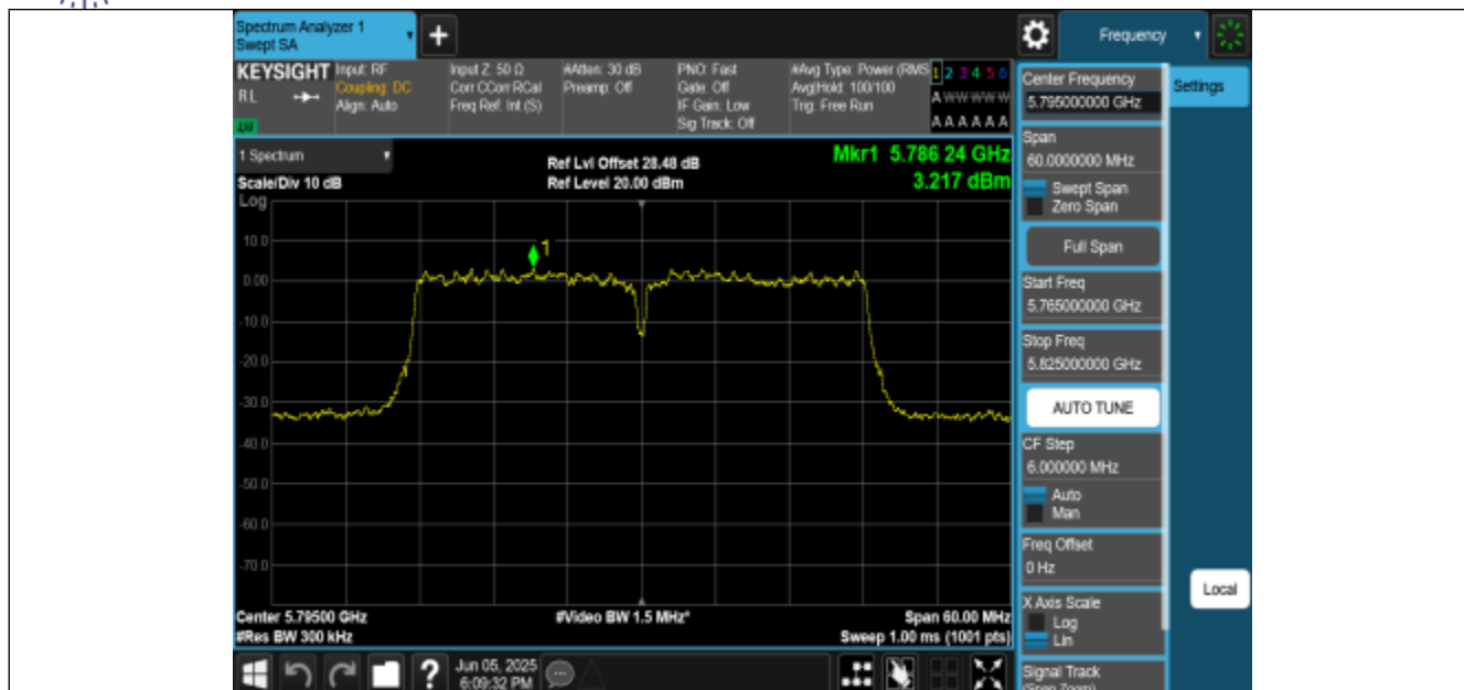
11N40MIMO-Ant0-5795-PASS
