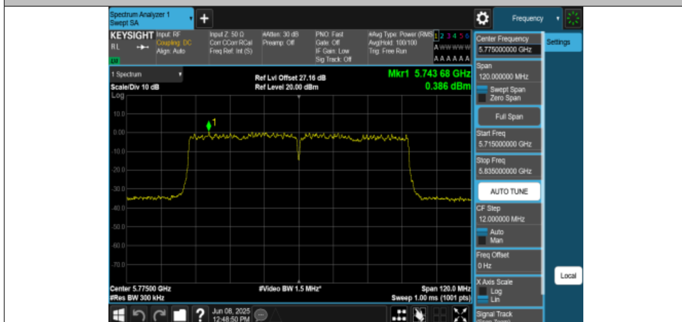
11AC80MIMO-Ant1-5775-PASS
