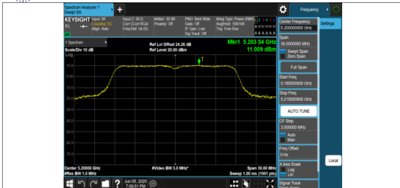
11AC20MIMO-Ant2-5200-PASS
