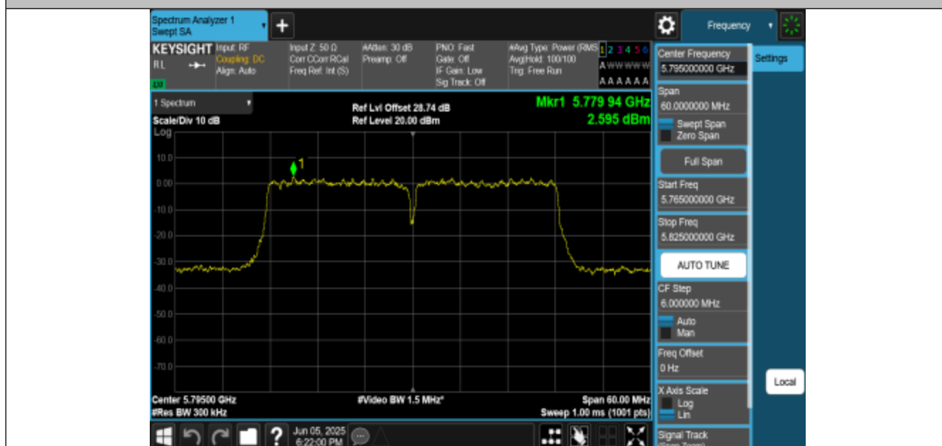
11N40MIMO-Ant3-5795-PASS
