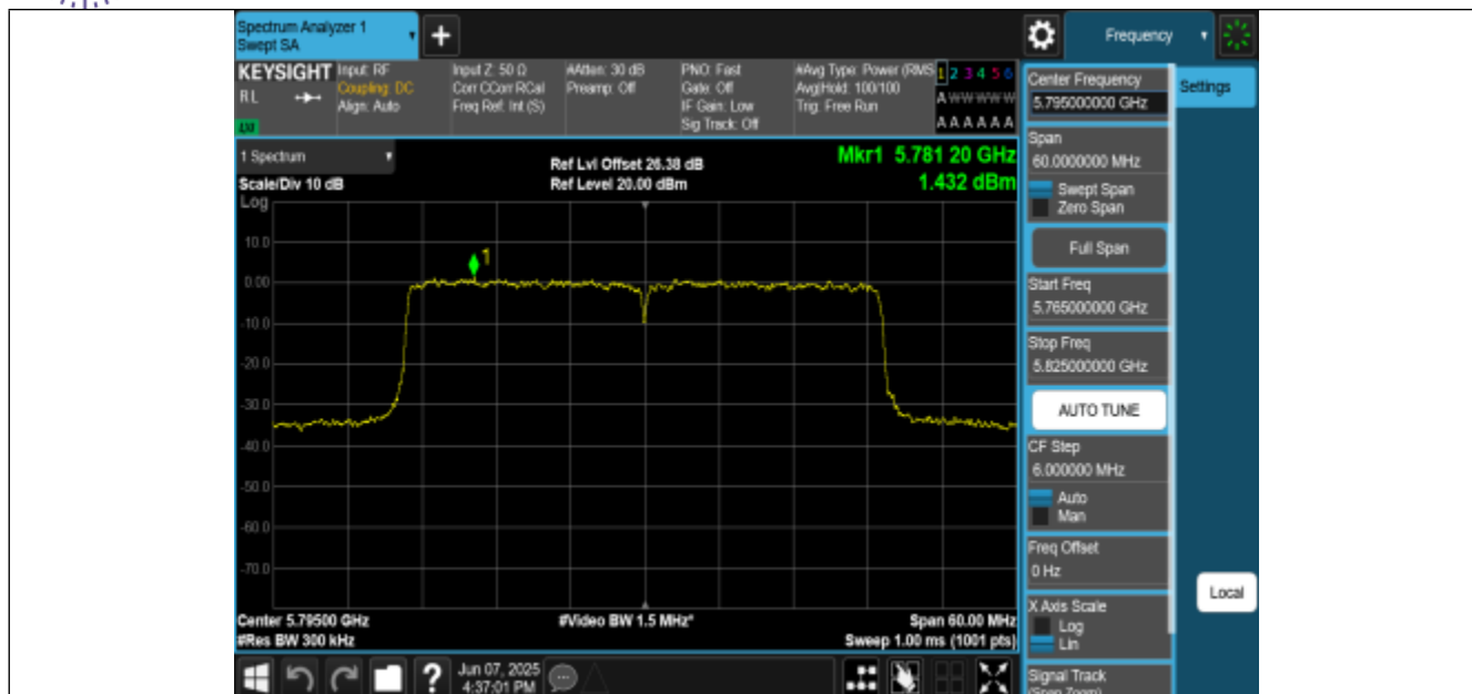
11AC40MIMO-Ant0-5795-PASS
