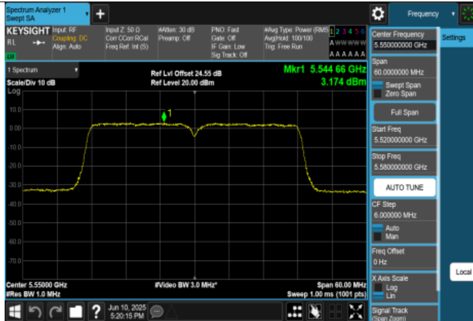
11AC40MIMO-Ant2-5550-PASS
