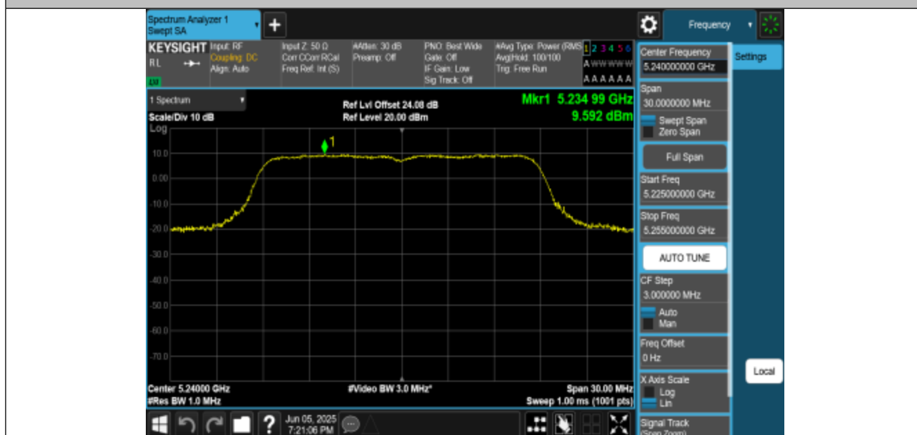
11AC20MIMO-Ant3-5240-PASS
