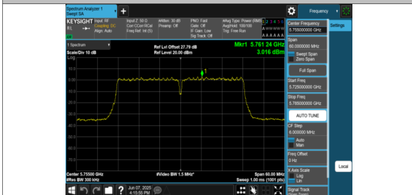
11AC40MIMO-Ant3-5755-PASS
