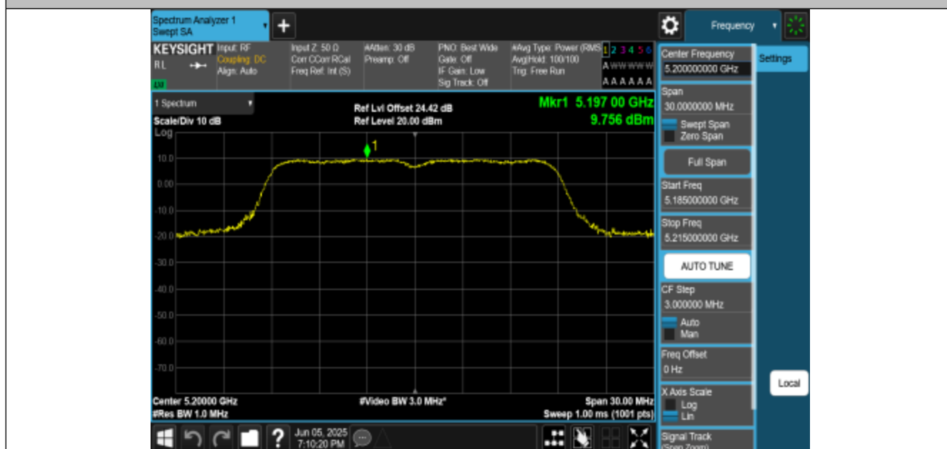
11AC20MIMO-Ant3-5200-PASS
