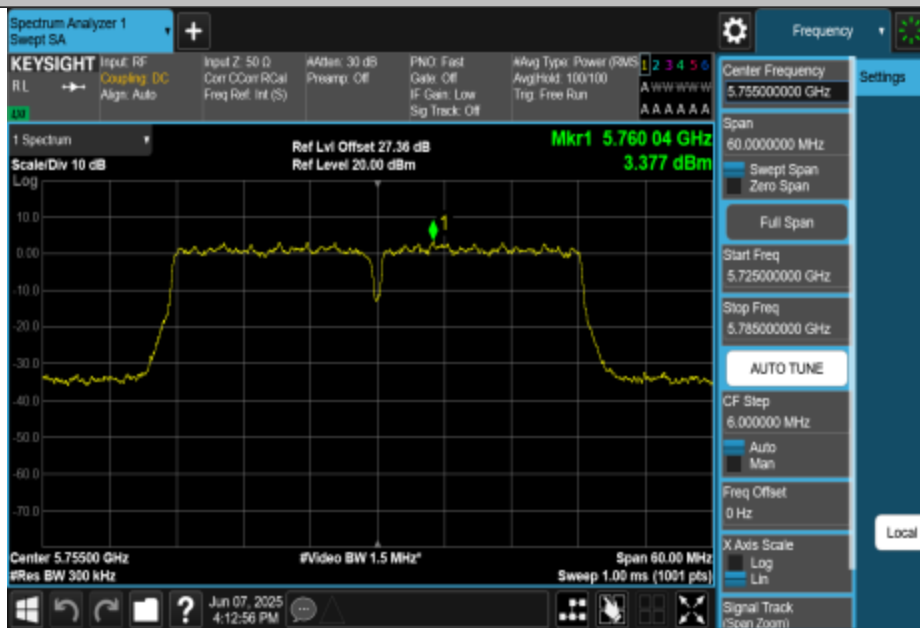
11AC40MIMO-Ant1-5755-PASS
