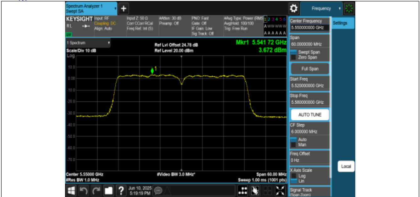
11AC40MIMO-Ant0-5550-PASS
