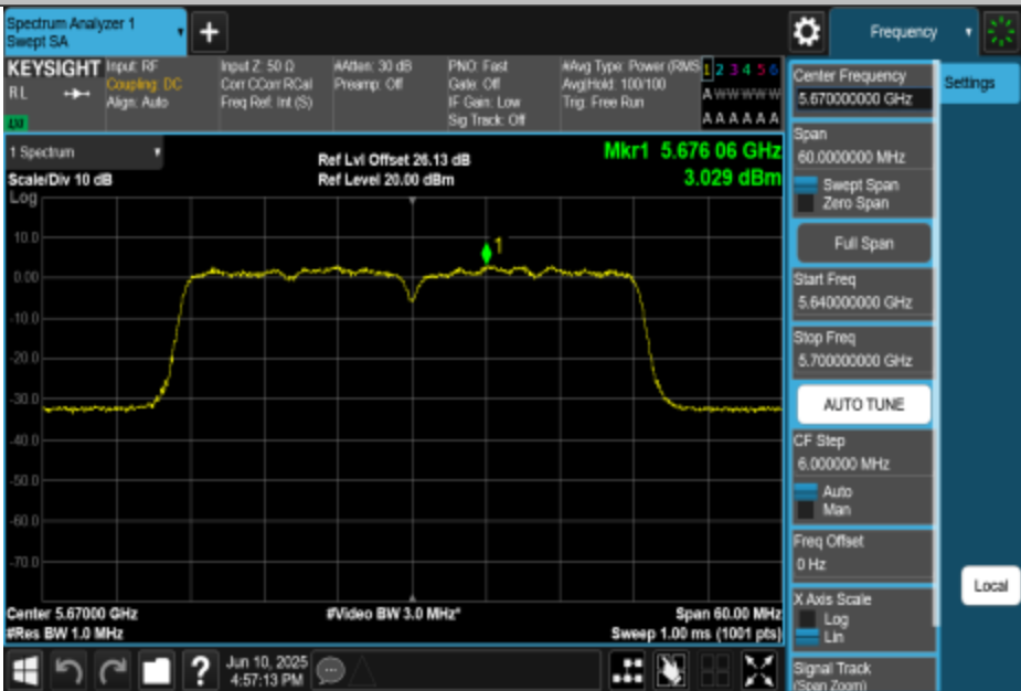
11N40MIMO-Ant1-5670-PASS
