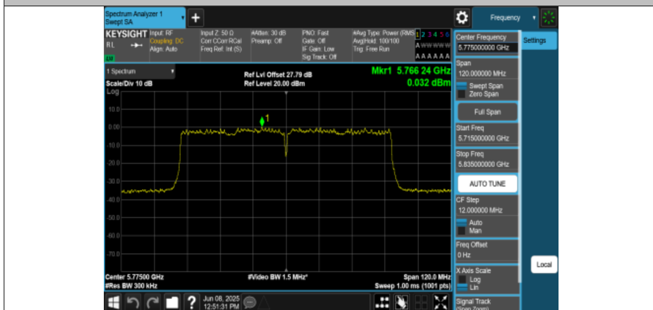
11AC80MIMO-Ant3-5775-PASS
