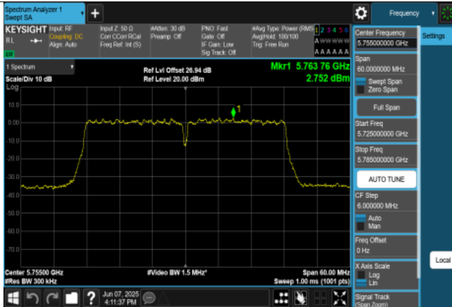
11AC40MIMO-Ant0-5755-PASS
