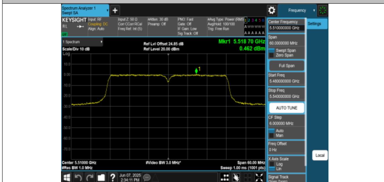
11AC40MIMO-Ant3-5510-PASS
