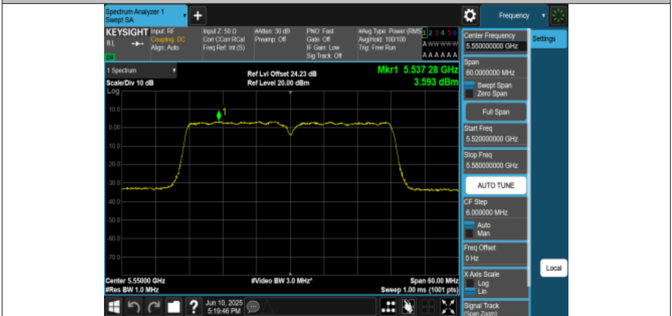
11AC40MIMO-Ant1-5550-PASS
