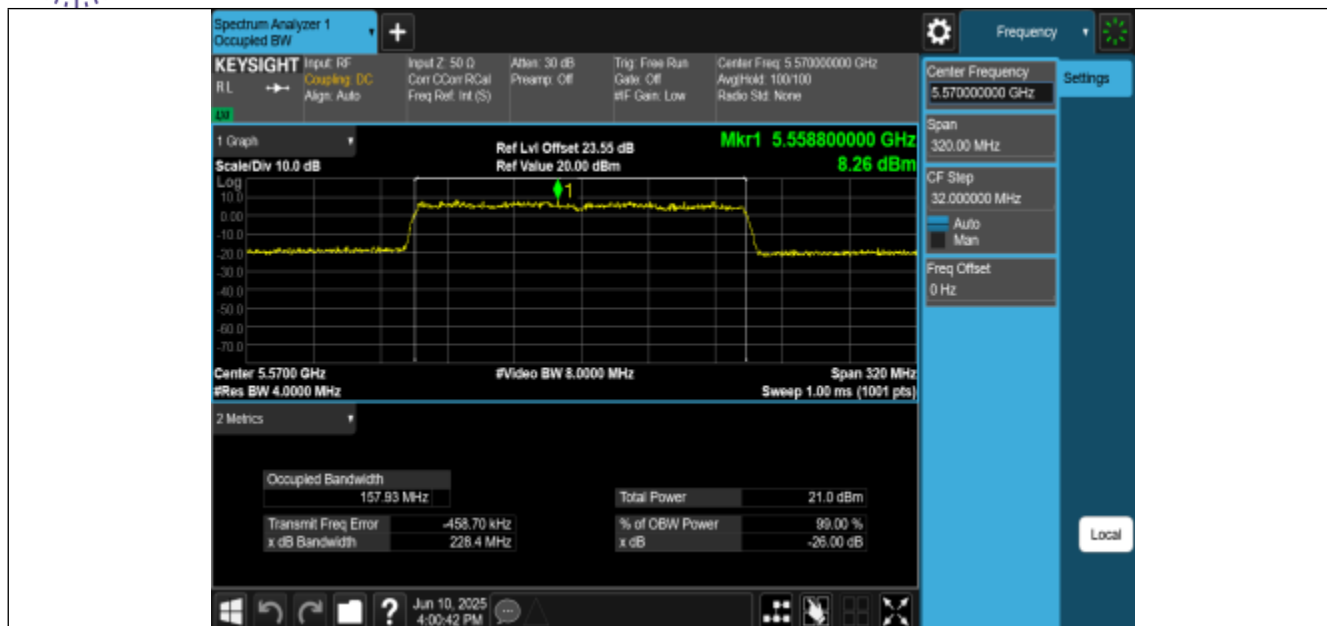
11BE160MIMO-Ant0-5570
