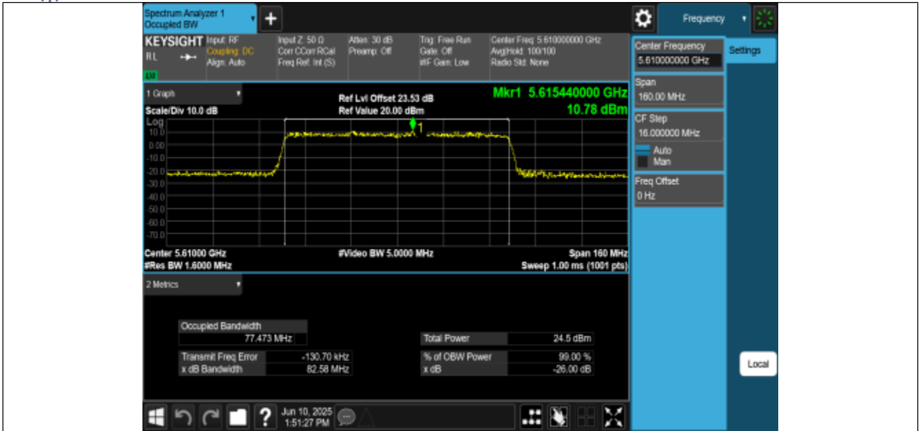
11BE80MIMO-Ant2-5610
