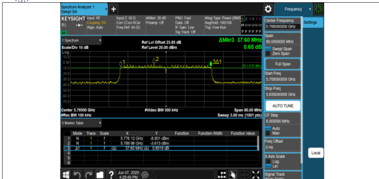
11AC40MIMO-Ant2-5795-PASS
