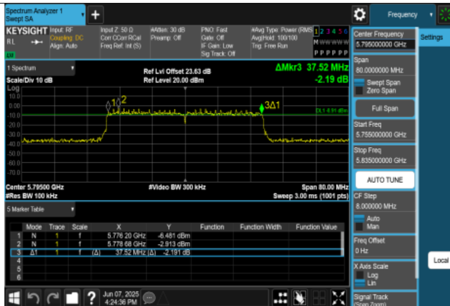
11AC40MIMO-Ant0-5795-PASS
