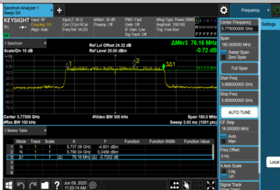
11AX80MIMO-Ant3-5775-PASS
