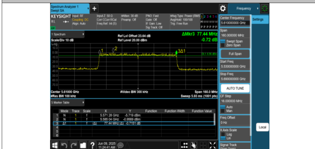
11AX80MIMO-Ant3-5610-PASS
