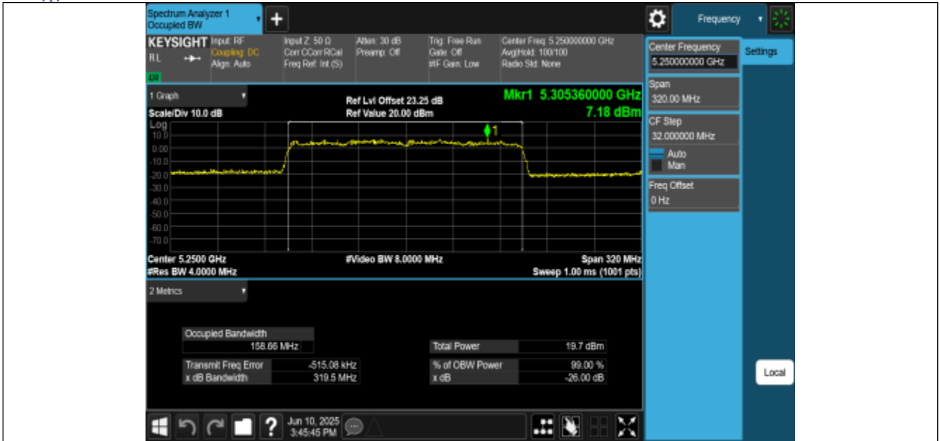
11BE160MIMO-Ant2-5250
