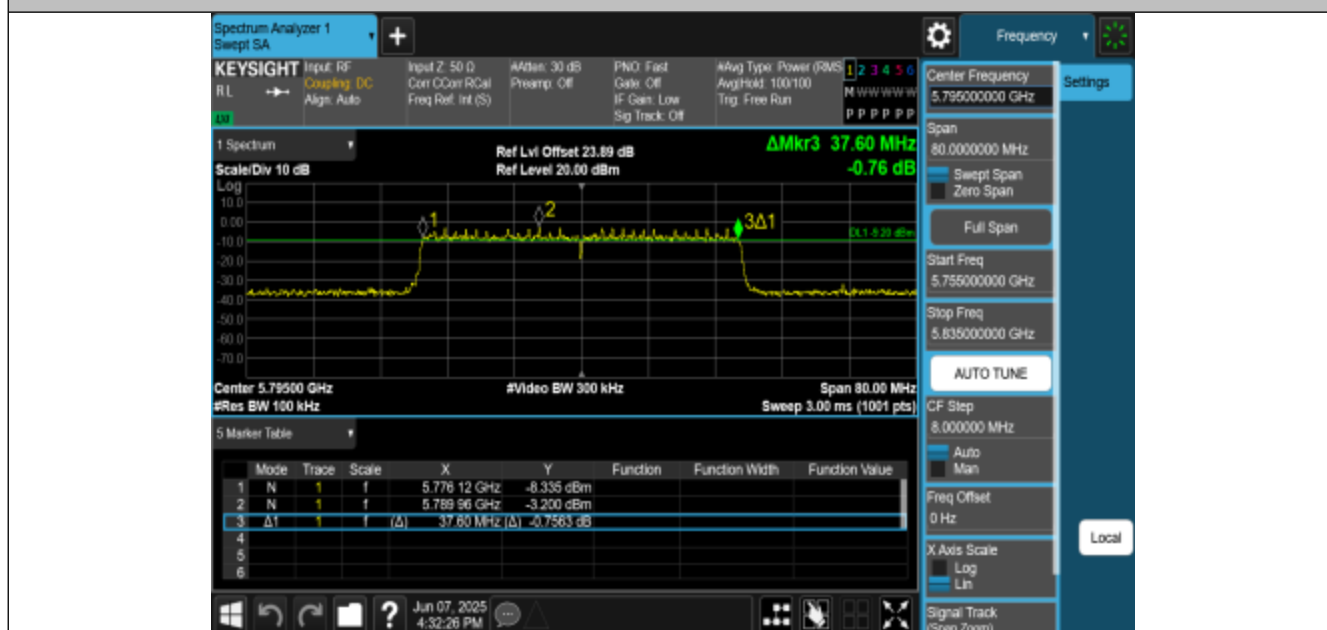
11AC40MIMO-Ant3-5795-PASS
