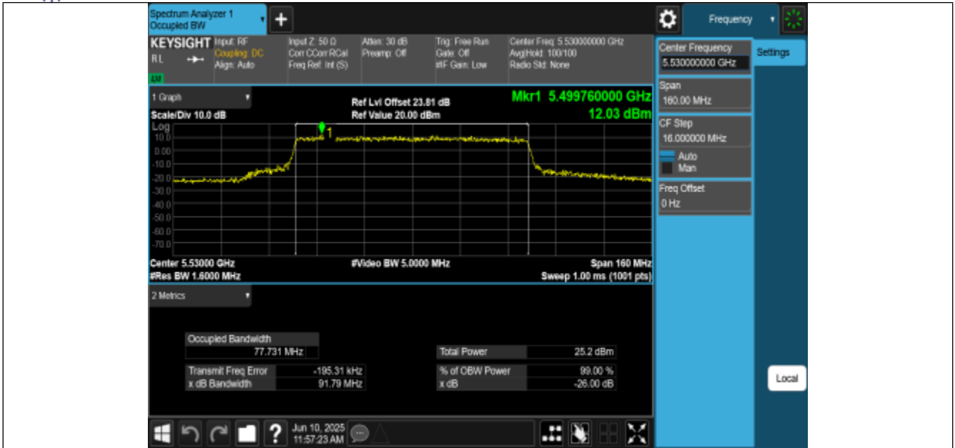
11BE80MIMO-Ant2-5530
