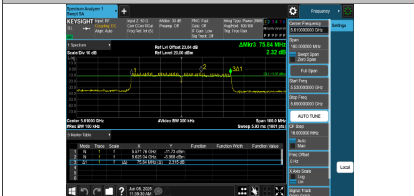
11AC80MIMO-Ant3-5610-PASS
