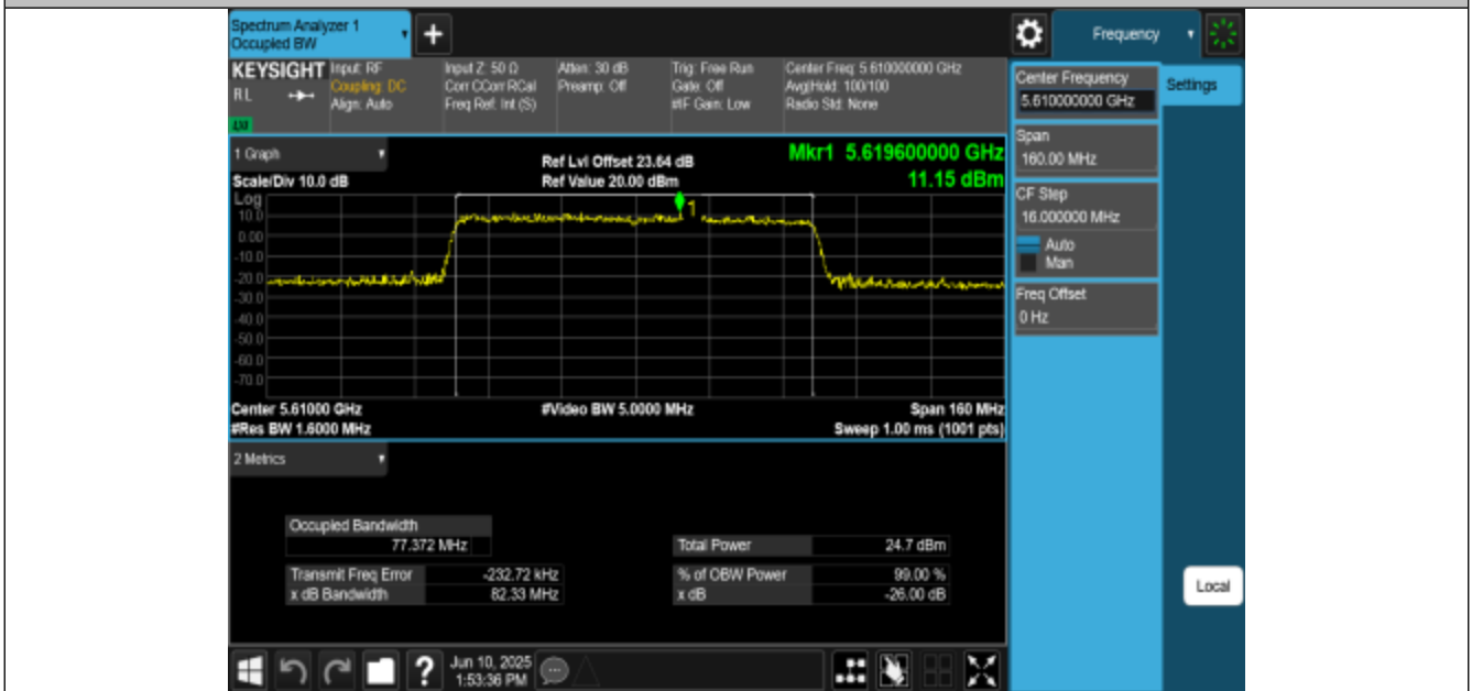
11BE80MIMO-Ant3-5610
