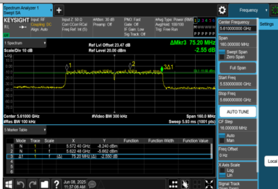
11AC80MIMO-Ant1-5610-PASS
