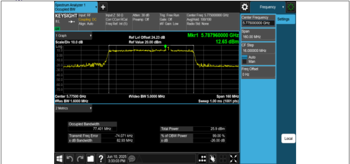
11BE80MIMO-Ant2-5775
