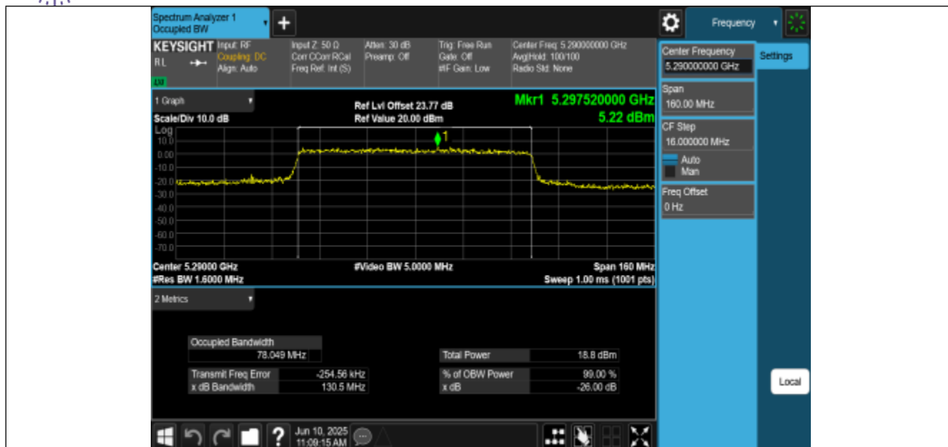
11BE80MIMO-Ant2-5290
