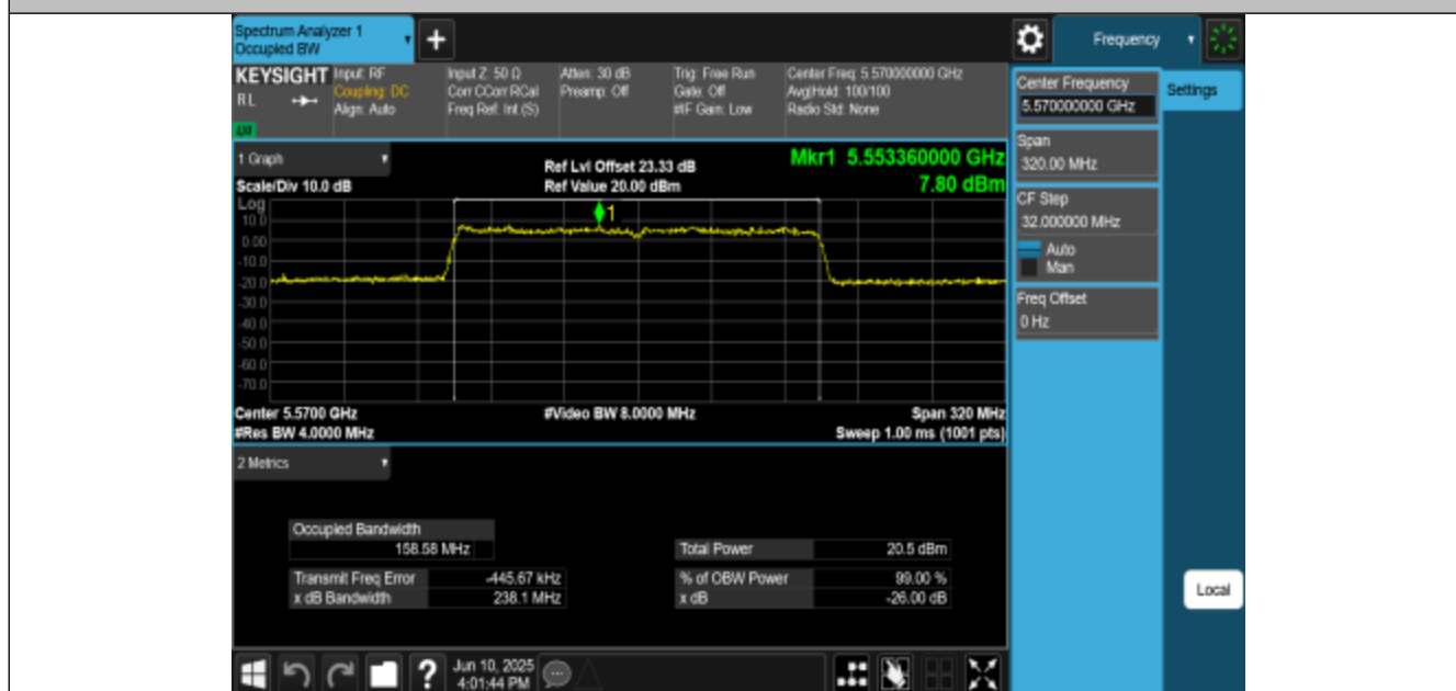
11BE160MIMO-Ant1-5570
