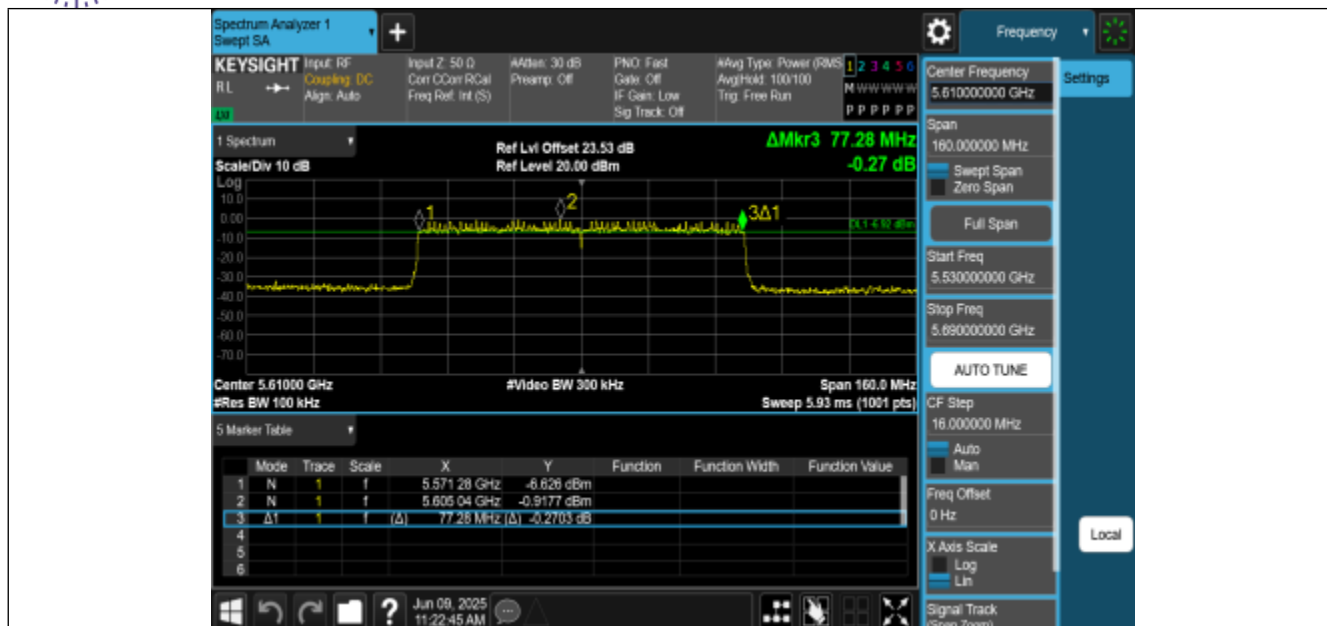
11AX80MIMO-Ant2-5610-PASS
