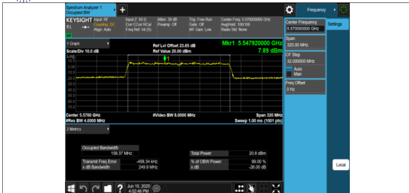
11BE160MIMO-Ant2-5570
