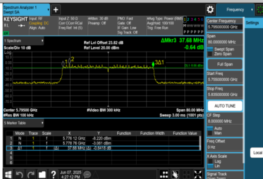
11AC40MIMO-Ant1-5795-PASS
