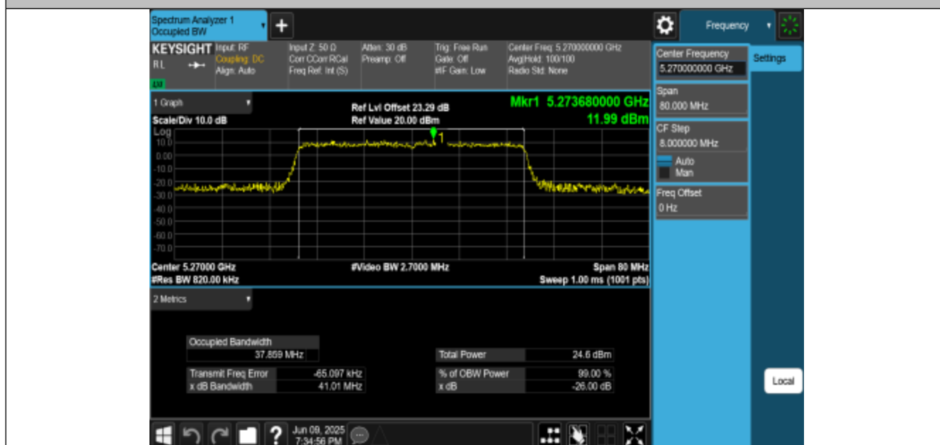
11BE40MIMO-Ant3-5270
