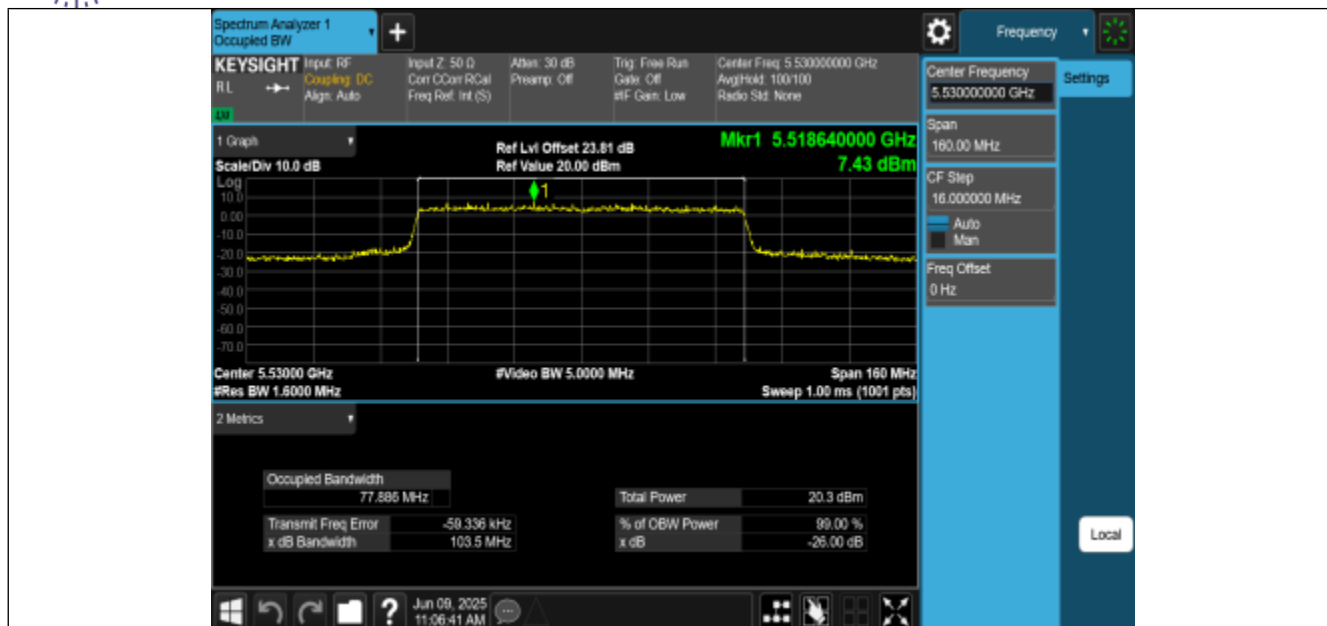
11AX80MIMO-Ant2-5530
