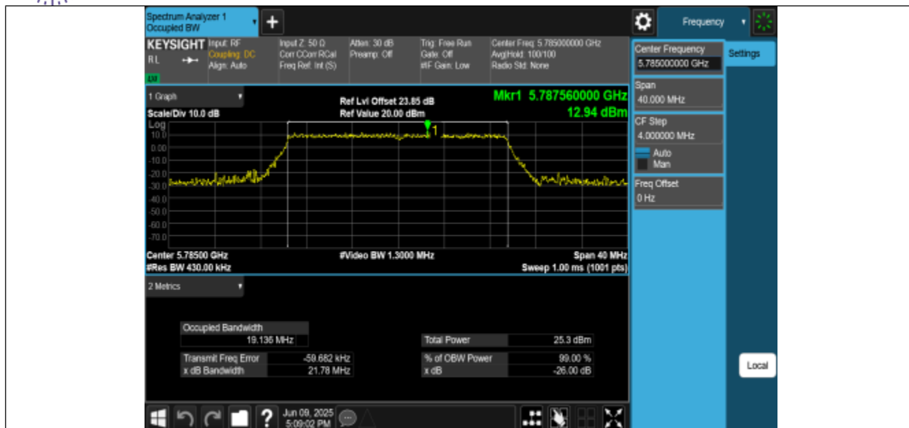
11BE20MIMO-Ant2-5785
