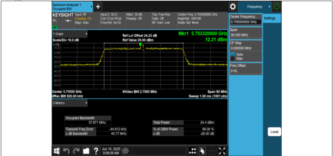
11BE40MIMO-Ant2-5755
