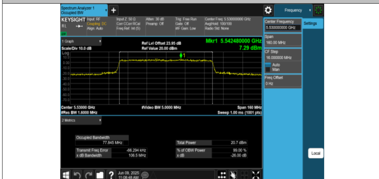
11AX80MIMO-Ant3-5530
