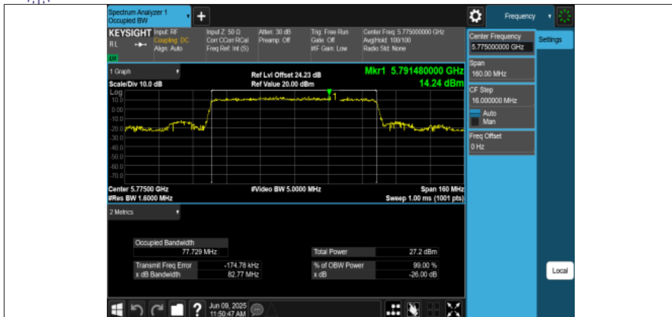
11AX80MIMO-Ant2-5775
