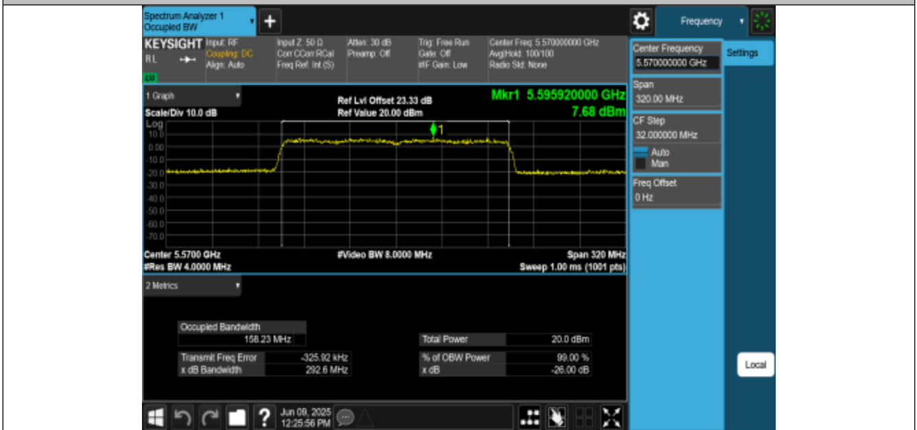
11AX160MIMO-Ant1-5570
