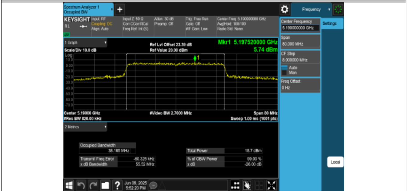
11BE40MIMO-Ant3-5190
