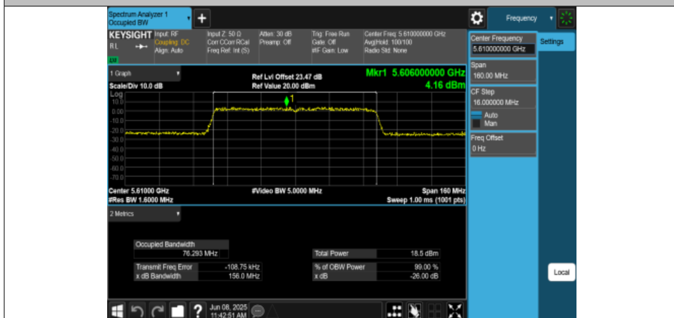
11AC80MIMO-Ant1-5610
