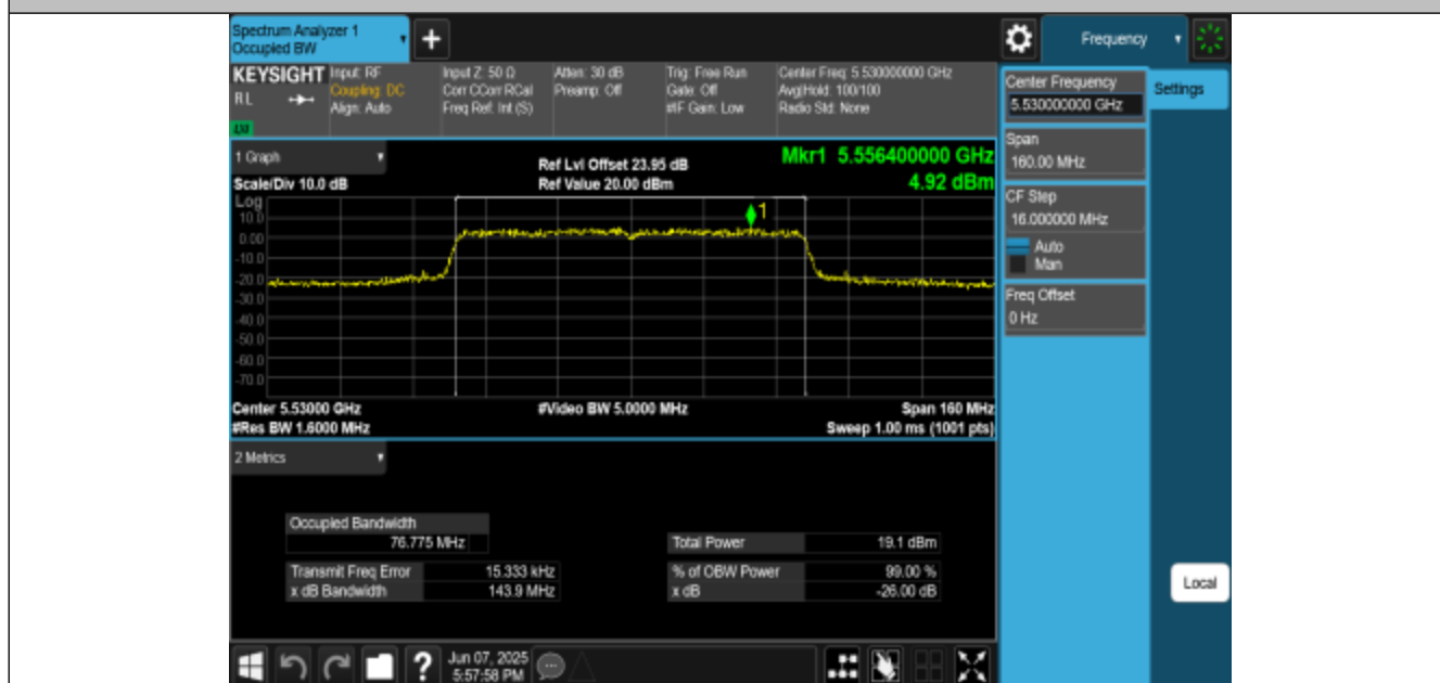
11AC80MIMO-Ant3-5530
