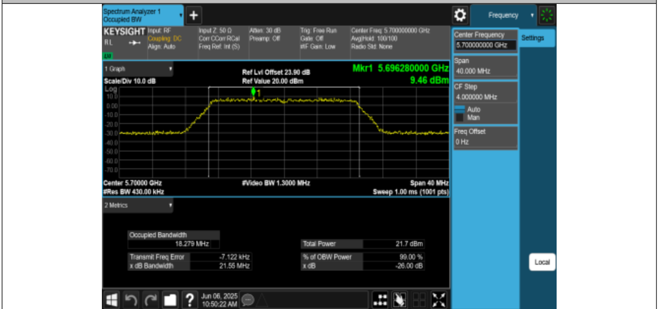
11AC20MIMO-Ant3-5700
