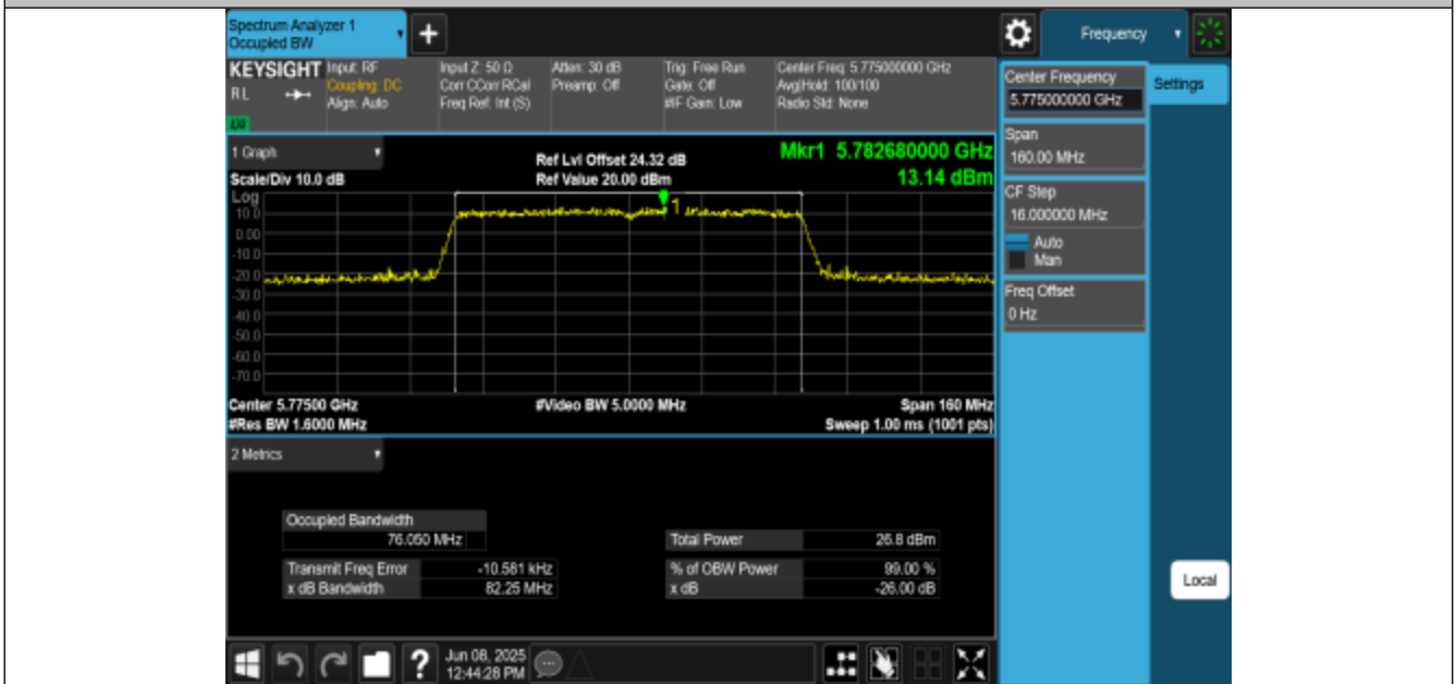
11AC80MIMO-Ant3-5775
