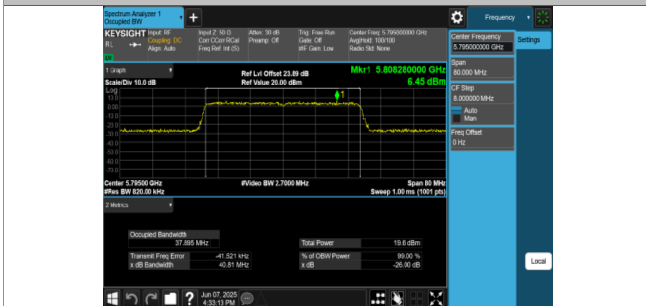
11AC40MIMO-Ant3-5795
