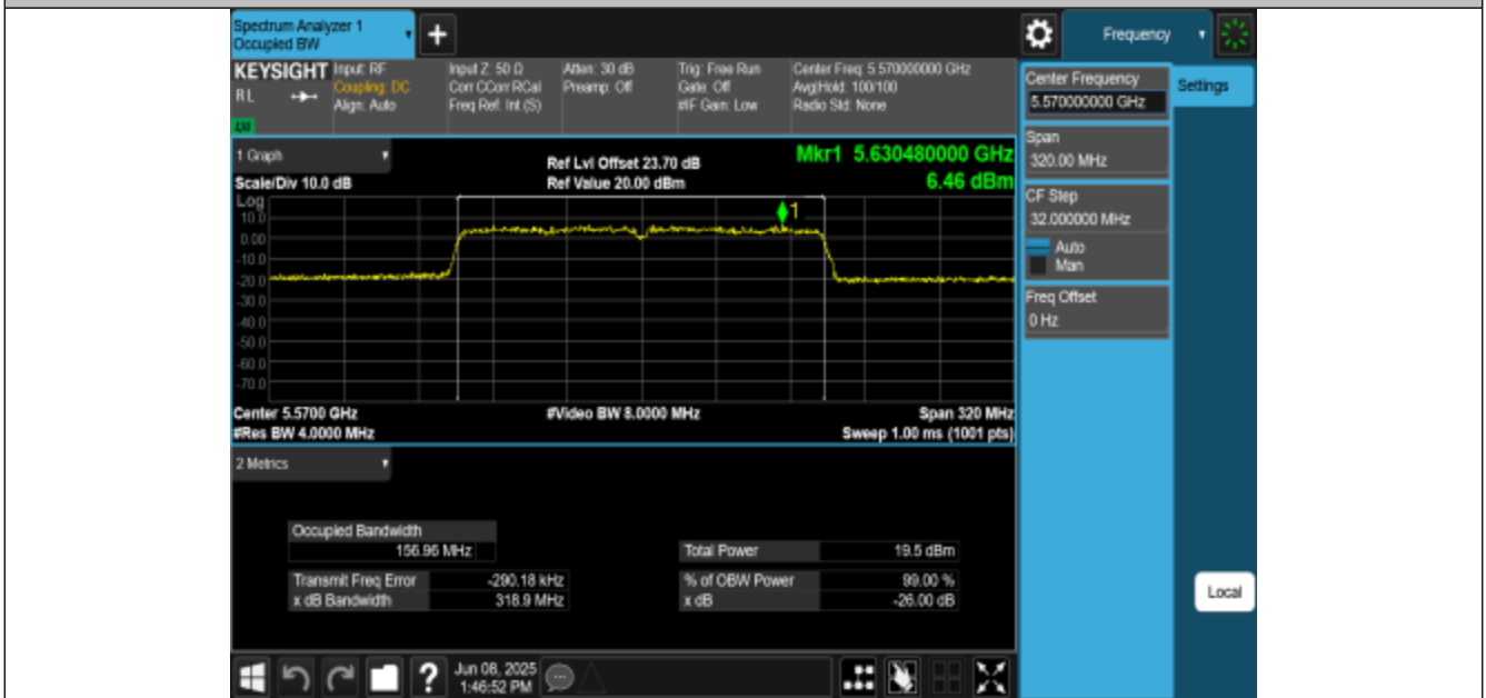
11AC160MIMO-Ant3-5570
