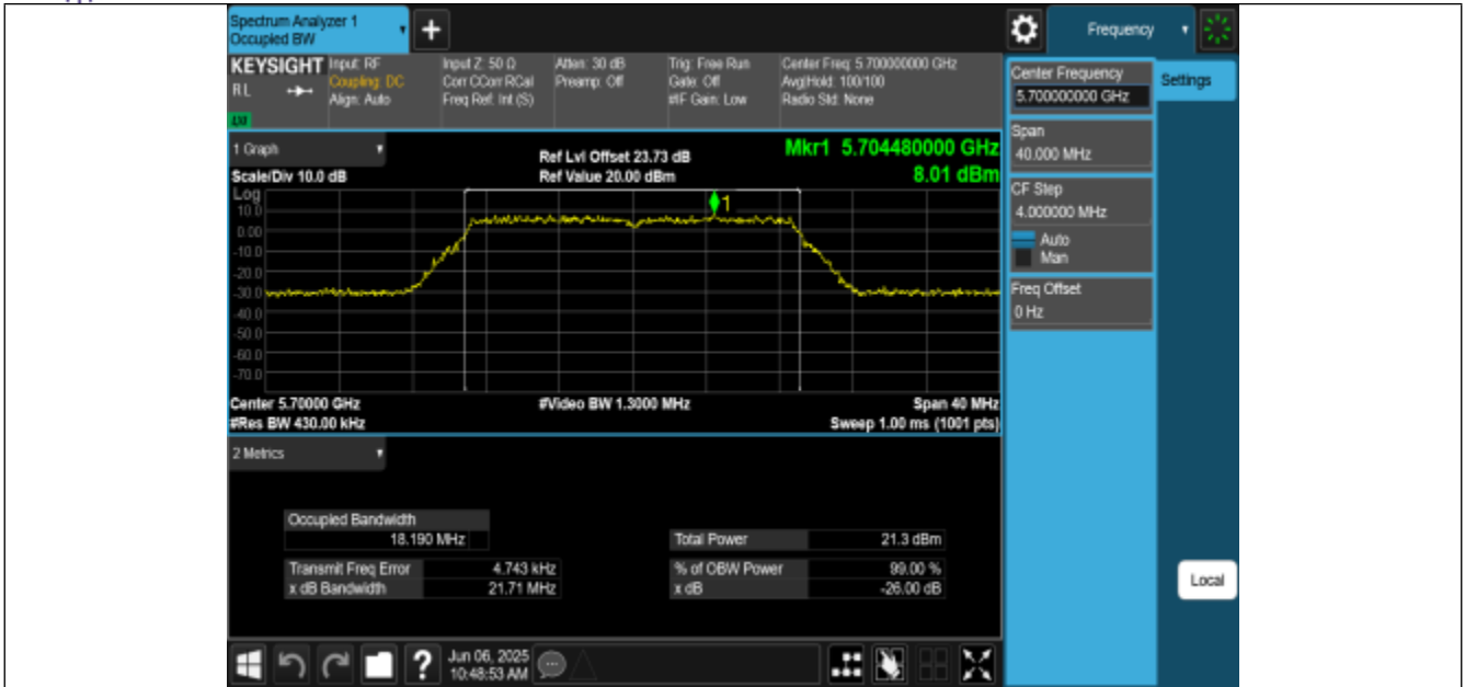
11AC20MIMO-Ant2-5700
