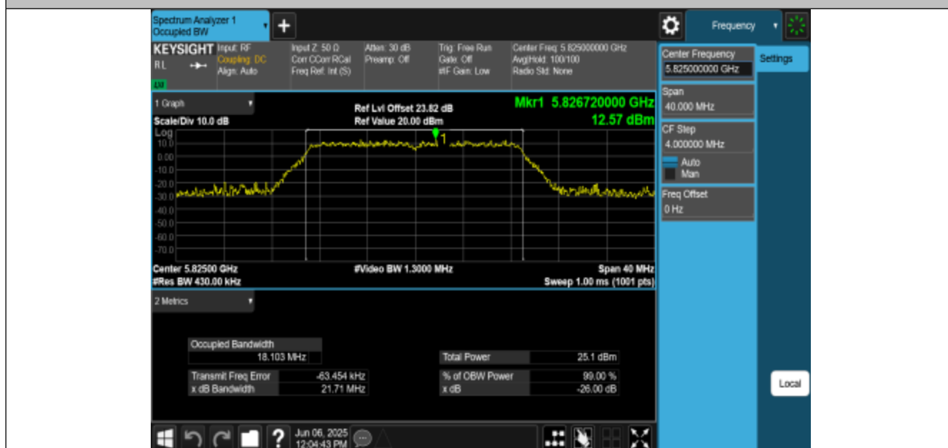
11AC20MIMO-Ant1-5825
