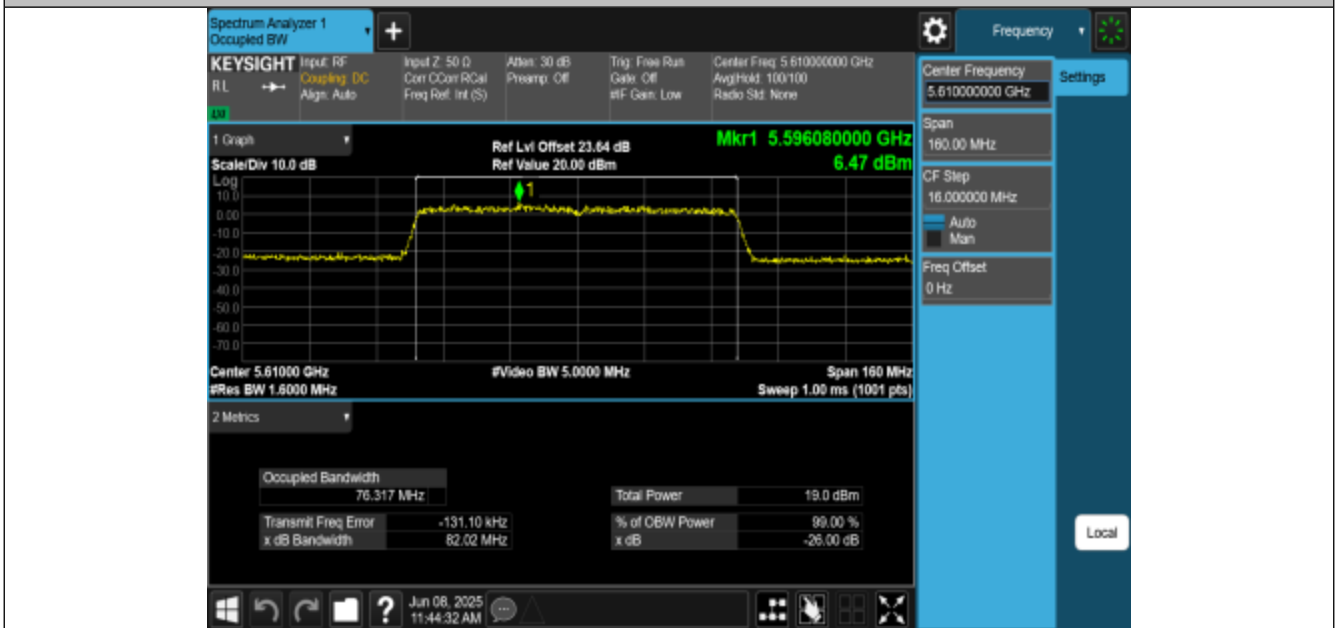
11AC80MIMO-Ant3-5610
