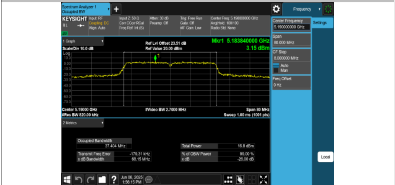
11AC40MIMO-Ant1-5190
