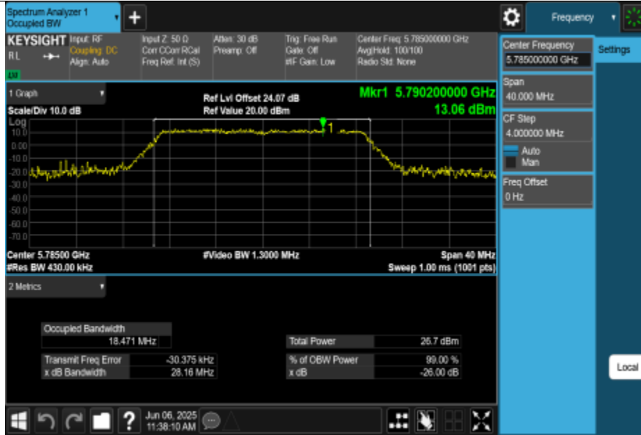
11AC20MIMO-Ant0-5785
