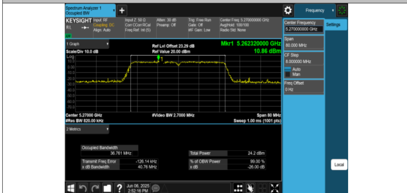
11AC40MIMO-Ant3-5270
