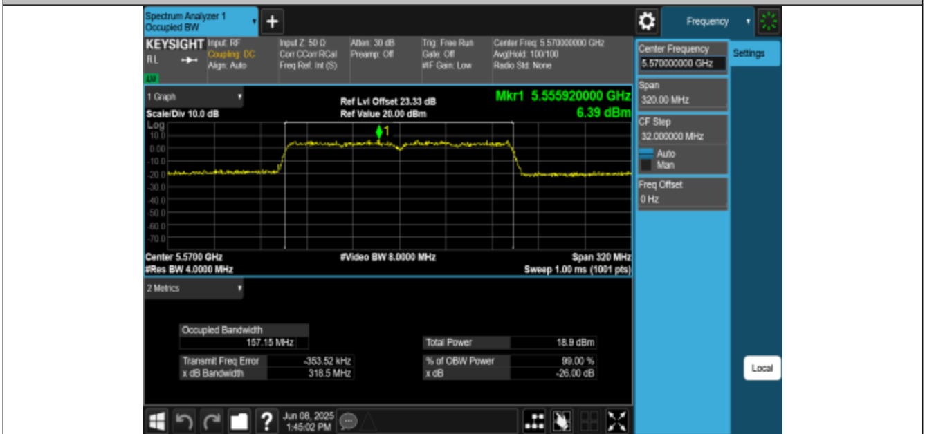
11AC160MIMO-Ant1-5570
