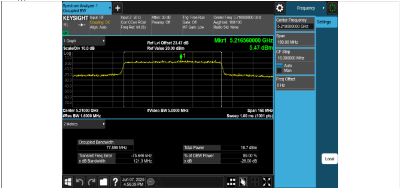
11AC80MIMO-Ant2-5210
