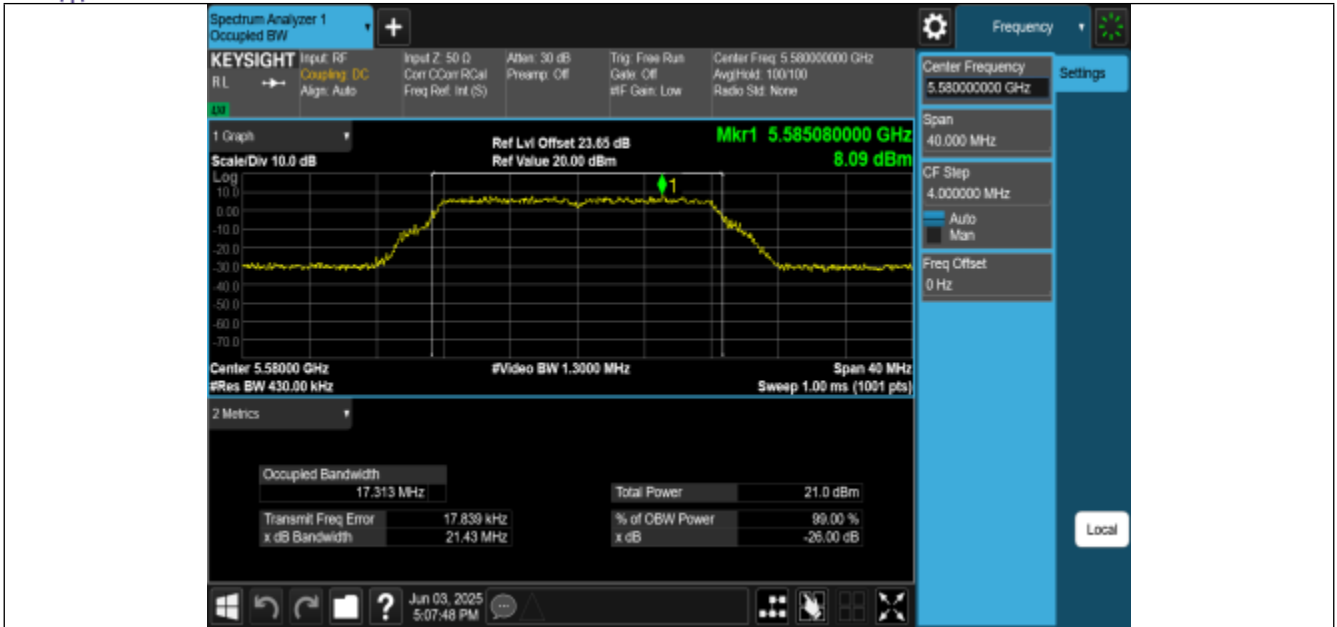
11A-CDD-Ant2-5580
