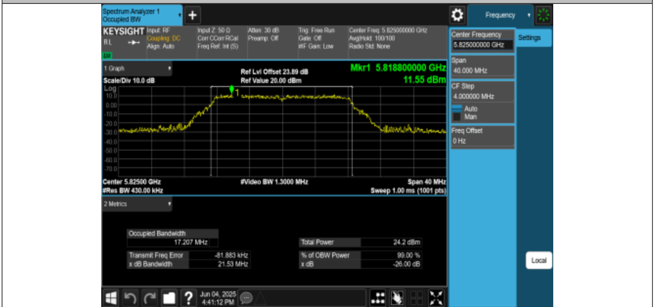
11A-CDD-Ant3-5825
