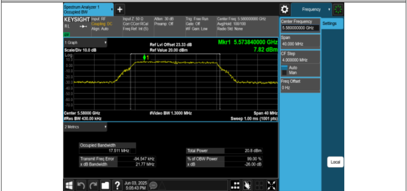
11A-CDD-Ant1-5580
