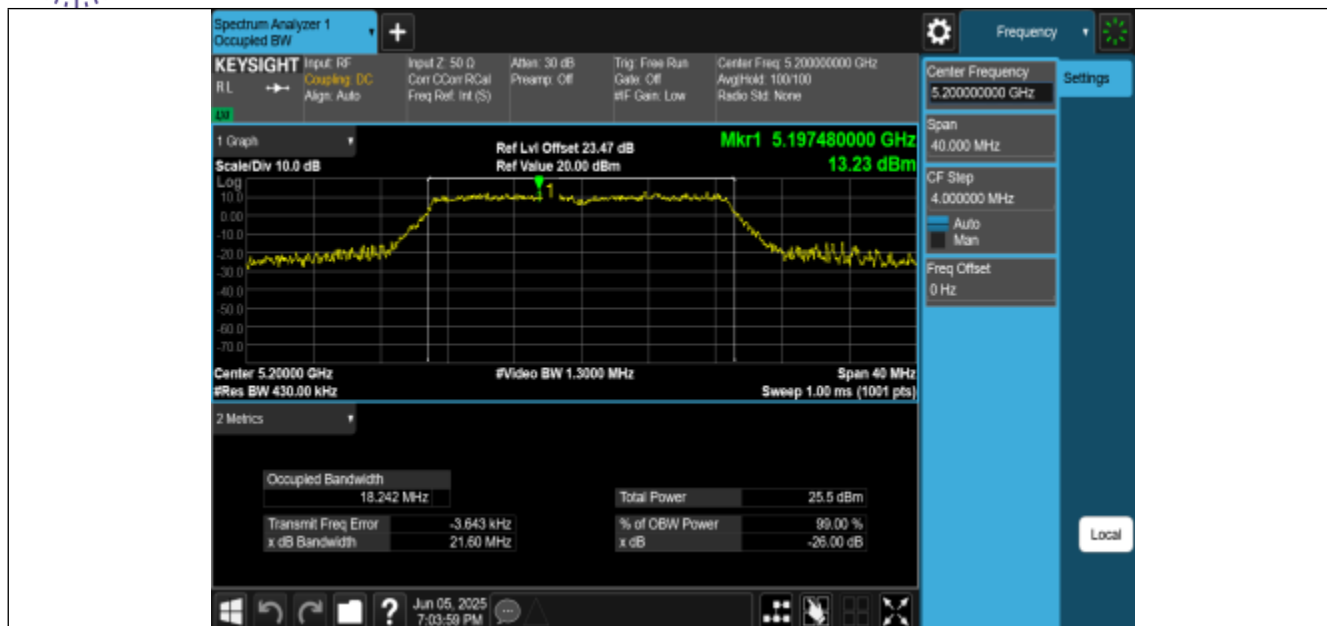
11AC20MIMO-Ant2-5200
