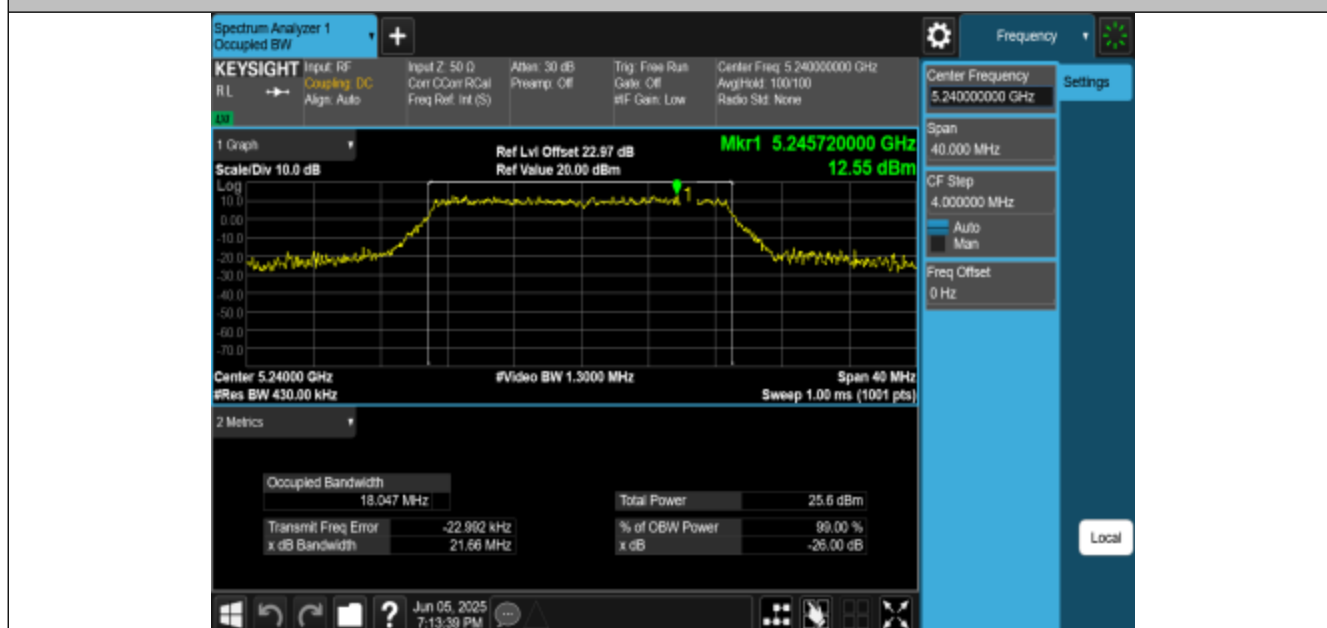
11AC20MIMO-Ant1-5240
