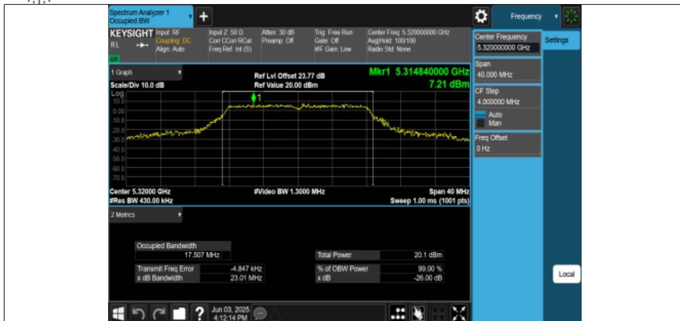
11A-CDD-Ant2-5320
