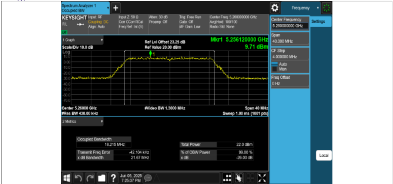
11AC20MIMO-Ant2-5260
