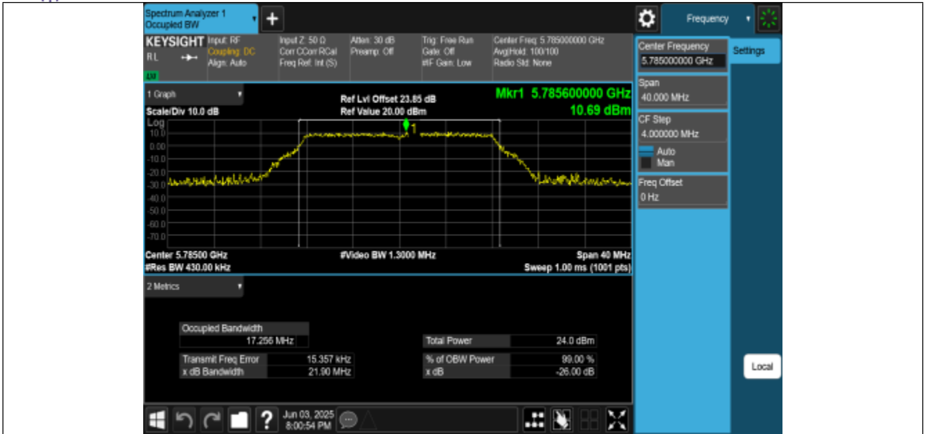
11A-CDD-Ant2-5785
