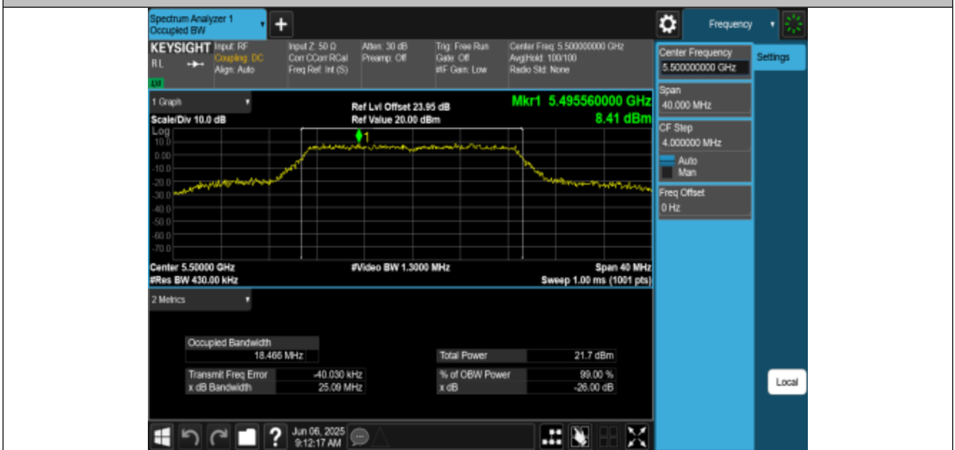
11AC20MIMO-Ant3-5500
