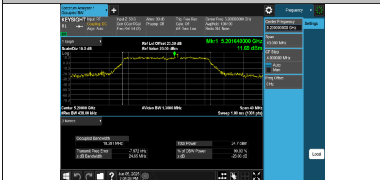
11AC20MIMO-Ant3-5200
