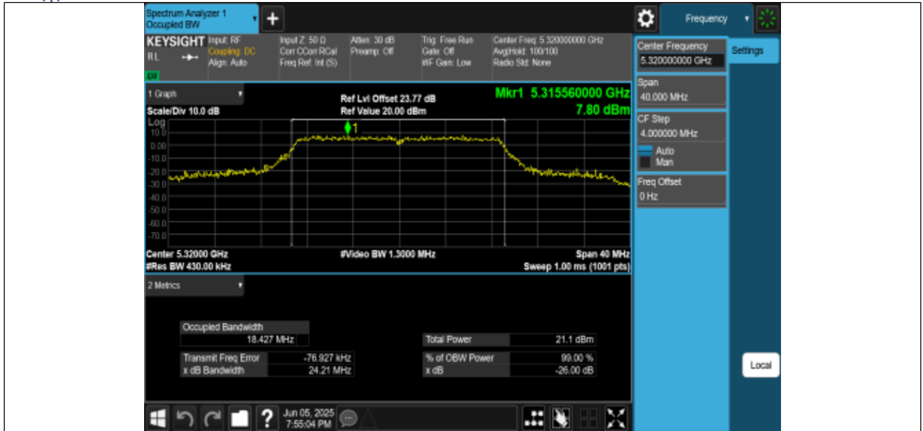
11AC20MIMO-Ant2-5320
