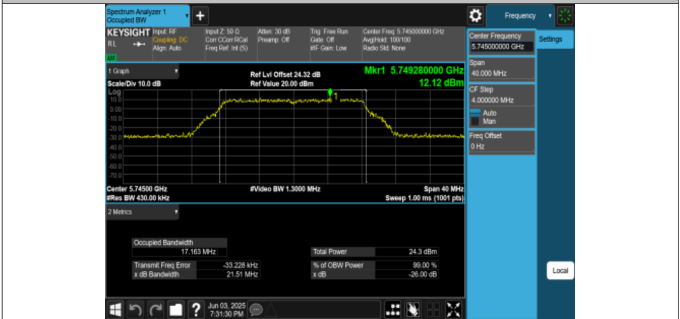
11A-CDD-Ant3-5745
