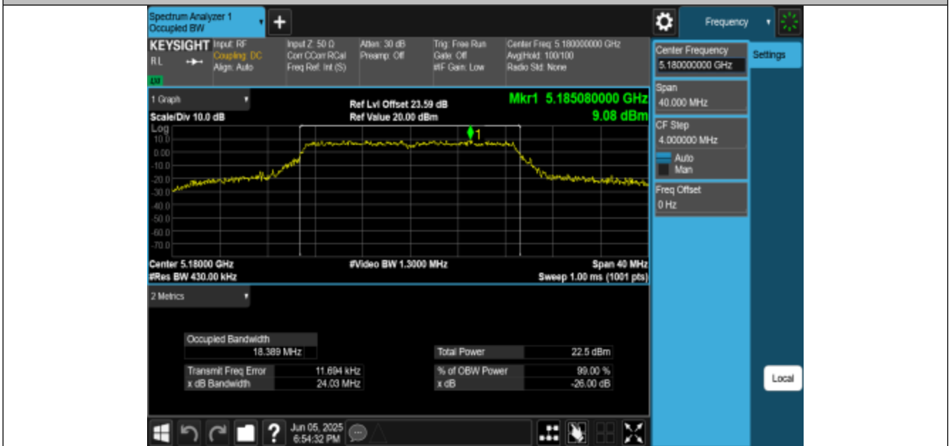
11AC20MIMO-Ant3-5180
