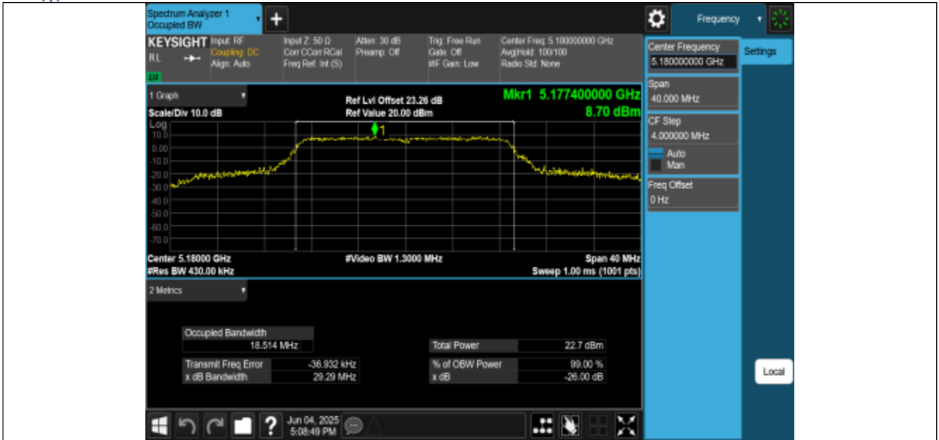
11N20MIMO-Ant0-5180
