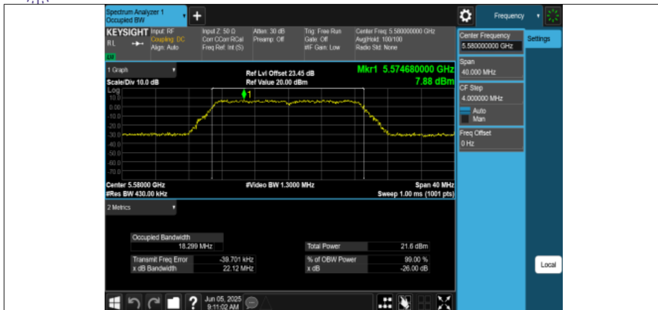
11N20MIMO-Ant0-5580
