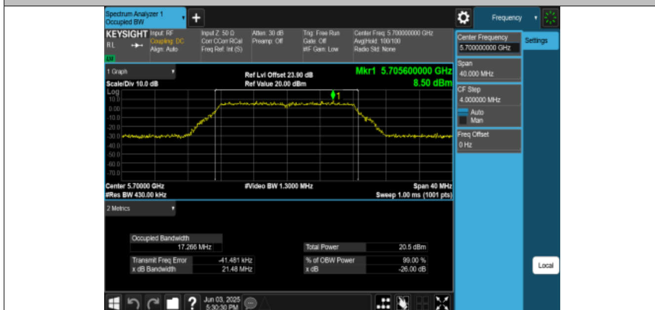
11A-CDD-Ant3-5700
