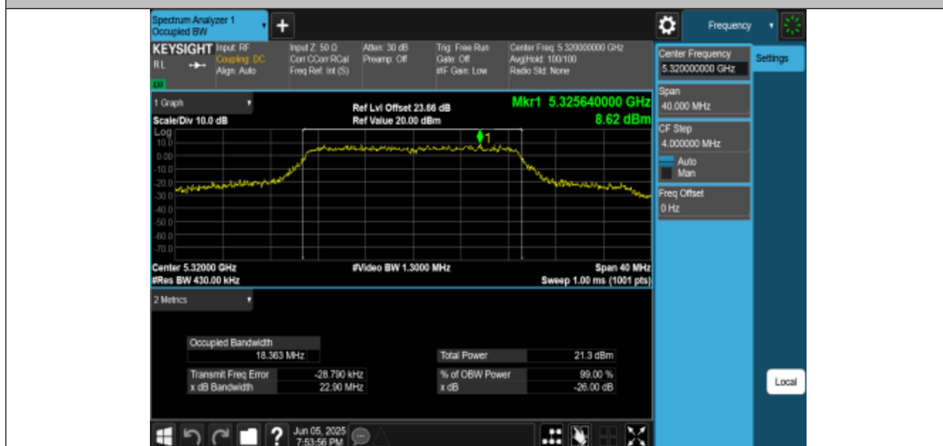
11AC20MIMO-Ant1-5320
