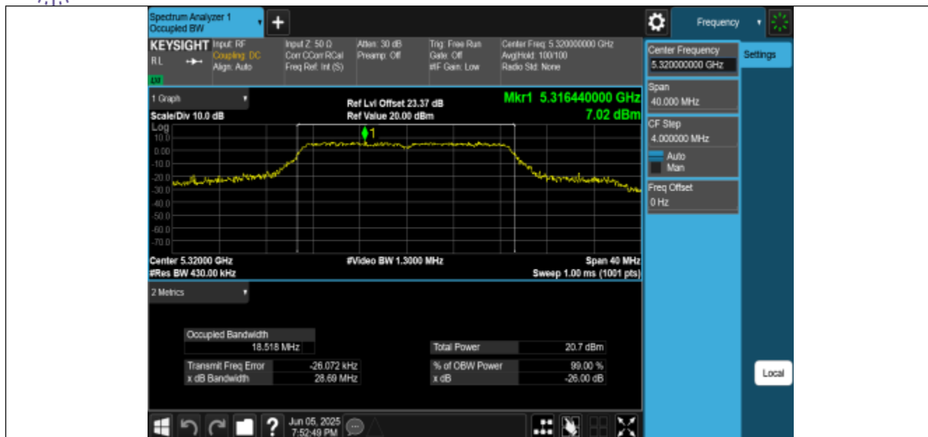
11AC20MIMO-Ant0-5320
