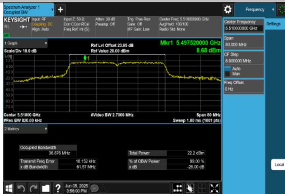
11N40MIMO-Ant3-5510
