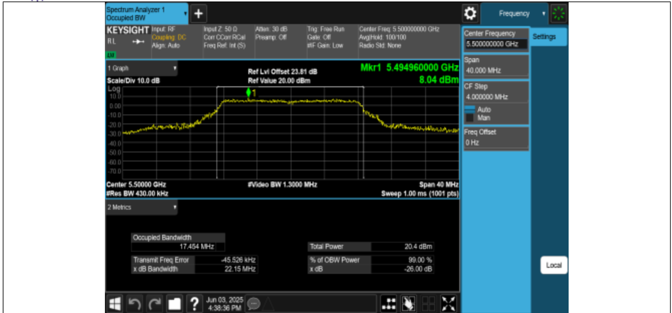
11A-CDD-Ant2-5500
