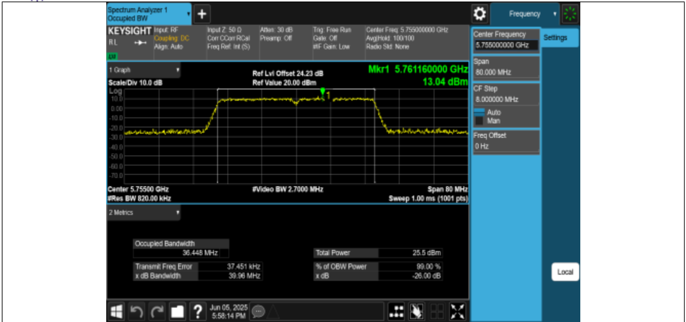
11N40MIMO-Ant2-5755
