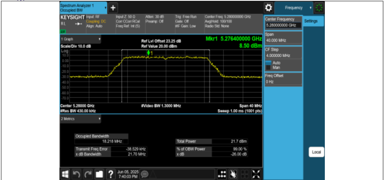
11AC20MIMO-Ant2-5280
