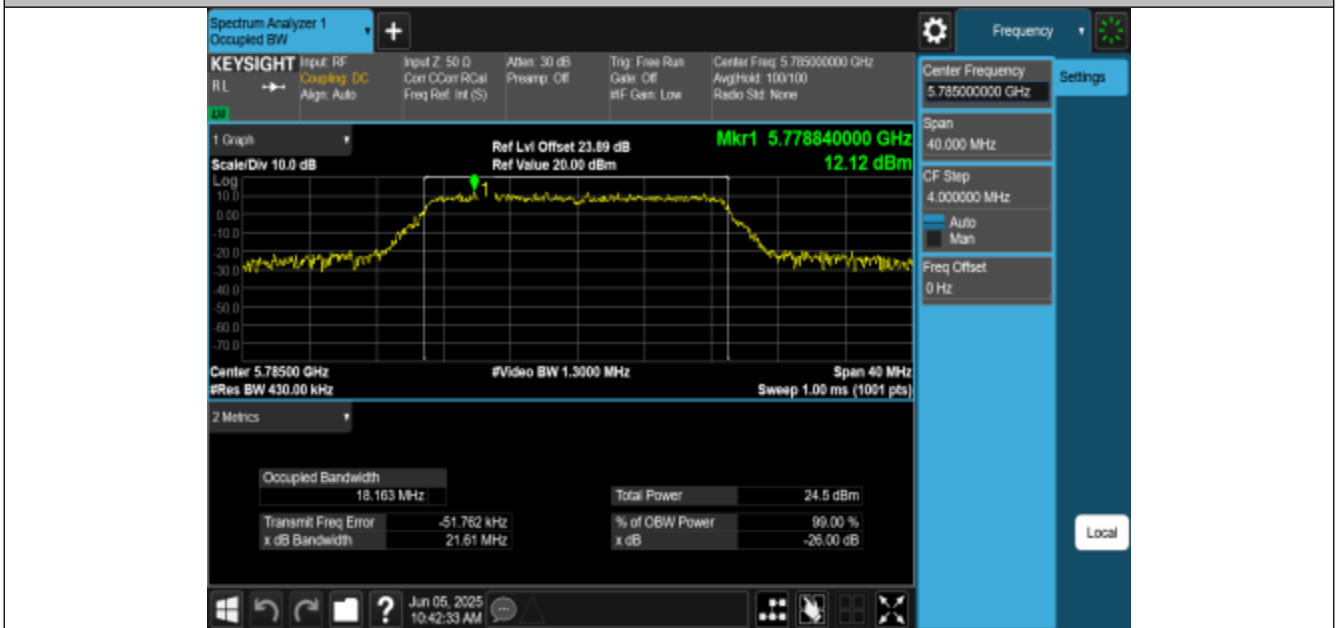
11N20MIMO-Ant3-5785
