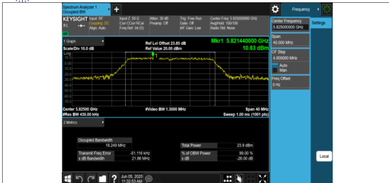
11N20MIMO-Ant2-5825
