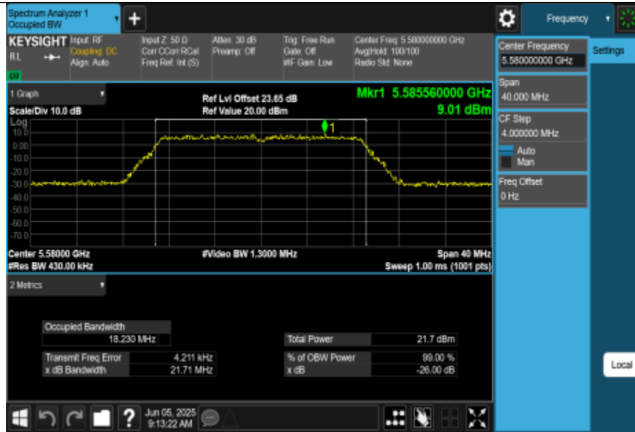
11N20MIMO-Ant2-5580
