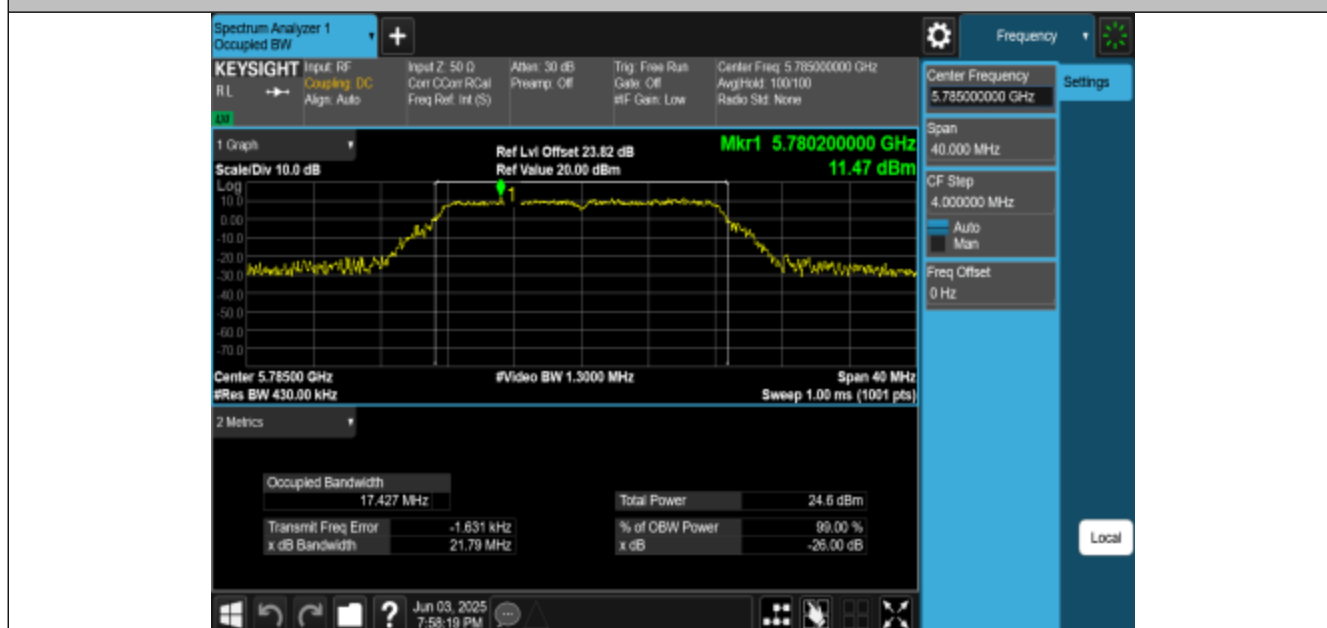
11A-CDD-Ant1-5785
