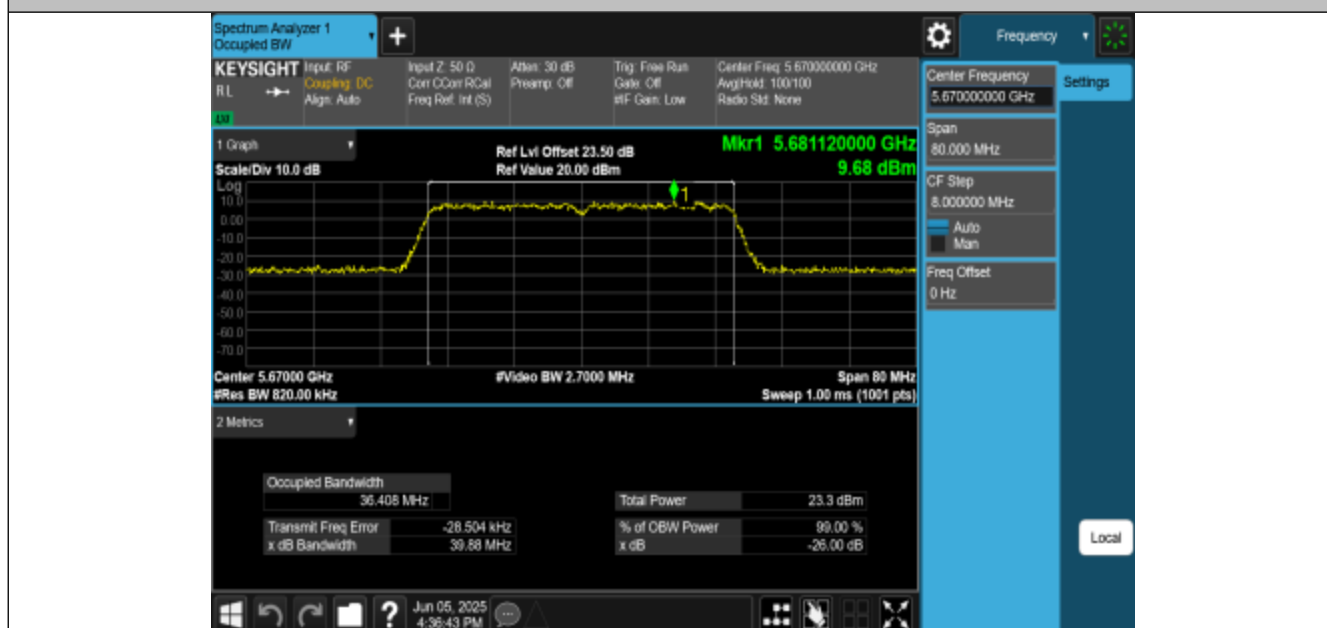
11N40MIMO-Ant1-5670
