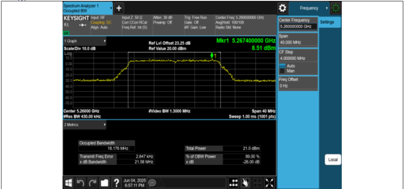
11N20MIMO-Ant2-5260
