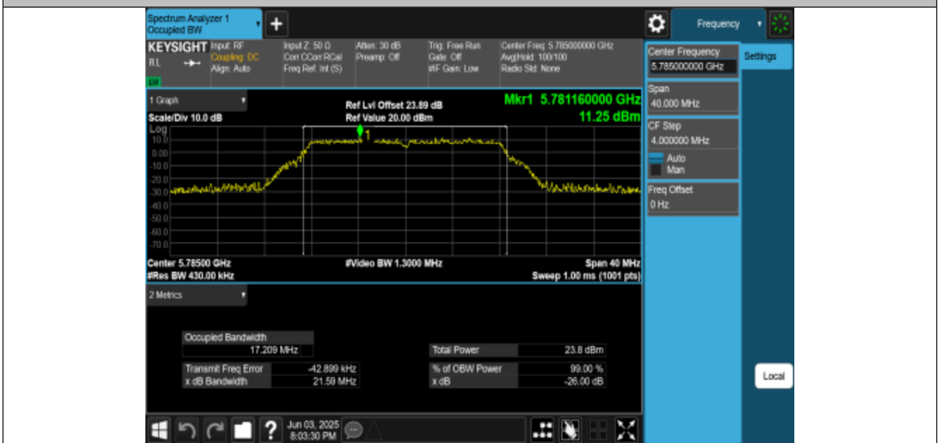
11A-CDD-Ant3-5785
