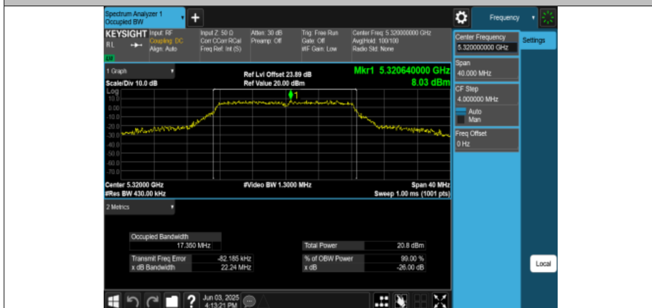
11A-CDD-Ant3-5320
