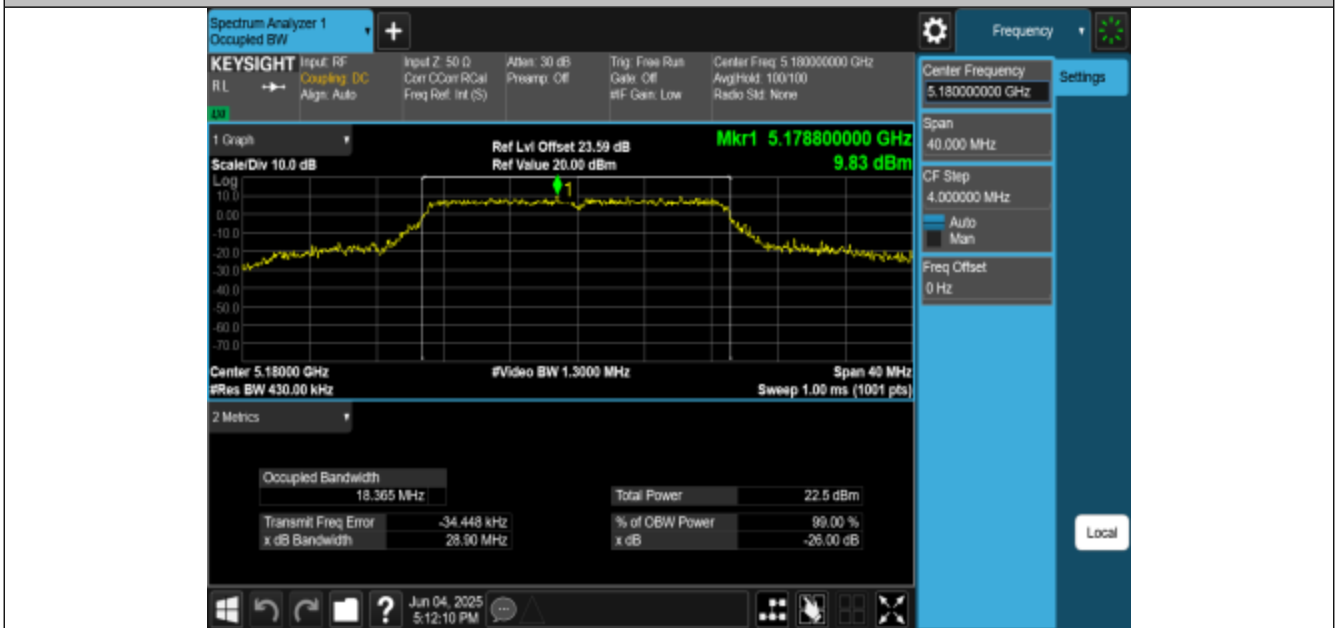
11N20MIMO-Ant3-5180
