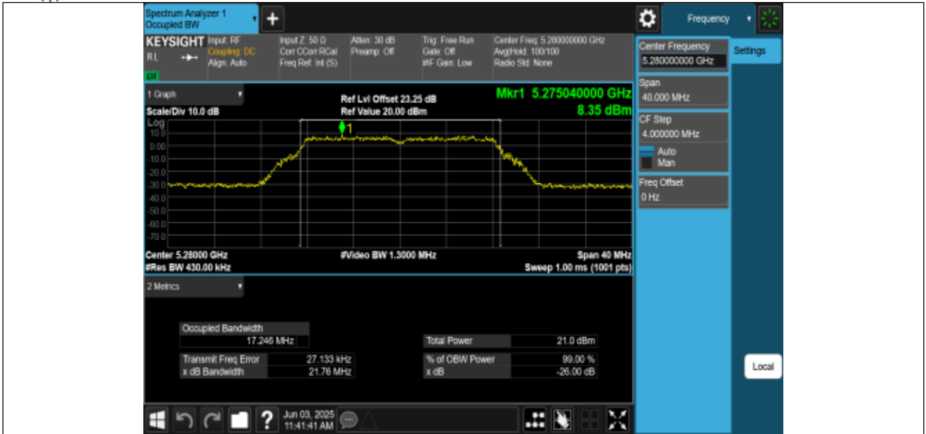
11A-CDD-Ant2-5280
