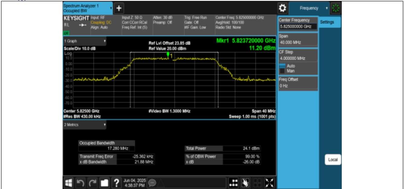
11A-CDD-Ant2-5825
