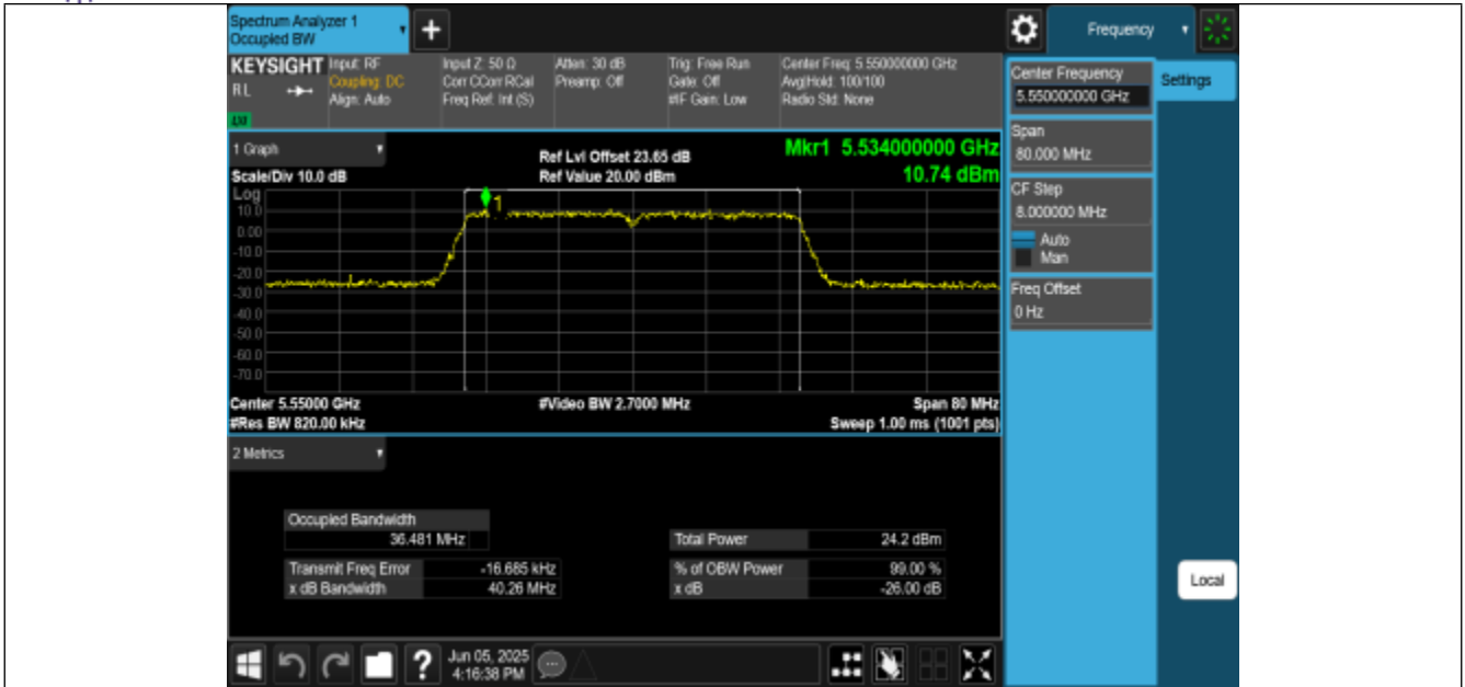
11N40MIMO-Ant2-5550
