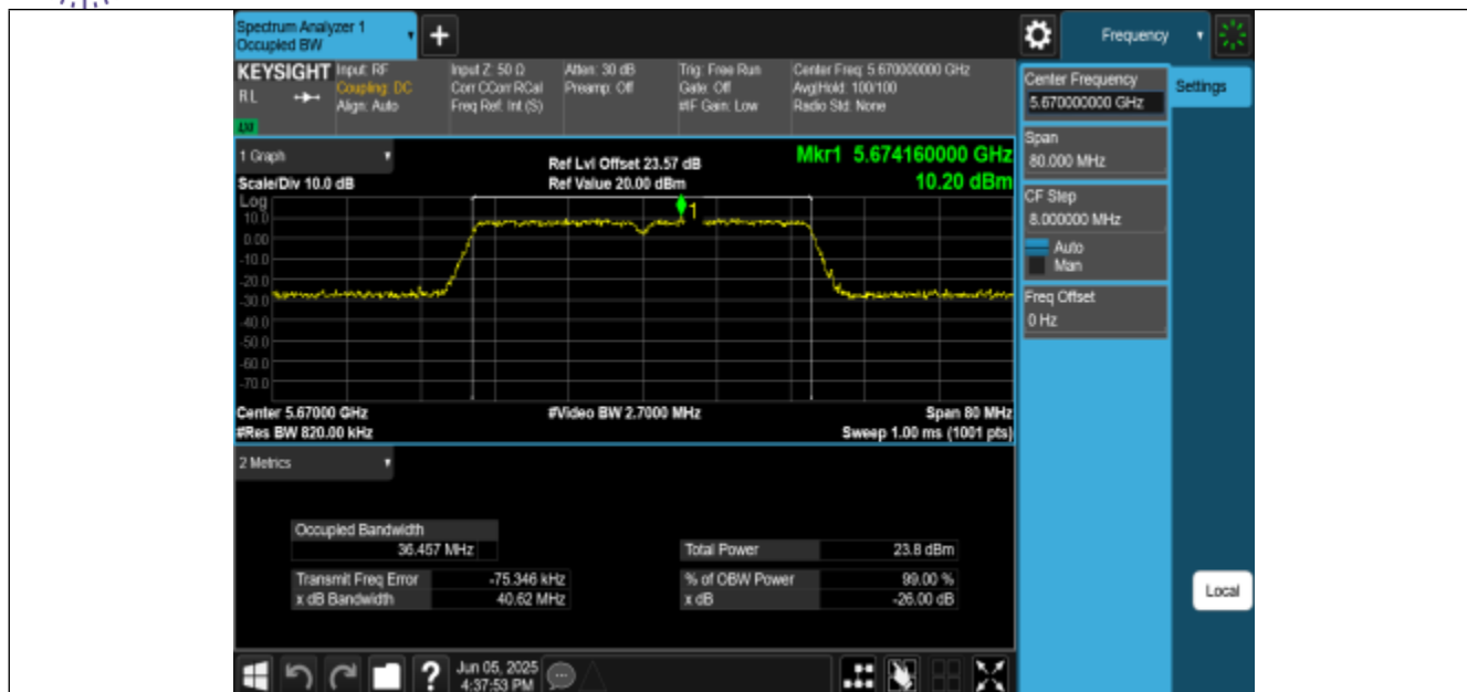
11N40MIMO-Ant2-5670
