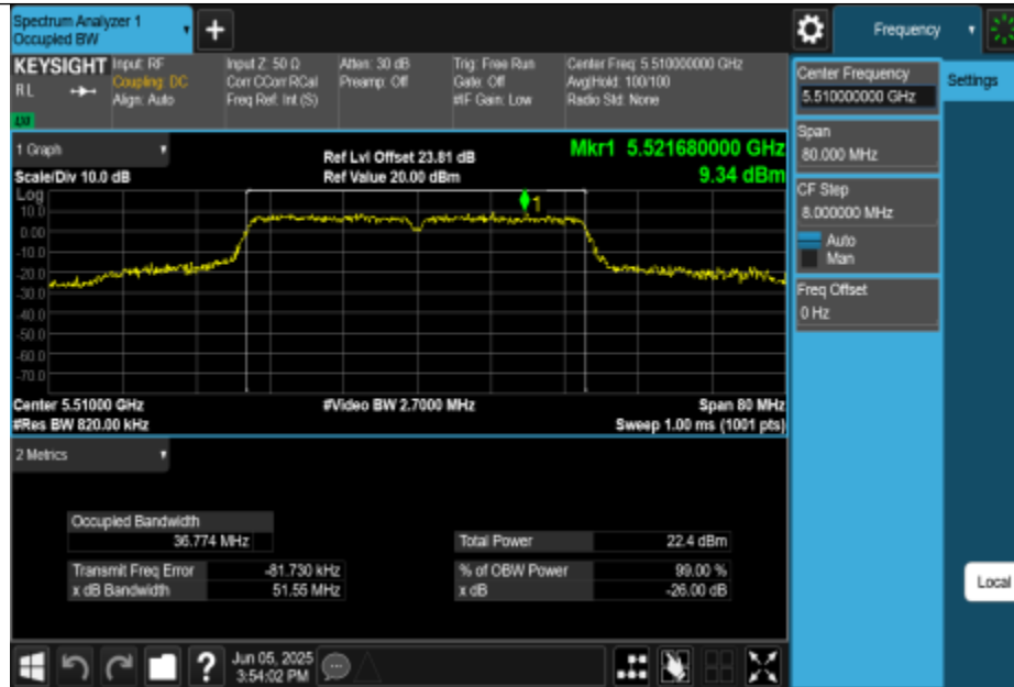
11N40MIMO-Ant2-5510
