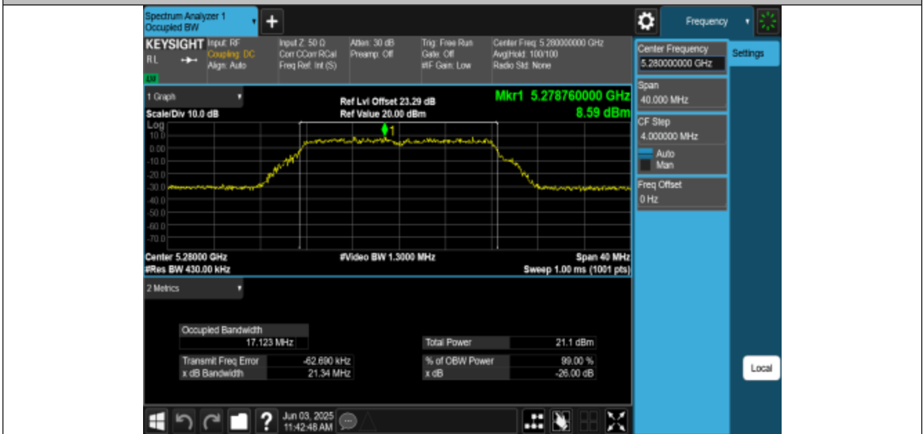
11A-CDD-Ant3-5280
