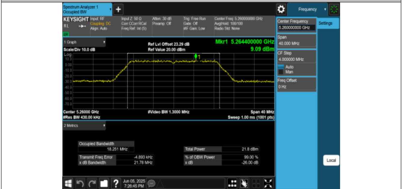
11AC20MIMO-Ant3-5260
