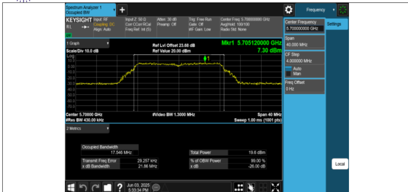
11A-CDD-Ant1-5700
