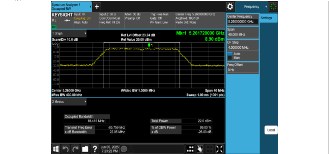
11AC20MIMO-Ant0-5260
