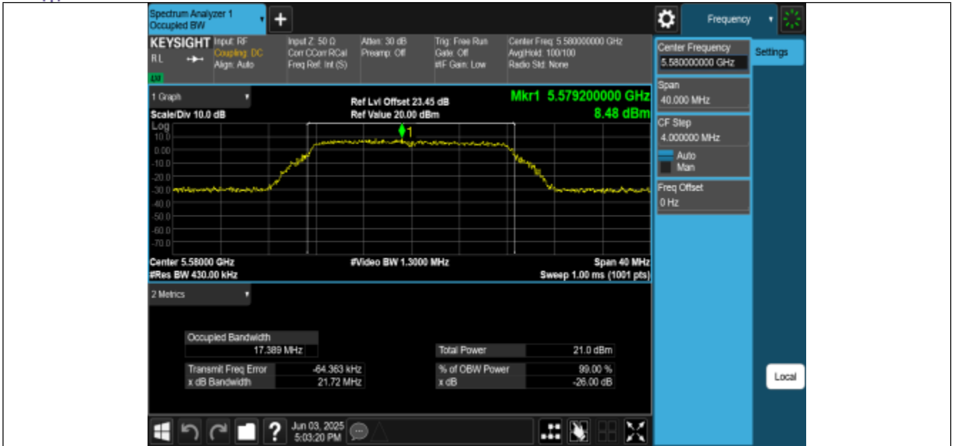
11A-CDD-Ant0-5580
