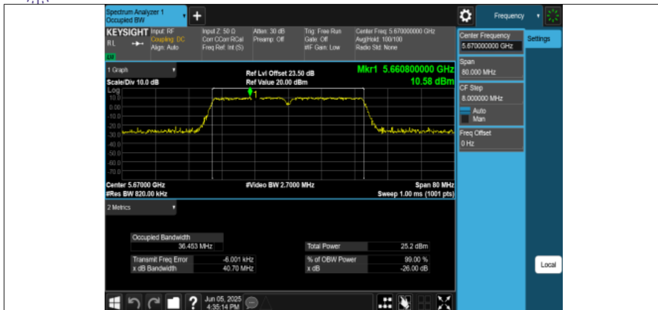
11N40MIMO-Ant0-5670
