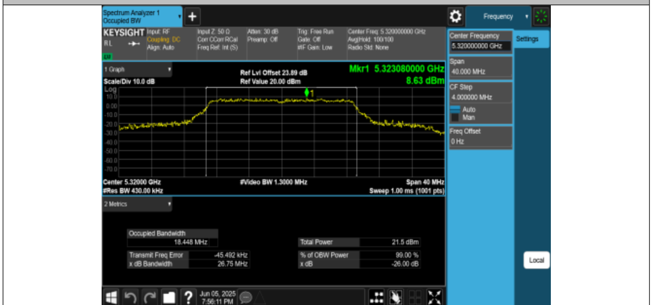
11AC20MIMO-Ant3-5320
