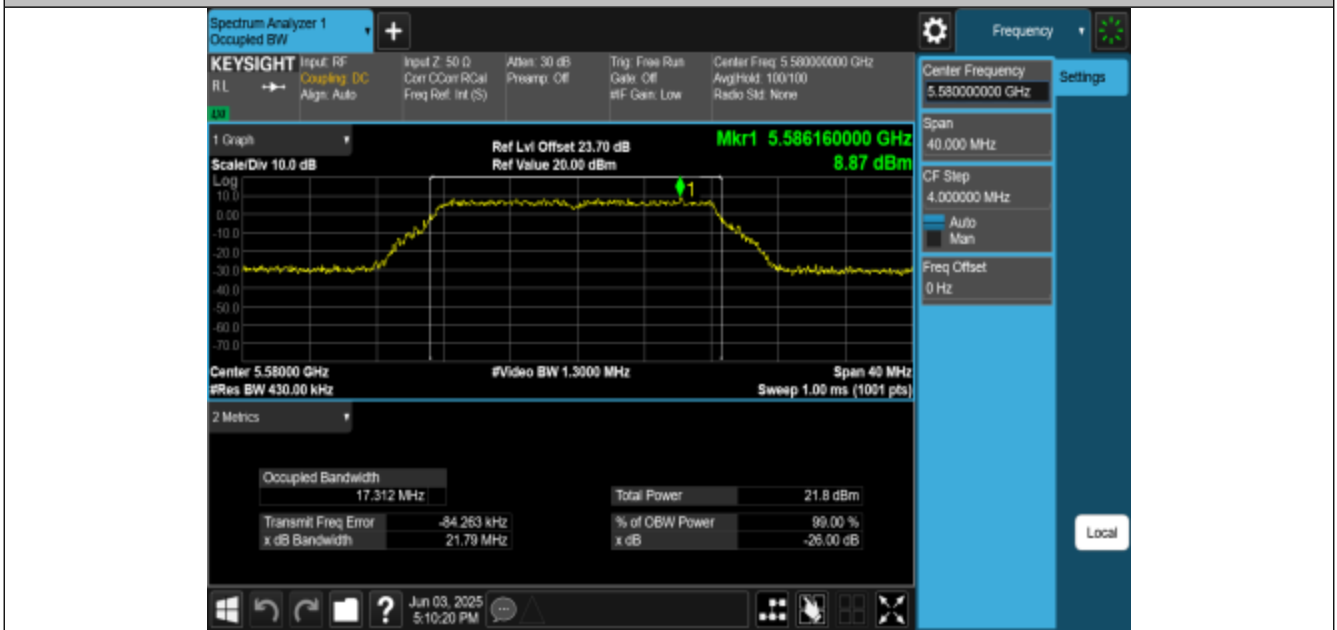
11A-CDD-Ant3-5580
