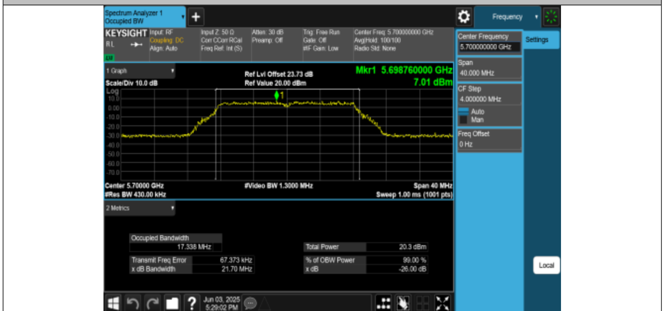
11A-CDD-Ant2-5700
