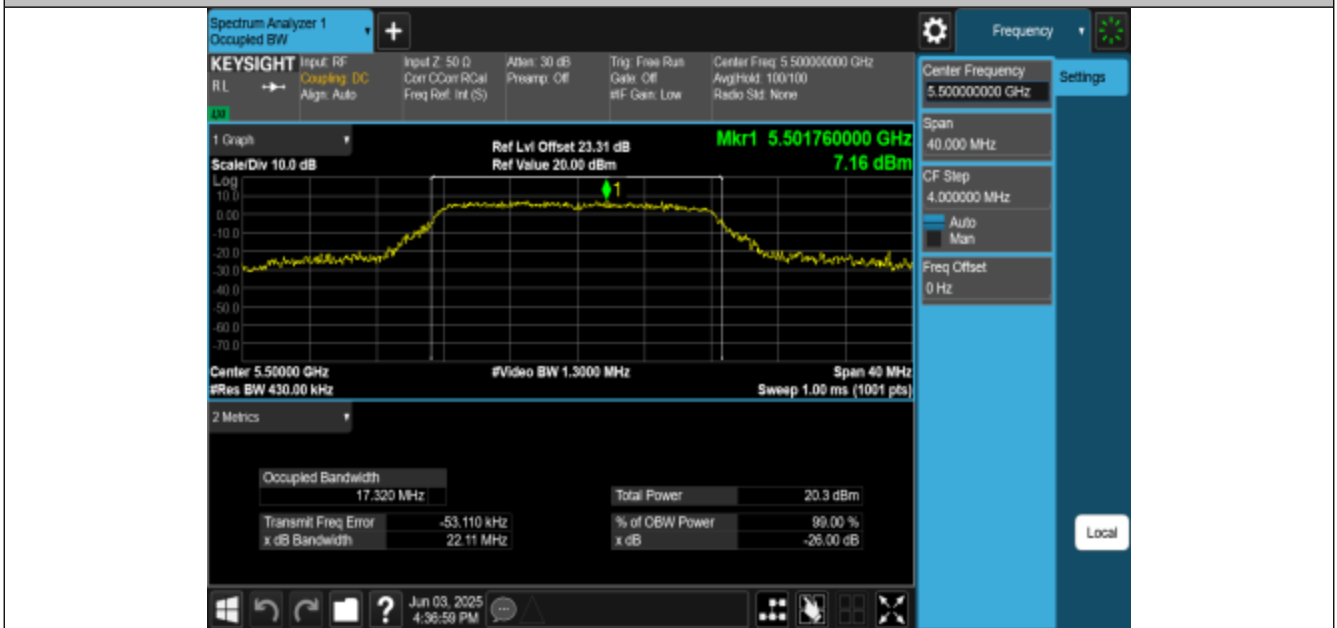
11A-CDD-Ant1-5500
