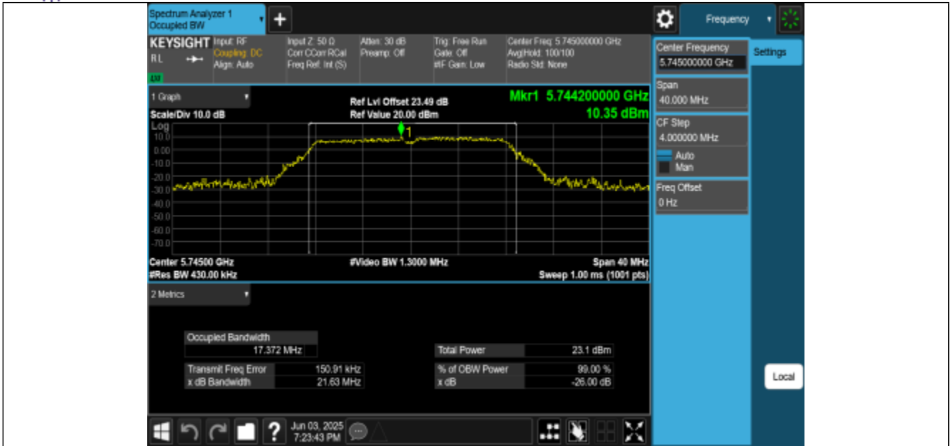
11A-CDD-Ant0-5745
