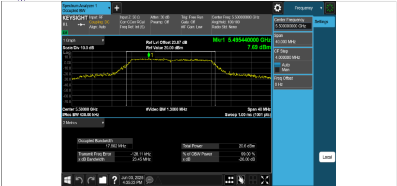
11A-CDD-Ant0-5500
