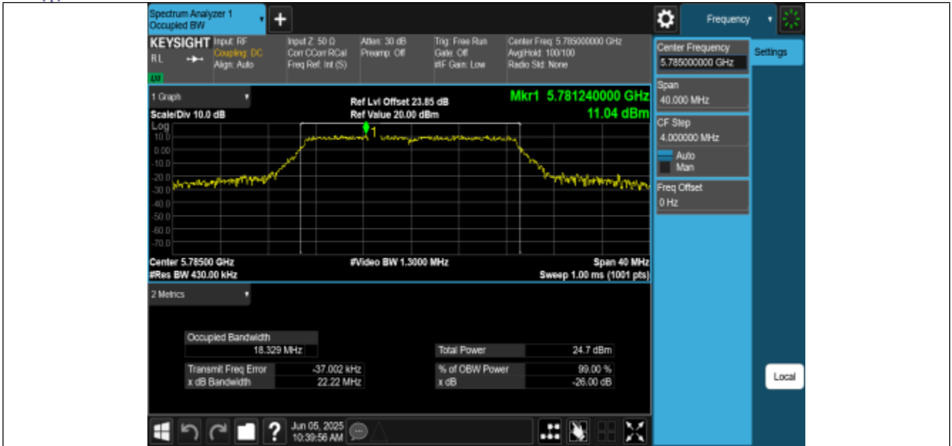
11N20MIMO-Ant2-5785
