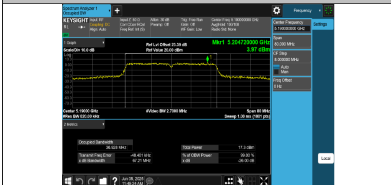
11N40MIMO-Ant3-5190
