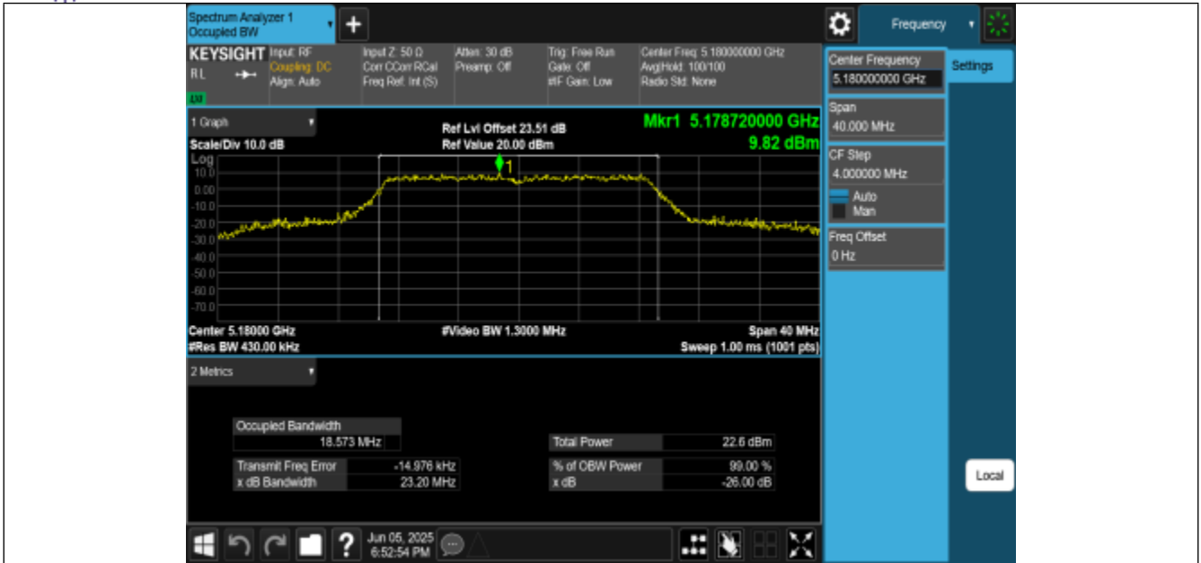
11AC20MIMO-Ant2-5180
