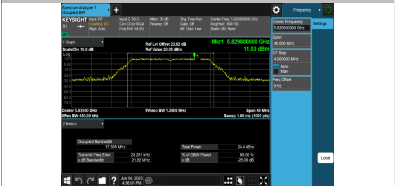
11A-CDD-Ant1-5825
