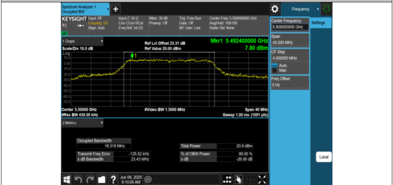
11AC20MIMO-Ant1-5500
