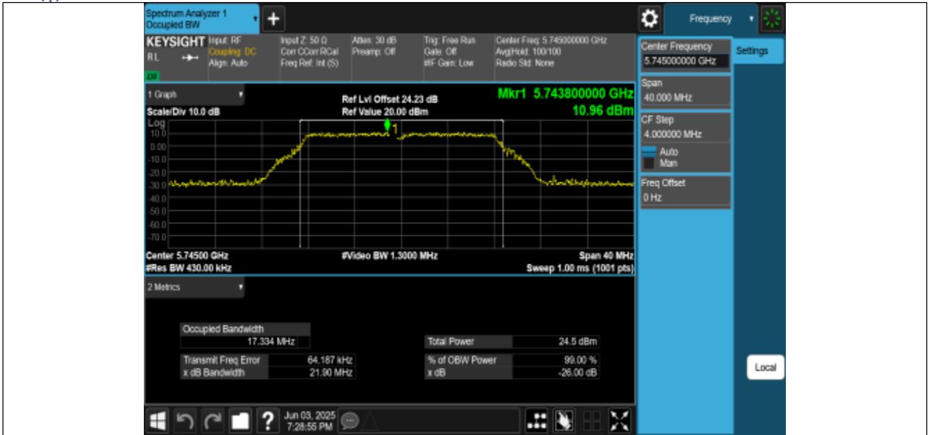
11A-CDD-Ant2-5745
