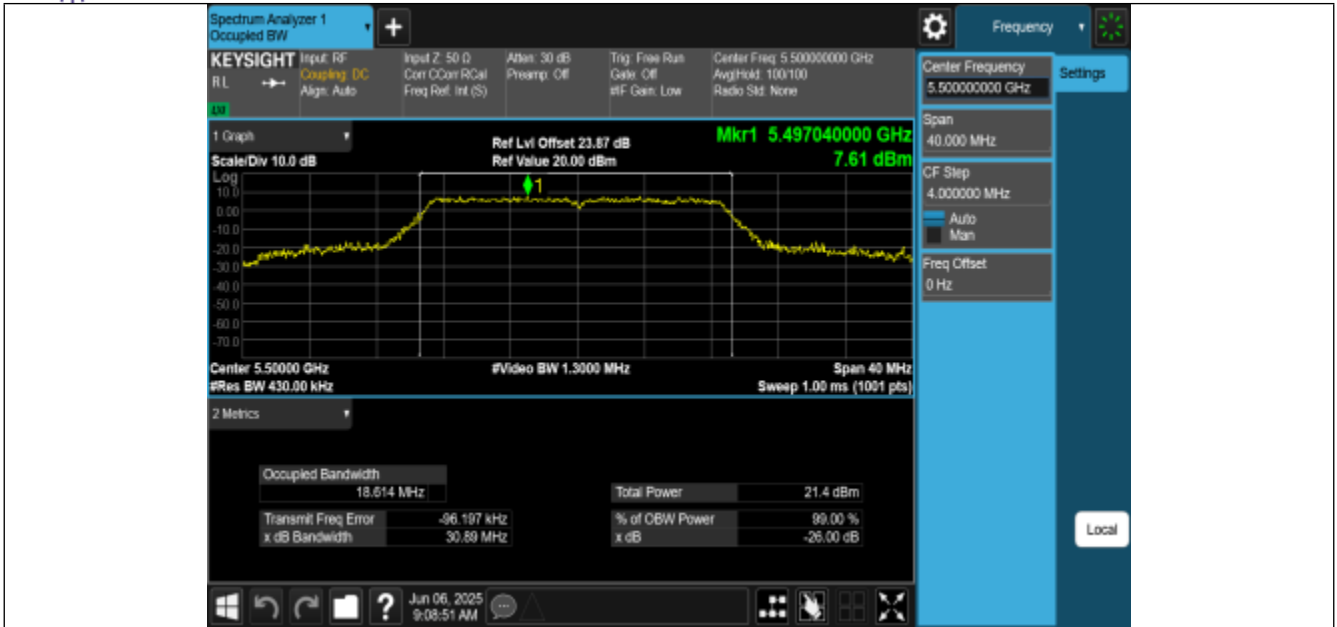
11AC20MIMO-Ant0-5500
