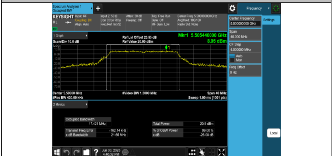
11A-CDD-Ant3-5500
