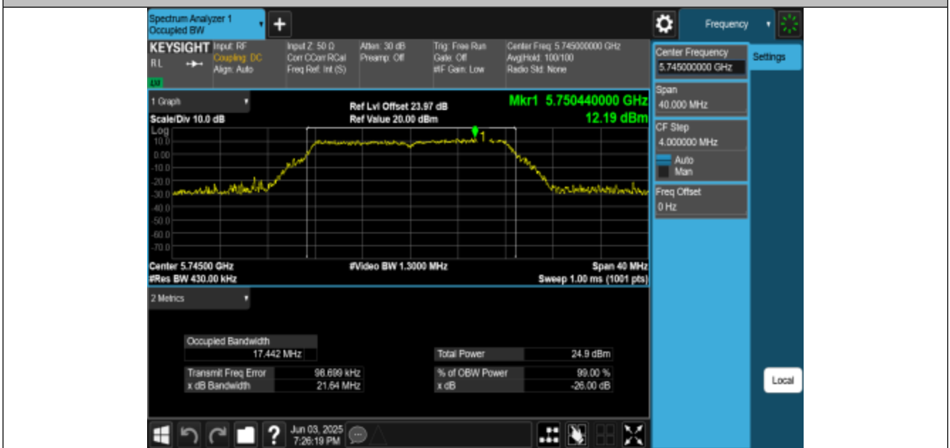
11A-CDD-Ant1-5745
