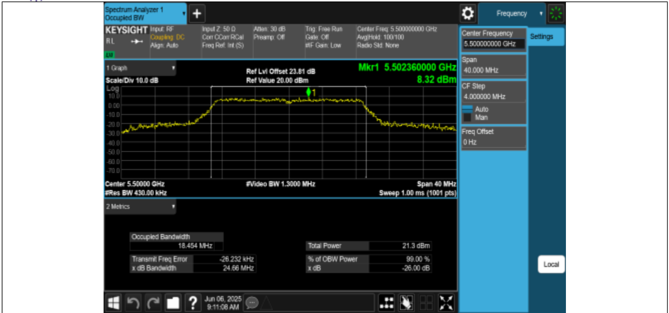
11AC20MIMO-Ant2-5500
