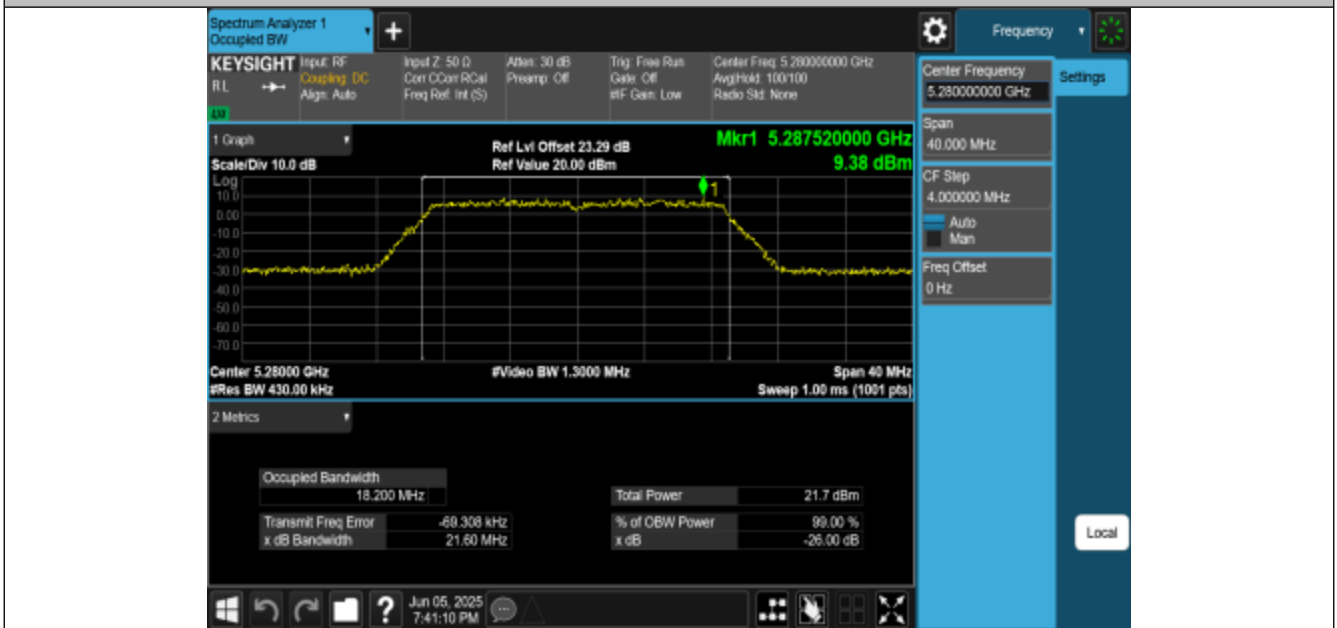
11AC20MIMO-Ant3-5280
