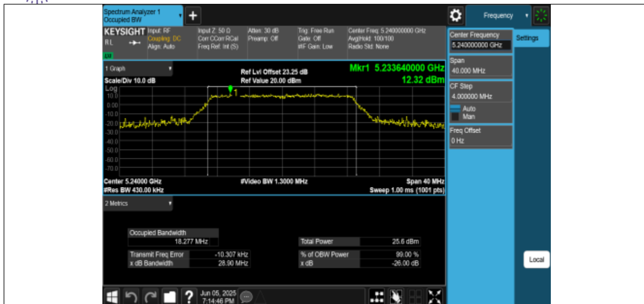
11AC20MIMO-Ant2-5240
