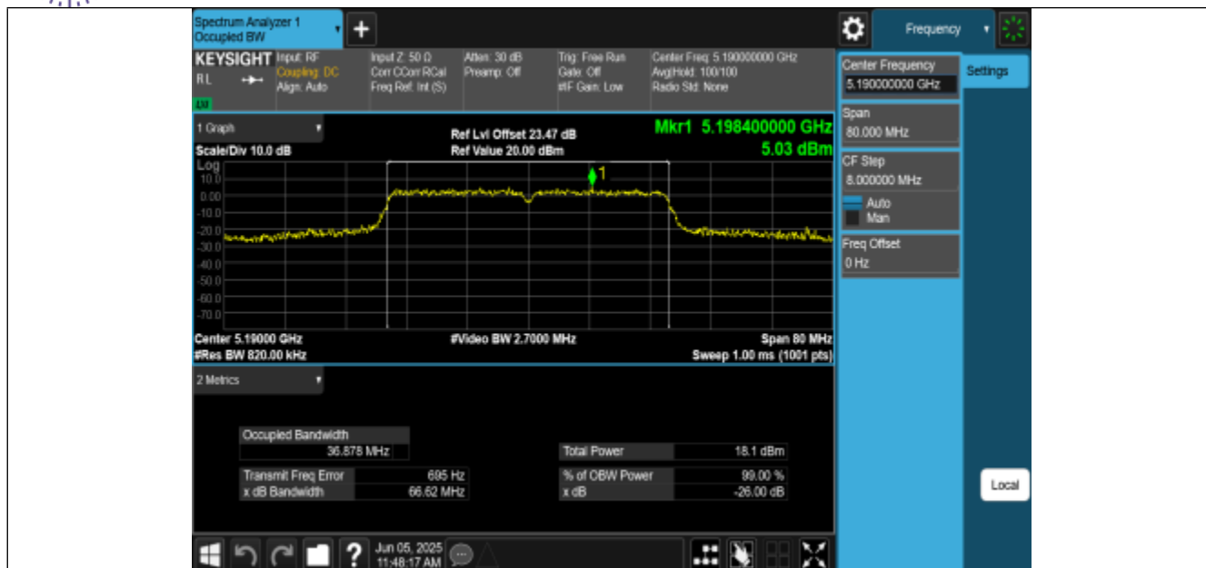
11N40MIMO-Ant2-5190
