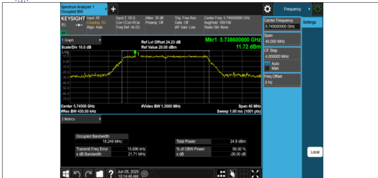
11N20MIMO-Ant2-5745
