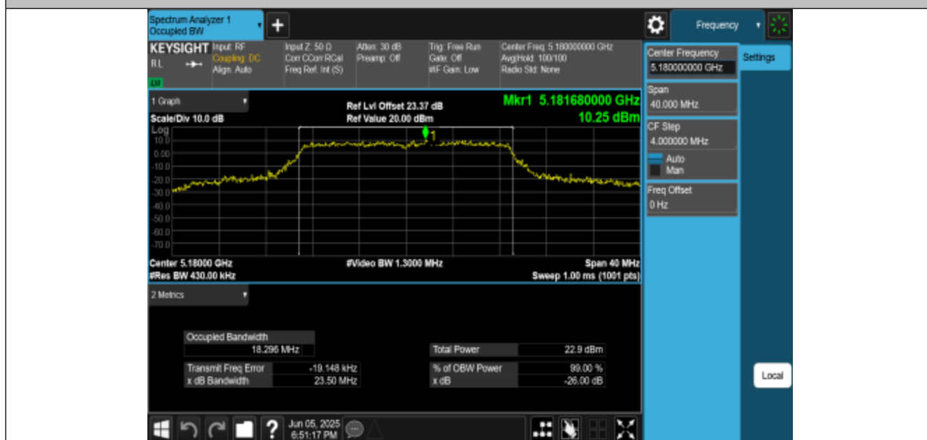
11AC20MIMO-Ant1-5180
