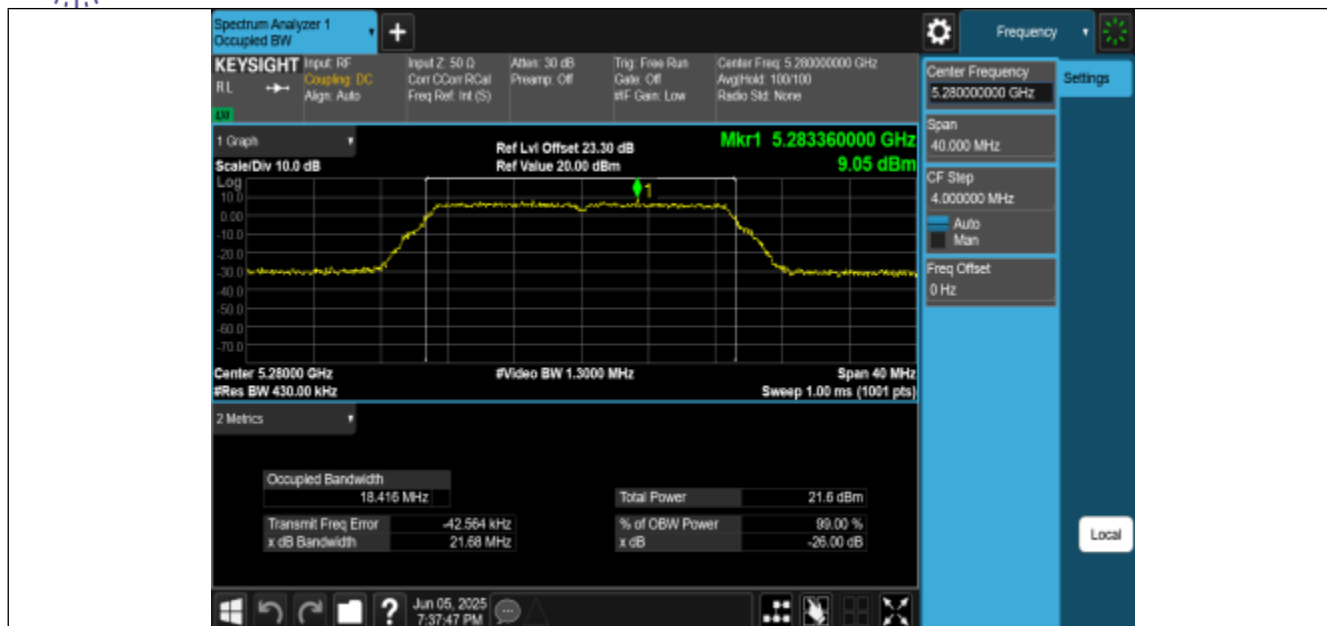
11AC20MIMO-Ant0-5280
