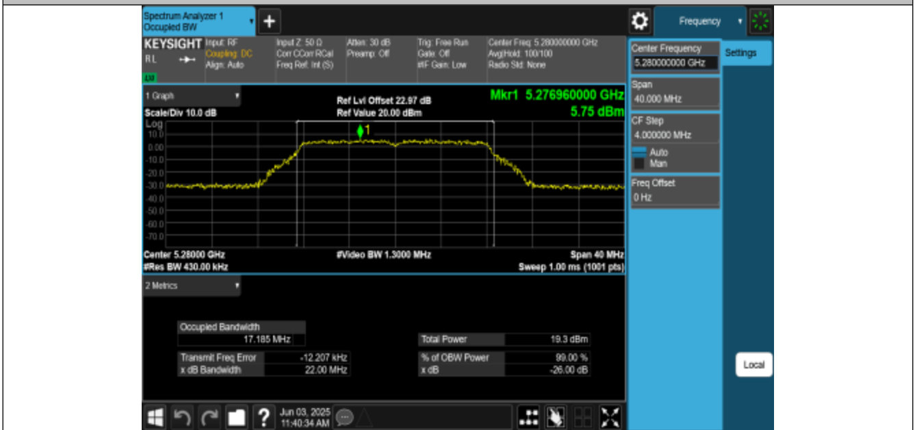
11A-CDD-Ant1-5280
