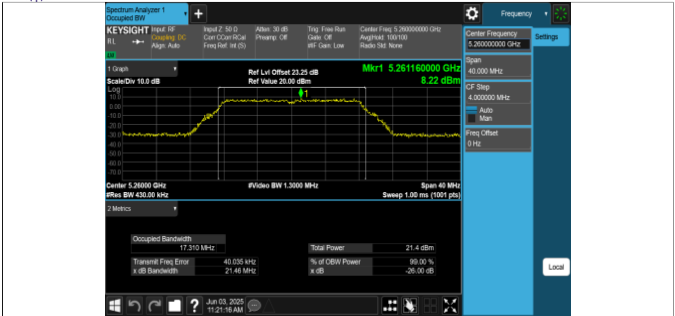
11A-CDD-Ant2-5260
