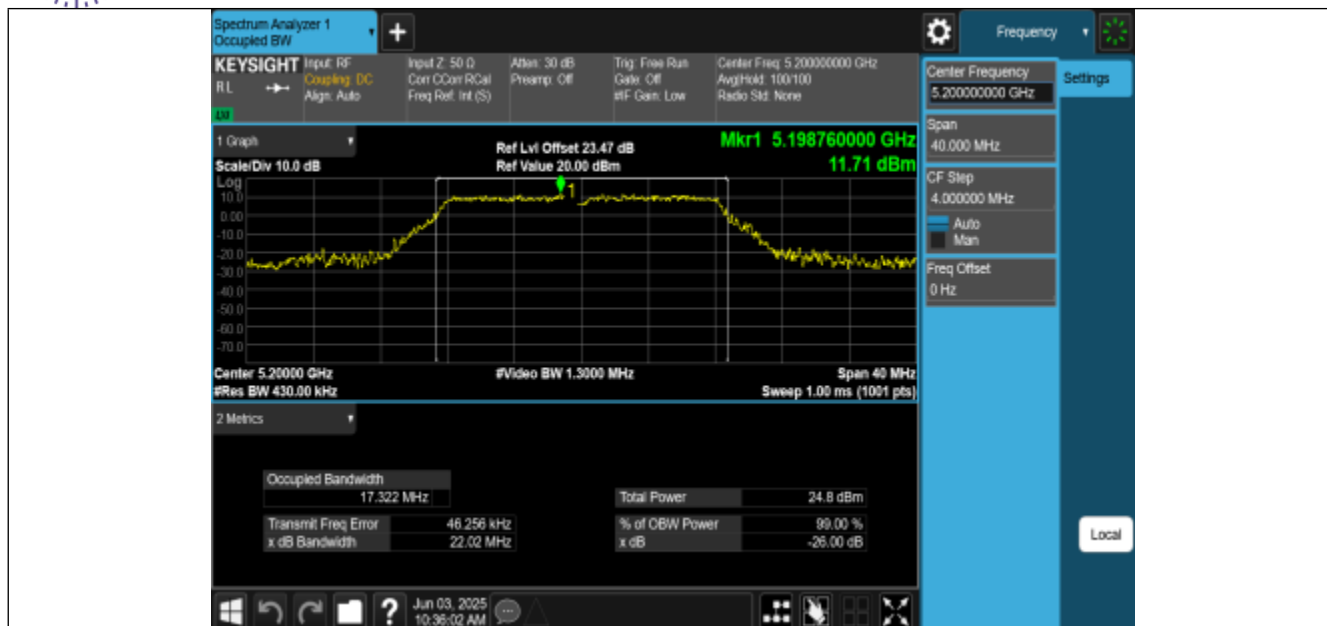
11A-CDD-Ant2-5200
