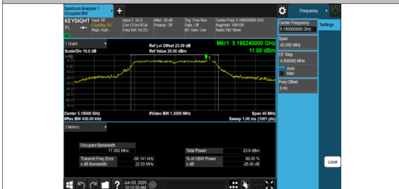
11A-CDD-Ant3-5180
