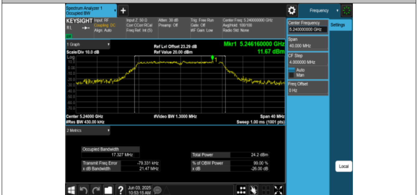
11A-CDD-Ant3-5240
