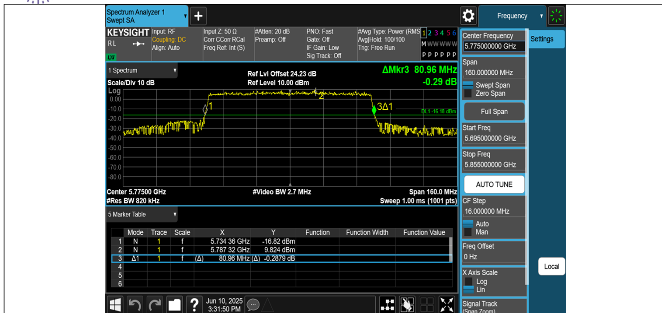
11BE80MIMO-Ant2-5775
