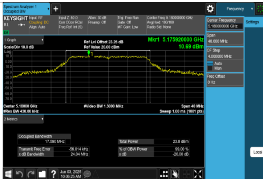
11A-CDD-Ant0-5180
