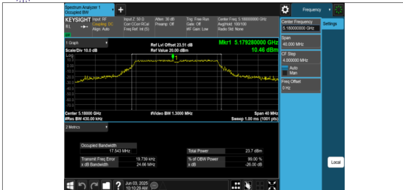
11A-CDD-Ant2-5180
