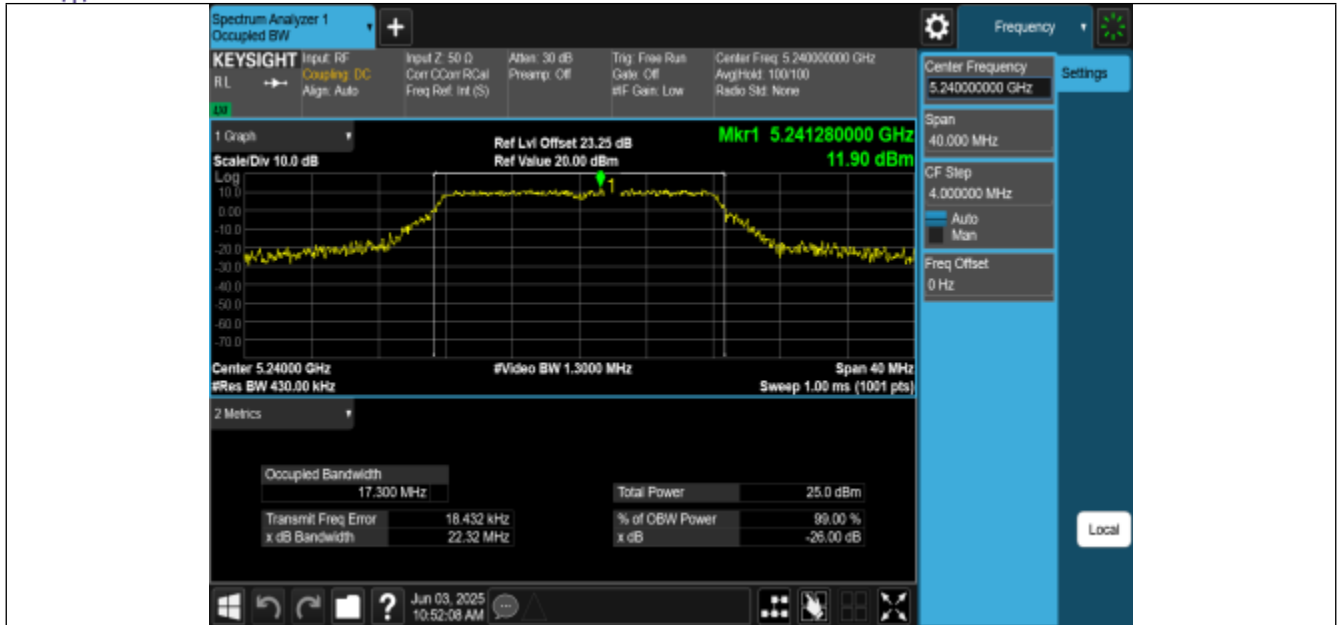
11A-CDD-Ant2-5240
