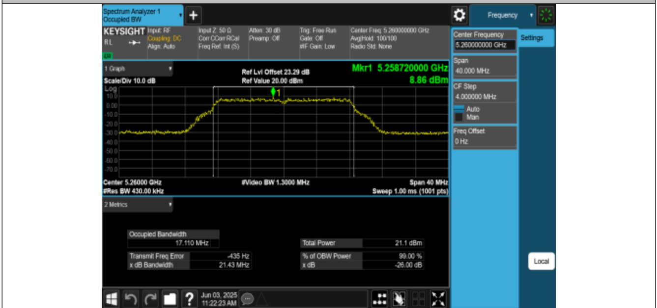
11A-CDD-Ant3-5260
