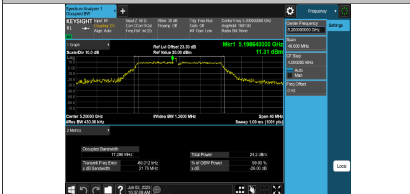
11A-CDD-Ant3-5200
