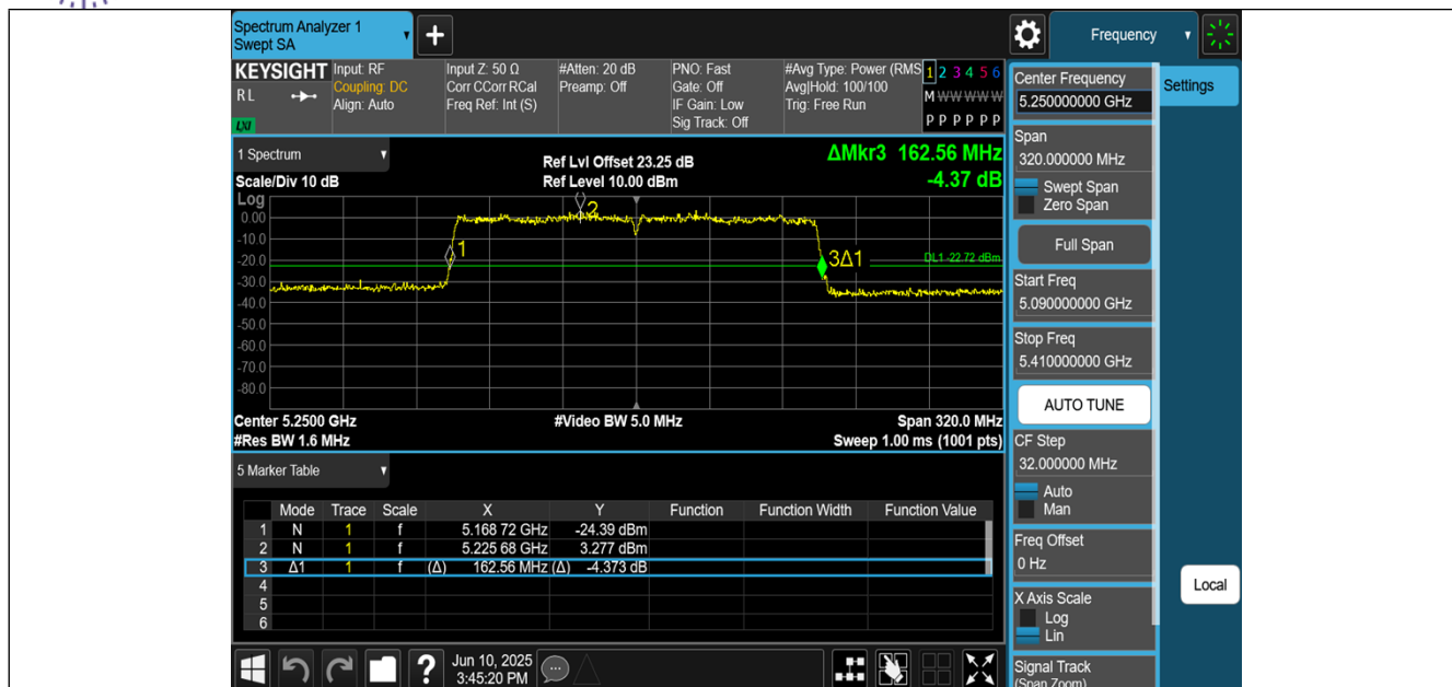
11BE160MIMO-Ant2-5250
