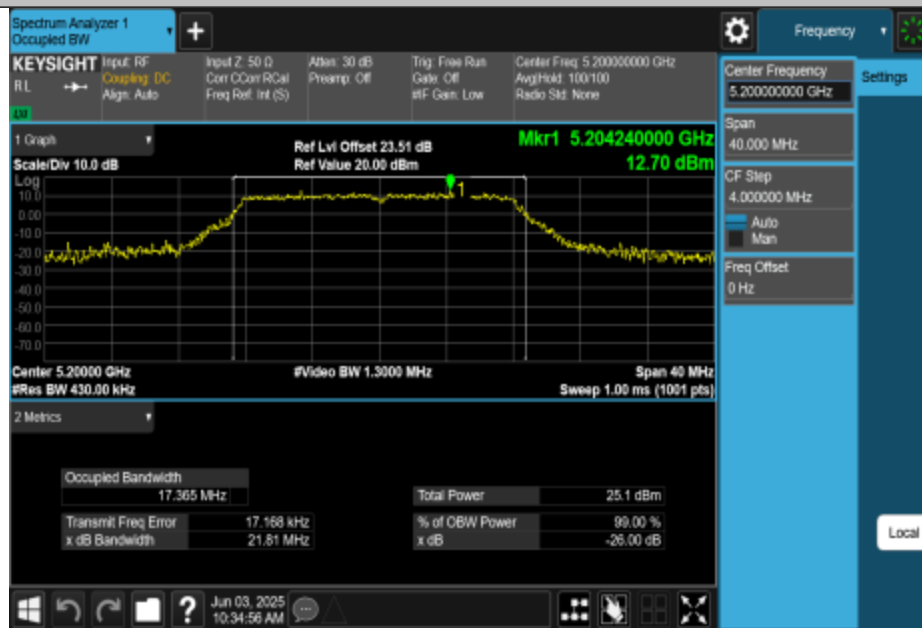
11A-CDD-Ant1-5200
