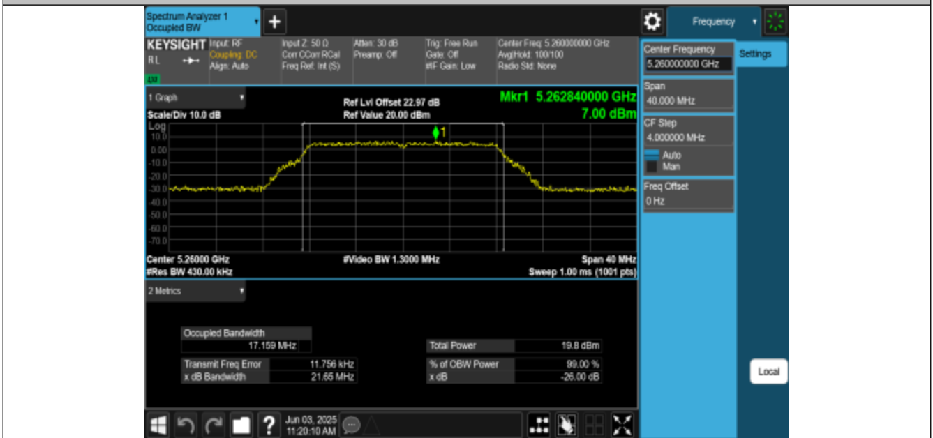
11A-CDD-Ant1-5260
