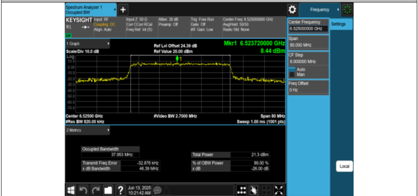
11BE40MIMO-Ant1-6525-PASS
