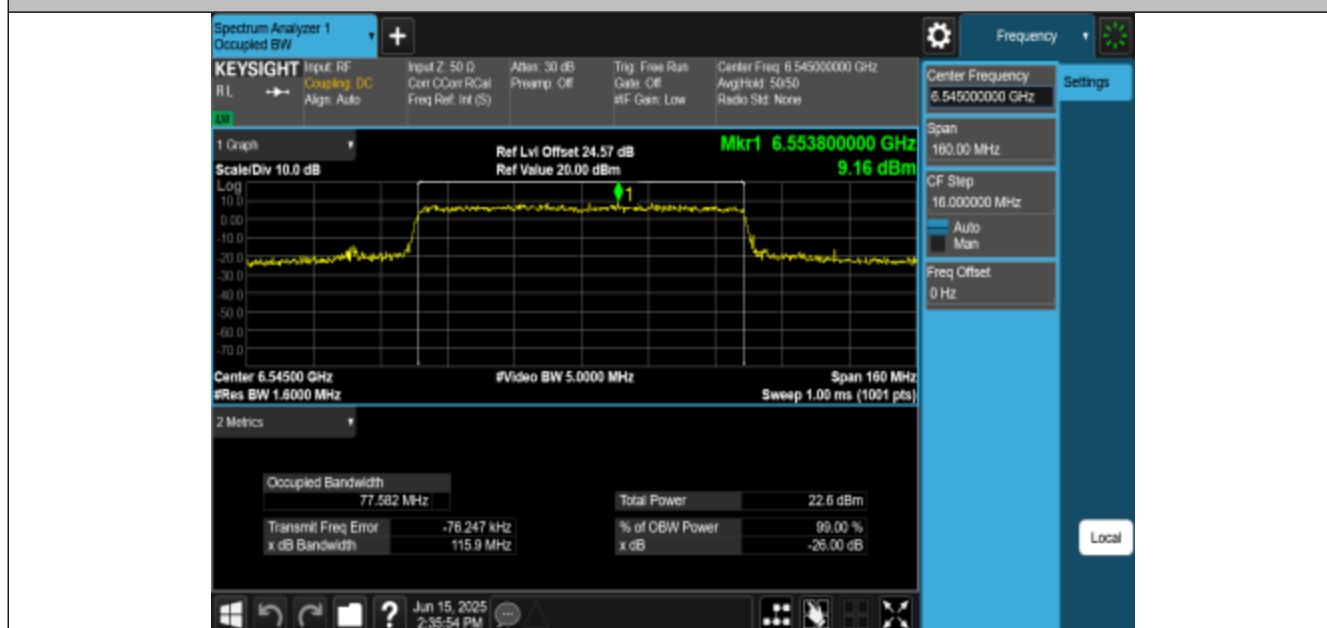
11BE80MIMO-Ant3-6545-PASS
