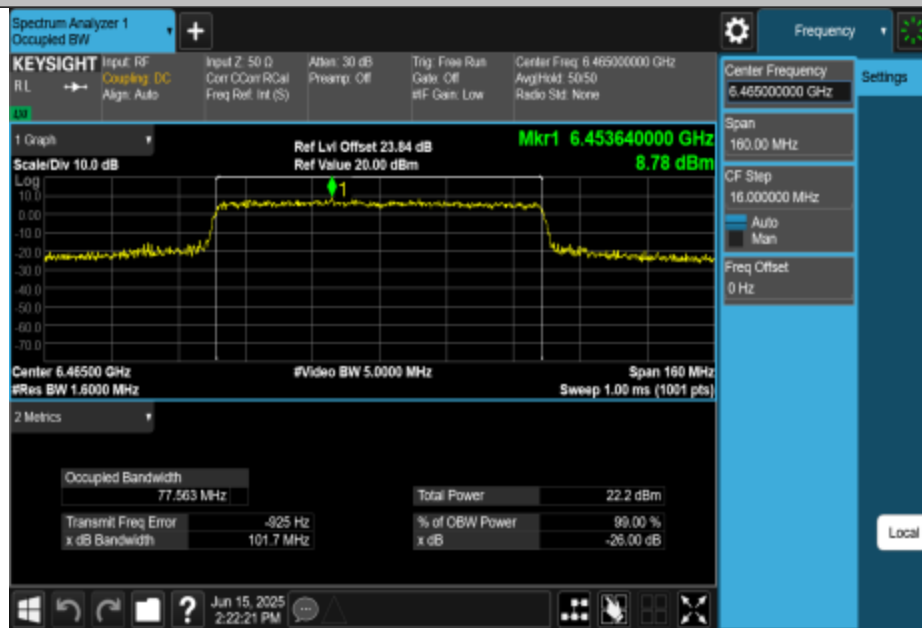
11BE80MIMO-Ant1-6465-PASS
