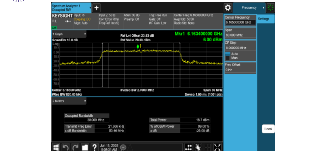
11BE40MIMO-Ant0-6165-PASS
