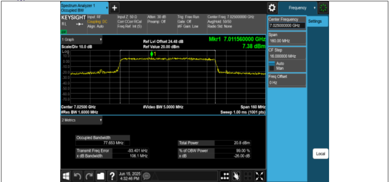
11BE80MIMO-Ant0-7025-PASS
