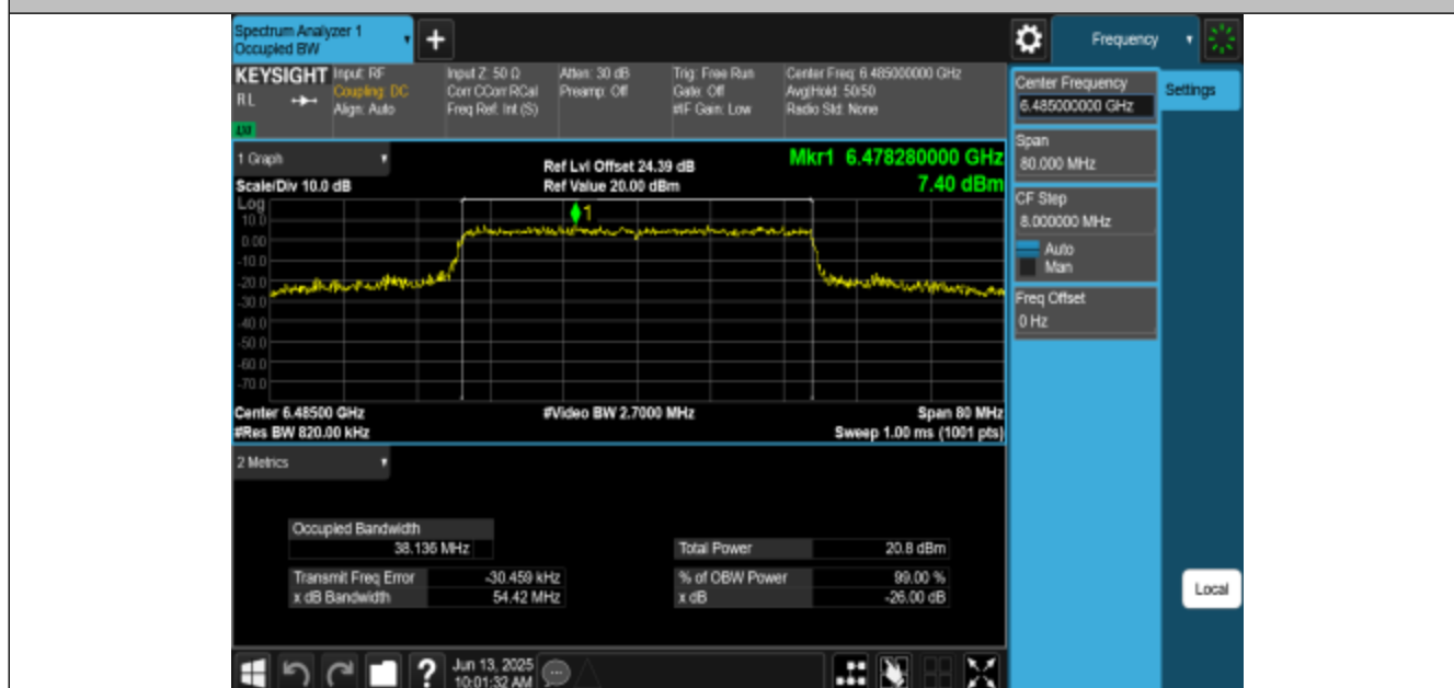
11BE40MIMO-Ant1-6485-PASS
