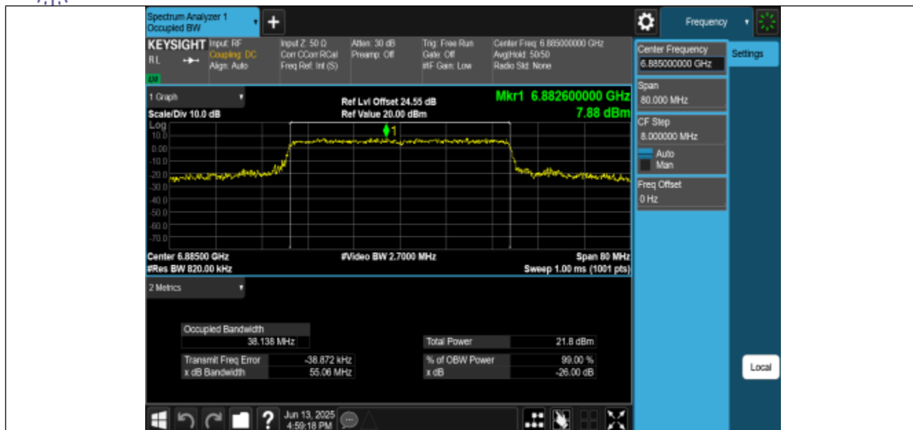
11BE40MIMO-Ant2-6885-PASS
