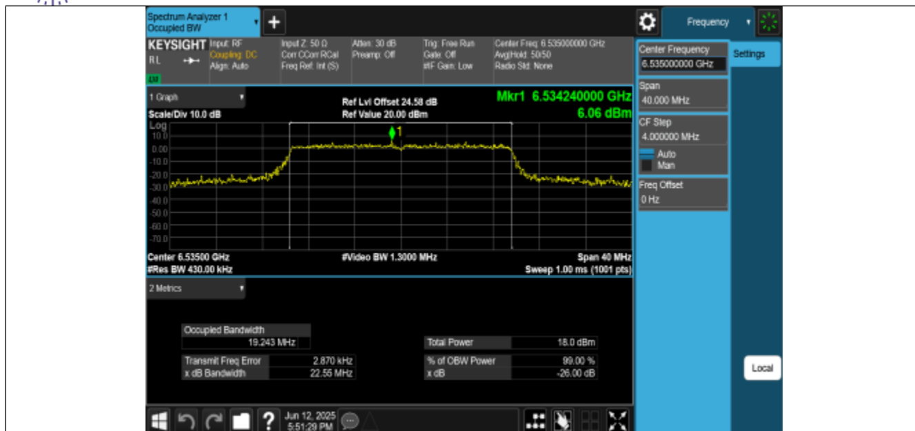
11BE20MIMO-Ant2-6535-PASS
