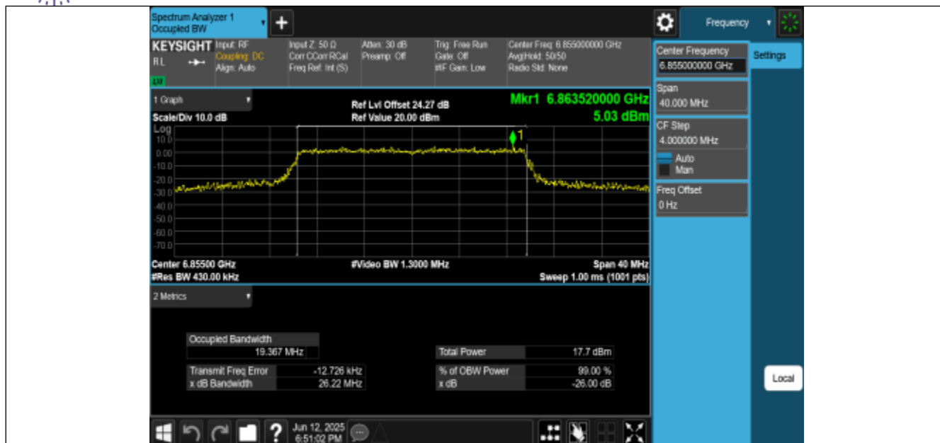
11BE20MIMO-Ant0-6855-PASS
