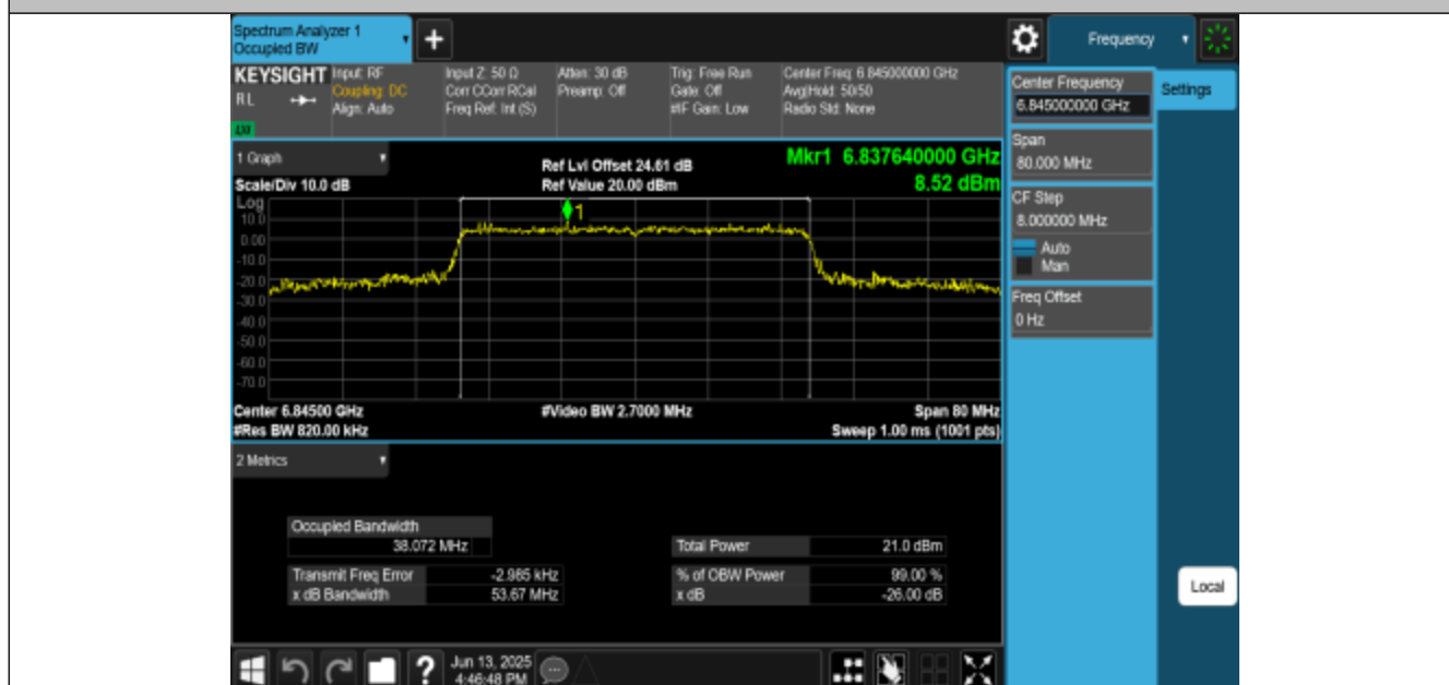
11BE40MIMO-Ant3-6845-PASS
