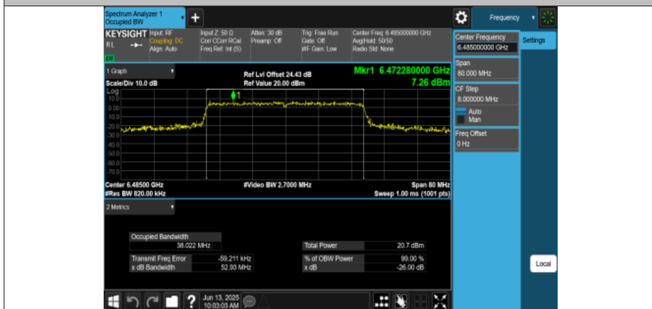
11BE40MIMO-Ant3-6485-PASS
