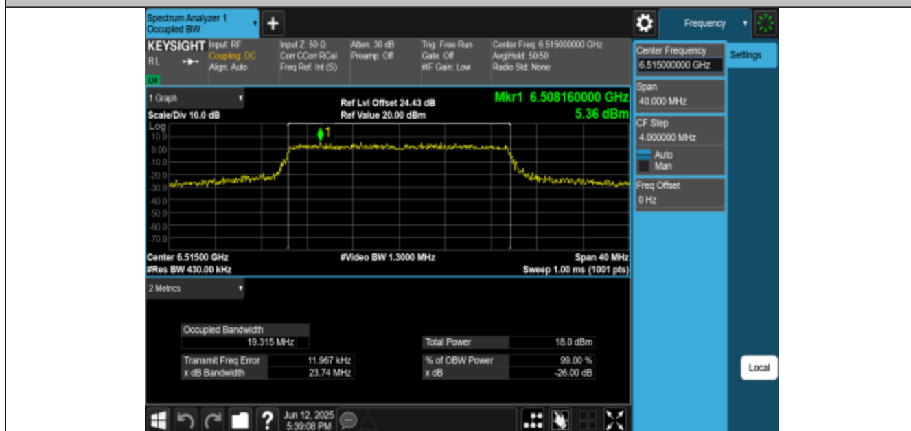
11BE20MIMO-Ant3-6515-PASS
