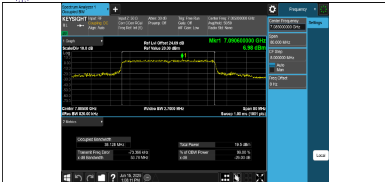
11BE40MIMO-Ant0-7085-PASS
