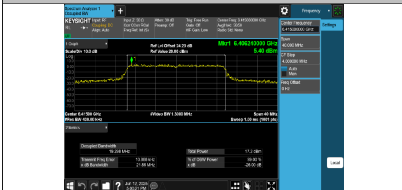
11BE20MIMO-Ant3-6415-PASS
