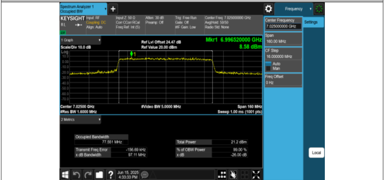
11BE80MIMO-Ant1-7025-PASS
