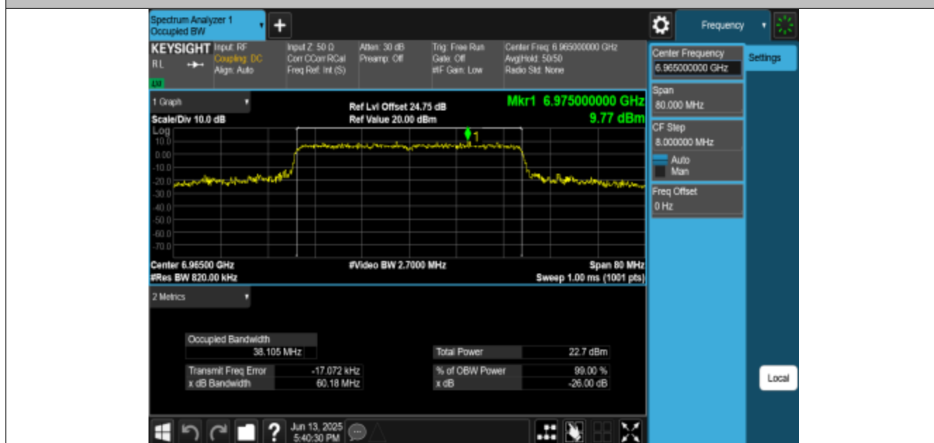
11BE40MIMO-Ant1-6965-PASS
