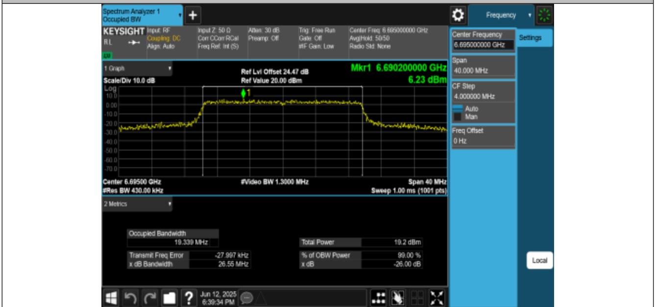
11BE20MIMO-Ant3-6695-PASS
