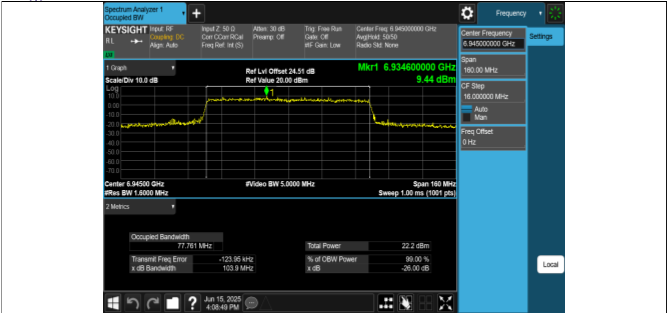
11BE80MIMO-Ant0-6945-PASS
