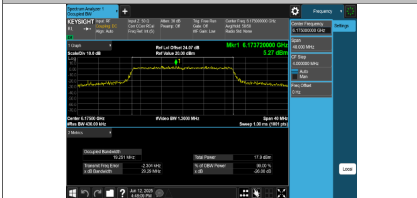
11BE20MIMO-Ant3-6175-PASS
