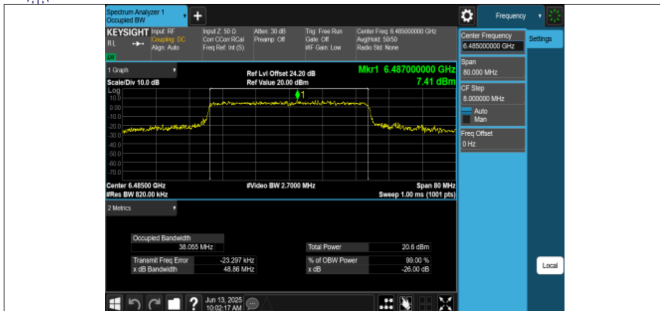
11BE40MIMO-Ant2-6485-PASS
