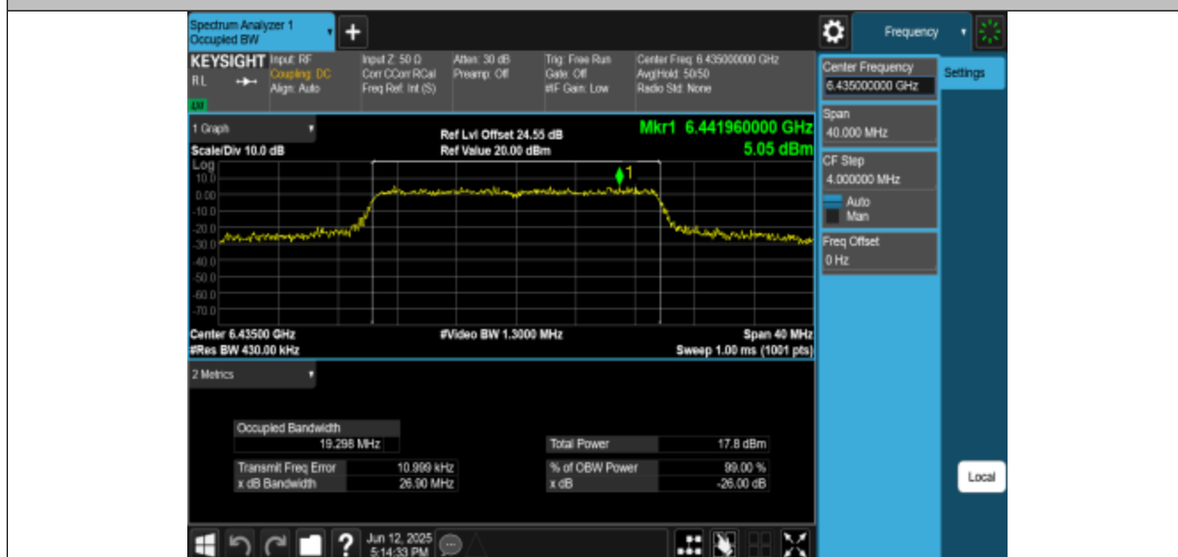
11BE20MIMO-Ant3-6435-PASS
