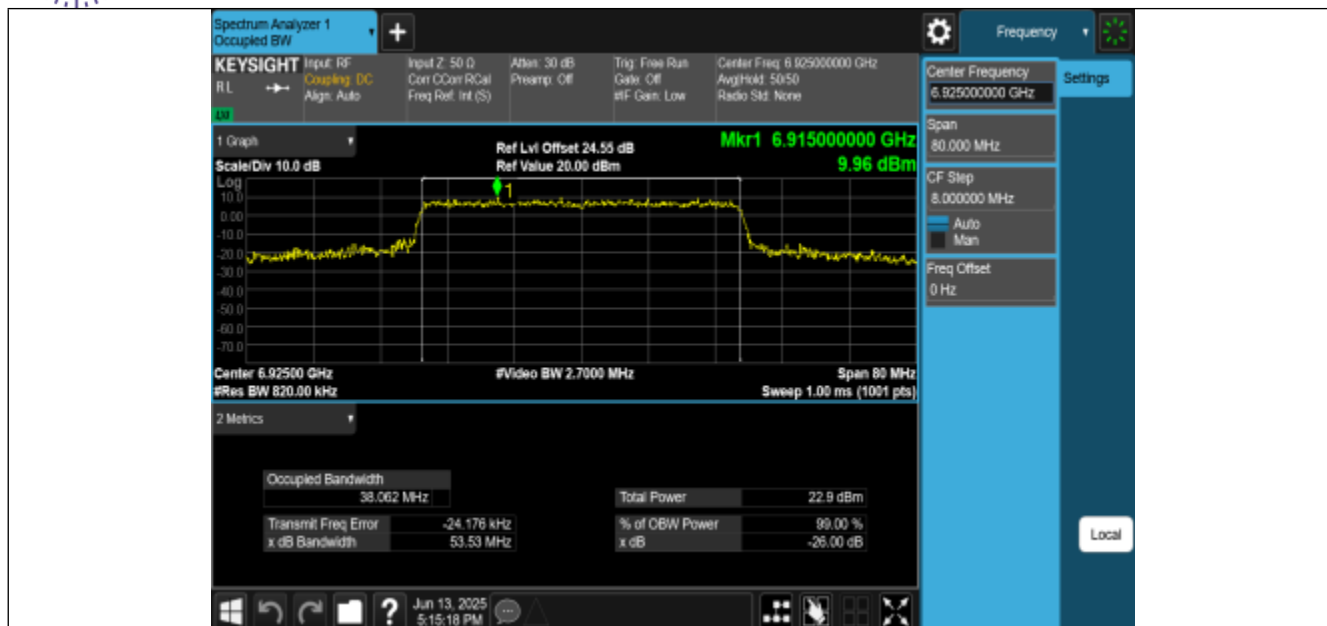
11BE40MIMO-Ant2-6925-PASS
