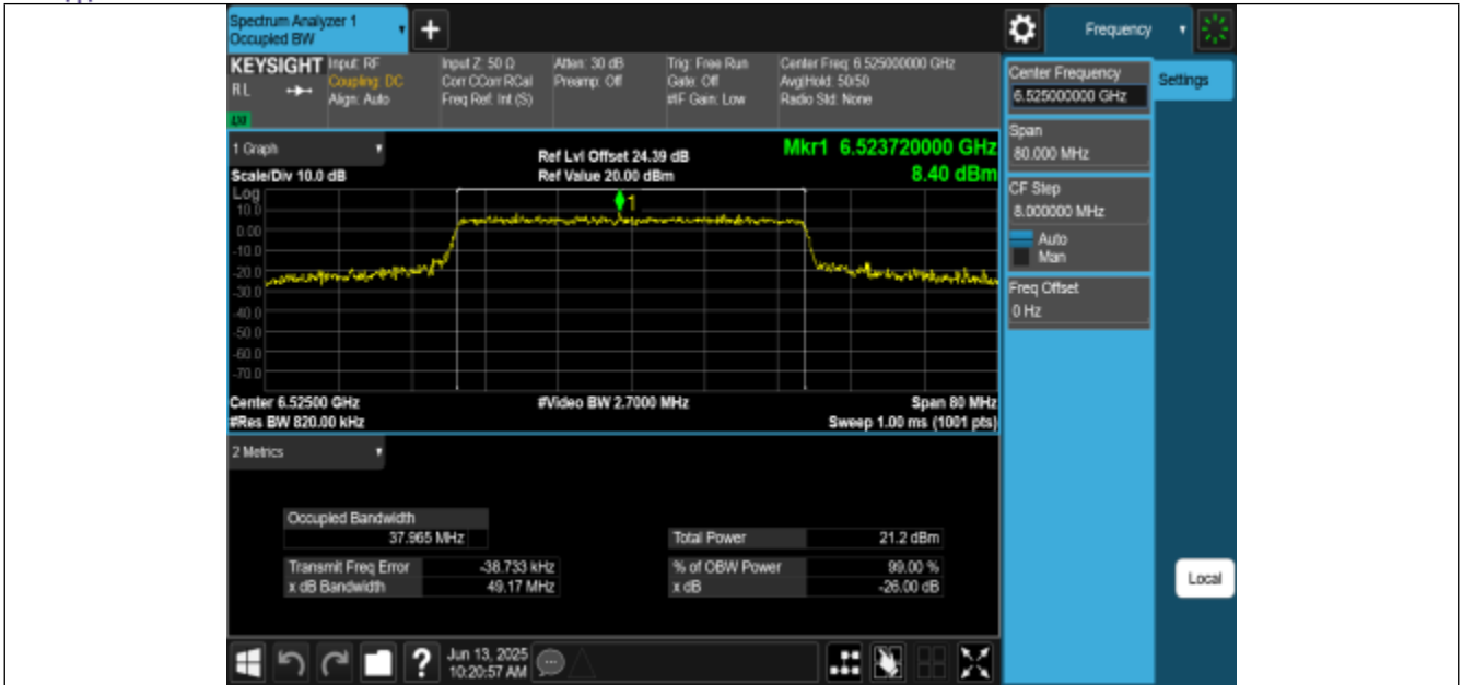
11BE40MIMO-Ant0-6525-PASS
