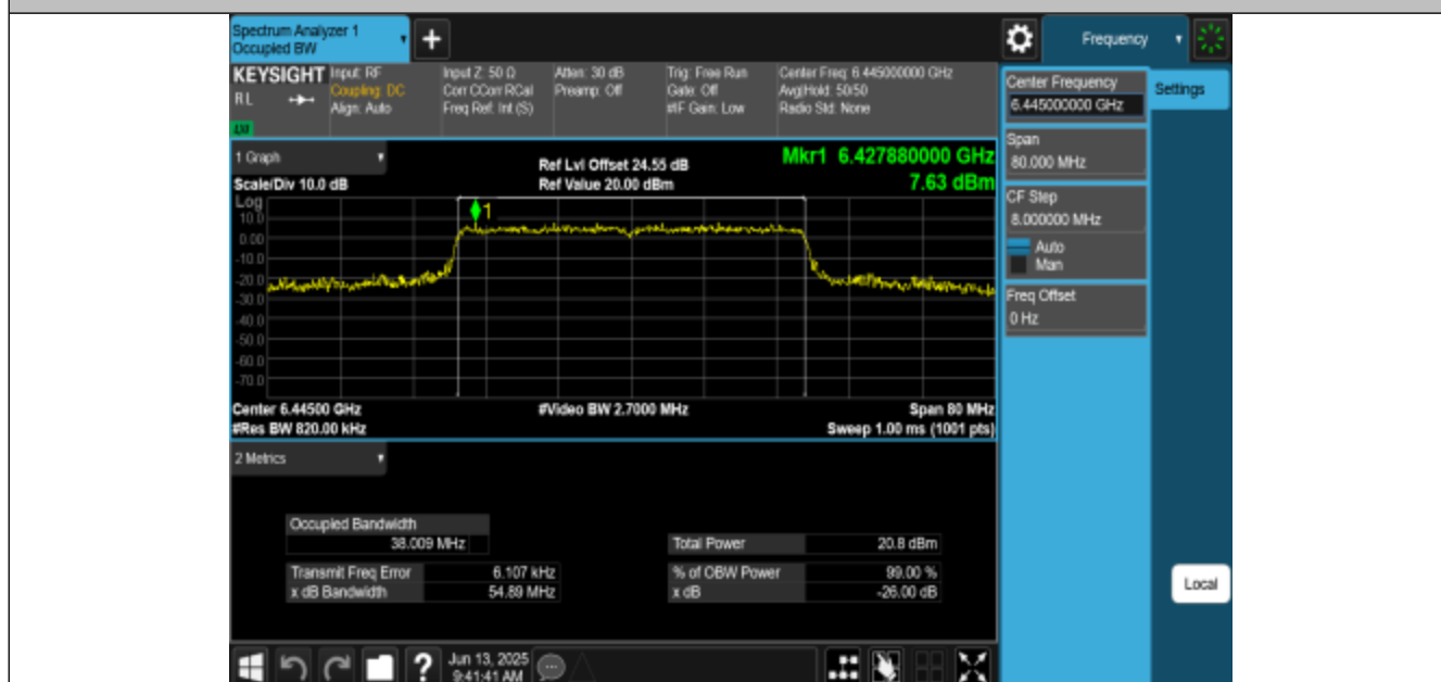
11BE40MIMO-Ant3-6445-PASS
