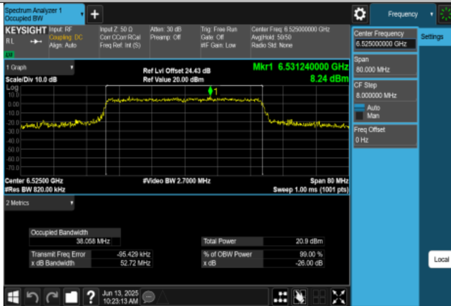
11BE40MIMO-Ant3-6525-PASS
