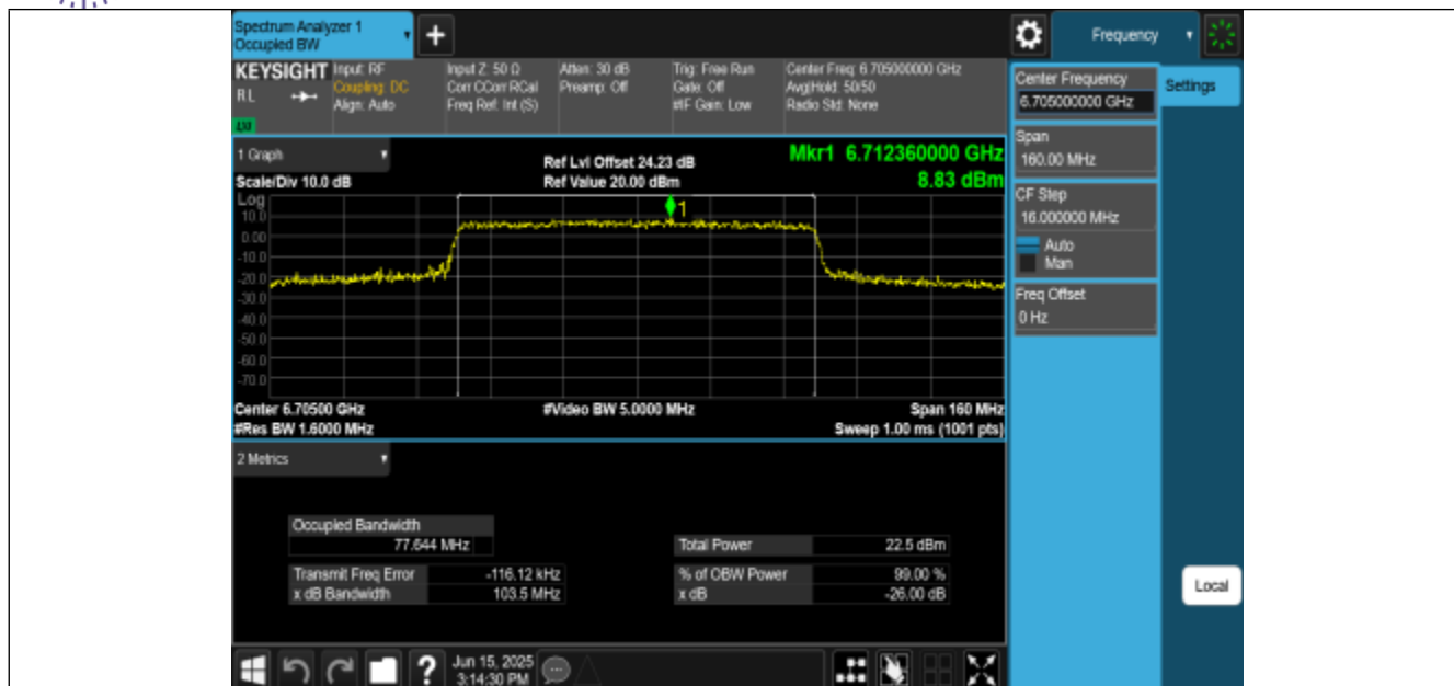
11BE80MIMO-Ant2-6705-PASS
