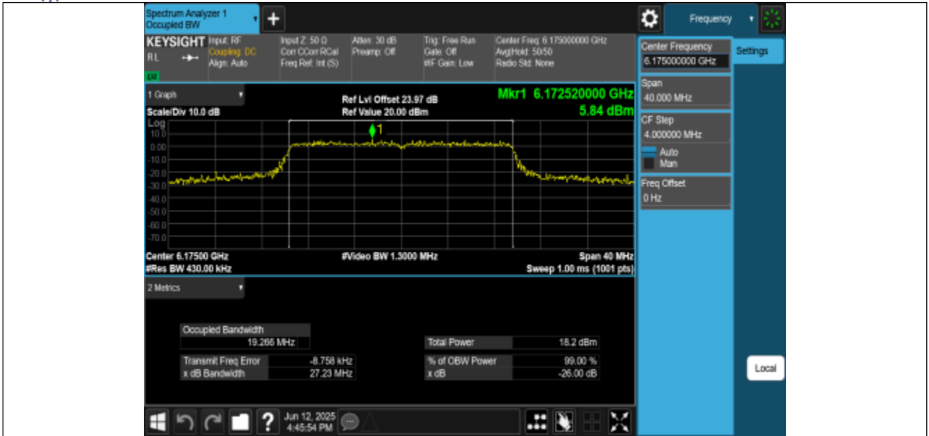
11BE20MIMO-Ant0-6175-PASS
