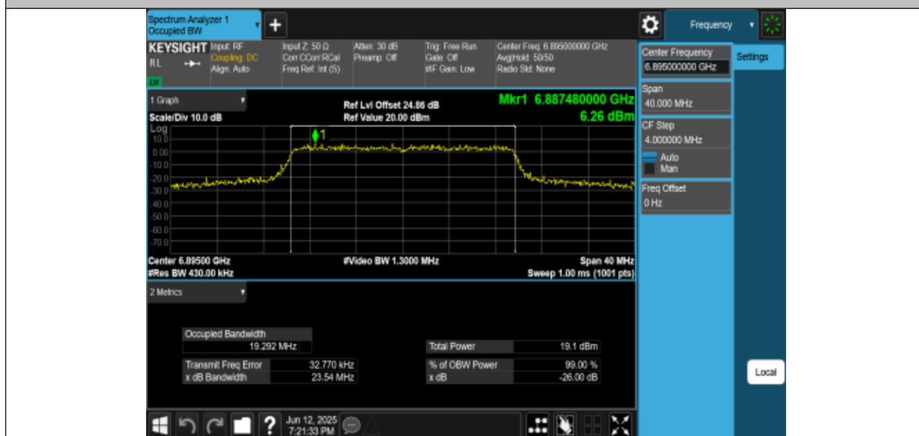
11BE20MIMO-Ant3-6895-PASS
