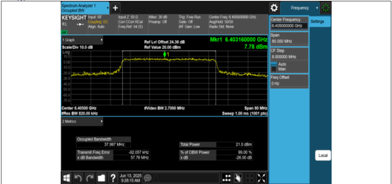
11BE40MIMO-Ant2-6405-PASS
