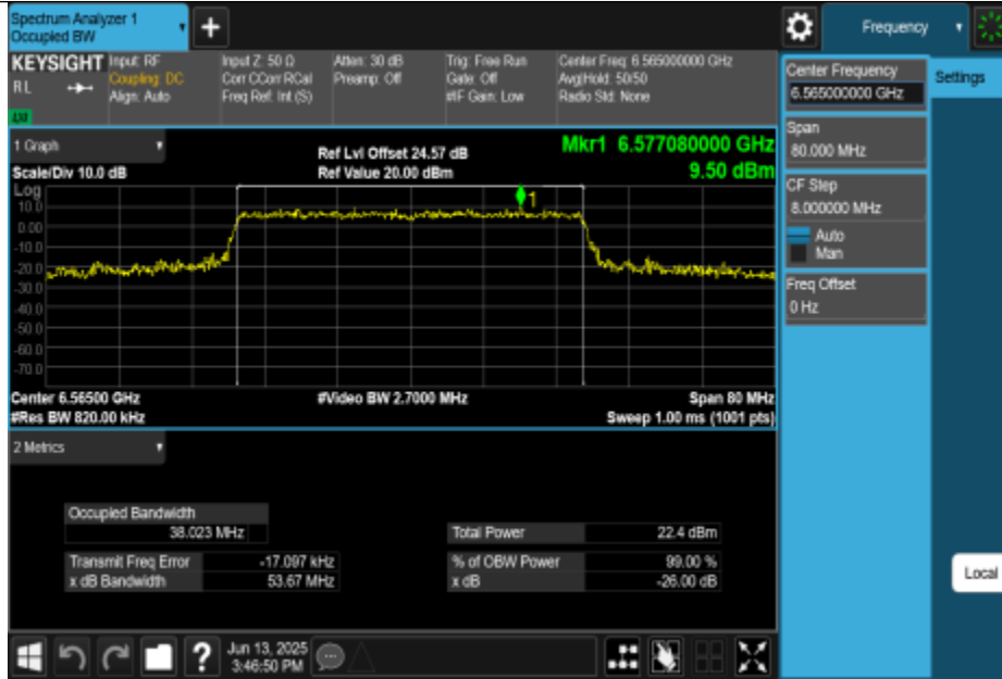
11BE40MIMO-Ant3-6565-PASS
