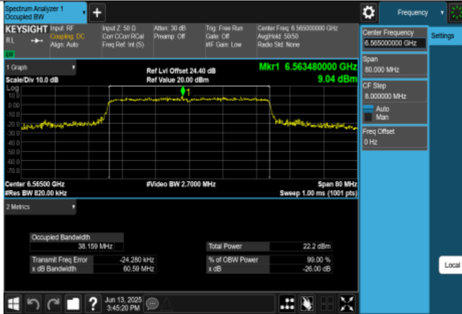
11BE40MIMO-Ant1-6565-PASS
