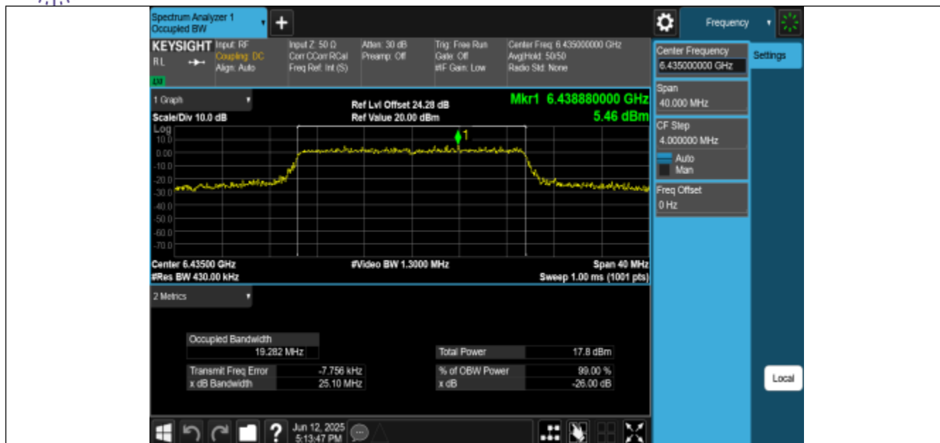
11BE20MIMO-Ant2-6435-PASS
