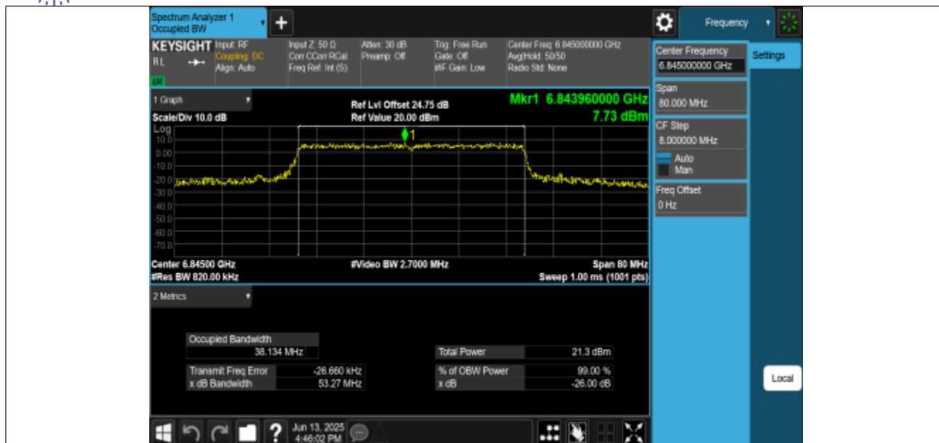
11BE40MIMO-Ant2-6845-PASS
