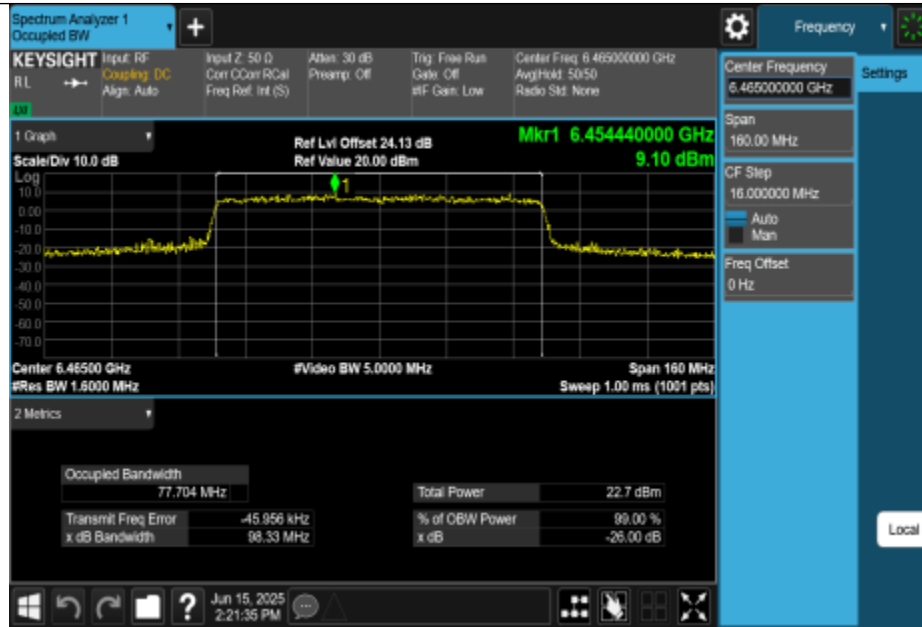
11BE80MIMO-Ant0-6465-PASS
