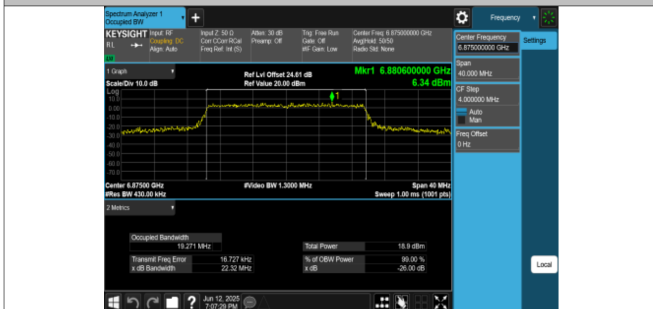
11BE20MIMO-Ant3-6875-PASS
