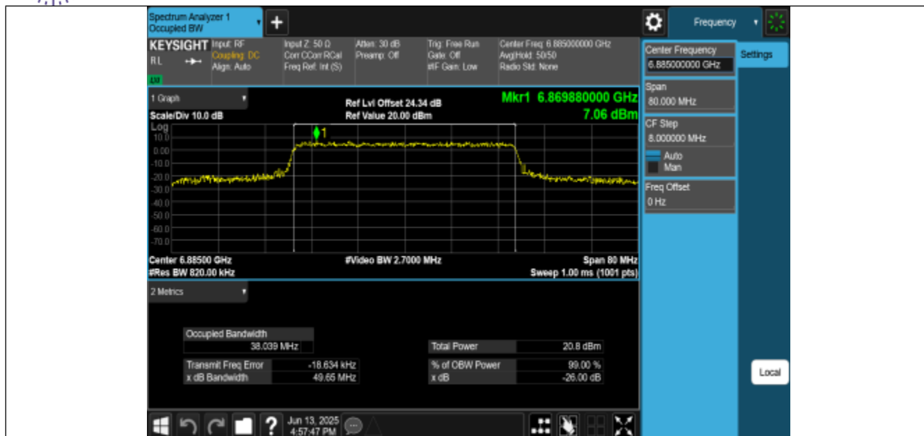
11BE40MIMO-Ant0-6885-PASS
