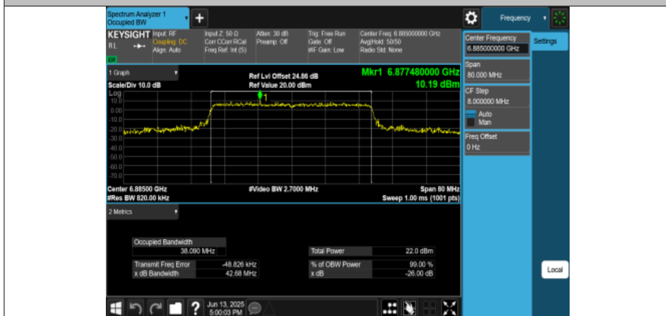
11BE40MIMO-Ant3-6885-PASS
