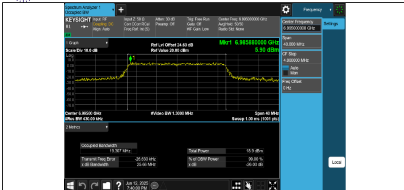
11BE20MIMO-Ant2-6995-PASS
