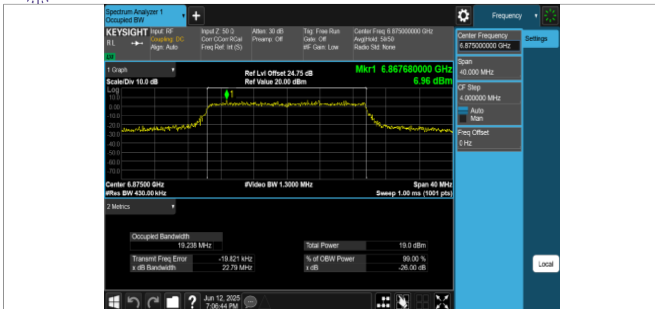
11BE20MIMO-Ant2-6875-PASS
