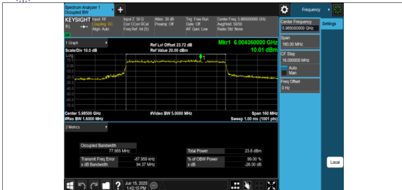
11BE80MIMO-Ant2-5985-PASS
