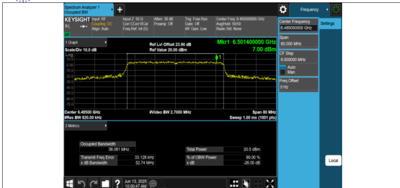
11BE40MIMO-Ant0-6485-PASS
