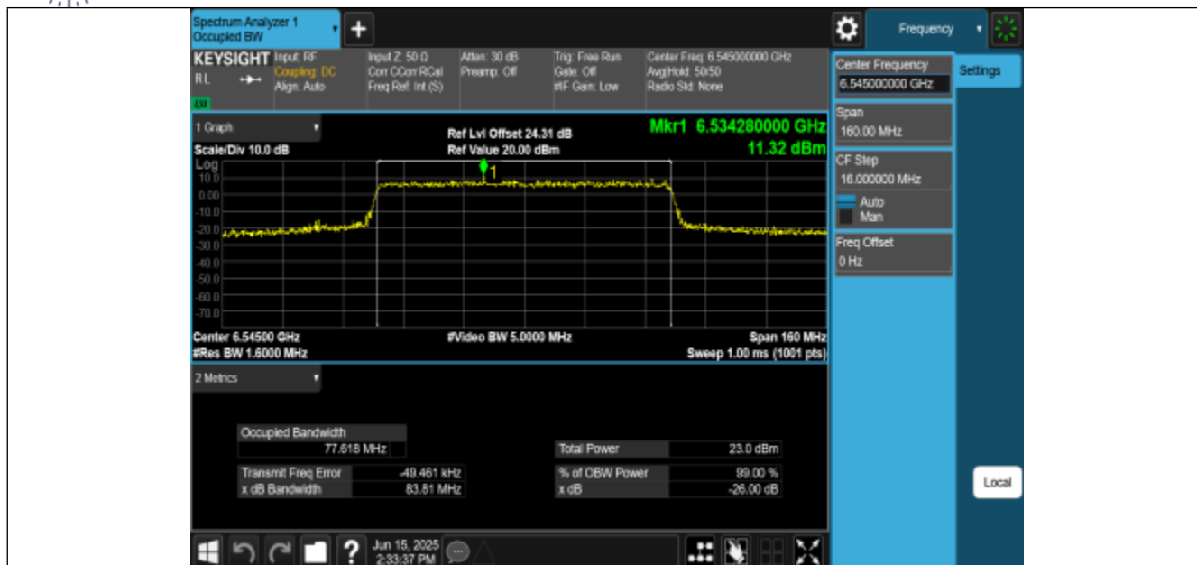
11BE80MIMO-Ant0-6545-PASS
