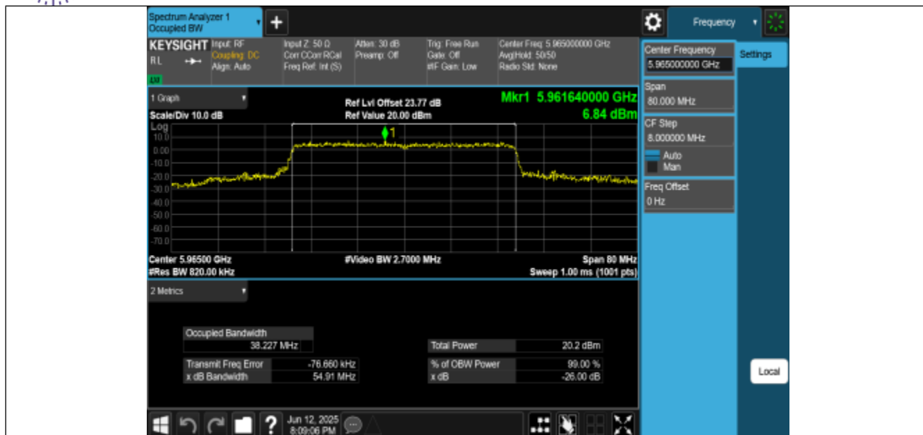
11BE40MIMO-Ant2-5965-PASS
