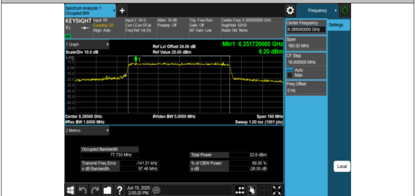
11BE80MIMO-Ant1-6385-PASS
