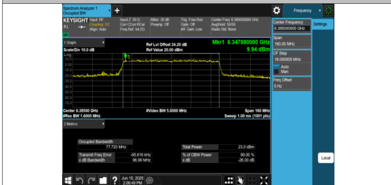
11BE80MIMO-Ant3-6385-PASS
