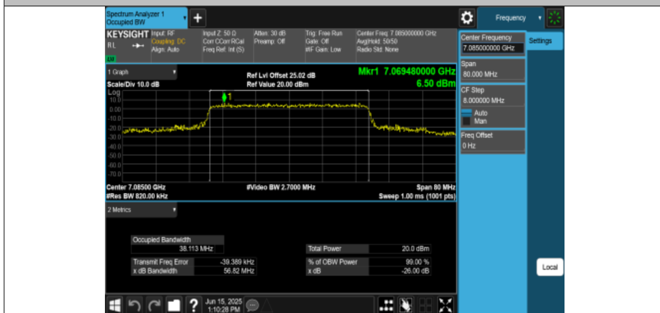
11BE40MIMO-Ant3-7085-PASS
