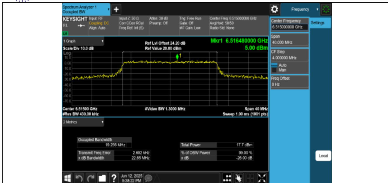
11BE20MIMO-Ant2-6515-PASS
