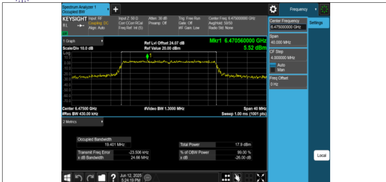
11BE20MIMO-Ant0-6475-PASS
