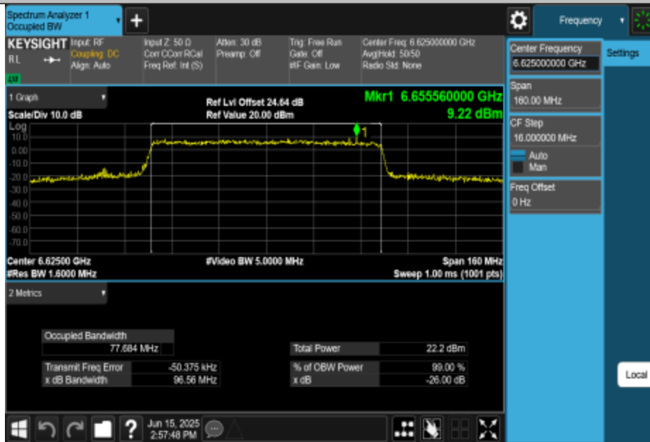
11BE80MIMO-Ant3-6625-PASS
