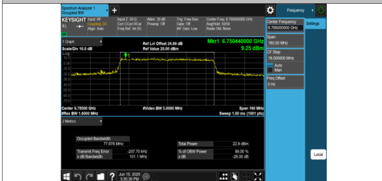
11BE80MIMO-Ant3-6785-PASS
