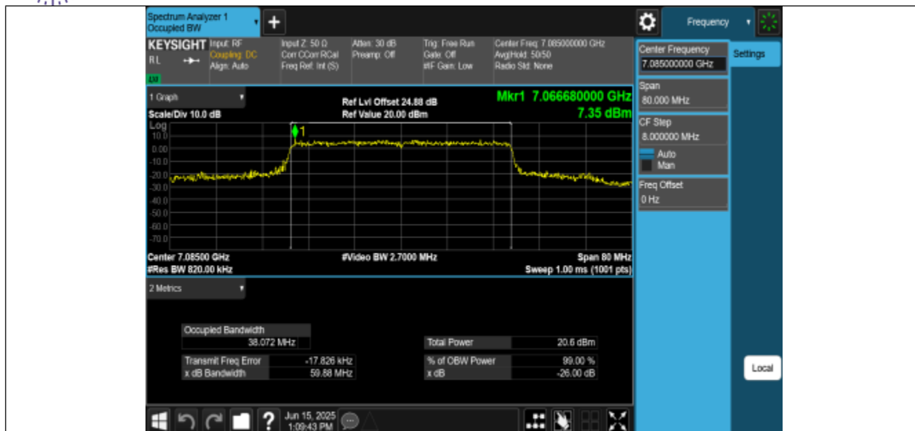
11BE40MIMO-Ant2-7085-PASS
