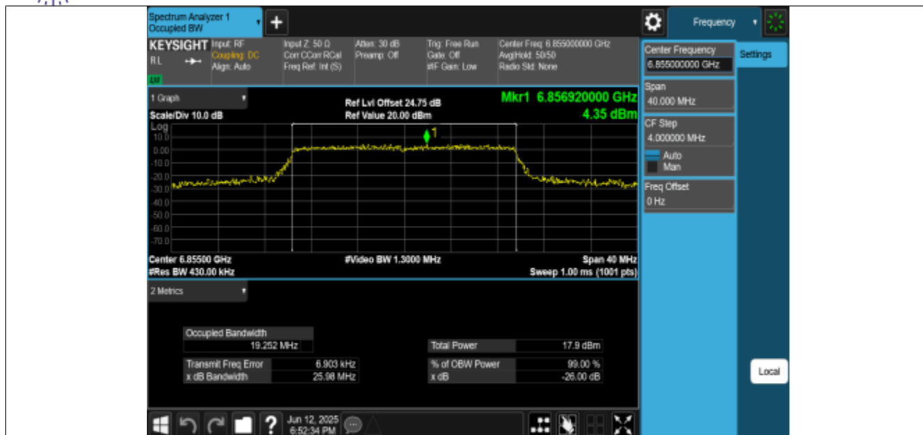
11BE20MIMO-Ant2-6855-PASS
