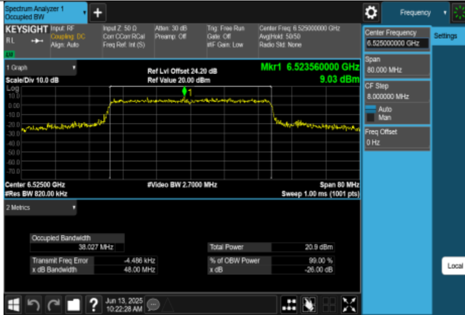
11BE40MIMO-Ant2-6525-PASS
