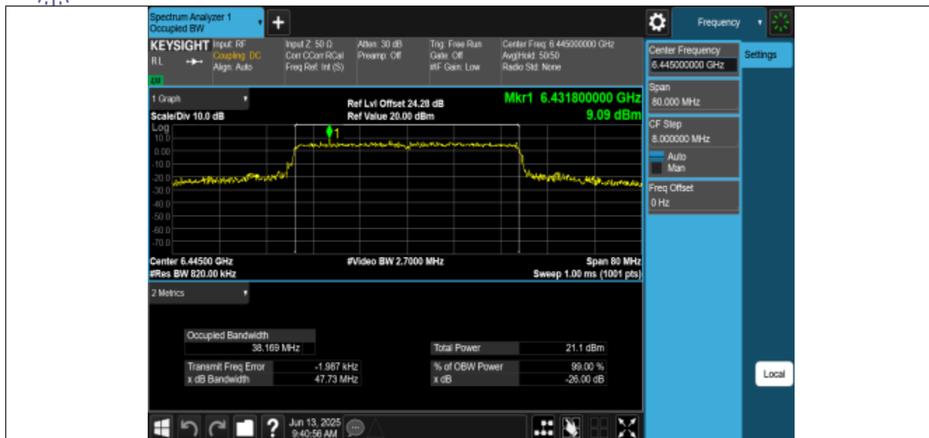
11BE40MIMO-Ant2-6445-PASS
