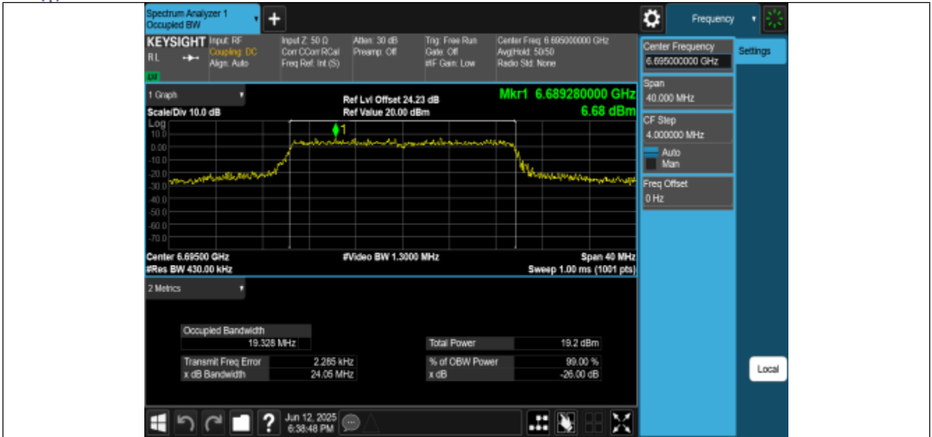
11BE20MIMO-Ant2-6695-PASS
