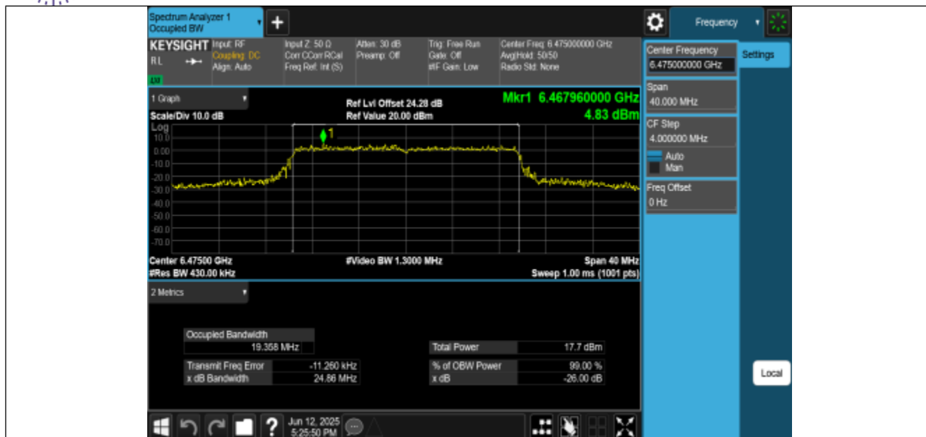
11BE20MIMO-Ant2-6475-PASS
