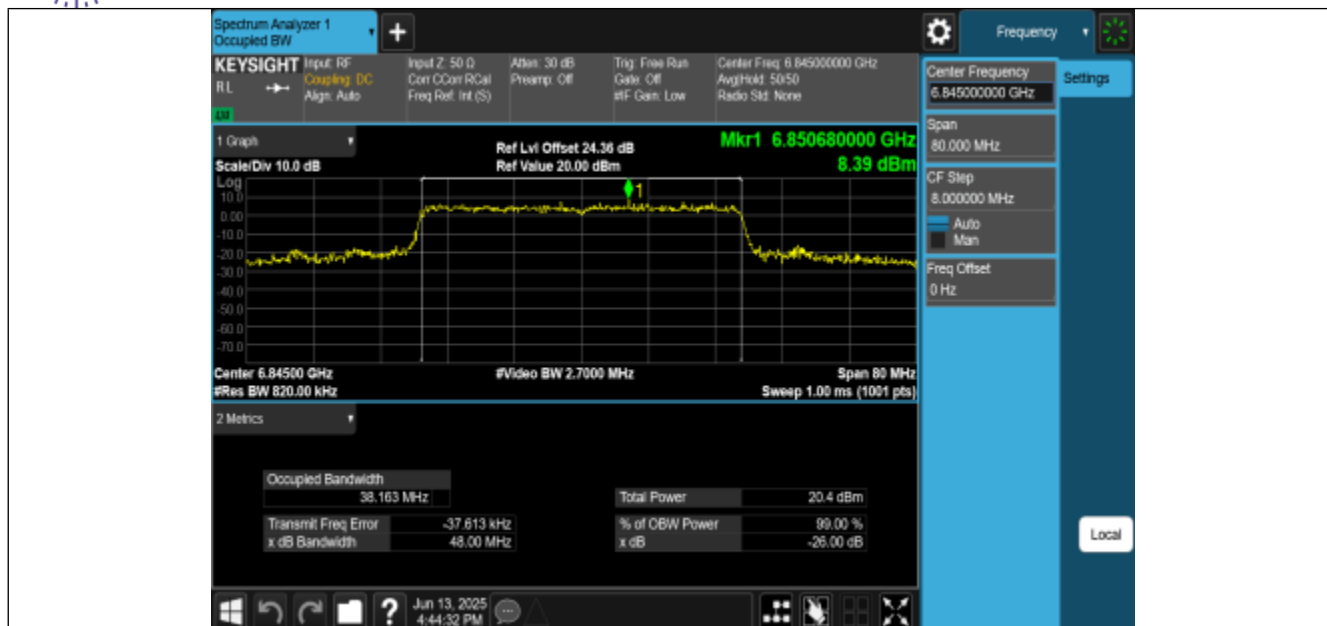
11BE40MIMO-Ant0-6845-PASS
