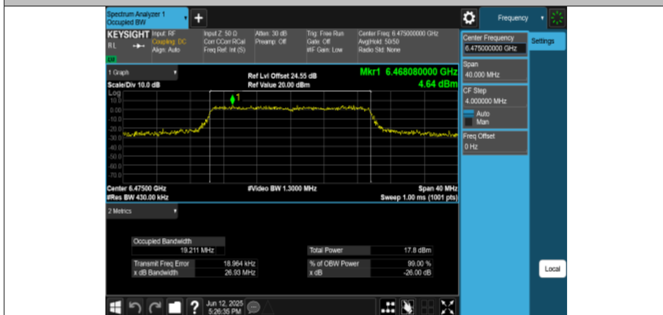
11BE20MIMO-Ant3-6475-PASS
