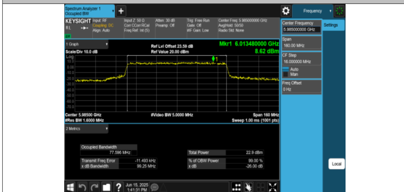
11BE80MIMO-Ant1-5985-PASS
