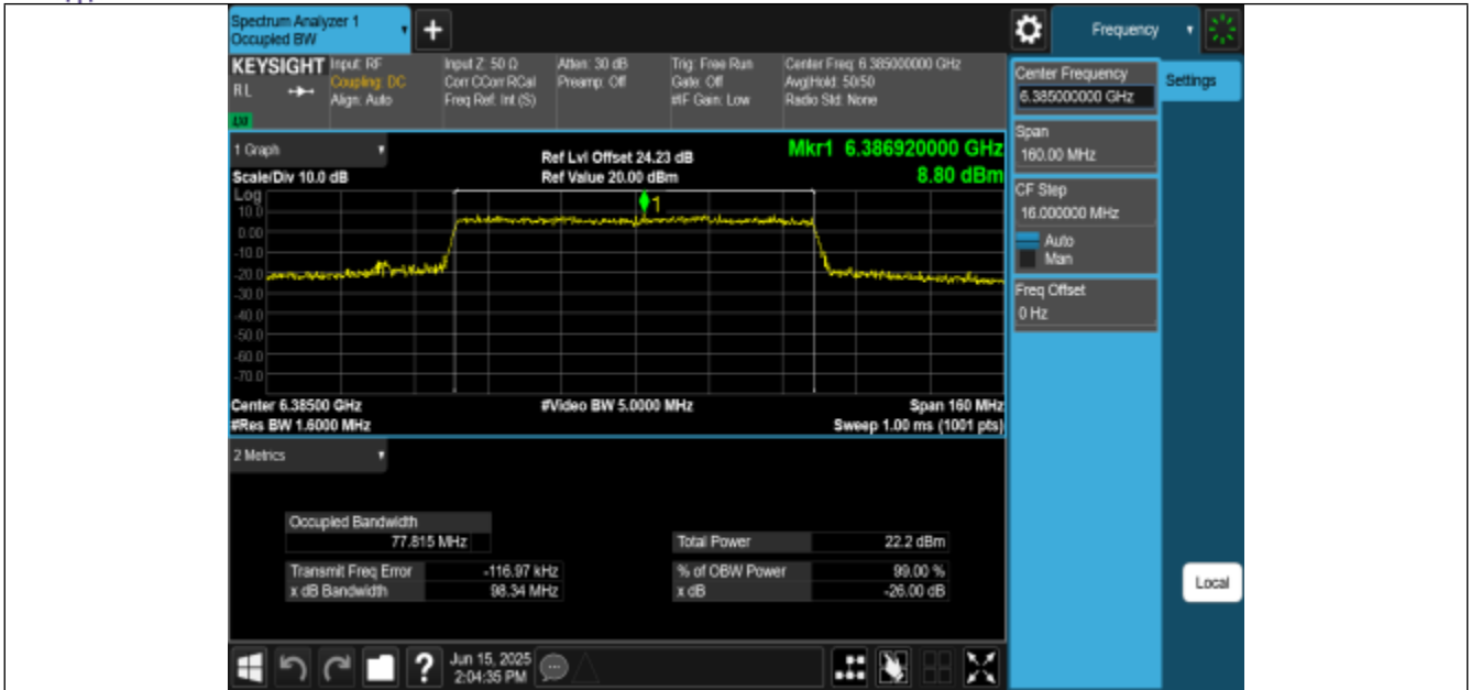
11BE80MIMO-Ant0-6385-PASS
