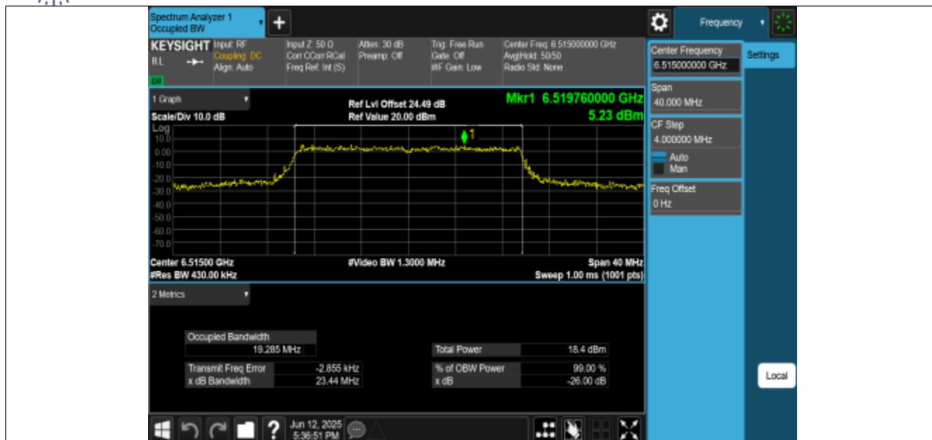
11BE20MIMO-Ant0-6515-PASS
