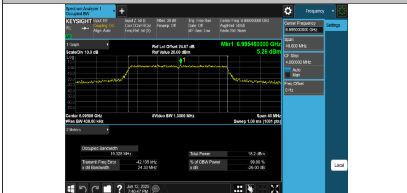
11BE20MIMO-Ant3-6995-PASS
