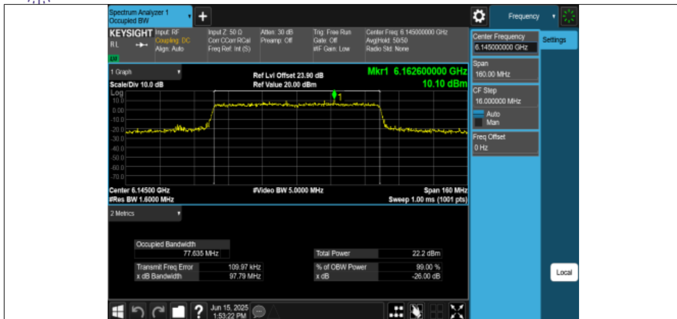
11BE80MIMO-Ant0-6145-PASS
