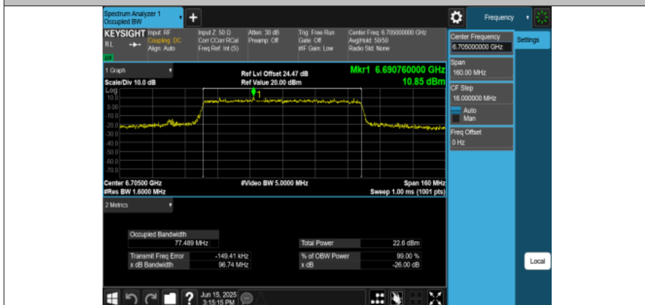
11BE80MIMO-Ant3-6705-PASS
