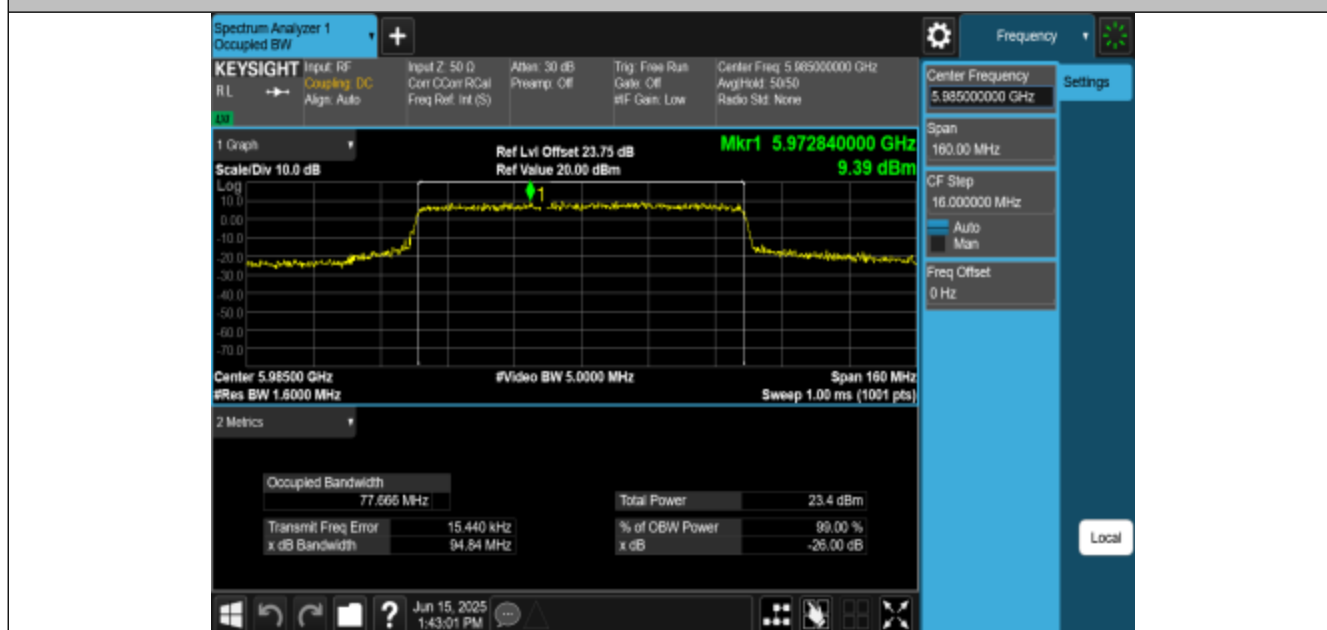
11BE80MIMO-Ant3-5985-PASS
