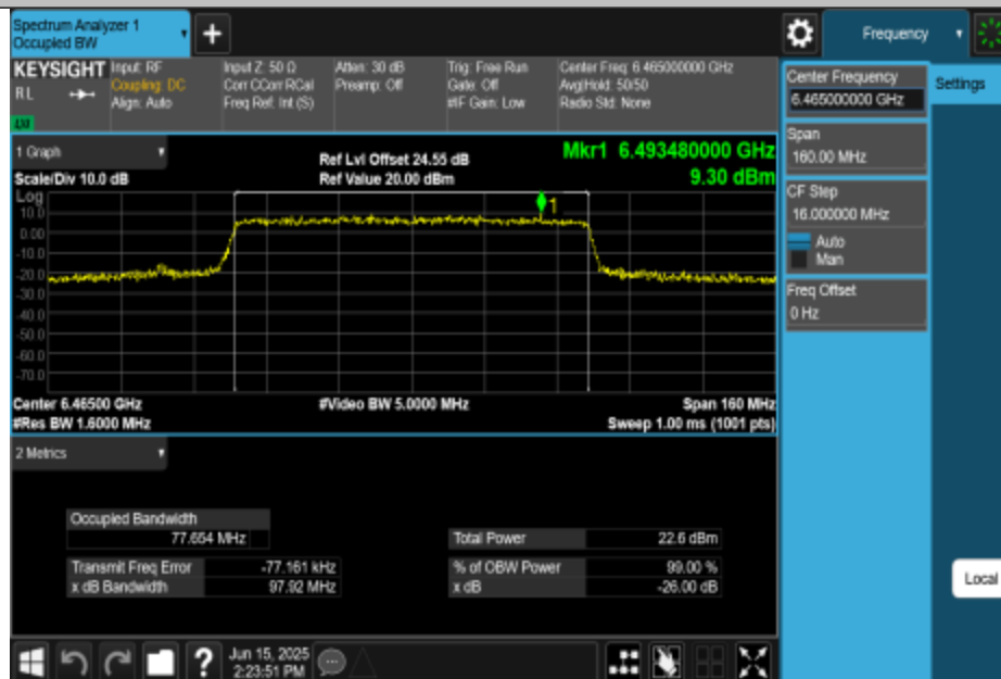
11BE80MIMO-Ant3-6465-PASS
