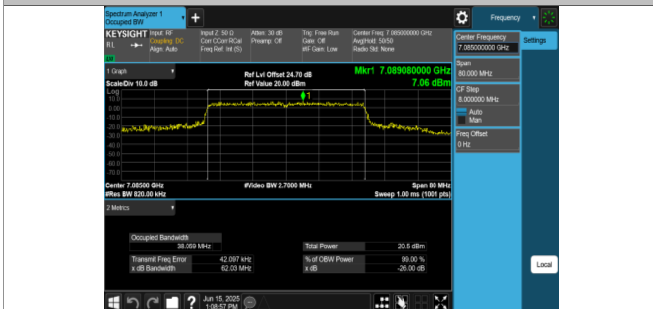
11BE40MIMO-Ant1-7085-PASS
