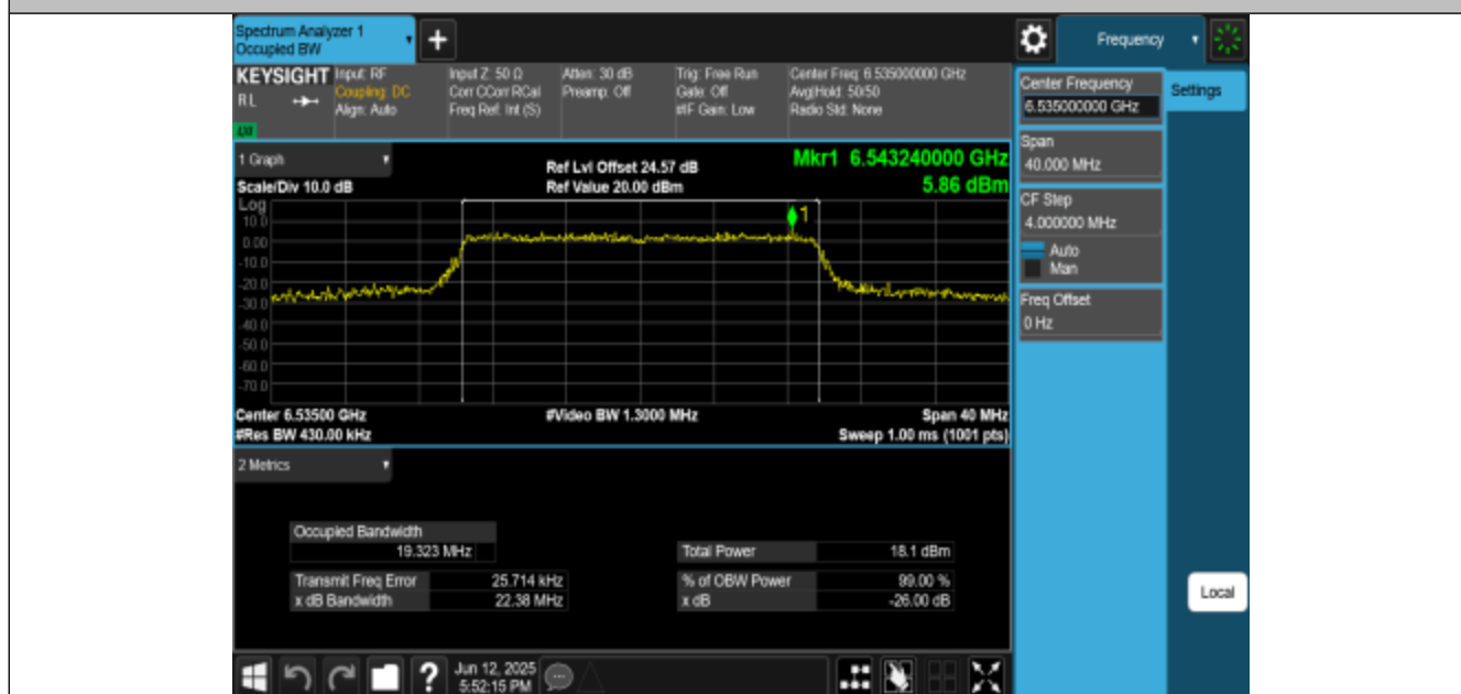
11BE20MIMO-Ant3-6535-PASS
