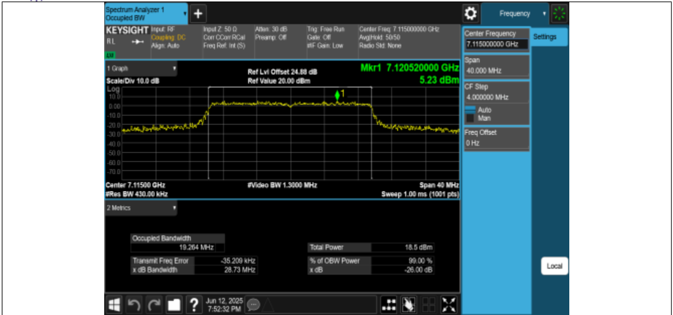
11BE20MIMO-Ant2-7115-PASS
