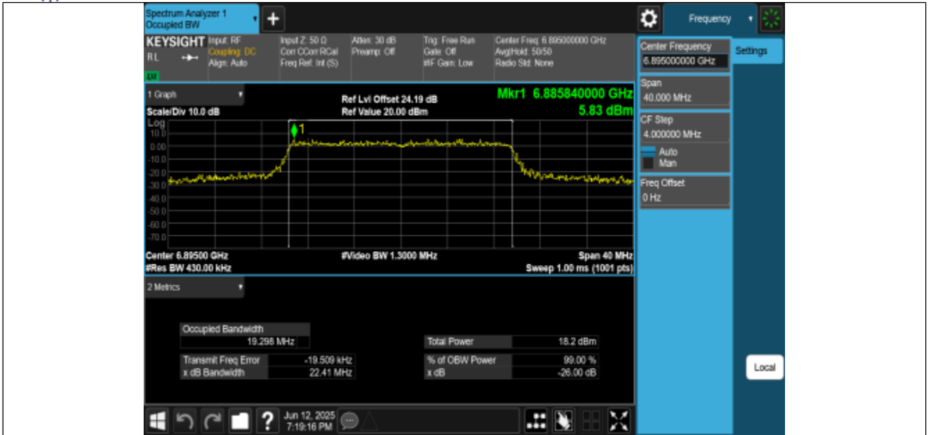
11BE20MIMO-Ant0-6895-PASS
