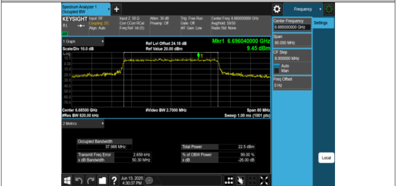
11BE40MIMO-Ant1-6685-PASS
