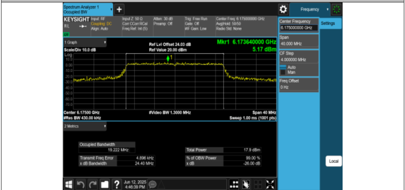
11BE20MIMO-Ant1-6175-PASS
