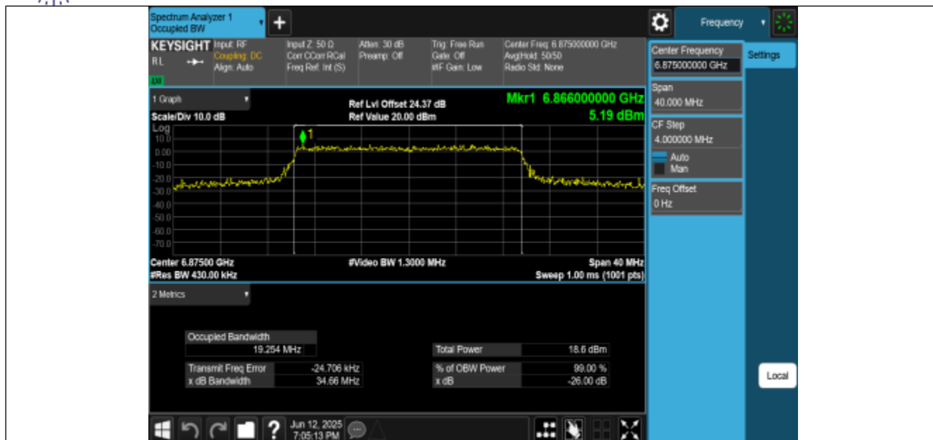
11BE20MIMO-Ant0-6875-PASS
