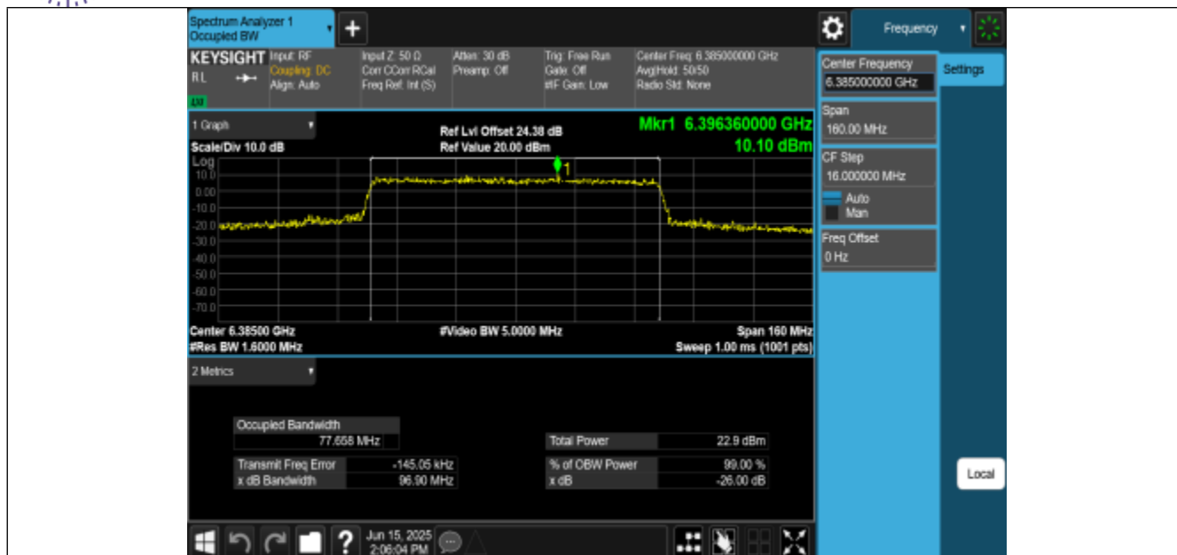
11BE80MIMO-Ant2-6385-PASS
