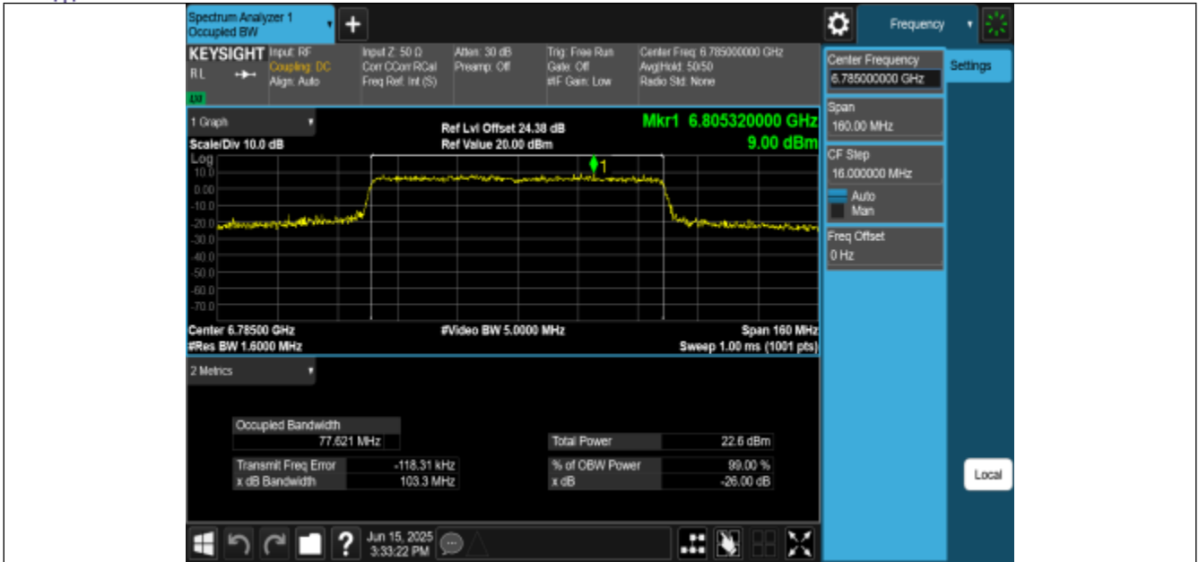
11BE80MIMO-Ant0-6785-PASS
