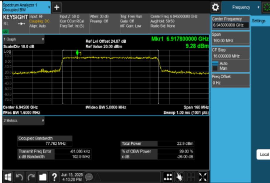
11BE80MIMO-Ant2-6945-PASS
