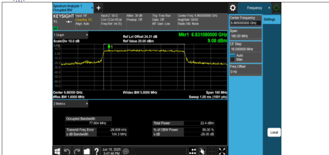
11BE80MIMO-Ant0-6865-PASS
