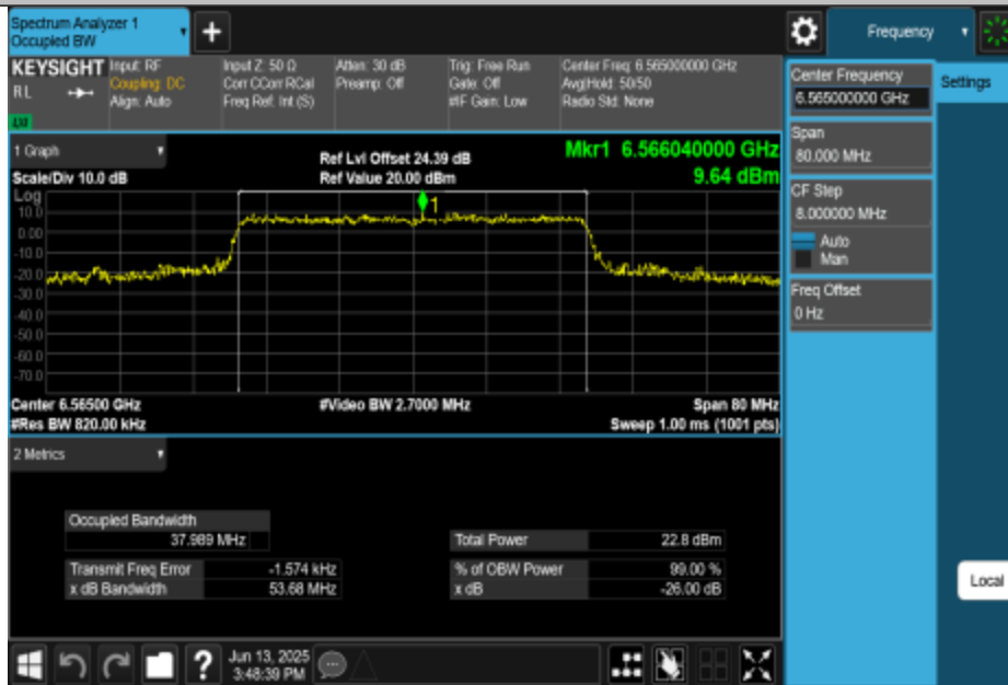
11BE40MIMO-Ant0-6565-PASS
