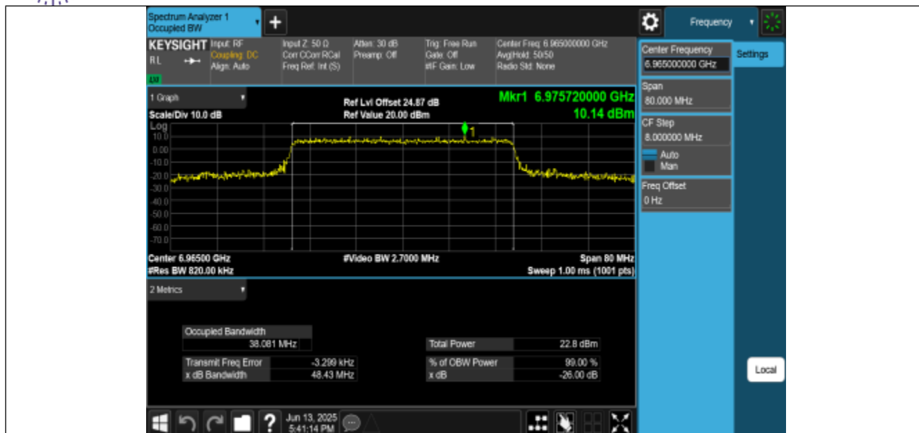
11BE40MIMO-Ant2-6965-PASS
