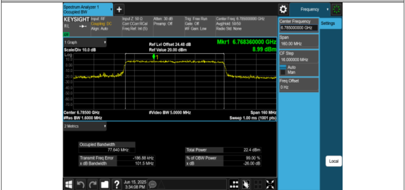
11BE80MIMO-Ant1-6785-PASS
