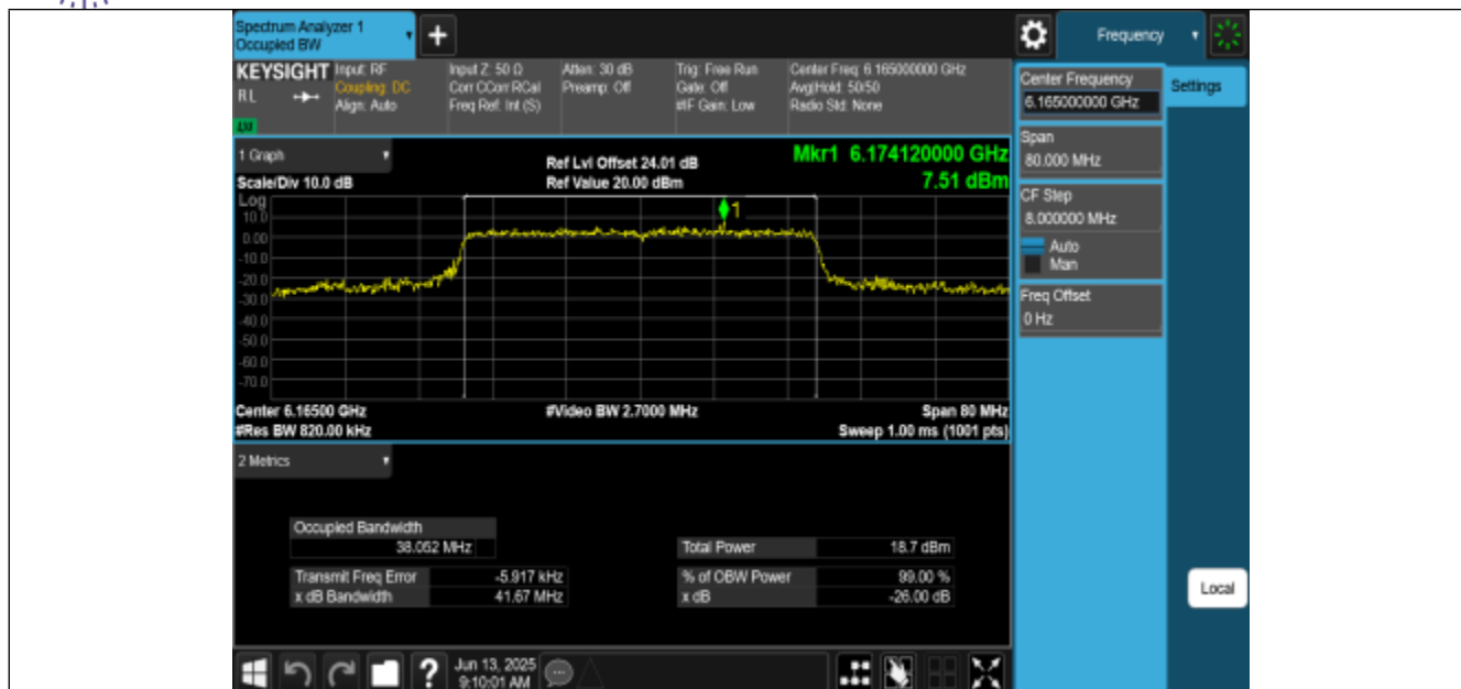
11BE40MIMO-Ant2-6165-PASS
