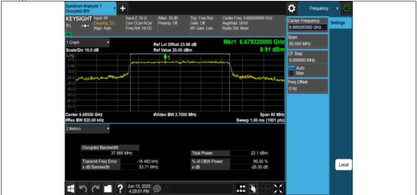
11BE40MIMO-Ant0-6685-PASS
