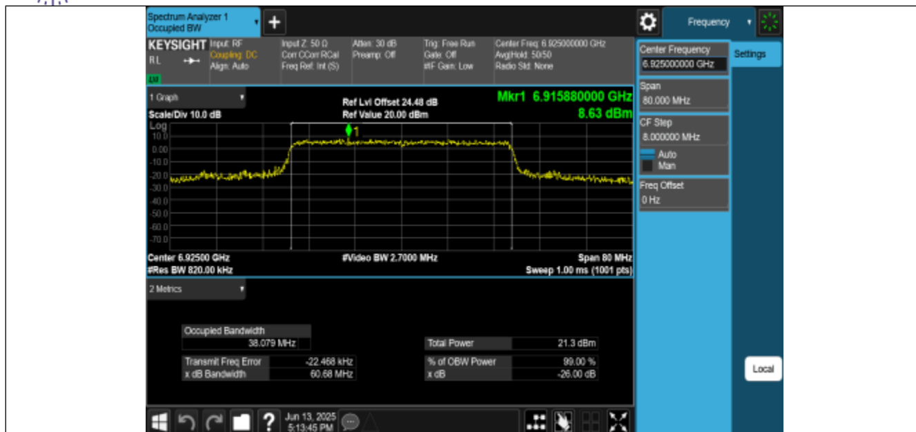
11BE40MIMO-Ant0-6925-PASS
