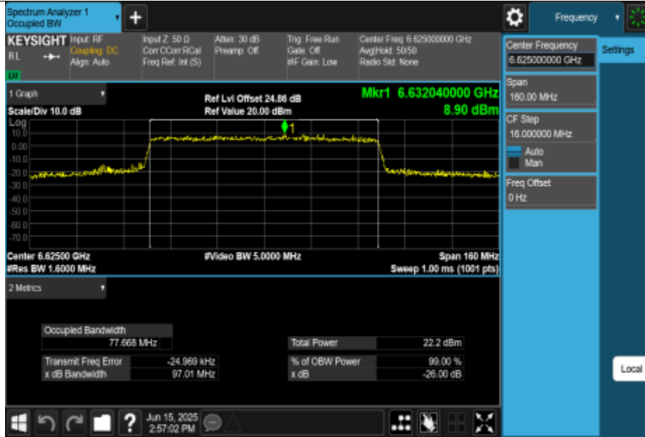
11BE80MIMO-Ant2-6625-PASS
