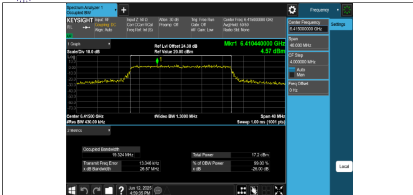
11BE20MIMO-Ant2-6415-PASS
