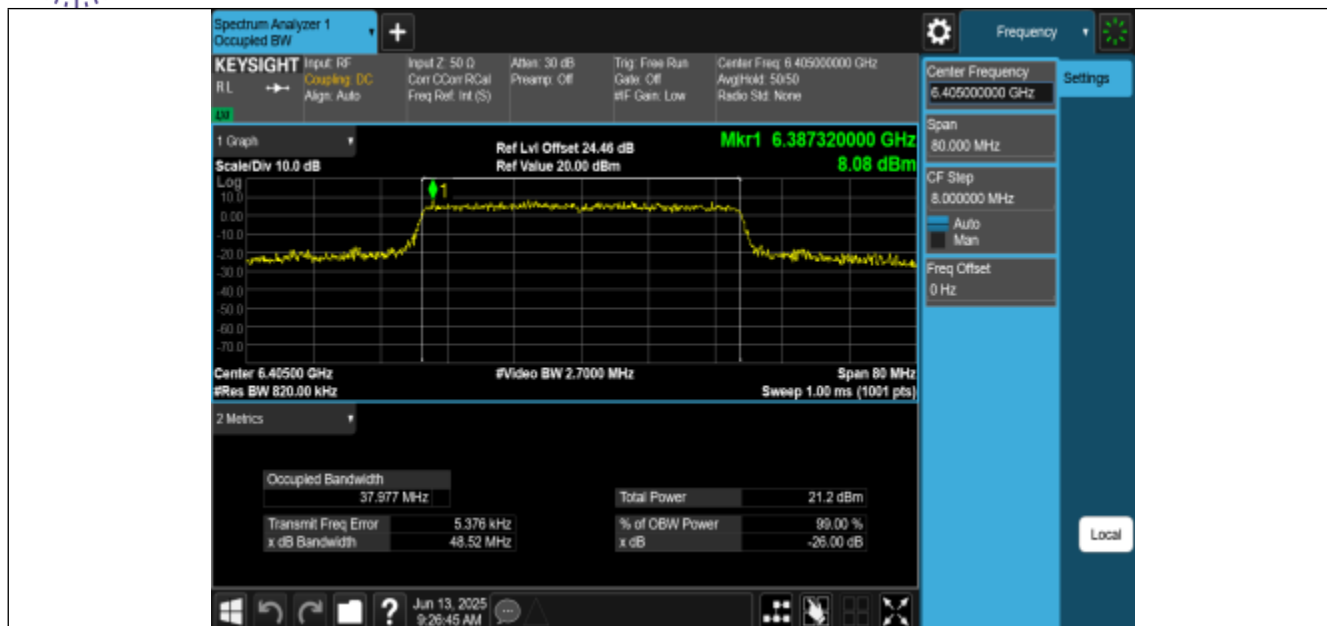
11BE40MIMO-Ant0-6405-PASS
