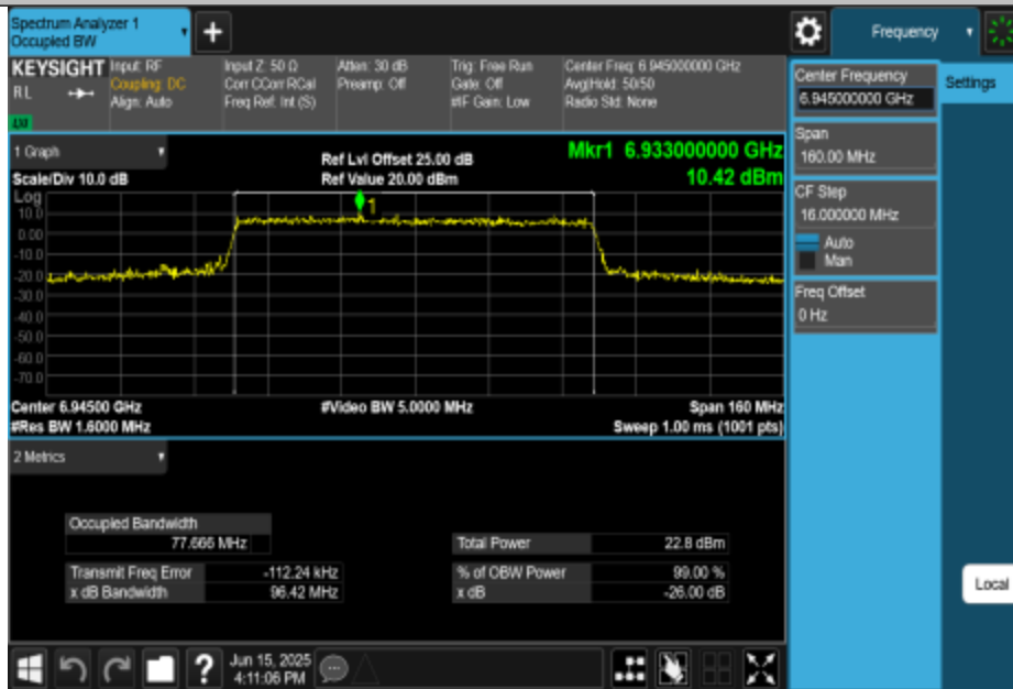
11BE80MIMO-Ant3-6945-PASS
