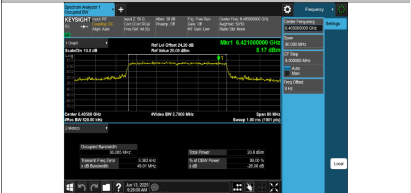
11BE40MIMO-Ant3-6405-PASS
