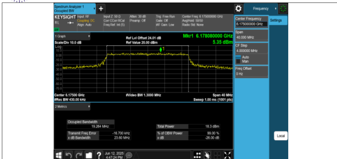
11BE20MIMO-Ant2-6175-PASS
