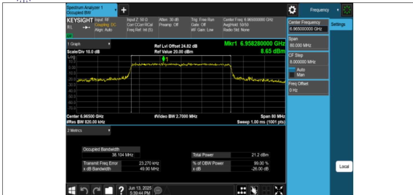
11BE40MIMO-Ant0-6965-PASS
