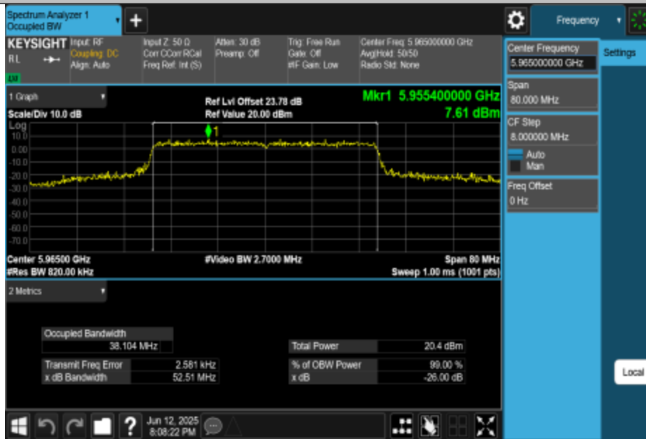
11BE40MIMO-Ant1-5965-PASS
