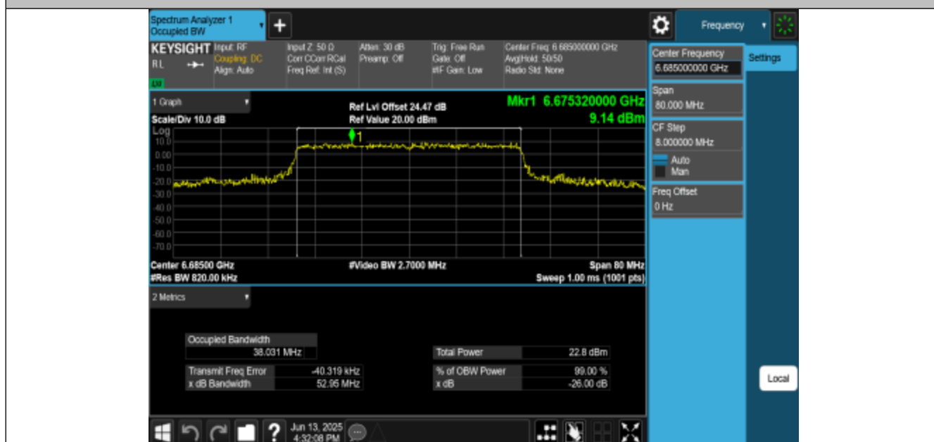
11BE40MIMO-Ant3-6685-PASS
