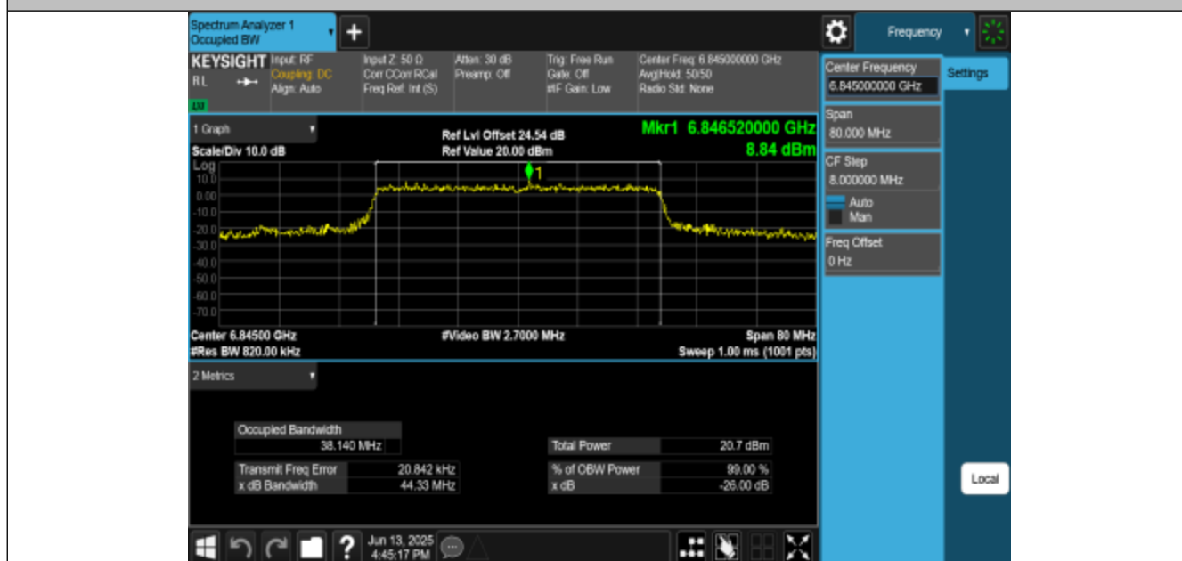
11BE40MIMO-Ant1-6845-PASS
