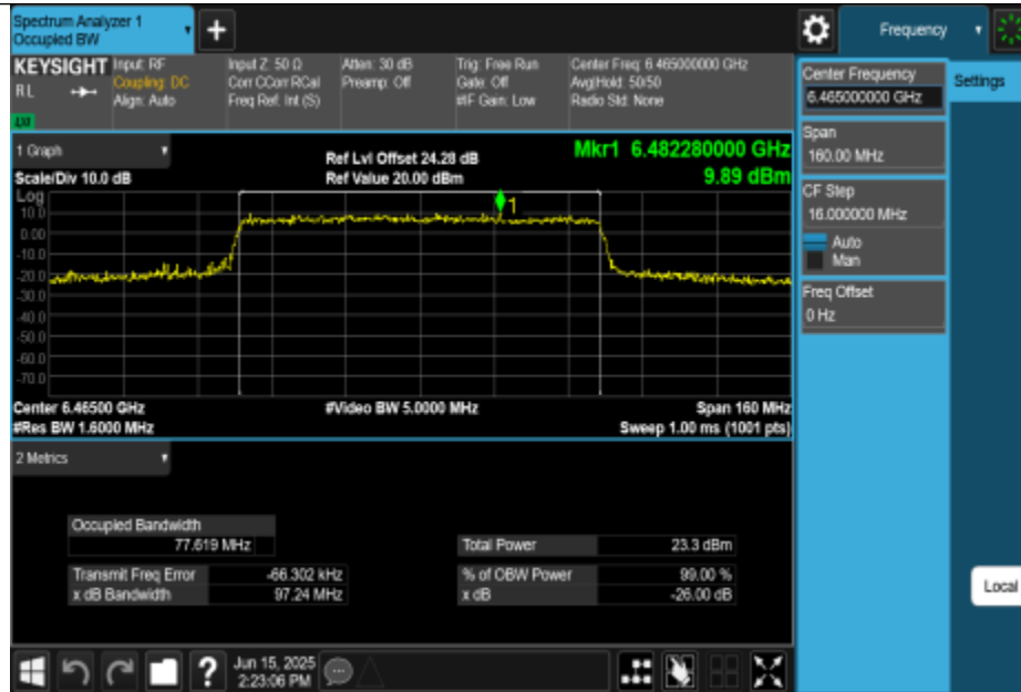
11BE80MIMO-Ant2-6465-PASS
