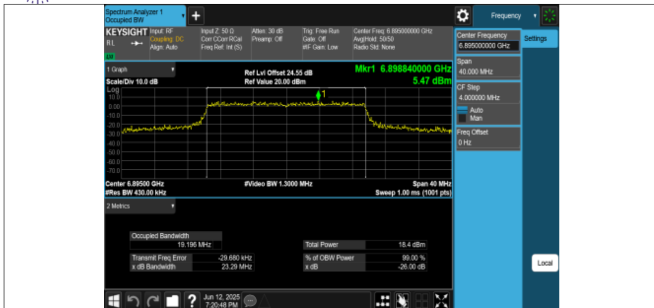
11BE20MIMO-Ant2-6895-PASS
