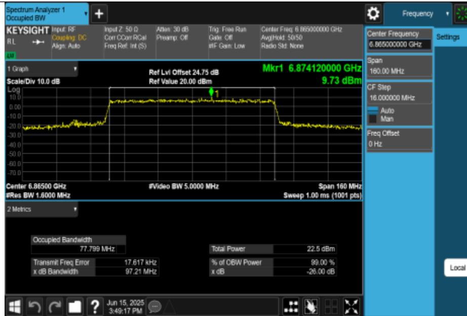
11BE80MIMO-Ant2-6865-PASS
