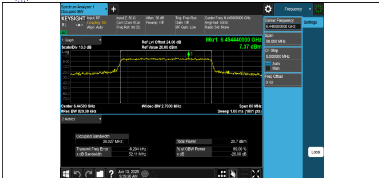
11BE40MIMO-Ant0-6445-PASS
