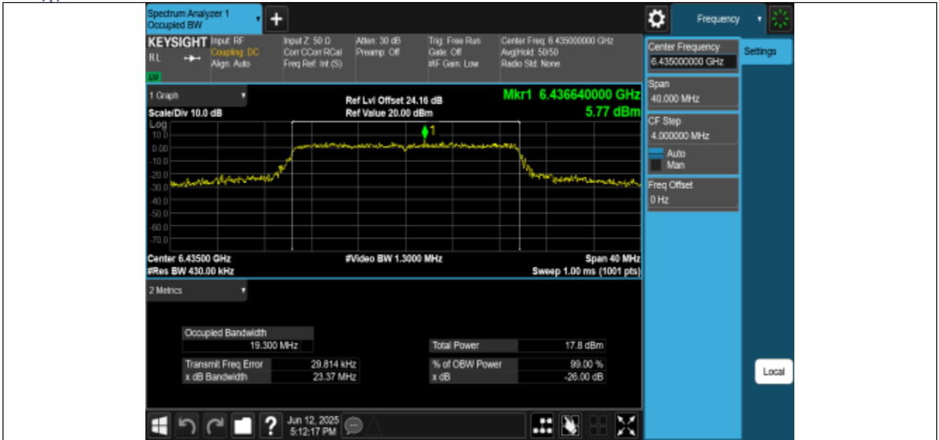
11BE20MIMO-Ant0-6435-PASS
