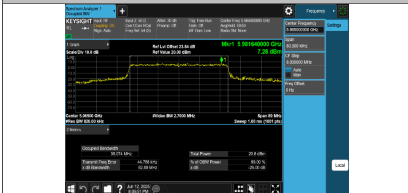
11BE40MIMO-Ant3-5965-PASS
