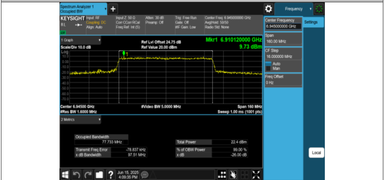
11BE80MIMO-Ant1-6945-PASS
