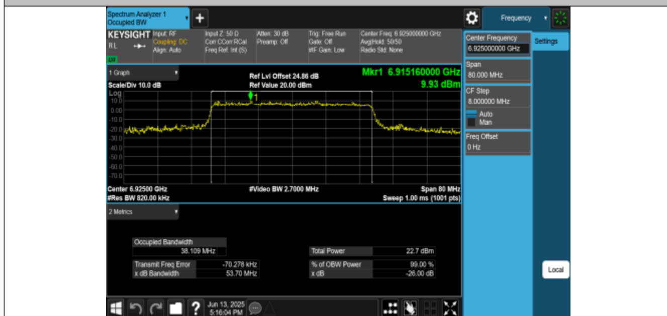
11BE40MIMO-Ant3-6925-PASS
