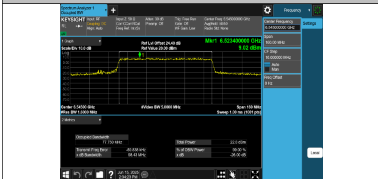
11BE80MIMO-Ant1-6545-PASS
