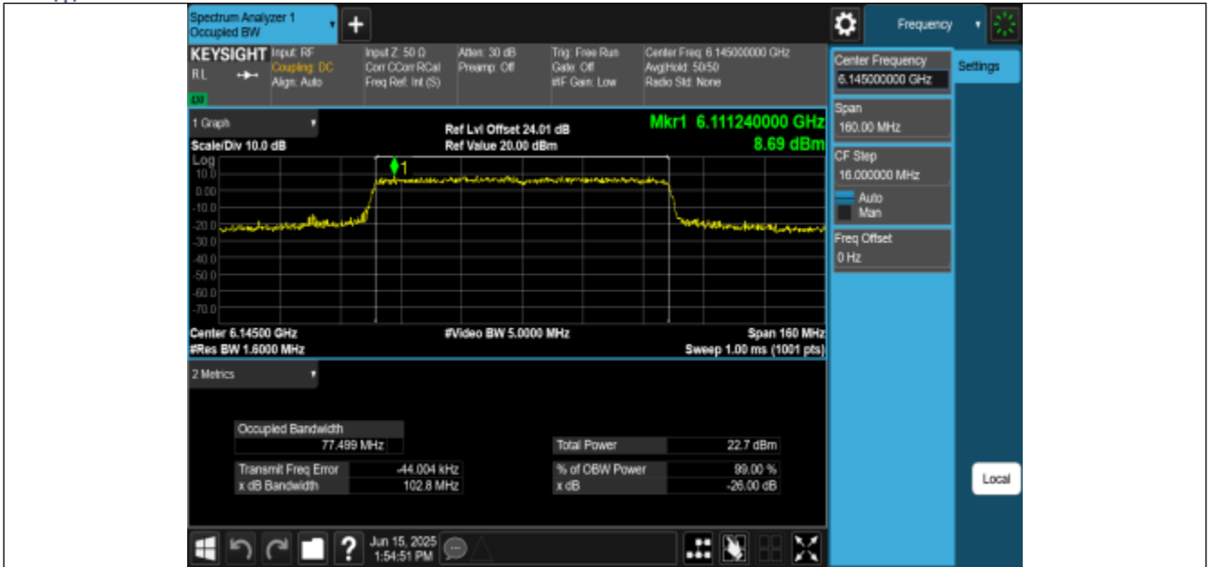
11BE80MIMO-Ant2-6145-PASS
