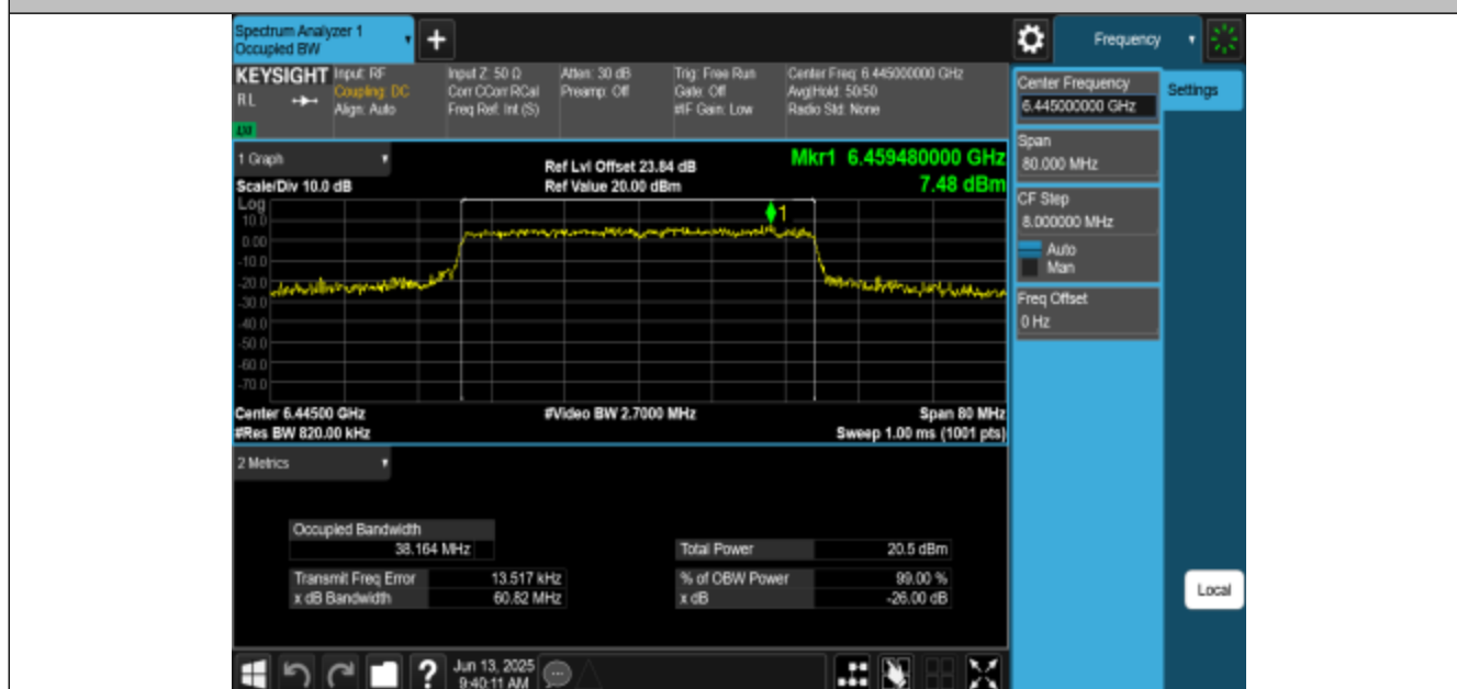
11BE40MIMO-Ant1-6445-PASS
