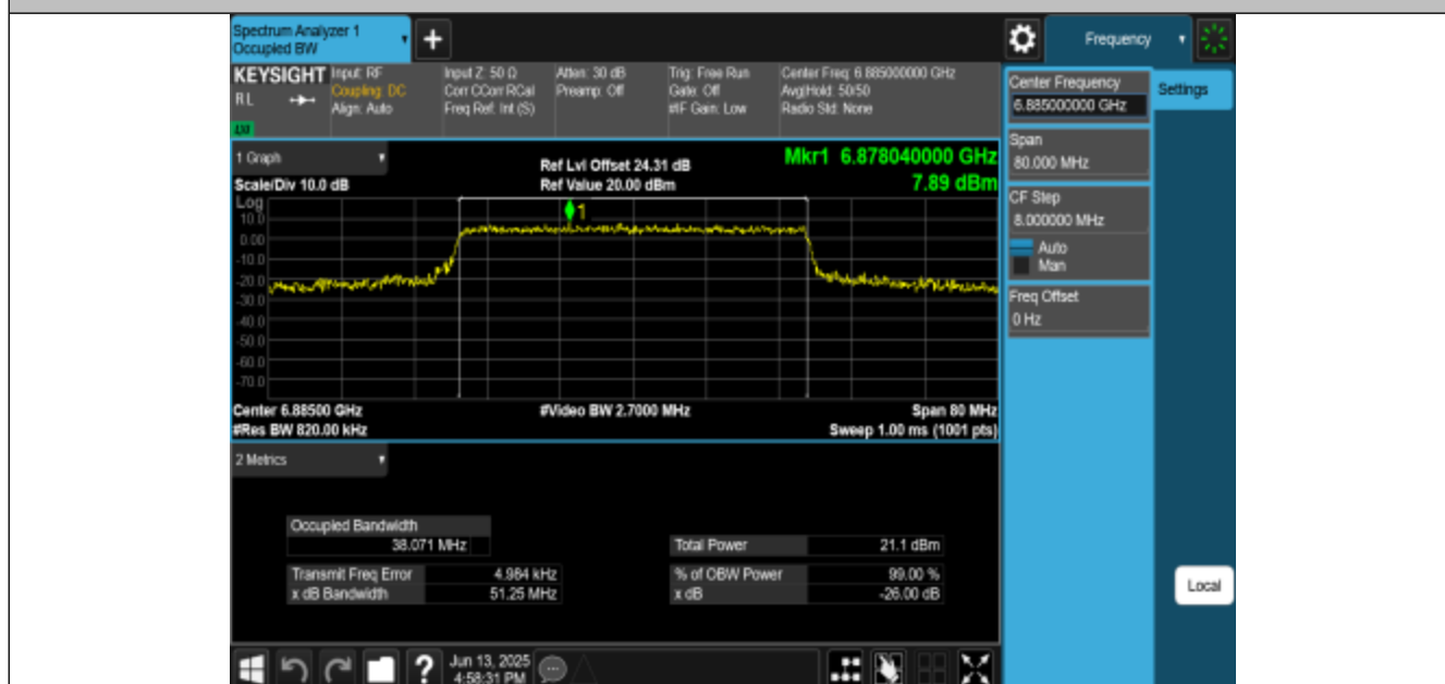
11BE40MIMO-Ant1-6885-PASS
