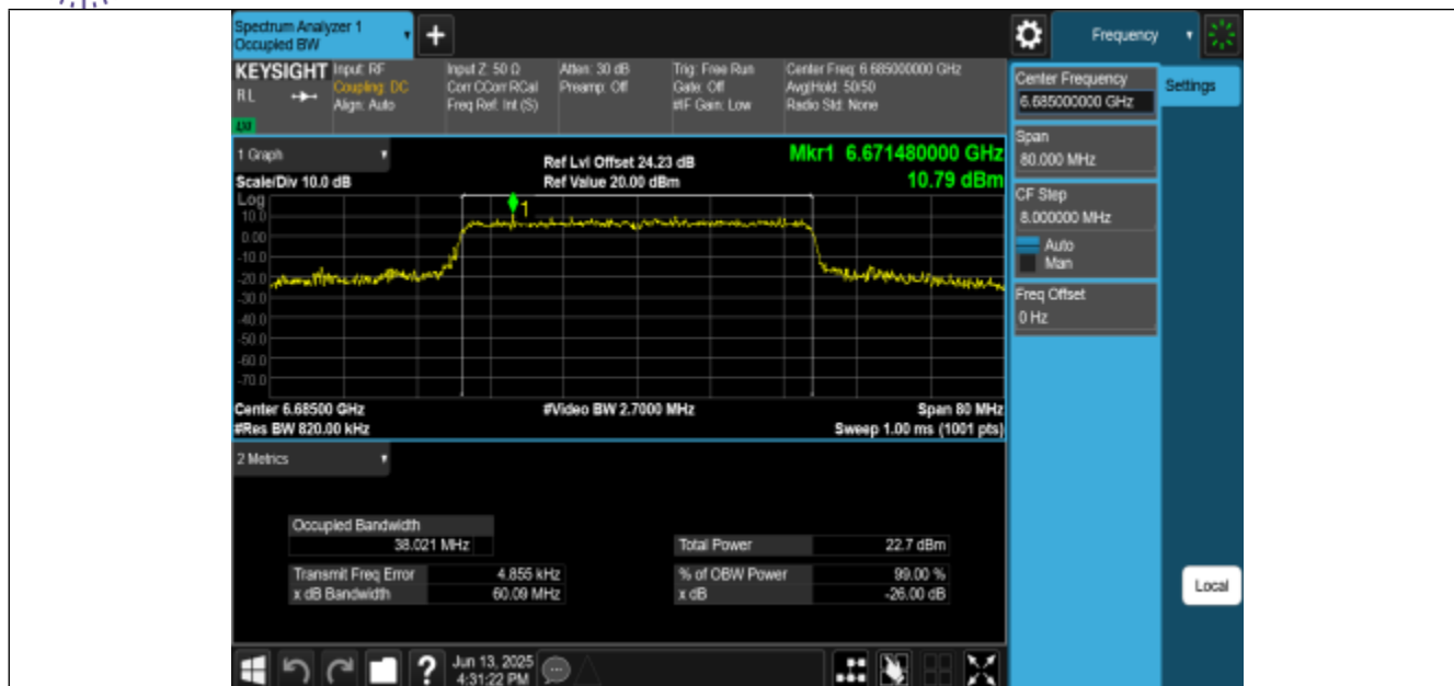
11BE40MIMO-Ant2-6685-PASS
