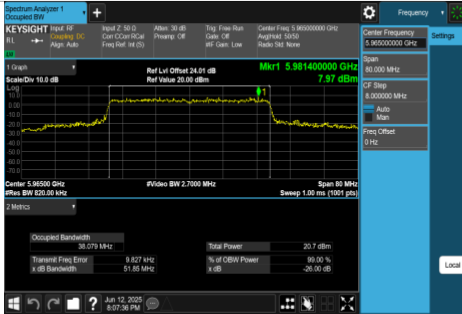
11BE40MIMO-Ant0-5965-PASS
