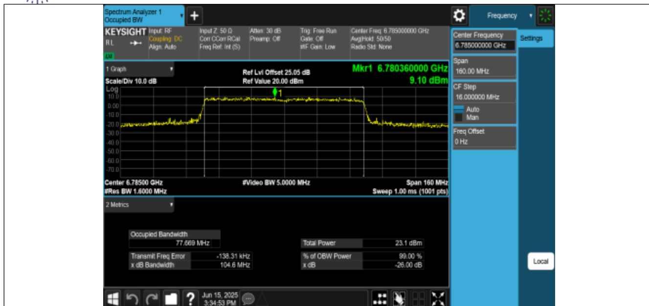
11BE80MIMO-Ant2-6785-PASS
