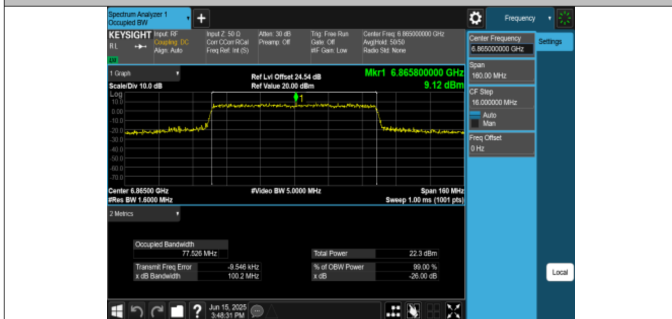
11BE80MIMO-Ant1-6865-PASS
