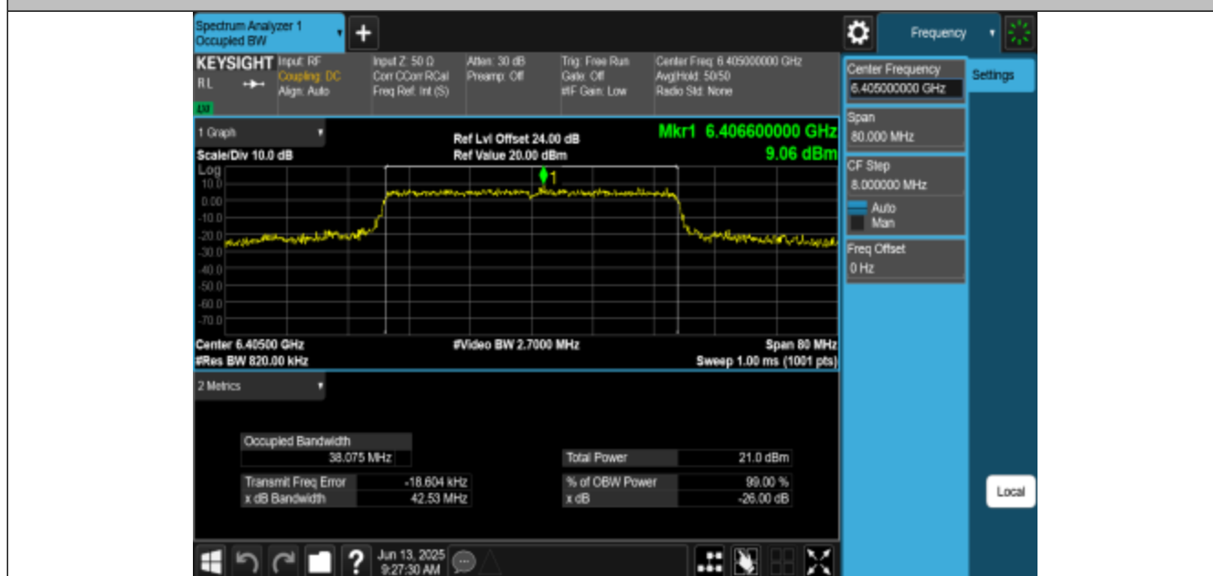
11BE40MIMO-Ant1-6405-PASS
