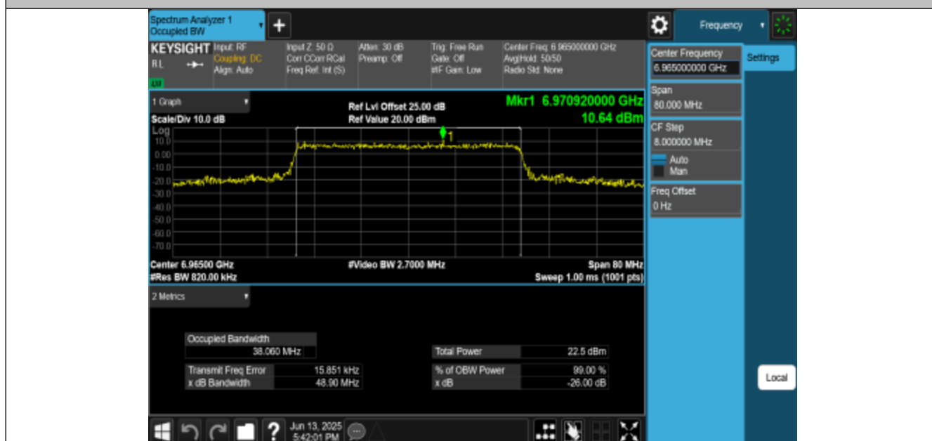
11BE40MIMO-Ant3-6965-PASS
