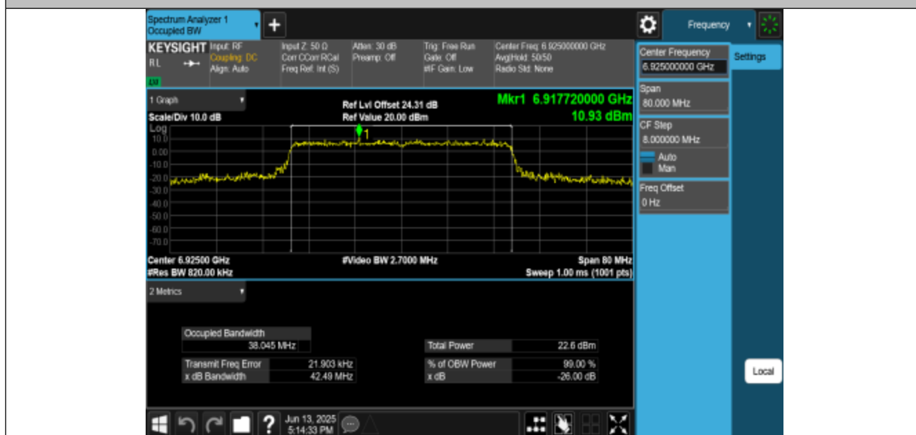
11BE40MIMO-Ant1-6925-PASS
