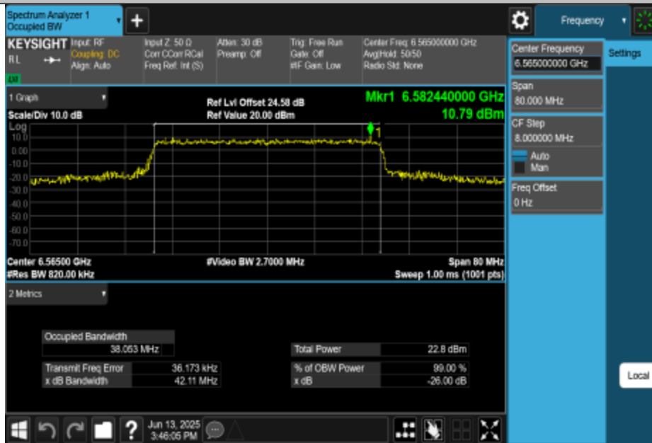
11BE40MIMO-Ant2-6565-PASS
