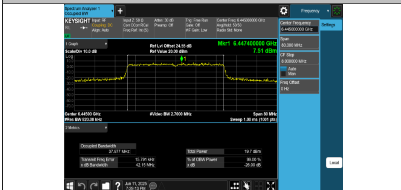
11AX40MIMO-Ant3-6445-PASS
