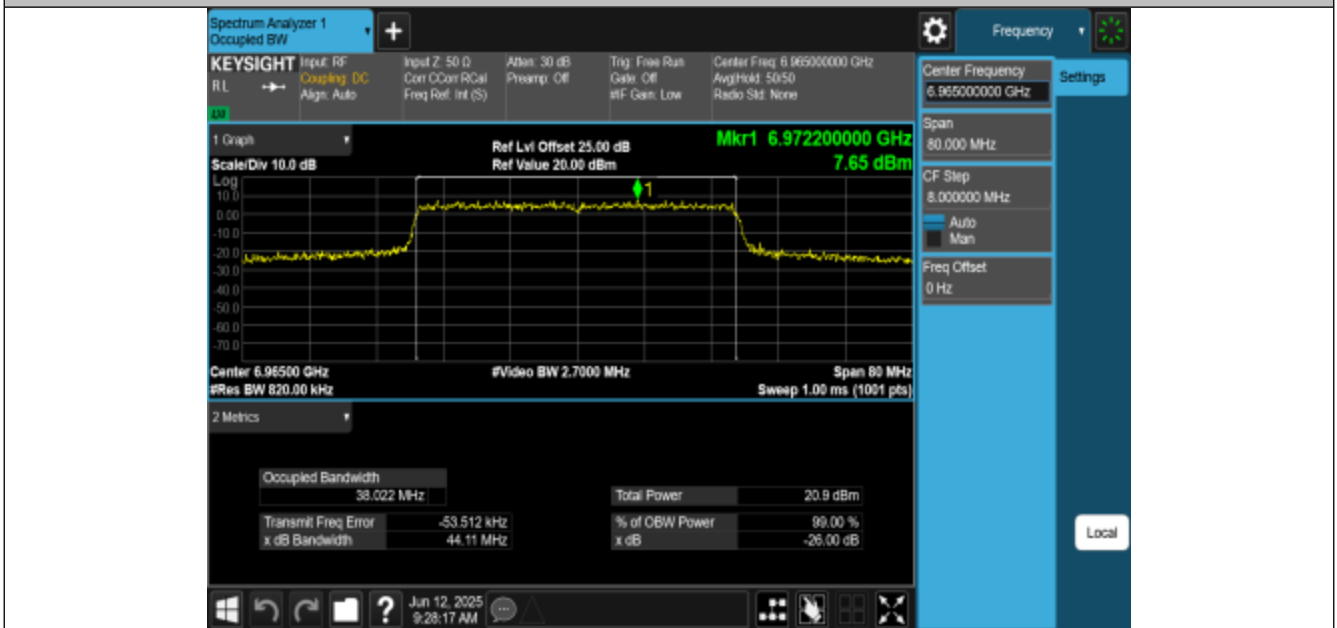
11AX40MIMO-Ant3-6965-PASS
