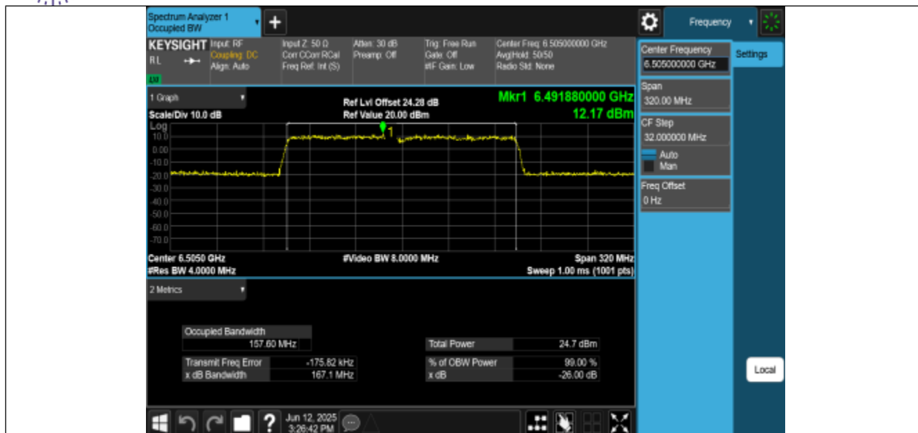
11AX160MIMO-Ant0-6505-PASS
