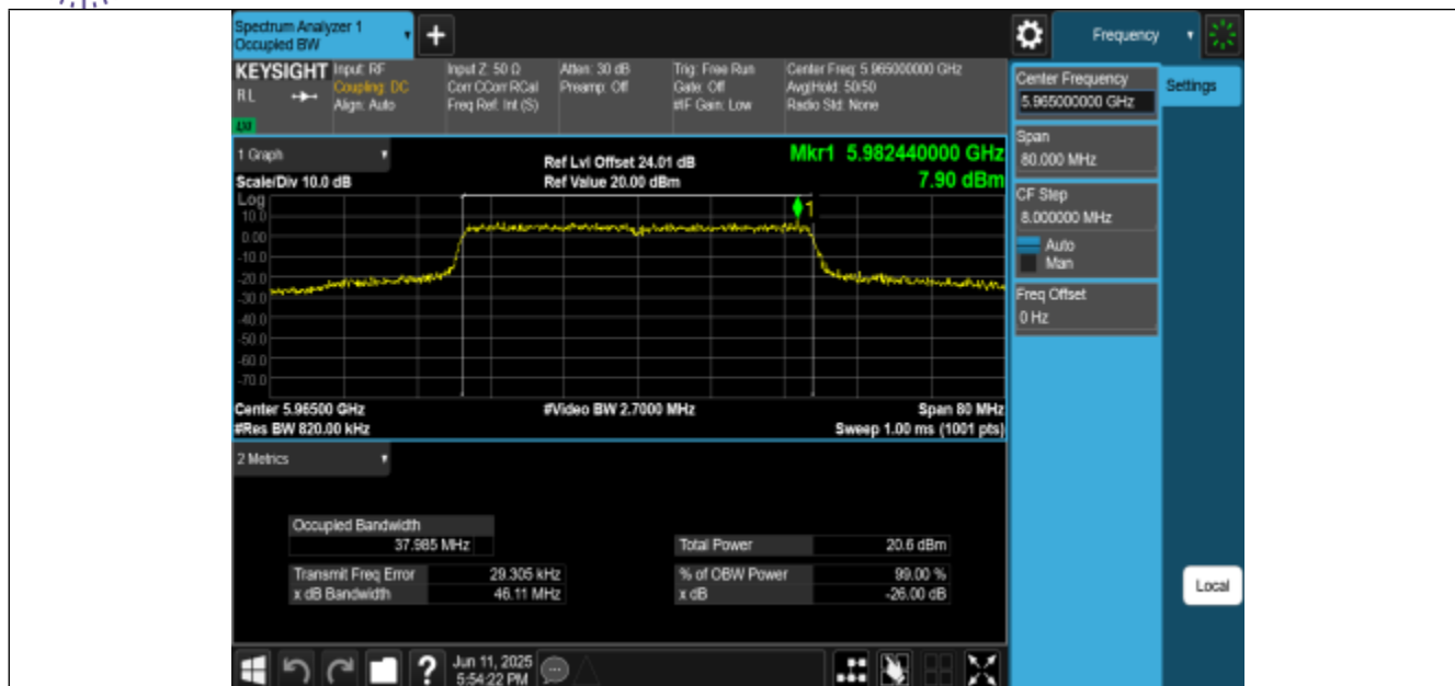
11AX40MIMO-Ant0-5965-PASS
