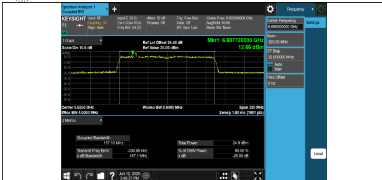
11AX160MIMO-Ant2-6665-PASS
