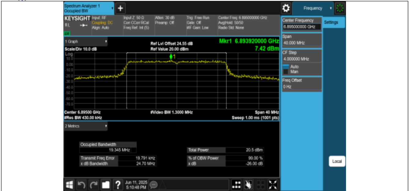
11AX20MIMO-Ant2-6895-PASS
