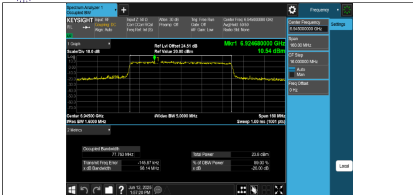
11AX80MIMO-Ant0-6945-PASS
