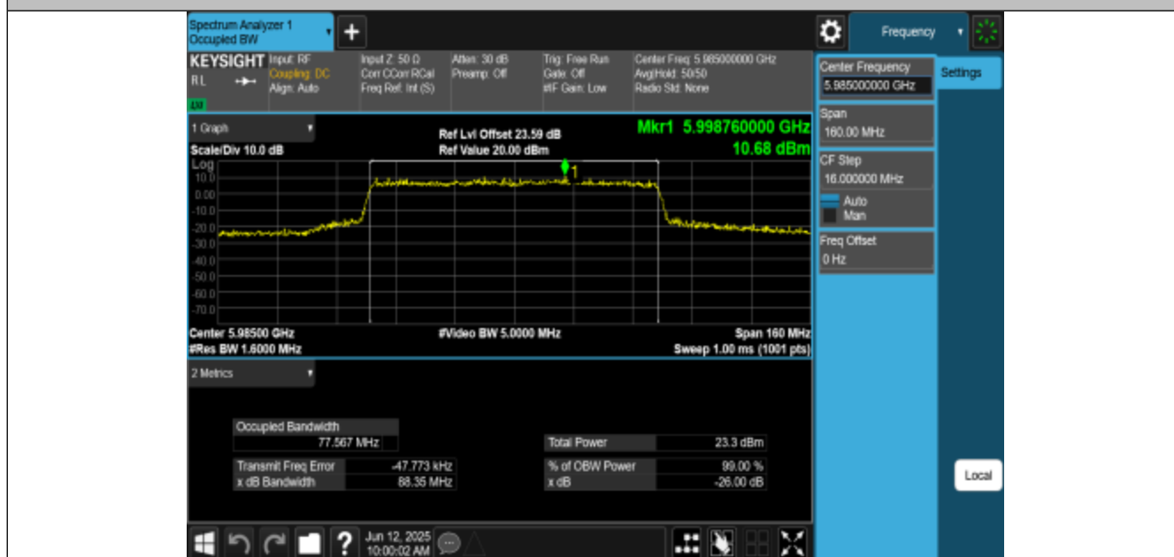
11AX80MIMO-Ant1-5985-PASS
