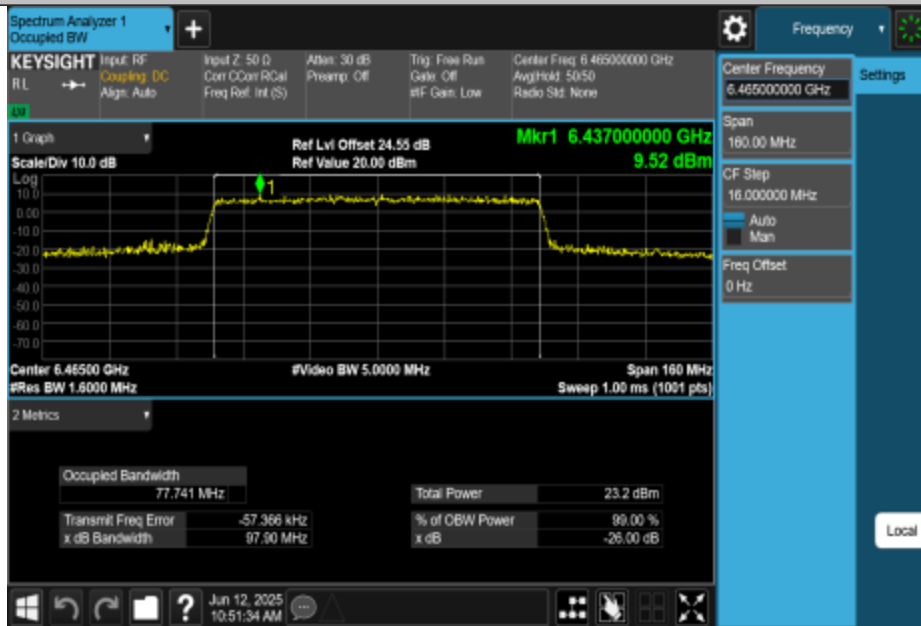
11AX80MIMO-Ant3-6465-PASS
