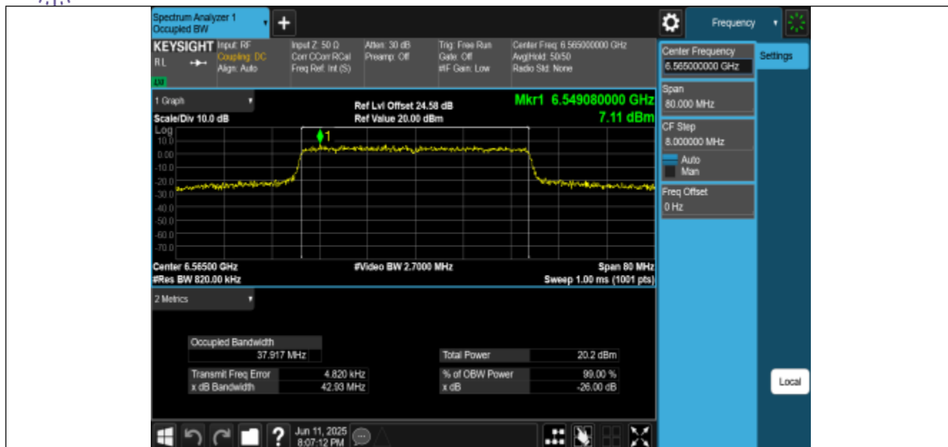
11AX40MIMO-Ant2-6565-PASS
