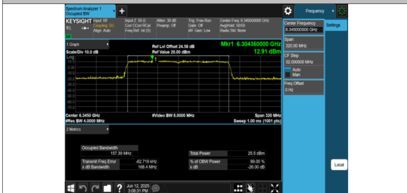
11AX160MIMO-Ant3-6345-PASS
