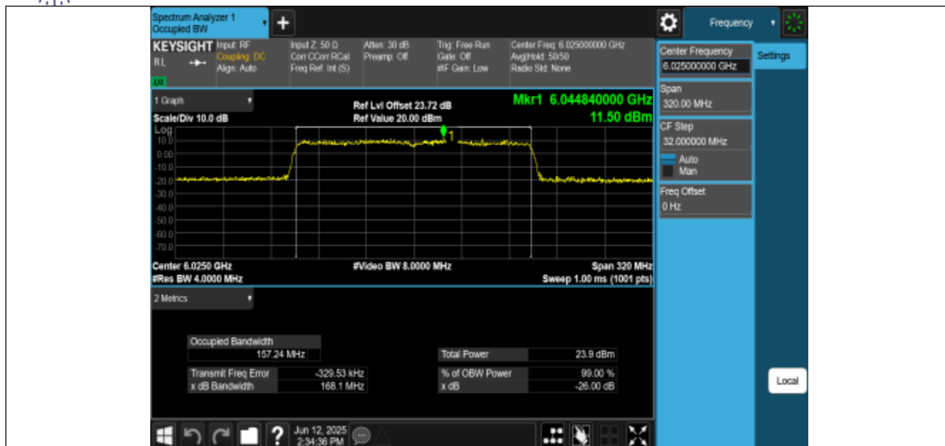
11AX160MIMO-Ant2-6025-PASS
