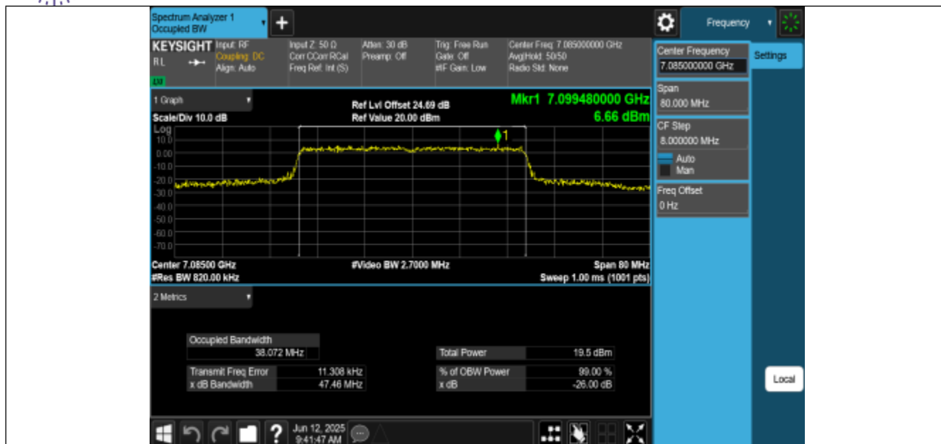
11AX40MIMO-Ant0-7085-PASS
