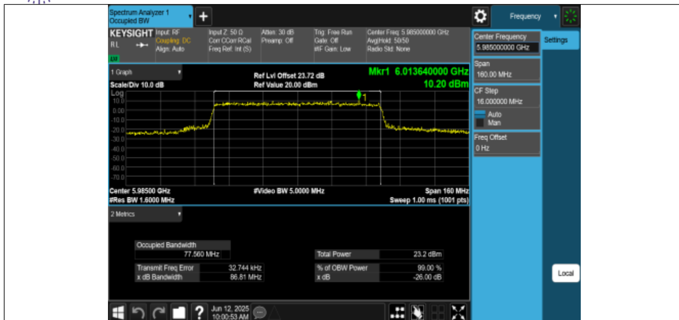
11AX80MIMO-Ant2-5985-PASS
