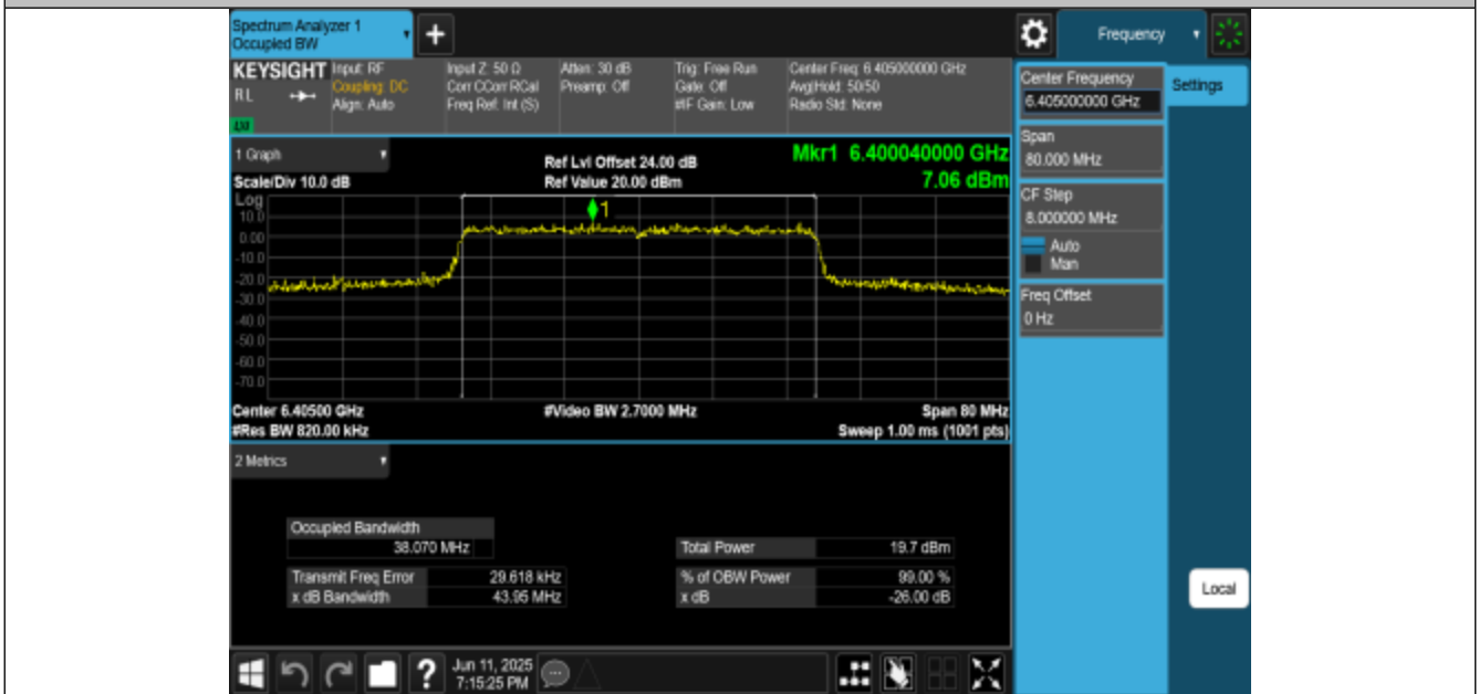
11AX40MIMO-Ant1-6405-PASS
