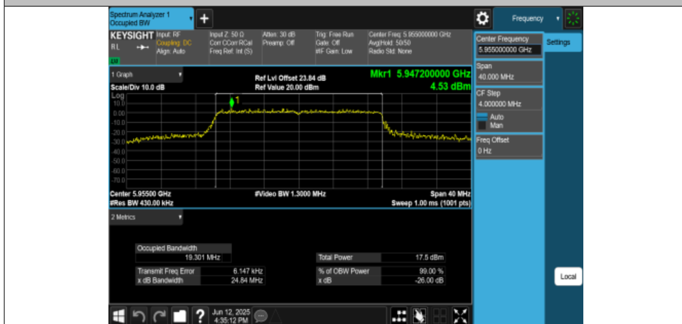
11BE20MIMO-Ant3-5955-PASS
