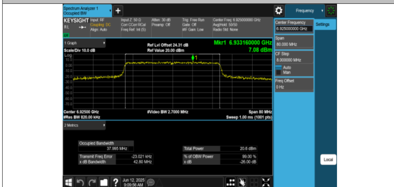
11AX40MIMO-Ant1-6925-PASS
