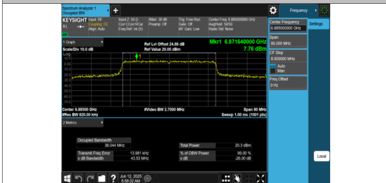
11AX40MIMO-Ant3-6885-PASS
