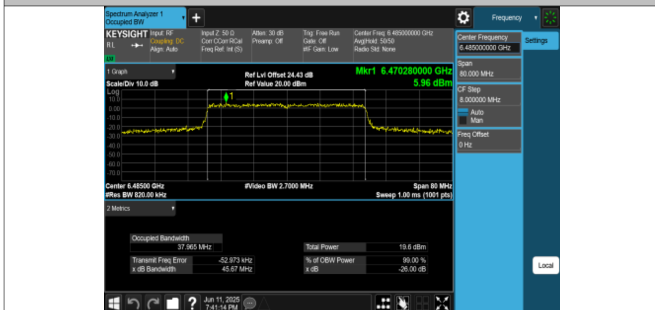
11AX40MIMO-Ant3-6485-PASS
