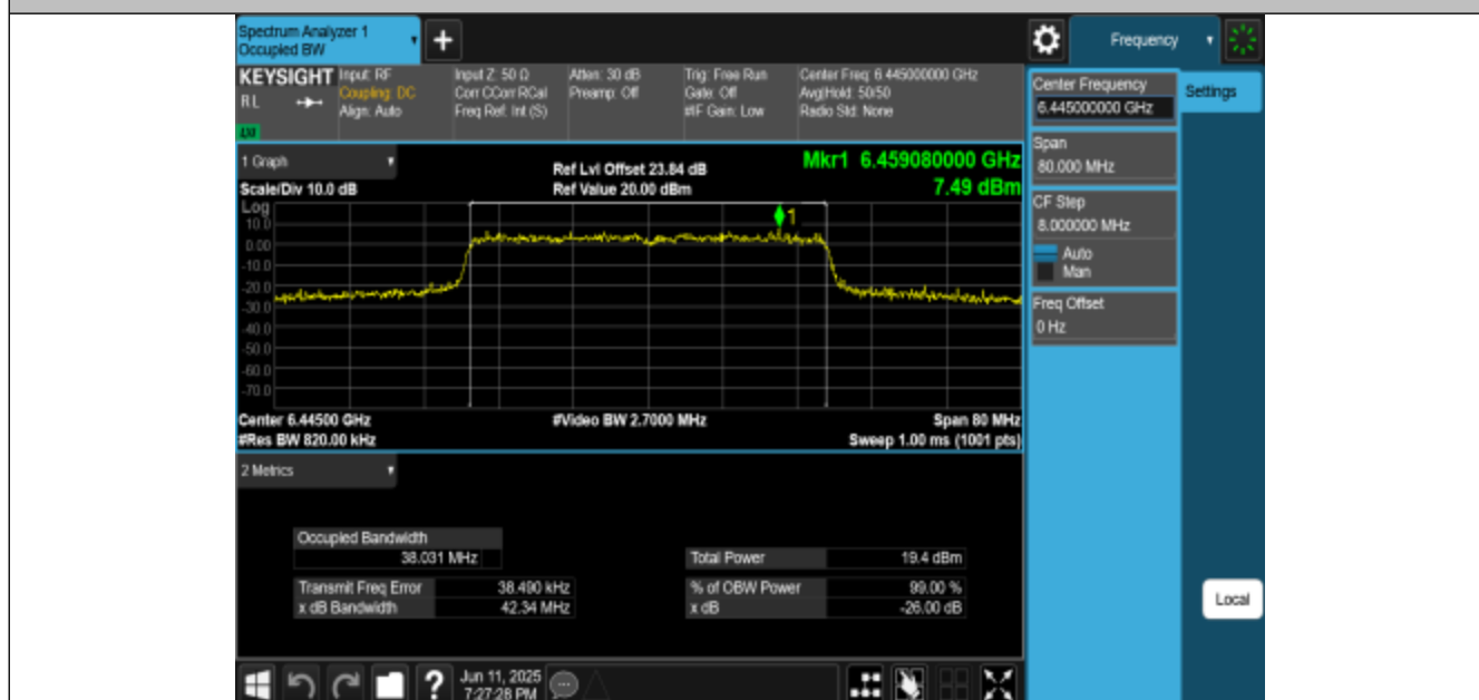
11AX40MIMO-Ant1-6445-PASS
