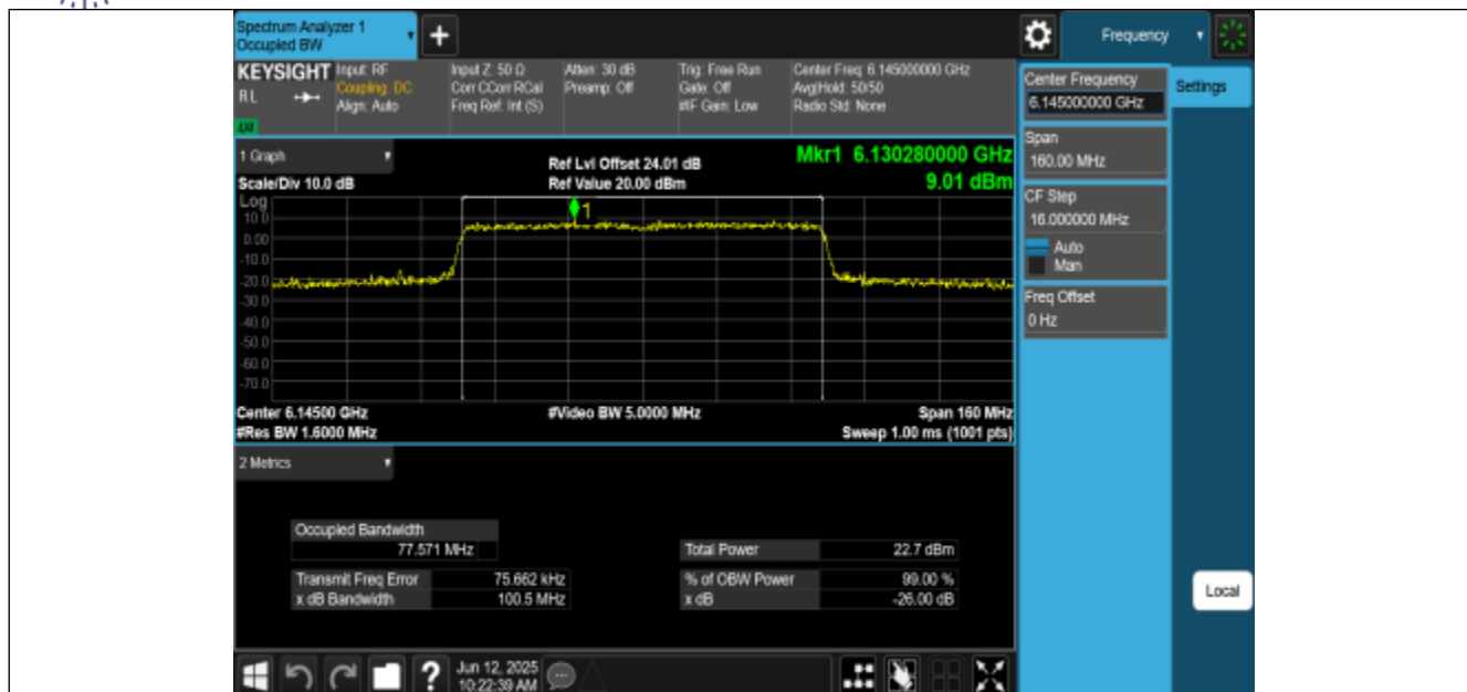
11AX80MIMO-Ant2-6145-PASS
