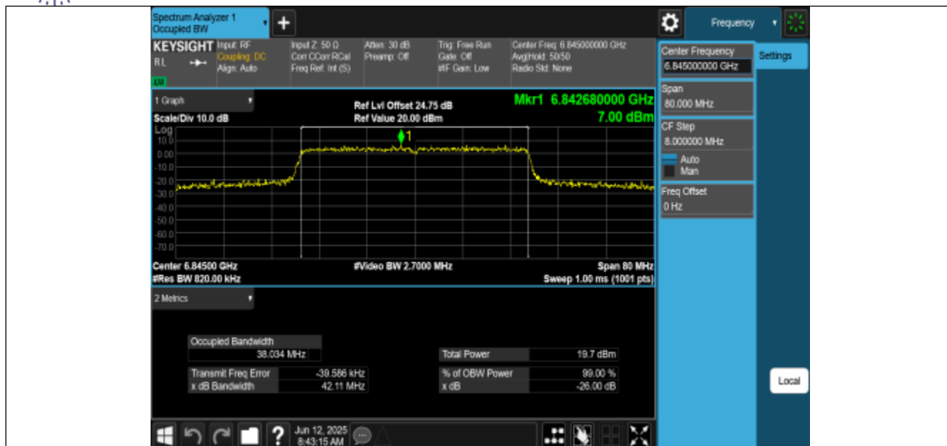
11AX40MIMO-Ant2-6845-PASS
