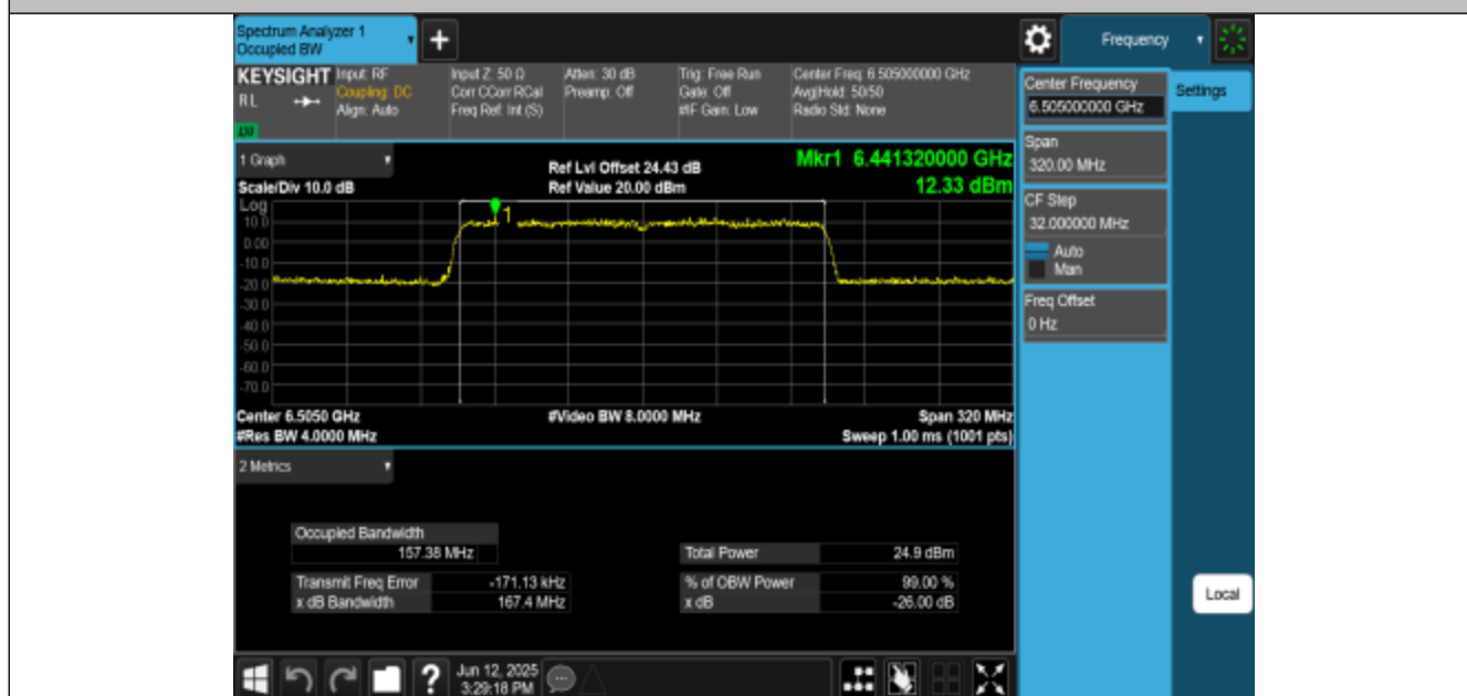
11AX160MIMO-Ant3-6505-PASS
