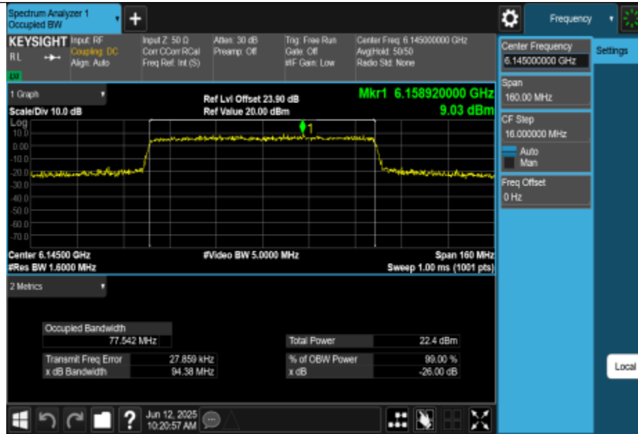
11AX80MIMO-Ant0-6145-PASS
