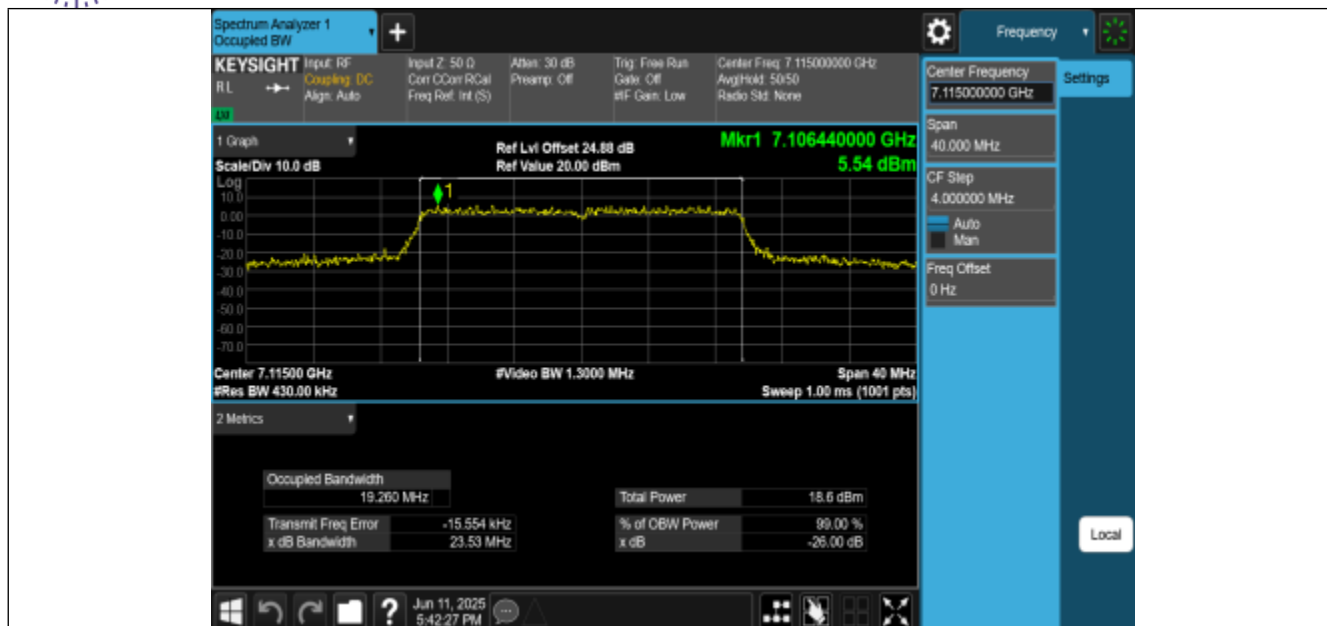
11AX20MIMO-Ant2-7115-PASS
