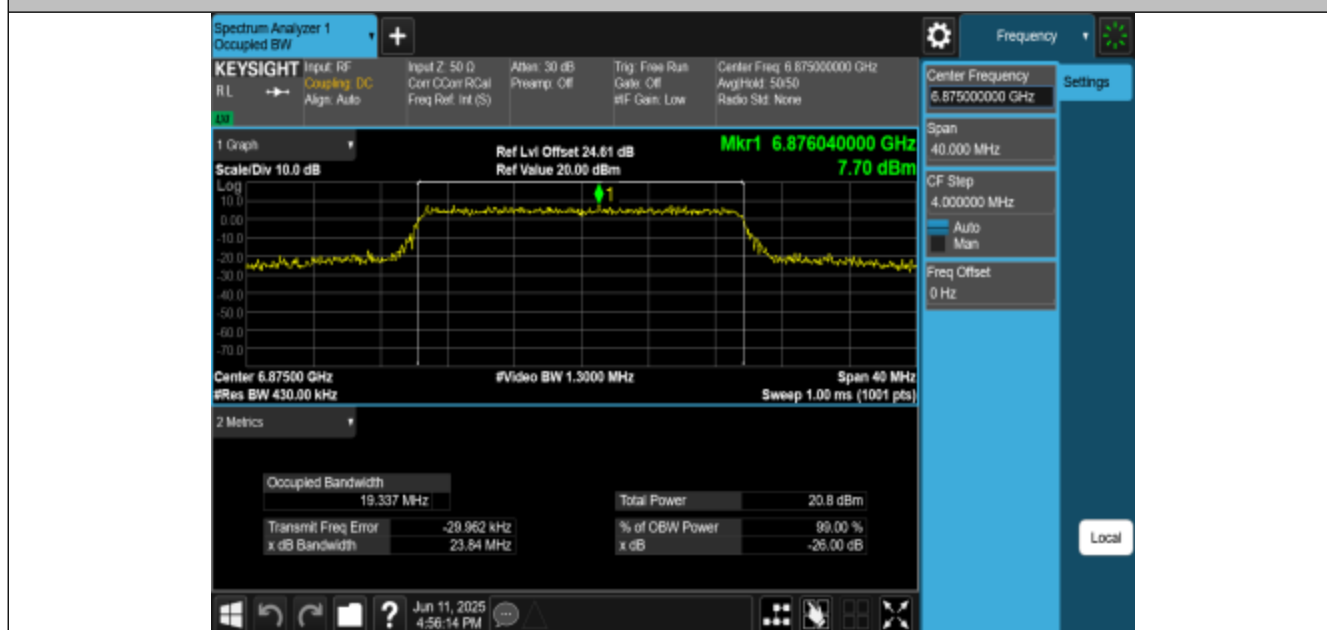
11AX20MIMO-Ant3-6875-PASS
