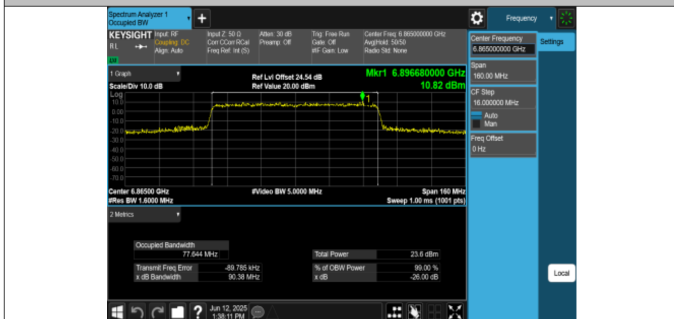
11AX80MIMO-Ant1-6865-PASS
