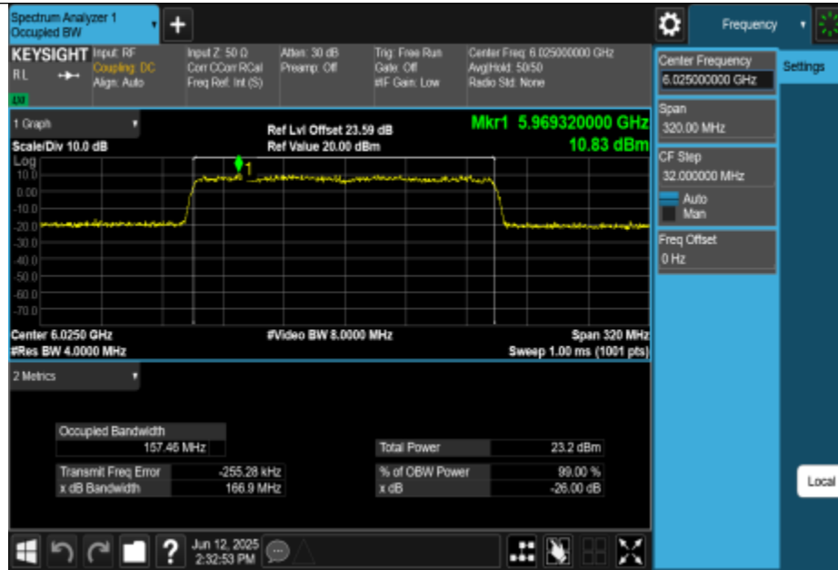
11AX160MIMO-Ant0-6025-PASS
