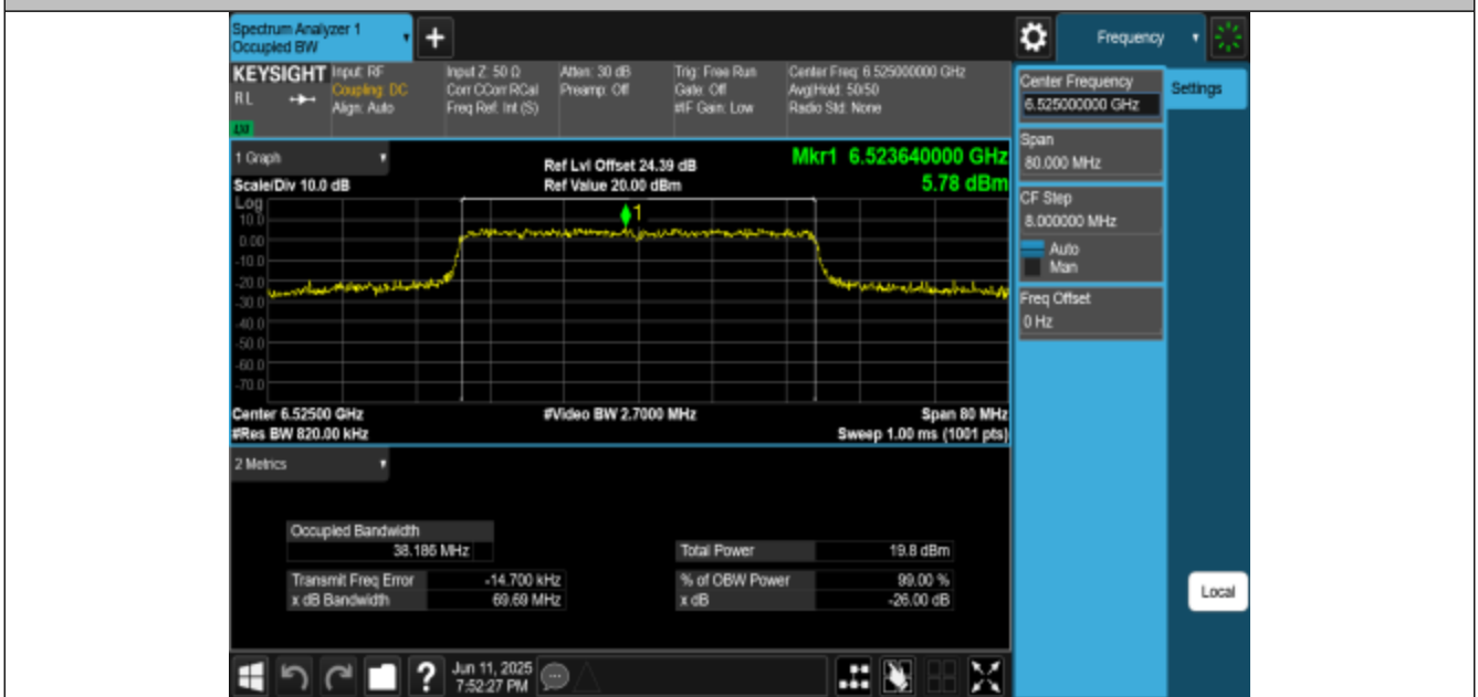
11AX40MIMO-Ant1-6525-PASS
