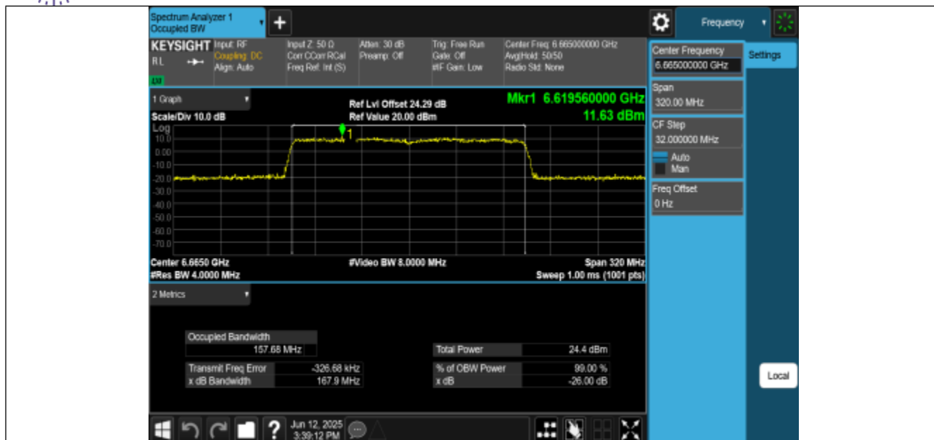
11AX160MIMO-Ant0-6665-PASS
