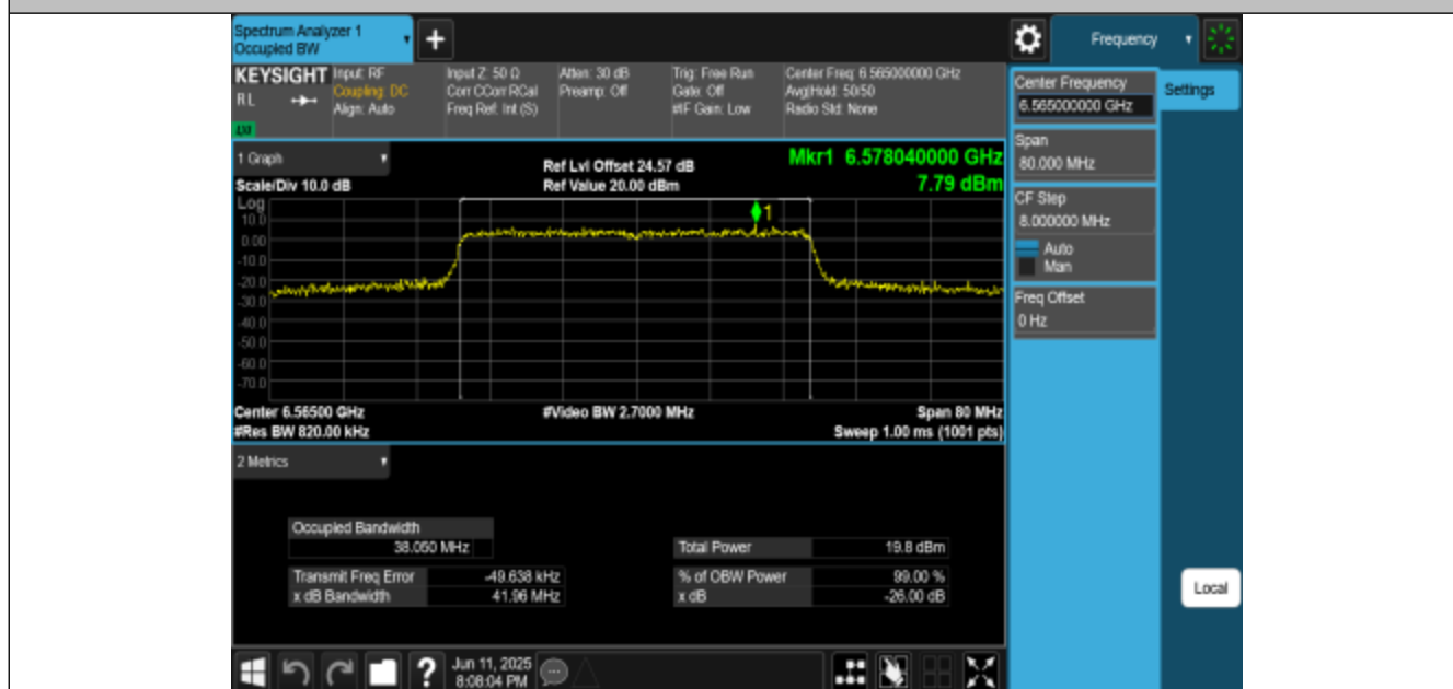
11AX40MIMO-Ant3-6565-PASS
