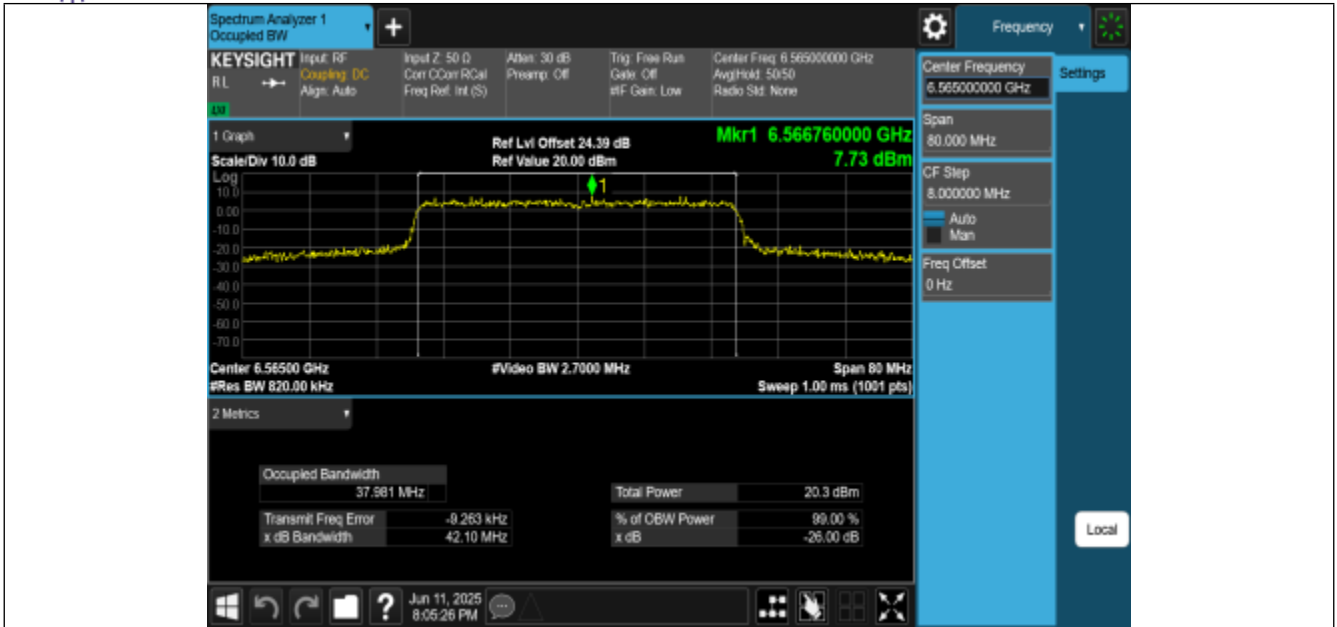
11AX40MIMO-Ant0-6565-PASS
