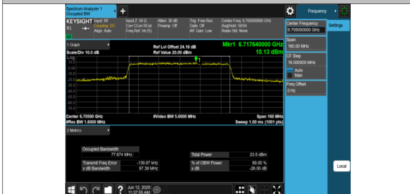
11AX80MIMO-Ant1-6705-PASS
