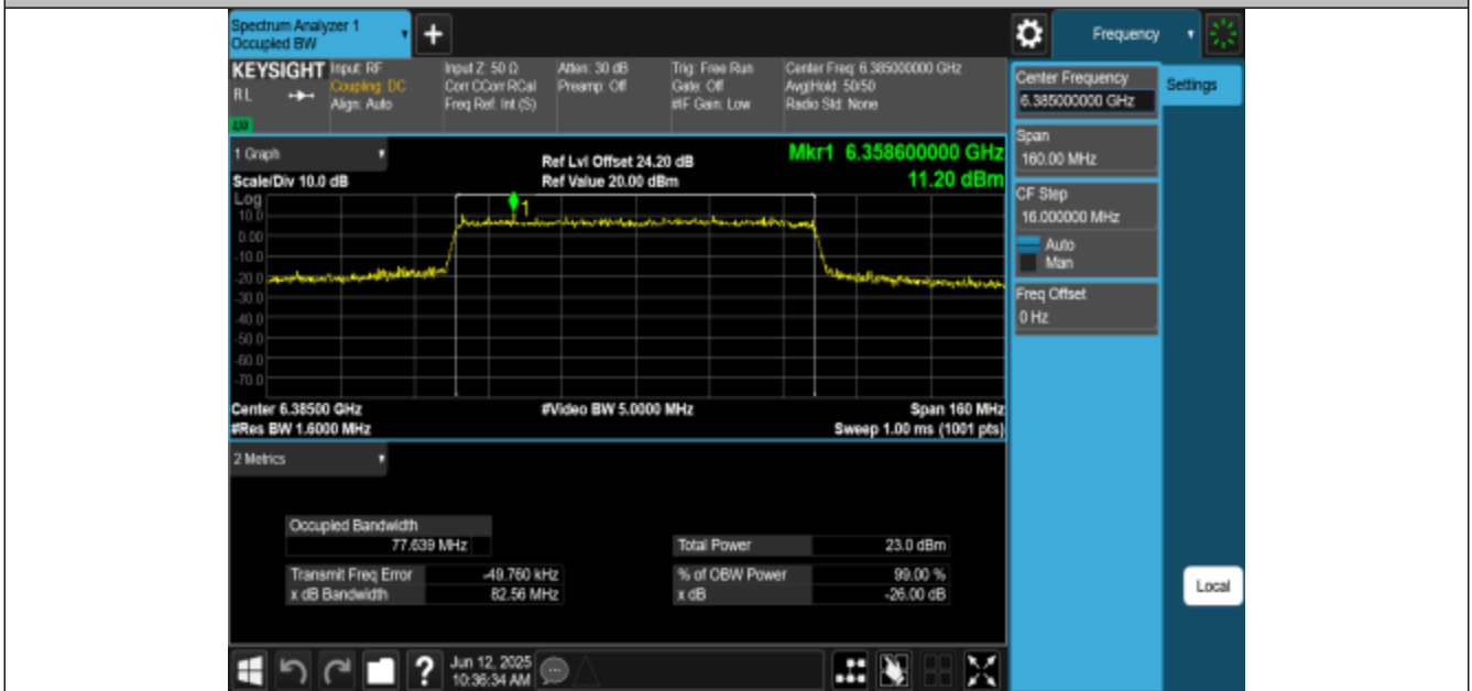
11AX80MIMO-Ant3-6385-PASS
