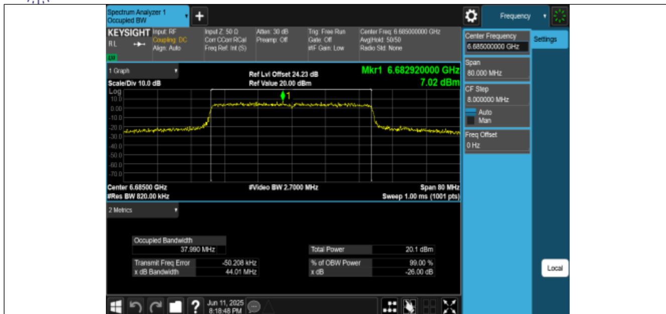
11AX40MIMO-Ant2-6685-PASS
