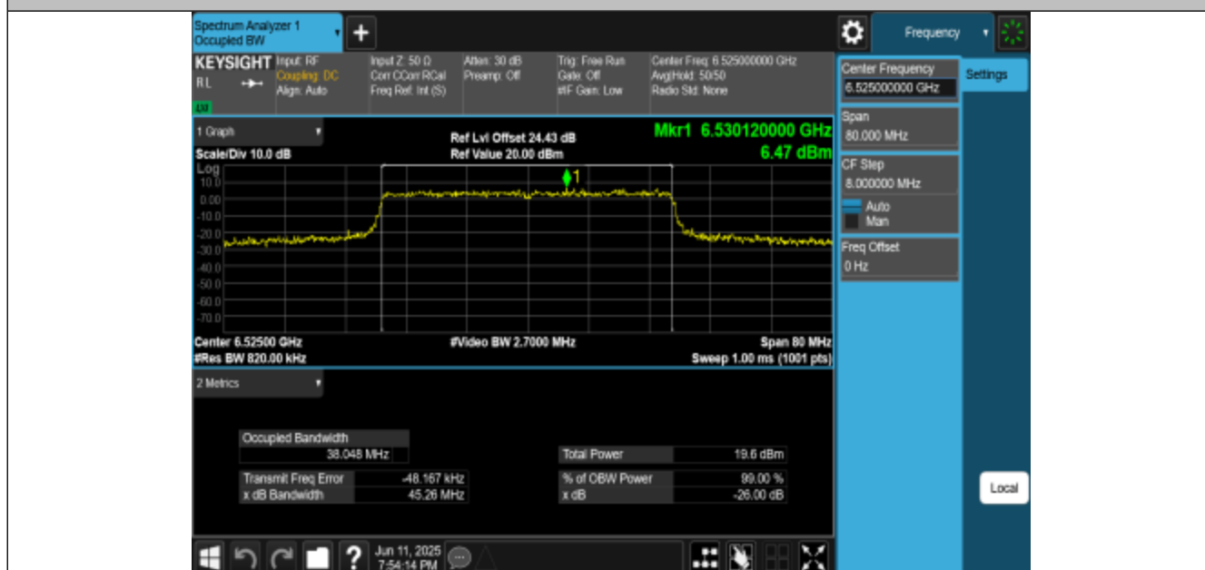
11AX40MIMO-Ant3-6525-PASS
