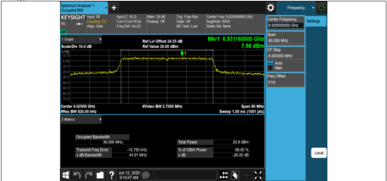
11AX40MIMO-Ant2-6925-PASS
