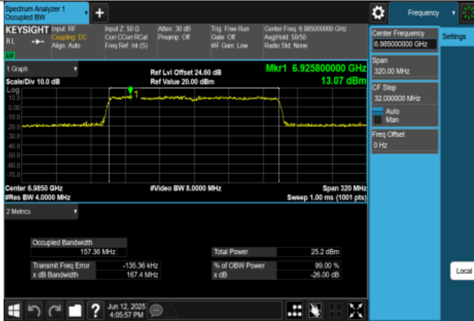
11AX160MIMO-Ant2-6985-PASS
