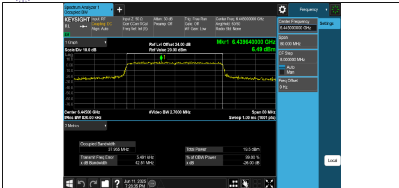
11AX40MIMO-Ant0-6445-PASS
