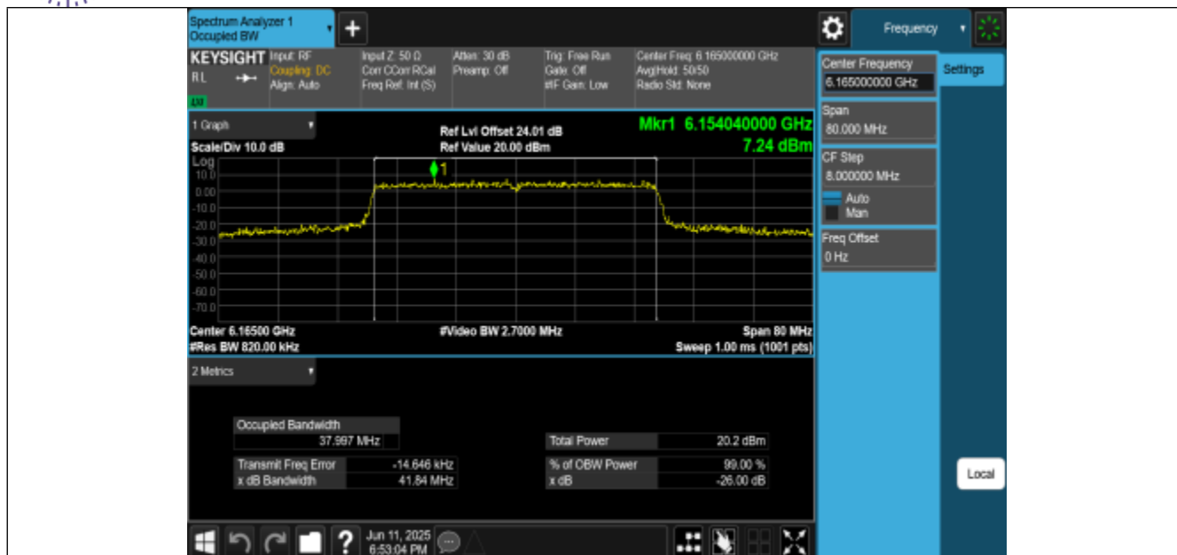
11AX40MIMO-Ant2-6165-PASS
