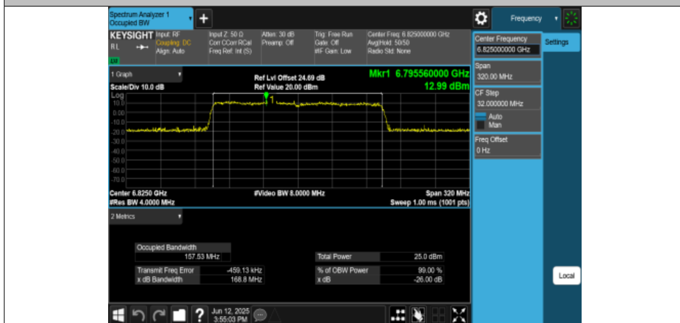
11AX160MIMO-Ant3-6825-PASS
