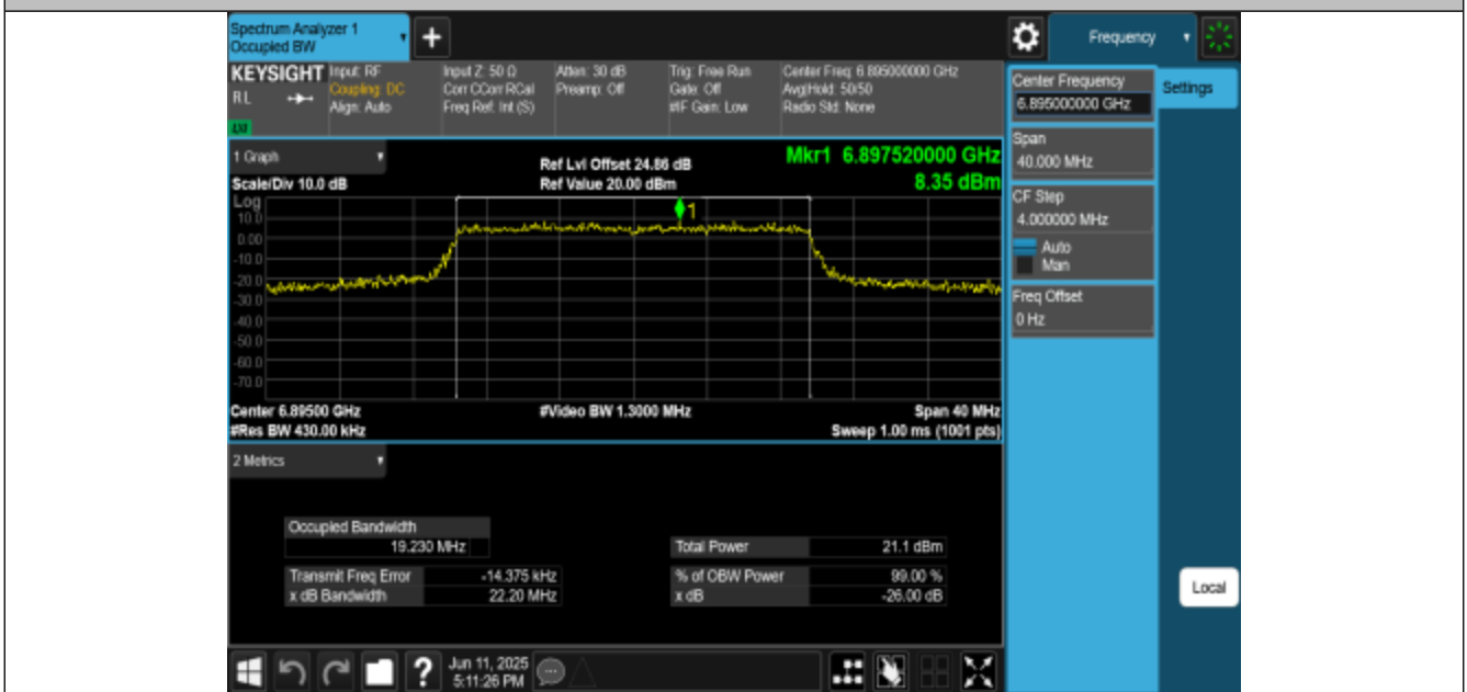
11AX20MIMO-Ant3-6895-PASS
