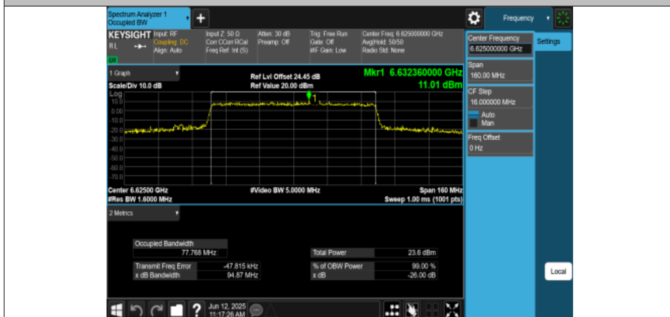
11AX80MIMO-Ant1-6625-PASS
