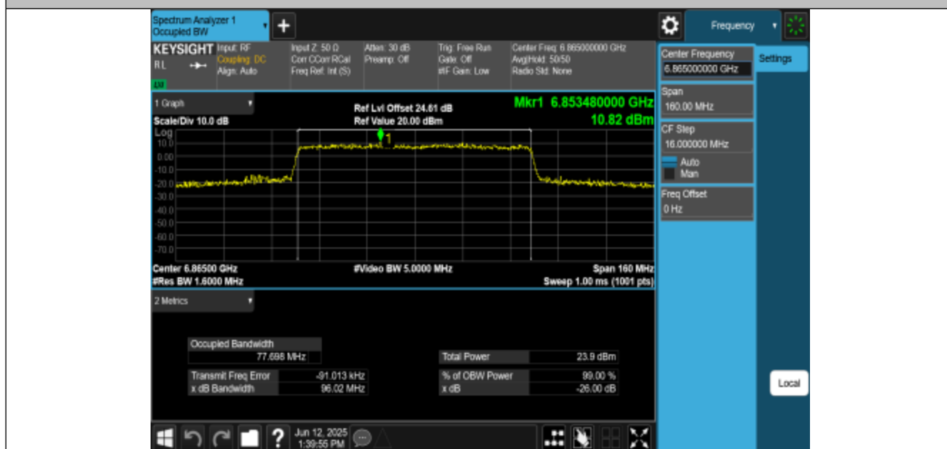
11AX80MIMO-Ant3-6865-PASS
