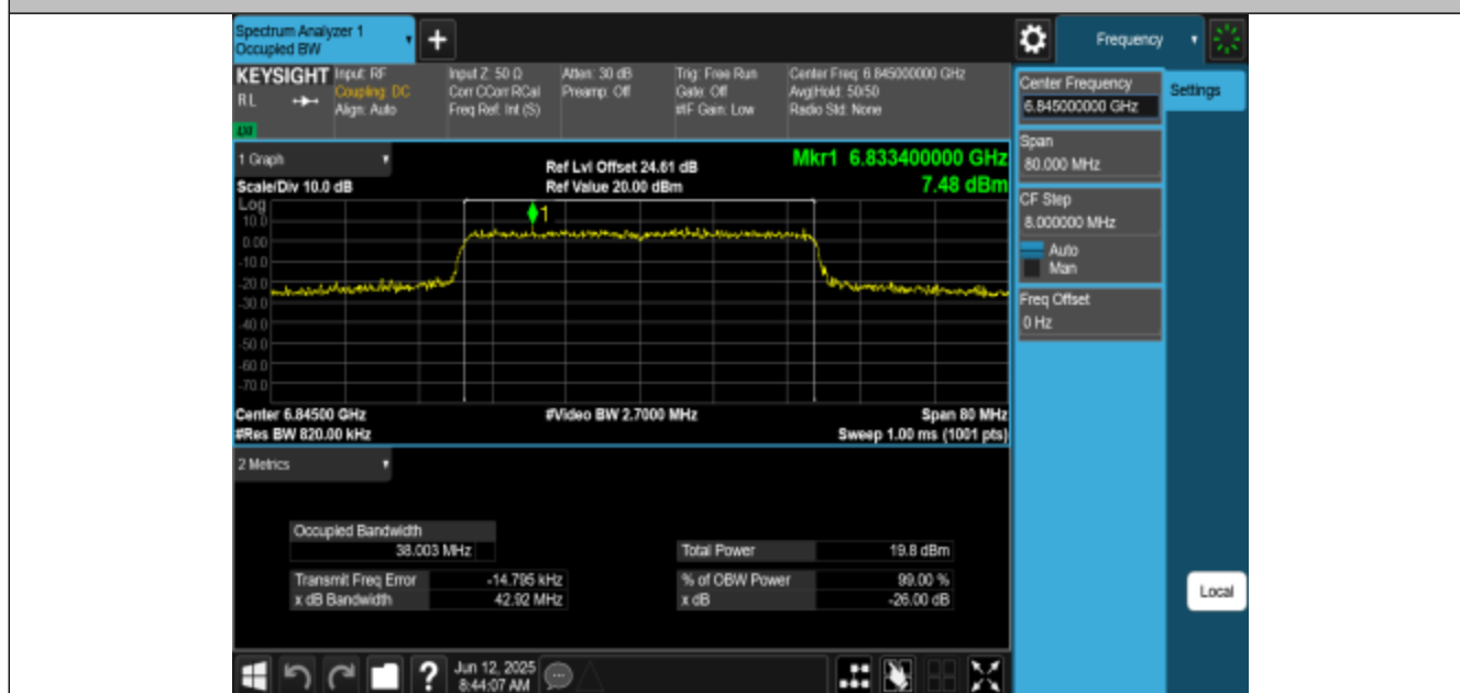
11AX40MIMO-Ant3-6845-PASS
