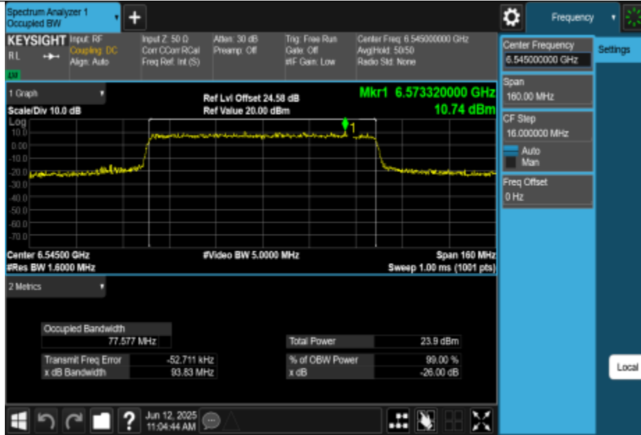
11AX80MIMO-Ant2-6545-PASS
