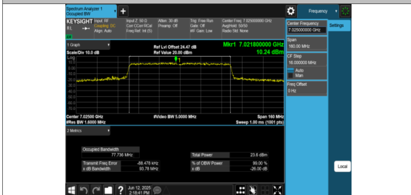
11AX80MIMO-Ant1-7025-PASS
