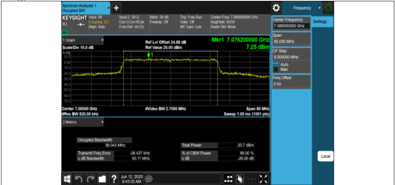
11AX40MIMO-Ant2-7085-PASS
