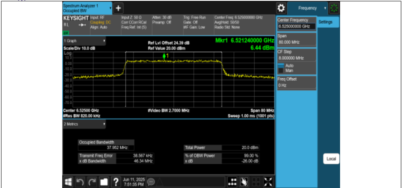
11AX40MIMO-Ant0-6525-PASS
