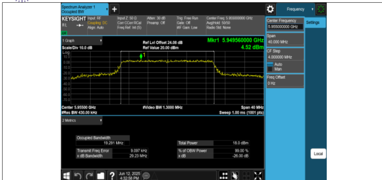
11BE20MIMO-Ant0-5955-PASS
