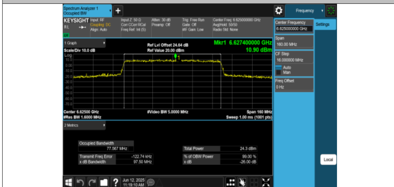
11AX80MIMO-Ant3-6625-PASS
