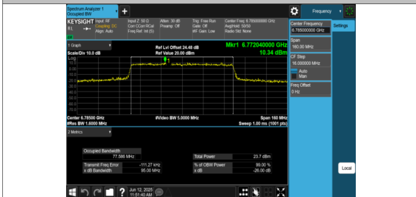
11AX80MIMO-Ant1-6785-PASS
