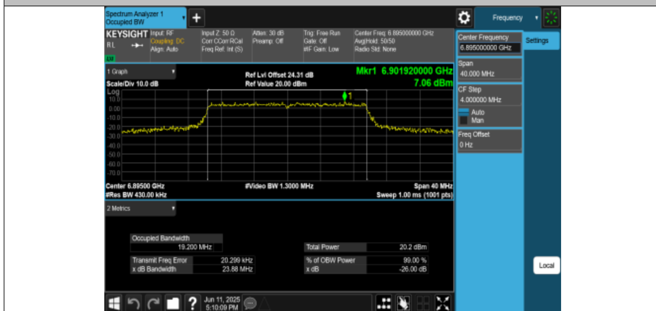
11AX20MIMO-Ant1-6895-PASS
