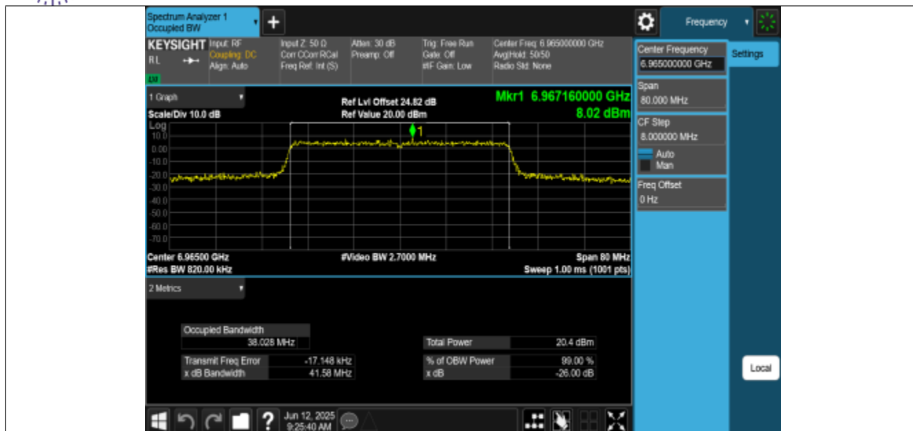
11AX40MIMO-Ant0-6965-PASS
