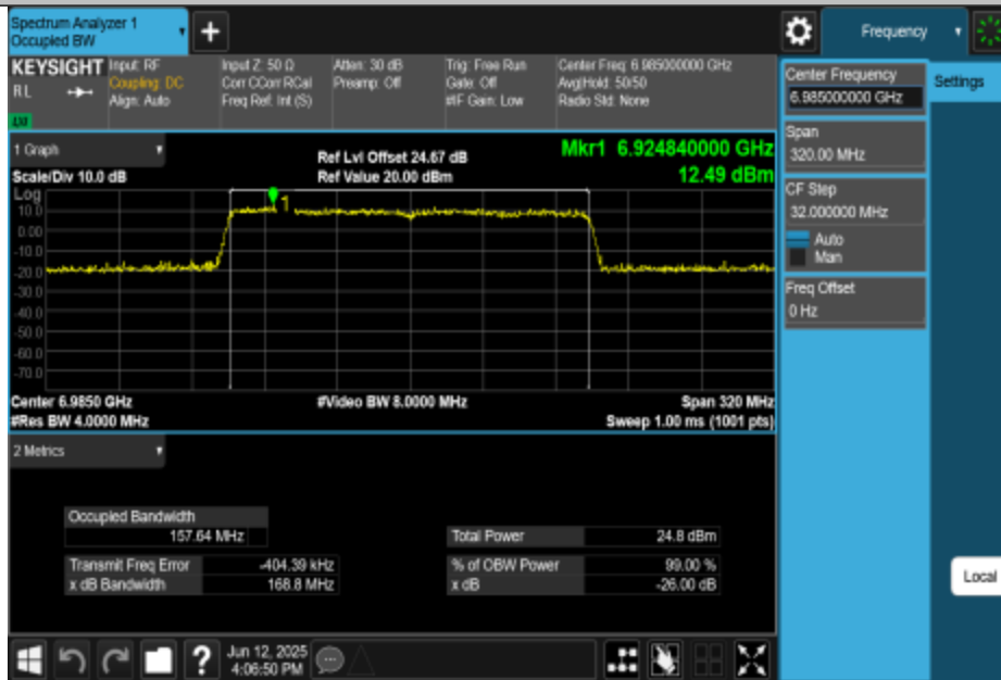
11AX160MIMO-Ant3-6985-PASS
