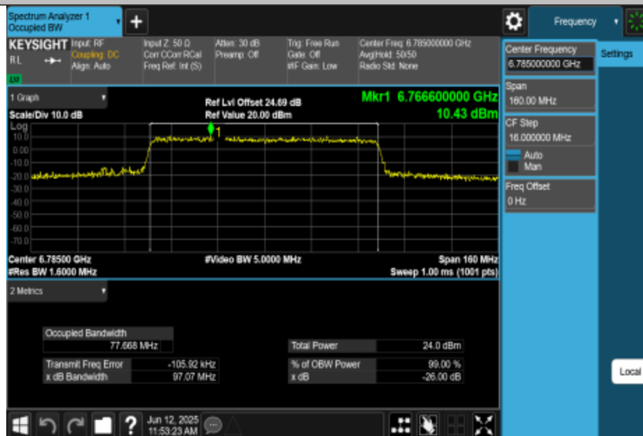
11AX80MIMO-Ant3-6785-PASS
