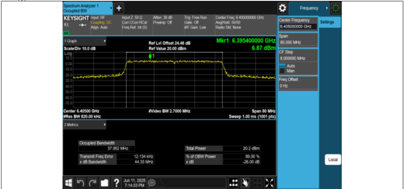
11AX40MIMO-Ant0-6405-PASS
