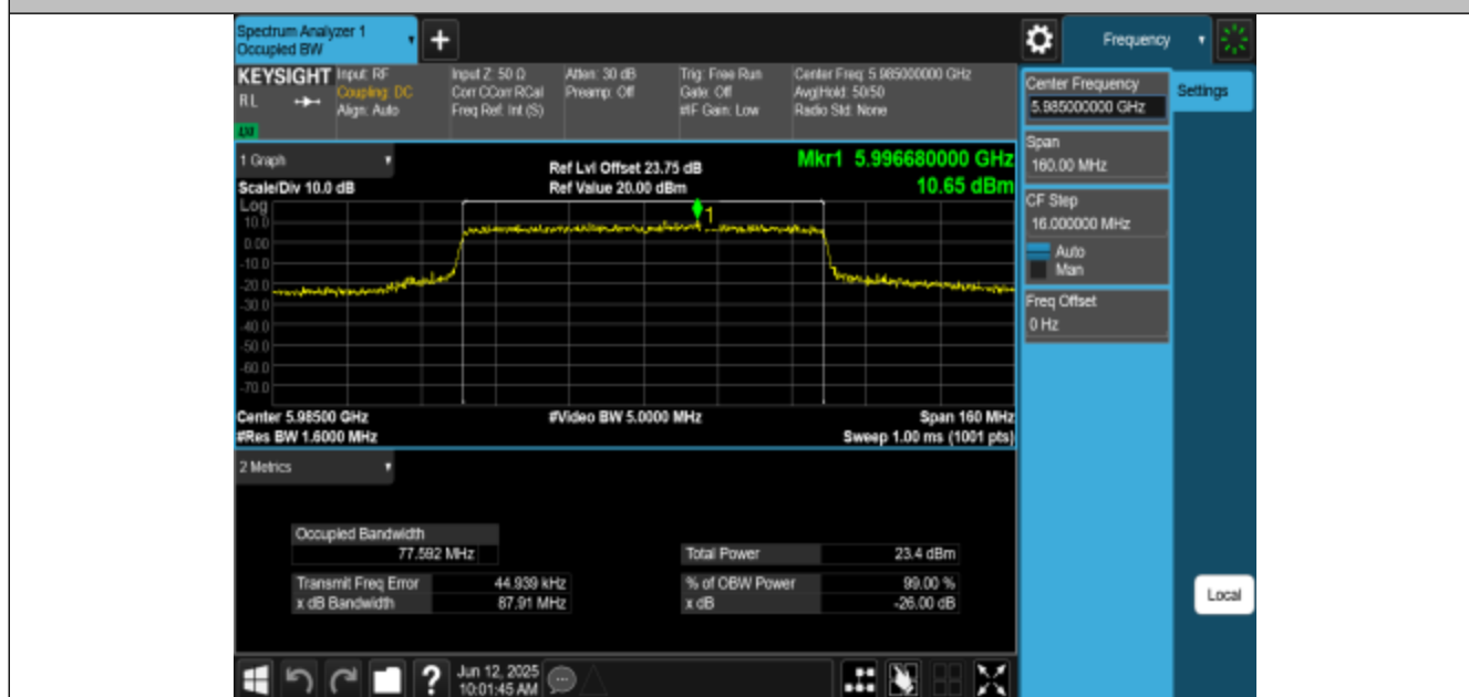
11AX80MIMO-Ant3-5985-PASS
