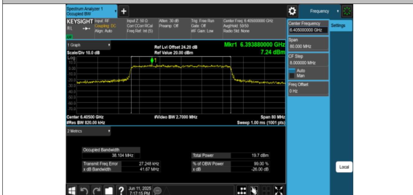
11AX40MIMO-Ant3-6405-PASS
