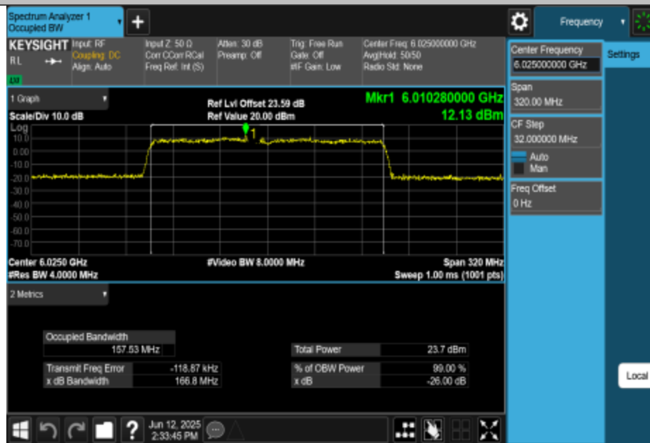
11AX160MIMO-Ant1-6025-PASS
