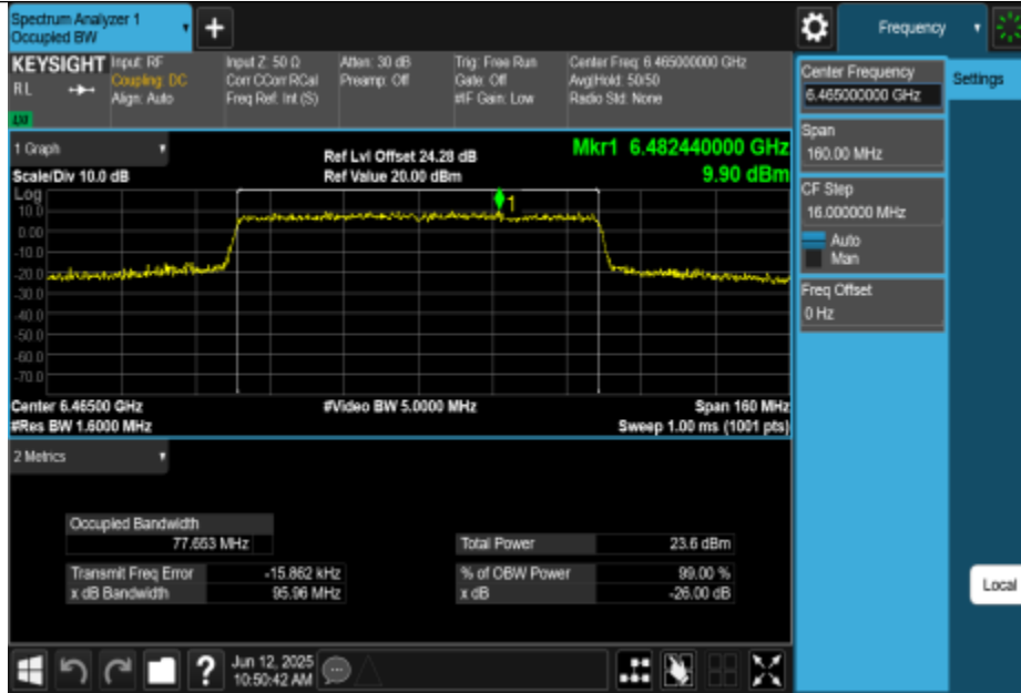
11AX80MIMO-Ant2-6465-PASS
