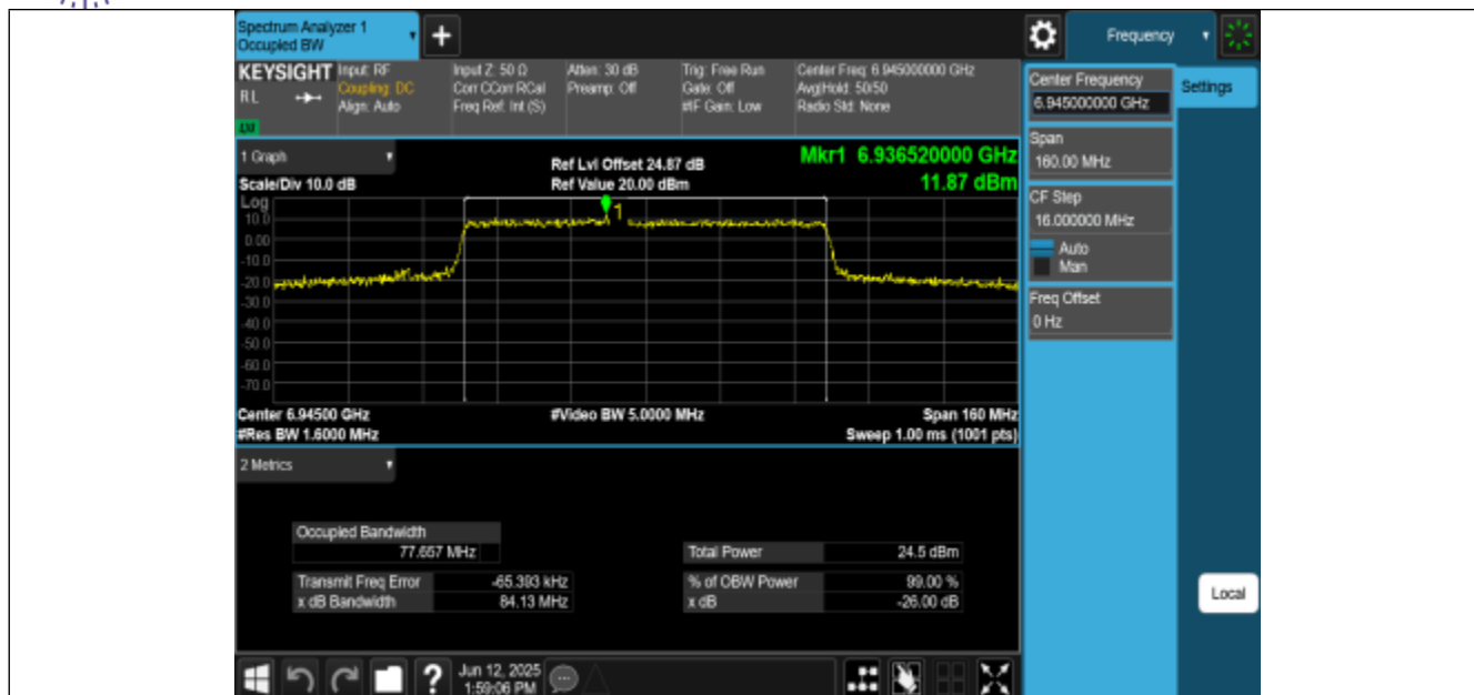
11AX80MIMO-Ant2-6945-PASS
