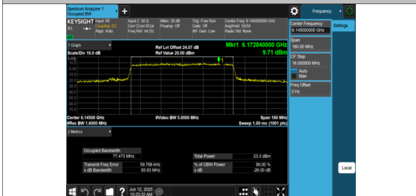
11AX80MIMO-Ant3-6145-PASS
