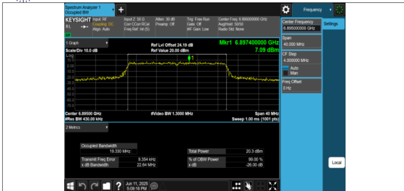
11AX20MIMO-Ant0-6895-PASS
