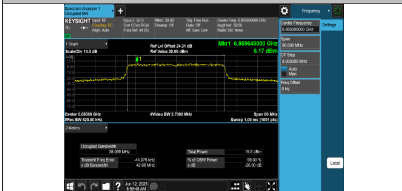
11AX40MIMO-Ant1-6885-PASS
