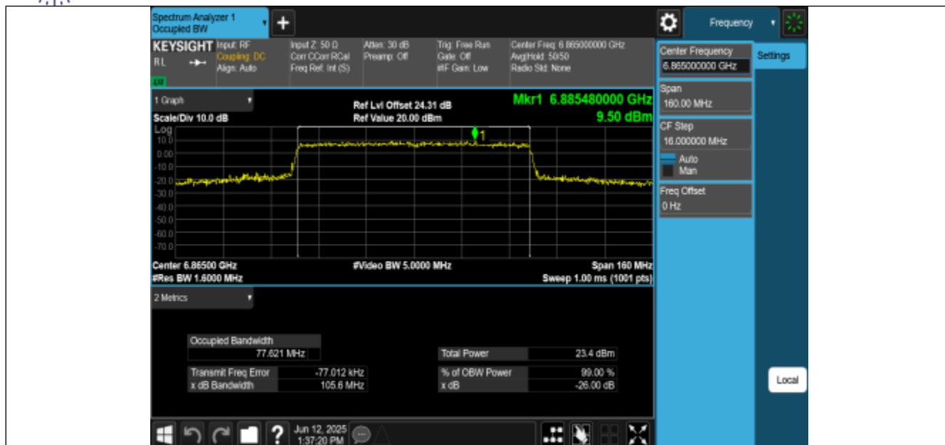
11AX80MIMO-Ant0-6865-PASS
