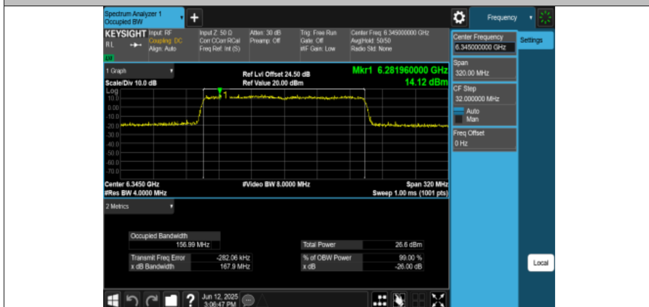
11AX160MIMO-Ant1-6345-PASS
