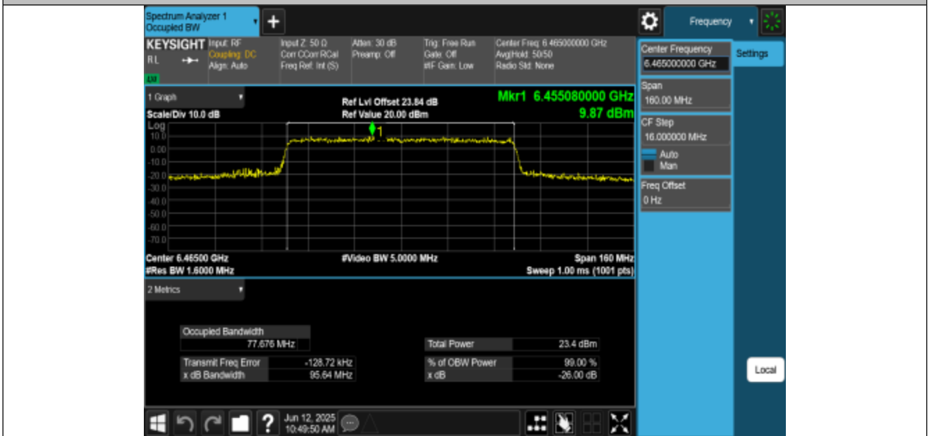
11AX80MIMO-Ant1-6465-PASS
