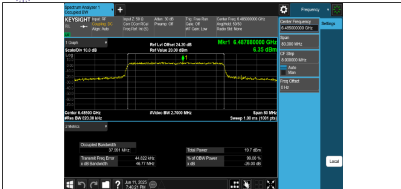
11AX40MIMO-Ant2-6485-PASS
