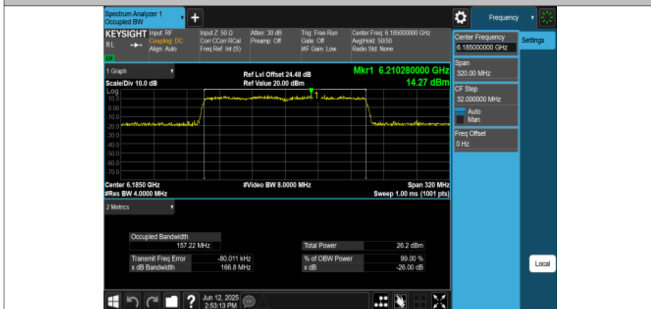
11AX160MIMO-Ant1-6185-PASS
