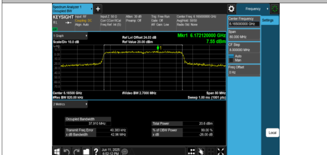
11AX40MIMO-Ant1-6165-PASS
