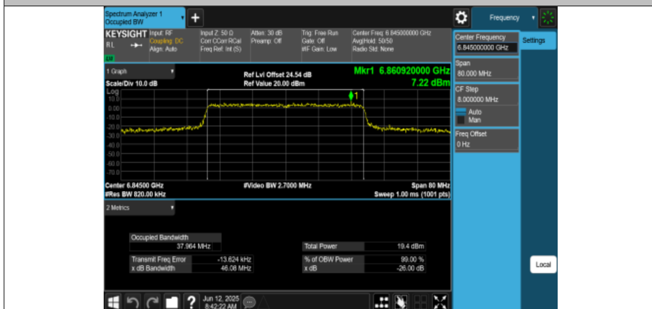
11AX40MIMO-Ant1-6845-PASS
