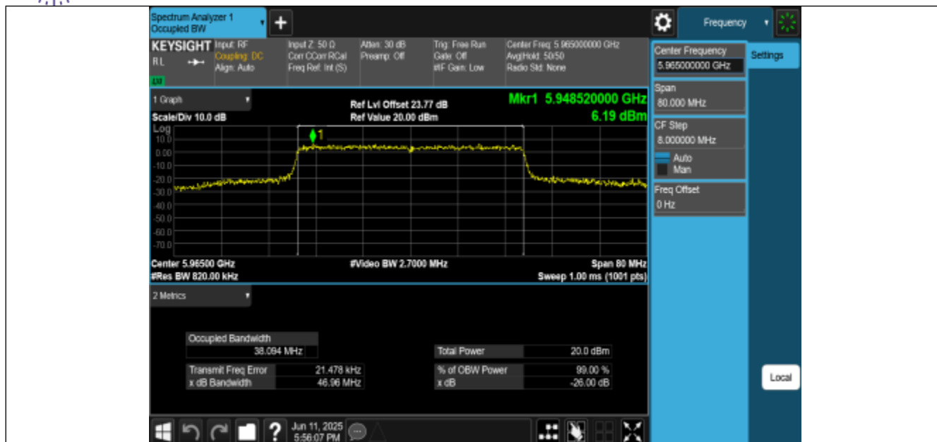
11AX40MIMO-Ant2-5965-PASS
