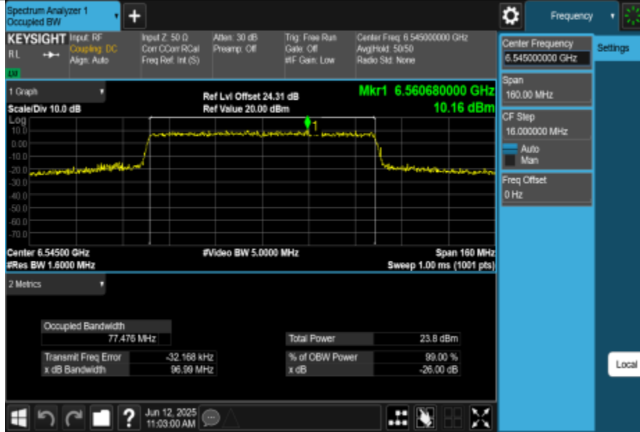
11AX80MIMO-Ant0-6545-PASS
