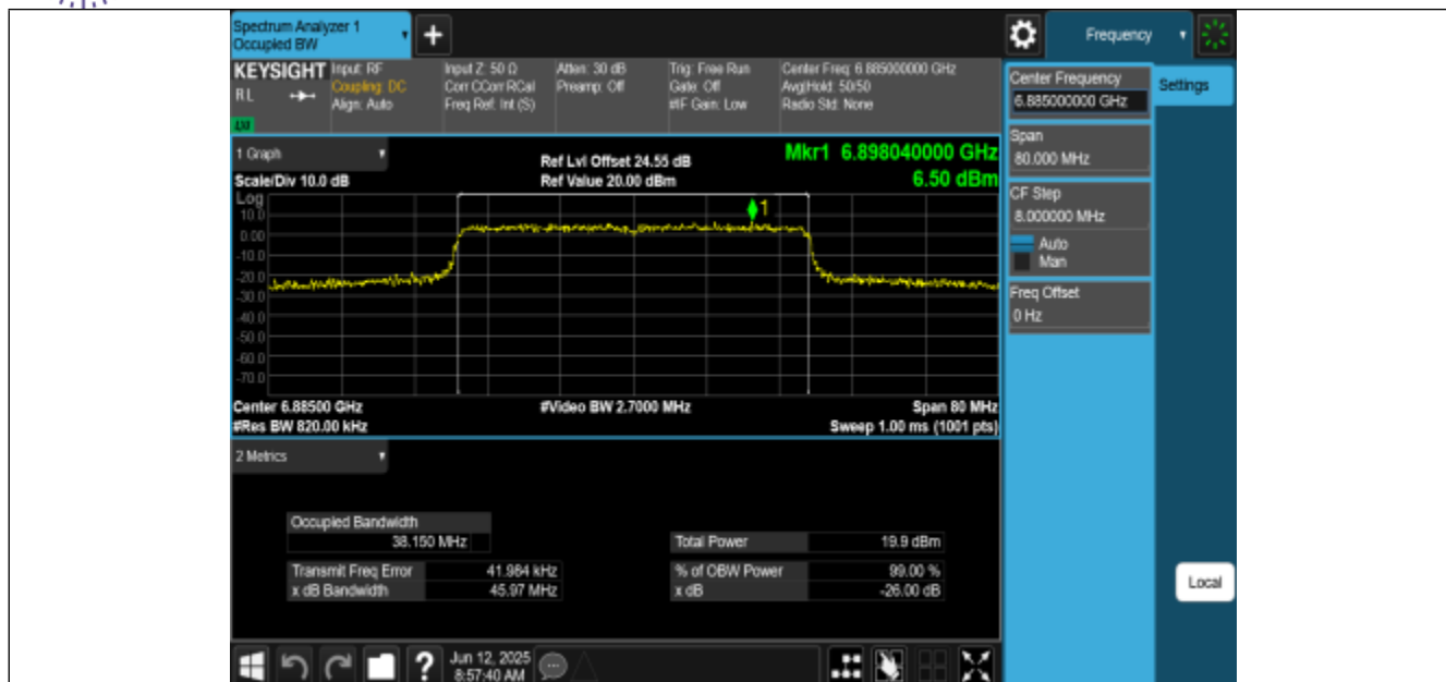
11AX40MIMO-Ant2-6885-PASS
