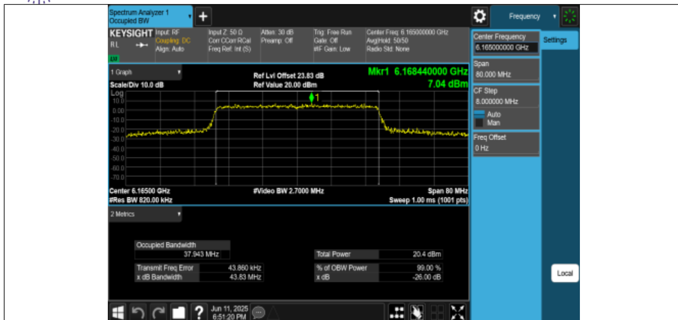
11AX40MIMO-Ant0-6165-PASS
