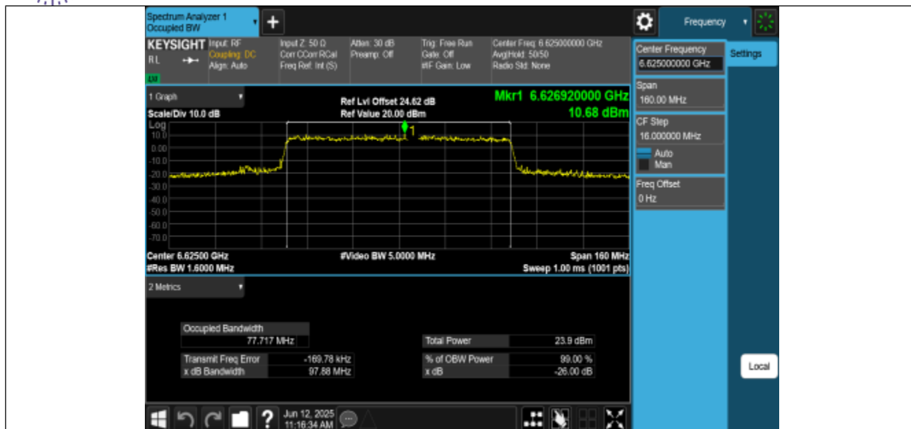
11AX80MIMO-Ant0-6625-PASS
