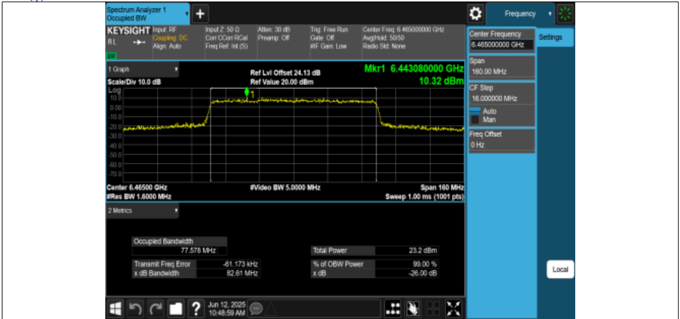
11AX80MIMO-Ant0-6465-PASS
