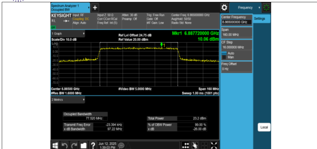
11AX80MIMO-Ant2-6865-PASS
