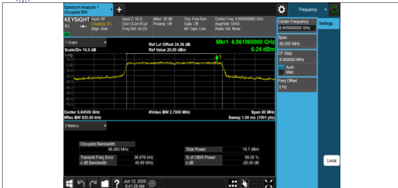
11AX40MIMO-Ant0-6845-PASS
