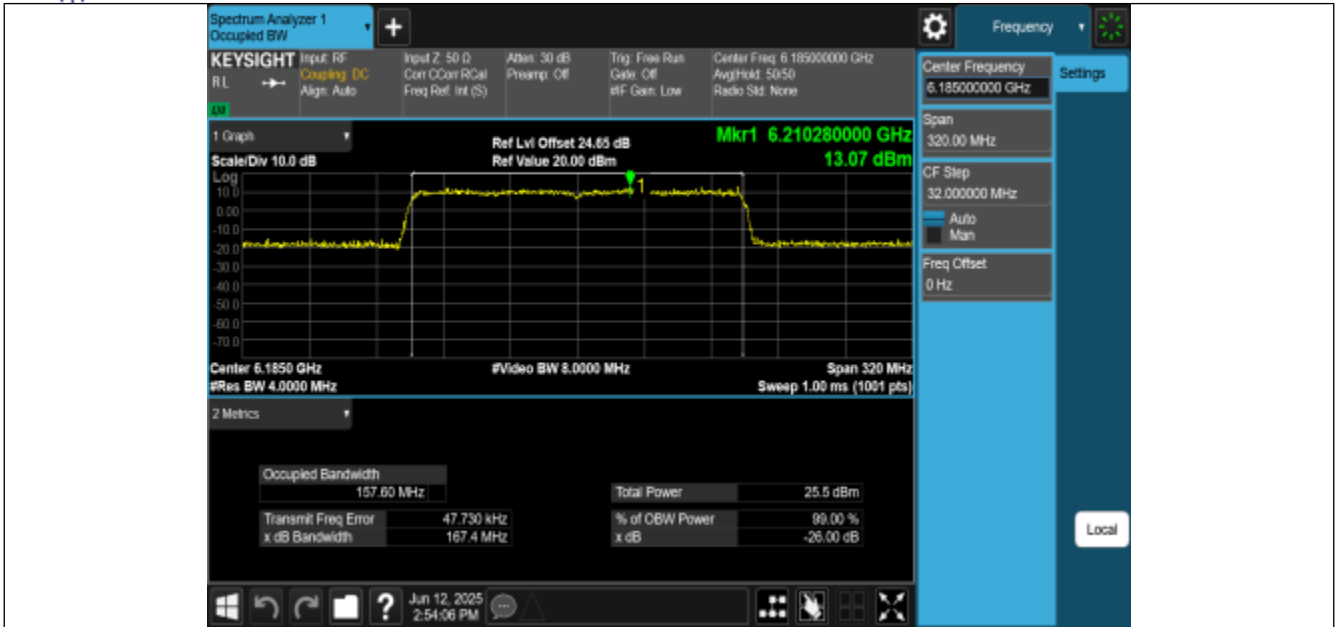
11AX160MIMO-Ant2-6185-PASS
