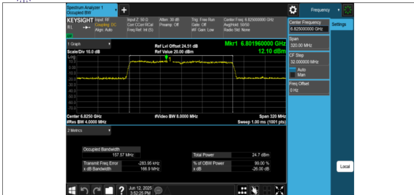
11AX160MIMO-Ant0-6825-PASS
