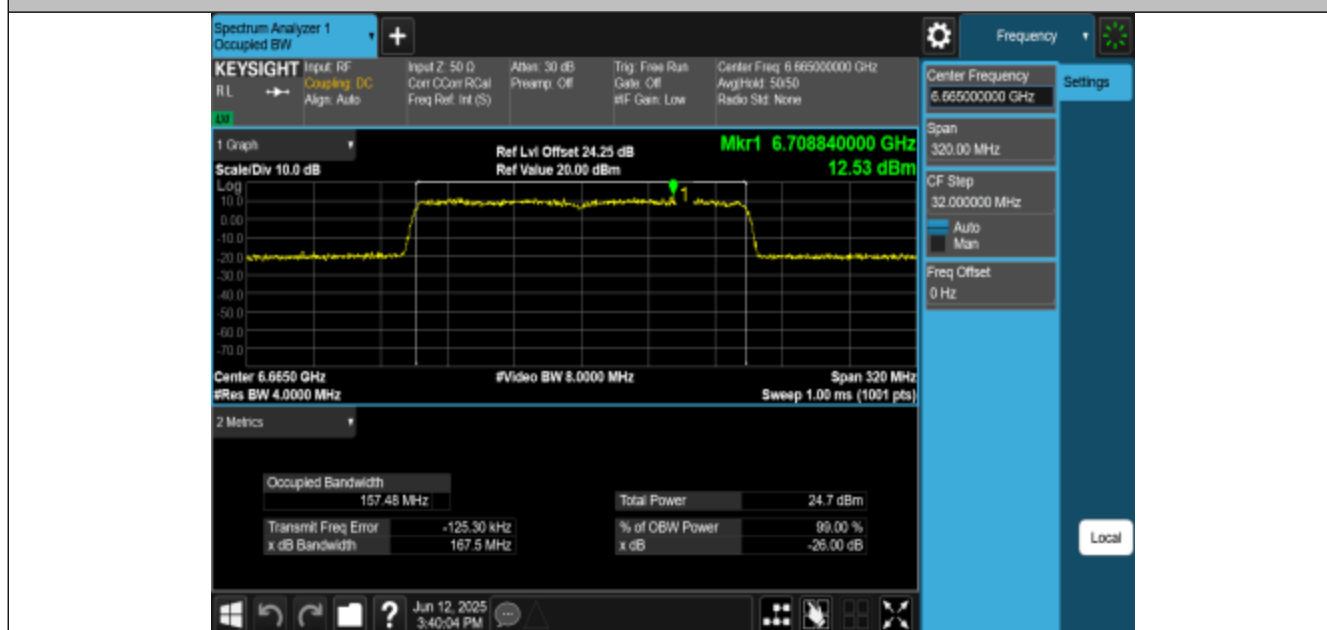
11AX160MIMO-Ant1-6665-PASS
