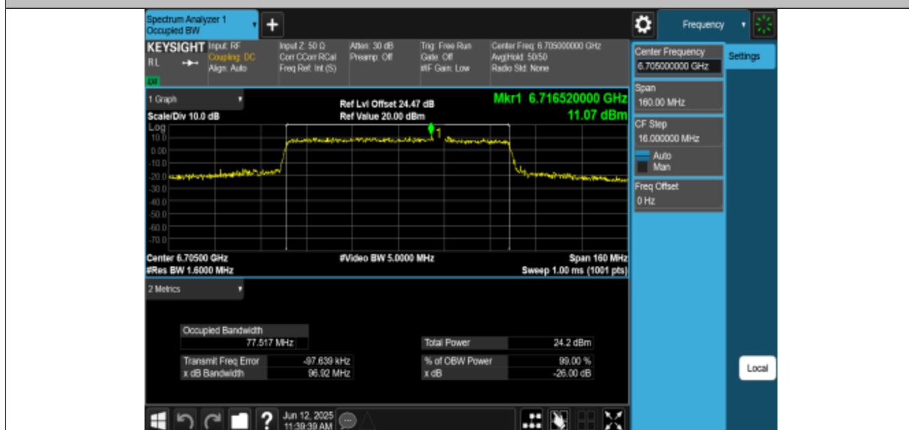
11AX80MIMO-Ant3-6705-PASS
