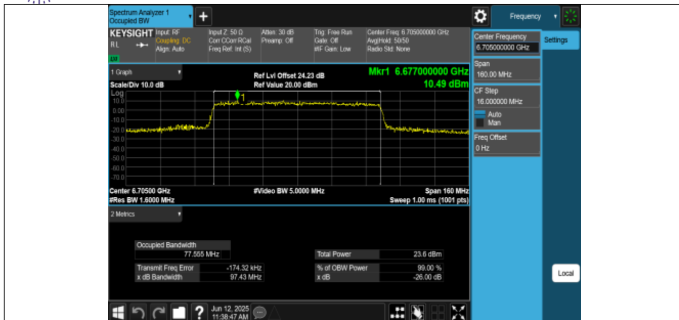
11AX80MIMO-Ant2-6705-PASS
