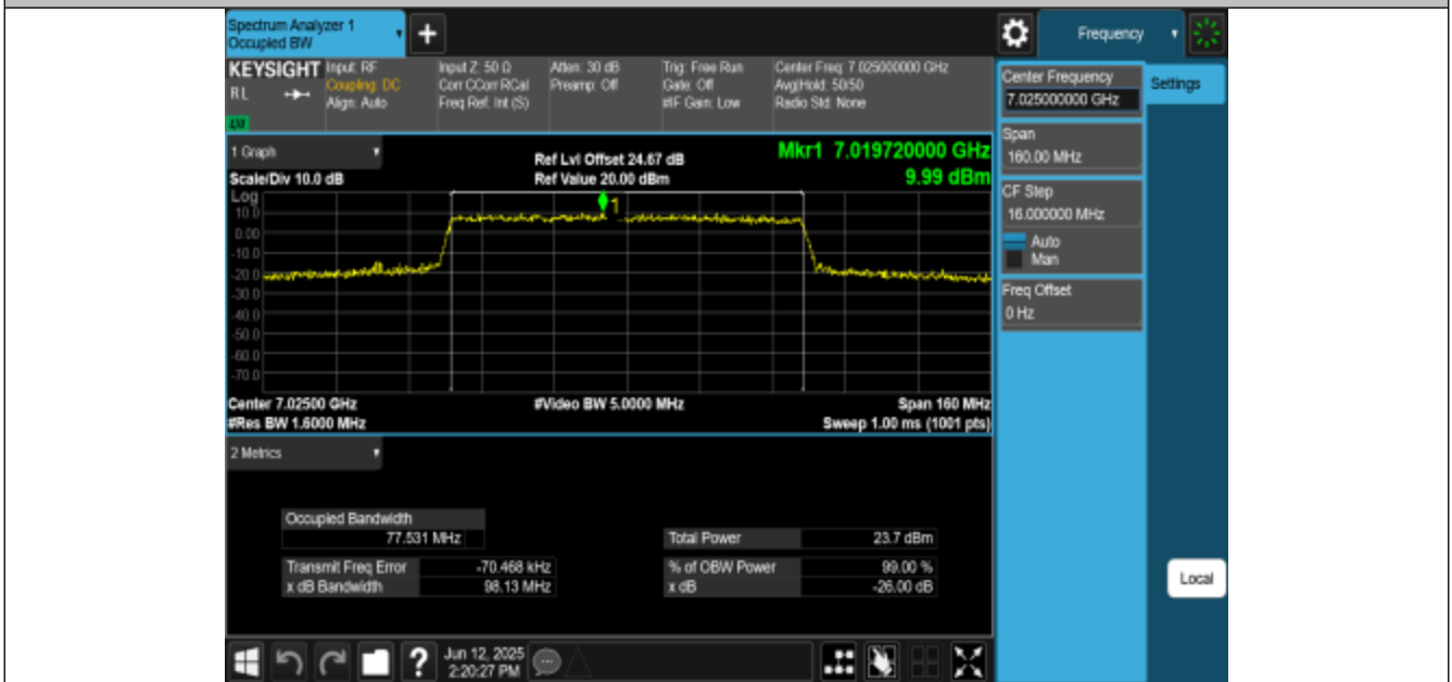
11AX80MIMO-Ant3-7025-PASS
