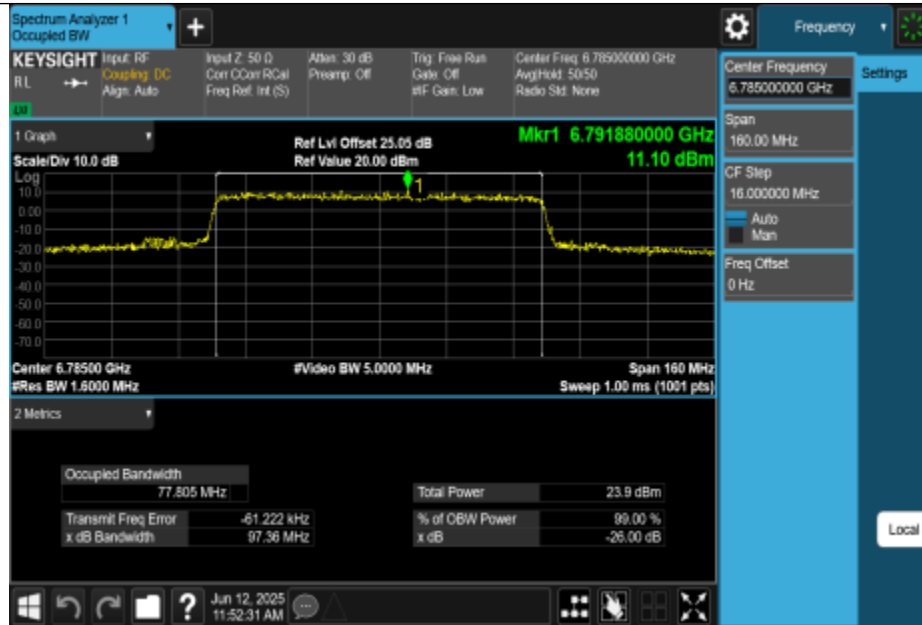
11AX80MIMO-Ant2-6785-PASS
