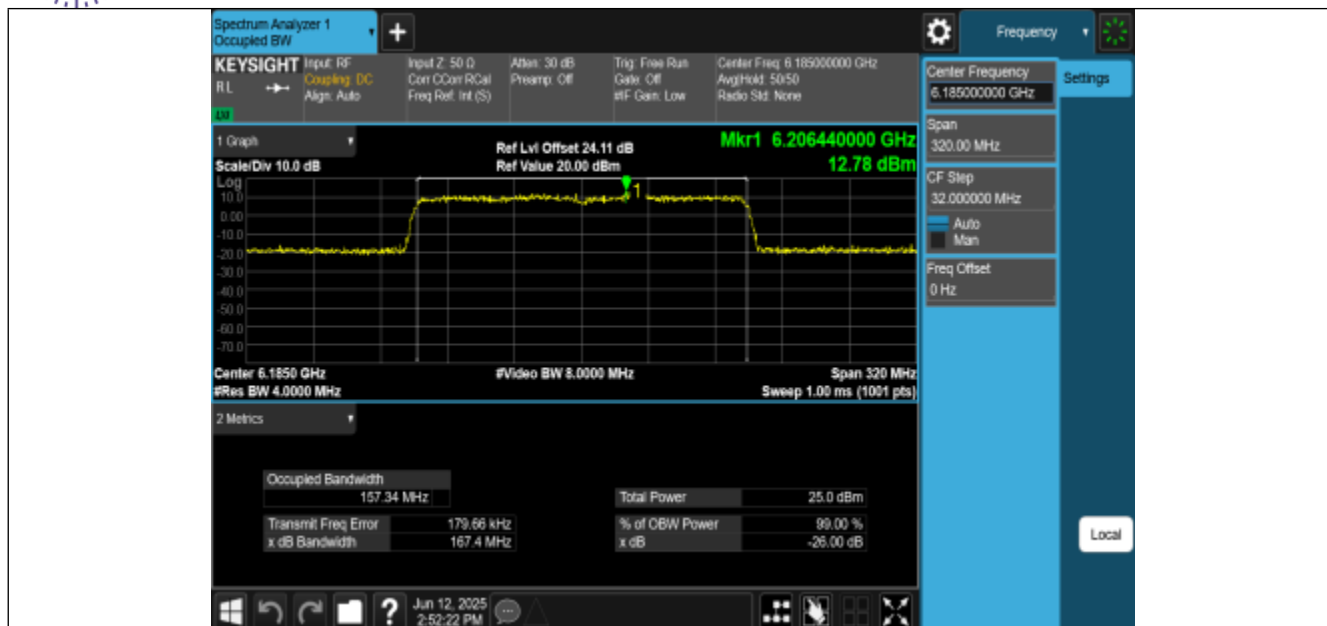
11AX160MIMO-Ant0-6185-PASS
