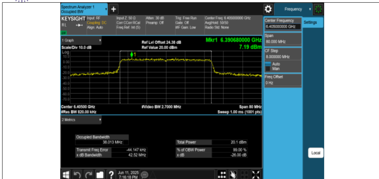
11AX40MIMO-Ant2-6405-PASS
