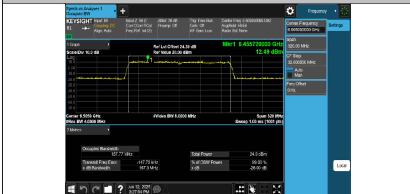
11AX160MIMO-Ant1-6505-PASS
