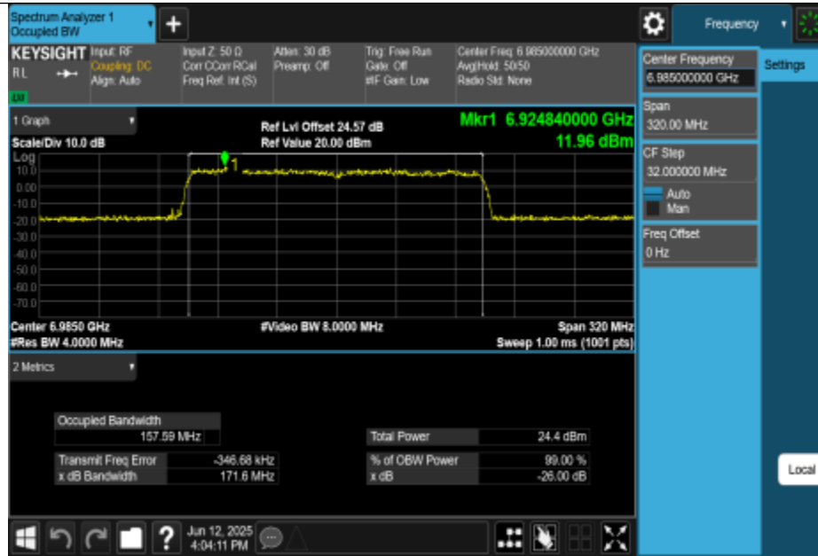
11AX160MIMO-Ant0-6985-PASS
