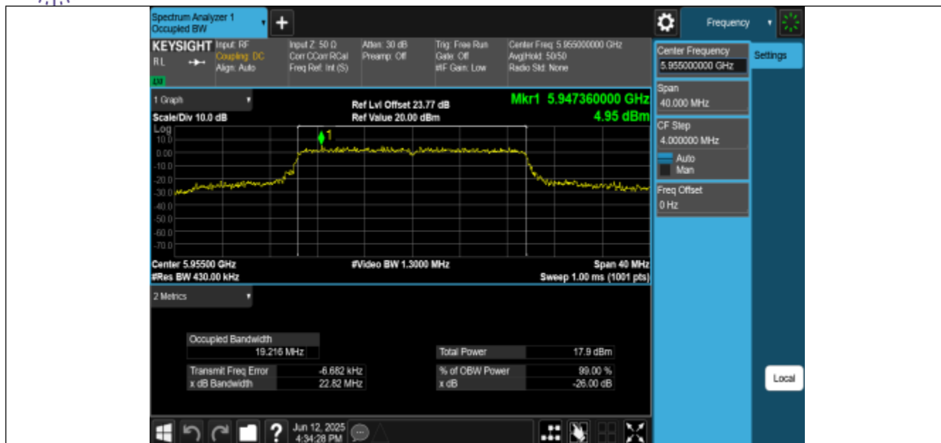
11BE20MIMO-Ant2-5955-PASS
