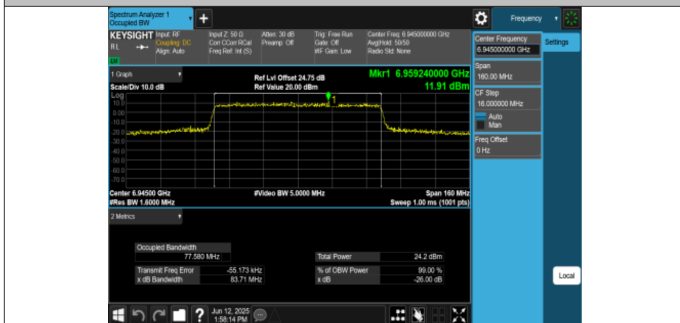
11AX80MIMO-Ant1-6945-PASS
