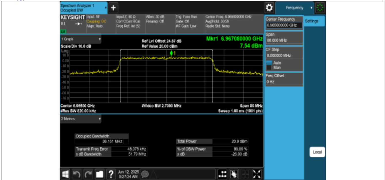
11AX40MIMO-Ant2-6965-PASS
