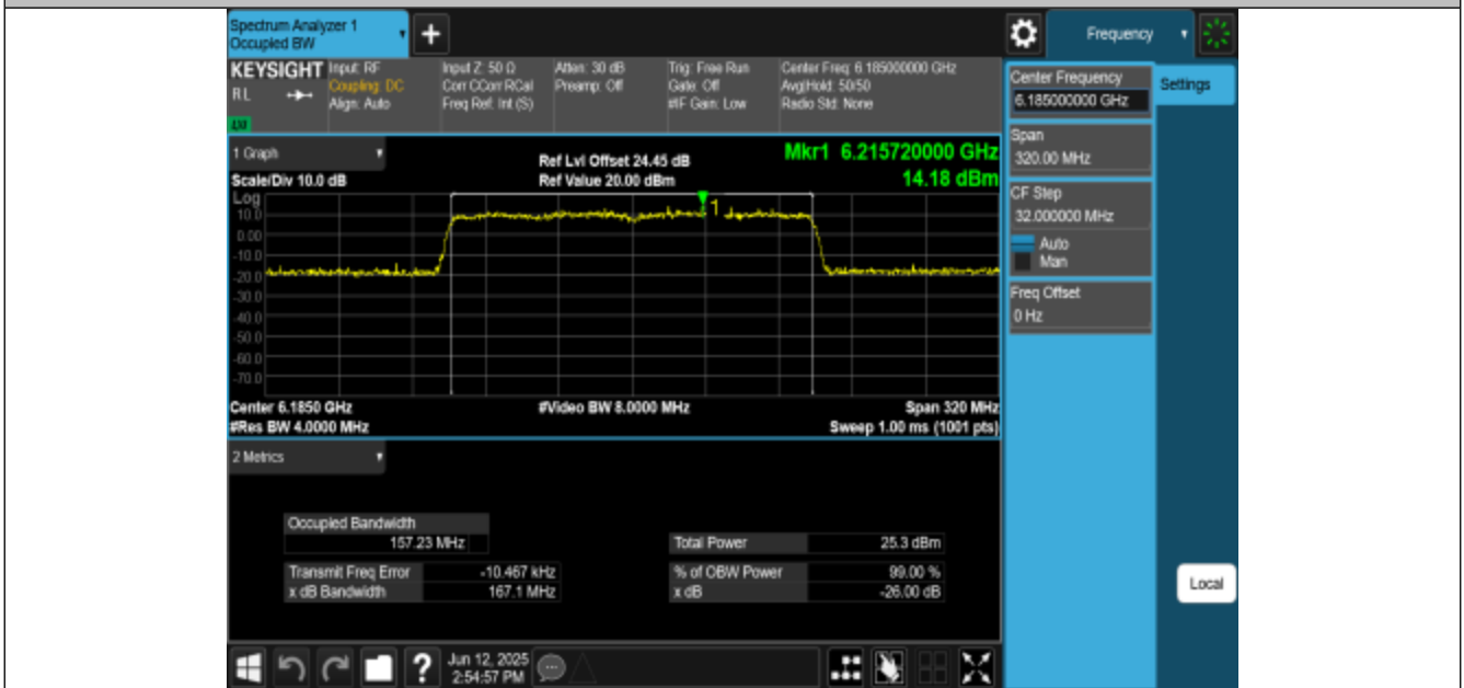
11AX160MIMO-Ant3-6185-PASS
