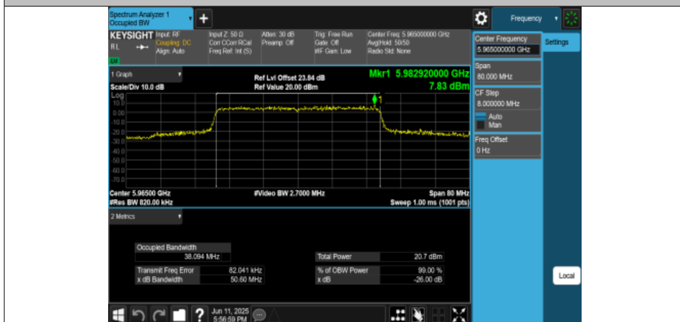
11AX40MIMO-Ant3-5965-PASS
