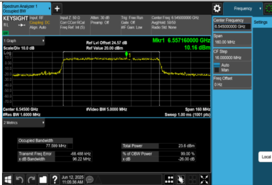
11AX80MIMO-Ant3-6545-PASS
