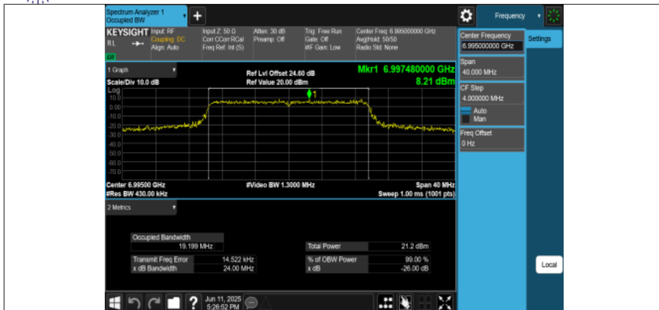
11AX20MIMO-Ant2-6995-PASS
