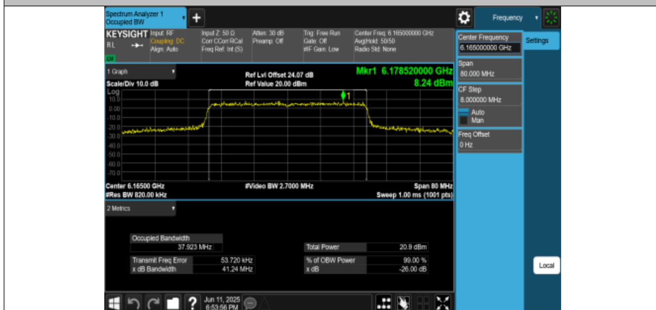
11AX40MIMO-Ant3-6165-PASS
