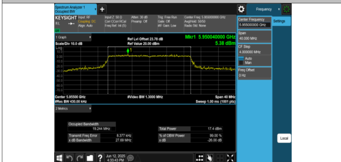
11BE20MIMO-Ant1-5955-PASS
