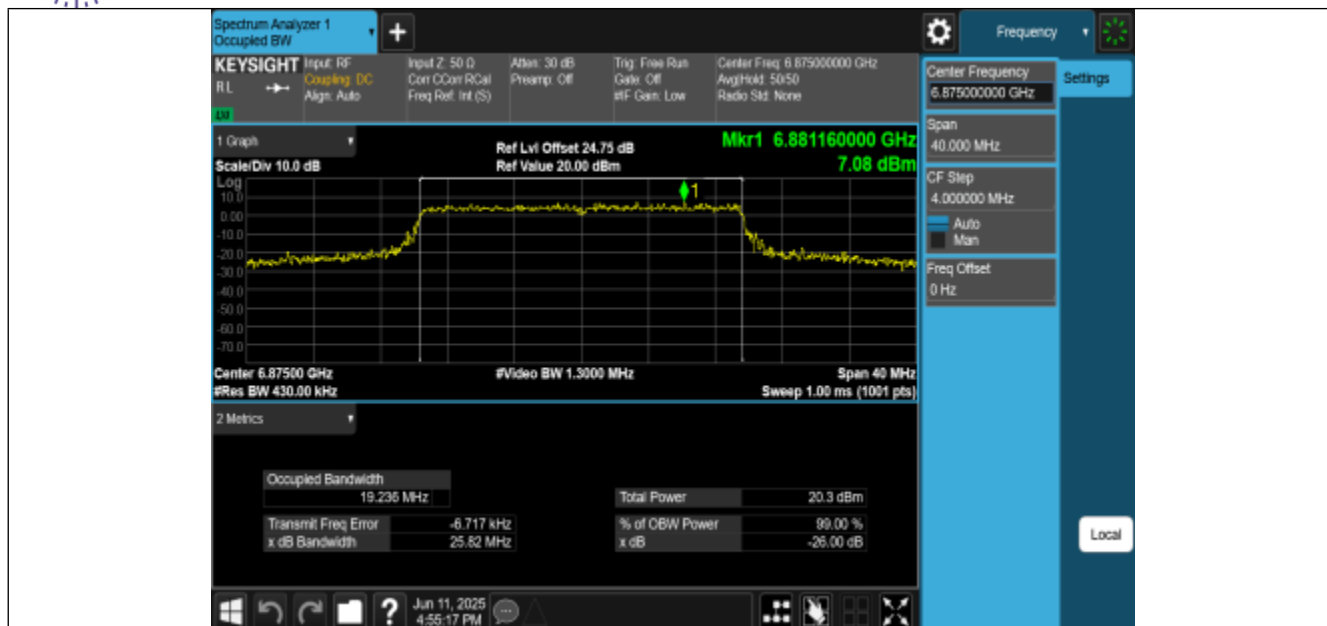
11AX20MIMO-Ant2-6875-PASS
