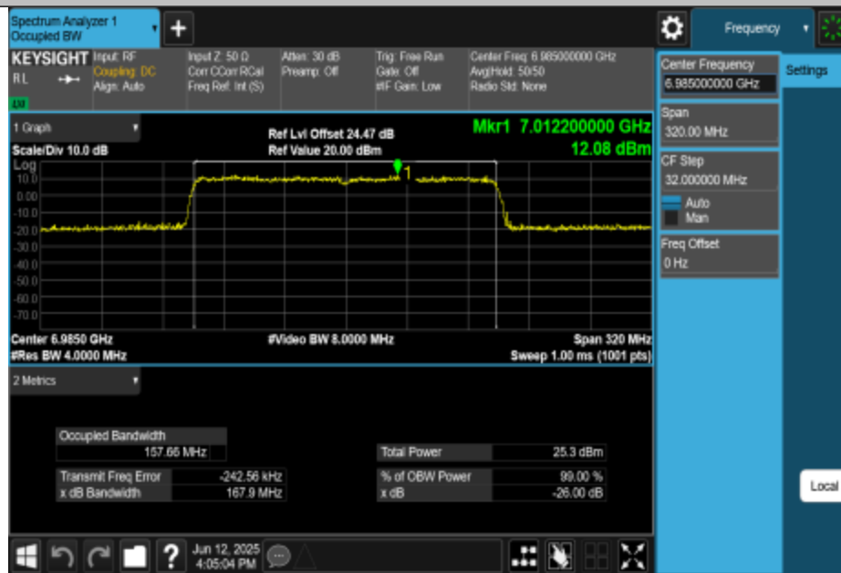
11AX160MIMO-Ant1-6985-PASS
