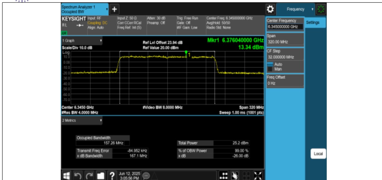
11AX160MIMO-Ant0-6345-PASS
