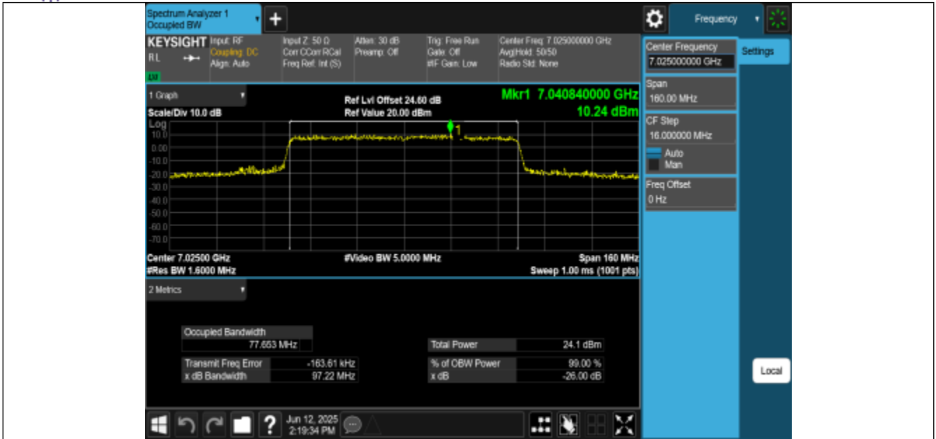
11AX80MIMO-Ant2-7025-PASS
