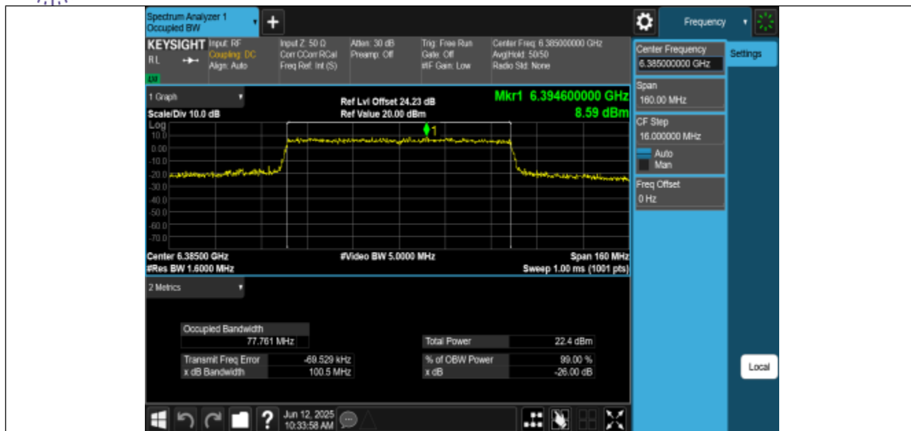
11AX80MIMO-Ant0-6385-PASS
