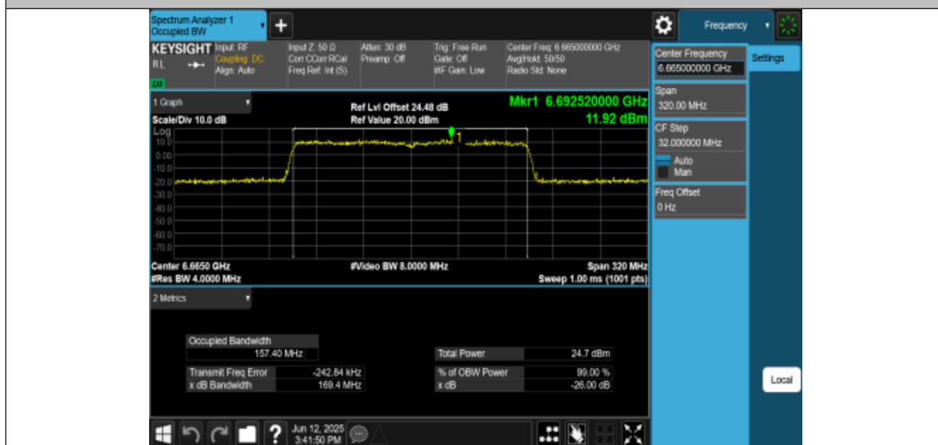
11AX160MIMO-Ant3-6665-PASS
