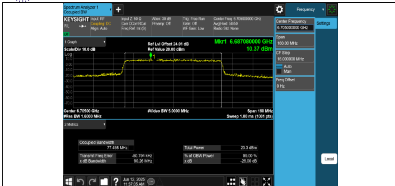
11AX80MIMO-Ant0-6705-PASS
