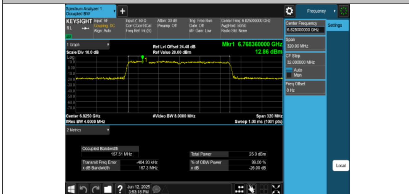
11AX160MIMO-Ant1-6825-PASS
