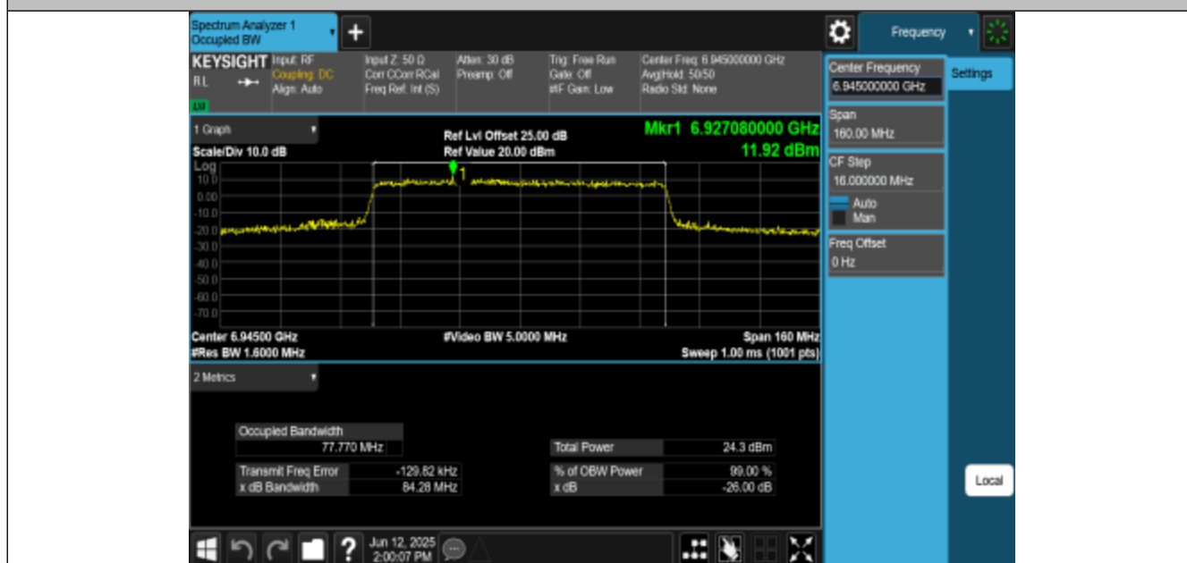
11AX80MIMO-Ant3-6945-PASS
