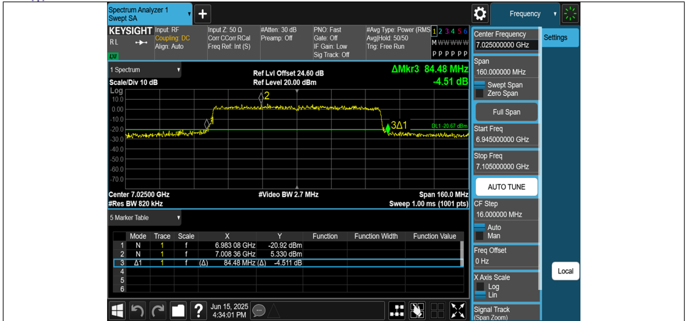
11BE80MIMO-Ant2-7025
