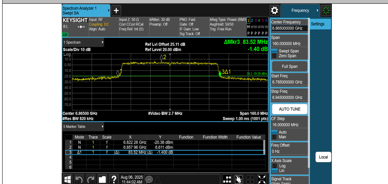
11BE80MIMO-Ant3-6865
