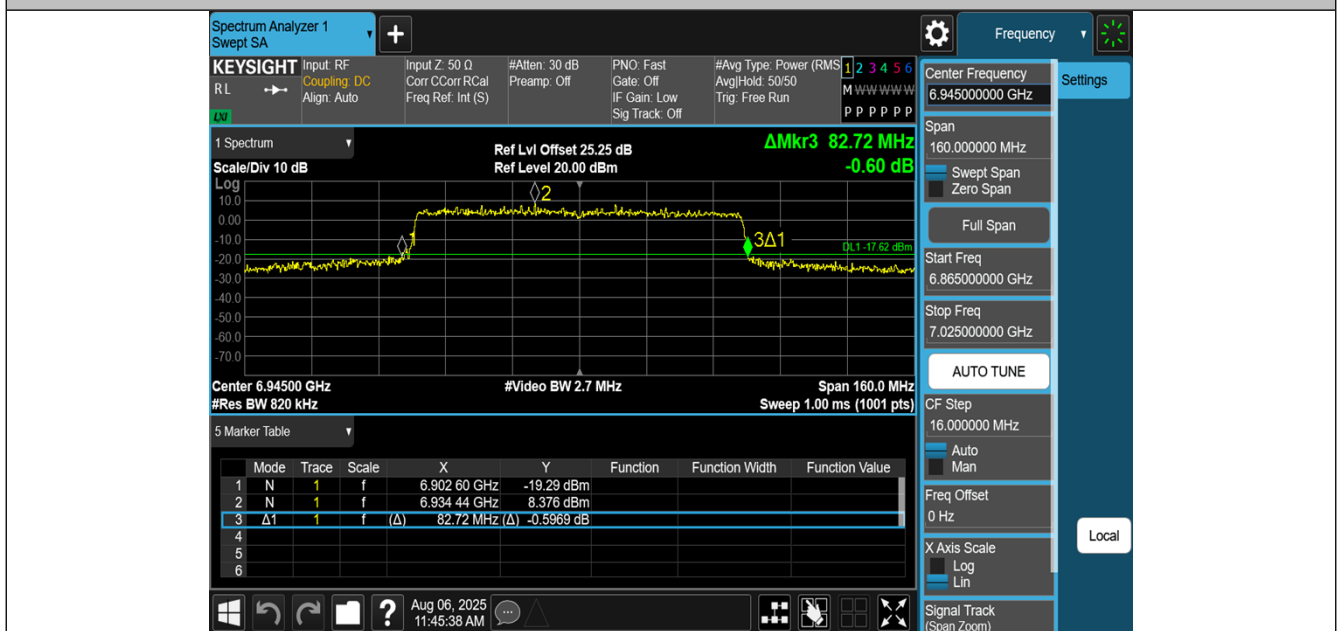
11BE80MIMO-Ant1-6945
