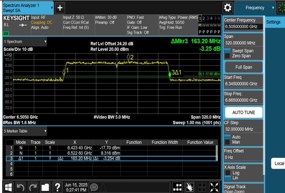
11BE160MIMO-Ant2-6505
