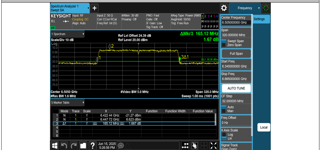
11BE160MIMO-Ant1-6505
