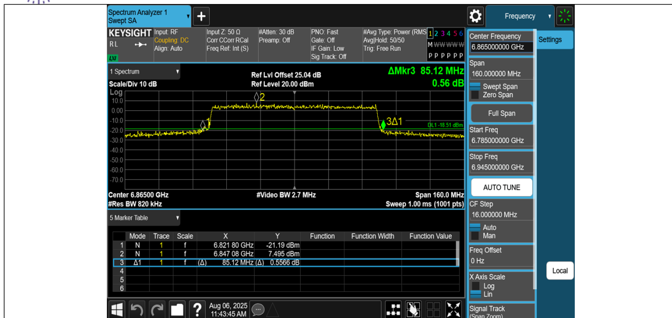
11BE80MIMO-Ant1-6865
