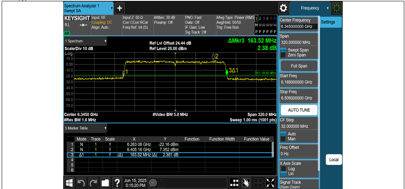
11BE160MIMO-Ant2-6345
