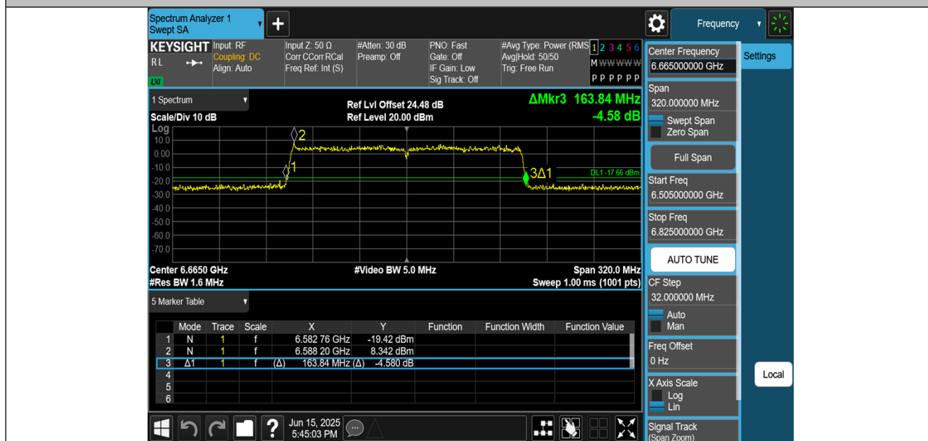
11BE160MIMO-Ant2-6665
