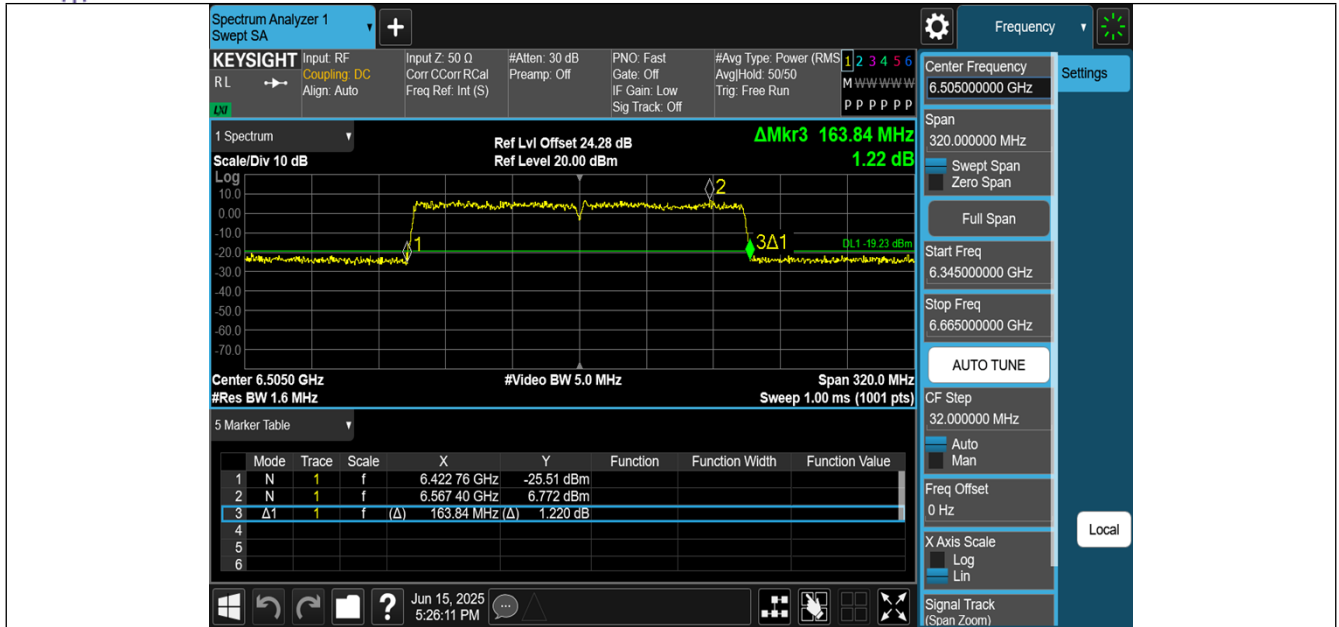
11BE160MIMO-Ant0-6505
