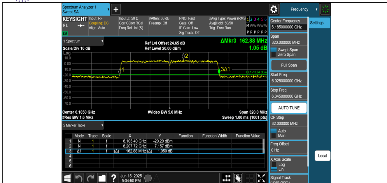
11BE160MIMO-Ant2-6185
