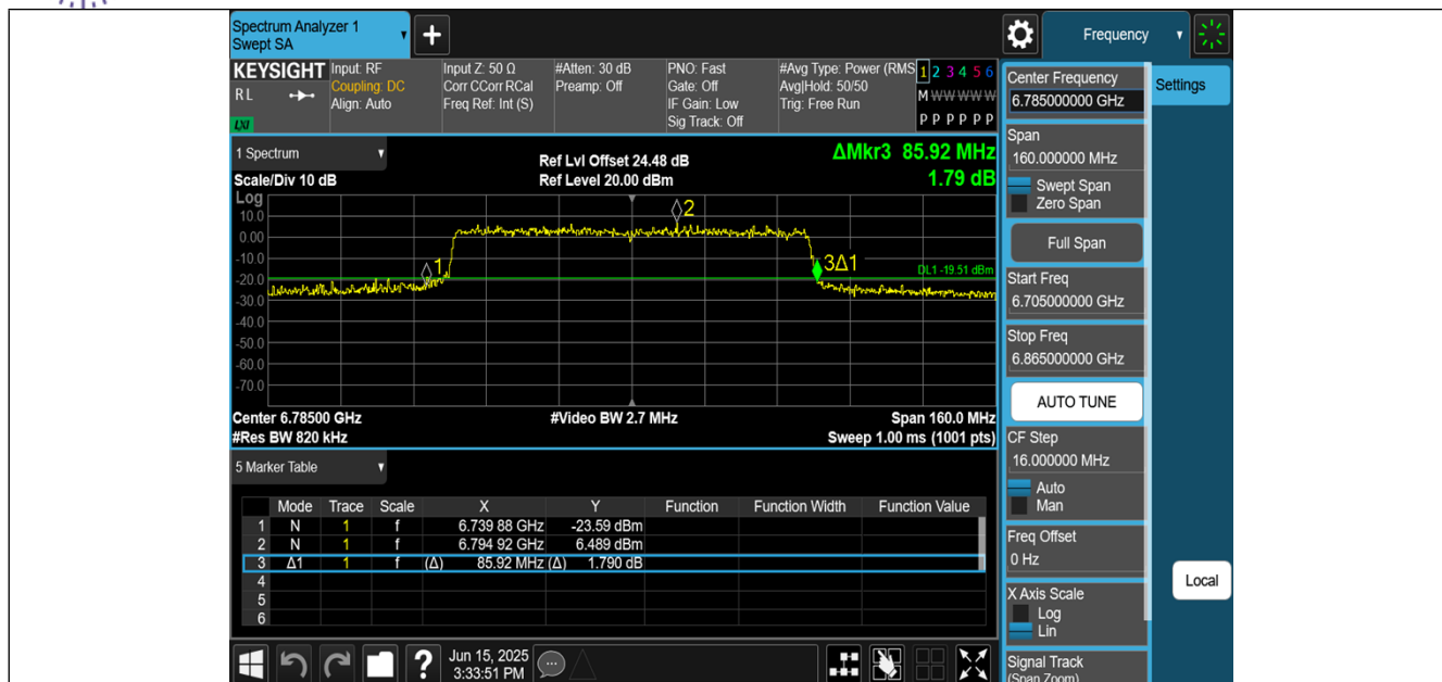
11BE80MIMO-Ant1-6785
