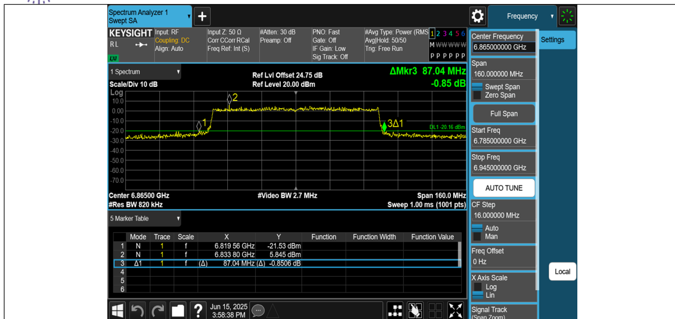
11BE80MIMO-Ant2-6865
