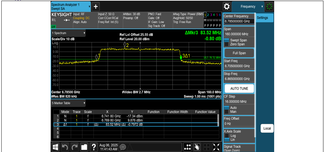
11BE80MIMO-Ant2-6785
