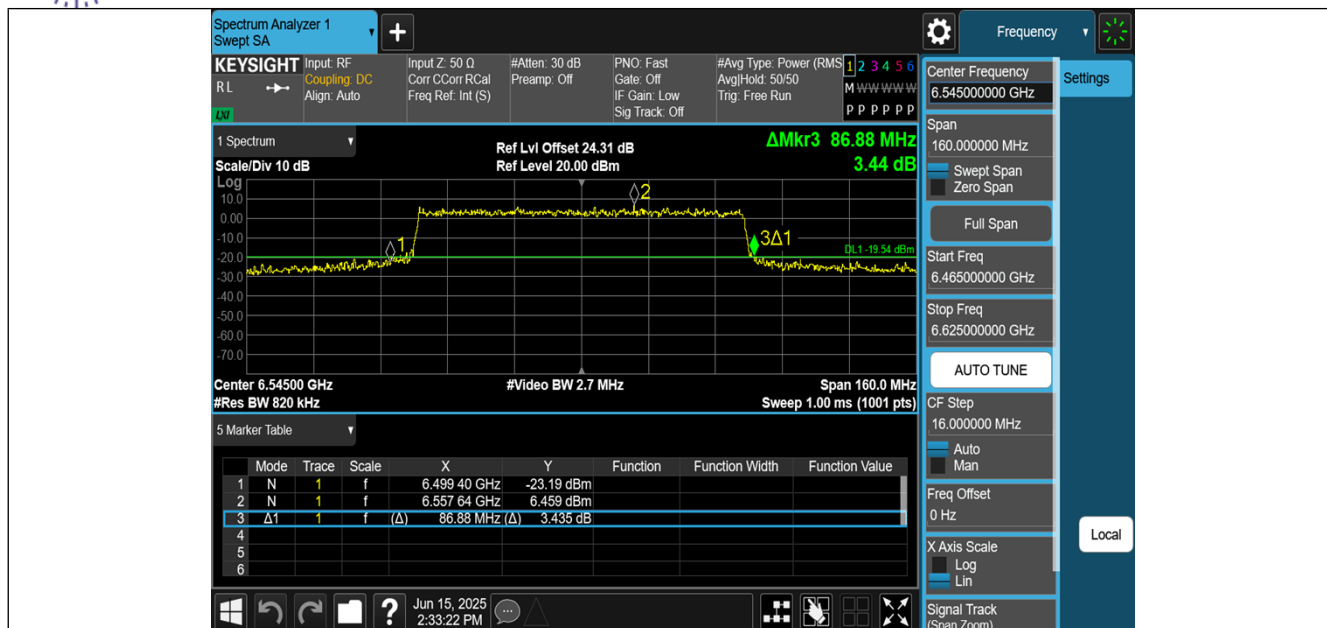
11BE80MIMO-Ant0-6545
