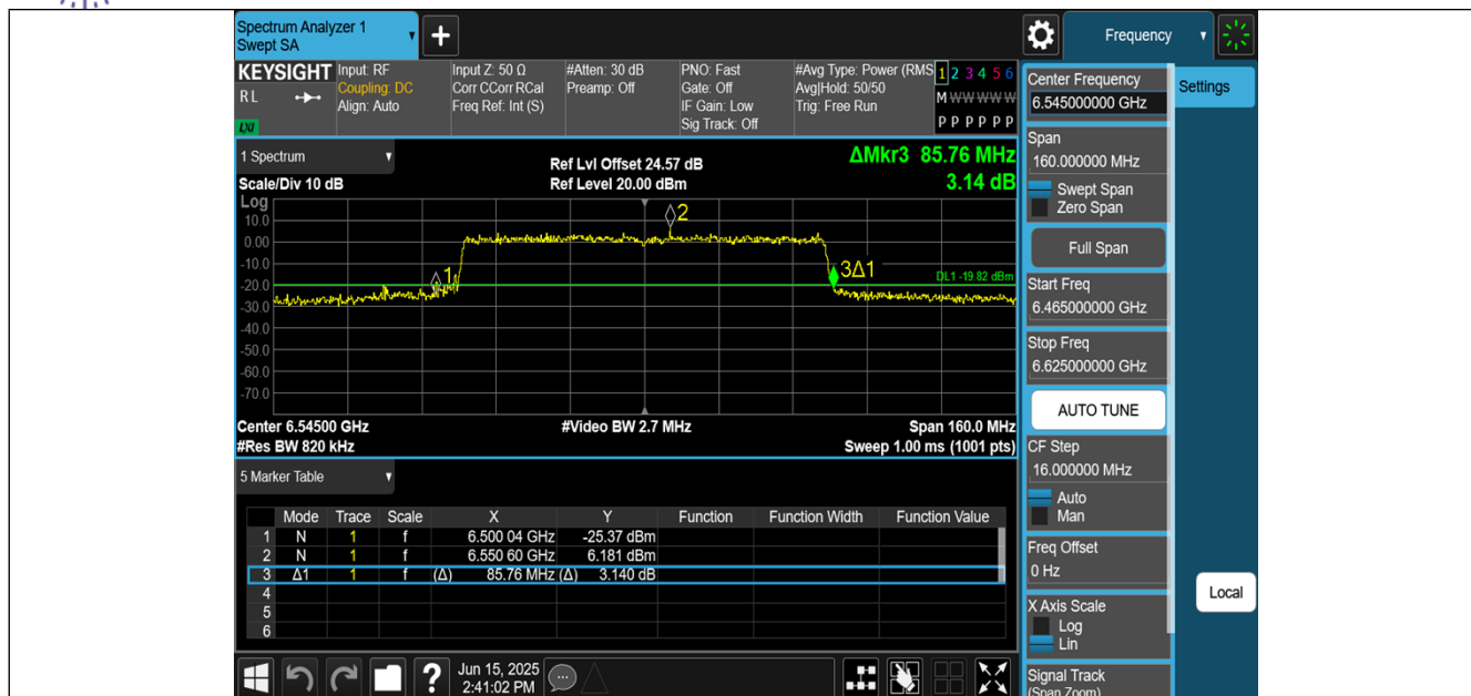
11BE80MIMO-Ant3-6545
