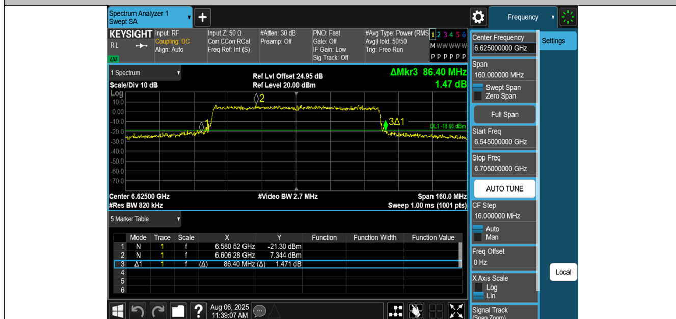
11BE80MIMO-Ant1-6625
