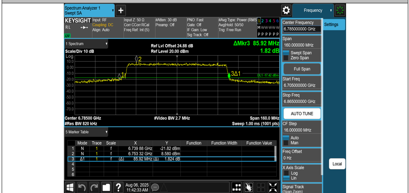
11BE80MIMO-Ant0-6785
