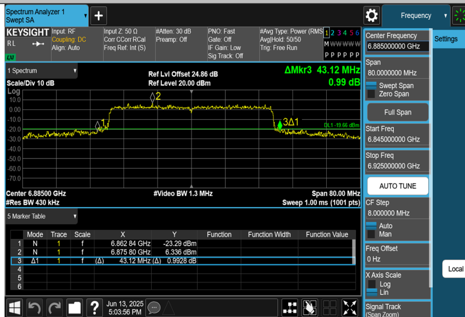
11BE40MIMO-Ant3-6885
