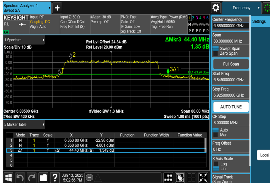
11BE40MIMO-Ant0-6885
