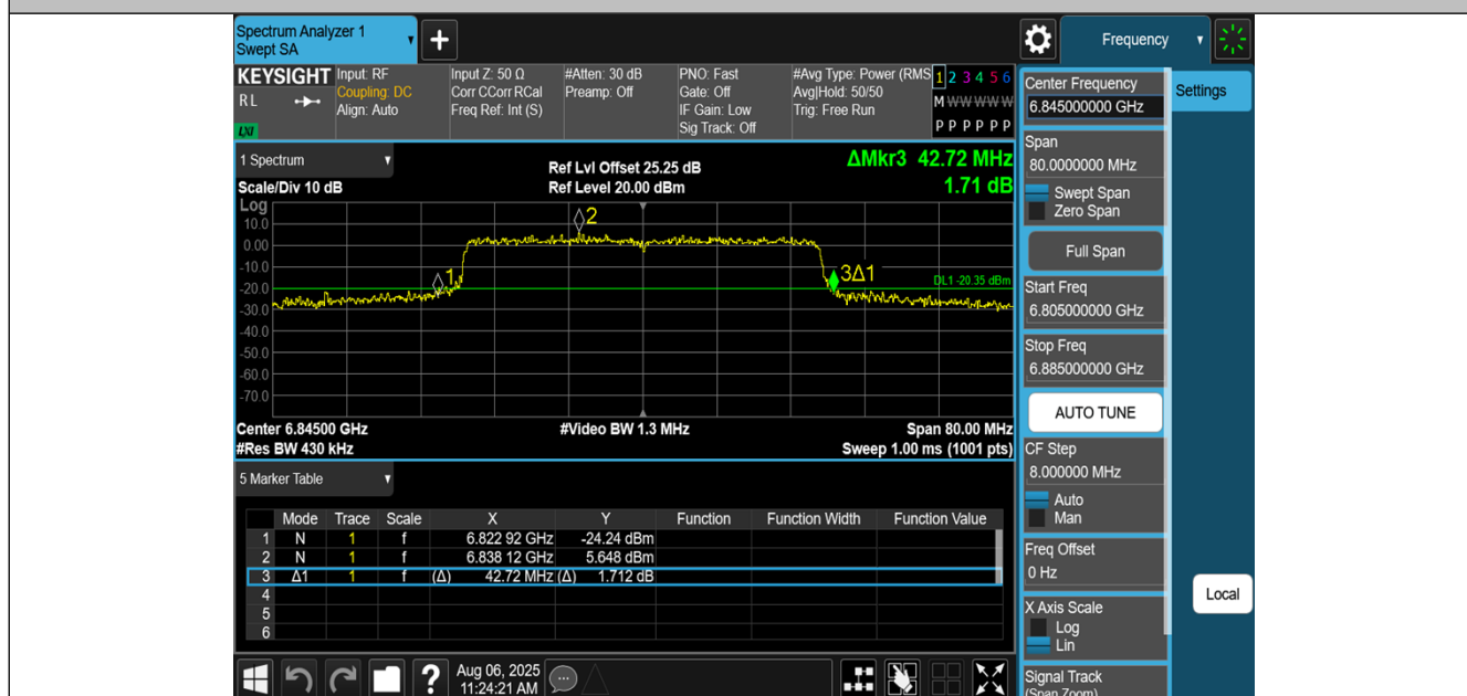
11BE40MIMO-Ant2-6845
