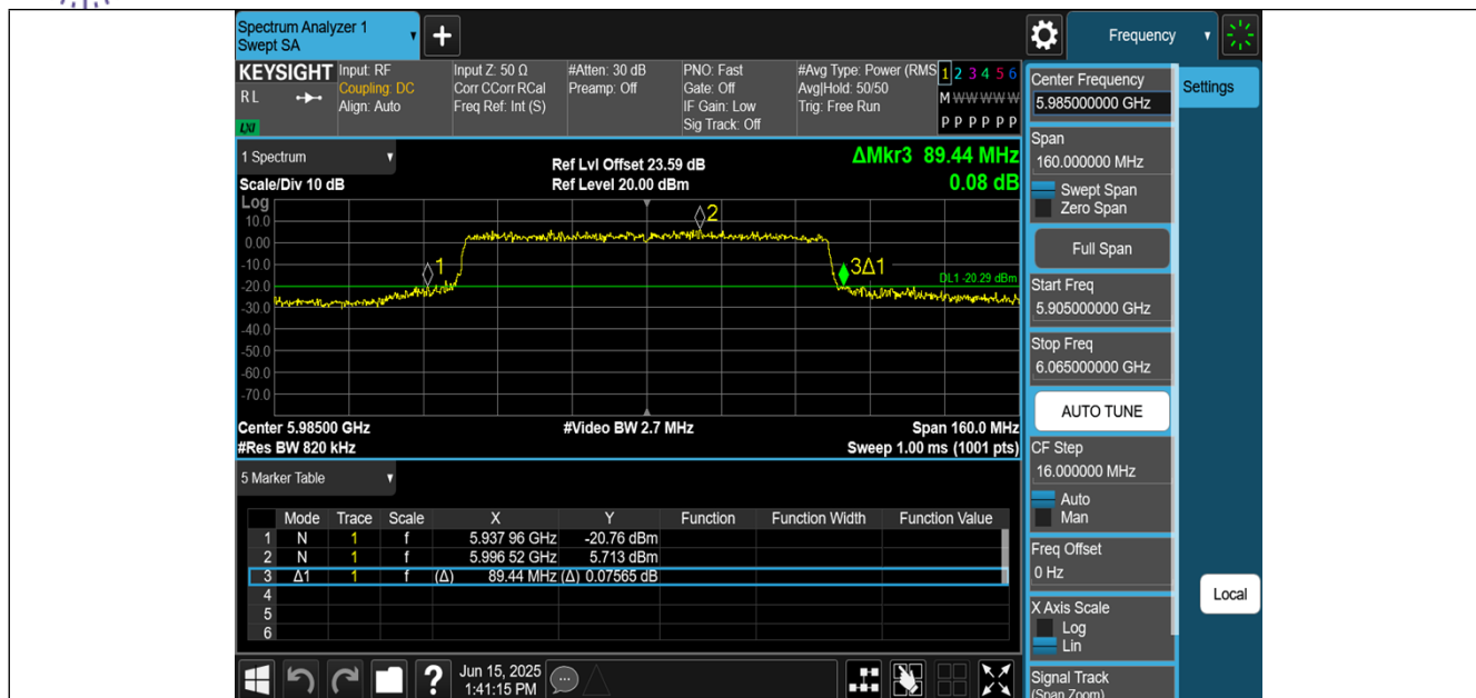
11BE80MIMO-Ant1-5985
