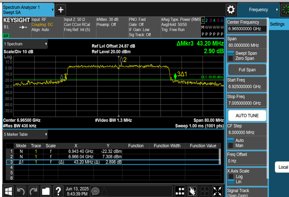
11BE40MIMO-Ant2-6965
