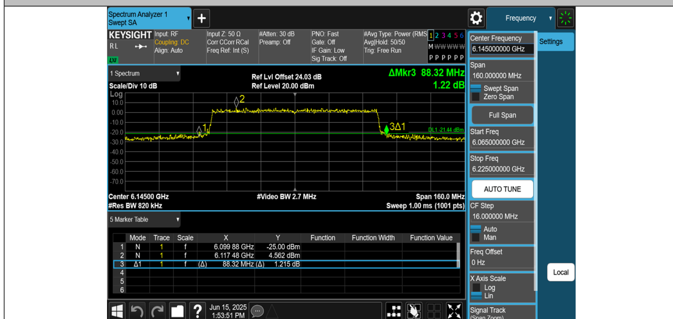
11BE80MIMO-Ant1-6145
