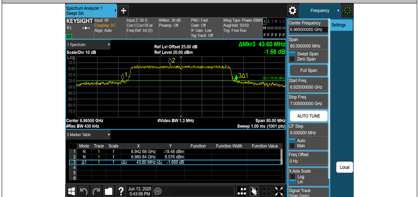
11BE40MIMO-Ant3-6965
