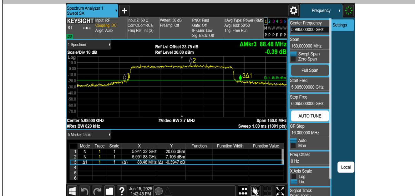
11BE80MIMO-Ant3-5985
