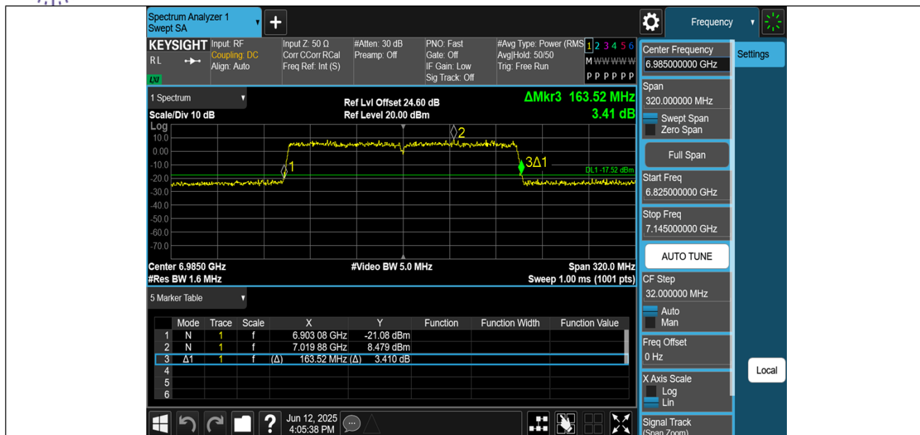
11AX160MIMO-Ant2-6985
