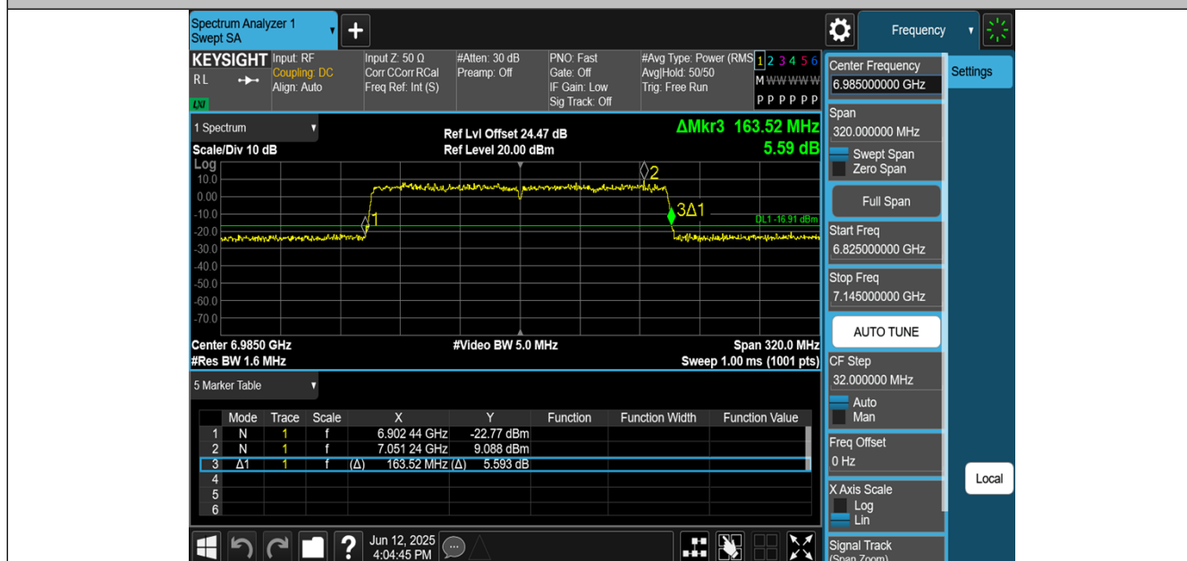
11AX160MIMO-Ant1-6985
