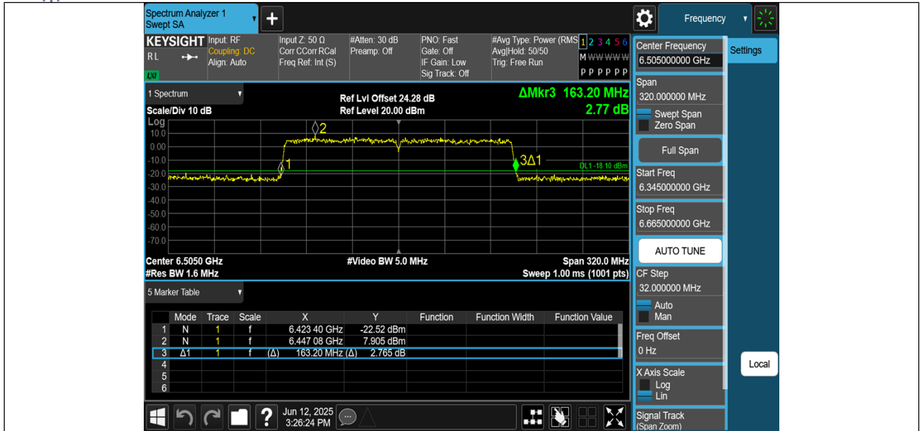
11AX160MIMO-Ant0-6505
