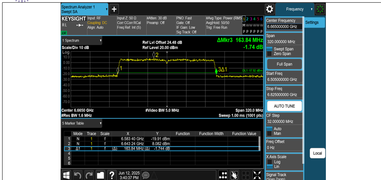
11AX160MIMO-Ant2-6665
