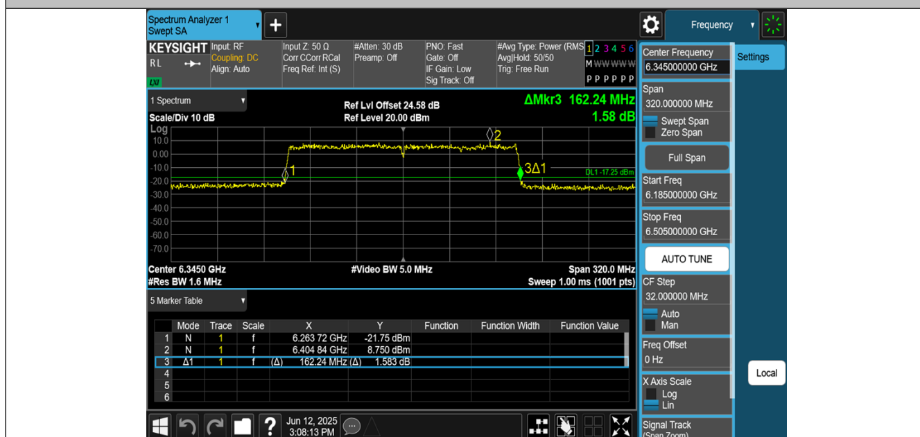
11AX160MIMO-Ant3-6345
