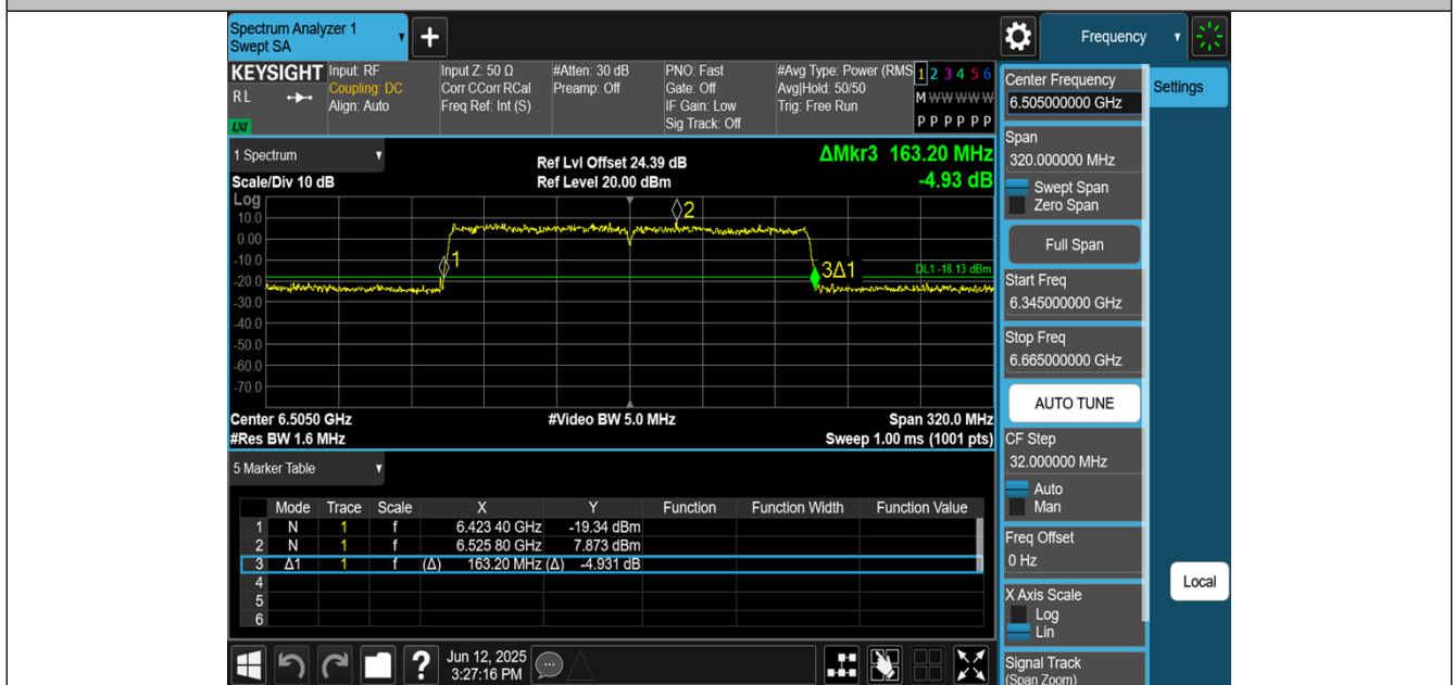
11AX160MIMO-Ant1-6505
