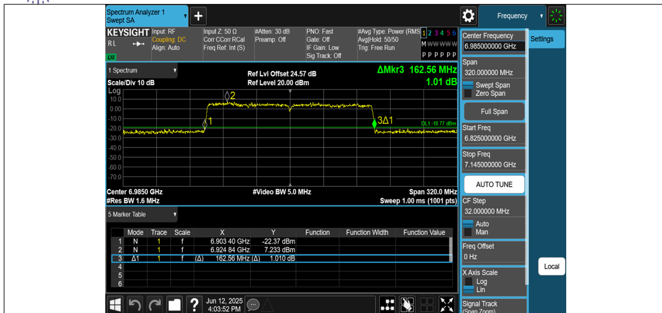
11AX160MIMO-Ant0-6985
