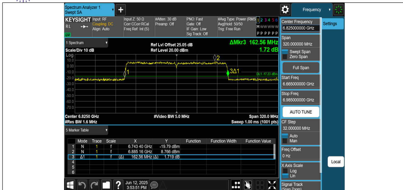
11AX160MIMO-Ant2-6825
