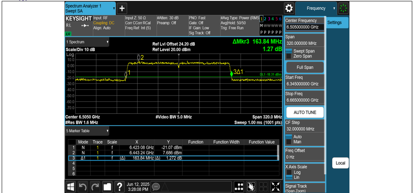
11AX160MIMO-Ant2-6505
