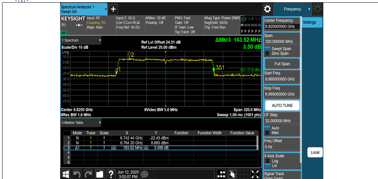
11AX160MIMO-Ant0-6825
