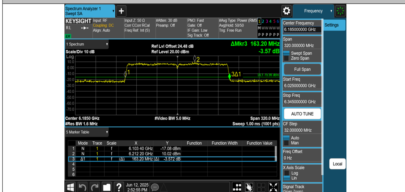
11AX160MIMO-Ant1-6185
