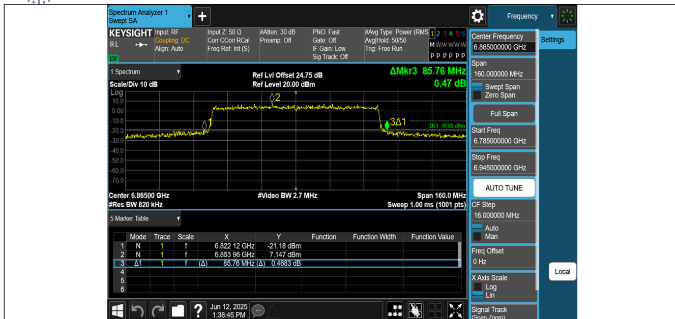
11AX80MIMO-Ant2-6865
