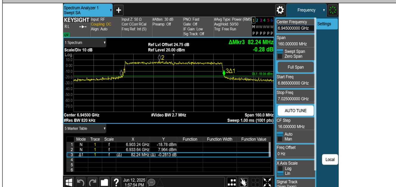
11AX80MIMO-Ant1-6945
