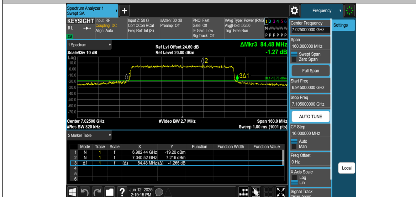
11AX80MIMO-Ant2-7025
