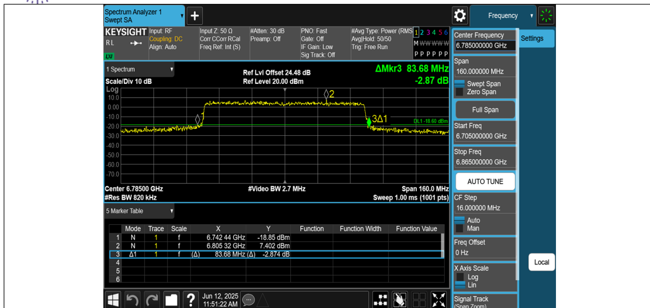
11AX80MIMO-Ant1-6785
