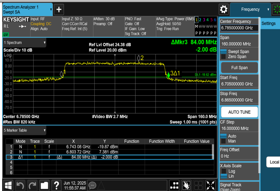
11AX80MIMO-Ant0-6785
