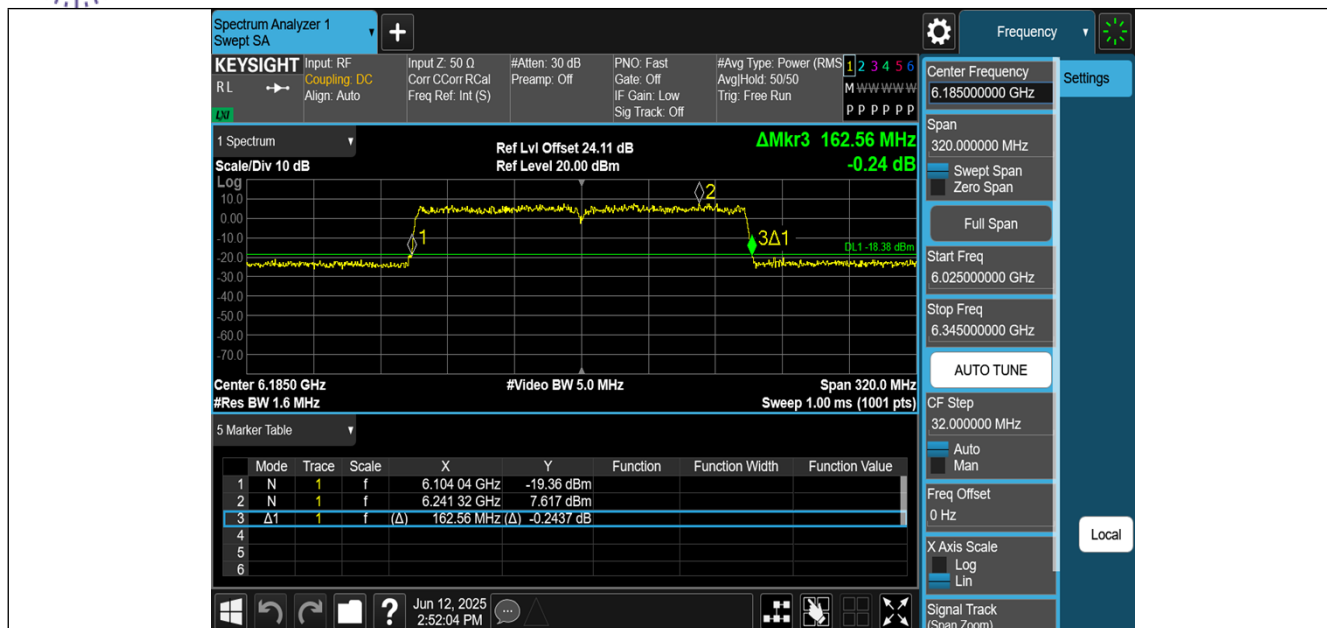
11AX160MIMO-Ant0-6185
