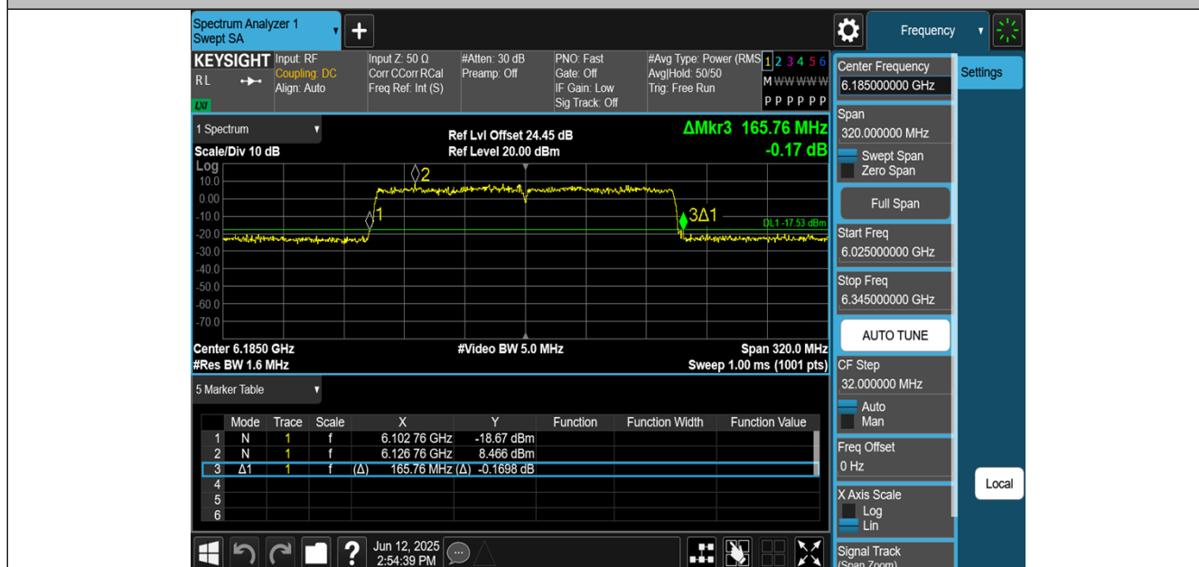
11AX160MIMO-Ant3-6185
