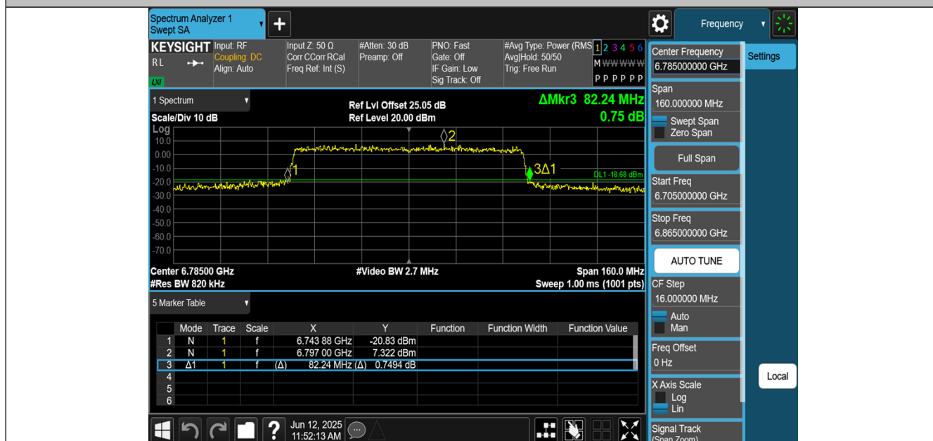
11AX80MIMO-Ant2-6785
