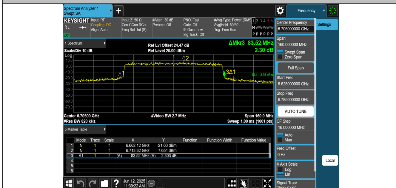
11AX80MIMO-Ant3-6705
