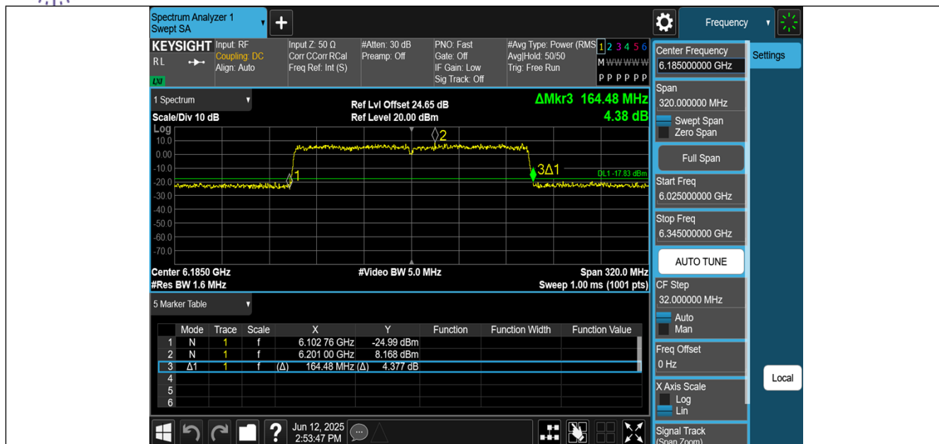
11AX160MIMO-Ant2-6185
