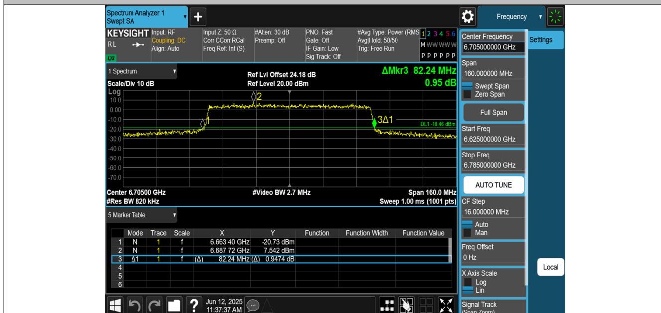
11AX80MIMO-Ant1-6705
