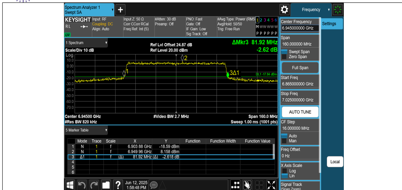
11AX80MIMO-Ant2-6945
