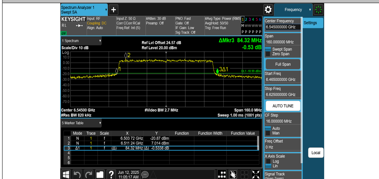
11AX80MIMO-Ant3-6545
