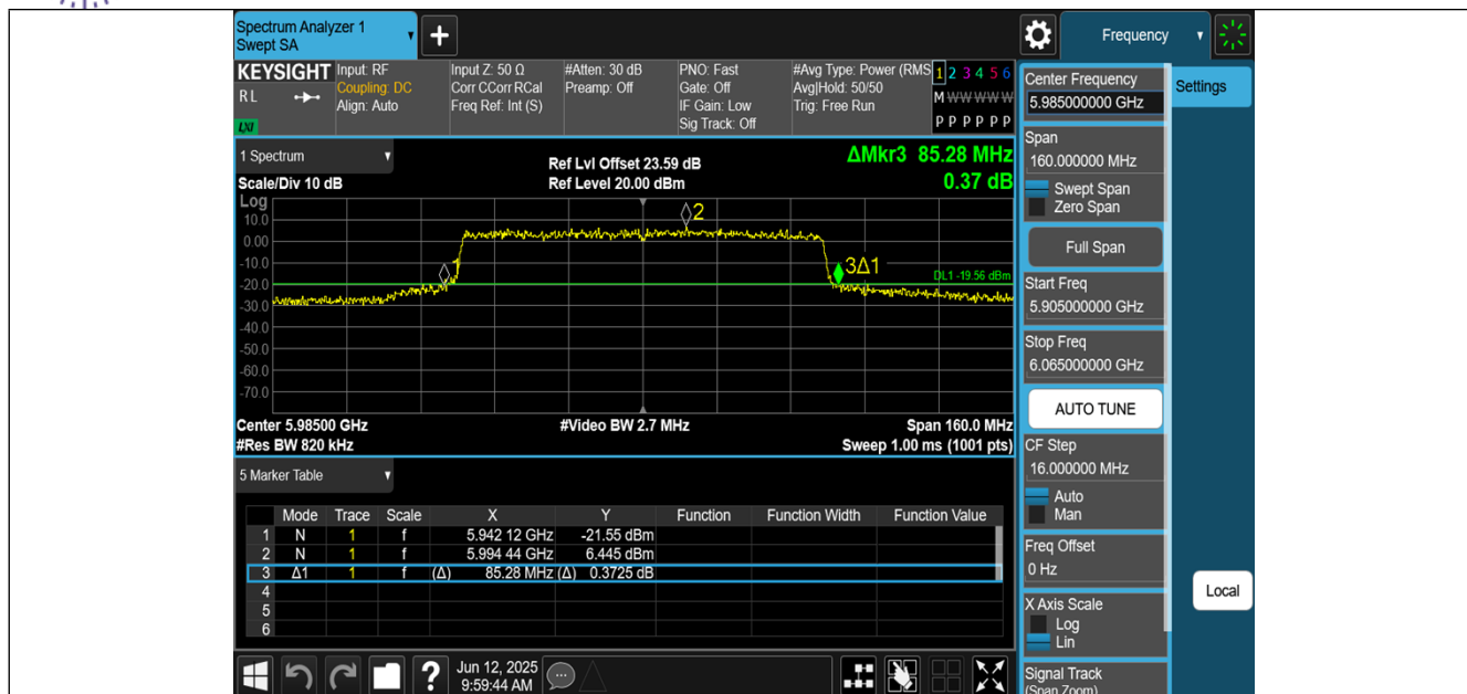
11AX80MIMO-Ant1-5985
