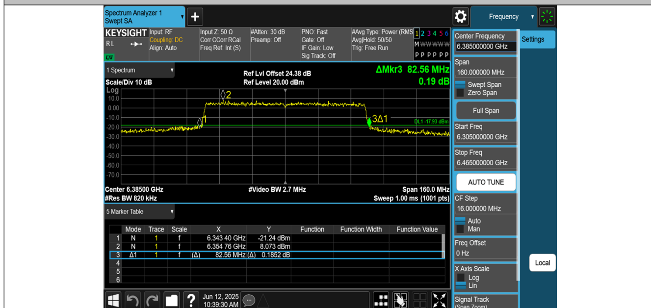
11AX80MIMO-Ant2-6385
