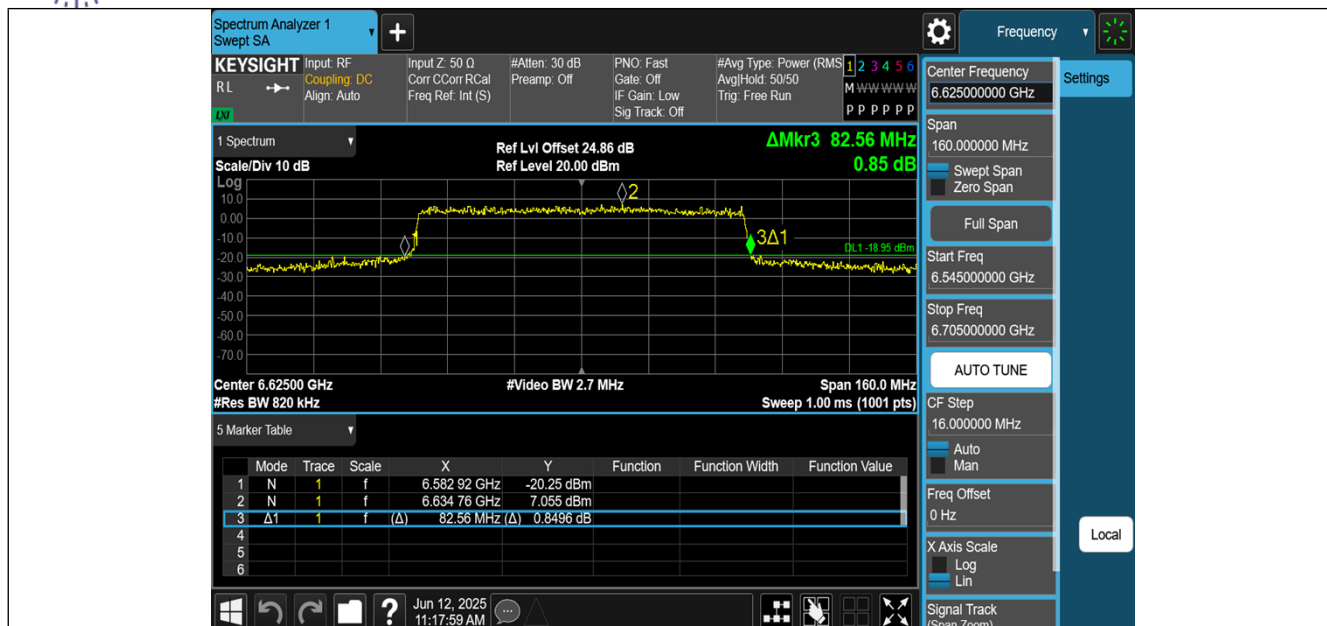
11AX80MIMO-Ant2-6625
