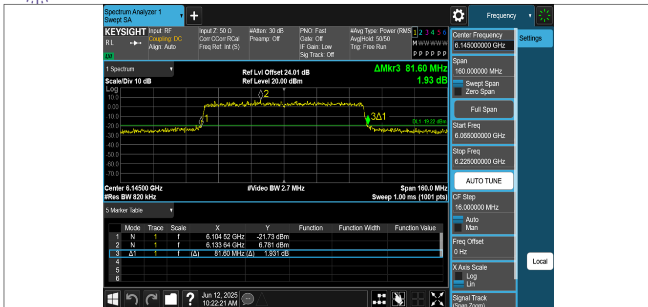
11AX80MIMO-Ant2-6145
