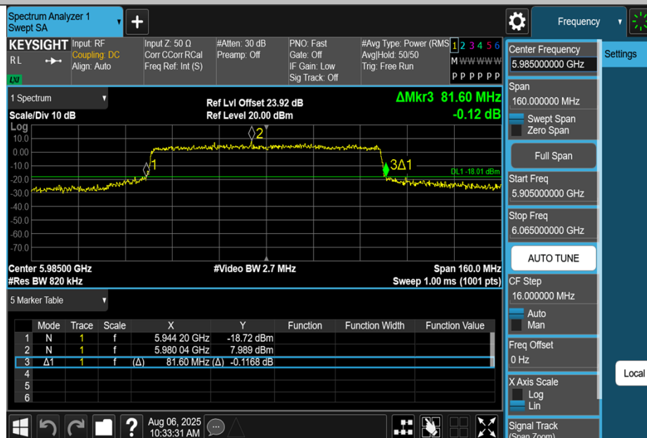
11AX80MIMO-Ant0-5985
