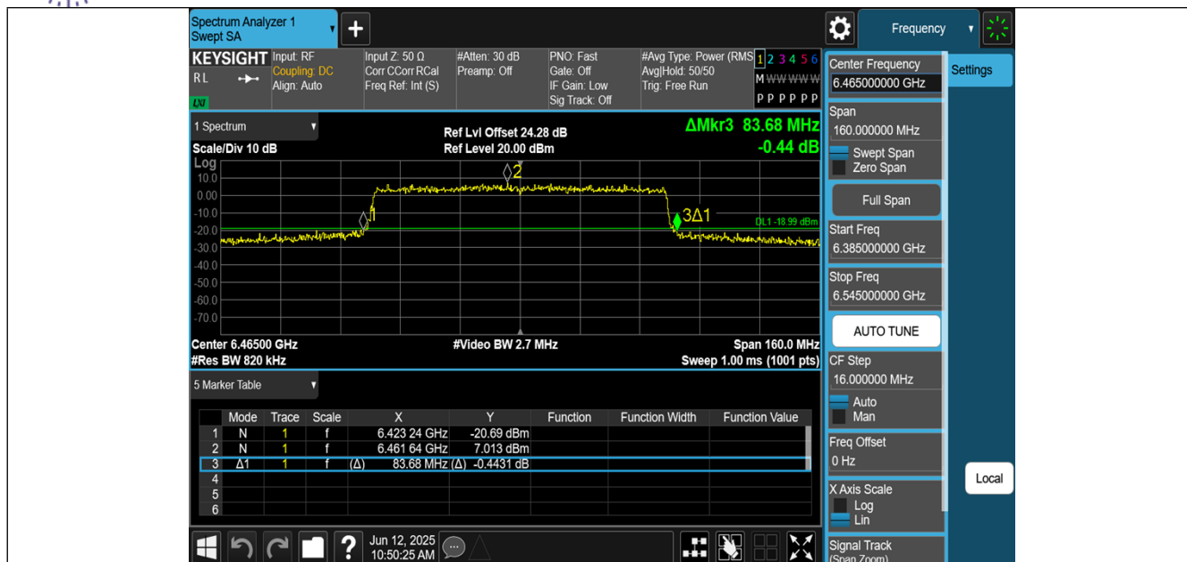
11AX80MIMO-Ant2-6465
