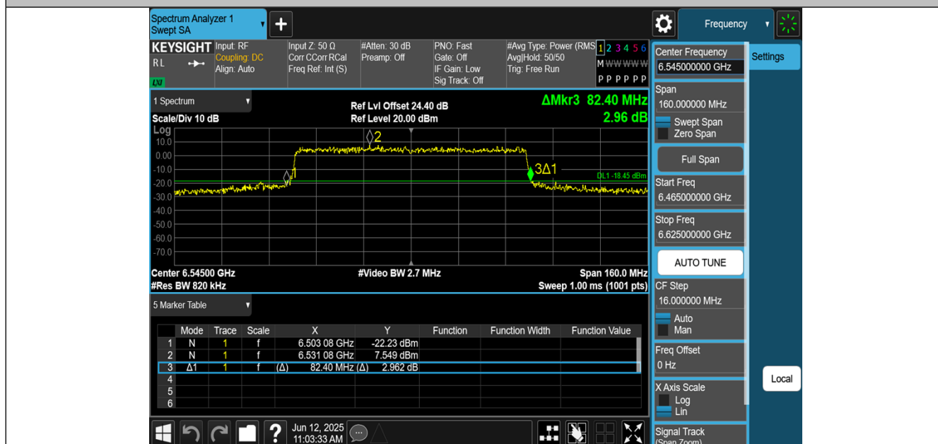
11AX80MIMO-Ant1-6545
