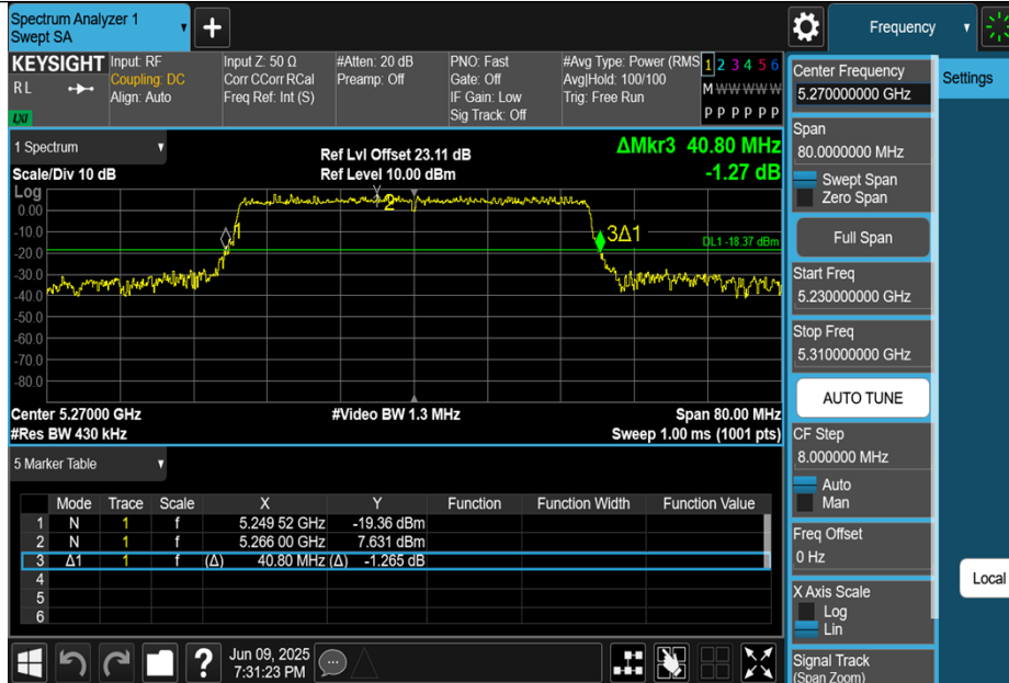
11BE40MIMO-Ant0-5270
