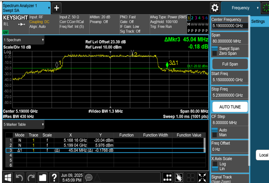
11BE40MIMO-Ant3-5190
