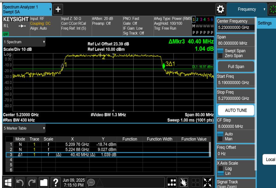
11BE40MIMO-Ant3-5230
