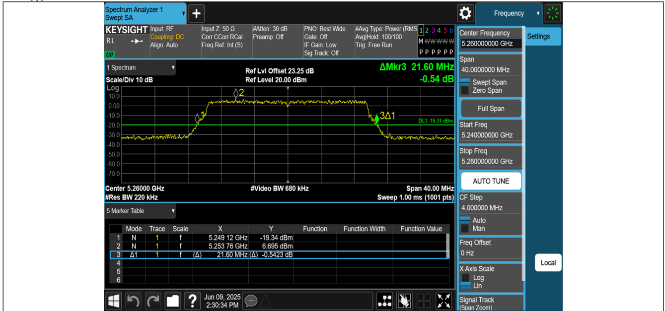
11BE20MIMO-Ant2-5260
