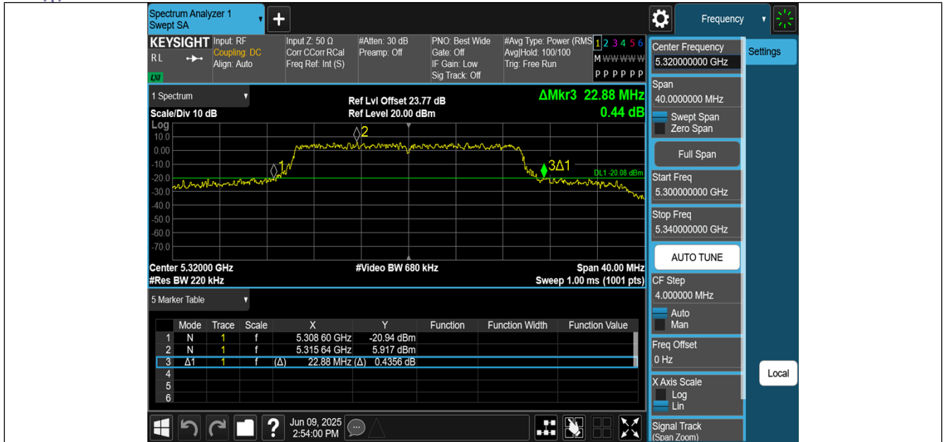
11BE20MIMO-Ant2-5320
