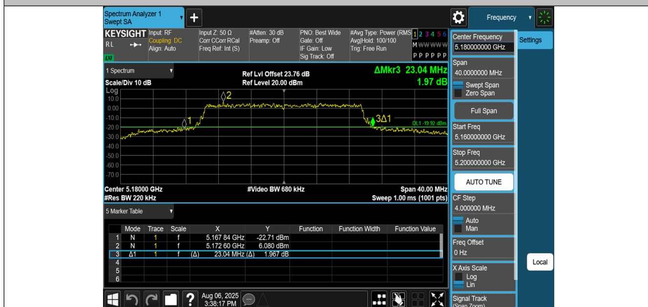
11BE20MIMO-Ant0-5180
