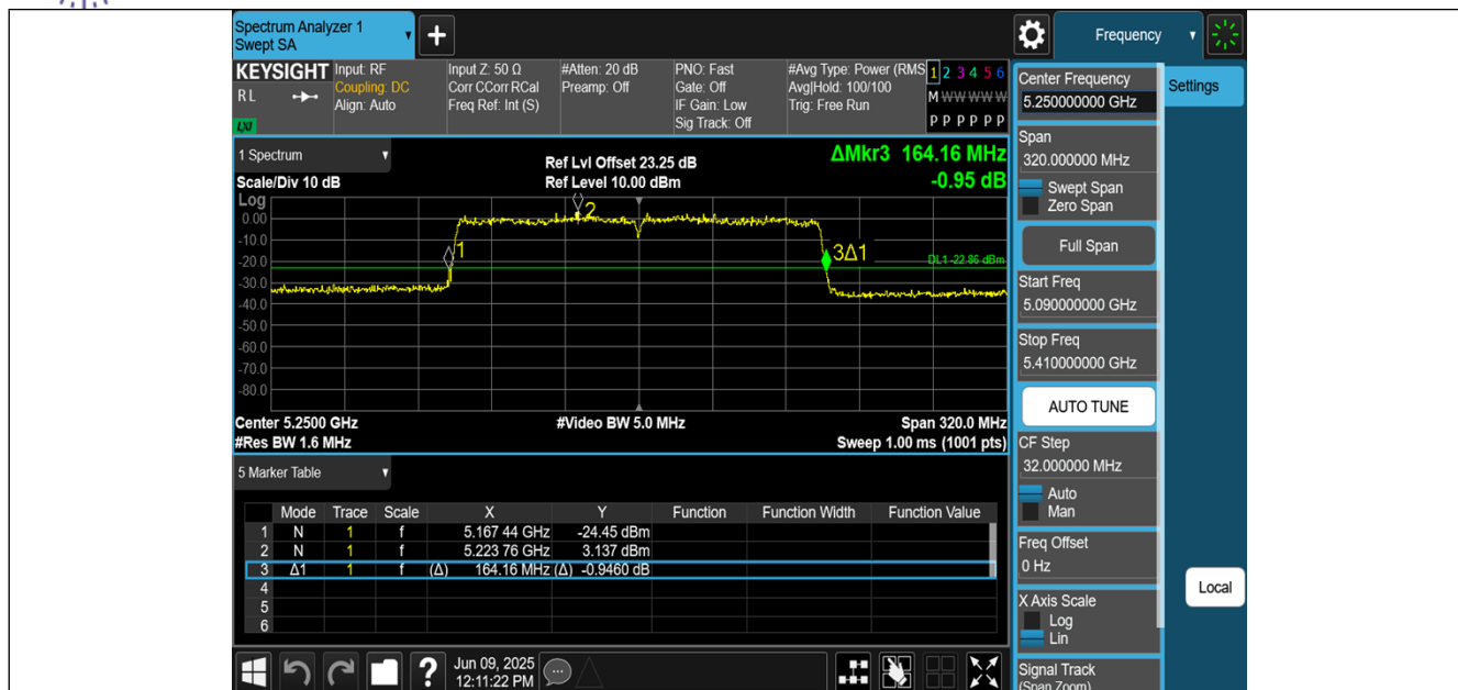
11AX160MIMO-Ant2-5250
