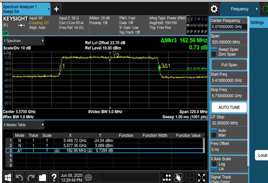
11AX160MIMO-Ant3-5570
