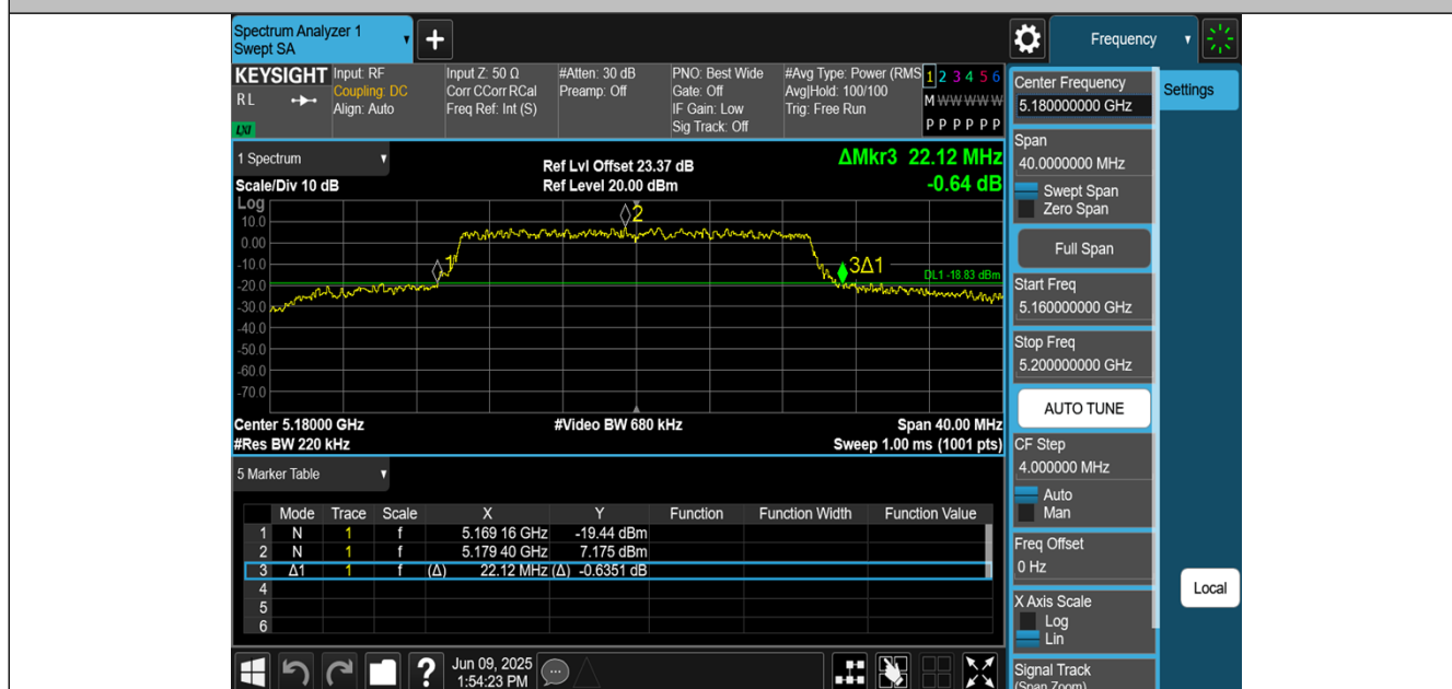
11BE20MIMO-Ant1-5180
