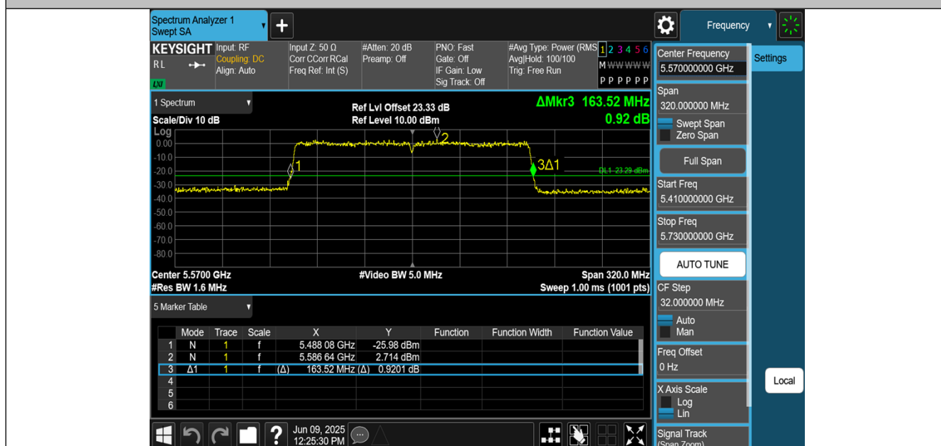
11AX160MIMO-Ant1-5570
