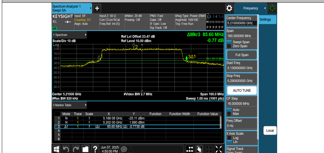
11AC80MIMO-Ant2-5210
