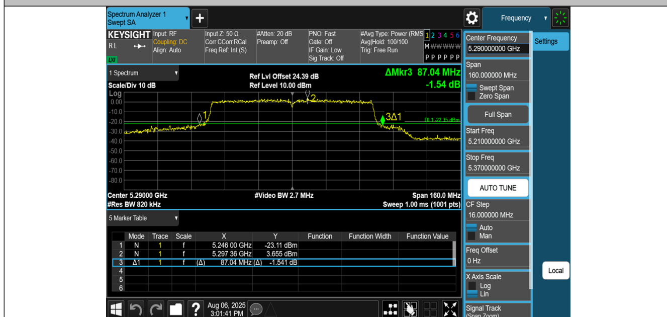
11AC80MIMO-Ant3-5290
