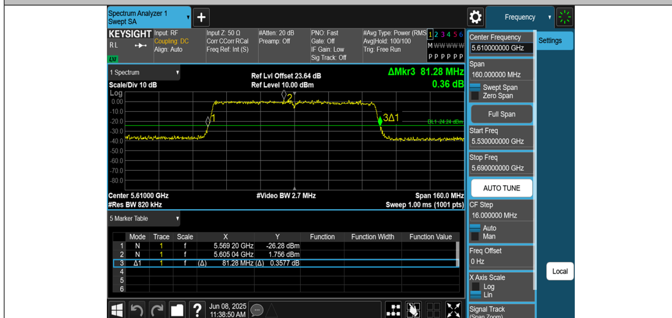
11AC80MIMO-Ant3-5610
