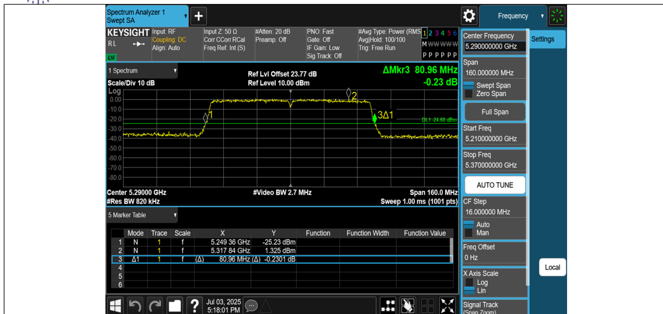
11AC80MIMO-Ant2-5290
