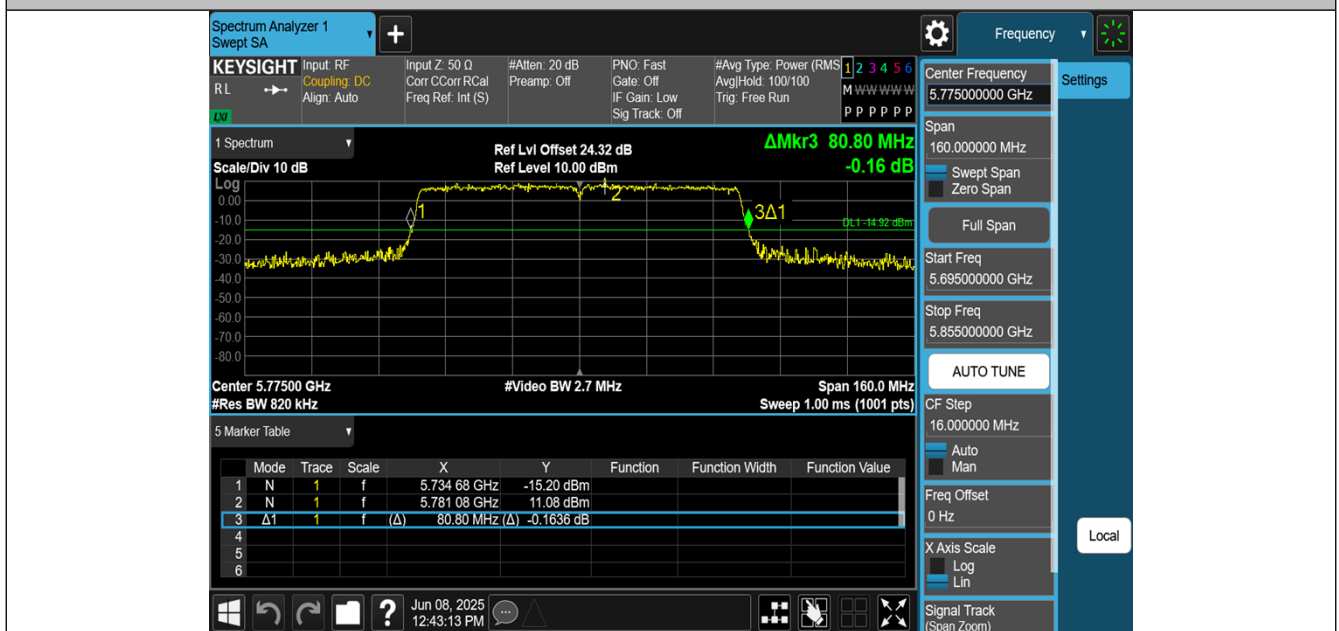
11AC80MIMO-Ant3-5775
