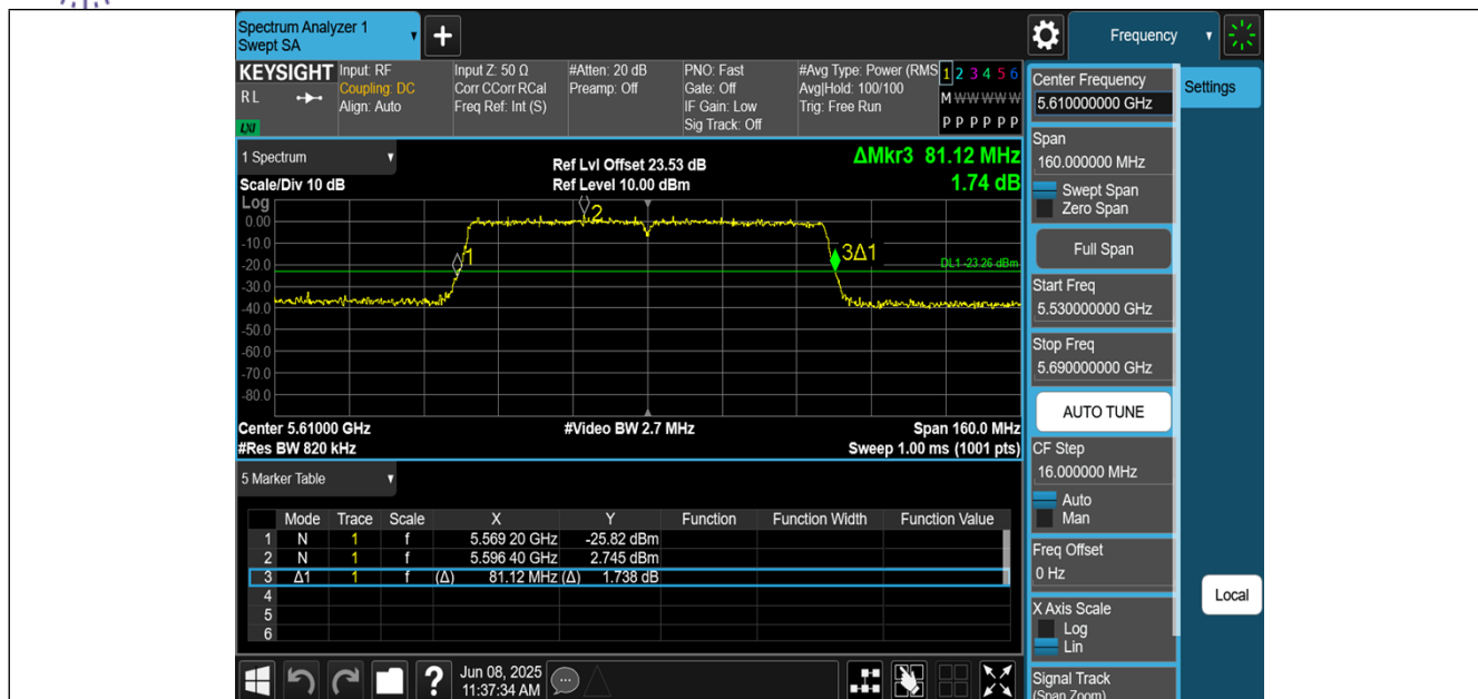
11AC80MIMO-Ant2-5610
