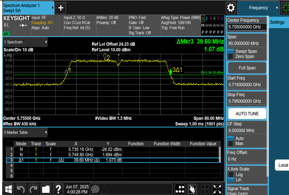
11AC40MIMO-Ant2-5755
