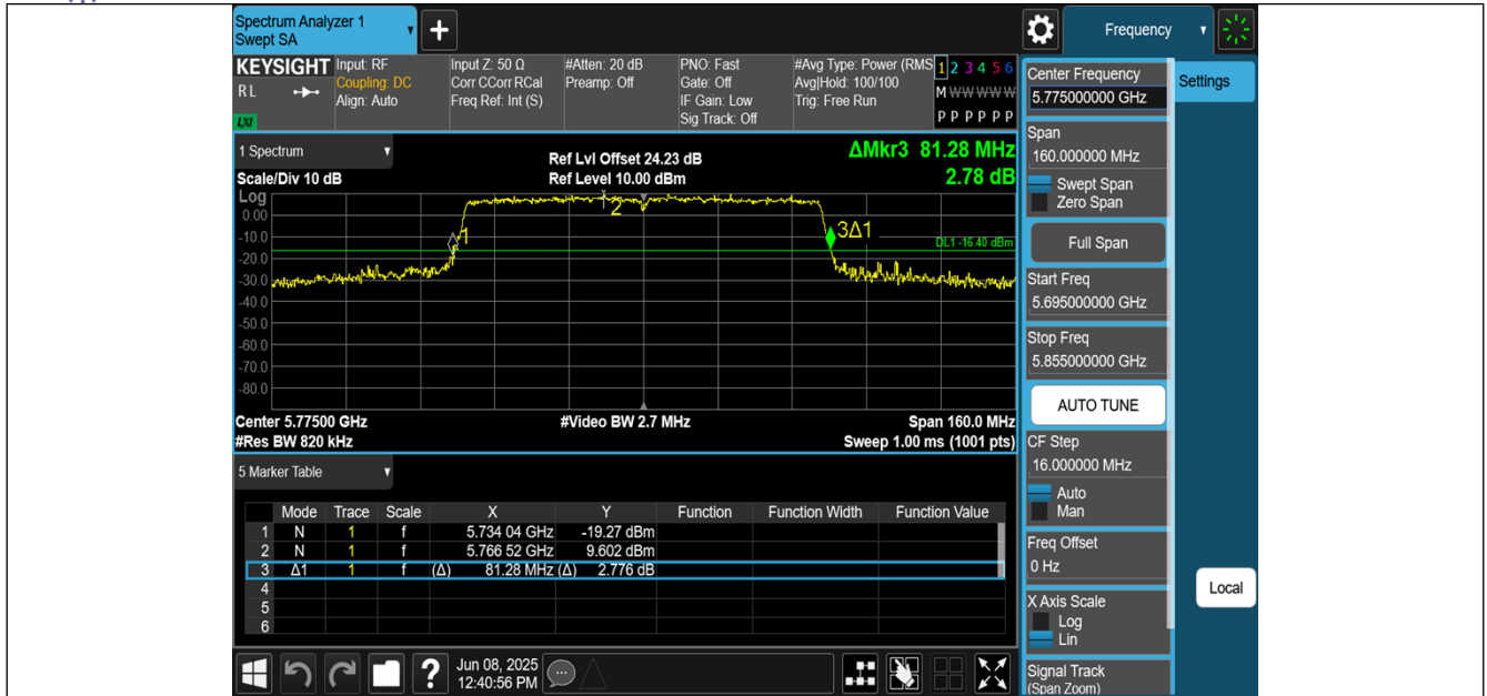
11AC80MIMO-Ant2-5775
