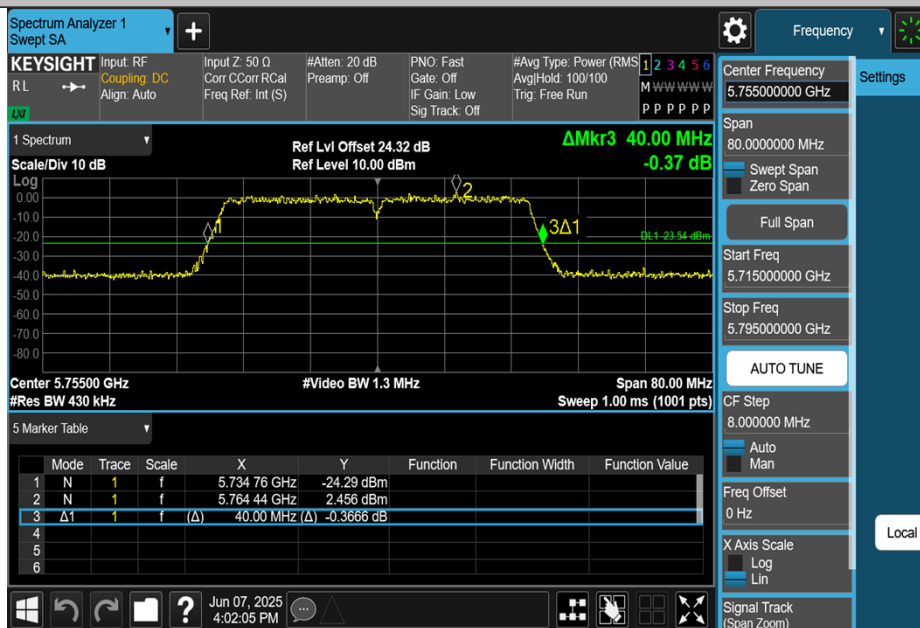
11AC40MIMO-Ant3-5755
