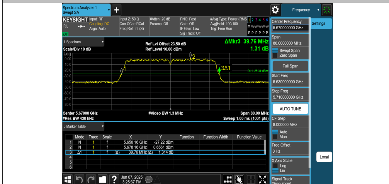
11AC40MIMO-Ant1-5670
