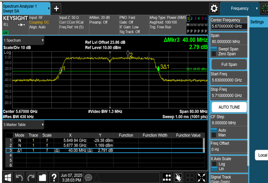
11AC40MIMO-Ant3-5670
