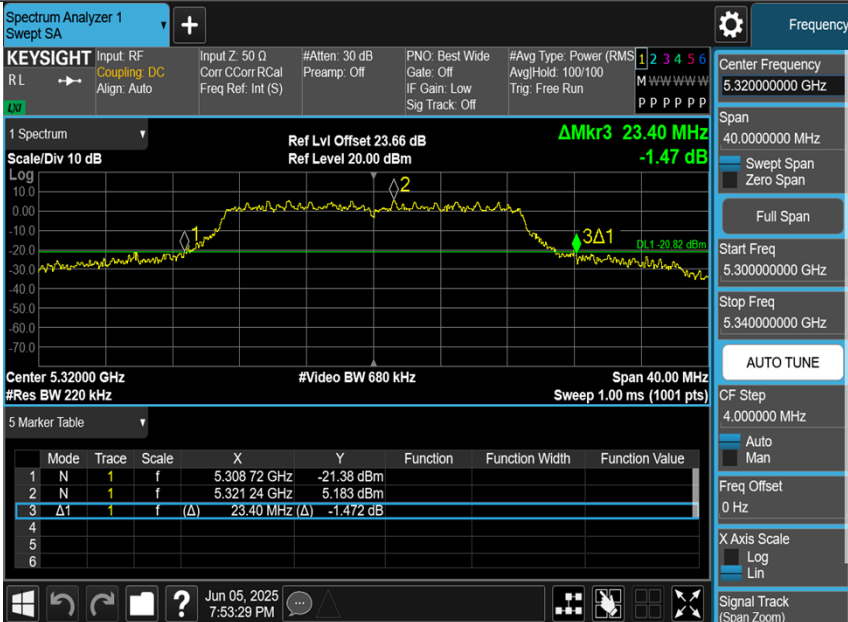
11AC20MIMO-Ant1-5320
