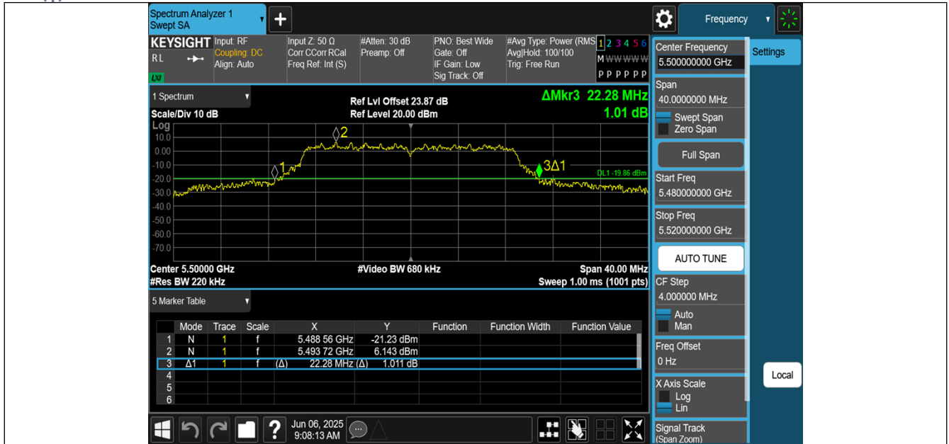
11AC20MIMO-Ant0-5500
