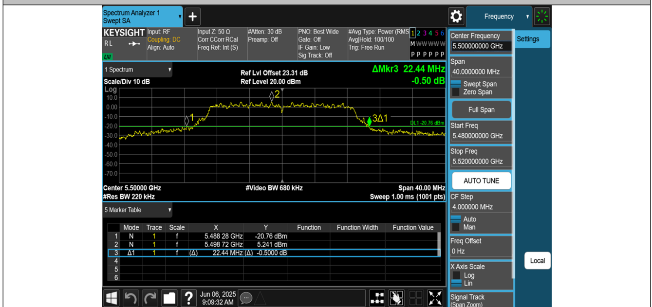
11AC20MIMO-Ant1-5500
