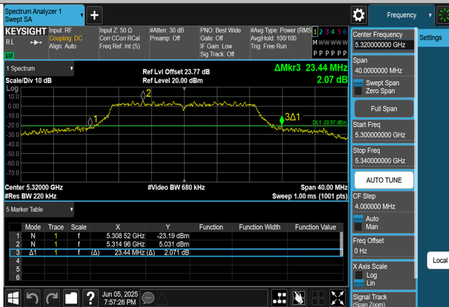
11AC20MIMO-Ant2-5320
