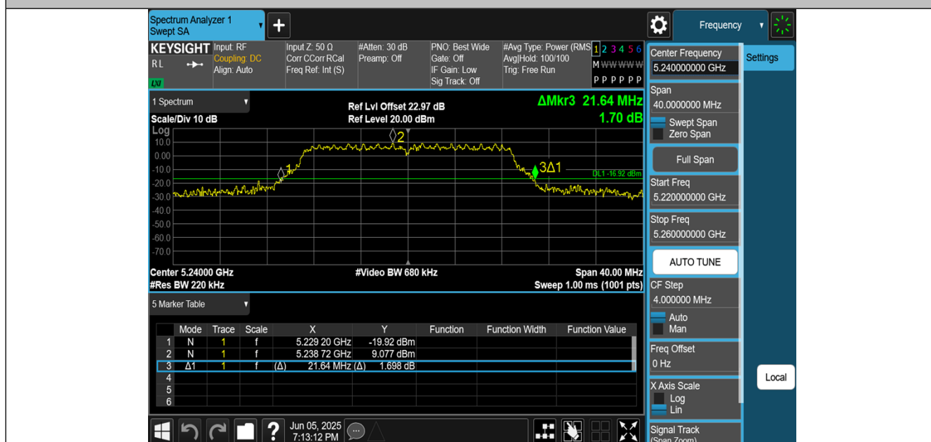
11AC20MIMO-Ant1-5240
