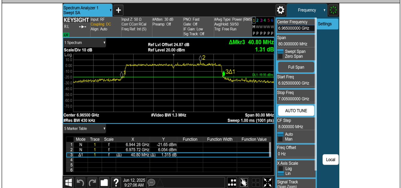
11AX40MIMO-Ant2-6965
