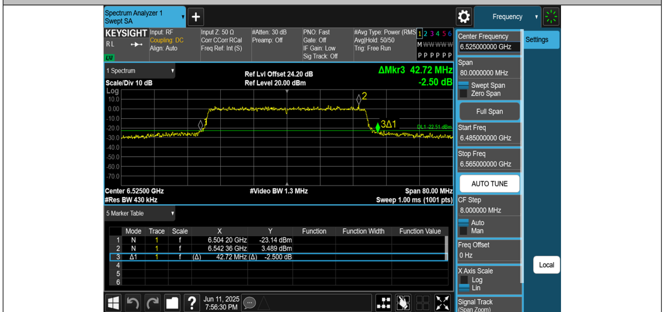
11AX40MIMO-Ant2-6525
