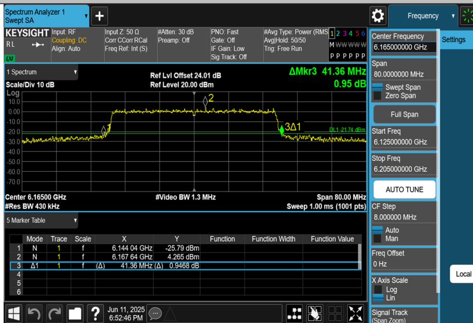
11AX40MIMO-Ant2-6165
