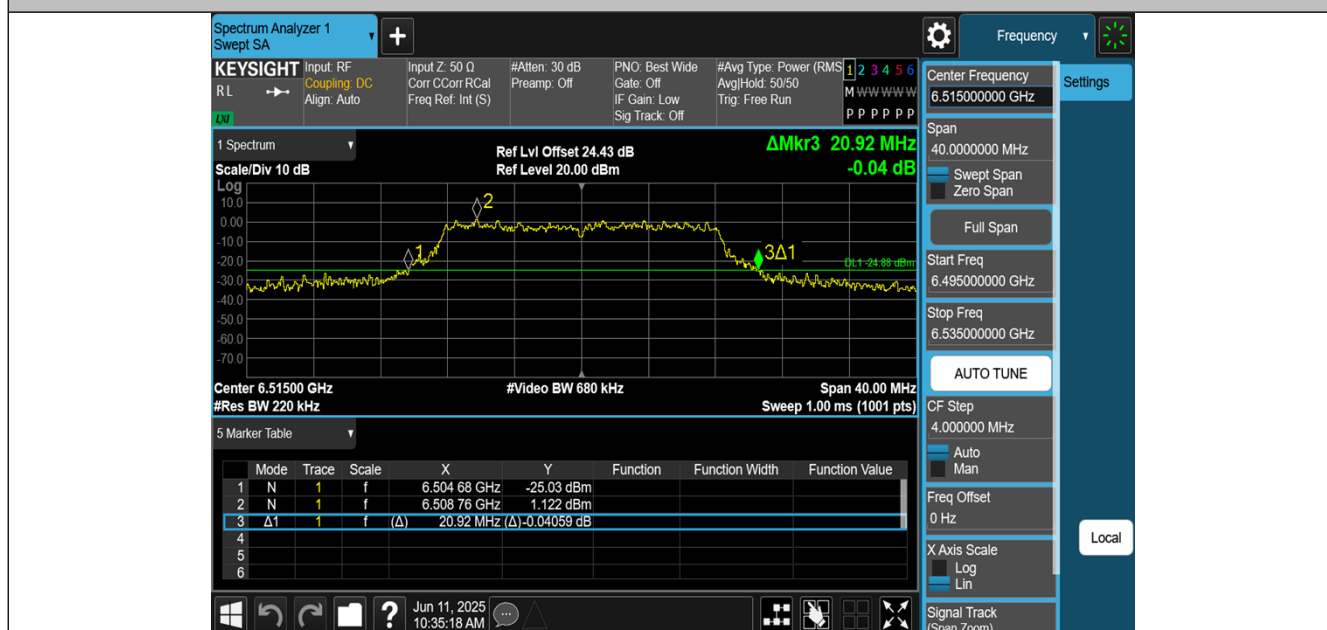
11A-CDD-Ant3-6515
