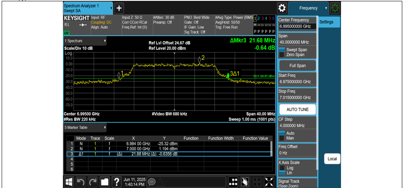
11A-CDD-Ant3-6995
