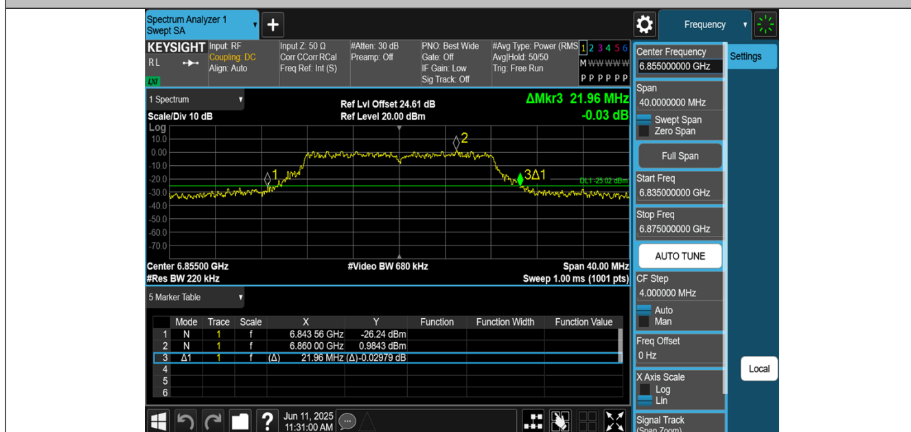
11A-CDD-Ant3-6855
