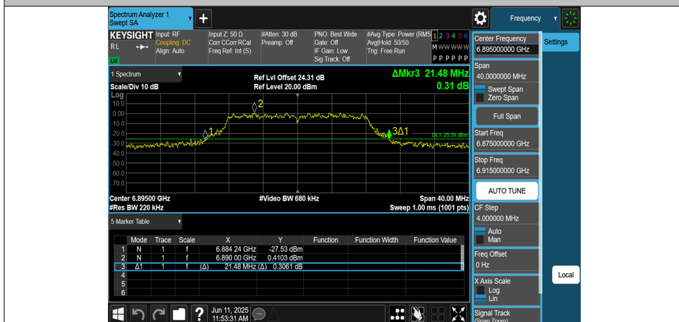
11A-CDD-Ant1-6895
