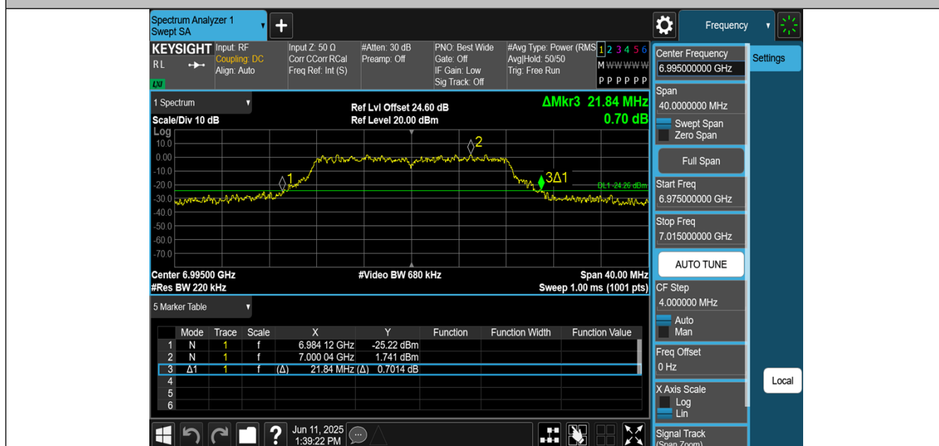
11A-CDD-Ant2-6995
