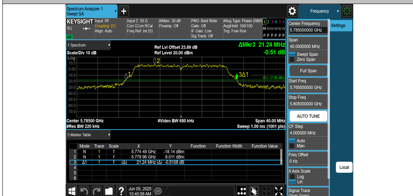
11N20MIMO-Ant3-5785
